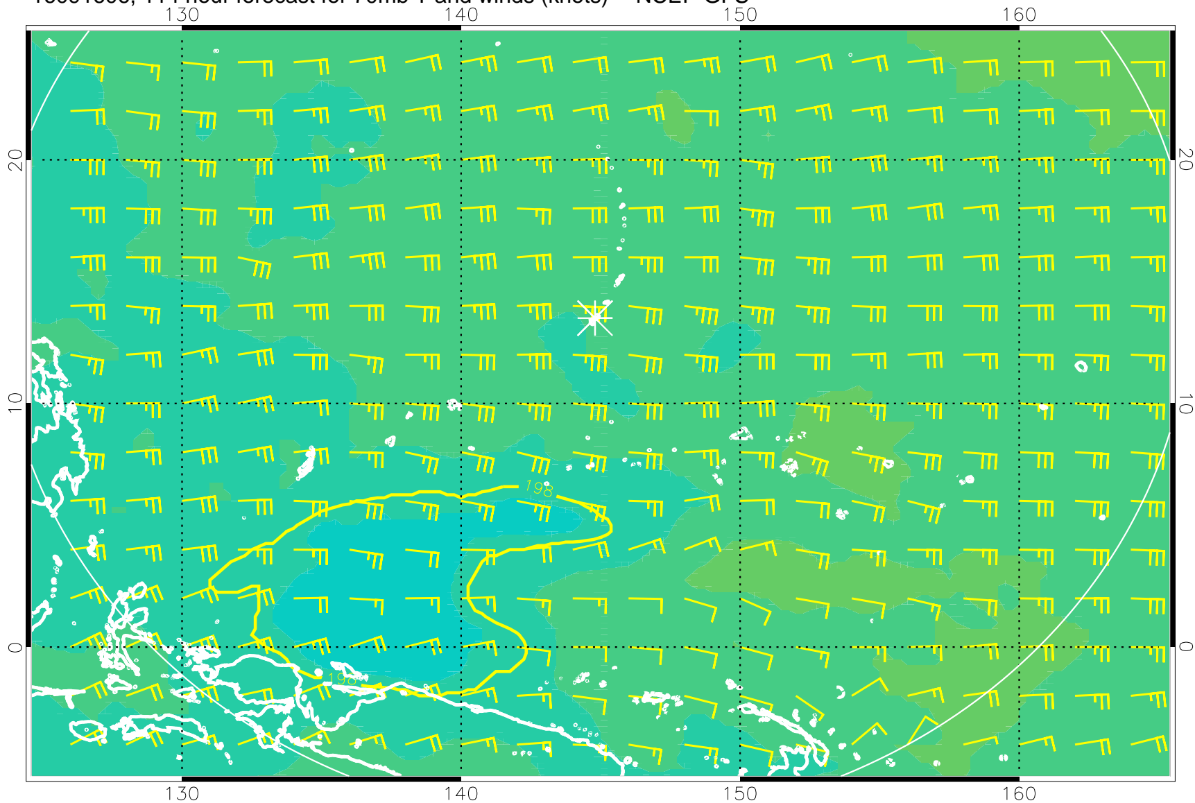
16091606, 114 hour forecast for 70mb T and winds (knots) -- NCEP GFS
