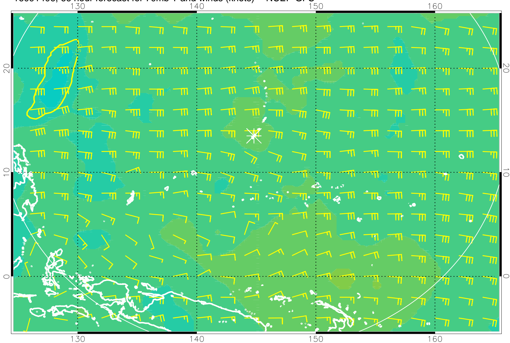
16091406, 66 hour forecast for 70mb T and winds (knots) -- NCEP GFS
