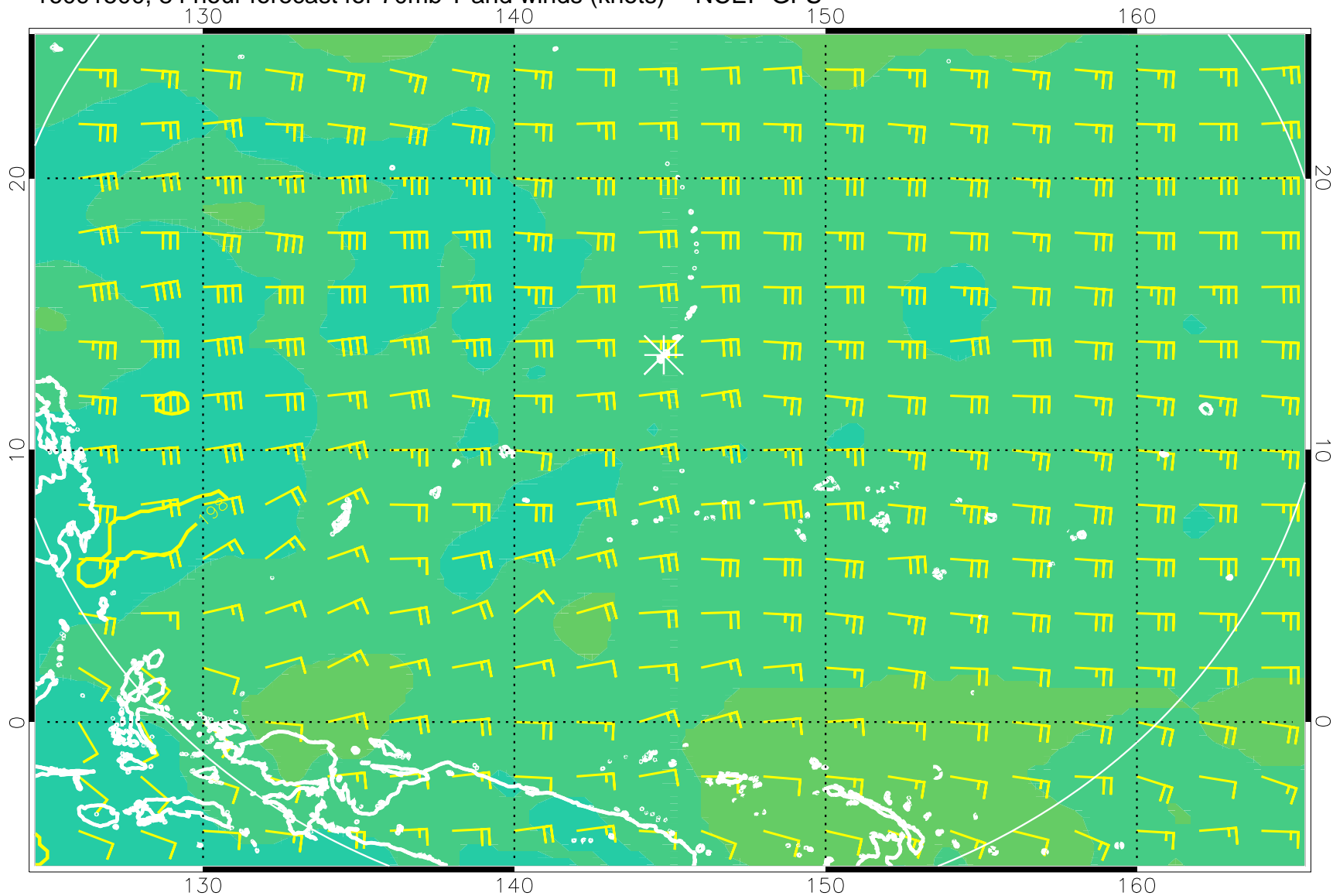
16091500, 84 hour forecast for 70mb T and winds (knots) -- NCEP GFS
