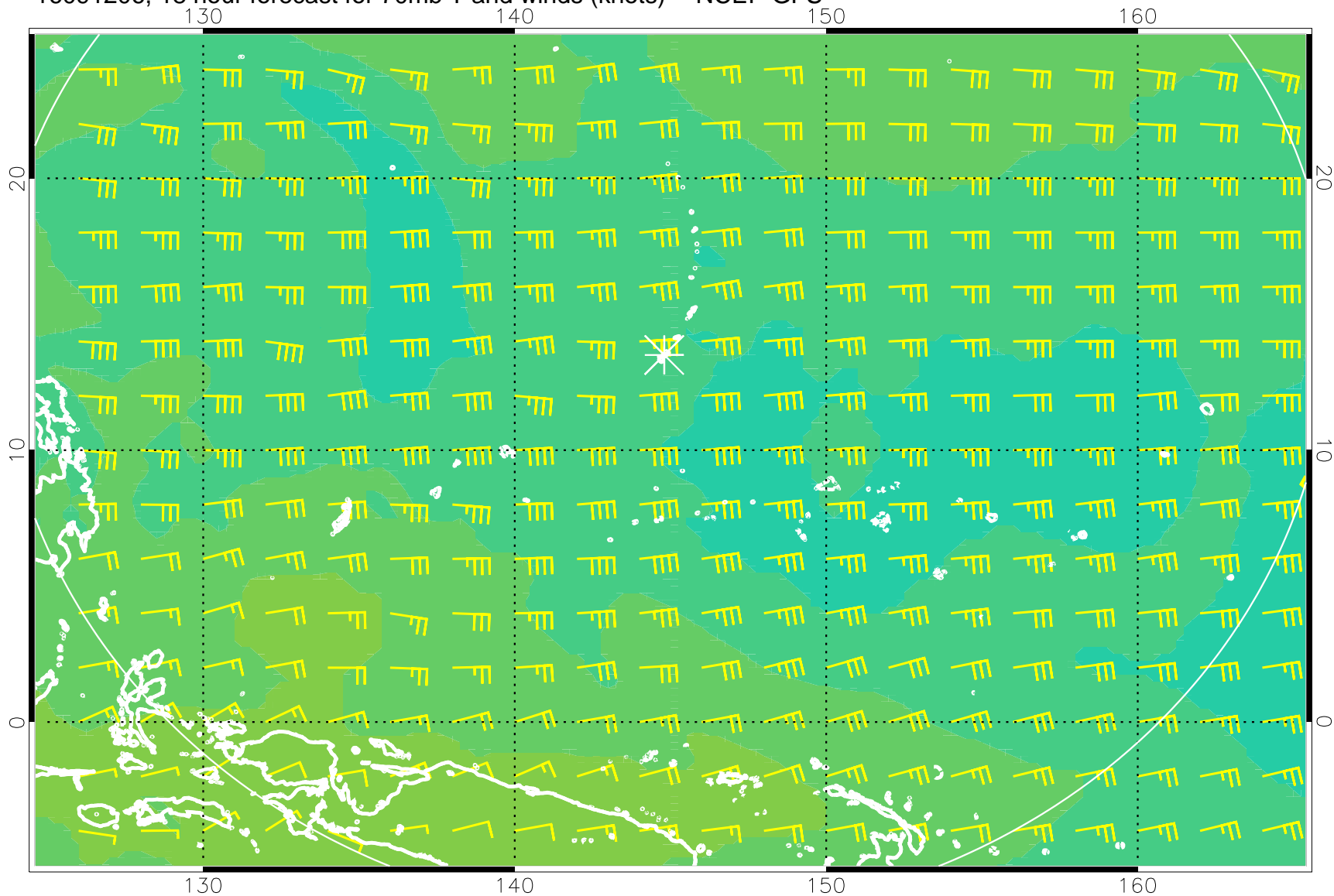
16091206, 18 hour forecast for 70mb T and winds (knots) -- NCEP GFS
