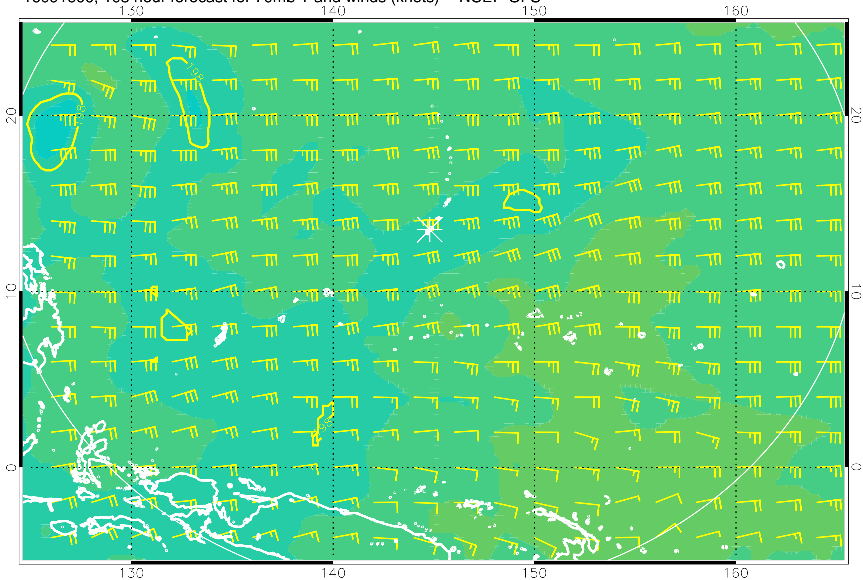
16091600, 108 hour forecast for 70mb T and winds (knots) -- NCEP GFS
