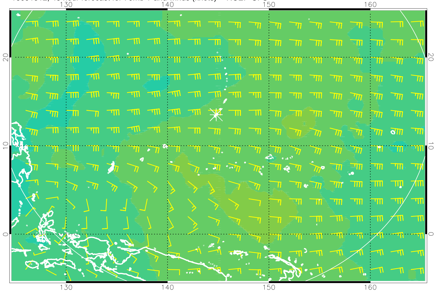
16091312, 48 hour forecast for 70mb T and winds (knots) -- NCEP GFS
