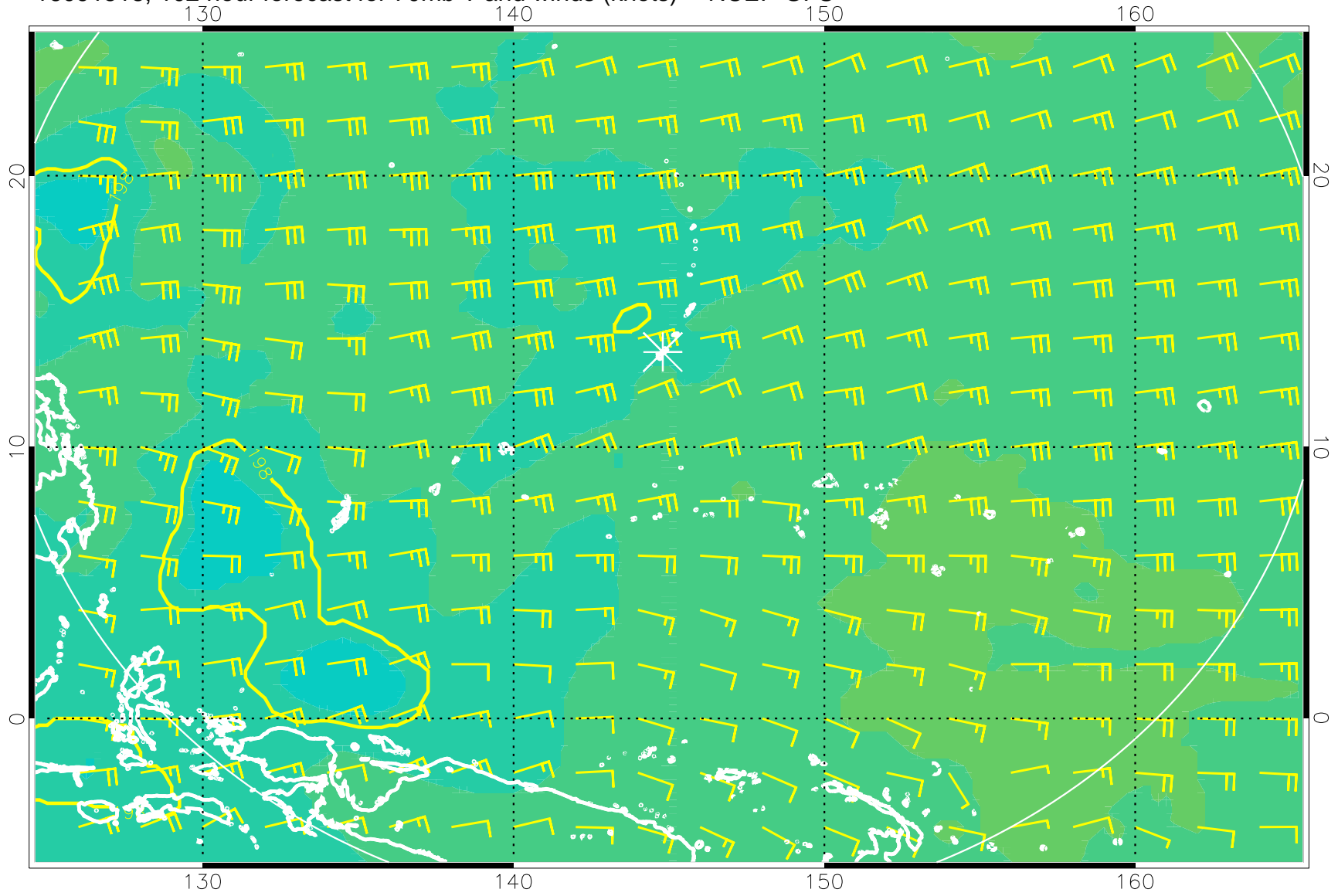
16091518, 102 hour forecast for 70mb T and winds (knots) -- NCEP GFS
