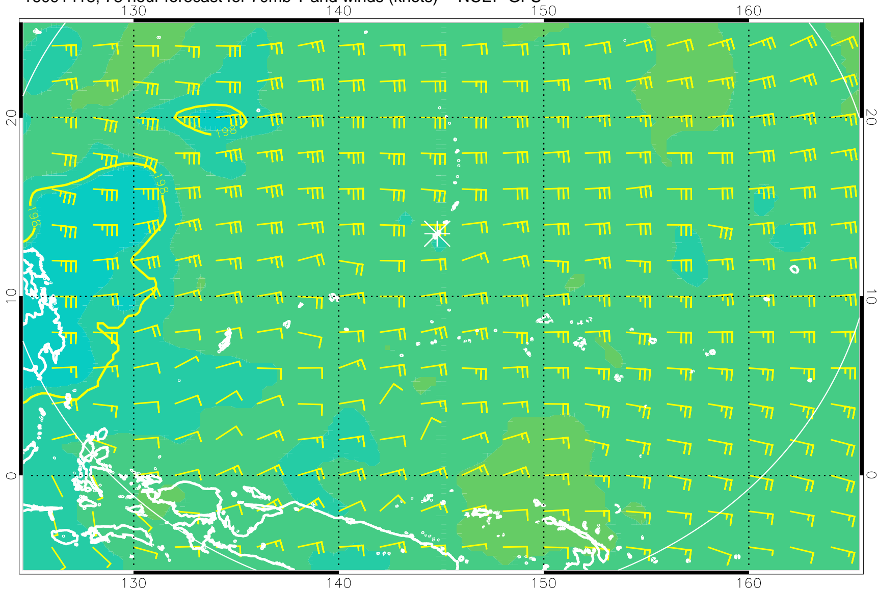
16091418, 78 hour forecast for 70mb T and winds (knots) -- NCEP GFS
