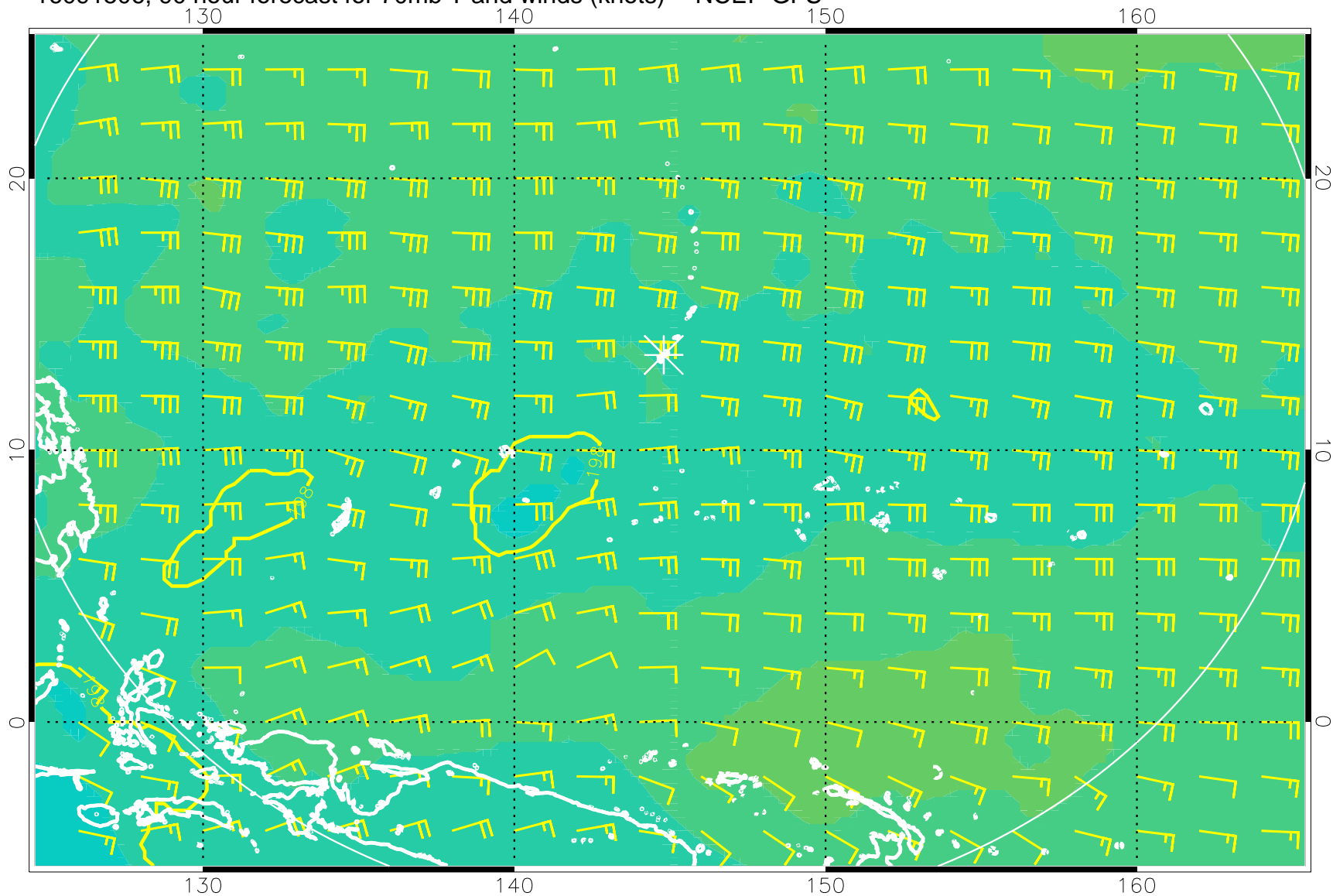
16091506, 90 hour forecast for 70mb T and winds (knots) -- NCEP GFS
