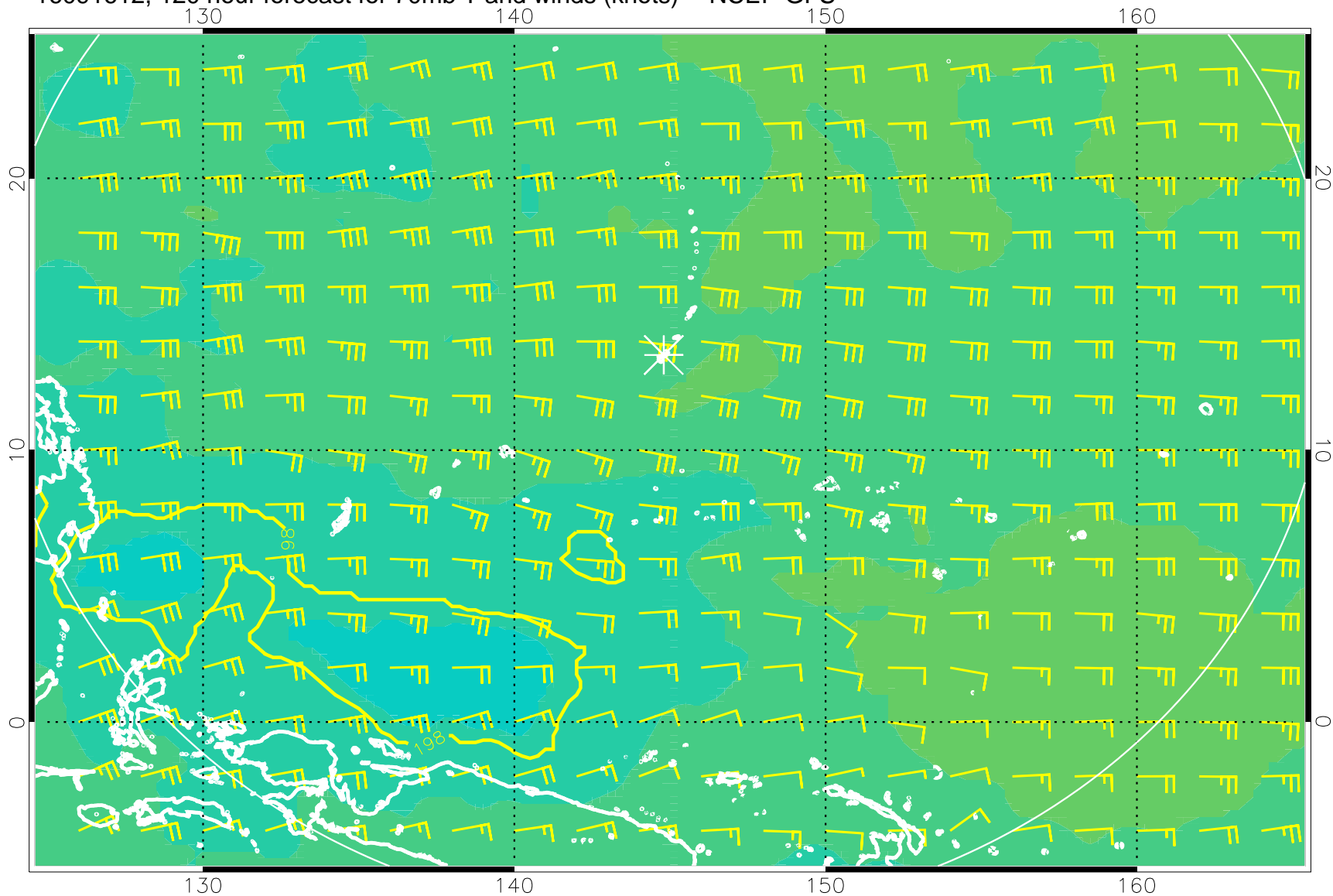
16091612, 120 hour forecast for 70mb T and winds (knots) -- NCEP GFS
