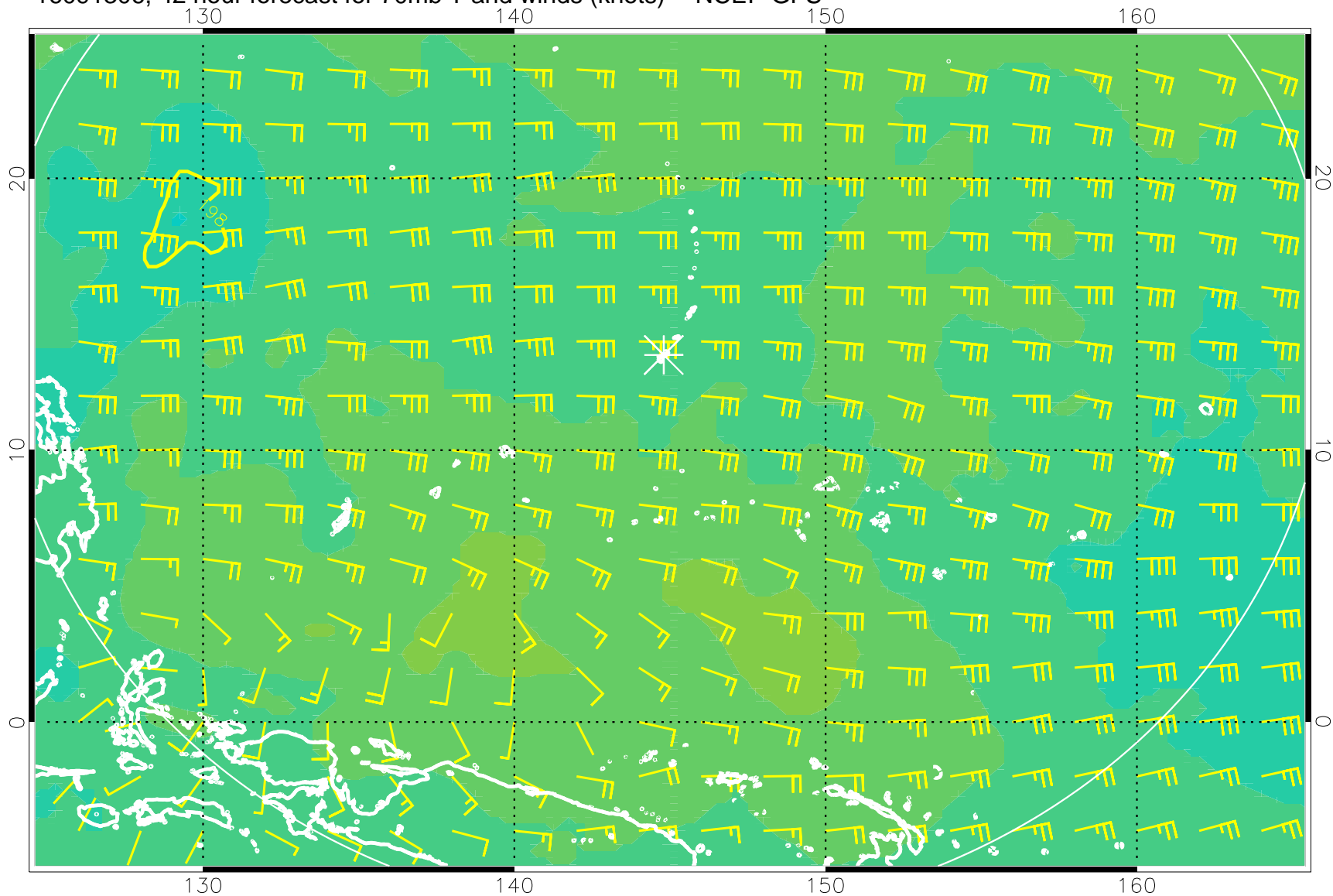
16091306, 42 hour forecast for 70mb T and winds (knots) -- NCEP GFS
