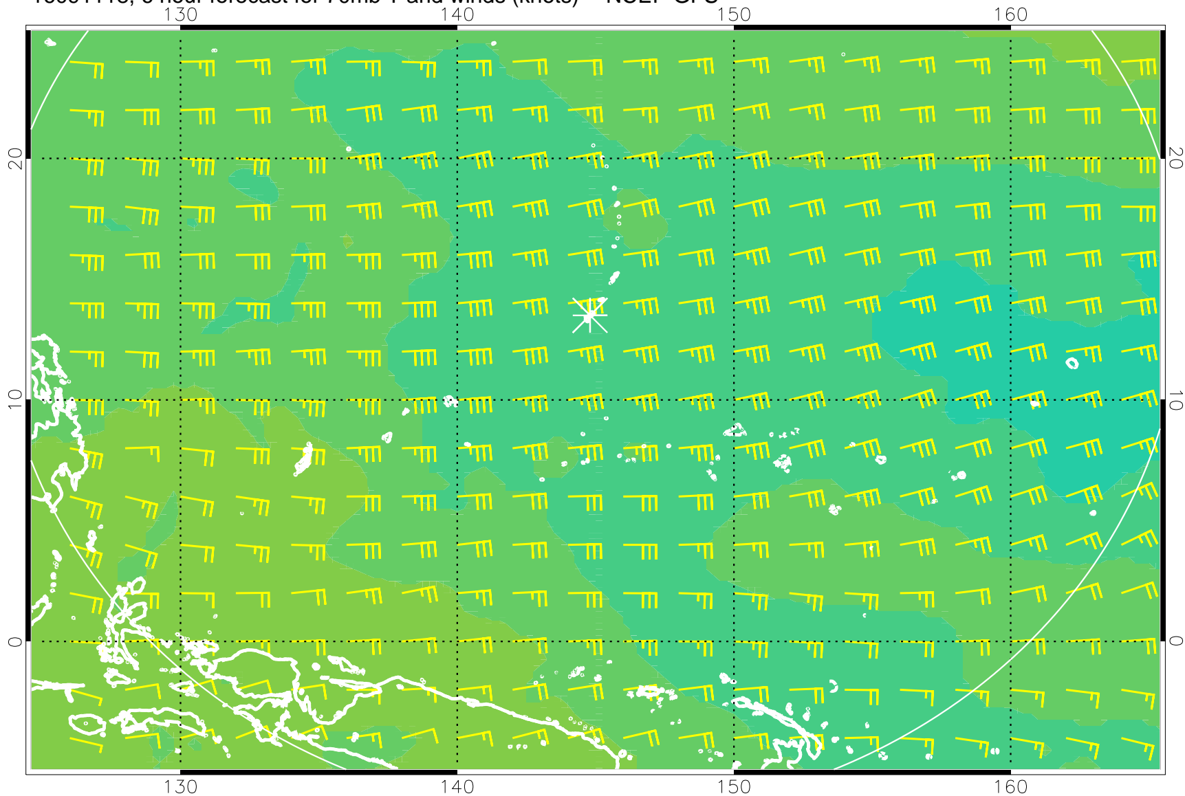
16091118, 6 hour forecast for 70mb T and winds (knots) -- NCEP GFS
