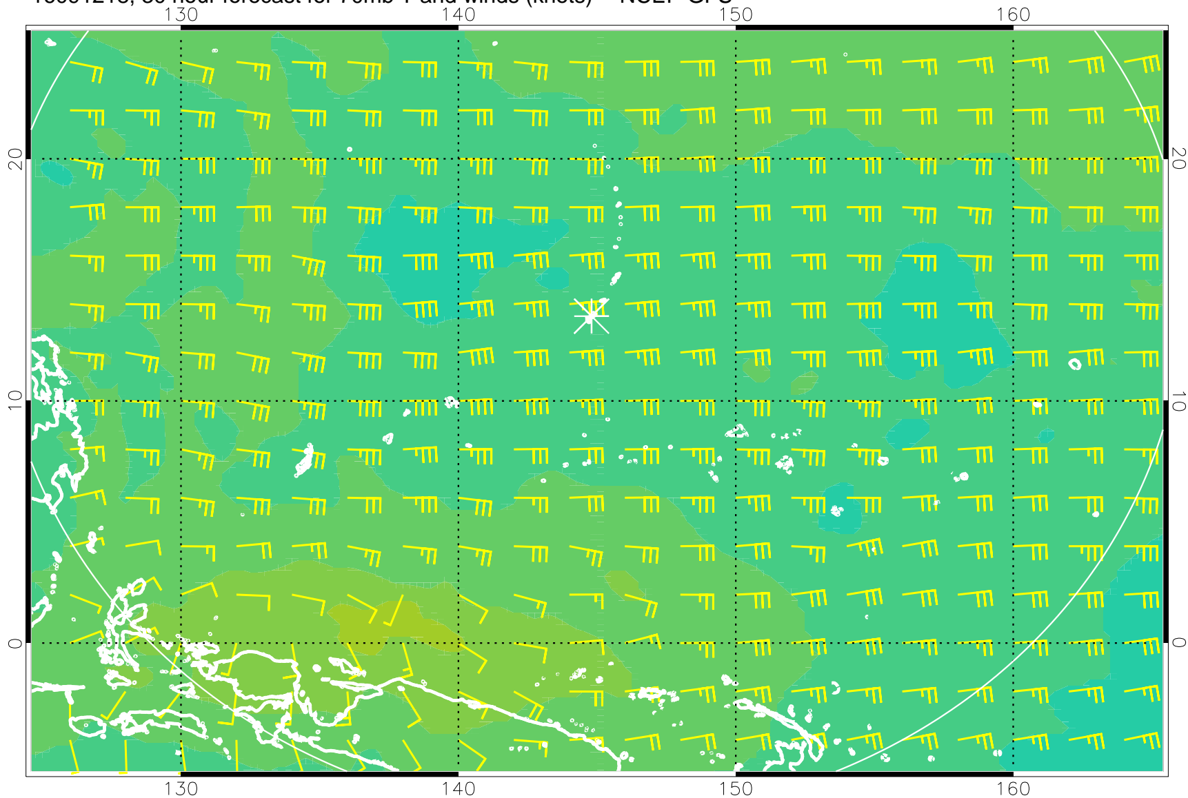
16091218, 30 hour forecast for 70mb T and winds (knots) -- NCEP GFS
