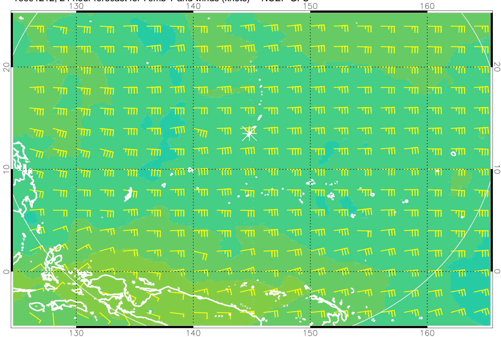
16091212, 24 hour forecast for 70mb T and winds (knots) -- NCEP GFS
