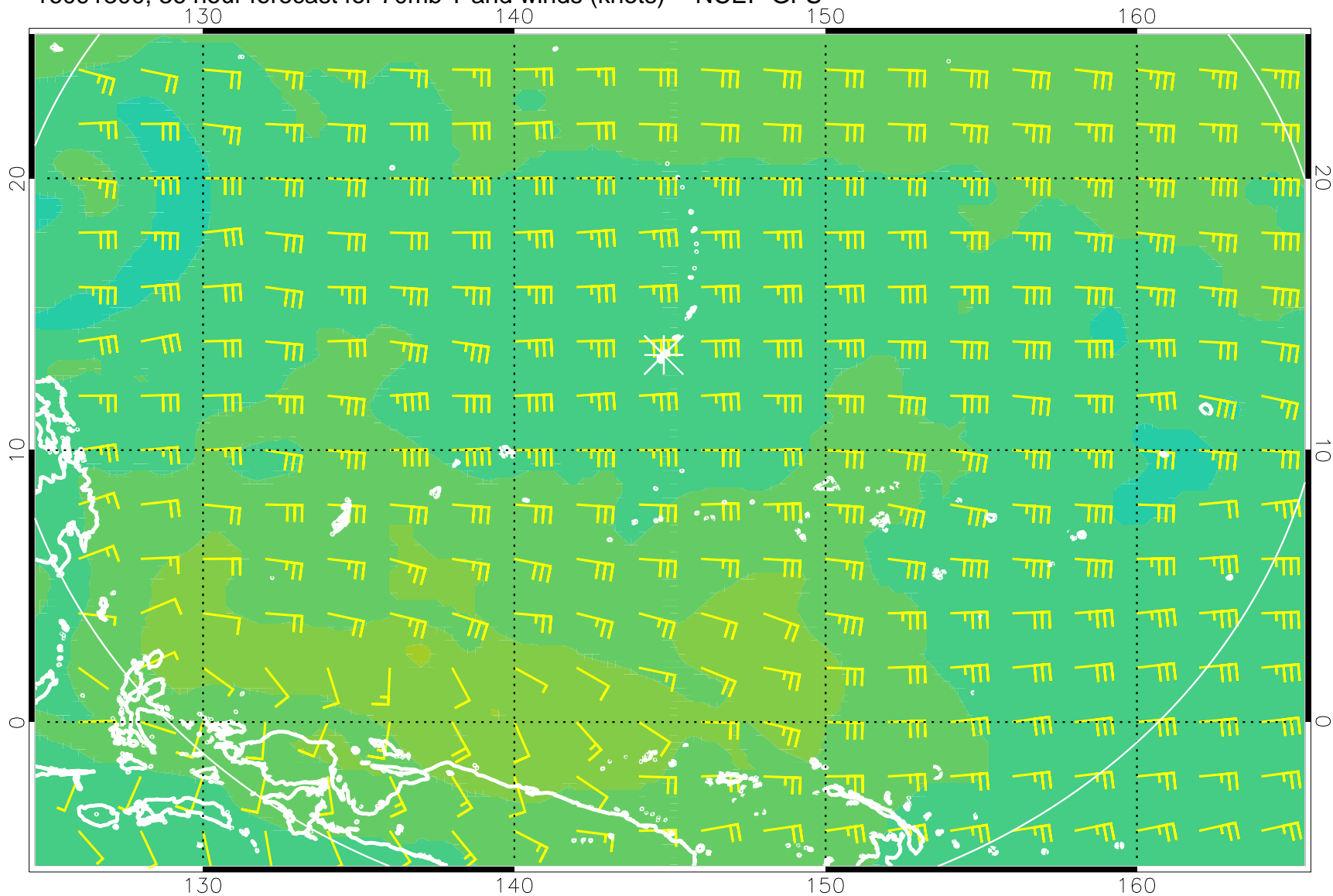
16091300, 36 hour forecast for 70mb T and winds (knots) -- NCEP GFS
