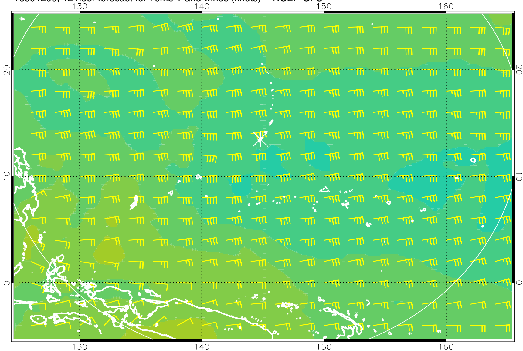
16091200, 12 hour forecast for 70mb T and winds (knots) -- NCEP GFS
