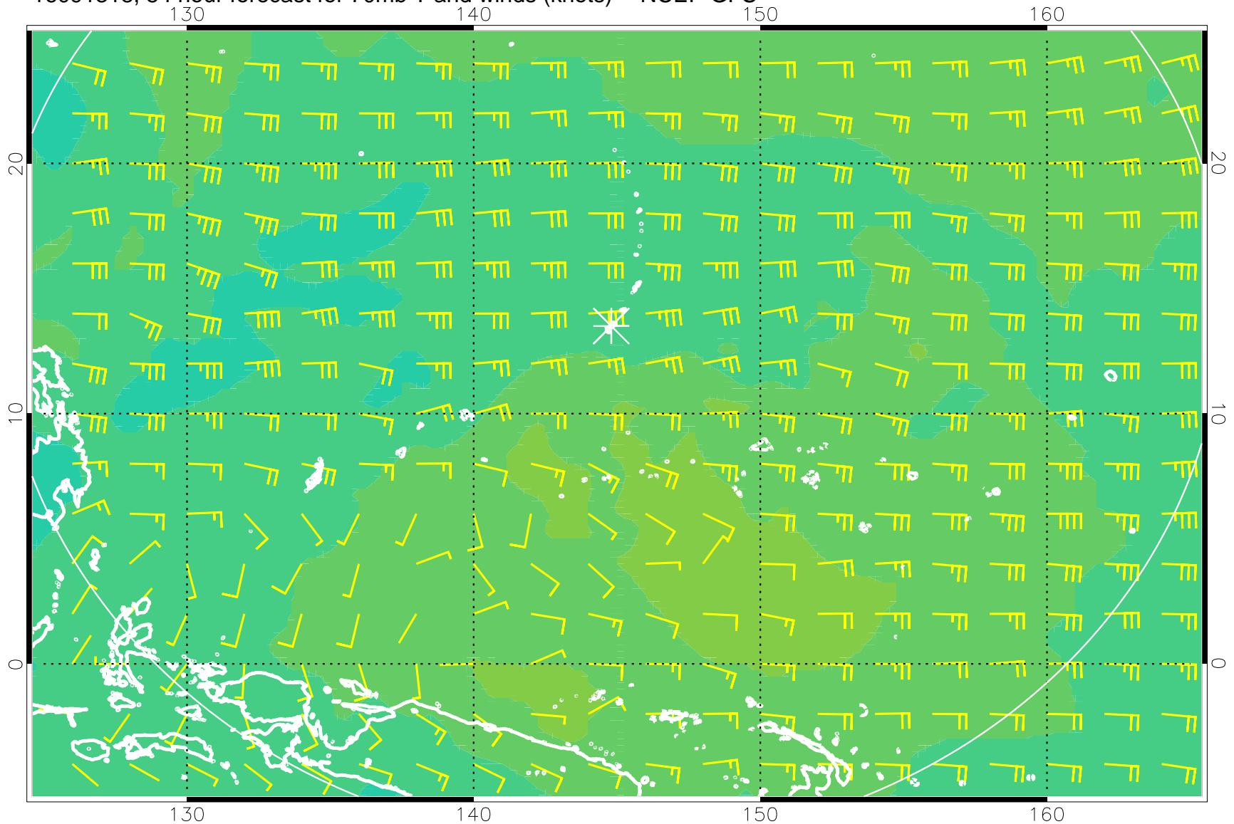
16091318, 54 hour forecast for 70mb T and winds (knots) -- NCEP GFS
