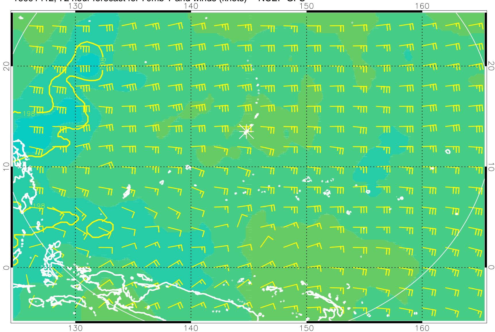
16091412, 72 hour forecast for 70mb T and winds (knots) -- NCEP GFS
