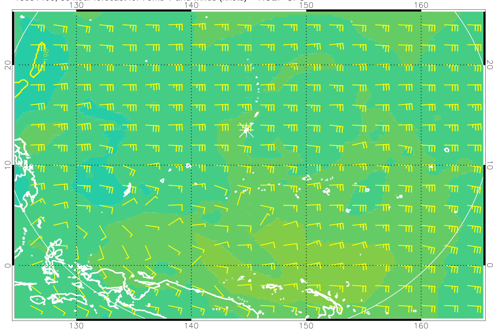
16091400, 60 hour forecast for 70mb T and winds (knots) -- NCEP GFS
