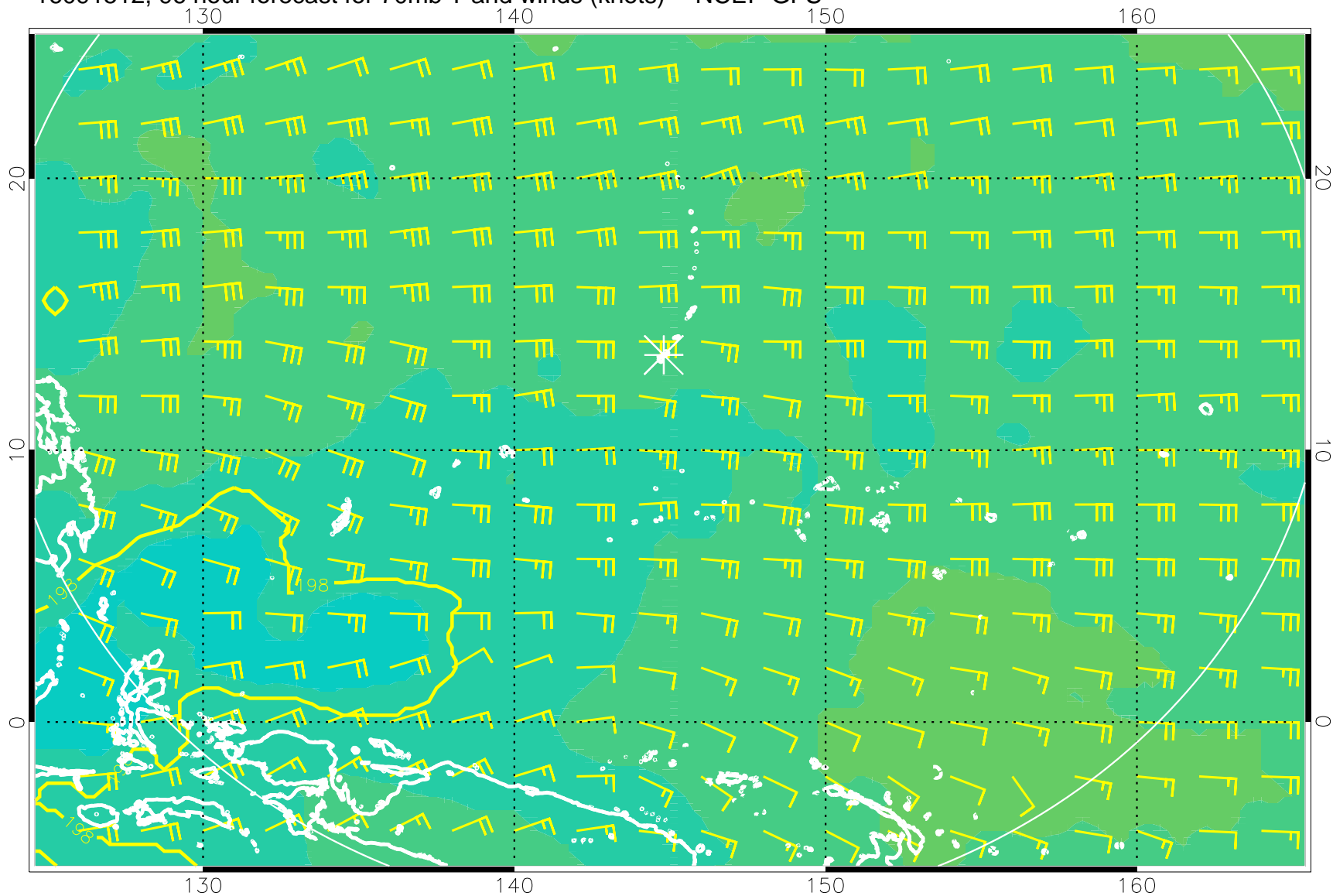
16091512, 96 hour forecast for 70mb T and winds (knots) -- NCEP GFS
