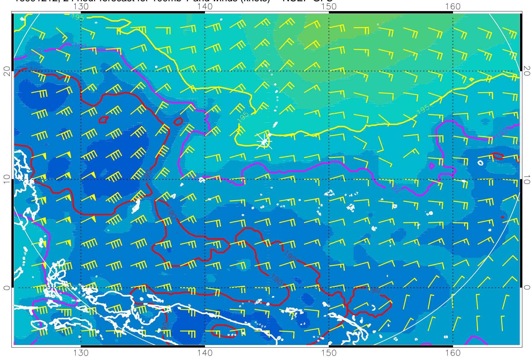
16091212, 24 hour forecast for 100mb T and winds (knots) -- NCEP GFS
