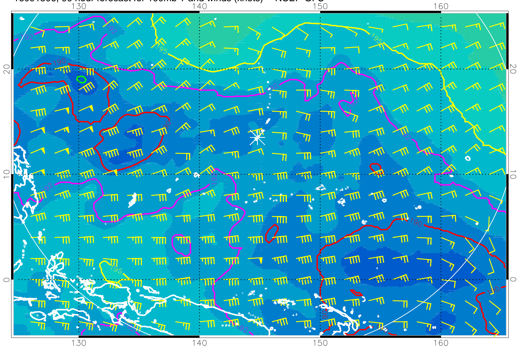
16091506, 90 hour forecast for 100mb T and winds (knots) -- NCEP GFS
