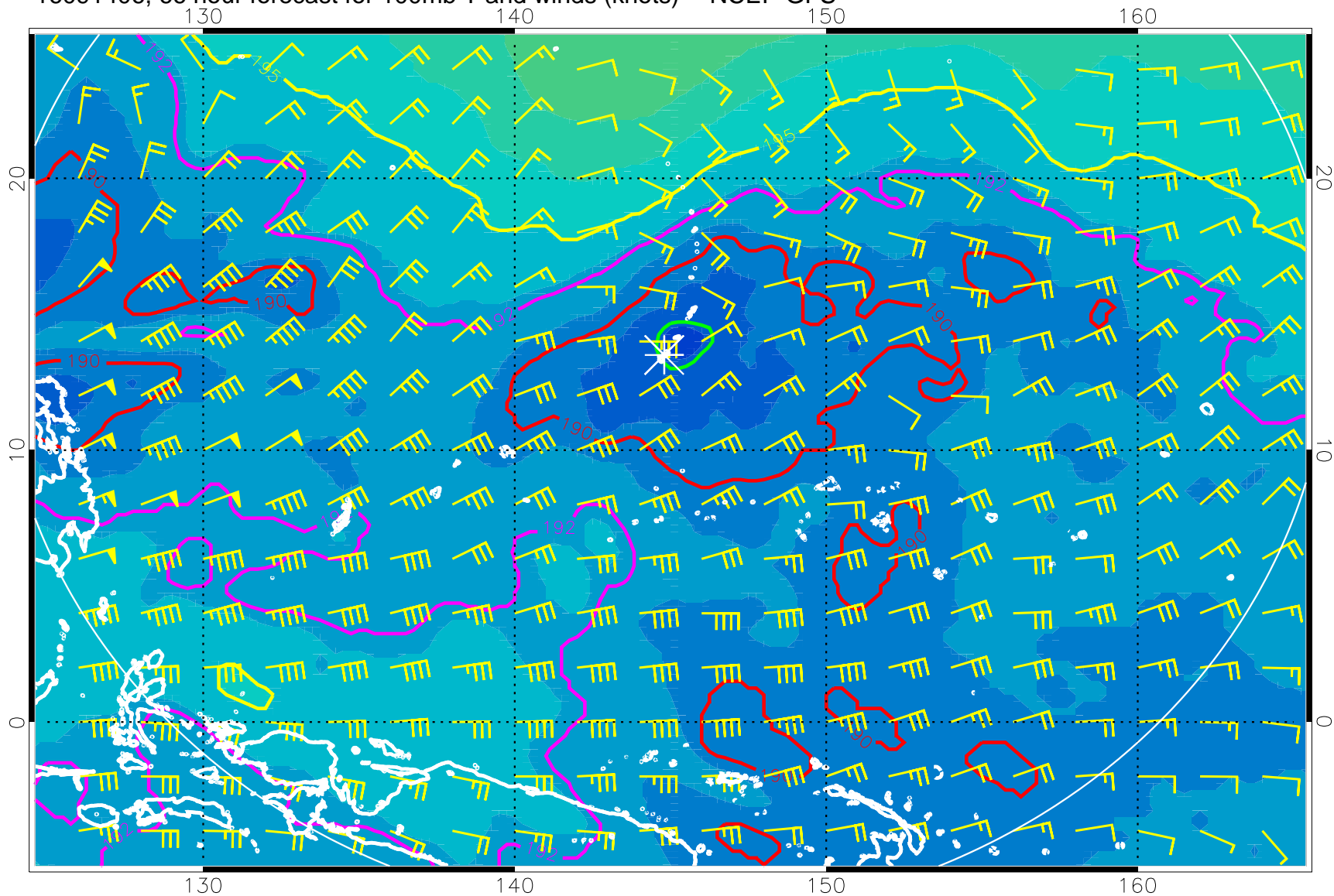
16091406, 66 hour forecast for 100mb T and winds (knots) -- NCEP GFS
