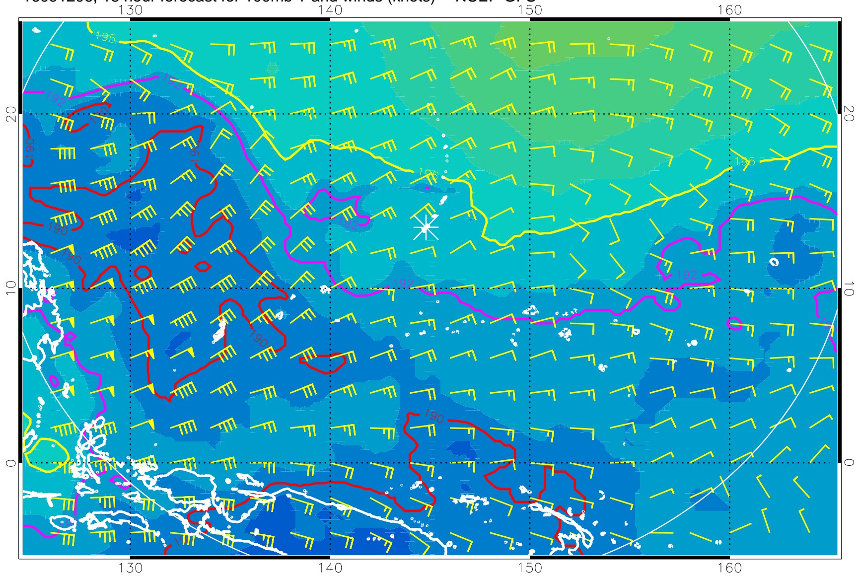
16091206, 18 hour forecast for 100mb T and winds (knots) -- NCEP GFS
