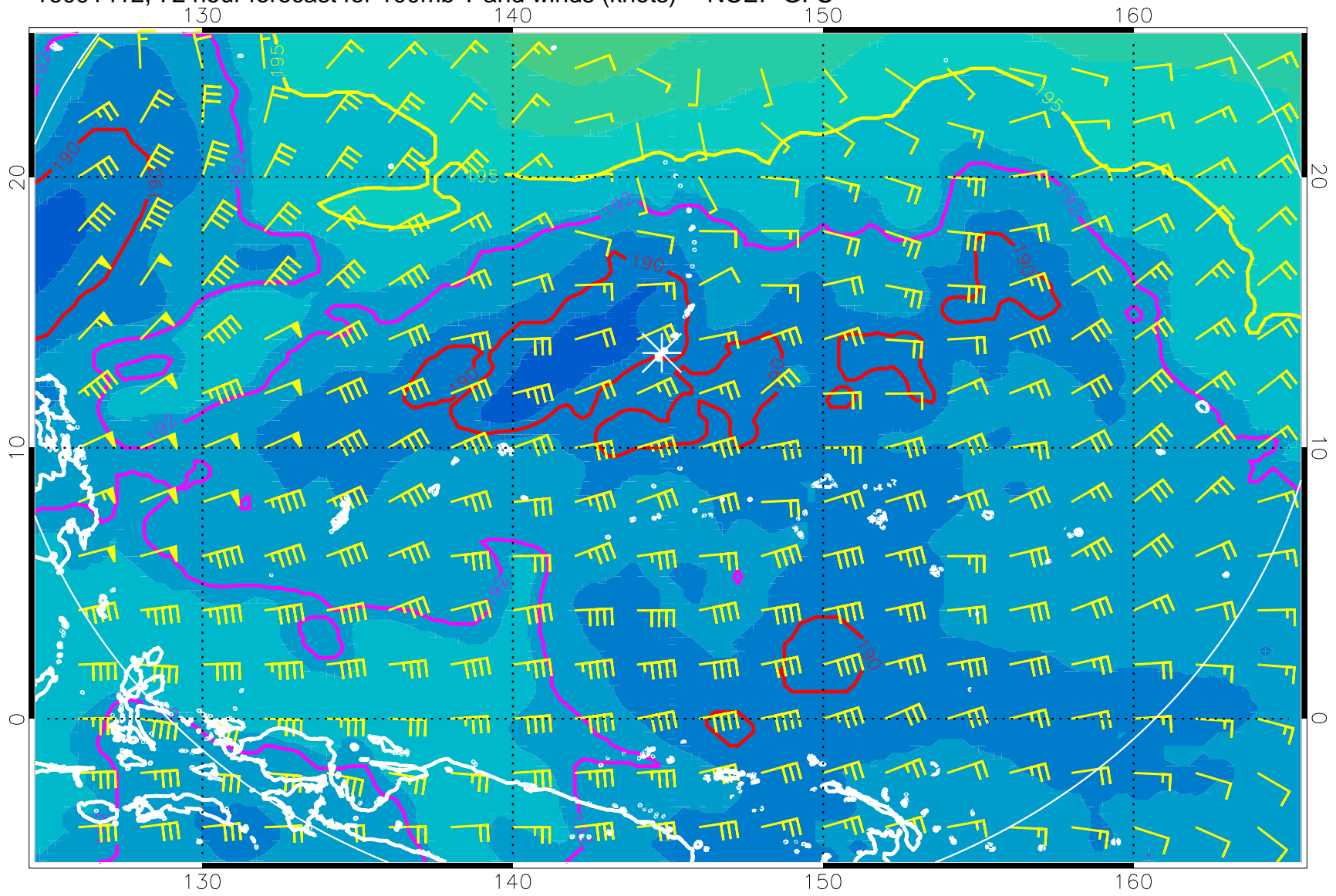
16091412, 72 hour forecast for 100mb T and winds (knots) -- NCEP GFS
