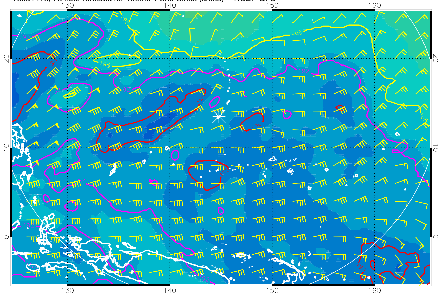
16091418, 78 hour forecast for 100mb T and winds (knots) -- NCEP GFS
