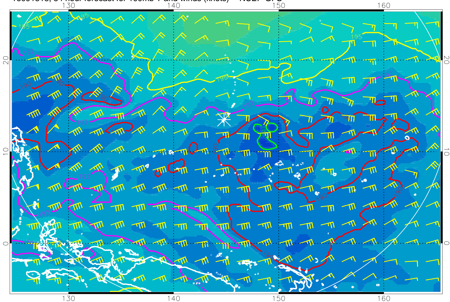
16091318, 54 hour forecast for 100mb T and winds (knots) -- NCEP GFS
