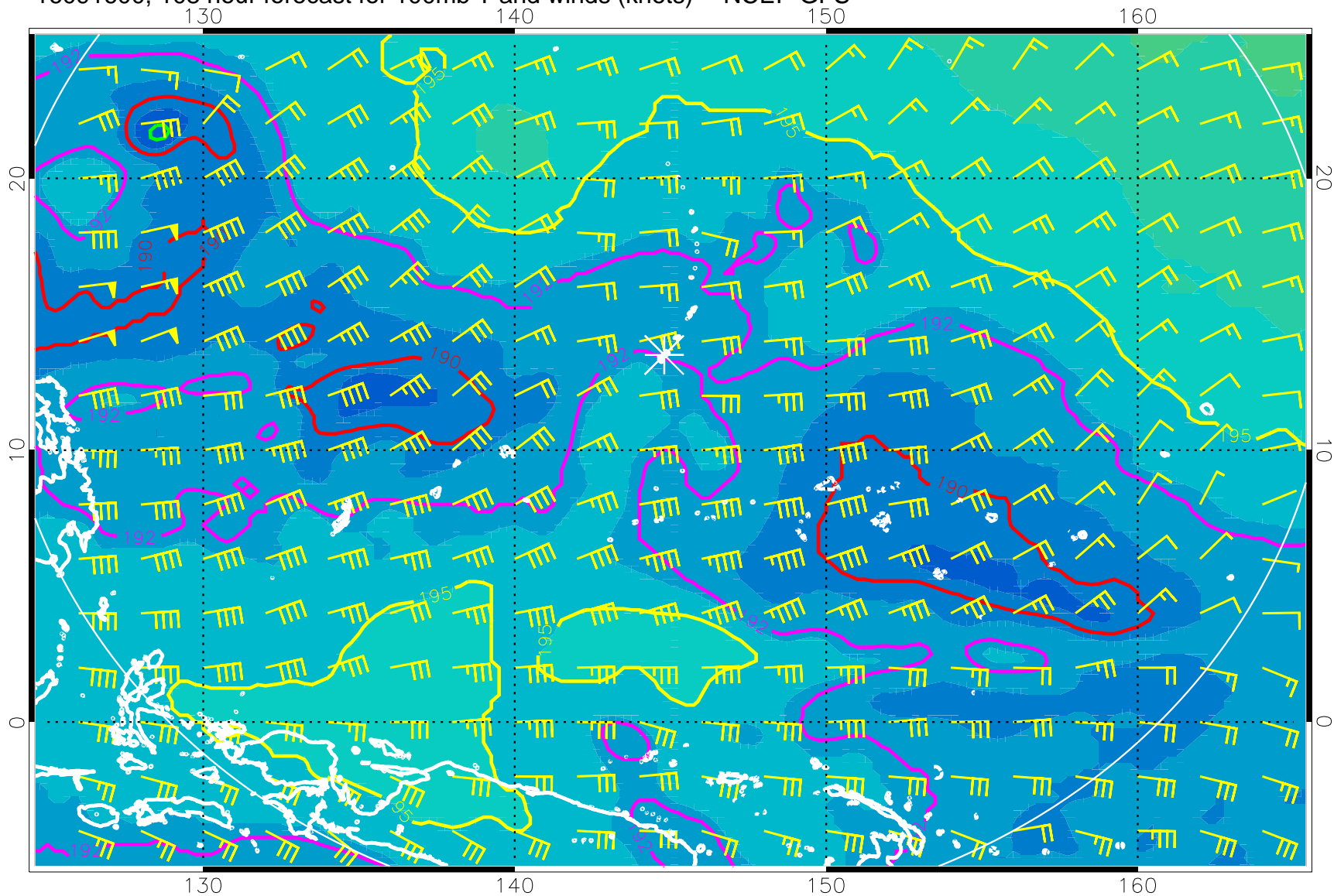
16091600, 108 hour forecast for 100mb T and winds (knots) -- NCEP GFS
