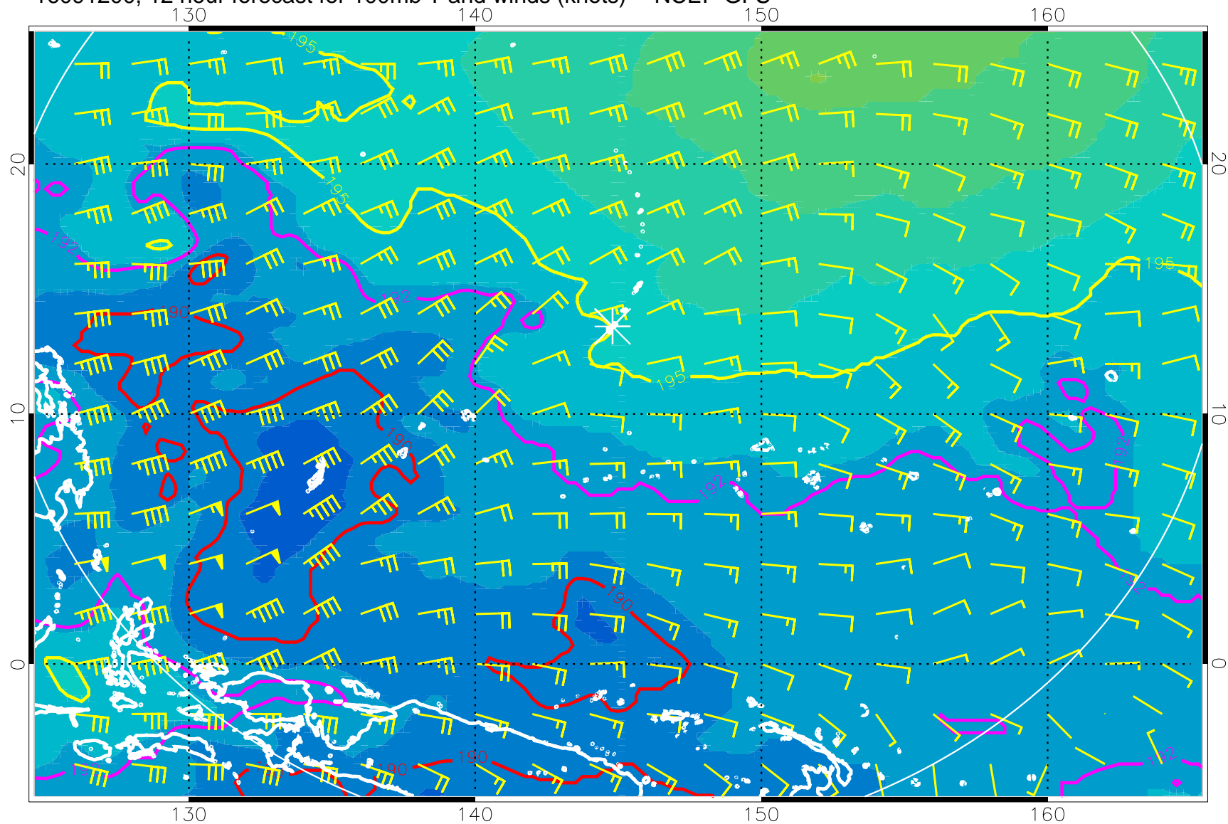
16091200, 12 hour forecast for 100mb T and winds (knots) -- NCEP GFS
