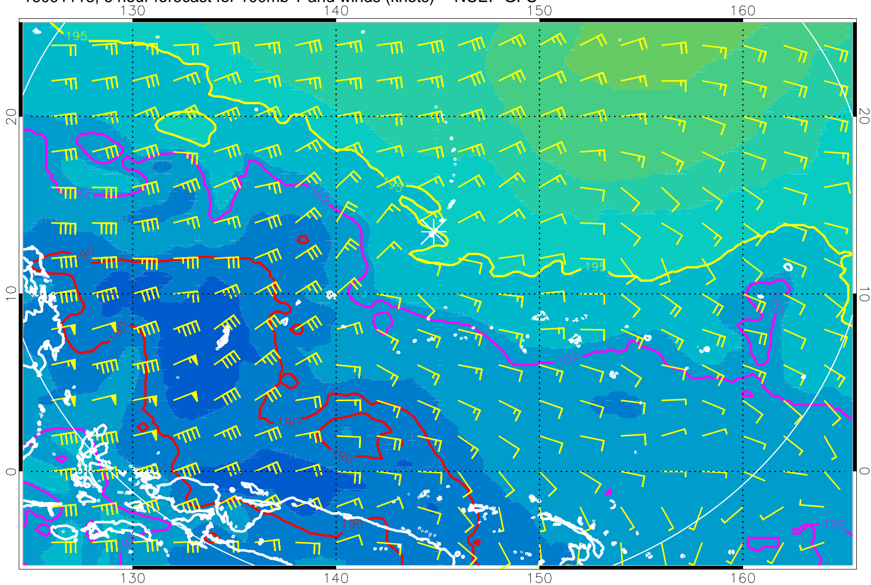
16091118, 6 hour forecast for 100mb T and winds (knots) -- NCEP GFS
