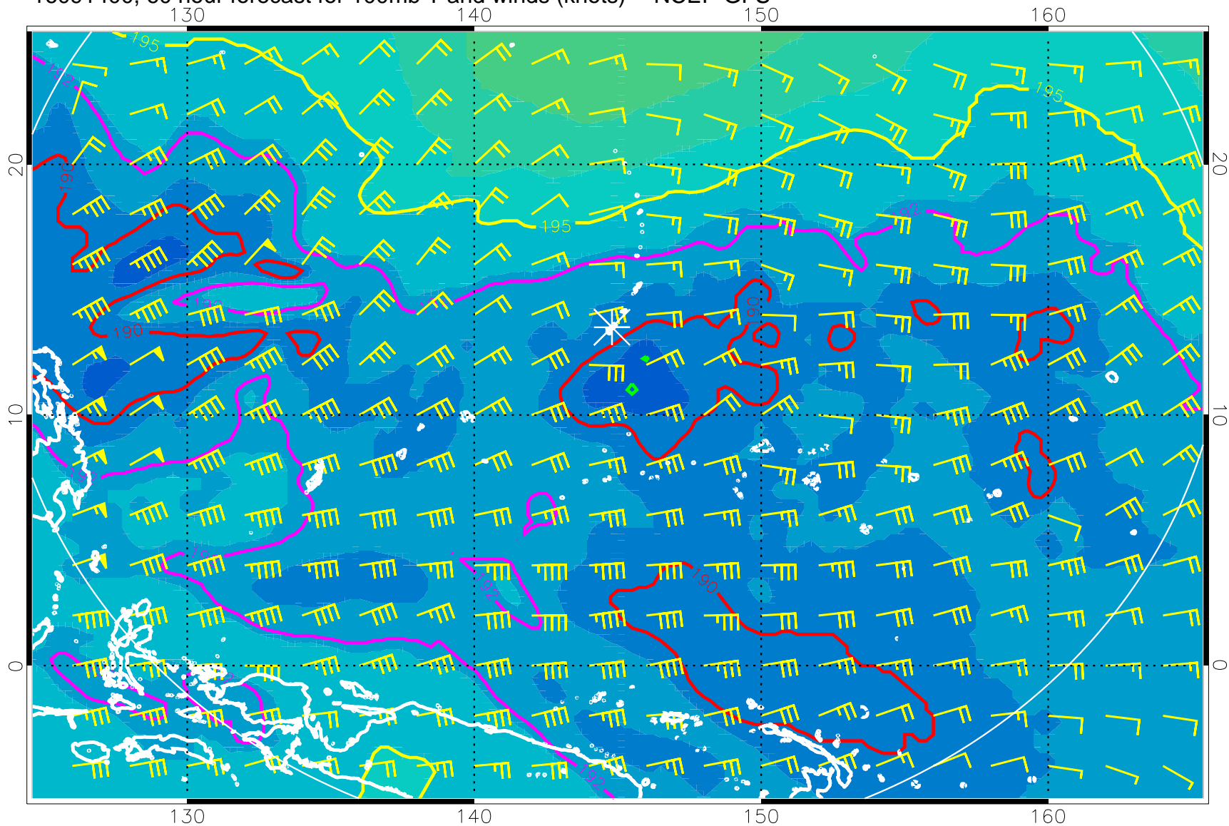
16091400, 60 hour forecast for 100mb T and winds (knots) -- NCEP GFS
