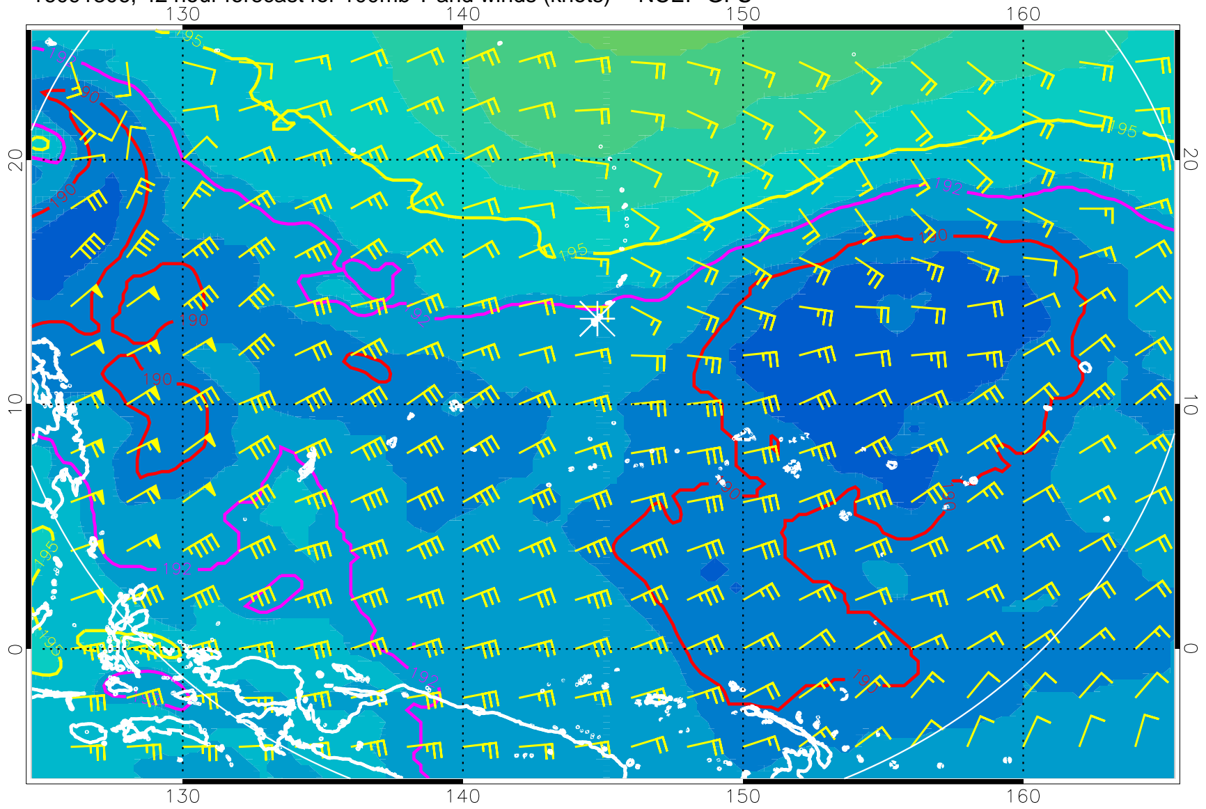
16091306, 42 hour forecast for 100mb T and winds (knots) -- NCEP GFS
