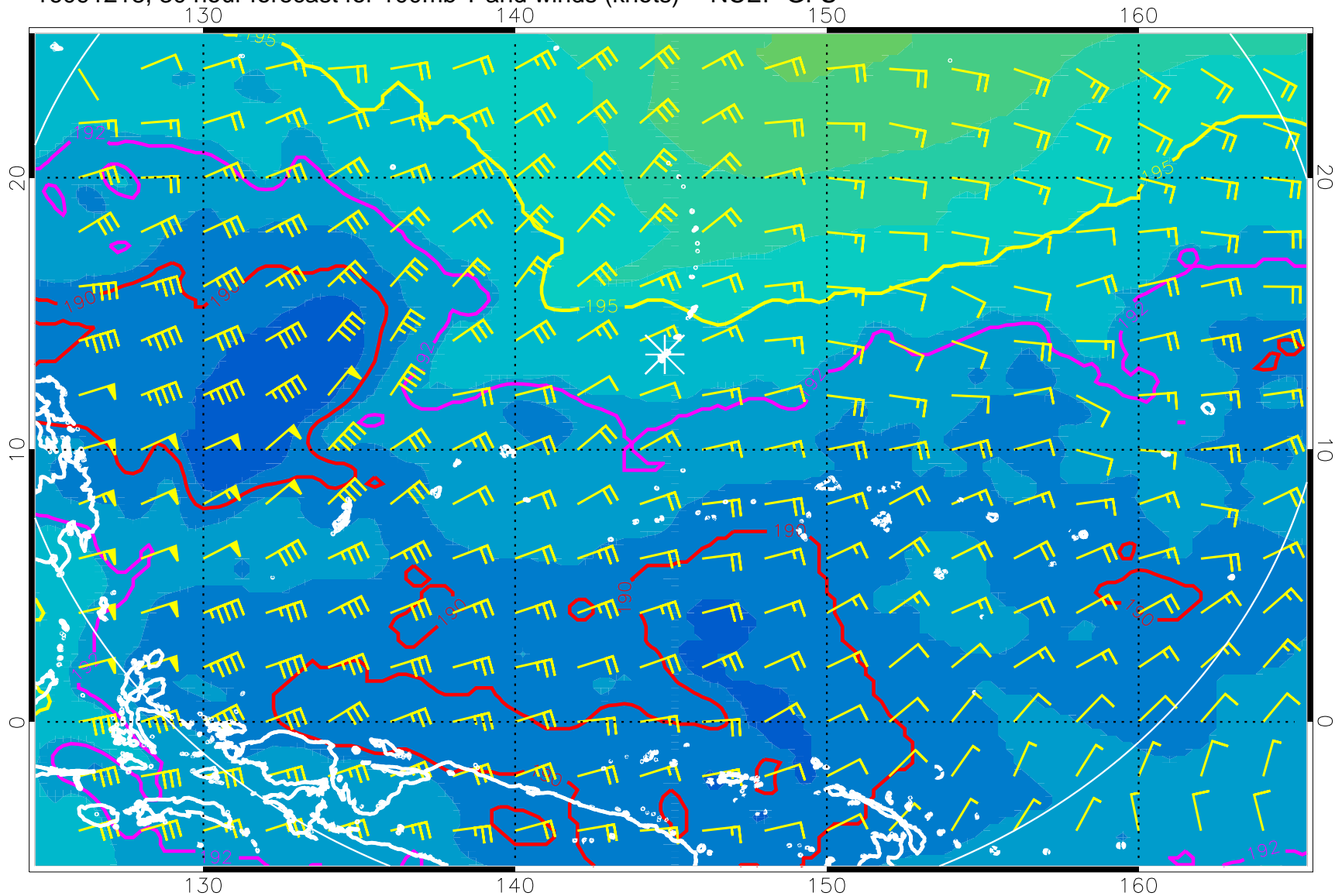
16091218, 30 hour forecast for 100mb T and winds (knots) -- NCEP GFS
