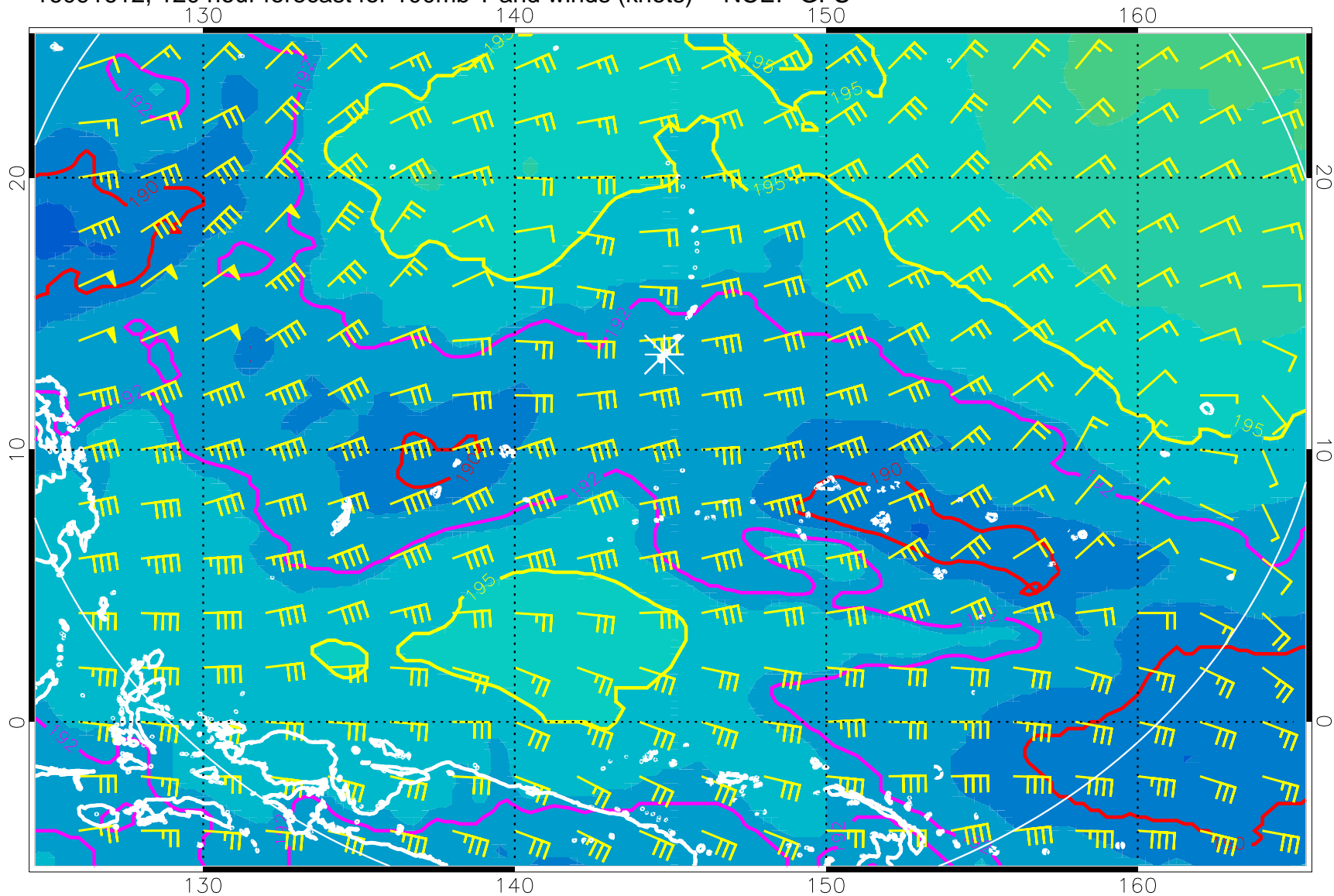
16091612, 120 hour forecast for 100mb T and winds (knots) -- NCEP GFS
