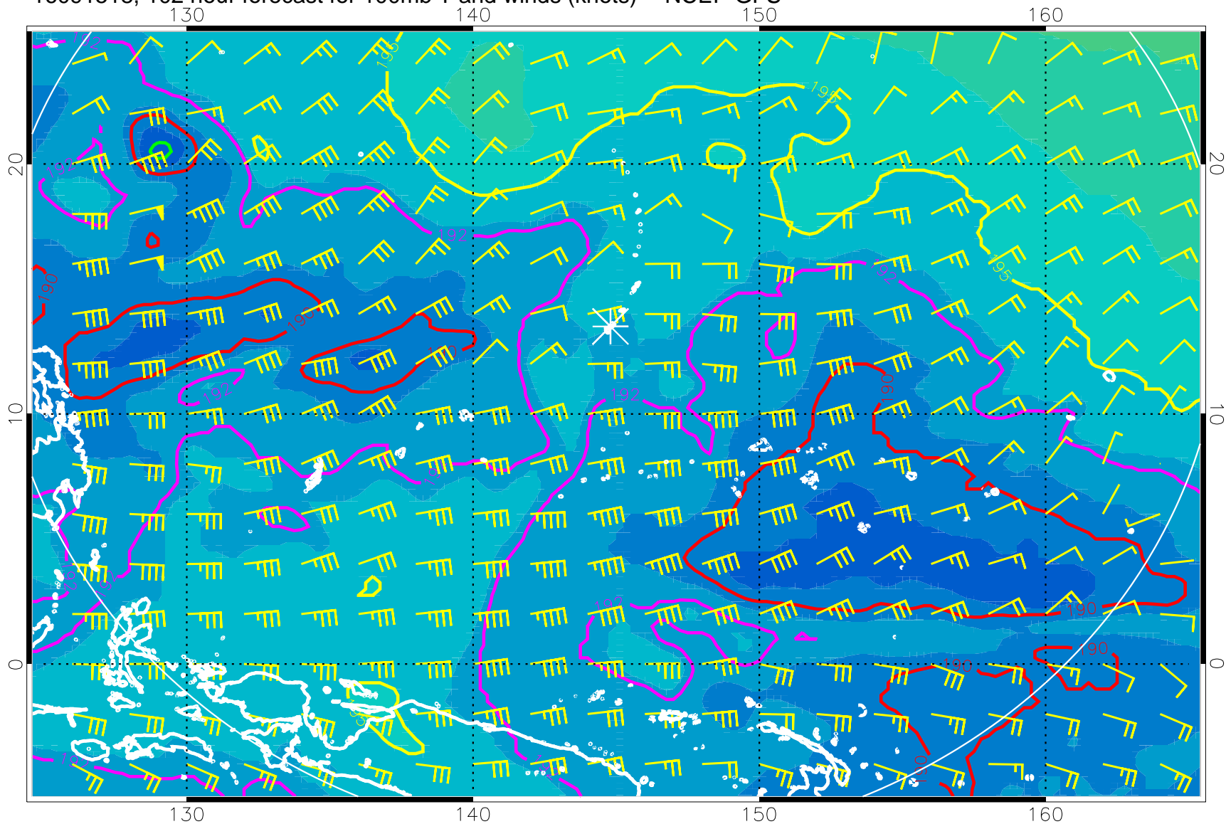
16091518, 102 hour forecast for 100mb T and winds (knots) -- NCEP GFS
