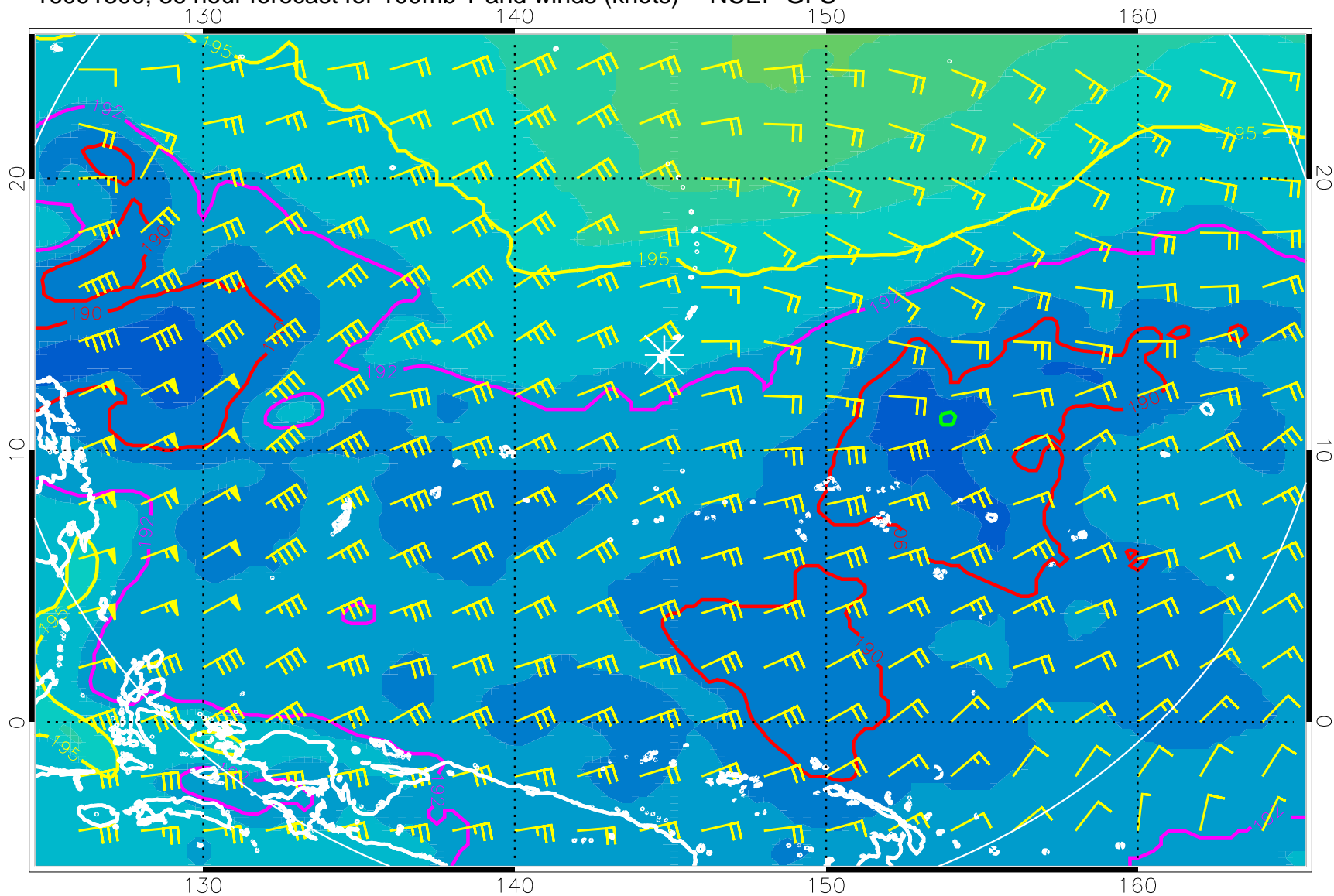
16091300, 36 hour forecast for 100mb T and winds (knots) -- NCEP GFS
