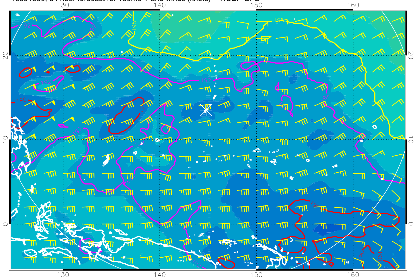
16091500, 84 hour forecast for 100mb T and winds (knots) -- NCEP GFS
