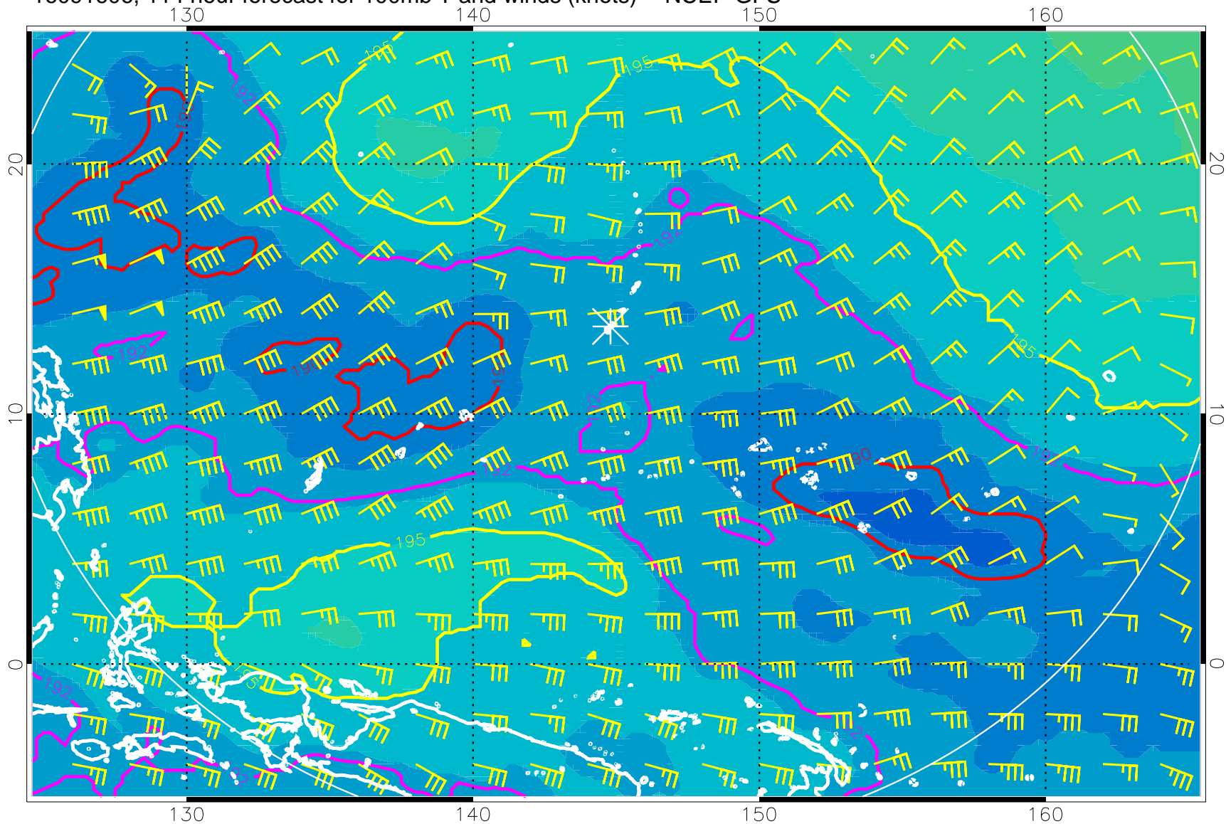
16091606, 114 hour forecast for 100mb T and winds (knots) -- NCEP GFS
