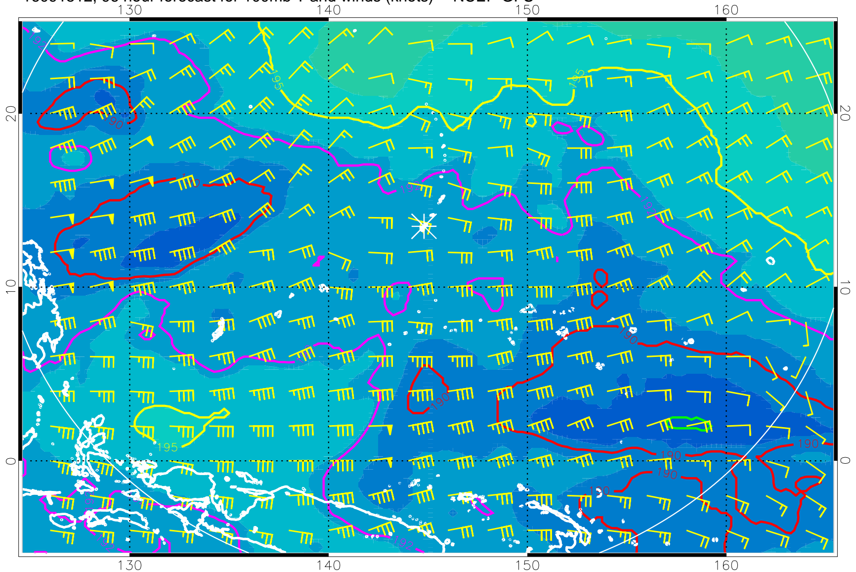
16091512, 96 hour forecast for 100mb T and winds (knots) -- NCEP GFS
