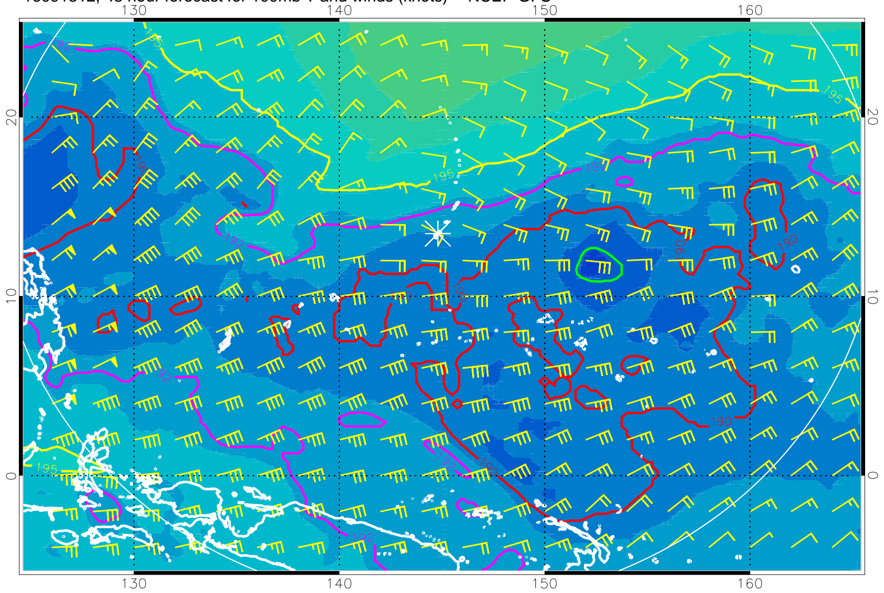
16091312, 48 hour forecast for 100mb T and winds (knots) -- NCEP GFS
