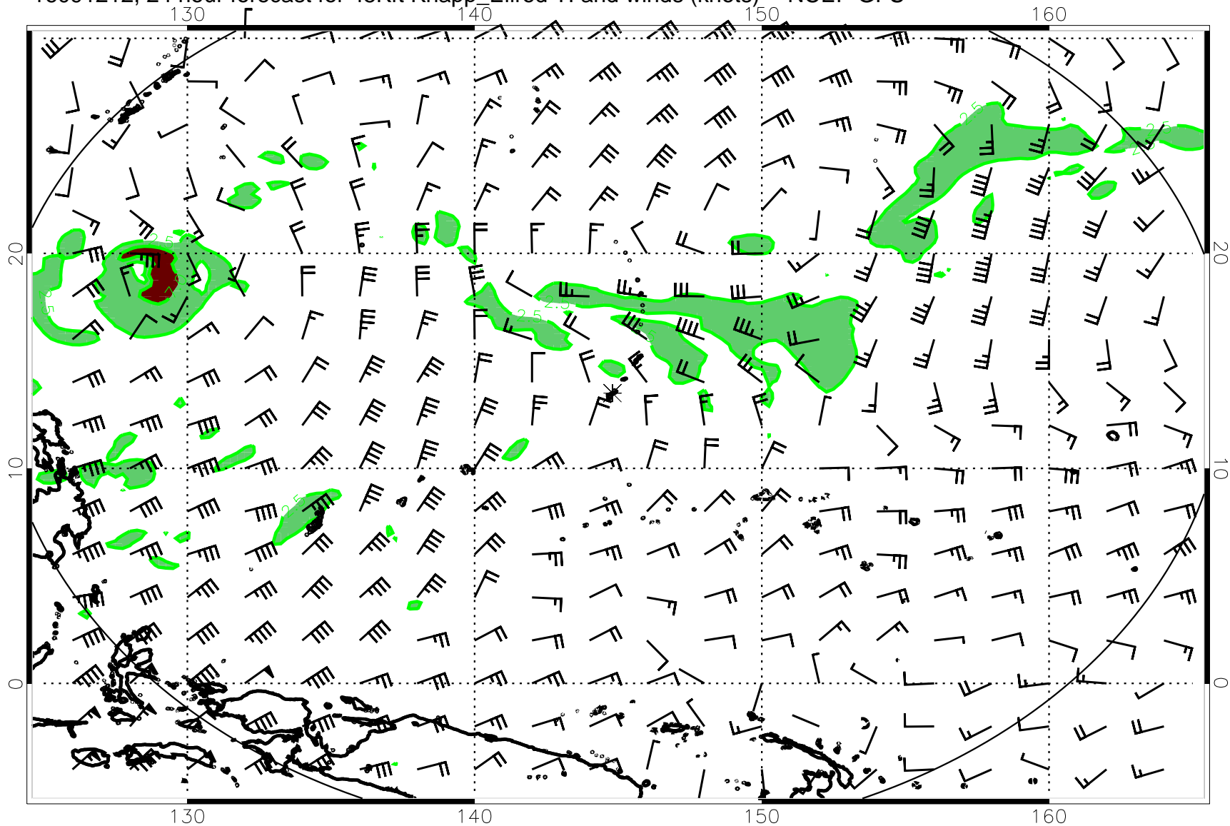
16091212, 24 hour forecast for 45Kft Knapp_Ellrod TI and winds (knots) -- NCEP GFS
