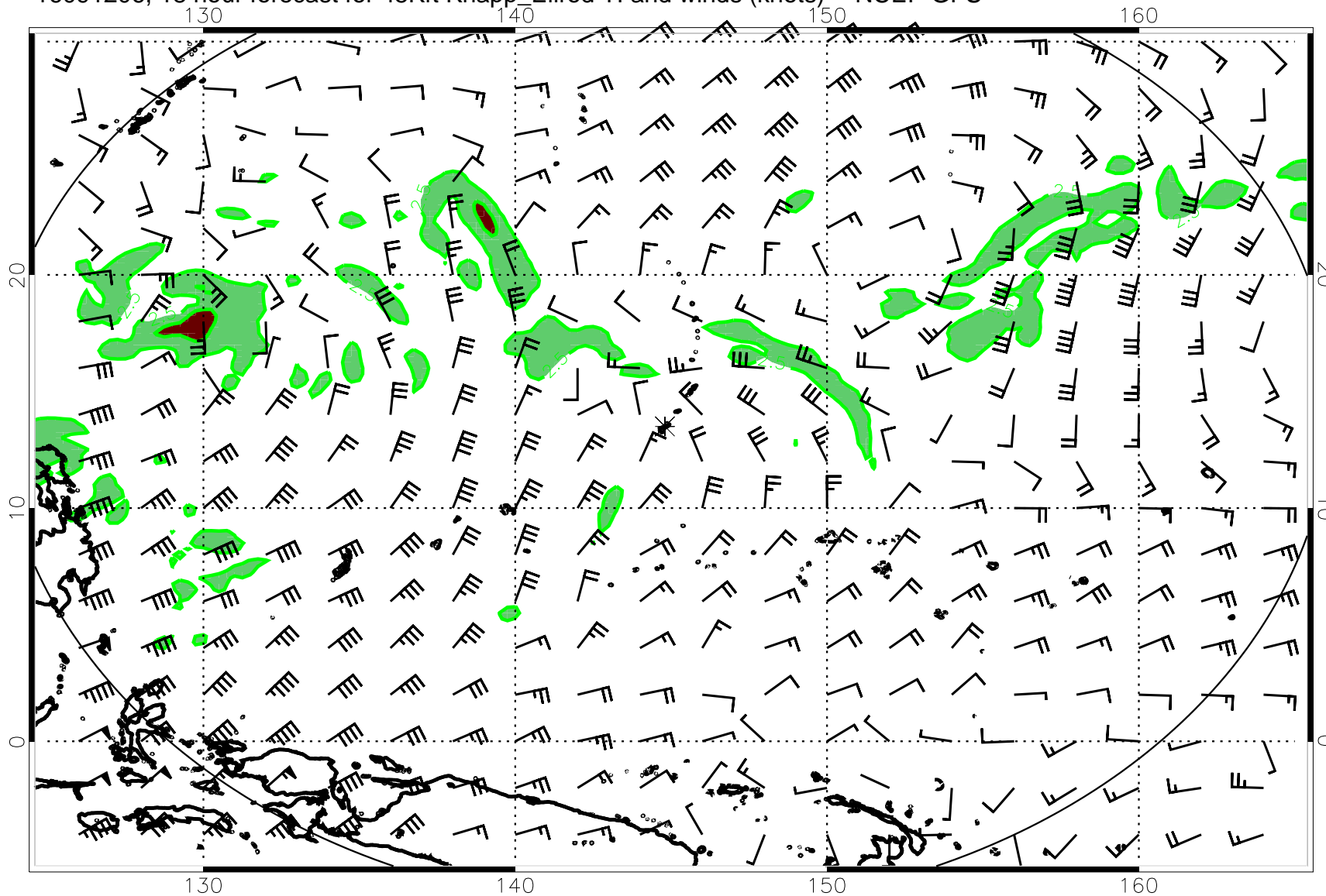
16091206, 18 hour forecast for 45Kft Knapp_Ellrod TI and winds (knots) -- NCEP GFS
