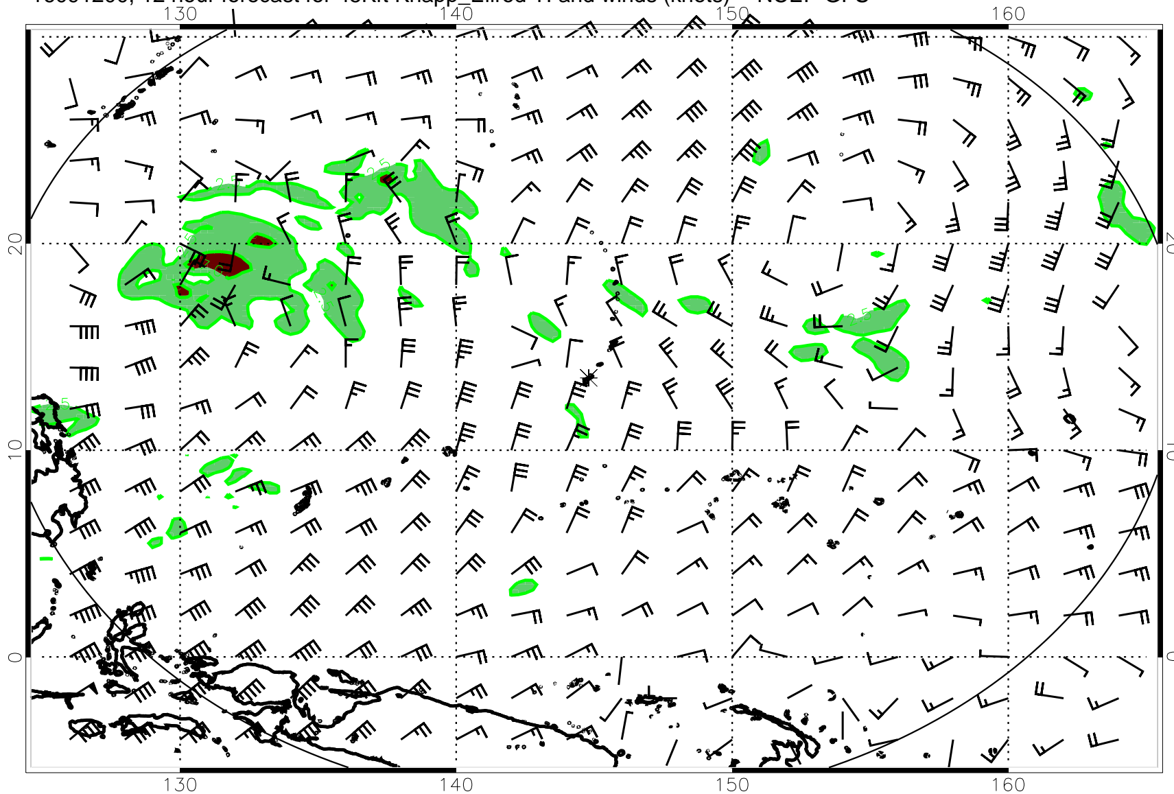
16091200, 12 hour forecast for 45Kft Knapp_Ellrod TI and winds (knots) -- NCEP GFS
