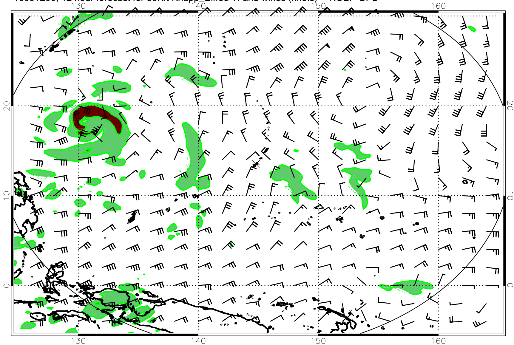
16091200, 12 hour forecast for 39Kft Knapp_Ellrod TI and winds (knots) -- NCEP GFS
