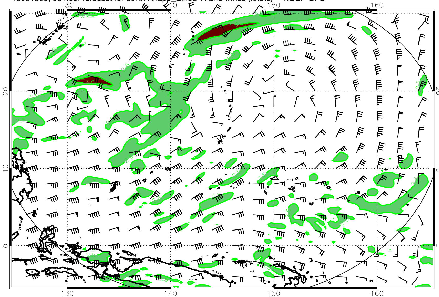
16091506, 90 hour forecast for 39Kft Knapp_Ellrod TI and winds (knots) -- NCEP GFS
