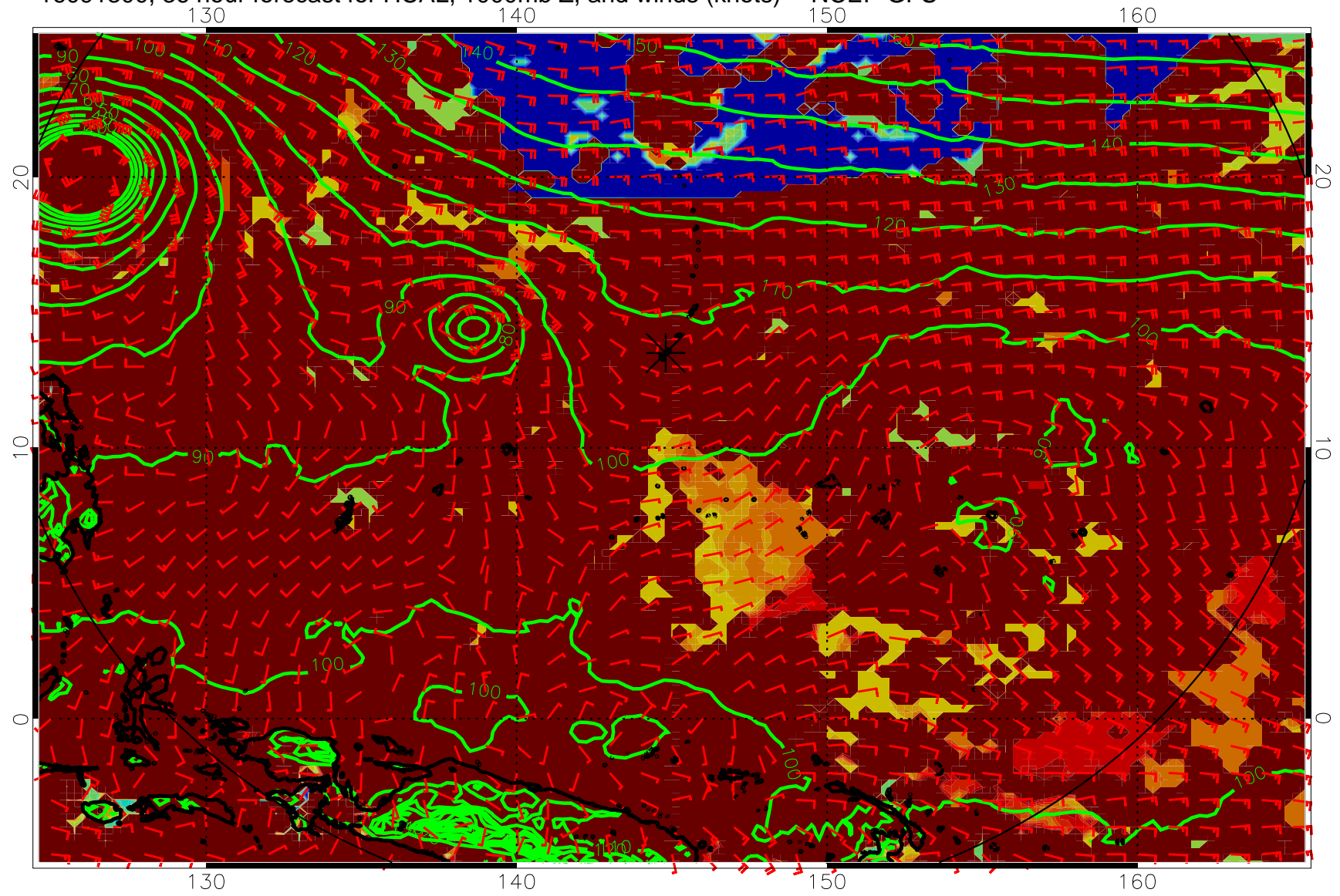
16091300, 36 hour forecast for HCAL, 1000mb Z, and winds (knots) -- NCEP GFS
