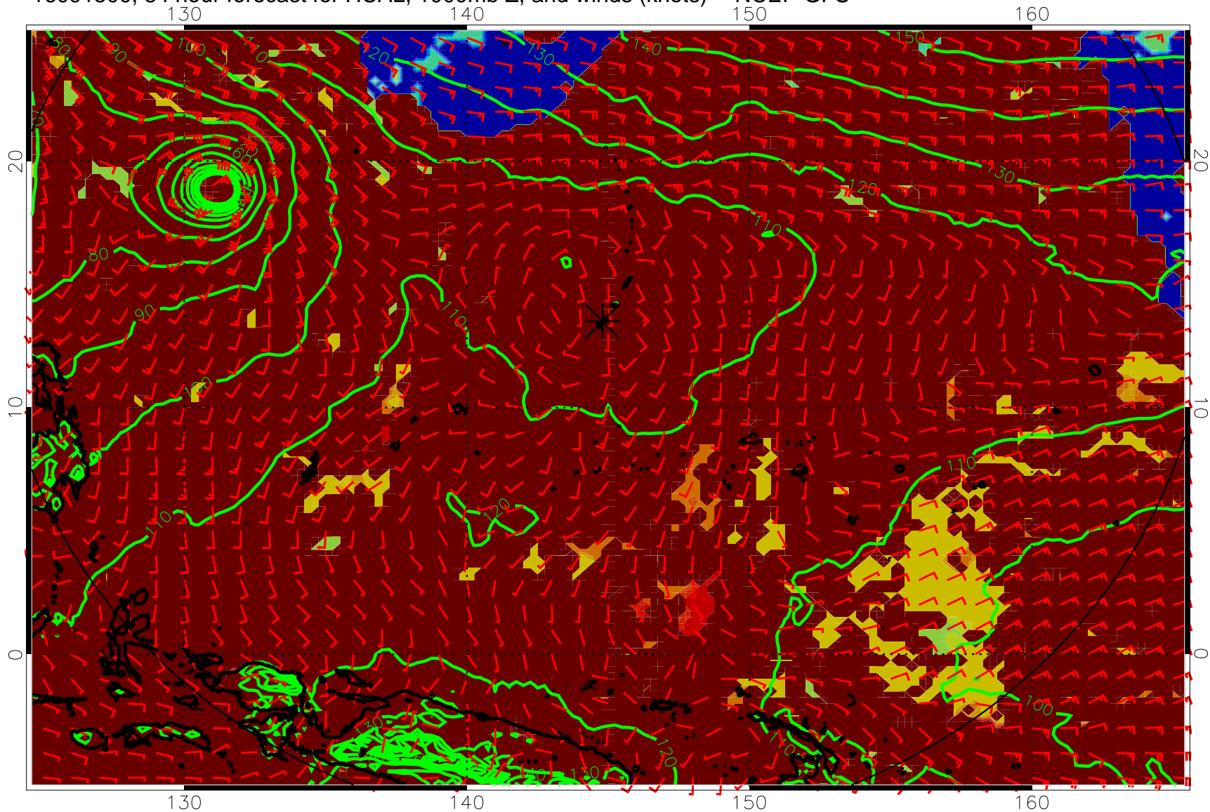
16091500, 84 hour forecast for HCAL, 1000mb Z, and winds (knots) -- NCEP GFS
