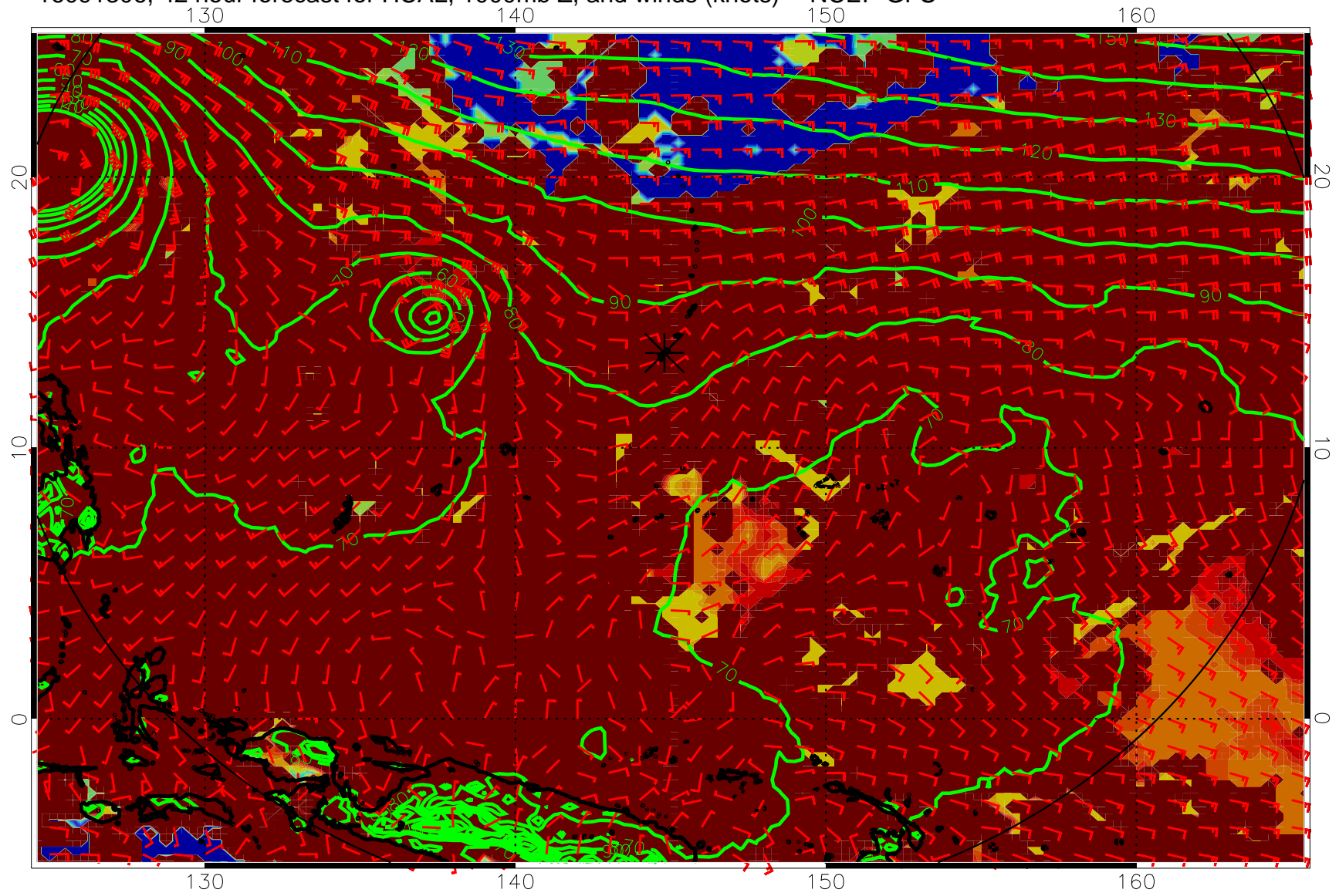
16091306, 42 hour forecast for HCAL, 1000mb Z, and winds (knots) -- NCEP GFS
