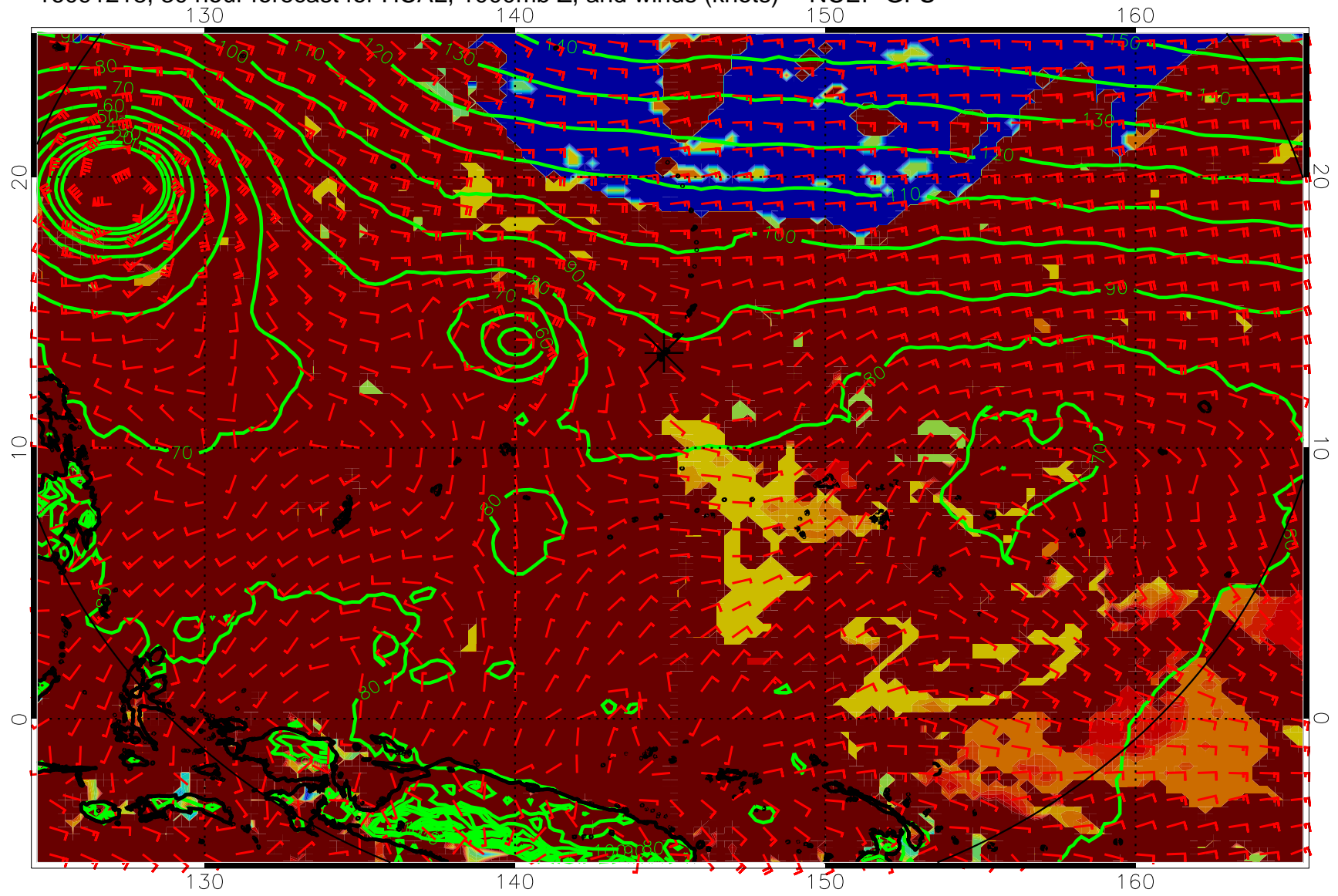
16091218, 30 hour forecast for HCAL, 1000mb Z, and winds (knots) -- NCEP GFS
