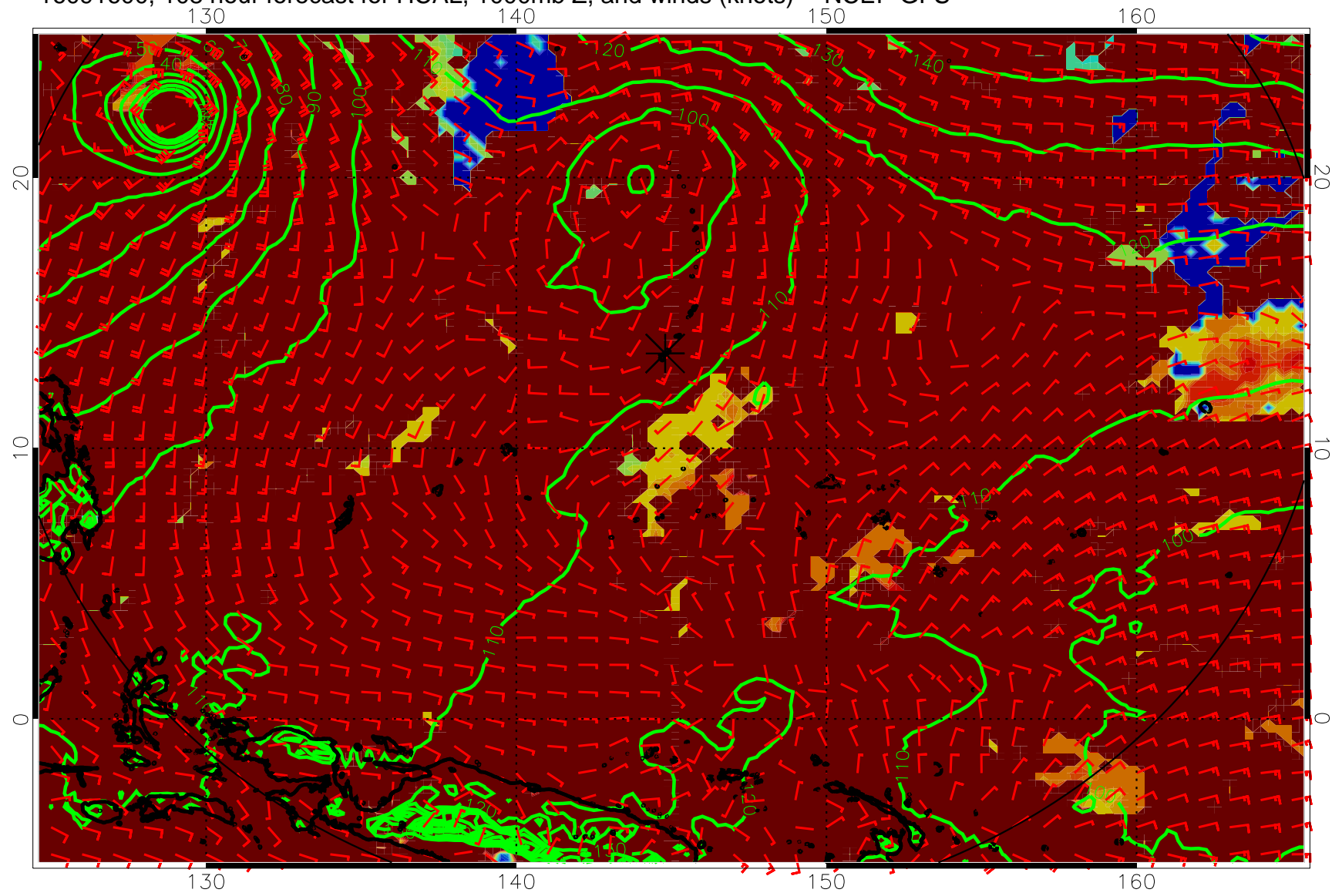
16091600, 108 hour forecast for HCAL, 1000mb Z, and winds (knots) -- NCEP GFS
