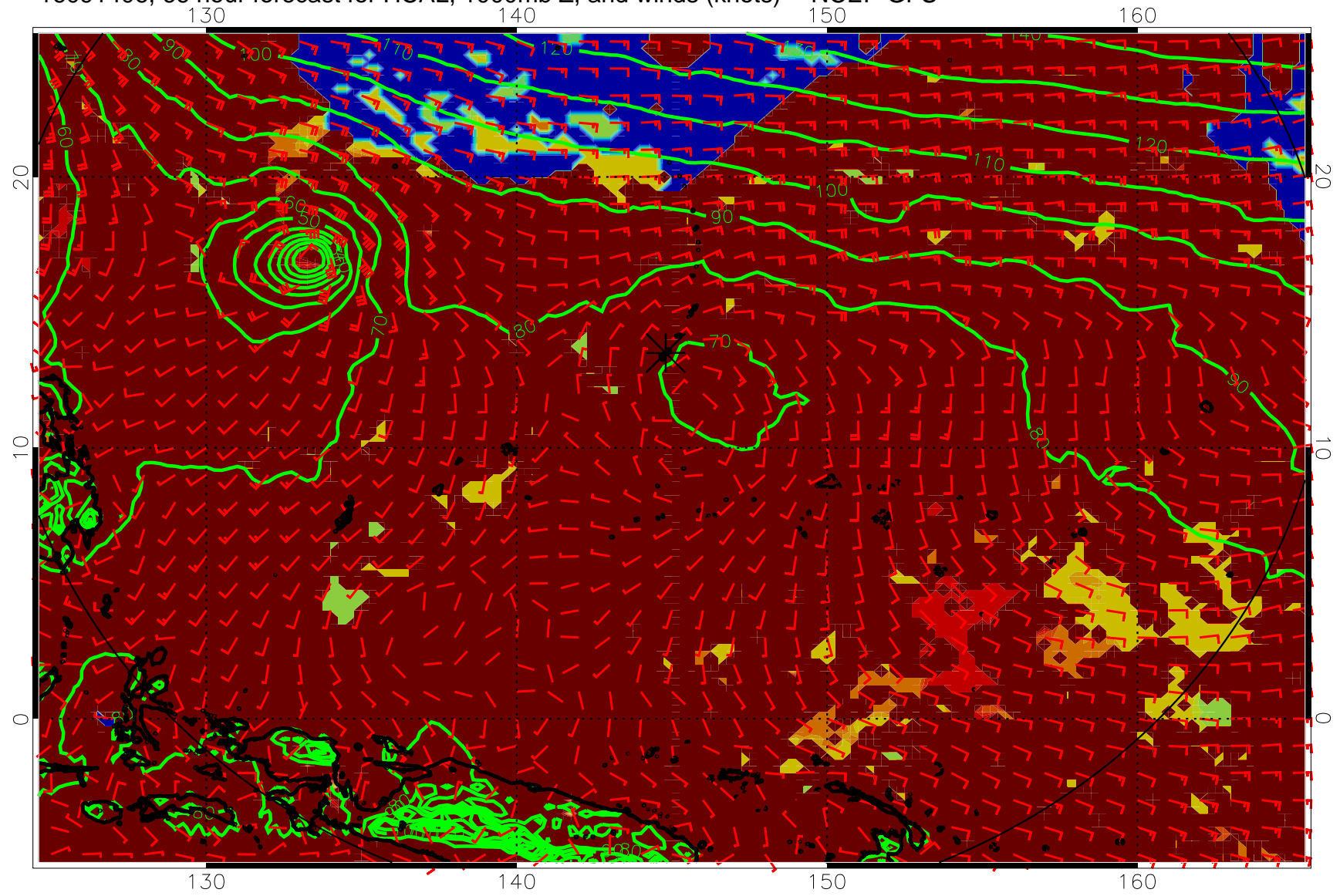
16091406, 66 hour forecast for HCAL, 1000mb Z, and winds (knots) -- NCEP GFS
