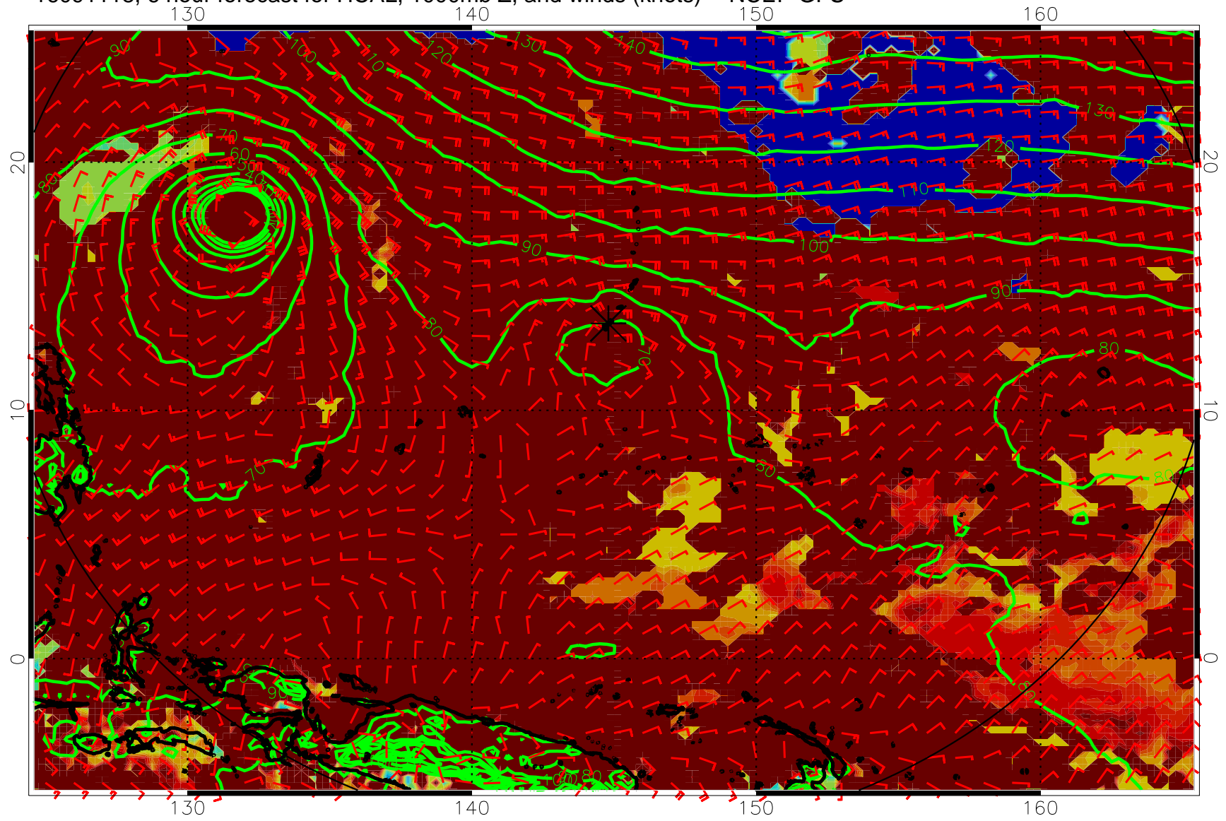
16091118, 6 hour forecast for HCAL, 1000mb Z, and winds (knots) -- NCEP GFS
