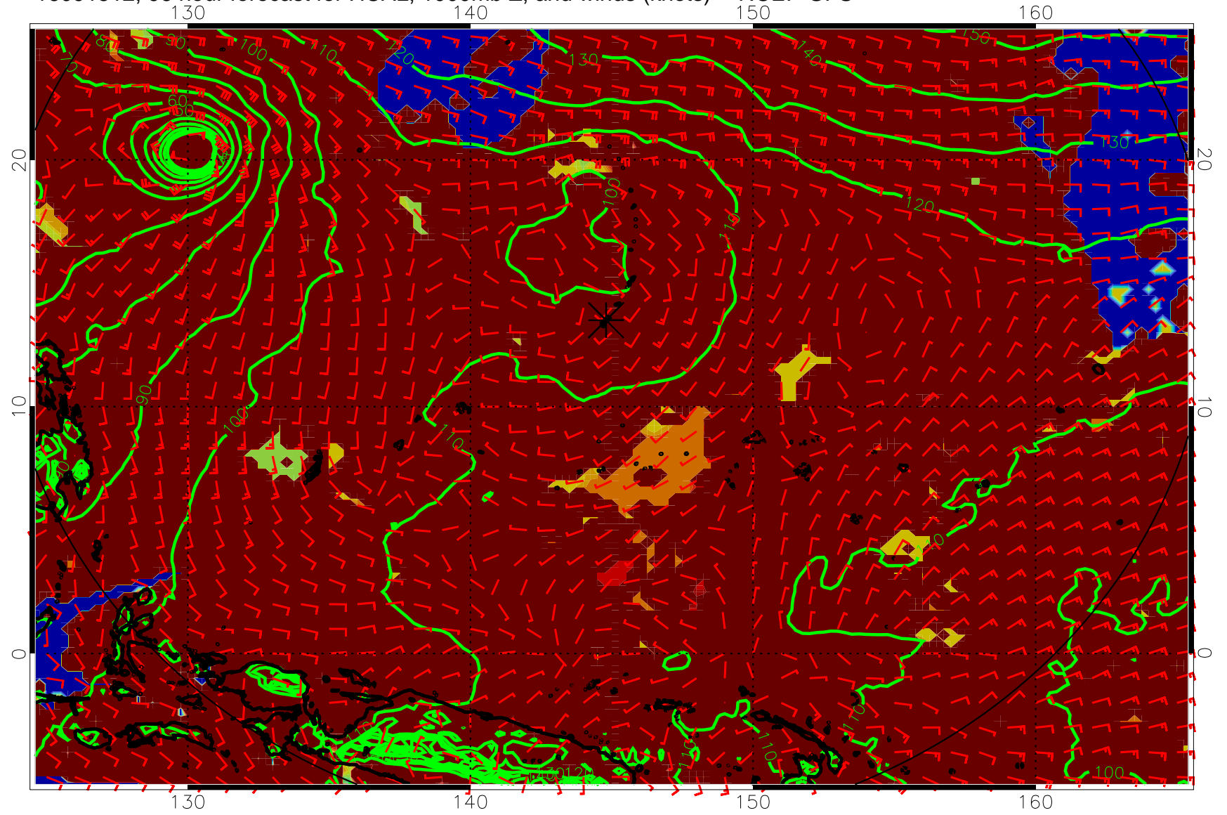
16091512, 96 hour forecast for HCAL, 1000mb Z, and winds (knots) -- NCEP GFS
