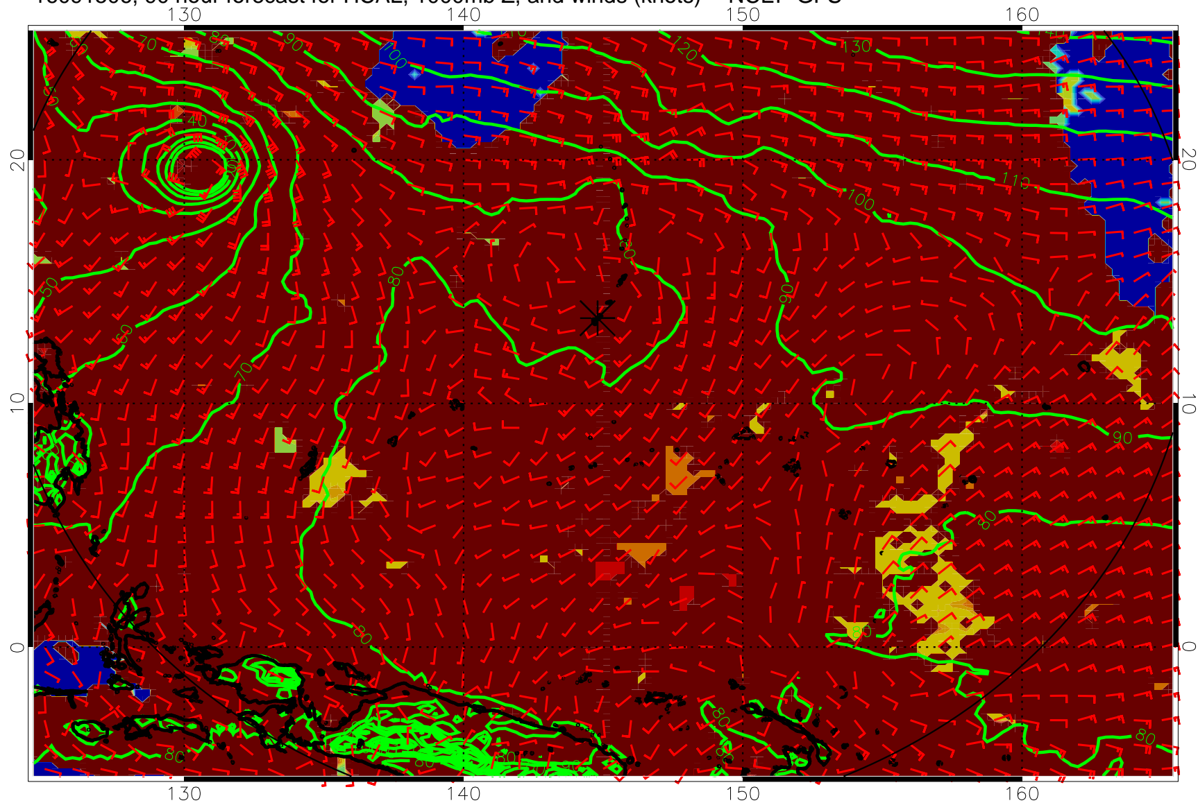
16091506, 90 hour forecast for HCAL, 1000mb Z, and winds (knots) -- NCEP GFS
