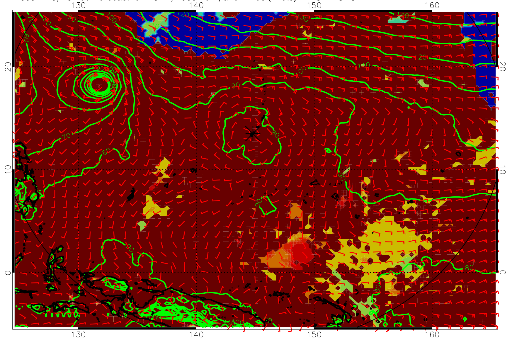
16091418, 78 hour forecast for HCAL, 1000mb Z, and winds (knots) -- NCEP GFS
