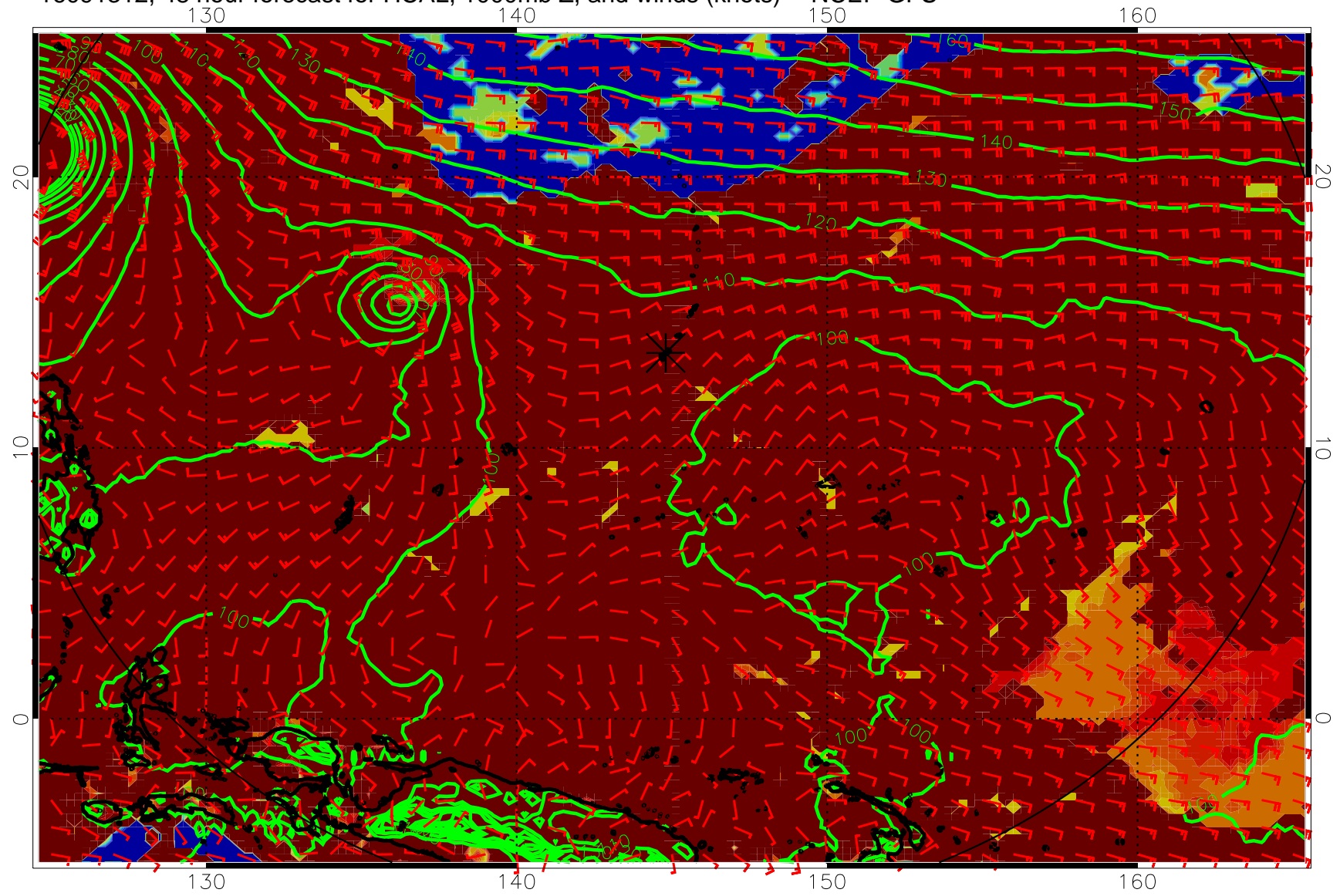
16091312, 48 hour forecast for HCAL, 1000mb Z, and winds (knots) -- NCEP GFS
