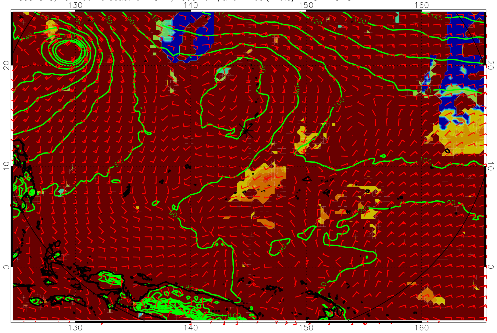
16091518, 102 hour forecast for HCAL, 1000mb Z, and winds (knots) -- NCEP GFS
