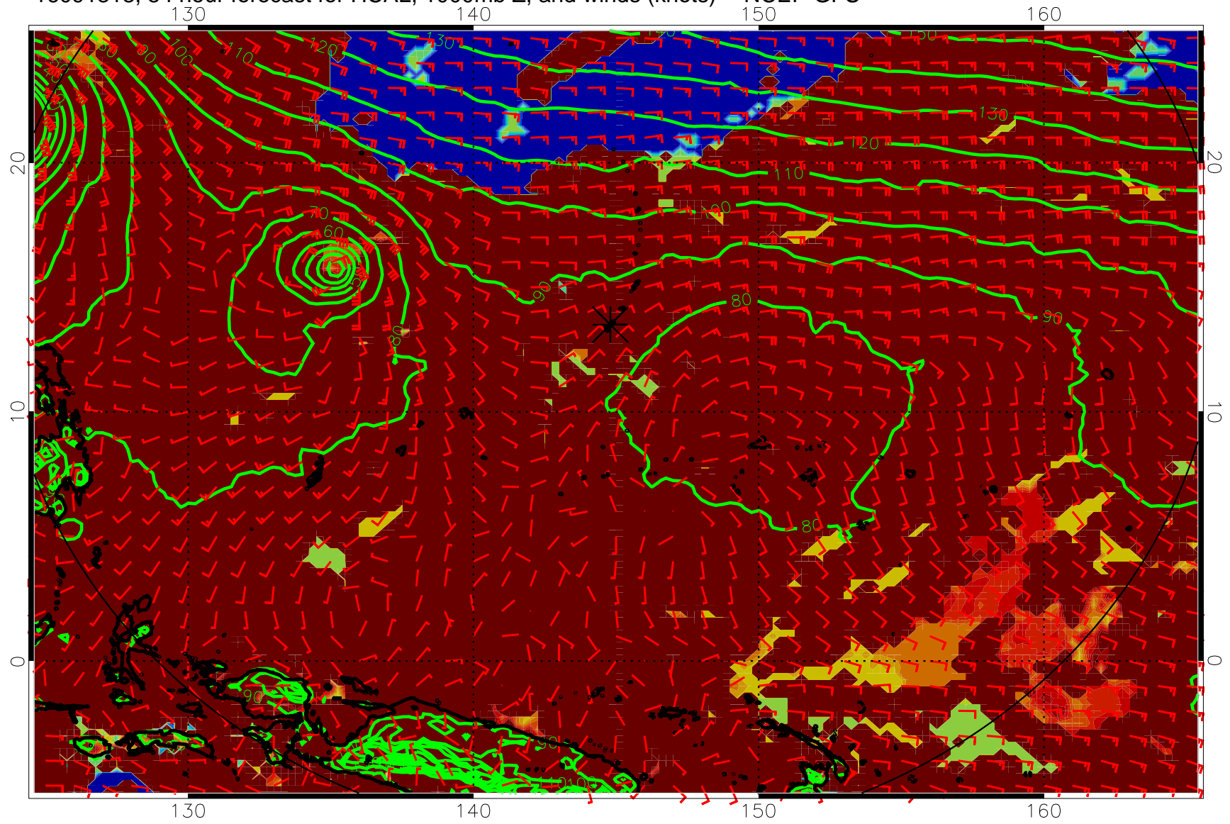
16091318, 54 hour forecast for HCAL, 1000mb Z, and winds (knots) -- NCEP GFS
