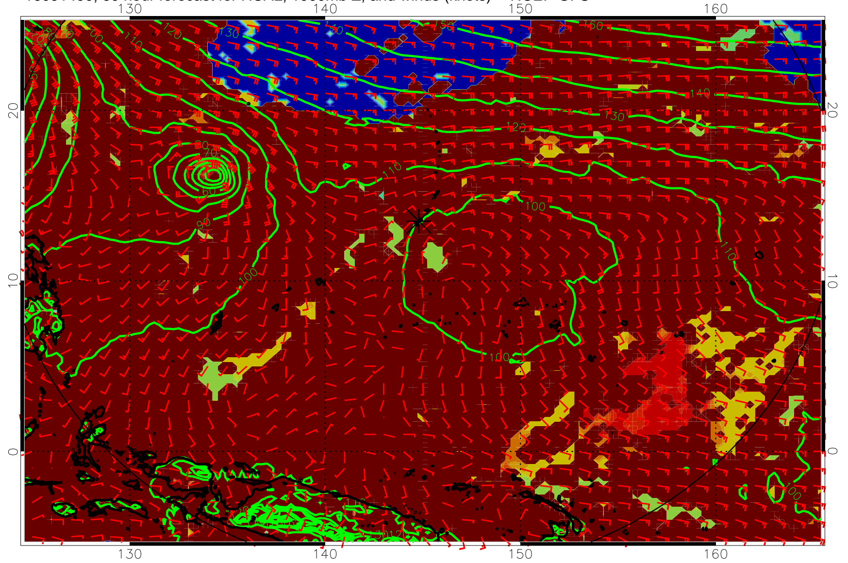
16091400, 60 hour forecast for HCAL, 1000mb Z, and winds (knots) -- NCEP GFS
