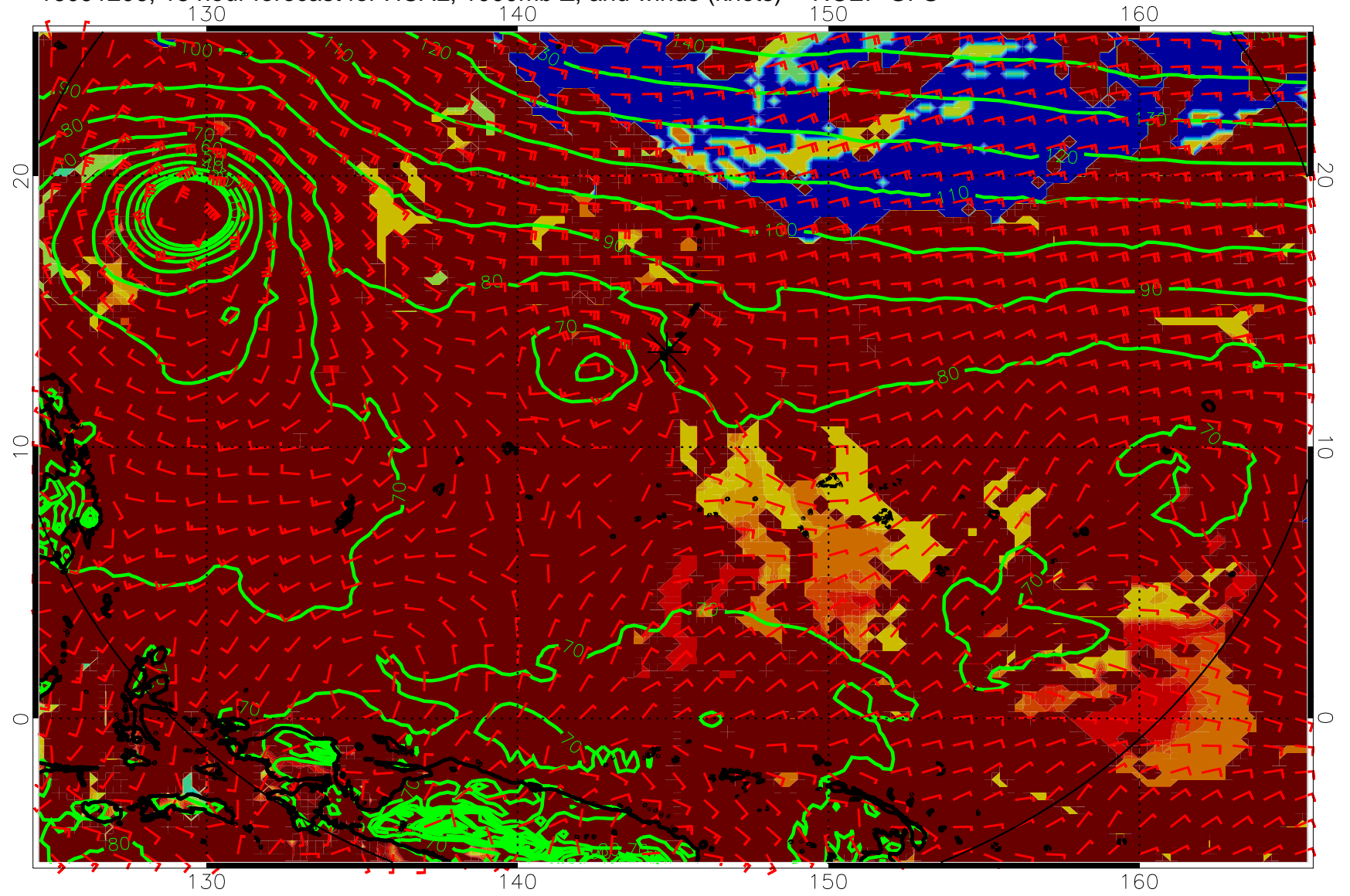
16091206, 18 hour forecast for HCAL, 1000mb Z, and winds (knots) -- NCEP GFS
