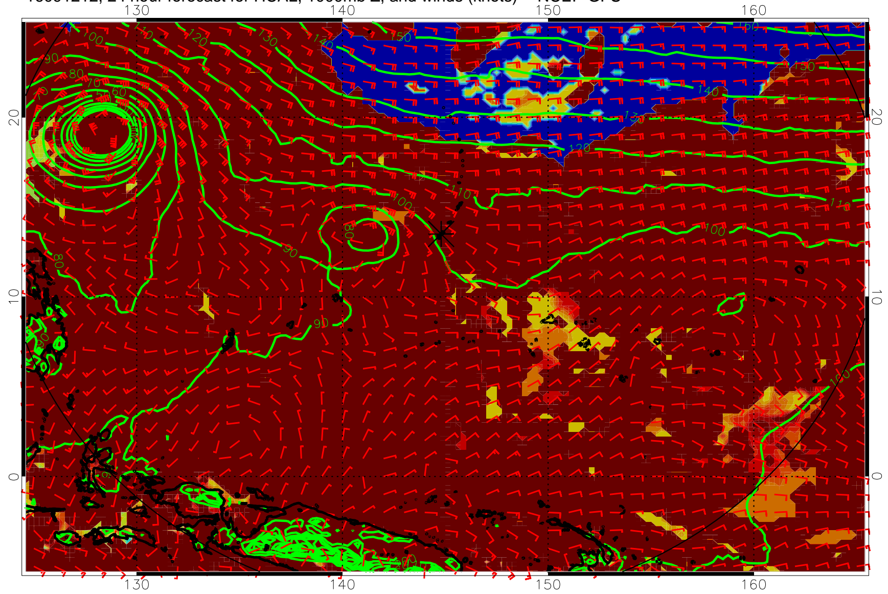
16091212, 24 hour forecast for HCAL, 1000mb Z, and winds (knots) -- NCEP GFS
