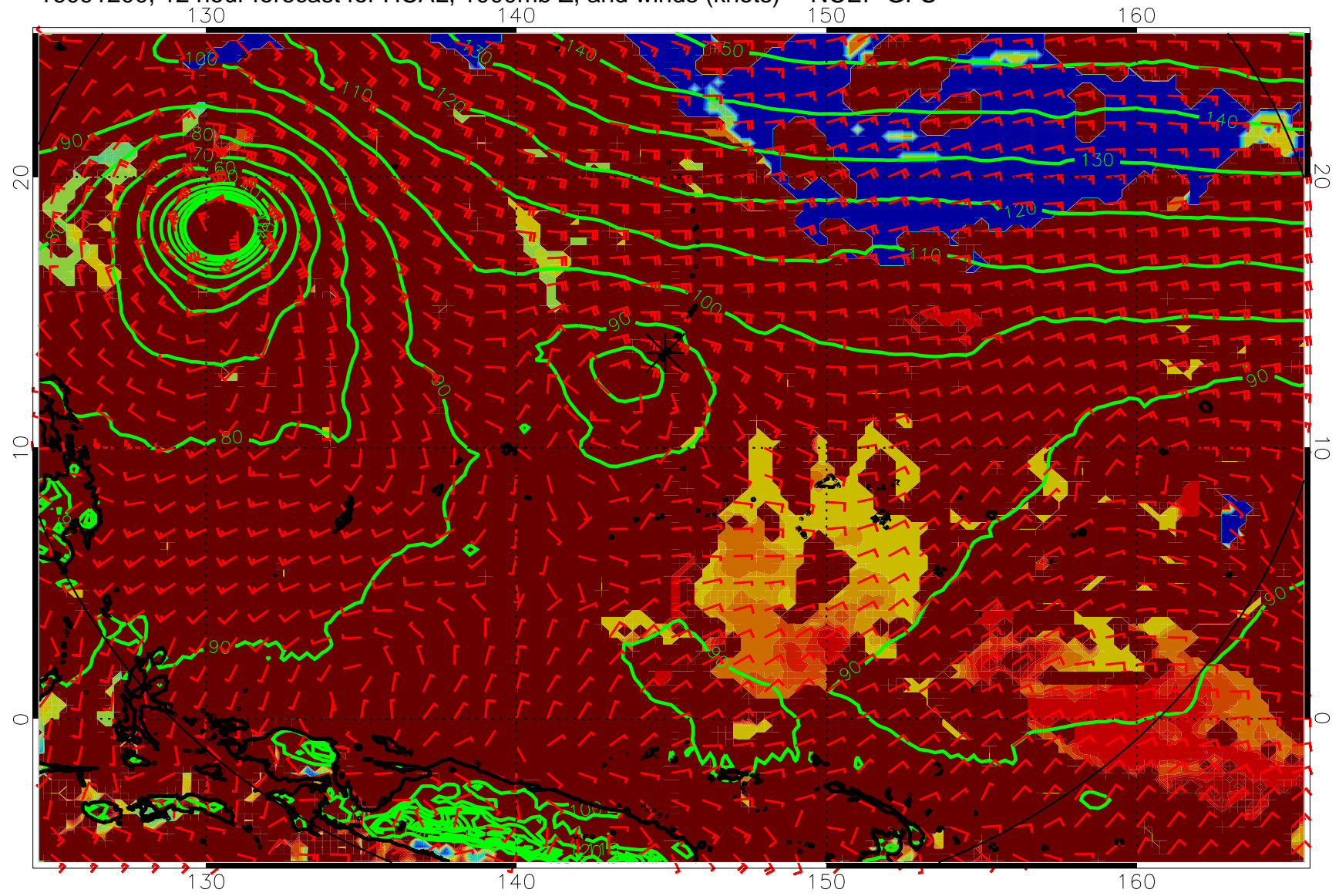
16091200, 12 hour forecast for HCAL, 1000mb Z, and winds (knots) -- NCEP GFS
