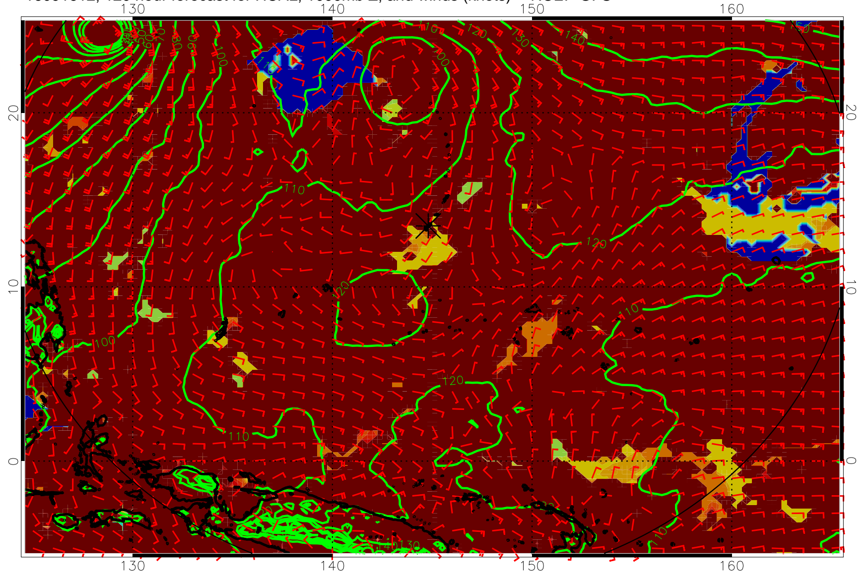
16091612, 120 hour forecast for HCAL, 1000mb Z, and winds (knots) -- NCEP GFS
