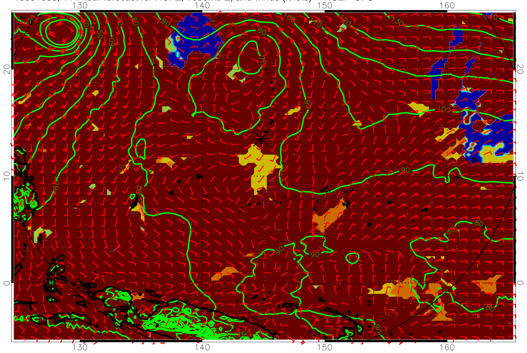
16091606, 114 hour forecast for HCAL, 1000mb Z, and winds (knots) -- NCEP GFS
