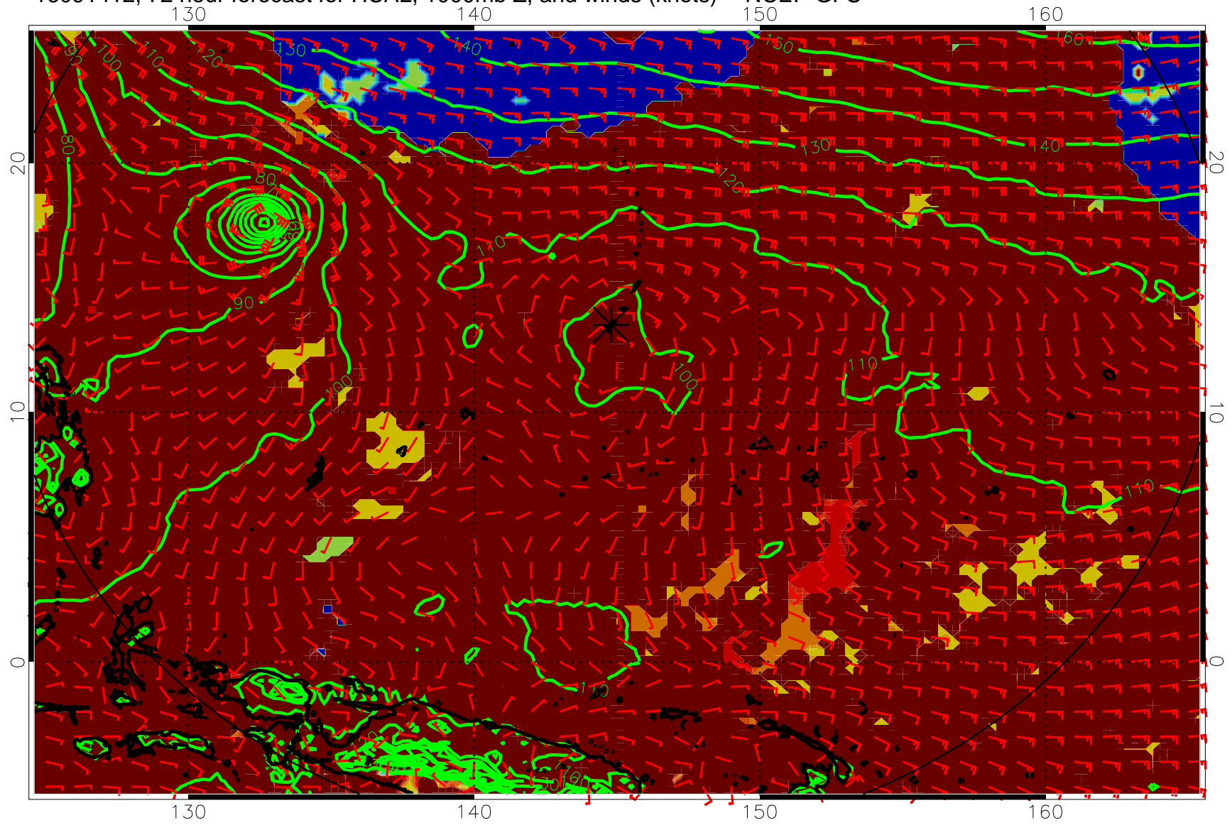
16091412, 72 hour forecast for HCAL, 1000mb Z, and winds (knots) -- NCEP GFS
