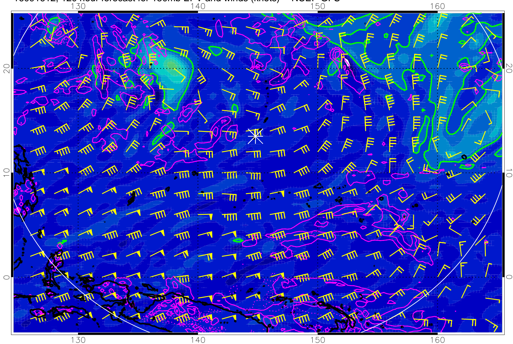
16091612, 120 hour forecast for 150mb EPV and winds (knots) -- NCEP GFS
