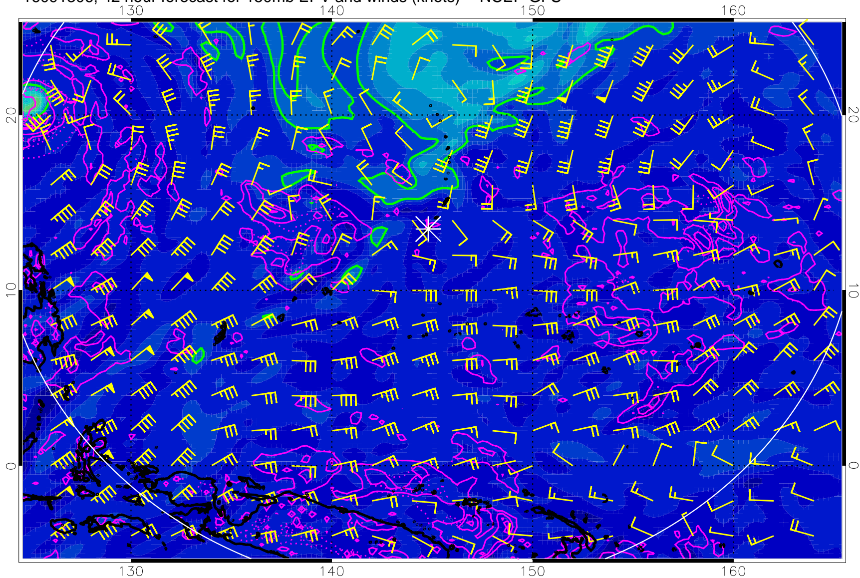
16091306, 42 hour forecast for 150mb EPV and winds (knots) -- NCEP GFS
