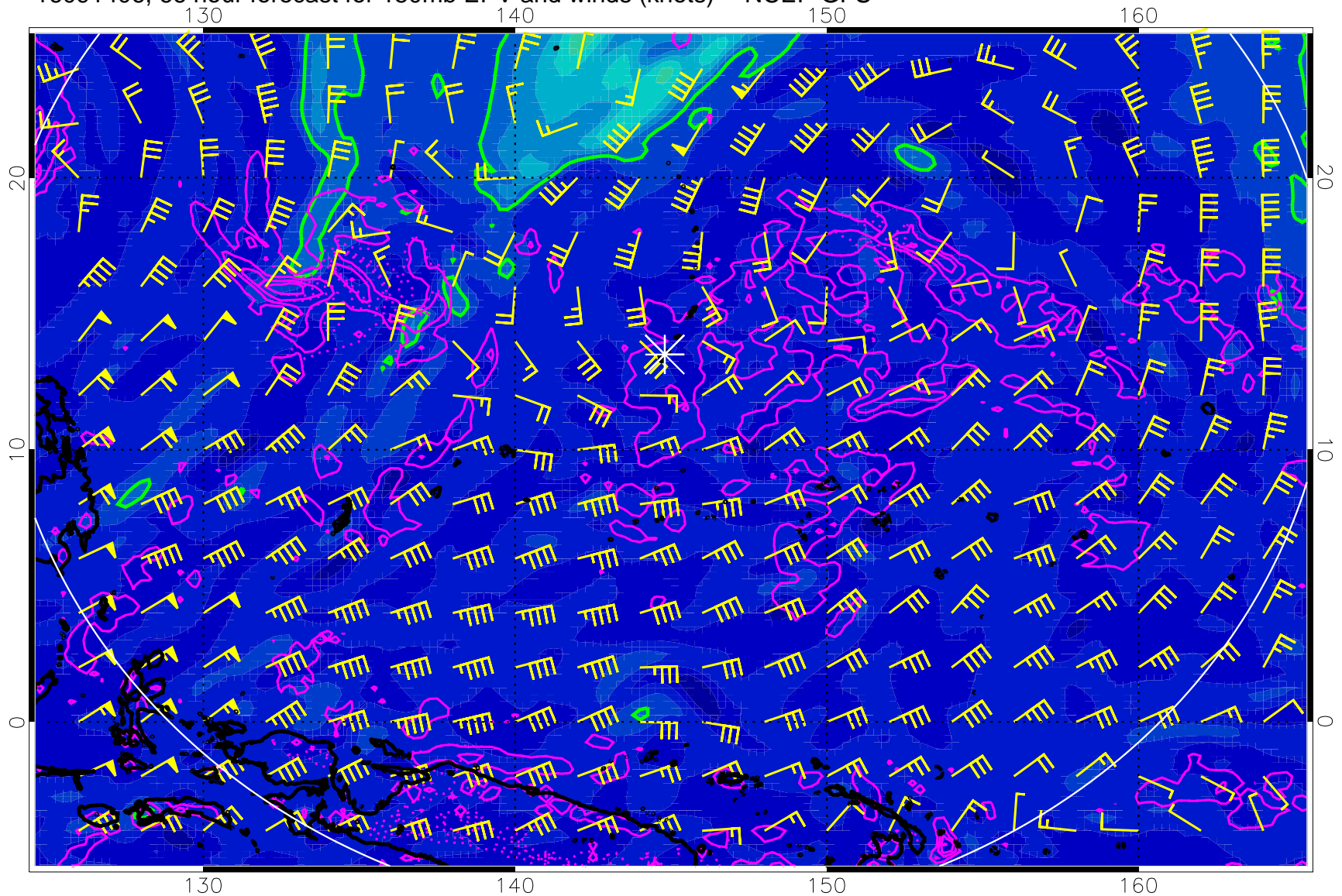
16091406, 66 hour forecast for 150mb EPV and winds (knots) -- NCEP GFS
