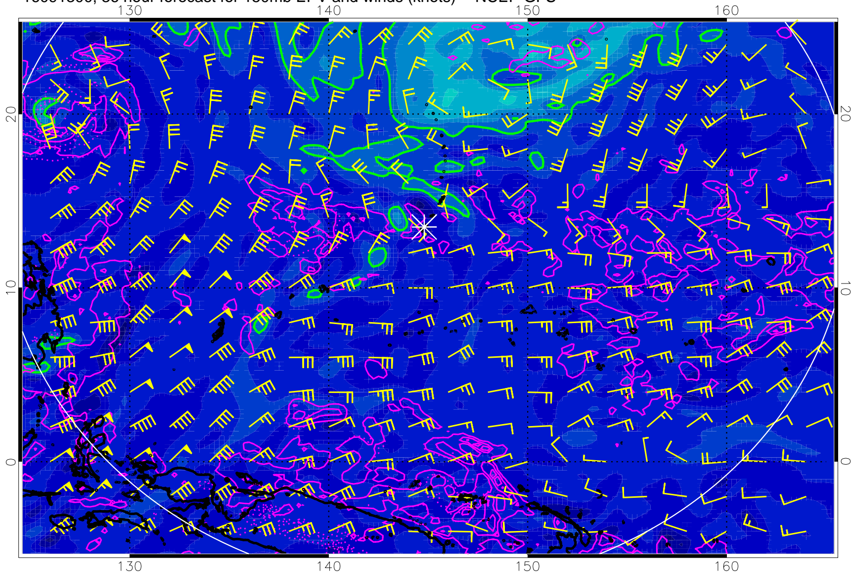
16091300, 36 hour forecast for 150mb EPV and winds (knots) -- NCEP GFS
