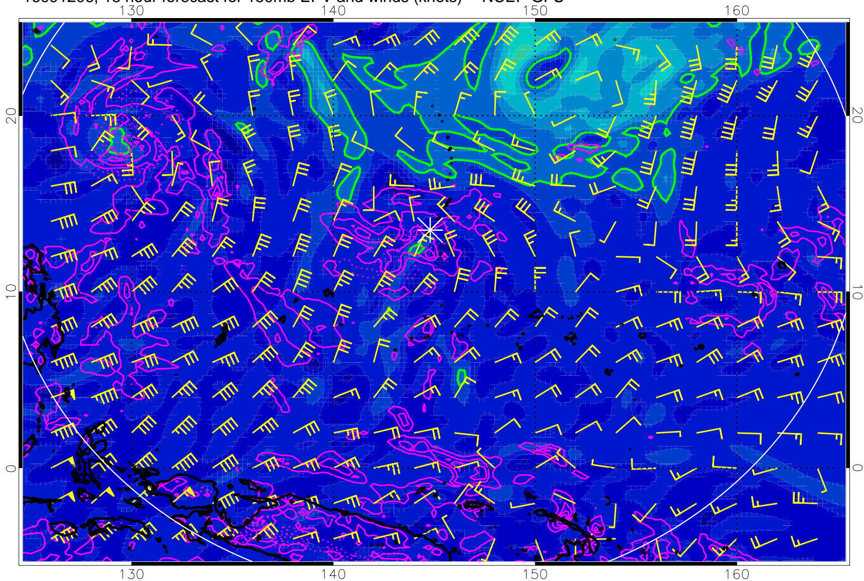
16091206, 18 hour forecast for 150mb EPV and winds (knots) -- NCEP GFS
