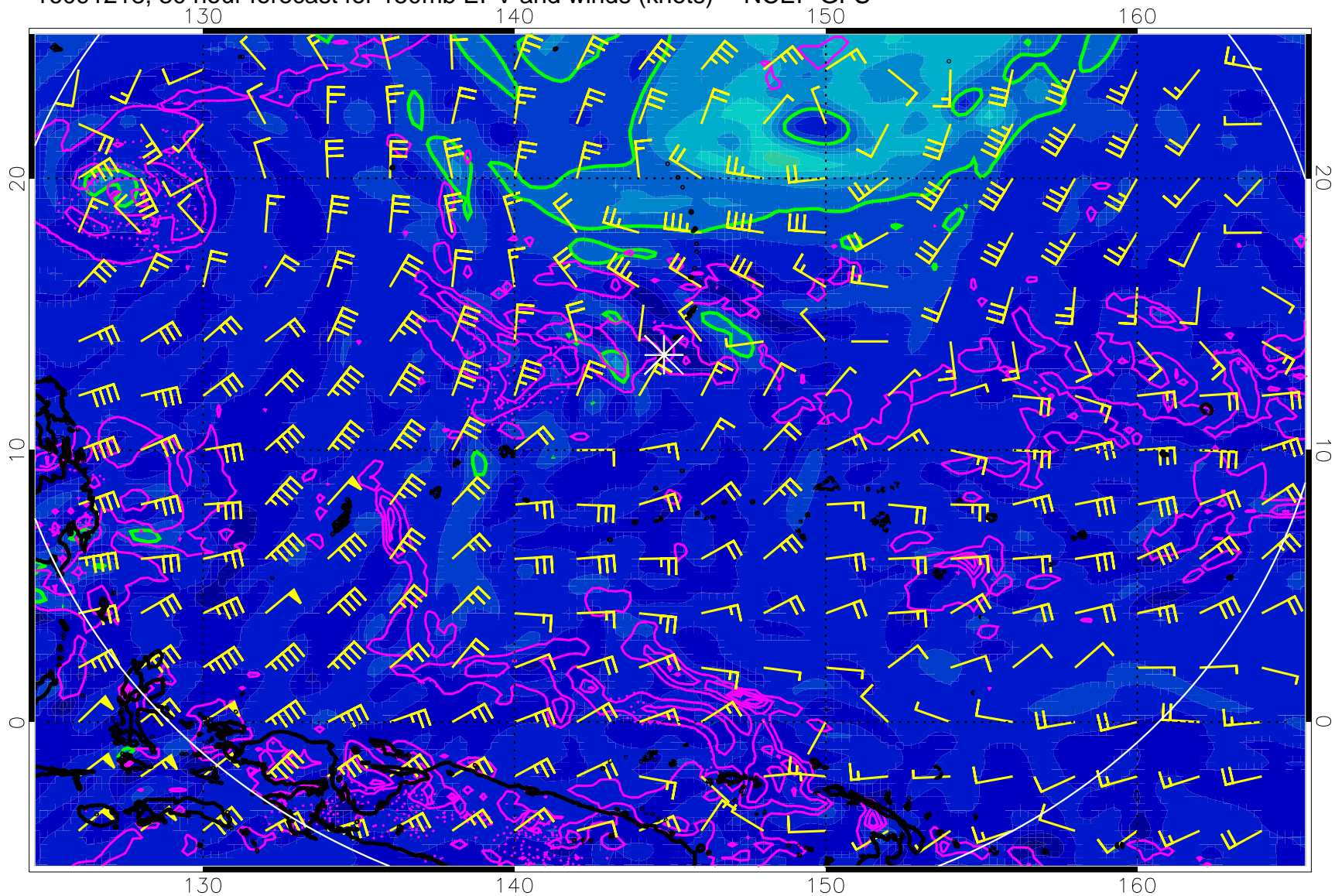
16091218, 30 hour forecast for 150mb EPV and winds (knots) -- NCEP GFS
