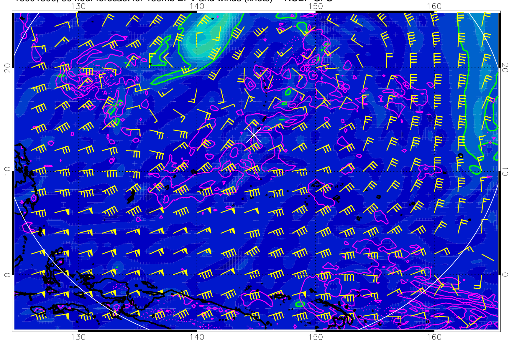
16091506, 90 hour forecast for 150mb EPV and winds (knots) -- NCEP GFS
