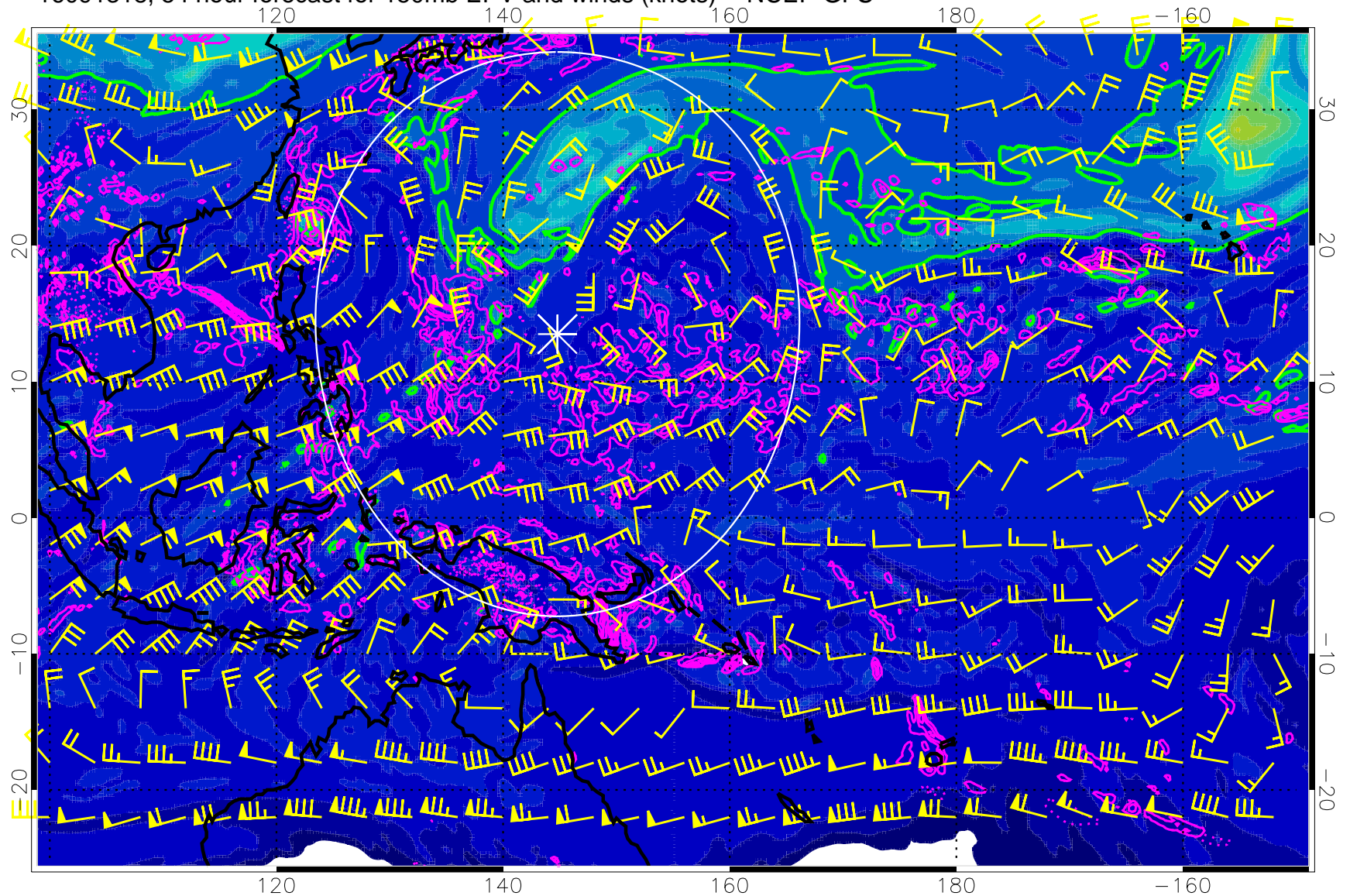
16091318, 54 hour forecast for 150mb EPV and winds (knots) -- NCEP GFS
