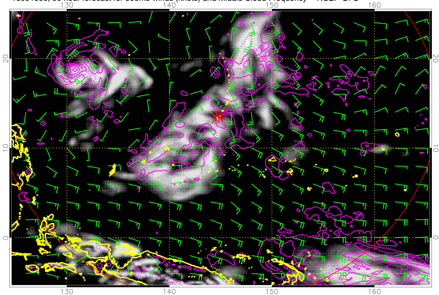
16091506, 90 hour forecast for 500mb winds (knots) and Middle Cloud Frequency -- NCEP GFS
