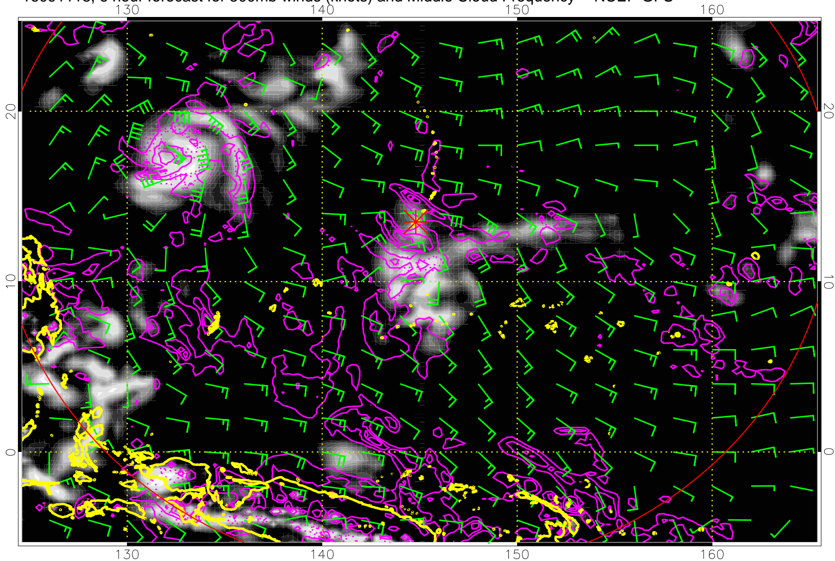
16091118, 6 hour forecast for 500mb winds (knots) and Middle Cloud Frequency -- NCEP GFS
