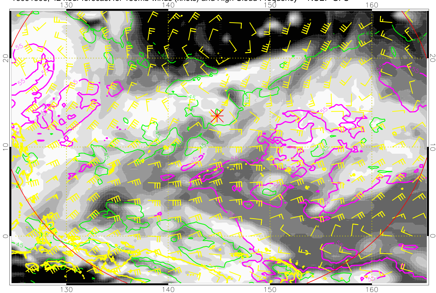
16091306, 42 hour forecast for 150mb winds (knots) and High Cloud Frequency -- NCEP GFS
