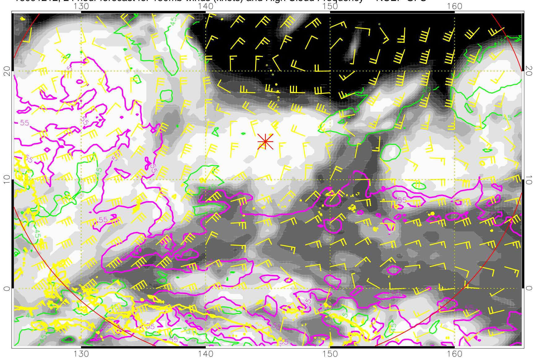
16091212, 24 hour forecast for 150mb winds (knots) and High Cloud Frequency -- NCEP GFS
