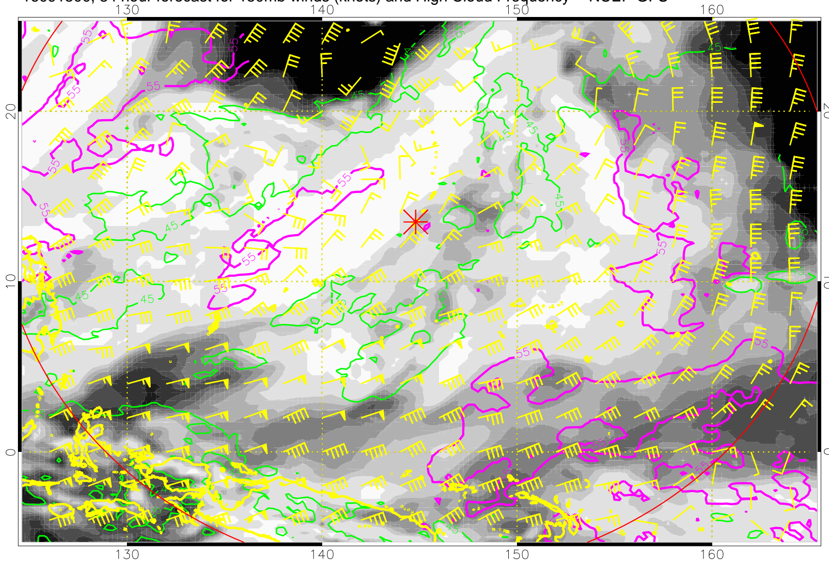
16091500, 84 hour forecast for 150mb winds (knots) and High Cloud Frequency -- NCEP GFS
