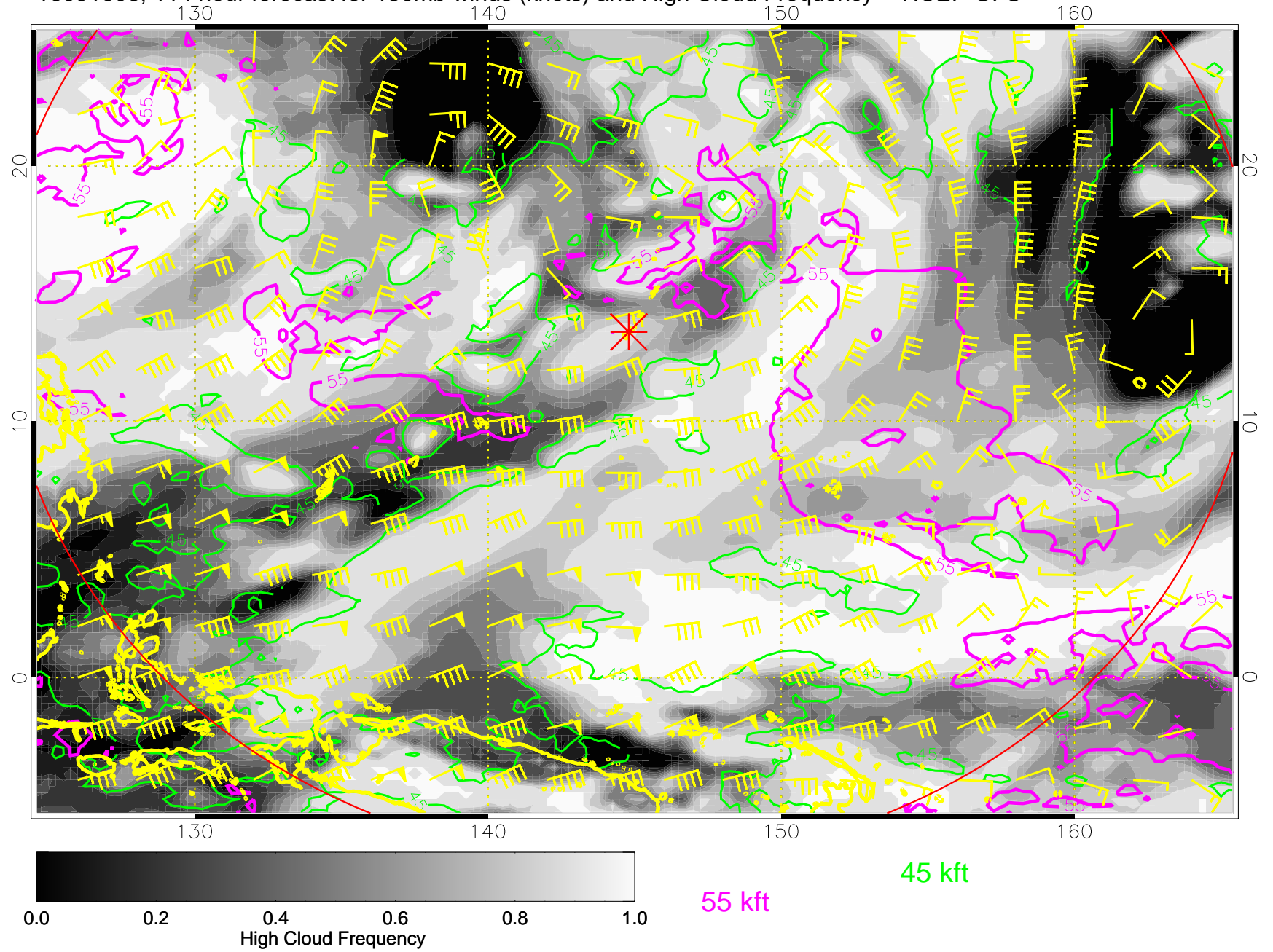
16091606, 114 hour forecast for 150mb winds (knots) and High Cloud Frequency -- NCEP GFS
