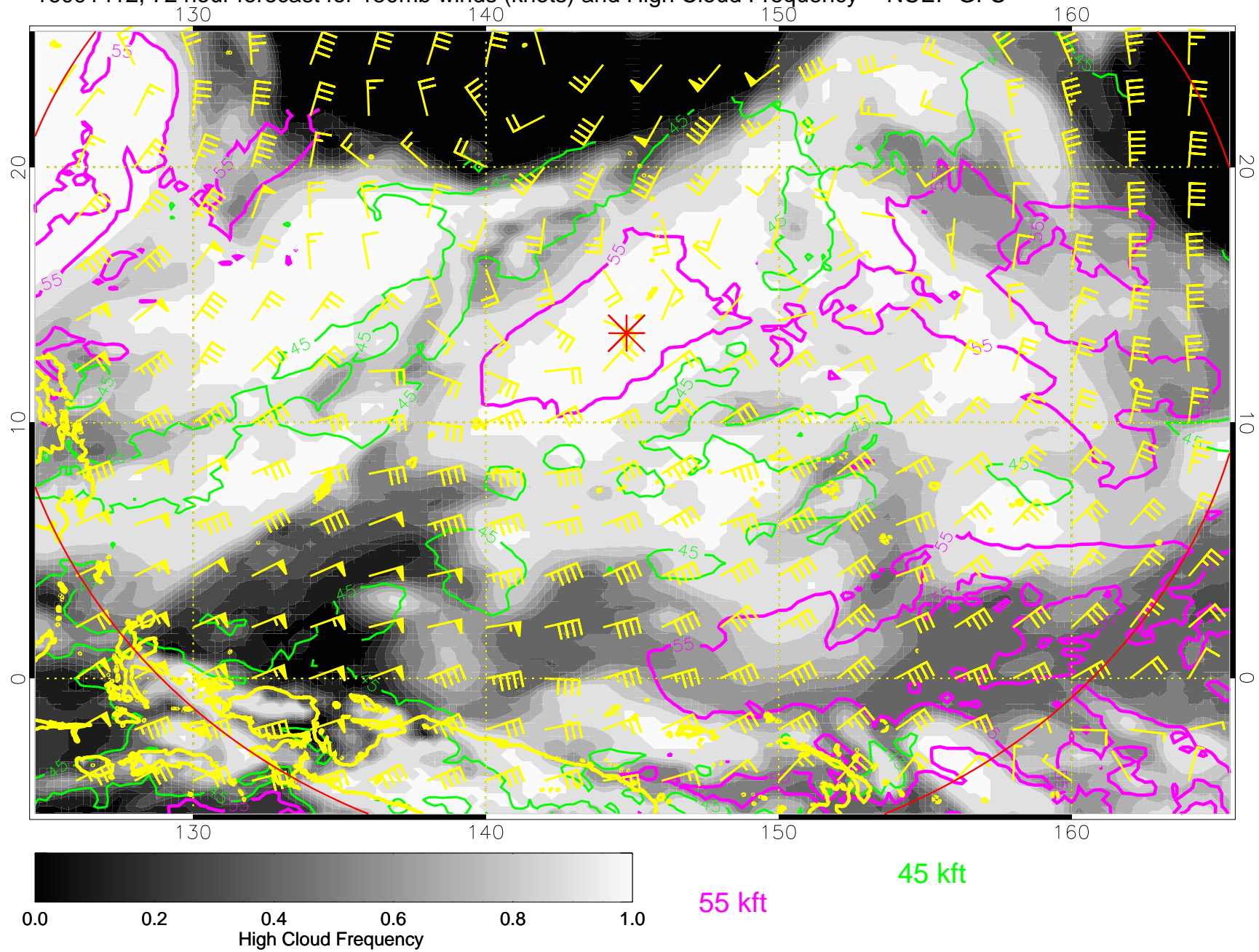
16091412, 72 hour forecast for 150mb winds (knots) and High Cloud Frequency -- NCEP GFS
