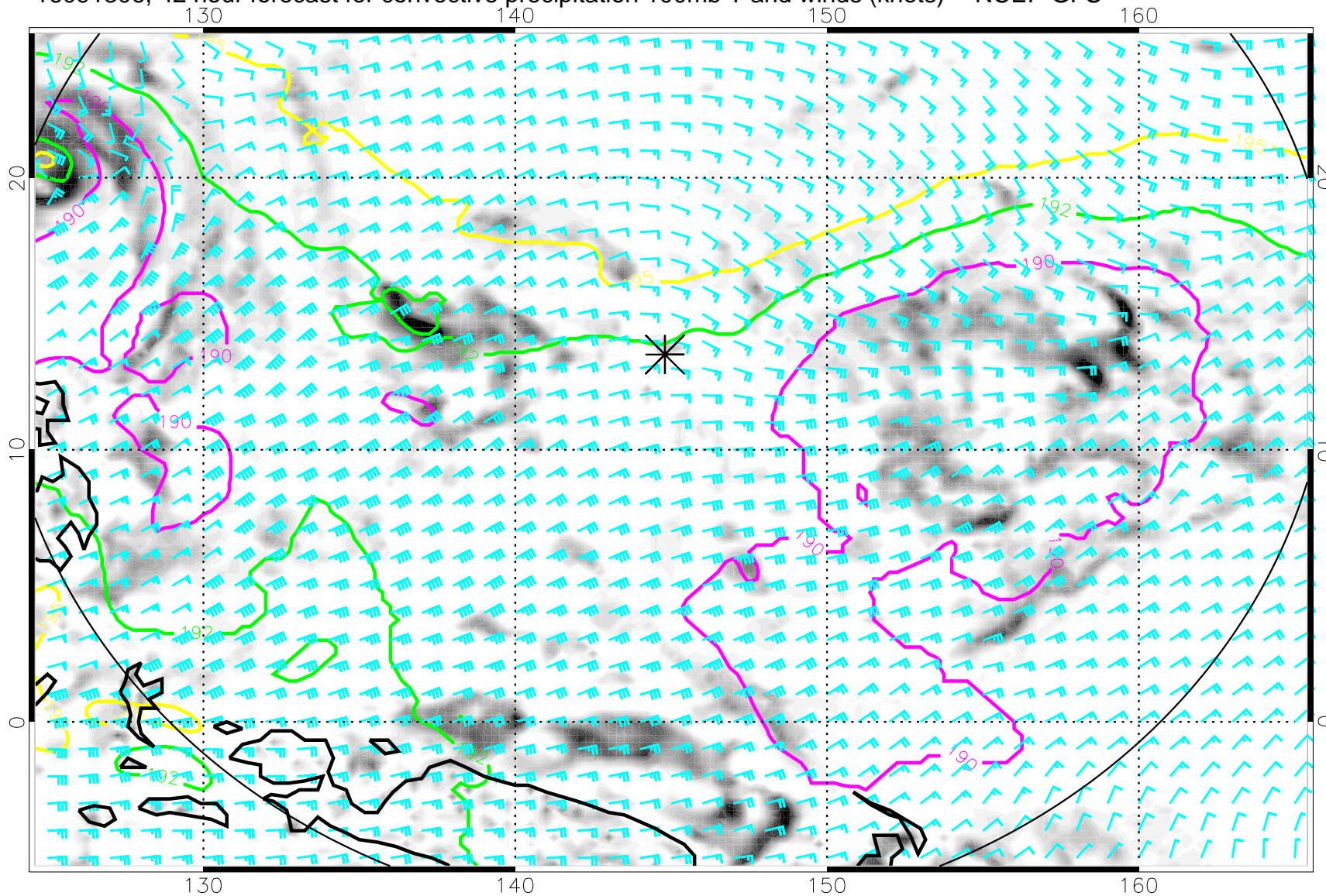
16091306, 42 hour forecast for convective precipitation 100mb T and winds (knots) -- NCEP GFS
