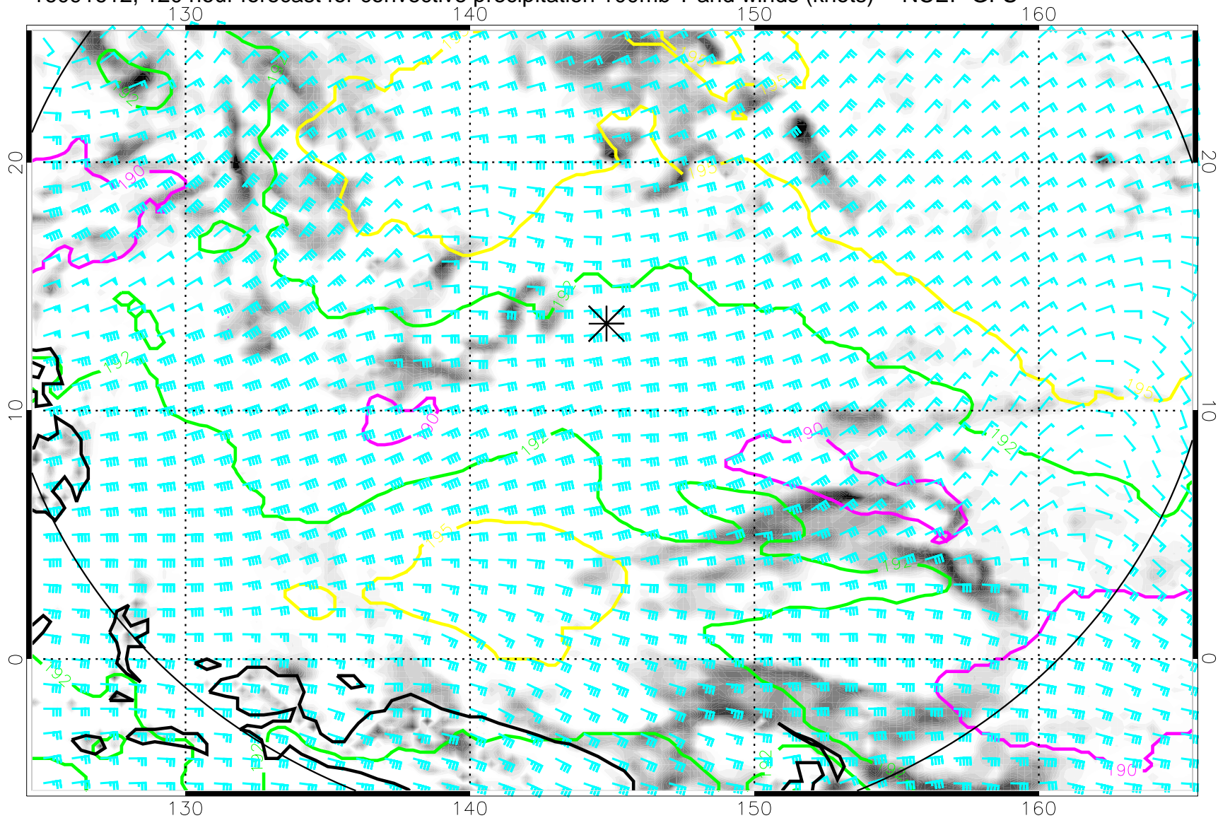
16091612, 120 hour forecast for convective precipitation 100mb T and winds (knots) -- NCEP GFS
