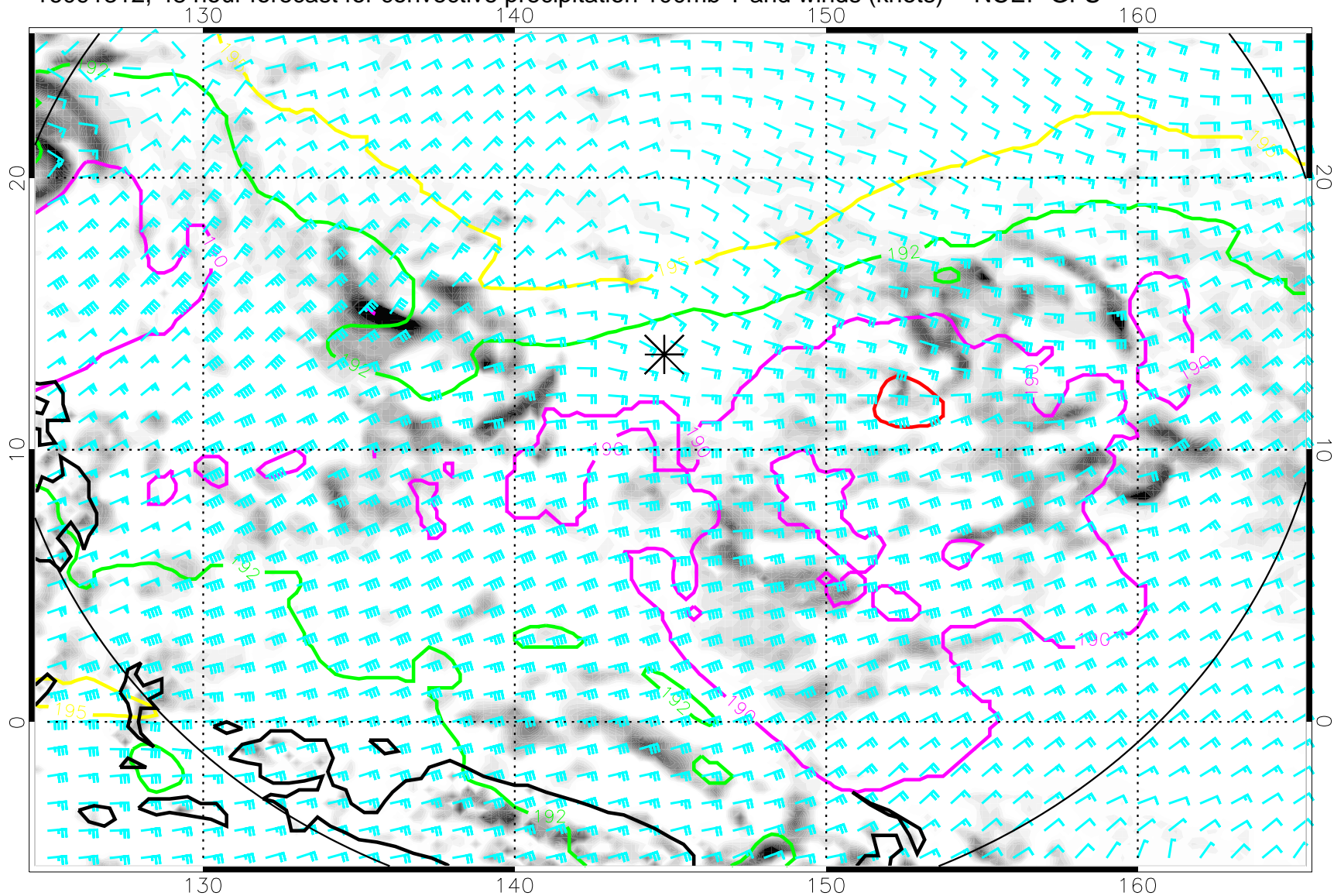
16091312, 48 hour forecast for convective precipitation 100mb T and winds (knots) -- NCEP GFS
