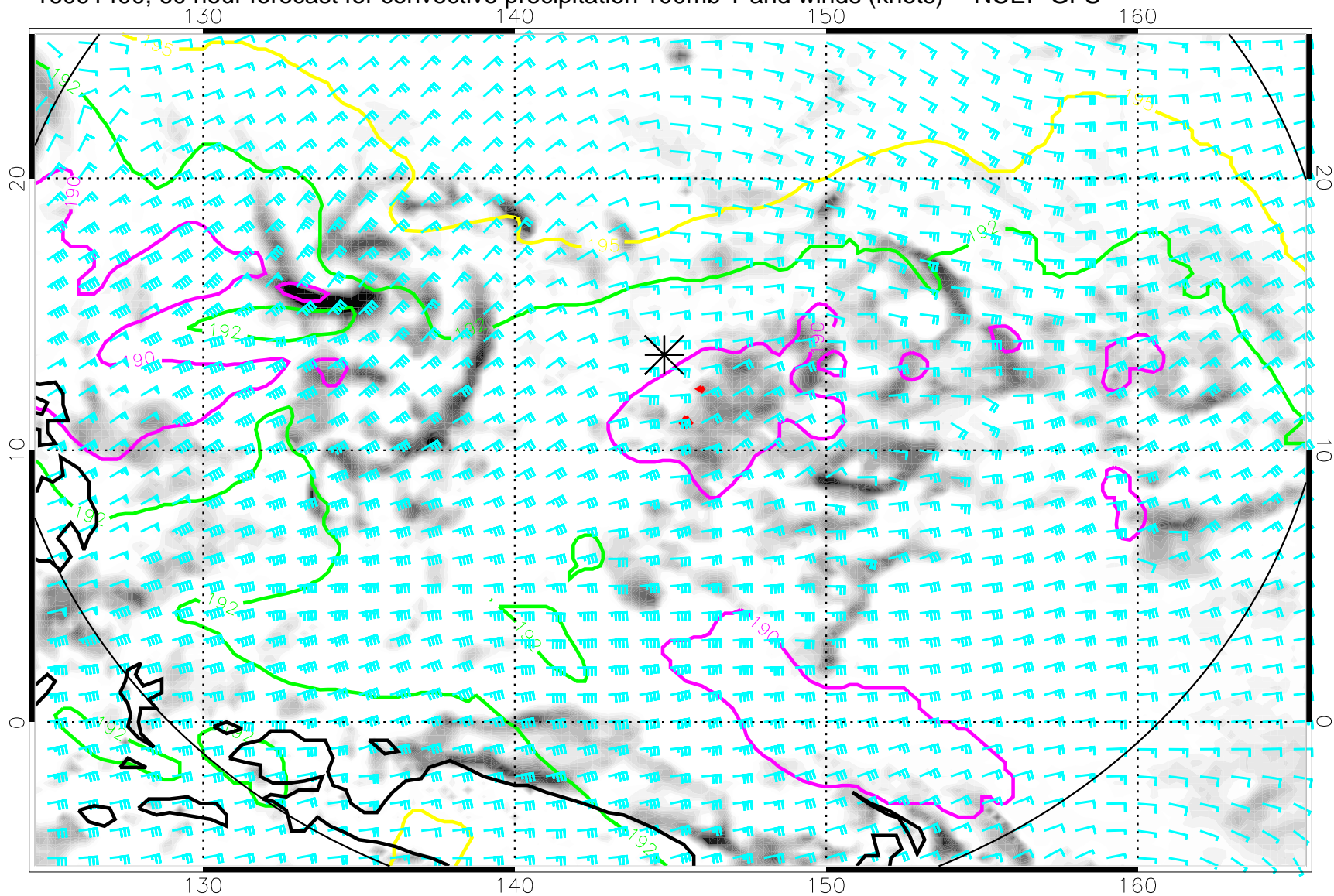
16091400, 60 hour forecast for convective precipitation 100mb T and winds (knots) -- NCEP GFS
