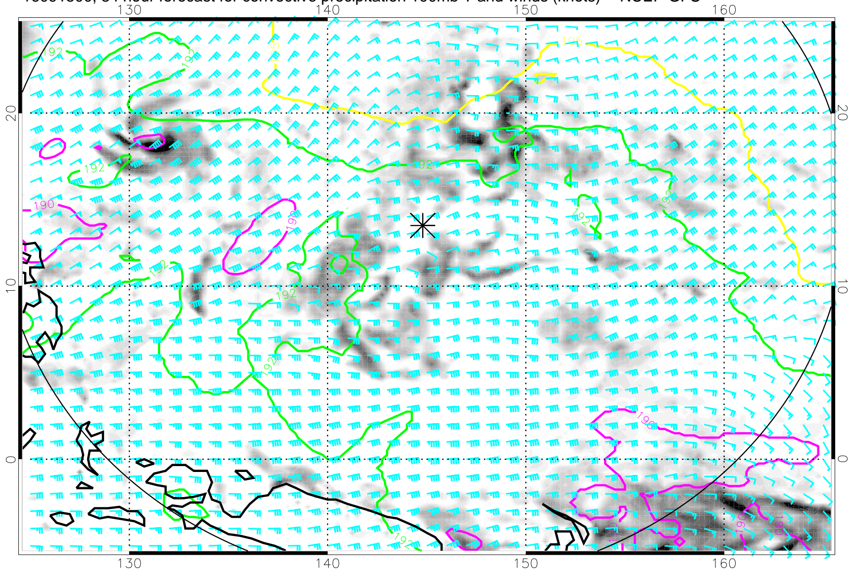
16091500, 84 hour forecast for convective precipitation 100mb T and winds (knots) -- NCEP GFS
