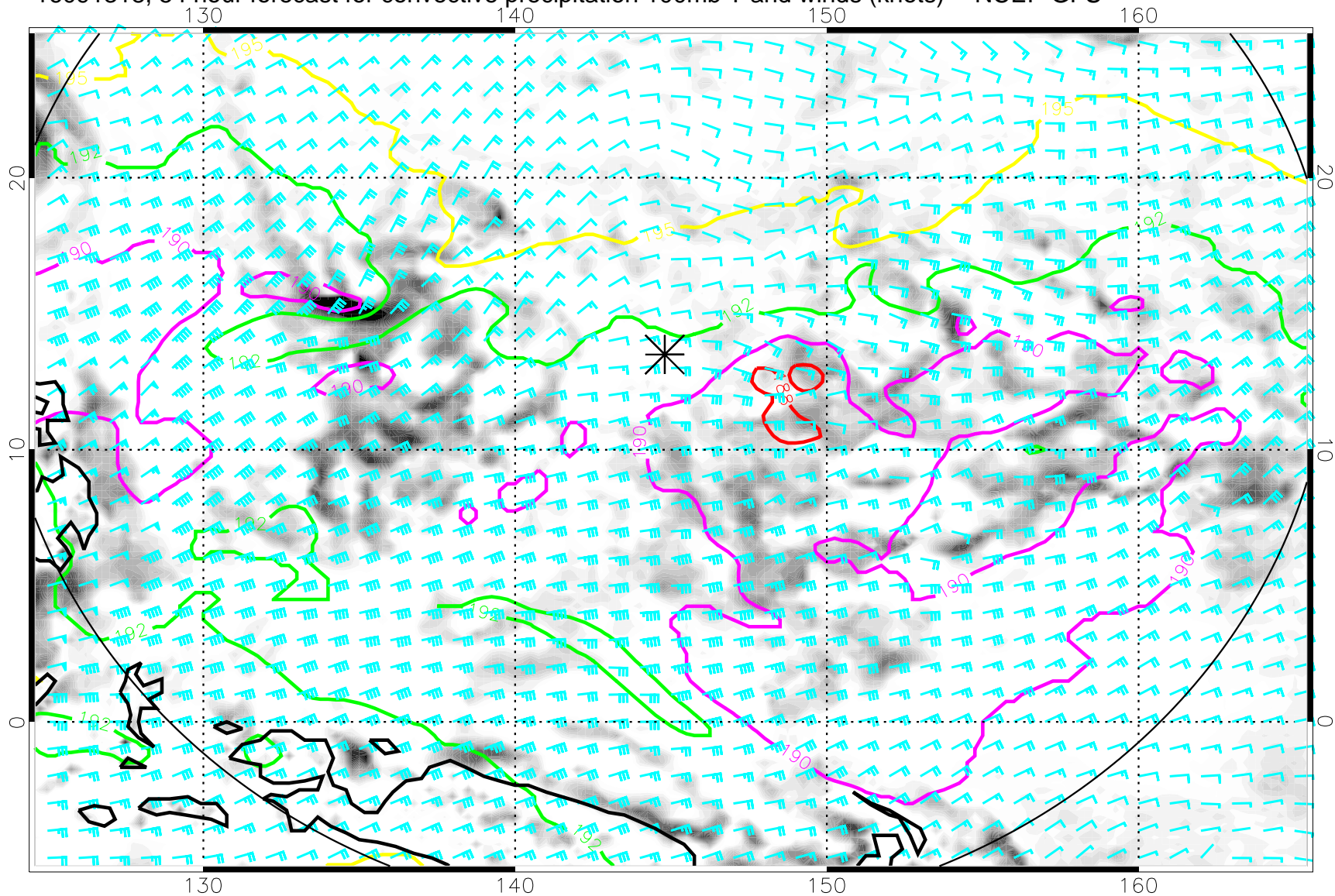
16091318, 54 hour forecast for convective precipitation 100mb T and winds (knots) -- NCEP GFS
