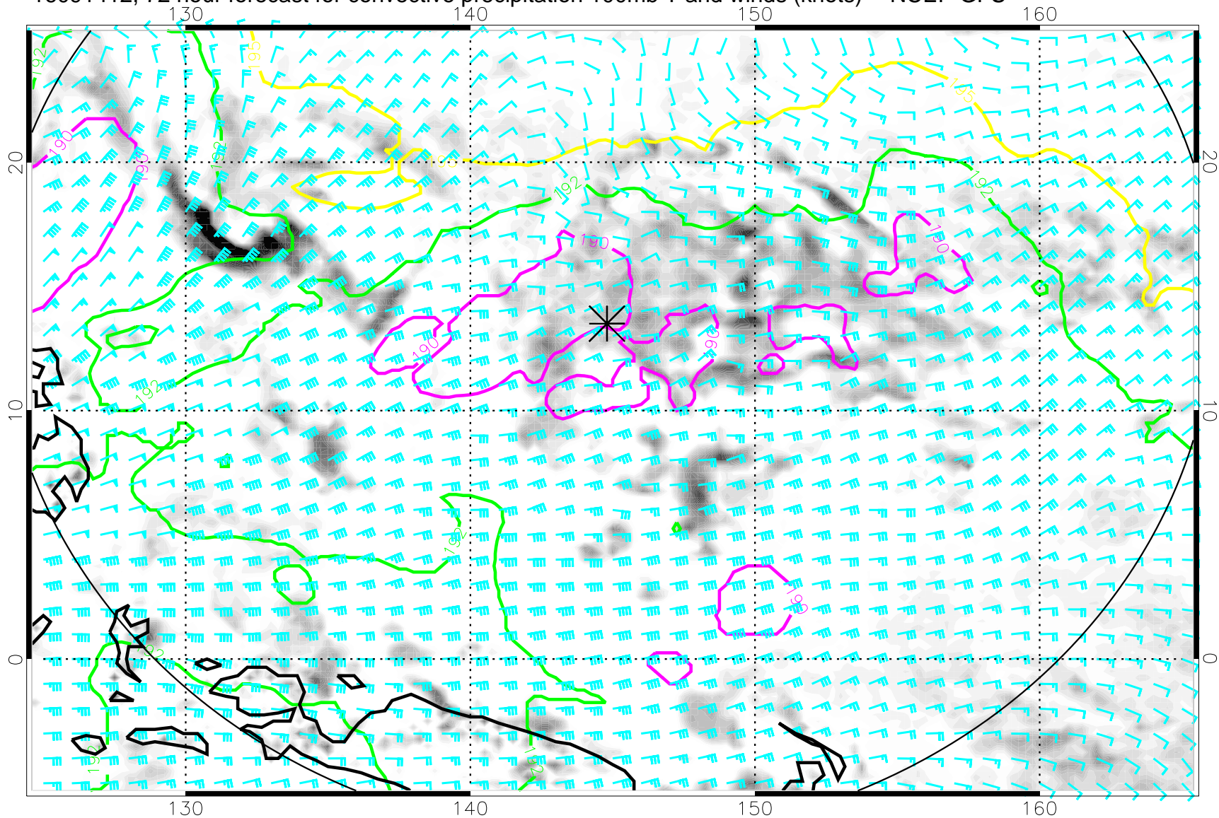
16091412, 72 hour forecast for convective precipitation 100mb T and winds (knots) -- NCEP GFS
