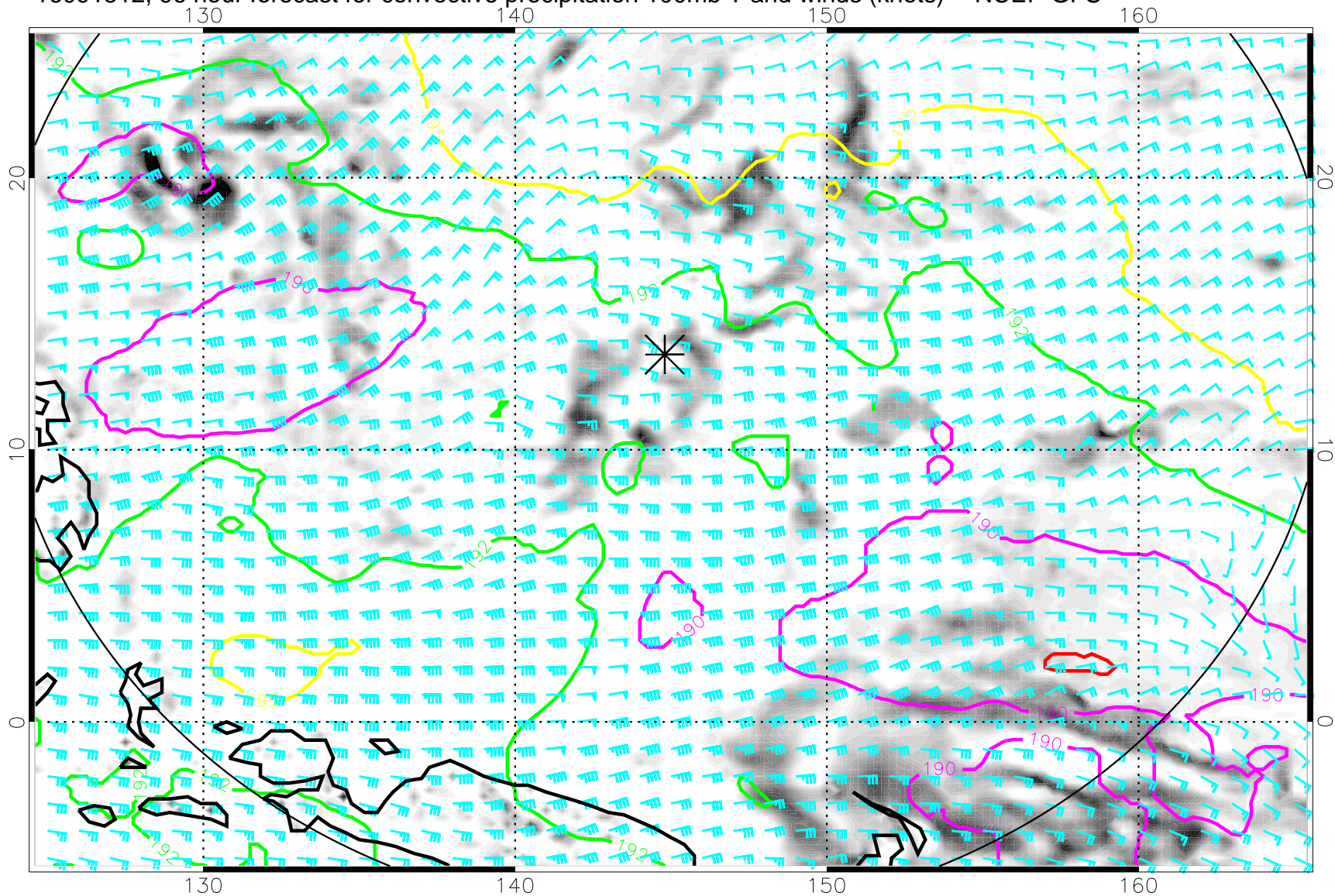
16091512, 96 hour forecast for convective precipitation 100mb T and winds (knots) -- NCEP GFS
