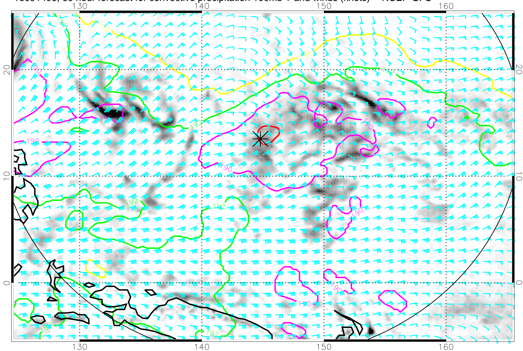
16091406, 66 hour forecast for convective precipitation 100mb T and winds (knots) -- NCEP GFS
