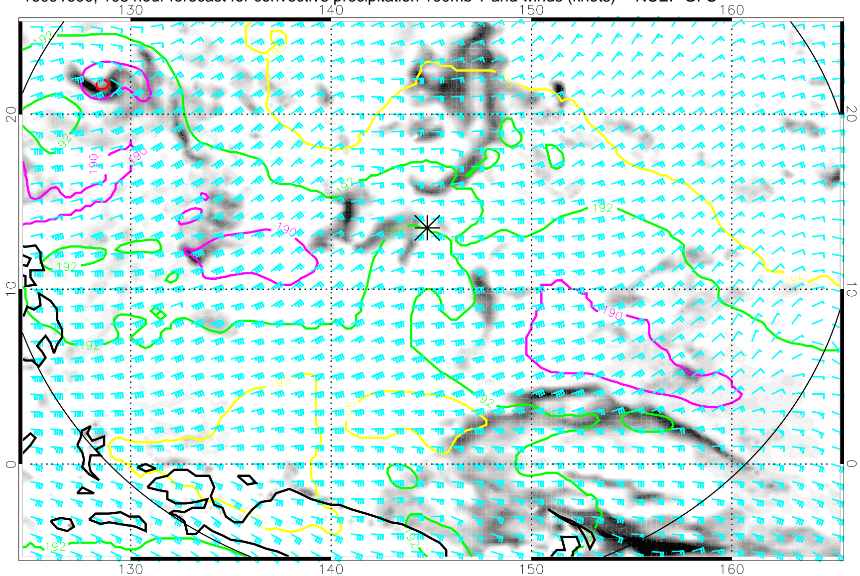
16091600, 108 hour forecast for convective precipitation 100mb T and winds (knots) -- NCEP GFS
