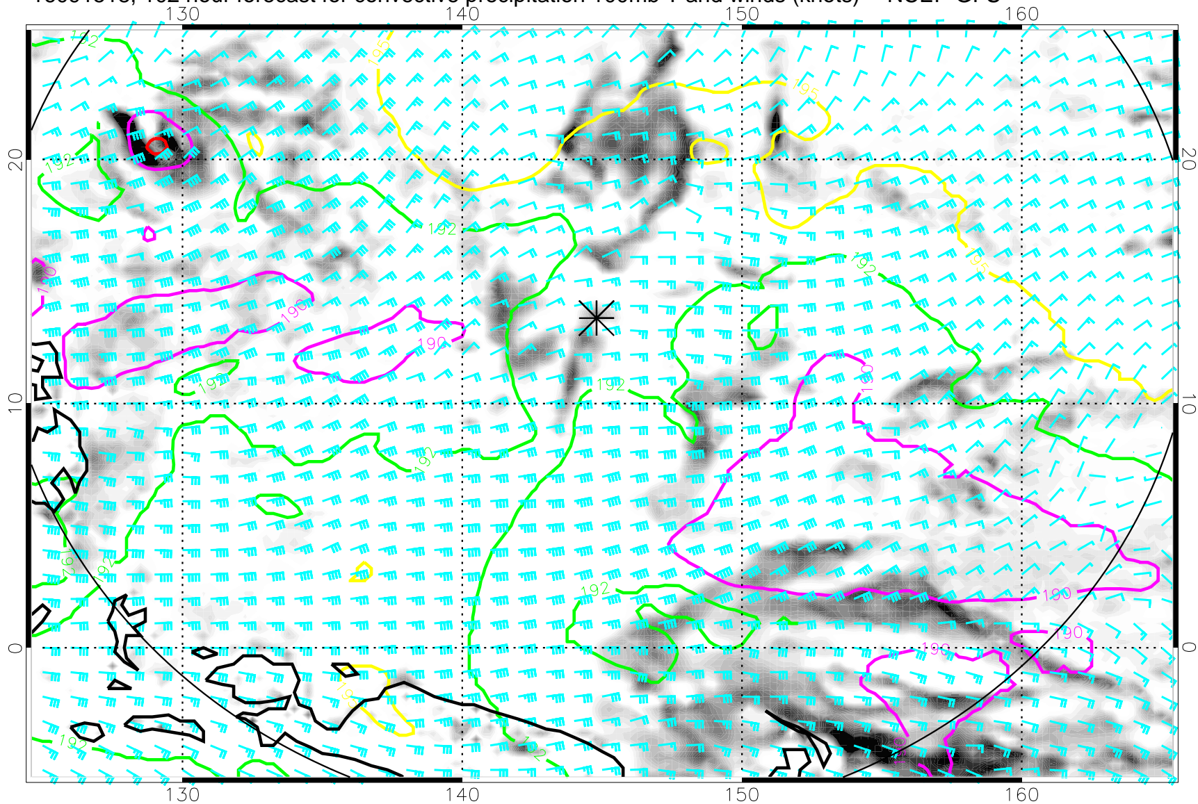
16091518, 102 hour forecast for convective precipitation 100mb T and winds (knots) -- NCEP GFS
