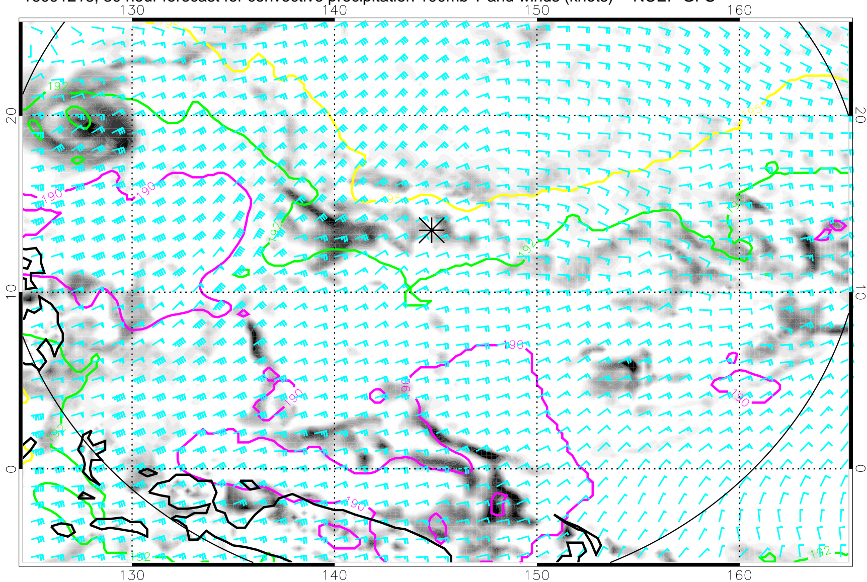
16091218, 30 hour forecast for convective precipitation 100mb T and winds (knots) -- NCEP GFS
