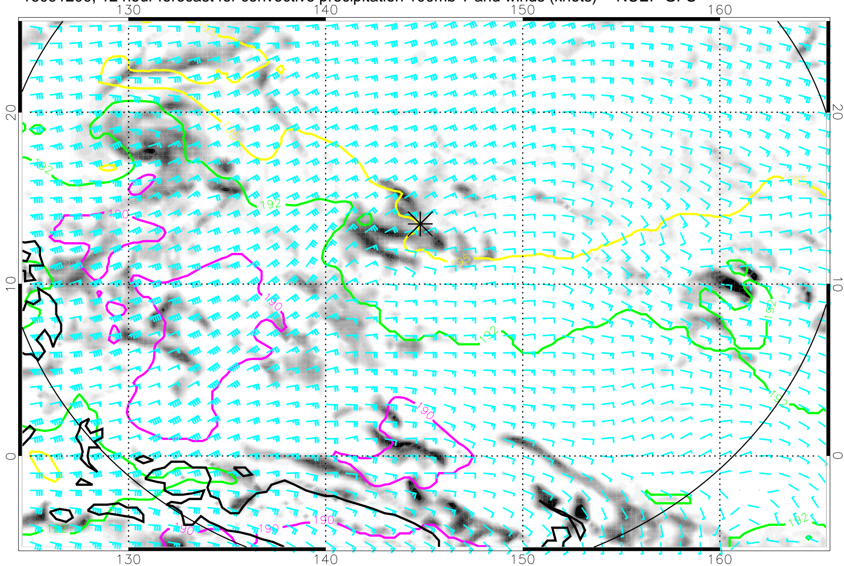
16091200, 12 hour forecast for convective precipitation 100mb T and winds (knots) -- NCEP GFS
