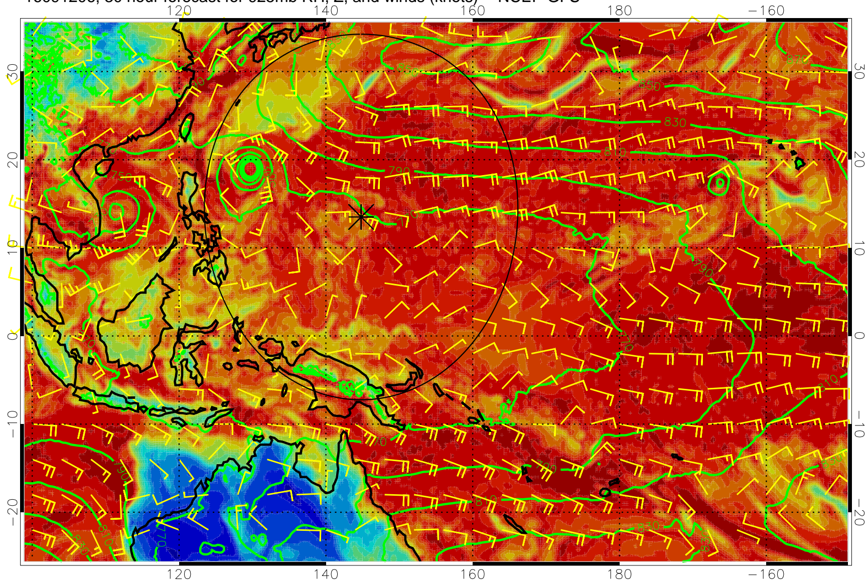
16091206, 30 hour forecast for 925mb RH, Z, and winds (knots) -- NCEP GFS
