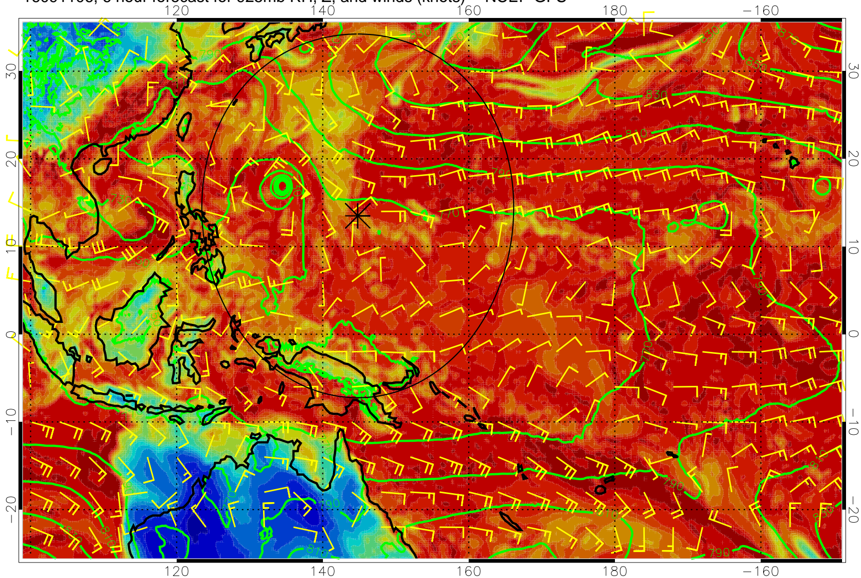
16091106, 6 hour forecast for 925mb RH, Z, and winds (knots) -- NCEP GFS
