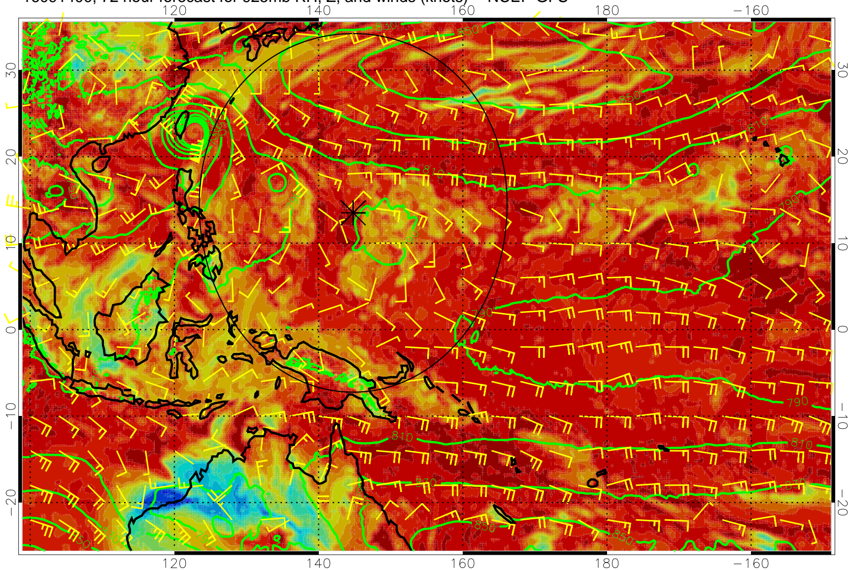
16091400, 72 hour forecast for 925mb RH, Z, and winds (knots) -- NCEP GFS
