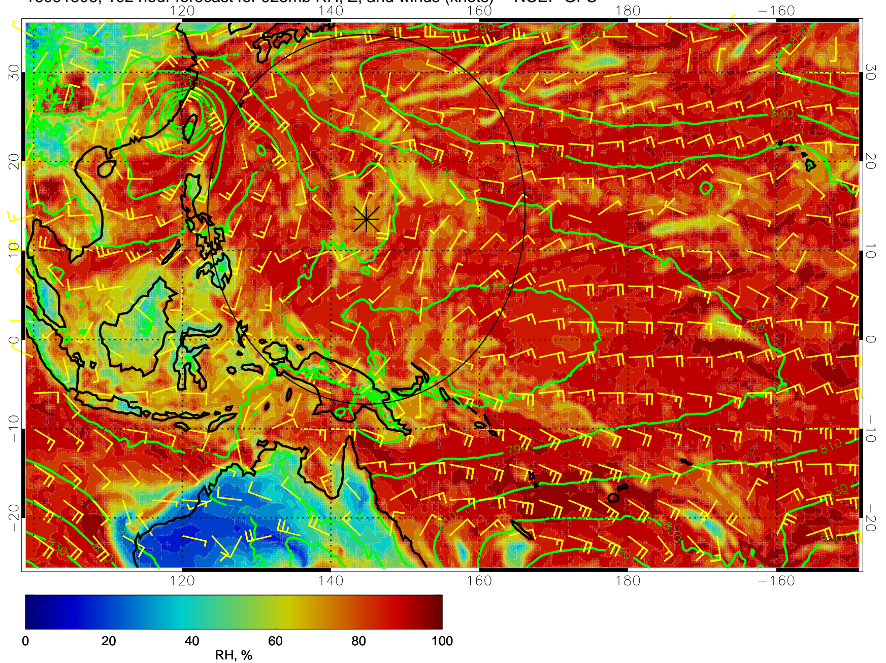
16091506, 102 hour forecast for 925mb RH, Z, and winds (knots) -- NCEP GFS
