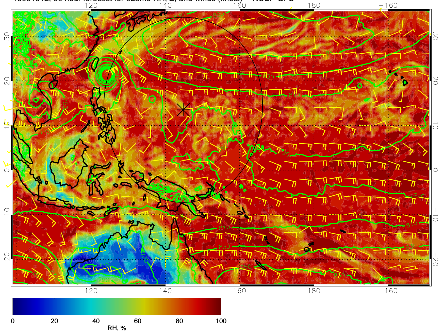
16091312, 60 hour forecast for 925mb RH, Z, and winds (knots) -- NCEP GFS
