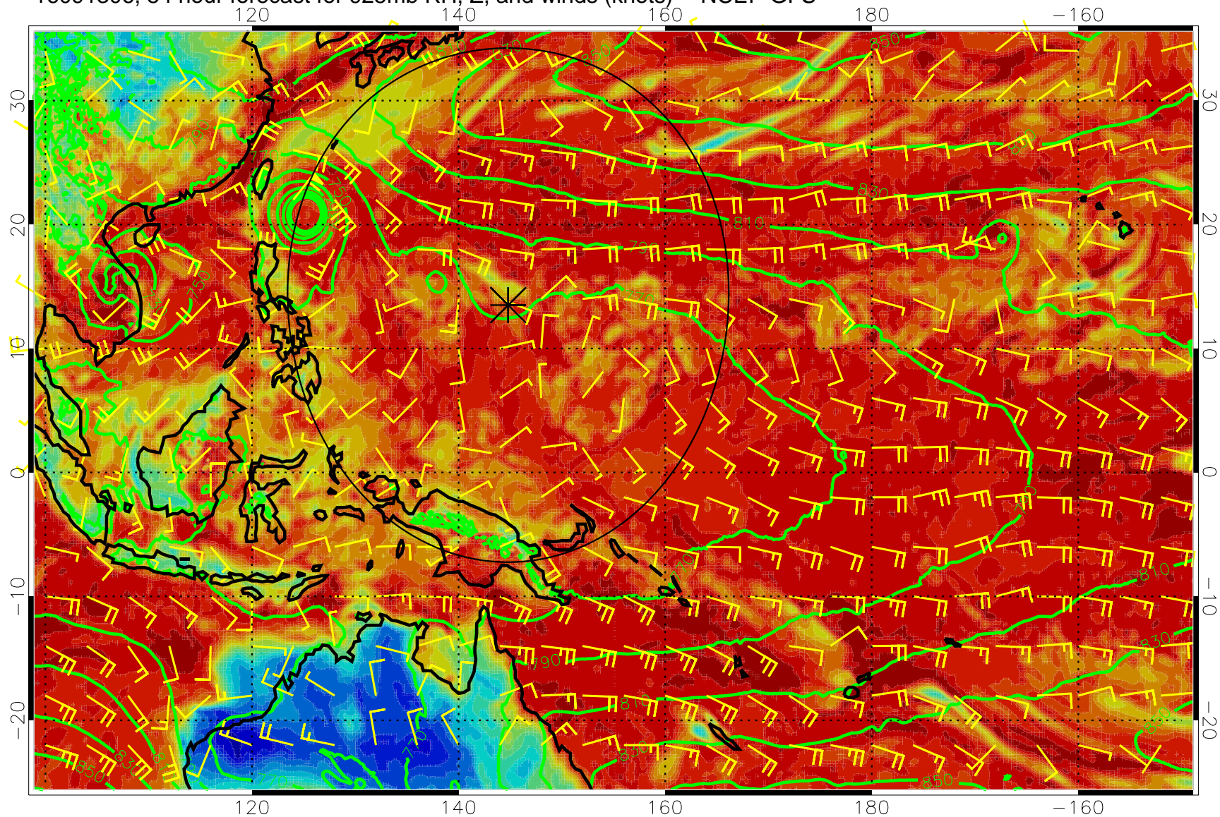
16091306, 54 hour forecast for 925mb RH, Z, and winds (knots) -- NCEP GFS
