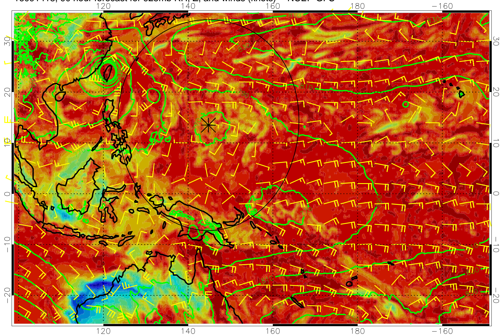
16091418, 90 hour forecast for 925mb RH, Z, and winds (knots) -- NCEP GFS
