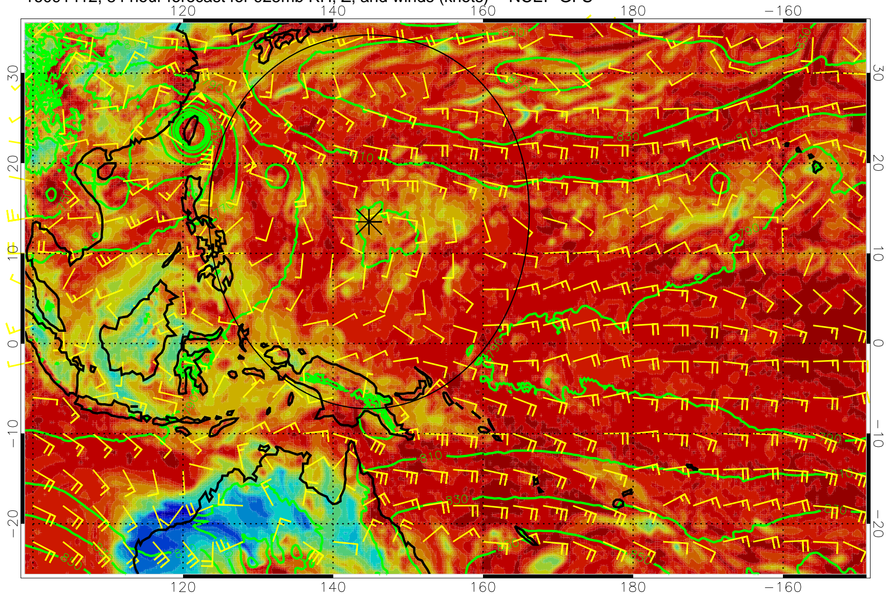
16091412, 84 hour forecast for 925mb RH, Z, and winds (knots) -- NCEP GFS
