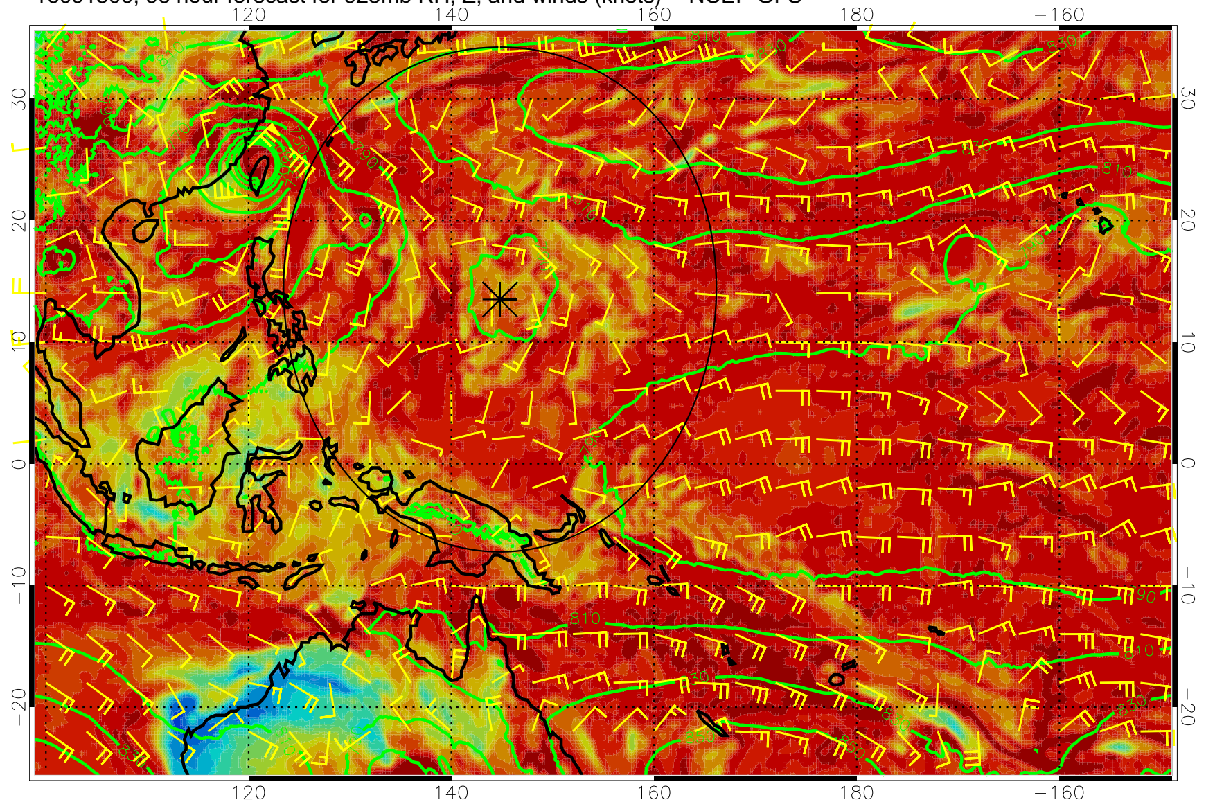
16091500, 96 hour forecast for 925mb RH, Z, and winds (knots) -- NCEP GFS
