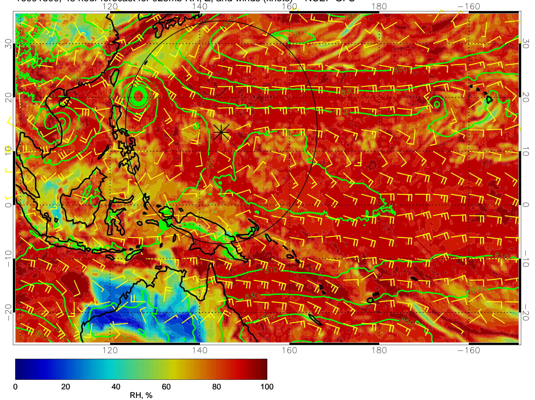
16091300, 48 hour forecast for 925mb RH, Z, and winds (knots) -- NCEP GFS
