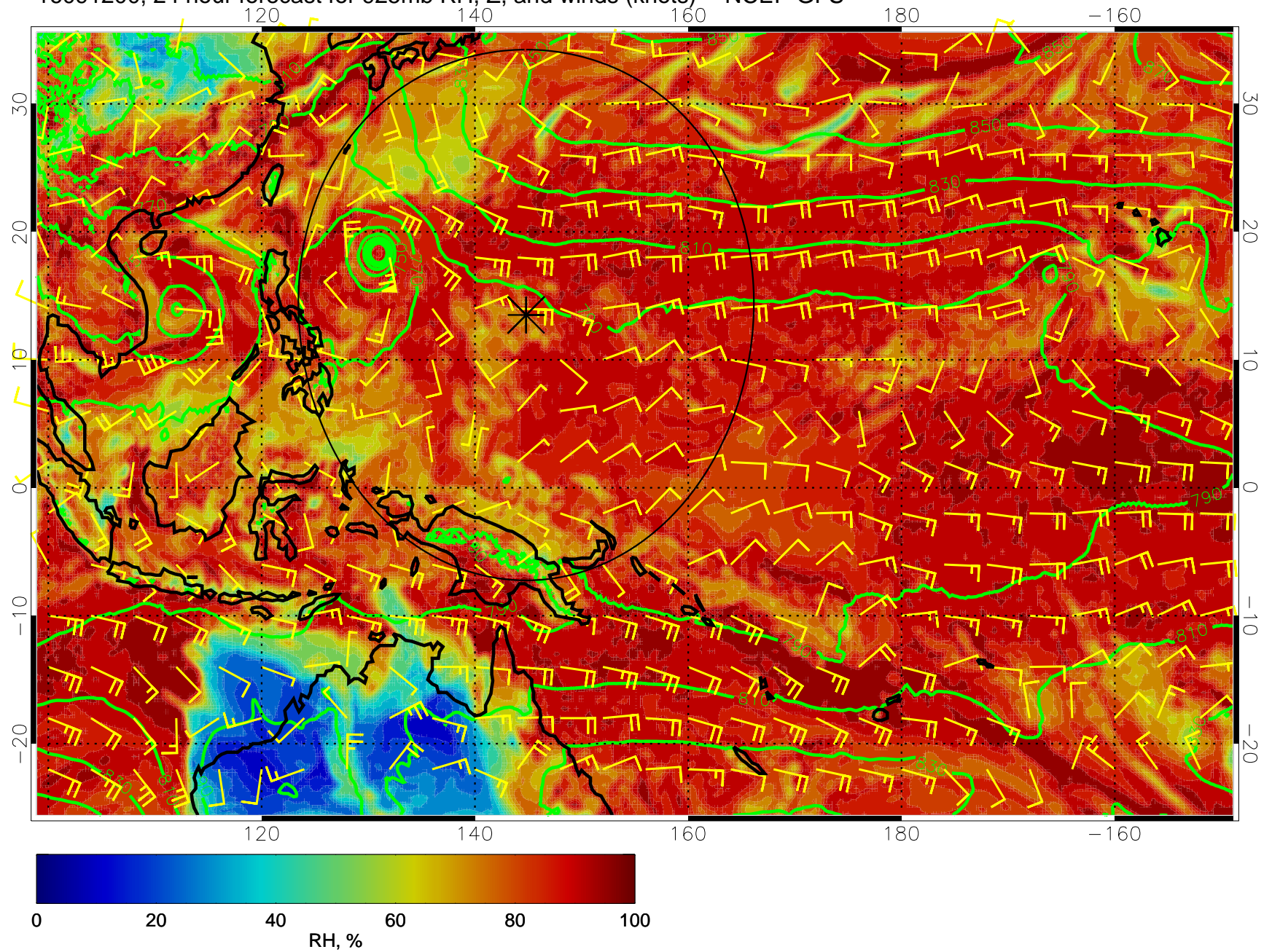
16091200, 24 hour forecast for 925mb RH, Z, and winds (knots) -- NCEP GFS
