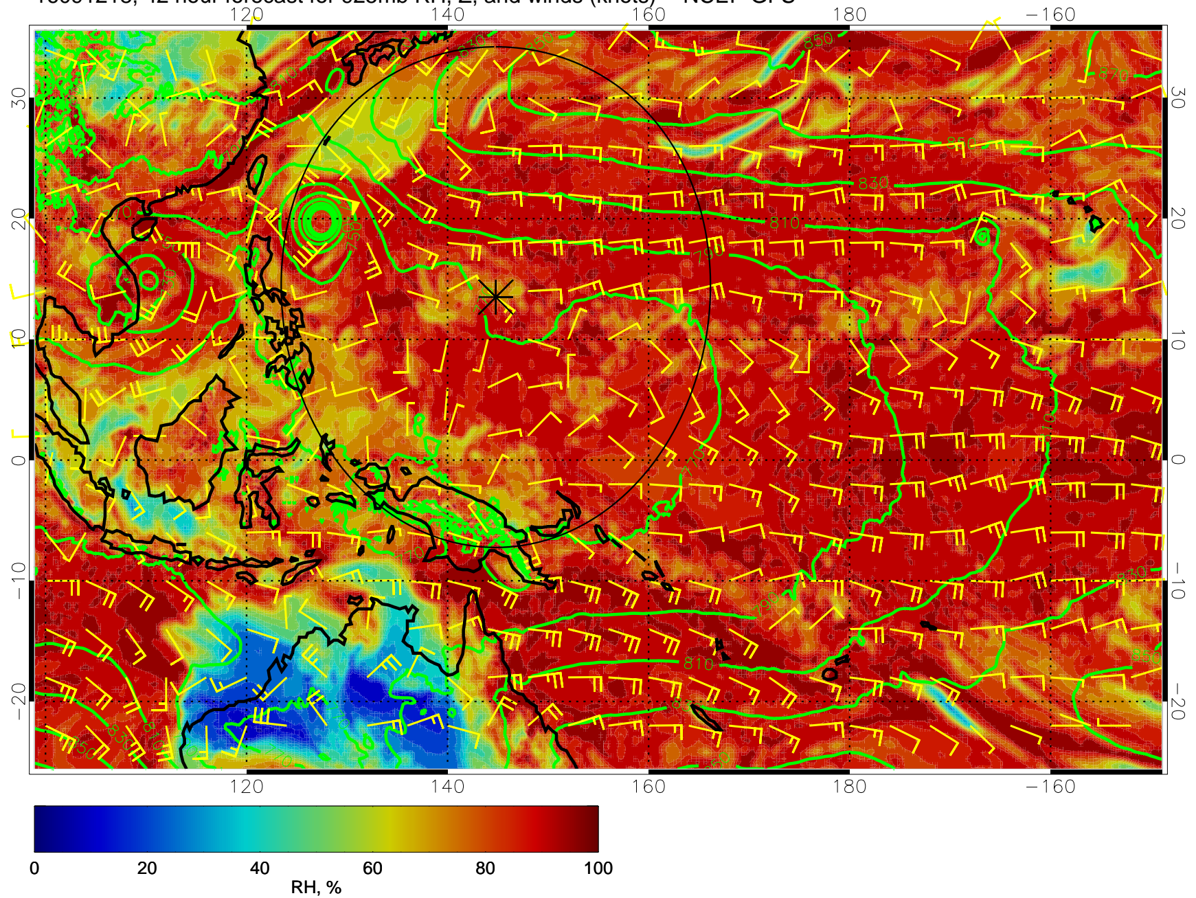
16091218, 42 hour forecast for 925mb RH, Z, and winds (knots) -- NCEP GFS
