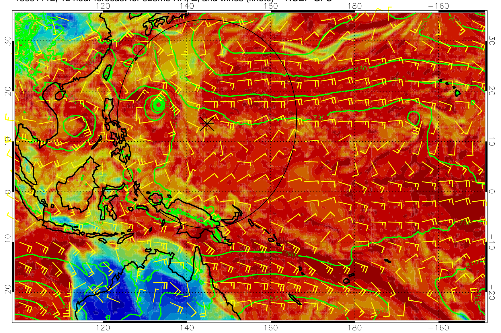
16091112, 12 hour forecast for 925mb RH, Z, and winds (knots) -- NCEP GFS
