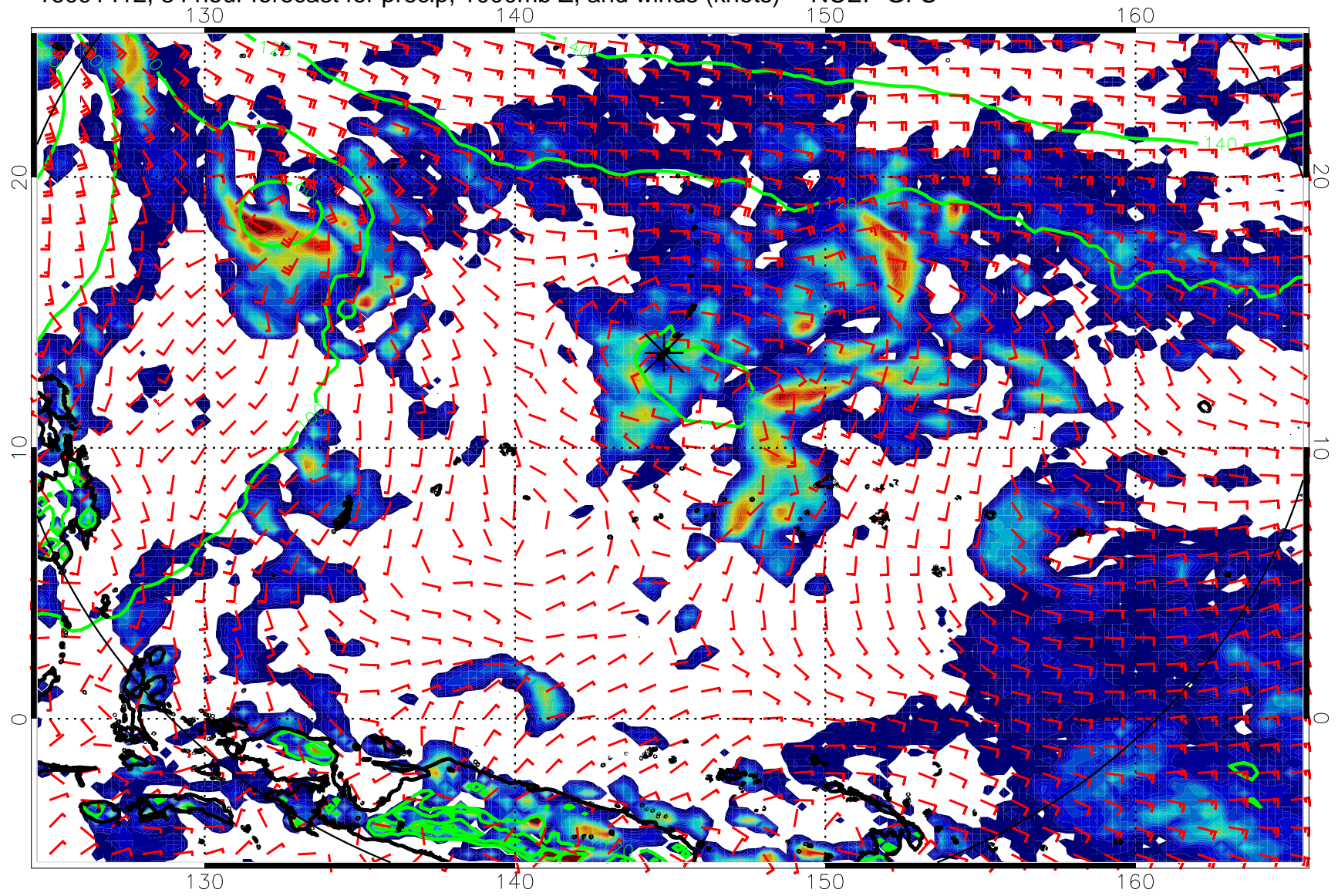
16091412, 84 hour forecast for precip, 1000mb Z, and winds (knots) -- NCEP GFS
