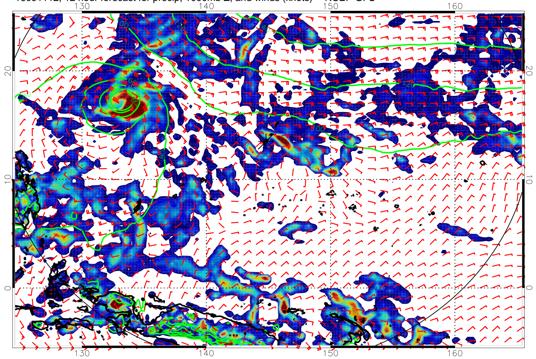
16091112, 12 hour forecast for precip, 1000mb Z, and winds (knots) -- NCEP GFS
