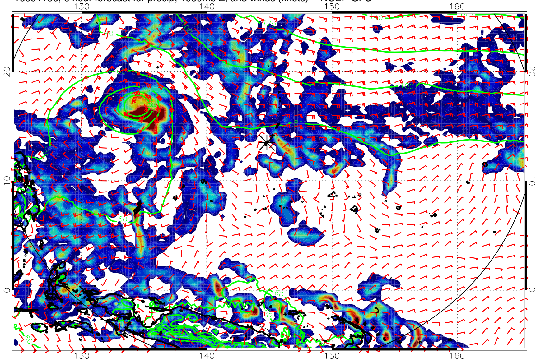
16091106, 6 hour forecast for precip, 1000mb Z, and winds (knots) -- NCEP GFS
