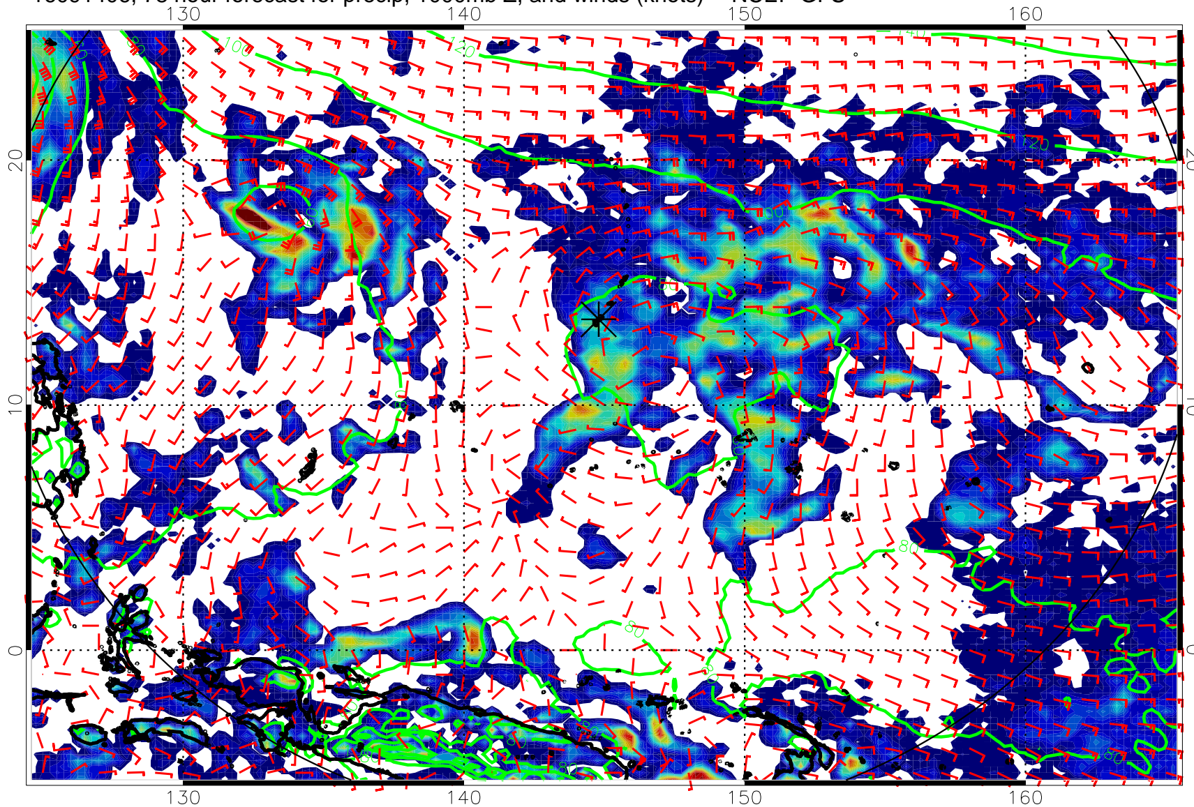
16091406, 78 hour forecast for precip, 1000mb Z, and winds (knots) -- NCEP GFS
