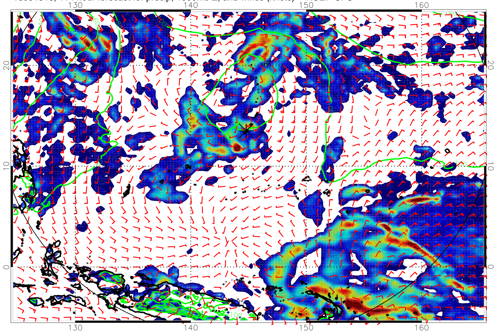
16091518, 114 hour forecast for precip, 1000mb Z, and winds (knots) -- NCEP GFS
