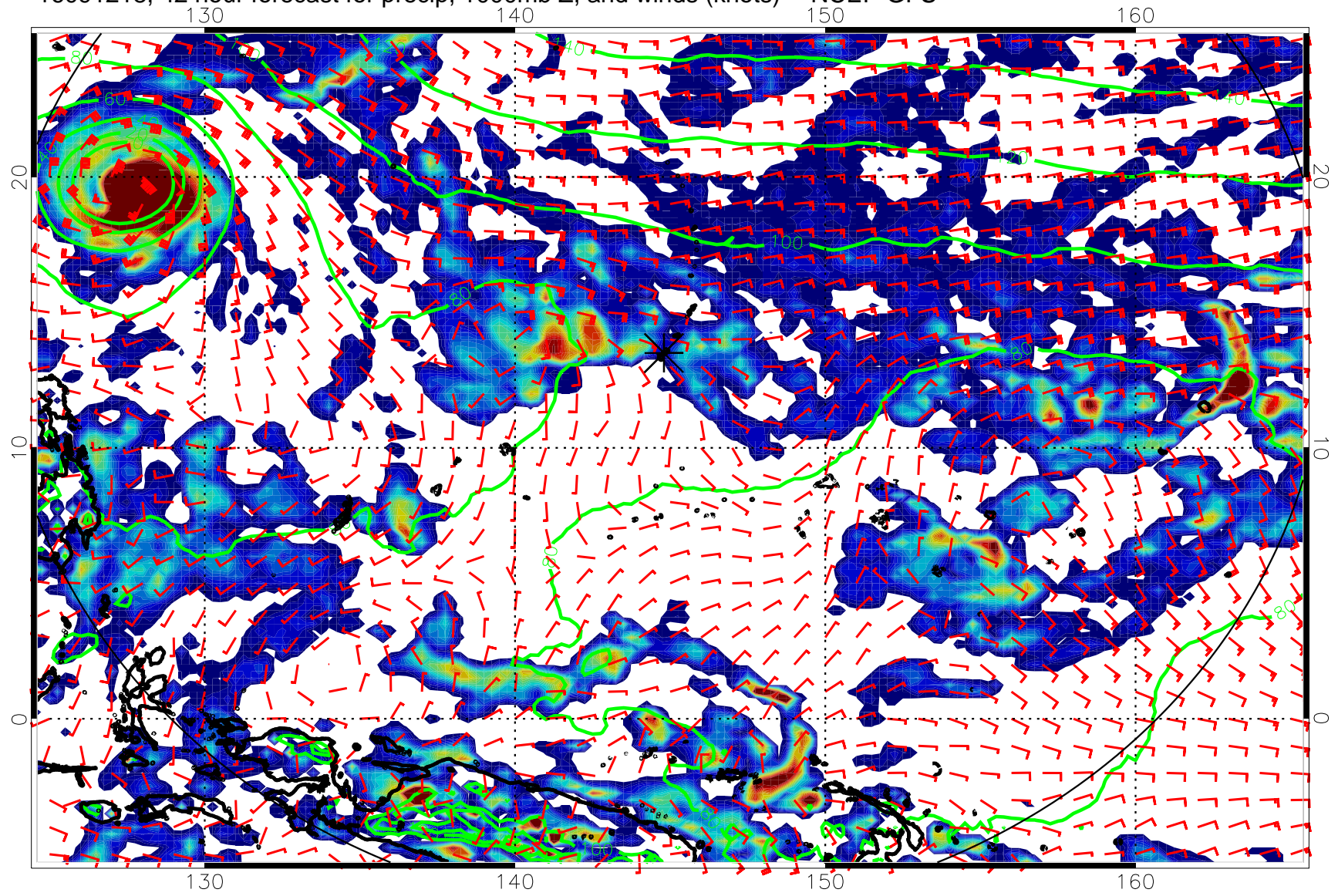
16091218, 42 hour forecast for precip, 1000mb Z, and winds (knots) -- NCEP GFS
