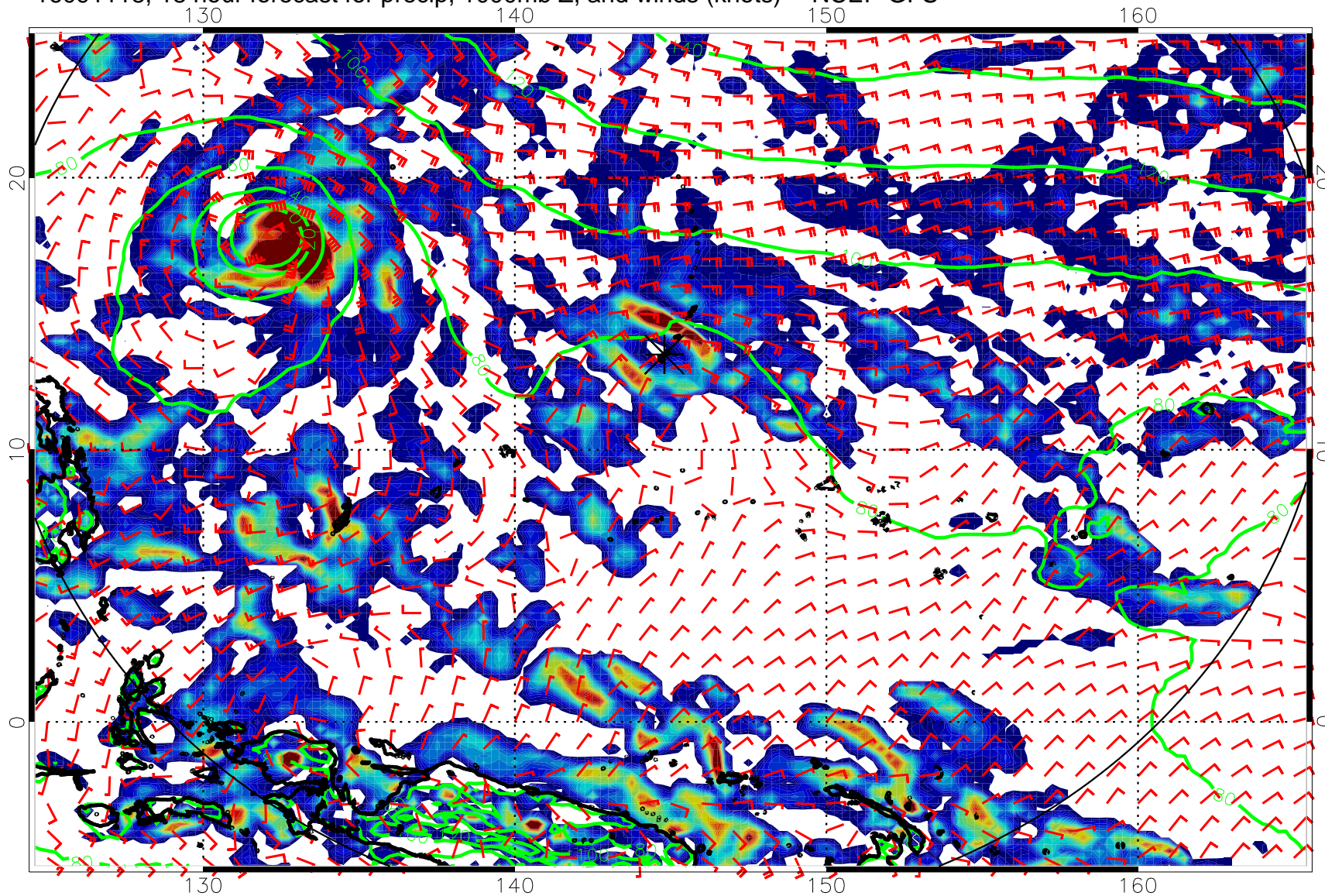
16091118, 18 hour forecast for precip, 1000mb Z, and winds (knots) -- NCEP GFS
