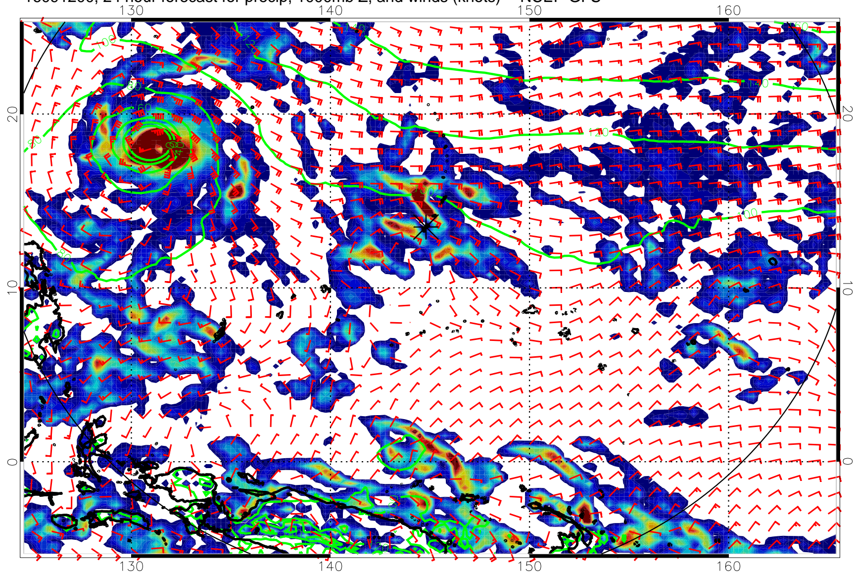
16091200, 24 hour forecast for precip, 1000mb Z, and winds (knots) -- NCEP GFS
