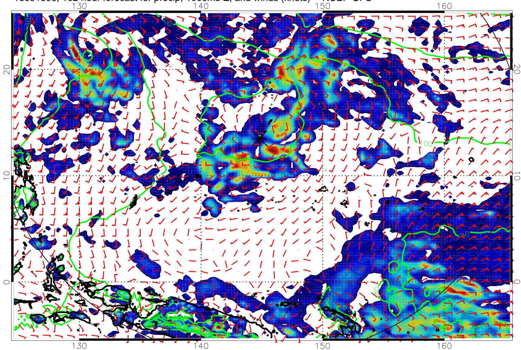
16091506, 102 hour forecast for precip, 1000mb Z, and winds (knots) -- NCEP GFS
