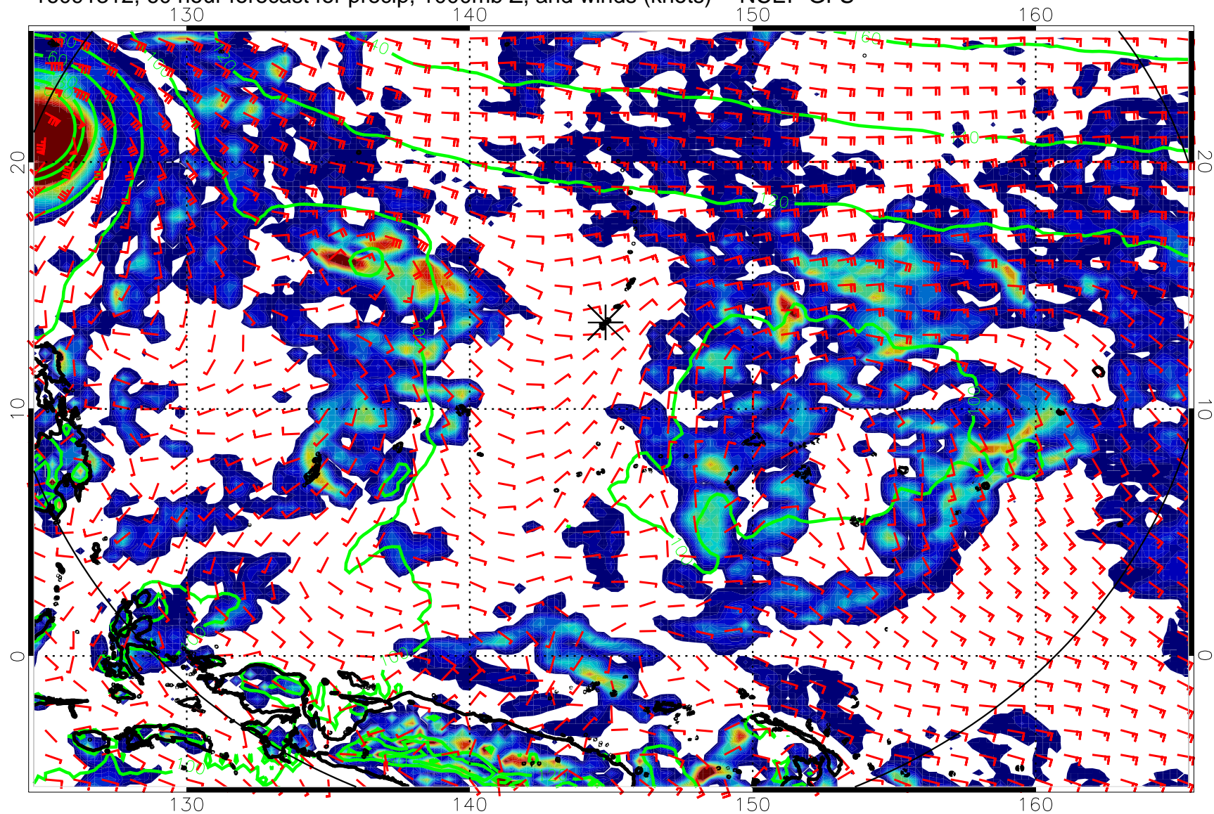
16091312, 60 hour forecast for precip, 1000mb Z, and winds (knots) -- NCEP GFS
