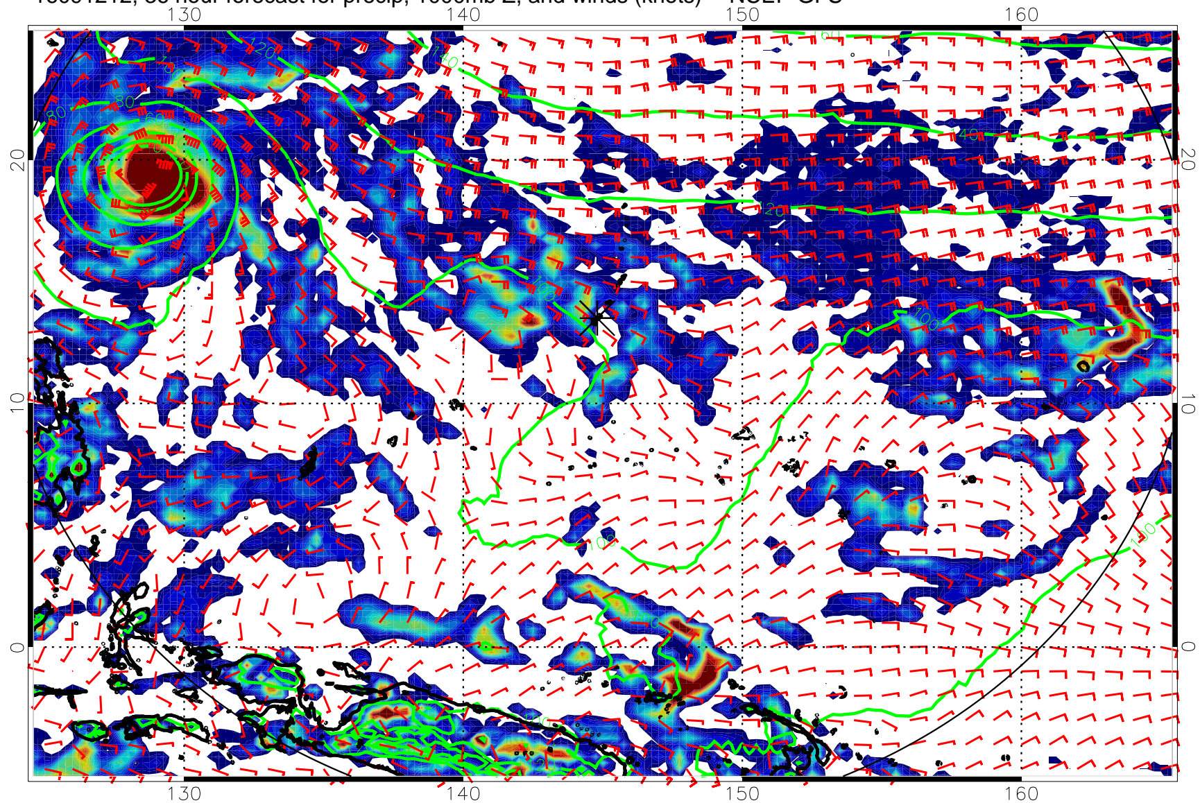
16091212, 36 hour forecast for precip, 1000mb Z, and winds (knots) -- NCEP GFS
