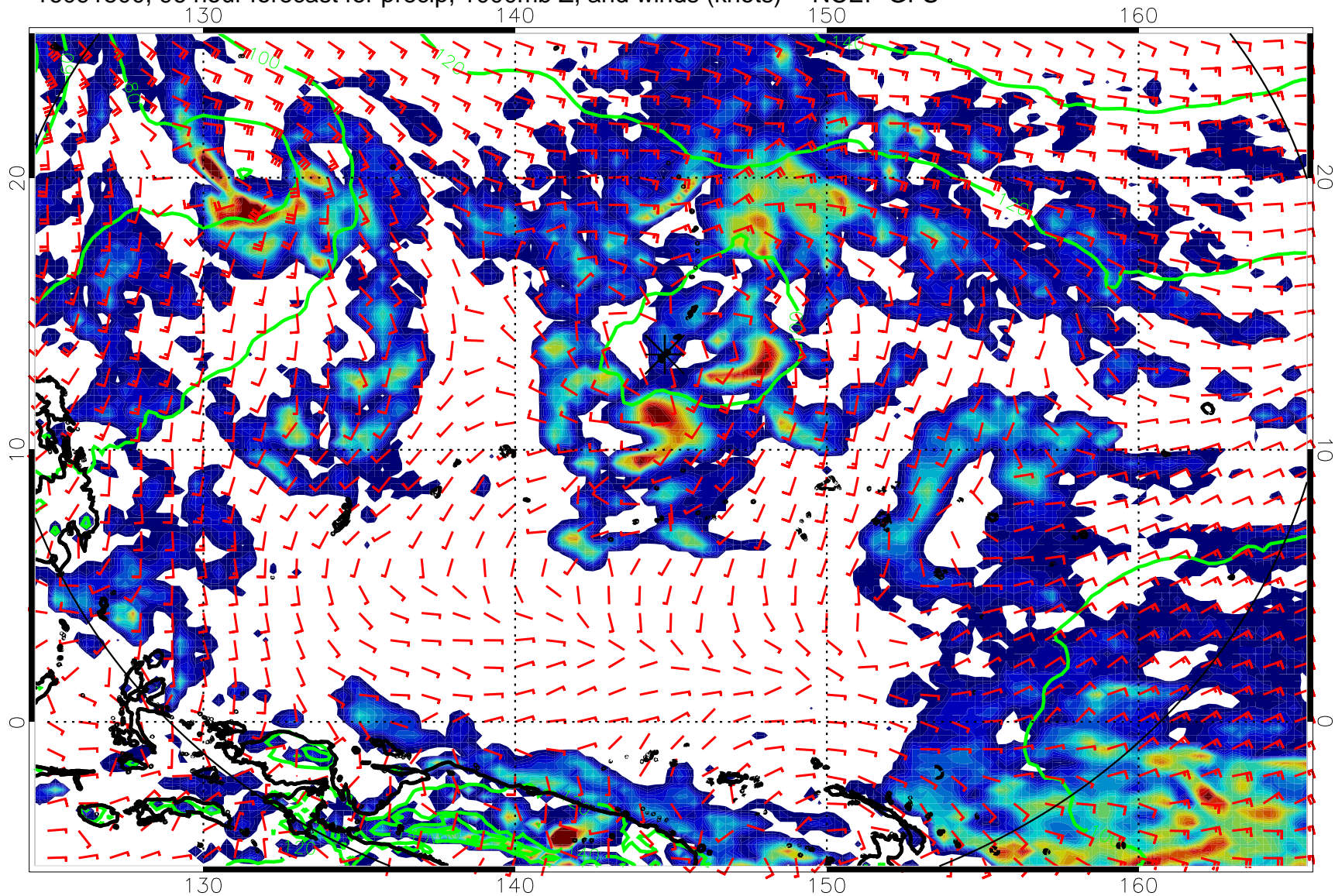
16091500, 96 hour forecast for precip, 1000mb Z, and winds (knots) -- NCEP GFS
