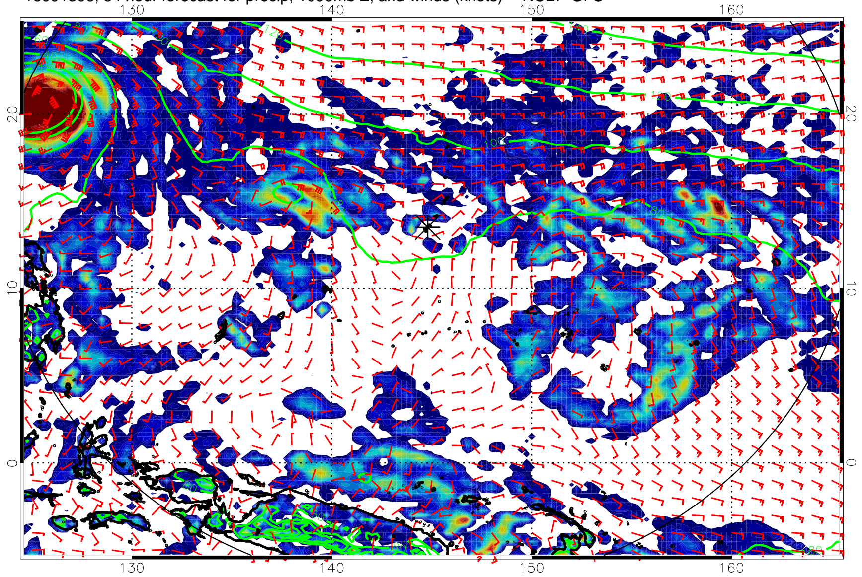
16091306, 54 hour forecast for precip, 1000mb Z, and winds (knots) -- NCEP GFS
