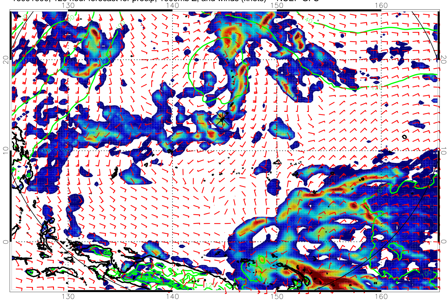
16091600, 120 hour forecast for precip, 1000mb Z, and winds (knots) -- NCEP GFS
