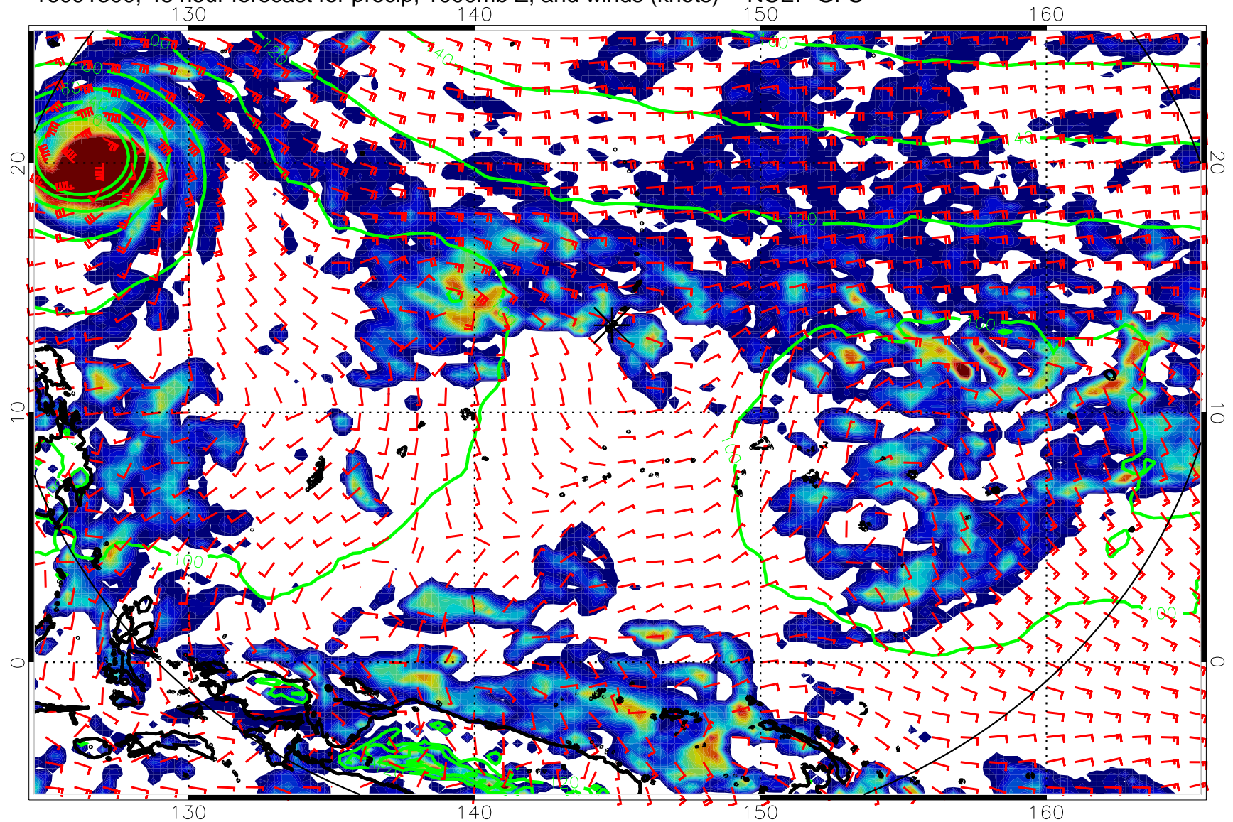
16091300, 48 hour forecast for precip, 1000mb Z, and winds (knots) -- NCEP GFS
