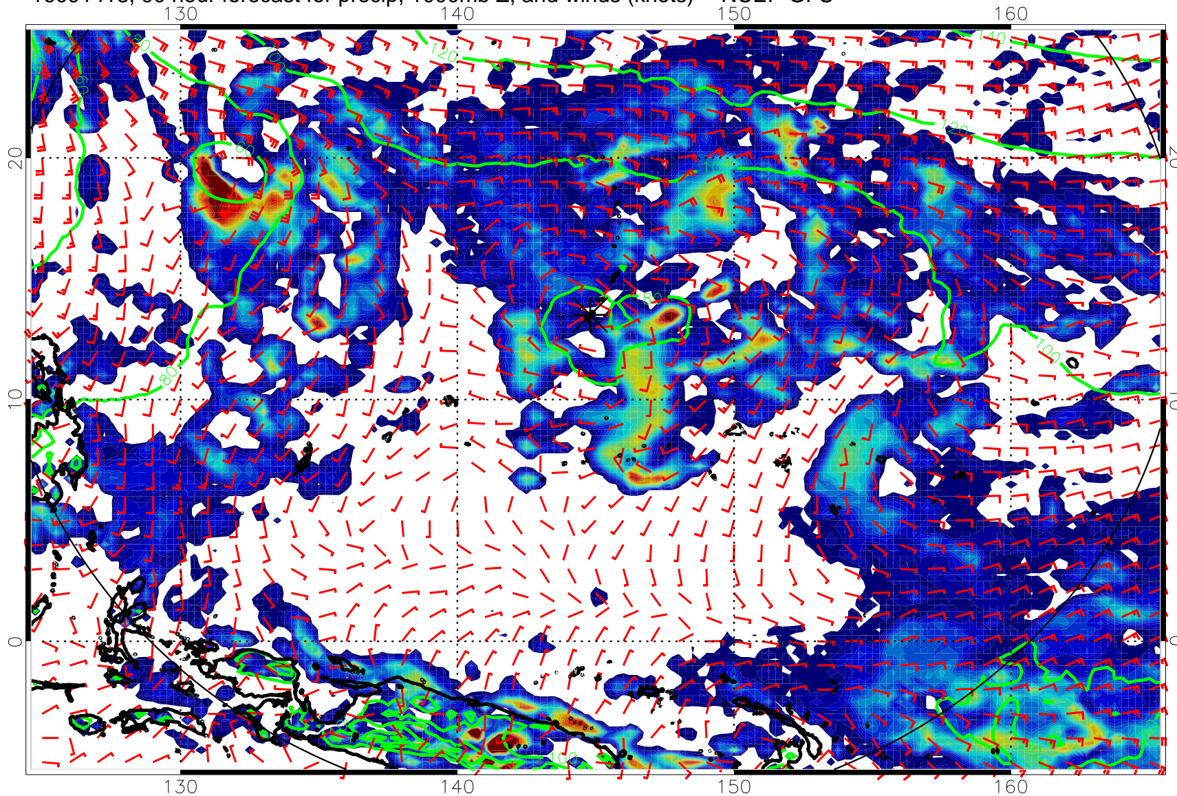
16091418, 90 hour forecast for precip, 1000mb Z, and winds (knots) -- NCEP GFS
