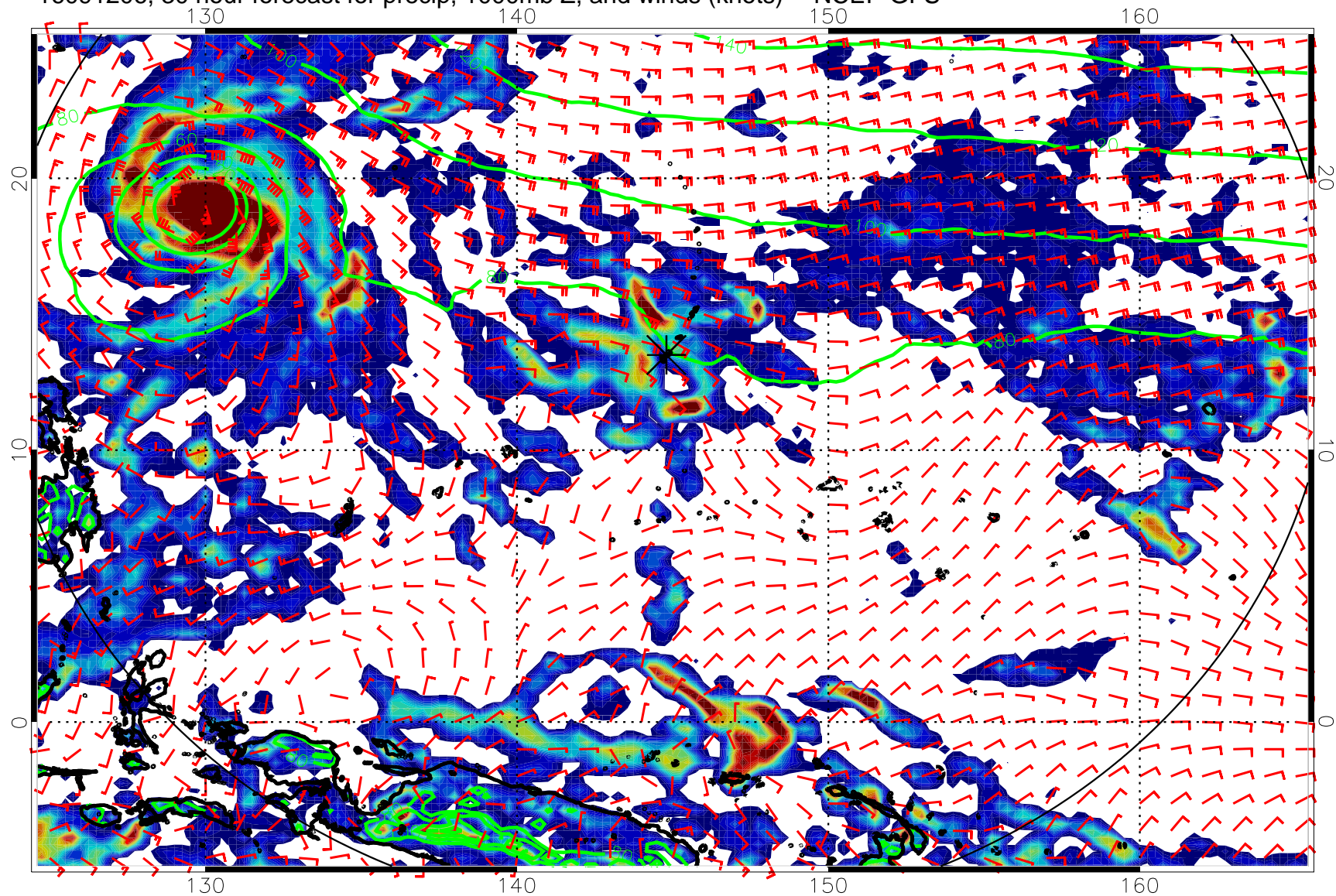
16091206, 30 hour forecast for precip, 1000mb Z, and winds (knots) -- NCEP GFS
