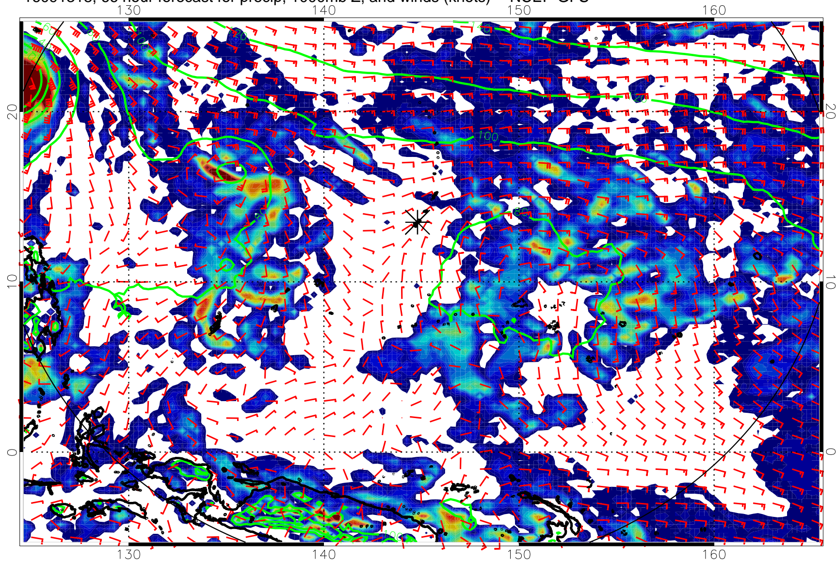
16091318, 66 hour forecast for precip, 1000mb Z, and winds (knots) -- NCEP GFS
