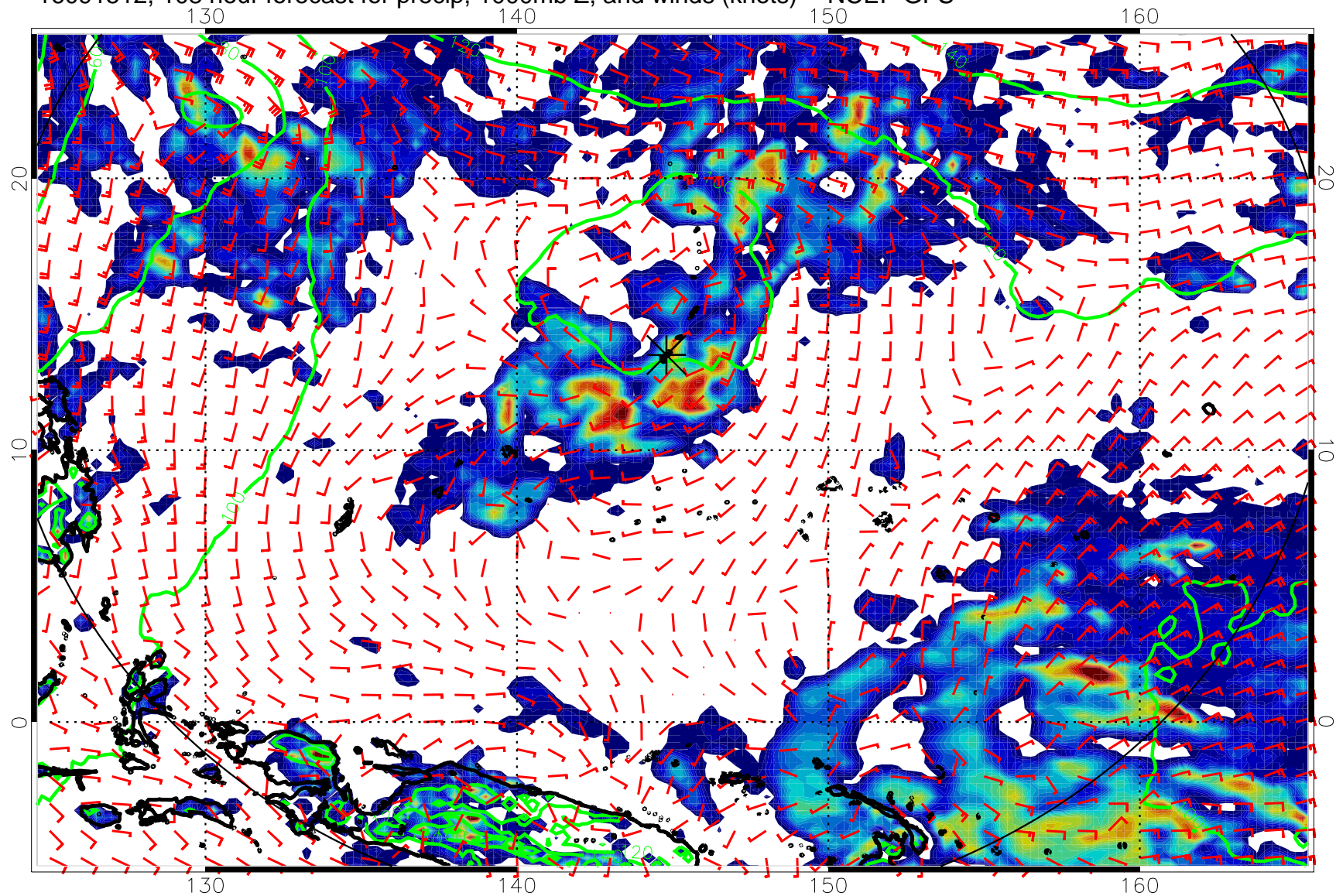
16091512, 108 hour forecast for precip, 1000mb Z, and winds (knots) -- NCEP GFS
