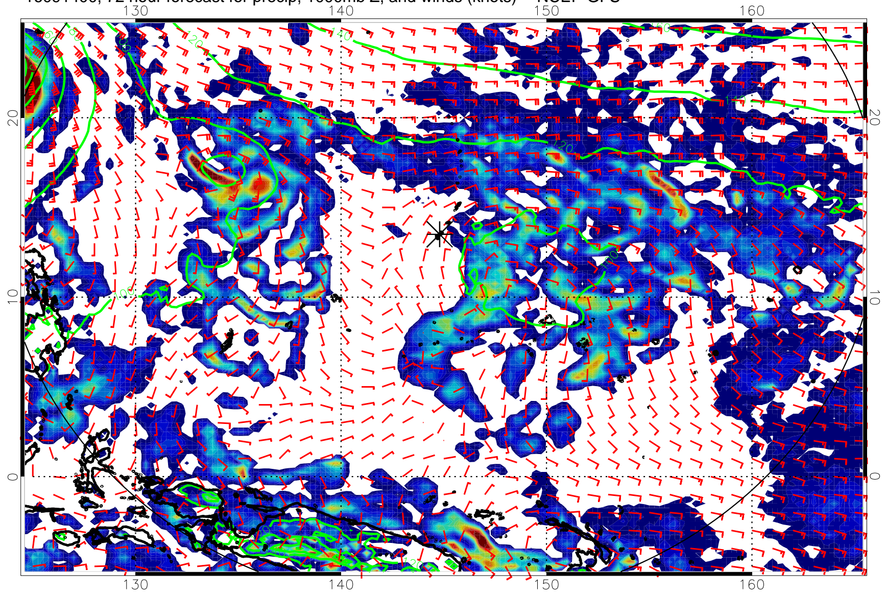
16091400, 72 hour forecast for precip, 1000mb Z, and winds (knots) -- NCEP GFS
