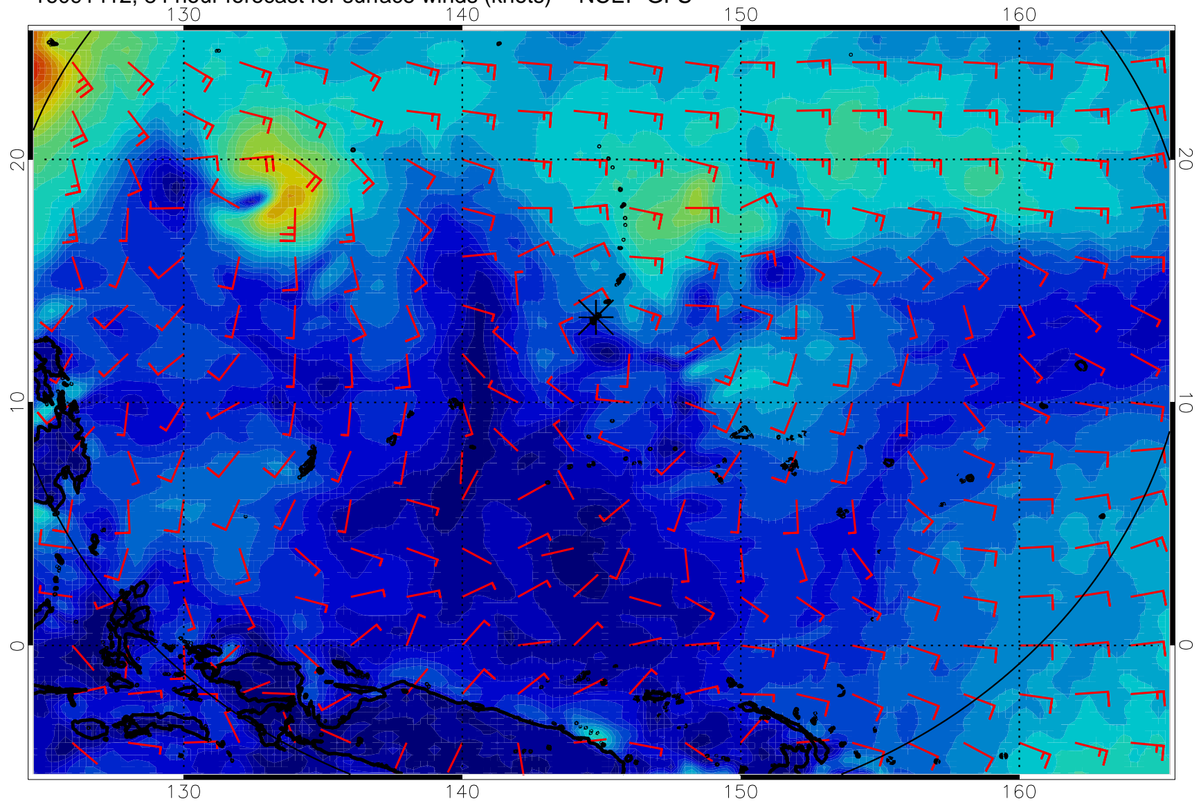
16091412, 84 hour forecast for surface winds (knots) -- NCEP GFS
