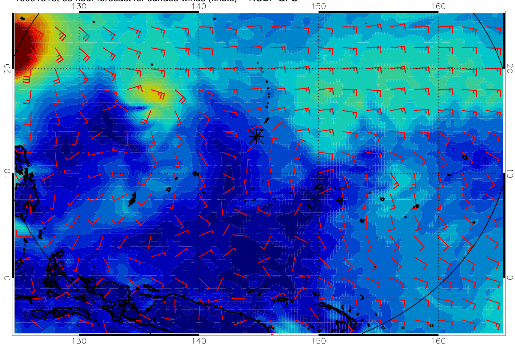
16091318, 66 hour forecast for surface winds (knots) -- NCEP GFS
