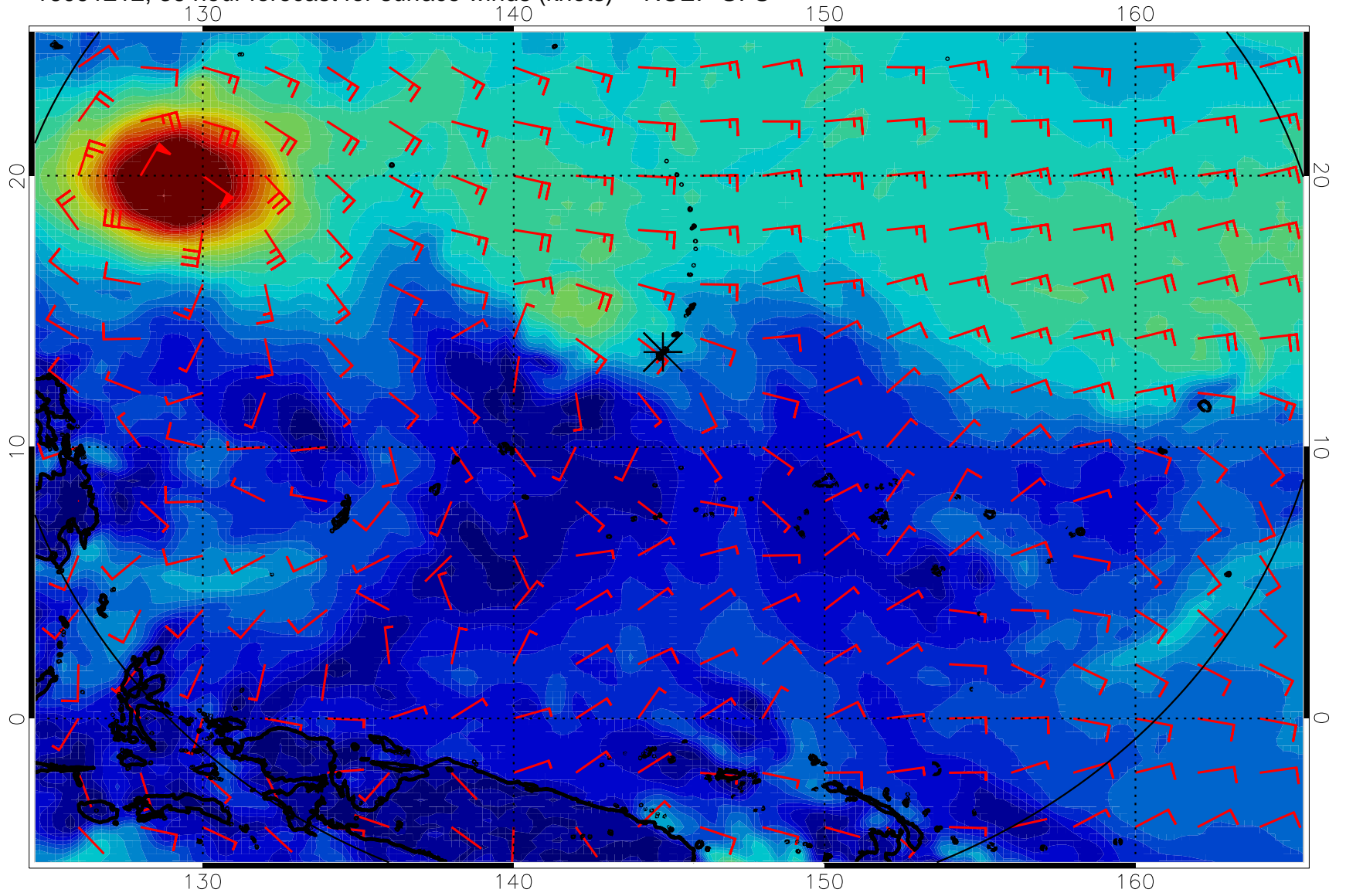
16091212, 36 hour forecast for surface winds (knots) -- NCEP GFS
