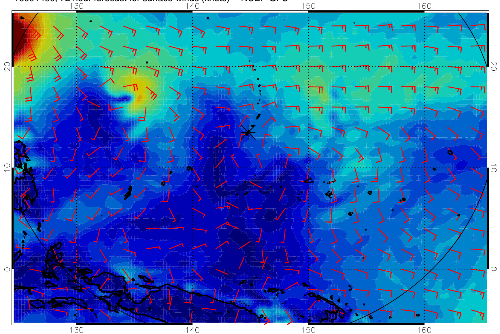
16091400, 72 hour forecast for surface winds (knots) -- NCEP GFS
