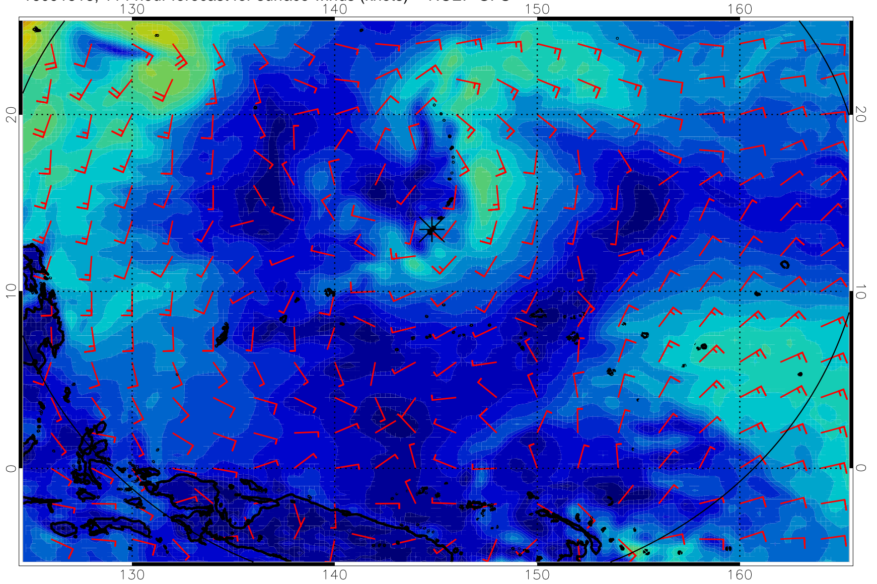
16091518, 114 hour forecast for surface winds (knots) -- NCEP GFS
