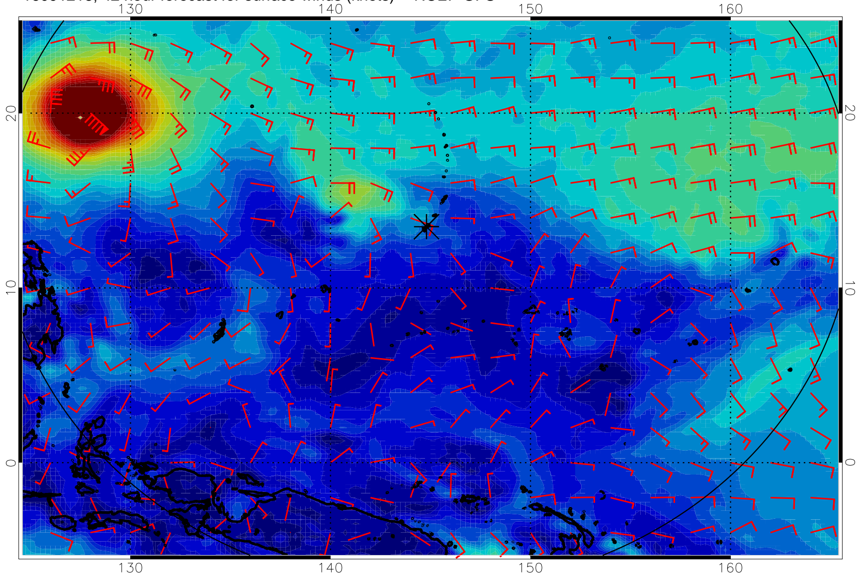
16091218, 42 hour forecast for surface winds (knots) -- NCEP GFS
