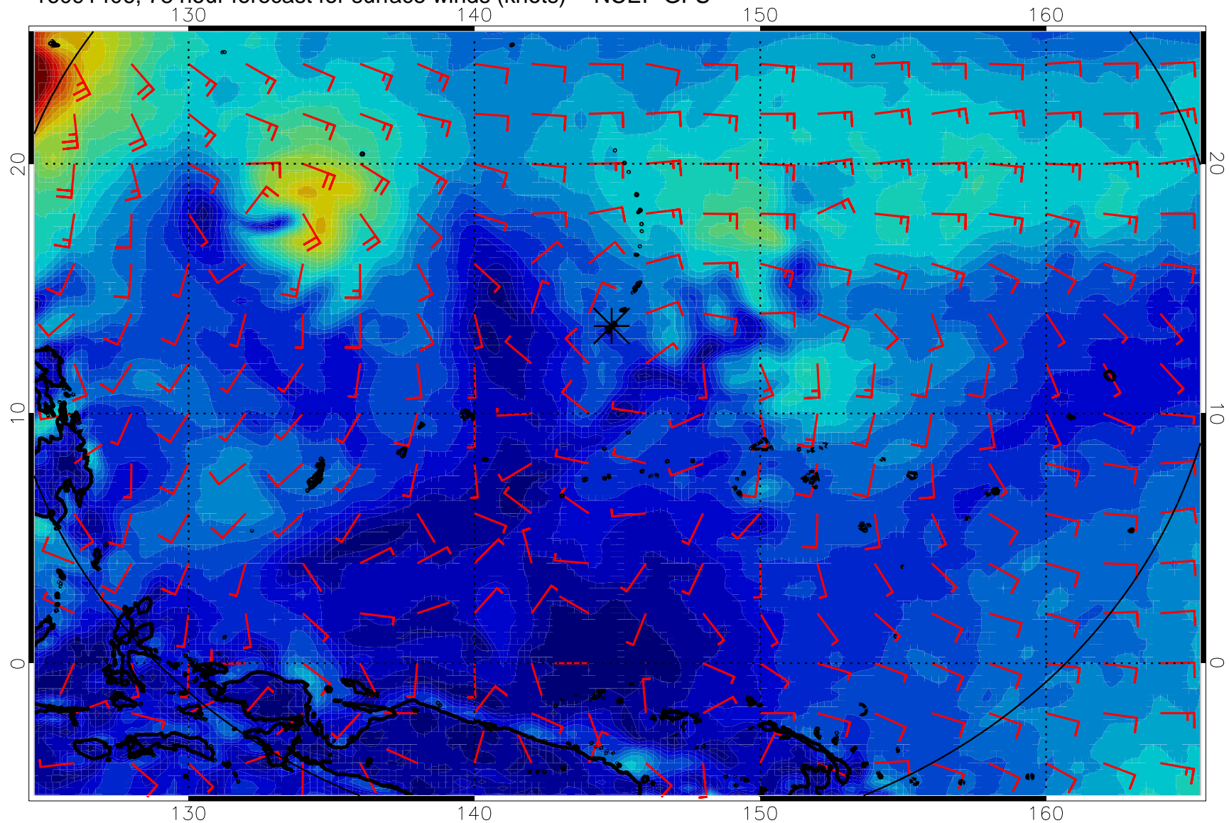
16091406, 78 hour forecast for surface winds (knots) -- NCEP GFS
