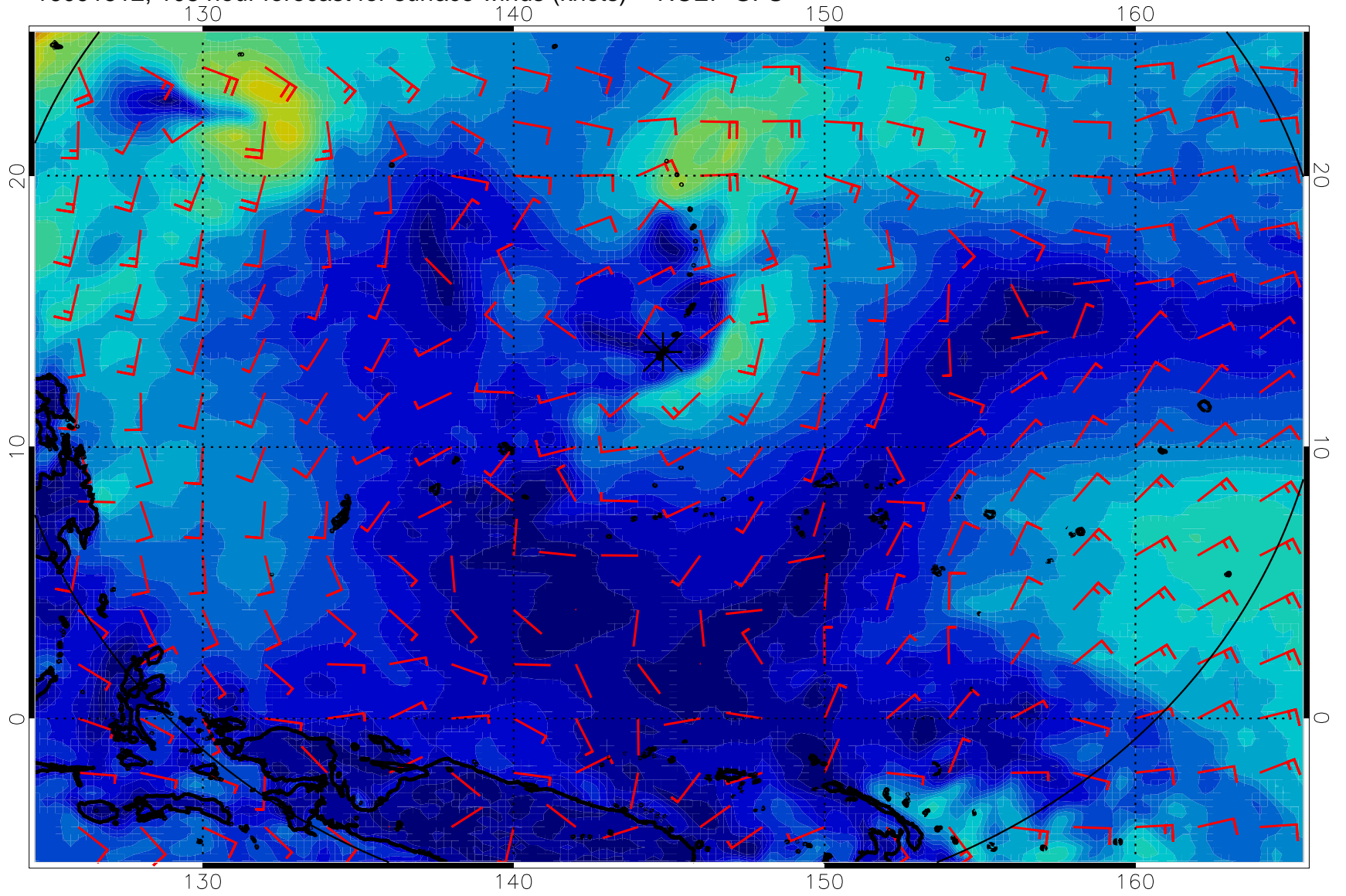
16091512, 108 hour forecast for surface winds (knots) -- NCEP GFS
