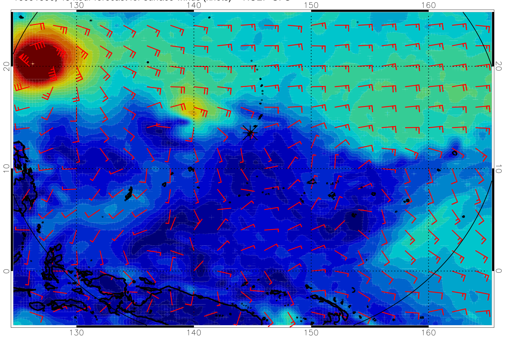
16091300, 48 hour forecast for surface winds (knots) -- NCEP GFS
