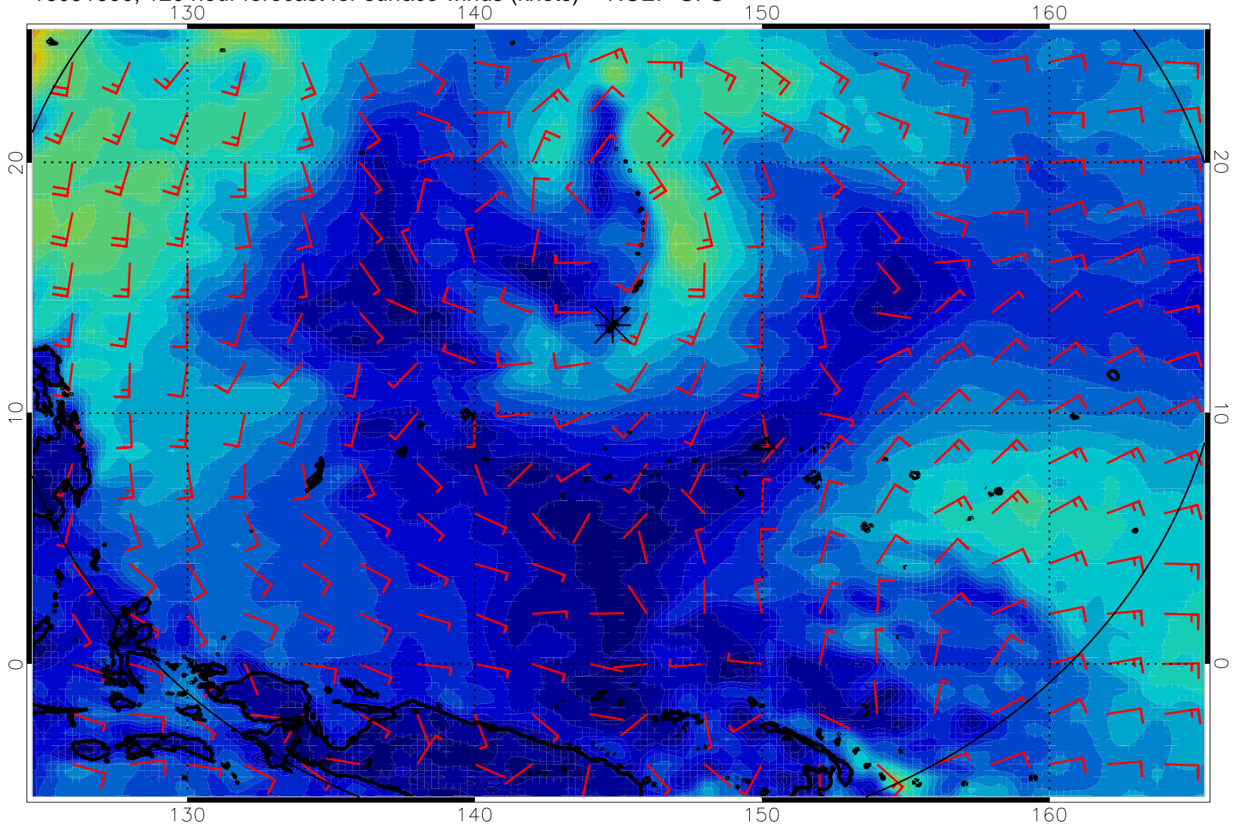
16091600, 120 hour forecast for surface winds (knots) -- NCEP GFS
