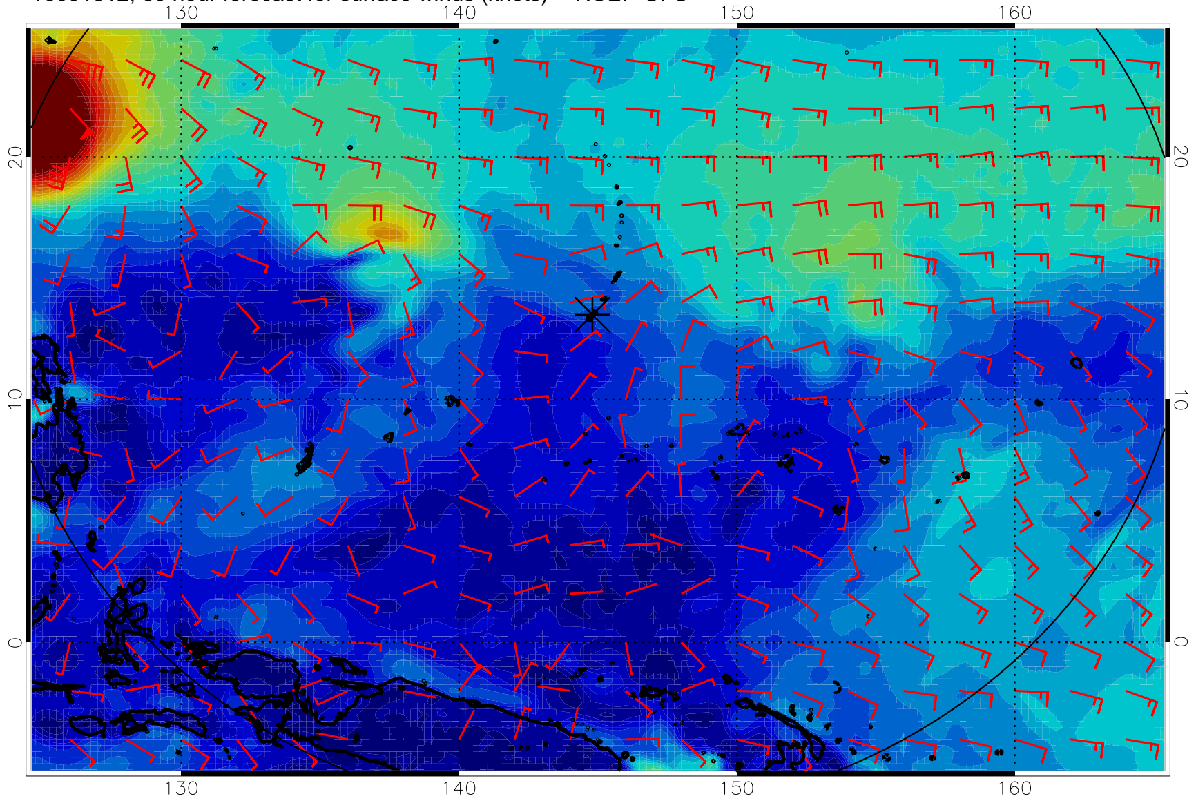
16091312, 60 hour forecast for surface winds (knots) -- NCEP GFS
