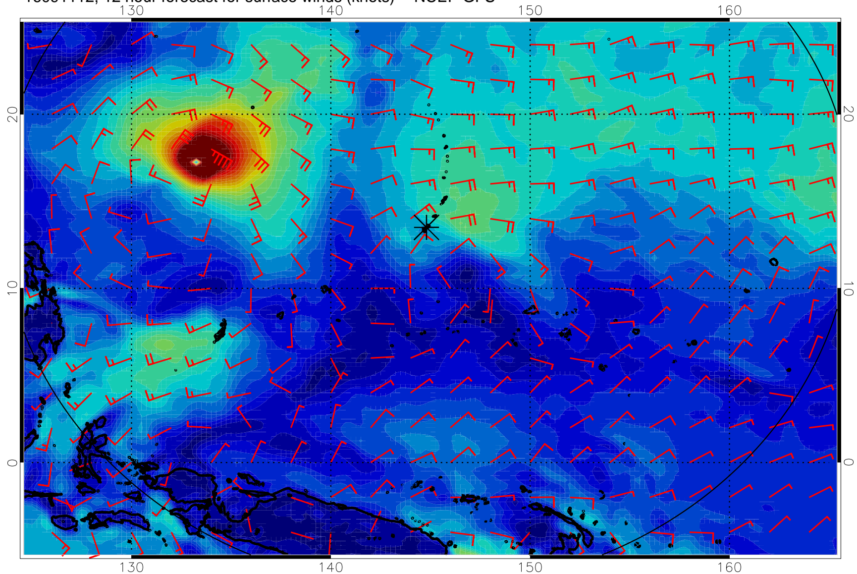
16091112, 12 hour forecast for surface winds (knots) -- NCEP GFS
