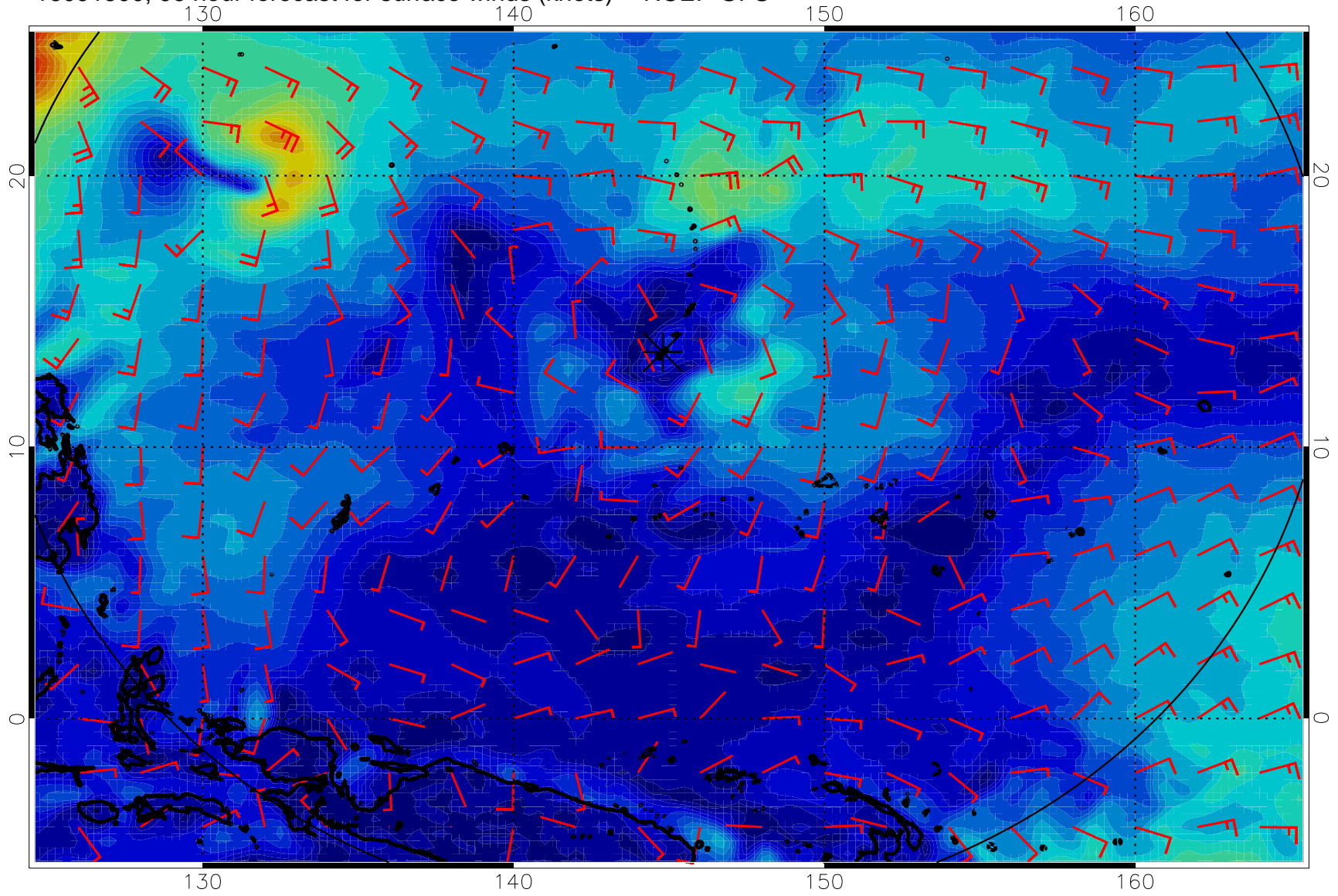
16091500, 96 hour forecast for surface winds (knots) -- NCEP GFS
