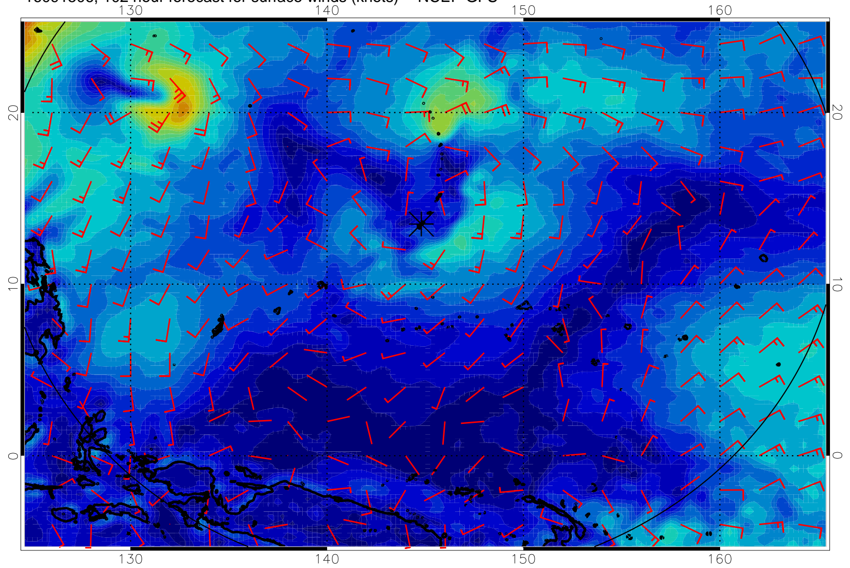
16091506, 102 hour forecast for surface winds (knots) -- NCEP GFS
