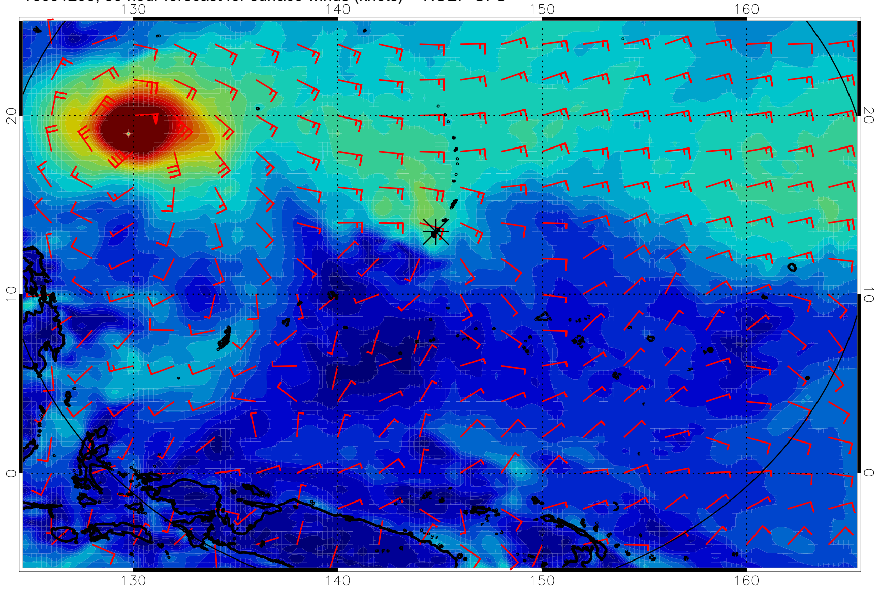
16091206, 30 hour forecast for surface winds (knots) -- NCEP GFS
