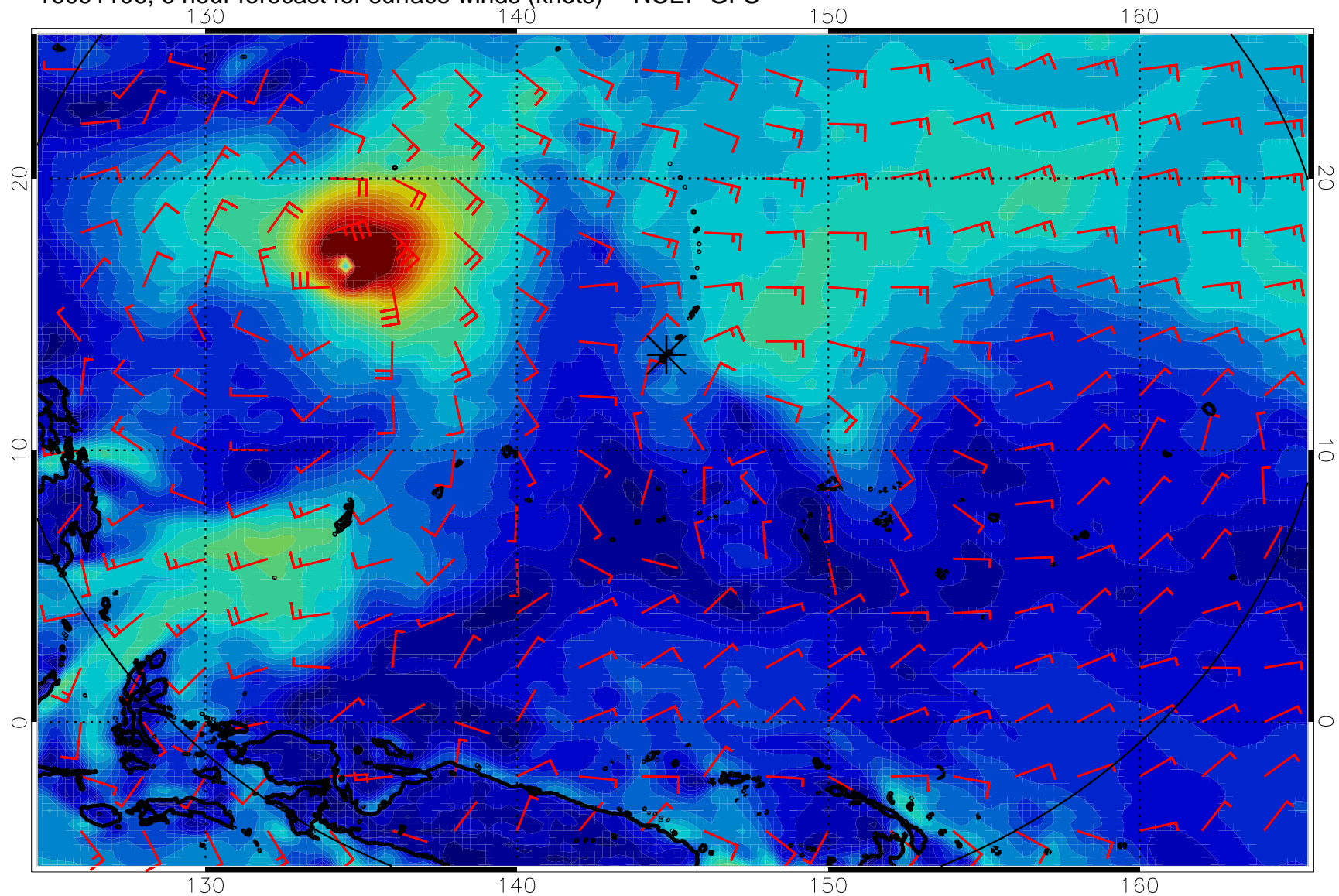
16091106, 6 hour forecast for surface winds (knots) -- NCEP GFS
