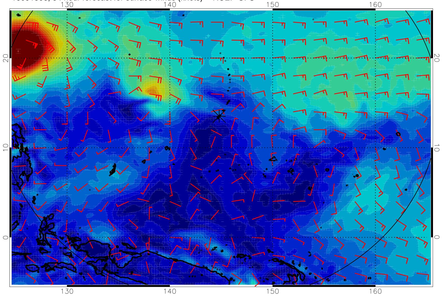
16091306, 54 hour forecast for surface winds (knots) -- NCEP GFS
