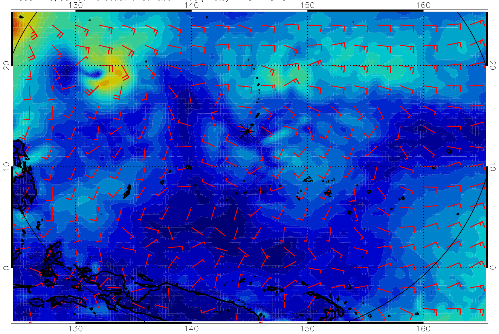
16091418, 90 hour forecast for surface winds (knots) -- NCEP GFS
