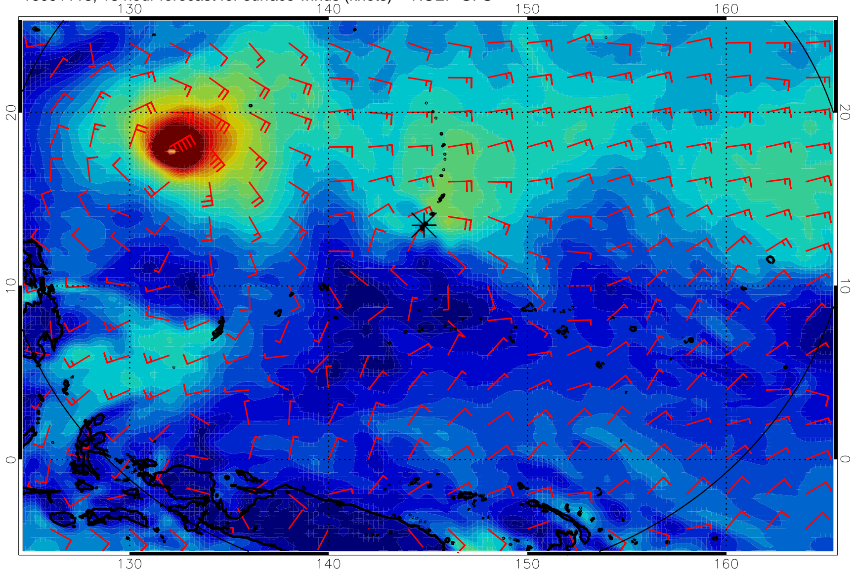
16091118, 18 hour forecast for surface winds (knots) -- NCEP GFS
