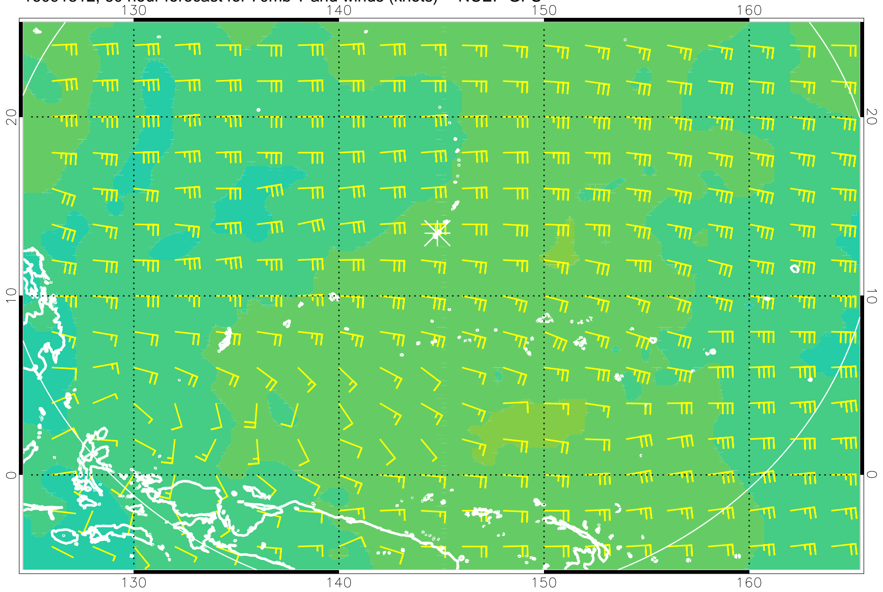
16091312, 60 hour forecast for 70mb T and winds (knots) -- NCEP GFS
