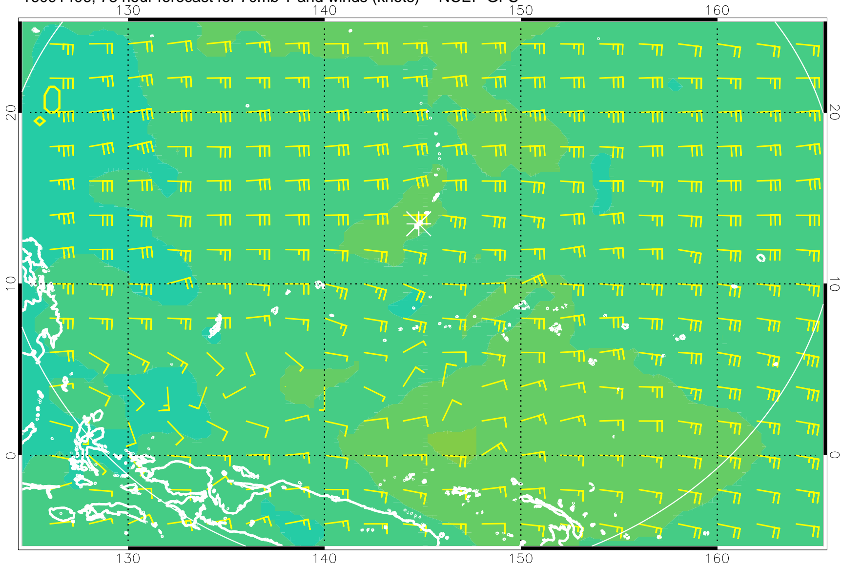
16091406, 78 hour forecast for 70mb T and winds (knots) -- NCEP GFS
