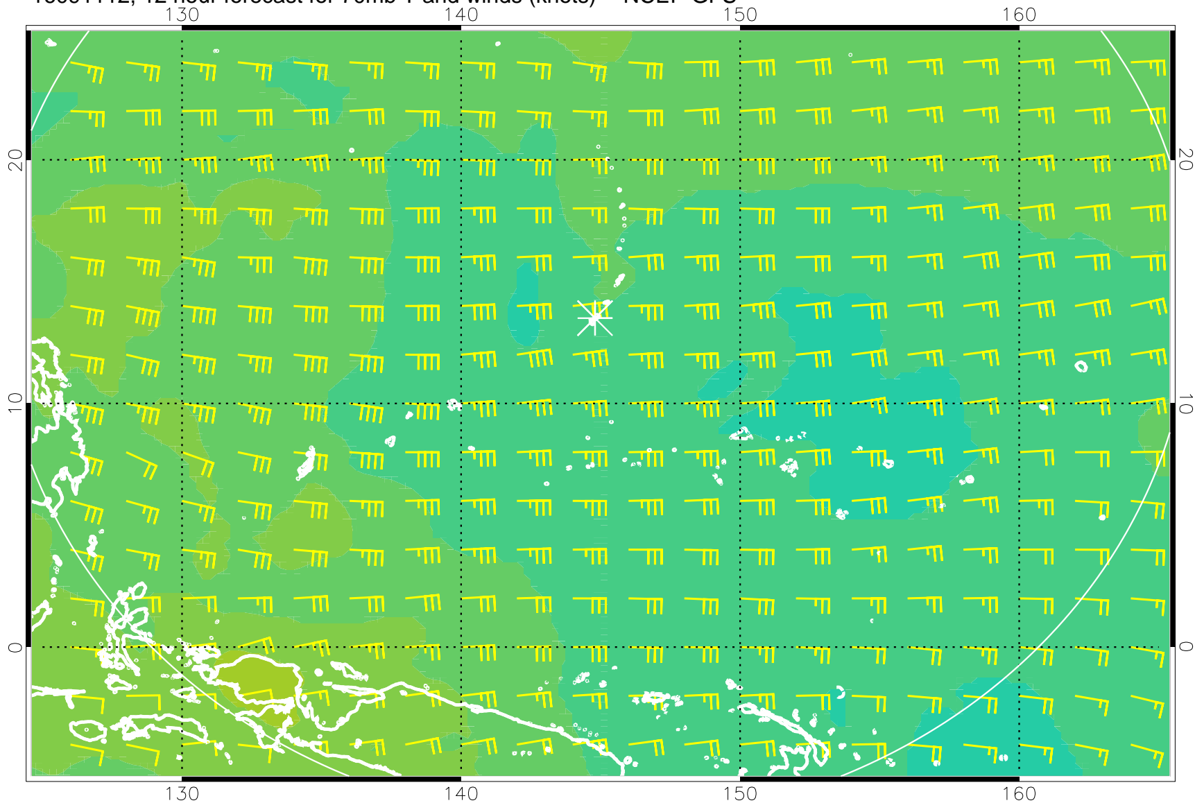
16091112, 12 hour forecast for 70mb T and winds (knots) -- NCEP GFS
