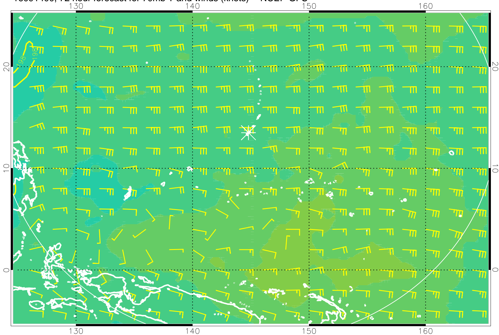
16091400, 72 hour forecast for 70mb T and winds (knots) -- NCEP GFS
