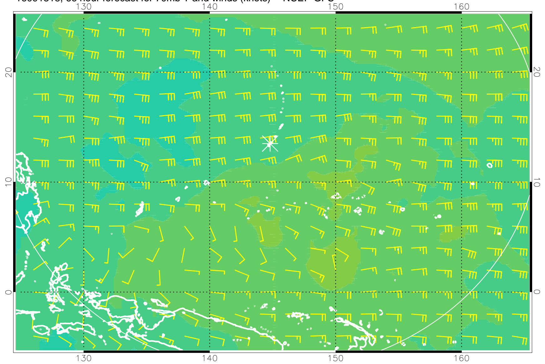
16091318, 66 hour forecast for 70mb T and winds (knots) -- NCEP GFS
