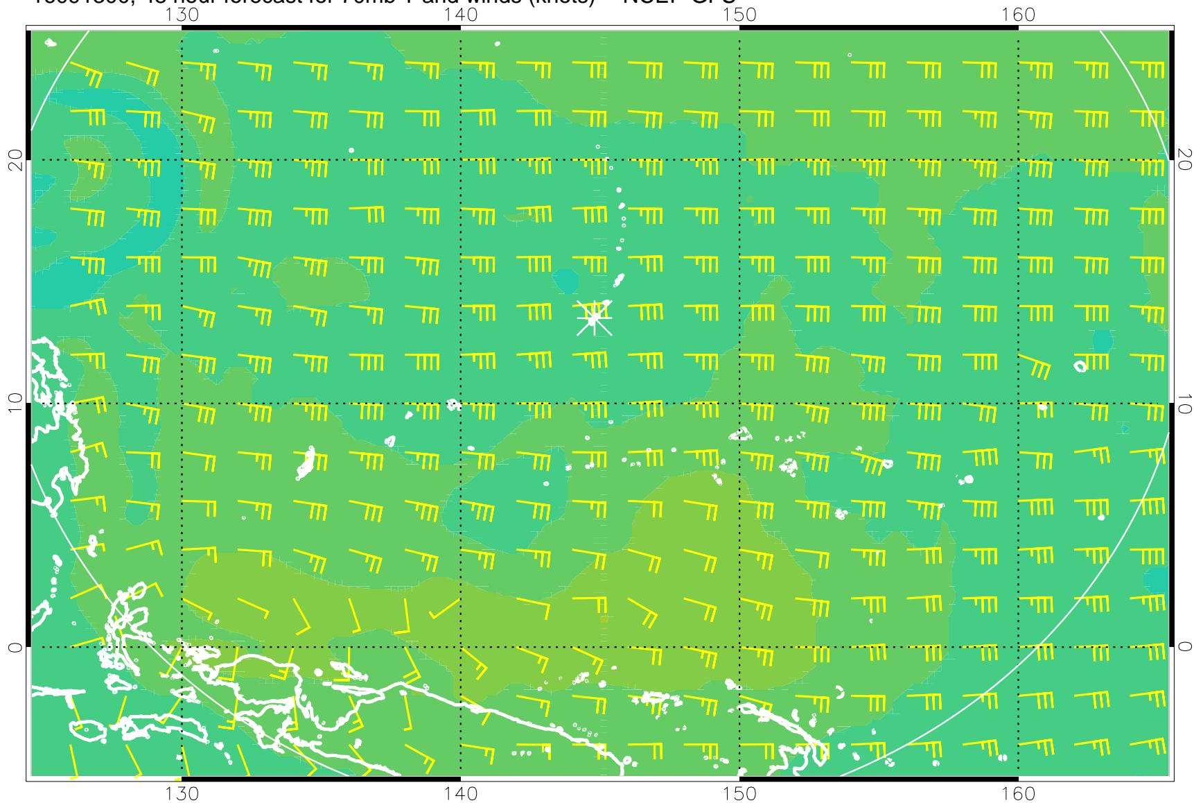
16091300, 48 hour forecast for 70mb T and winds (knots) -- NCEP GFS
