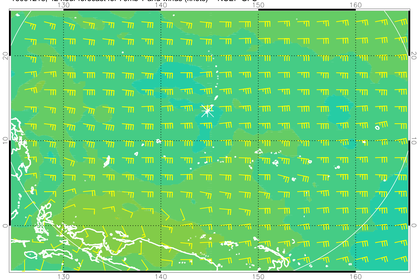
16091218, 42 hour forecast for 70mb T and winds (knots) -- NCEP GFS
