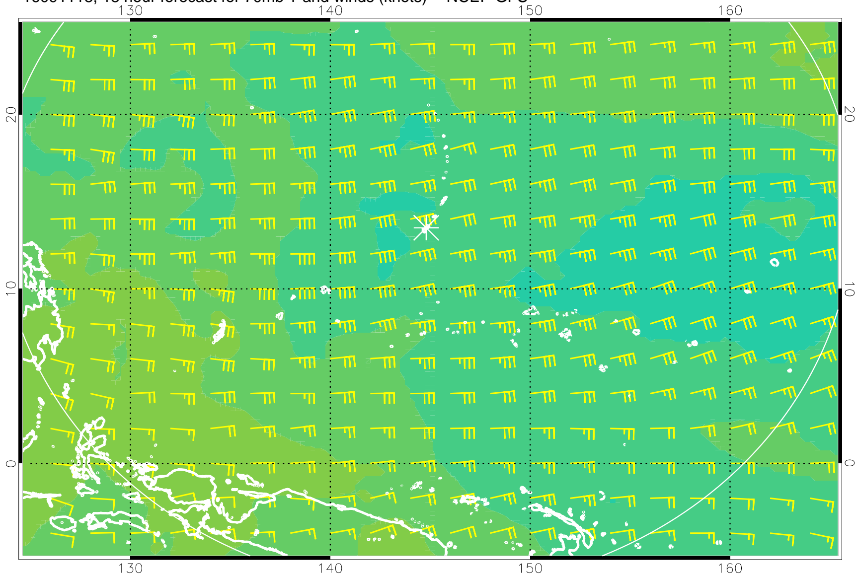
16091118, 18 hour forecast for 70mb T and winds (knots) -- NCEP GFS
