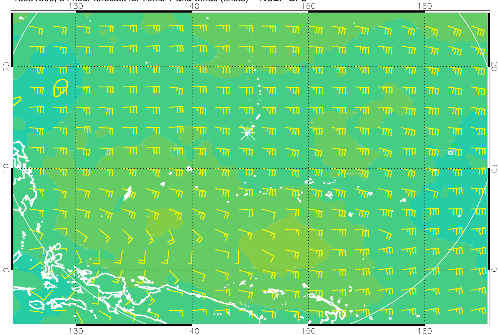
16091306, 54 hour forecast for 70mb T and winds (knots) -- NCEP GFS
