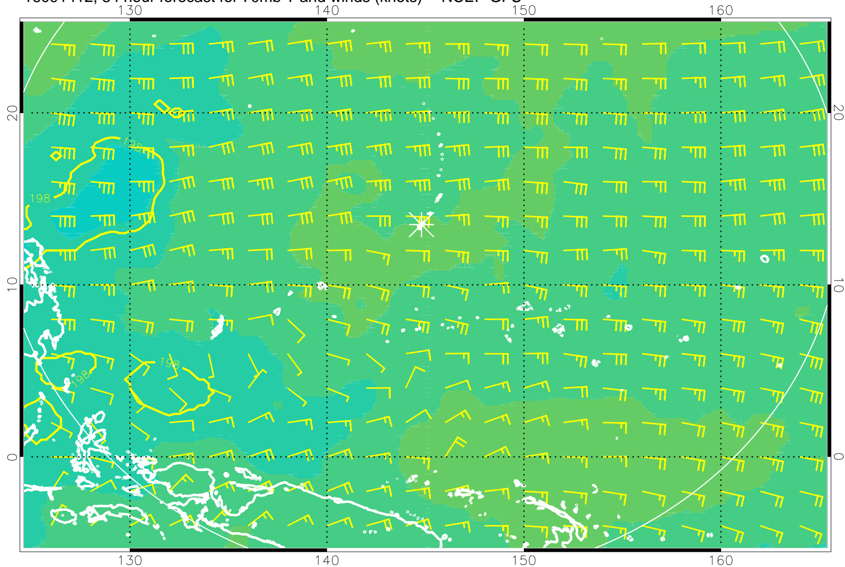
16091412, 84 hour forecast for 70mb T and winds (knots) -- NCEP GFS
