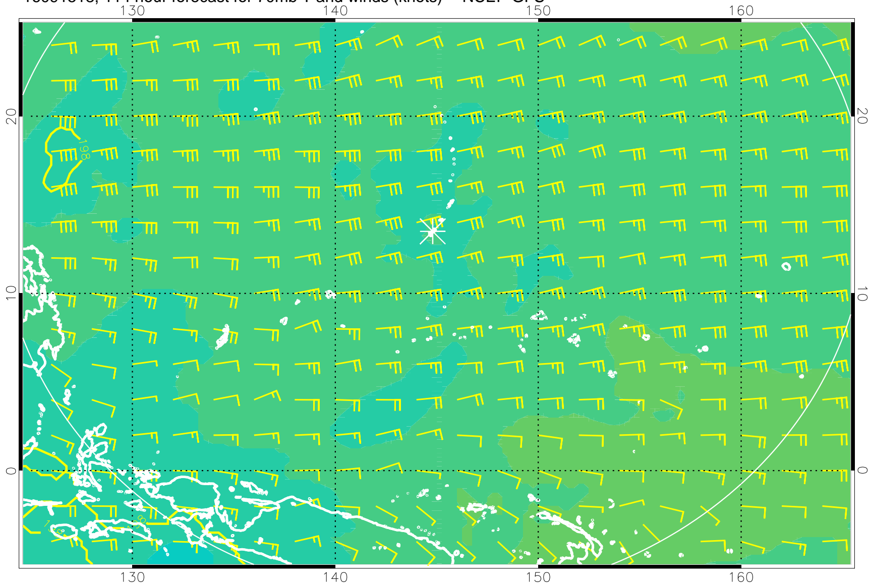
16091518, 114 hour forecast for 70mb T and winds (knots) -- NCEP GFS
