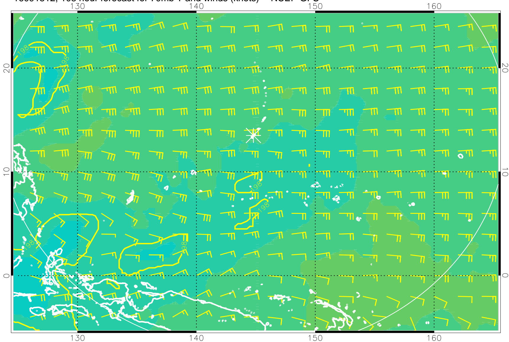
16091512, 108 hour forecast for 70mb T and winds (knots) -- NCEP GFS
