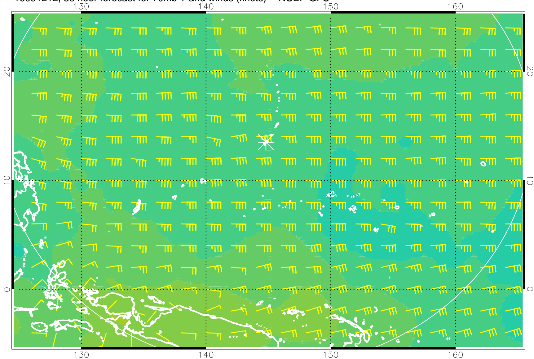
16091212, 36 hour forecast for 70mb T and winds (knots) -- NCEP GFS
