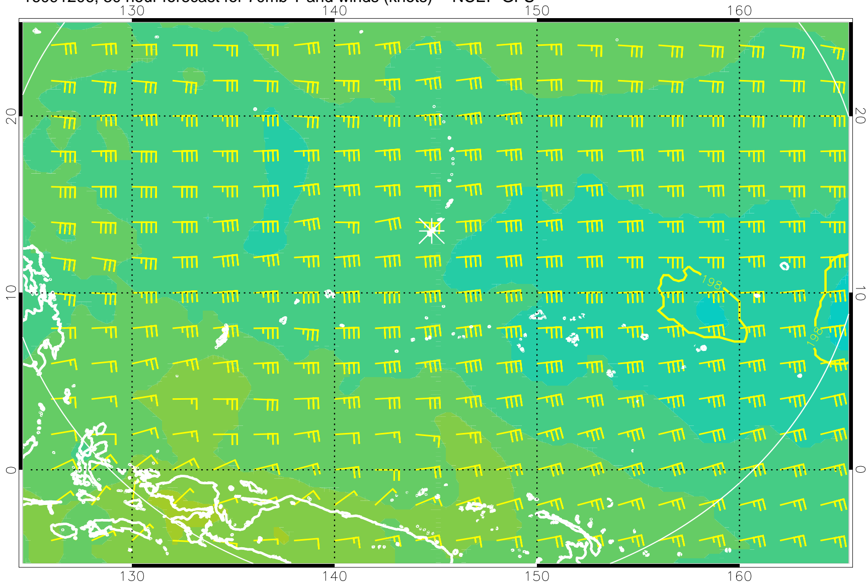
16091206, 30 hour forecast for 70mb T and winds (knots) -- NCEP GFS
