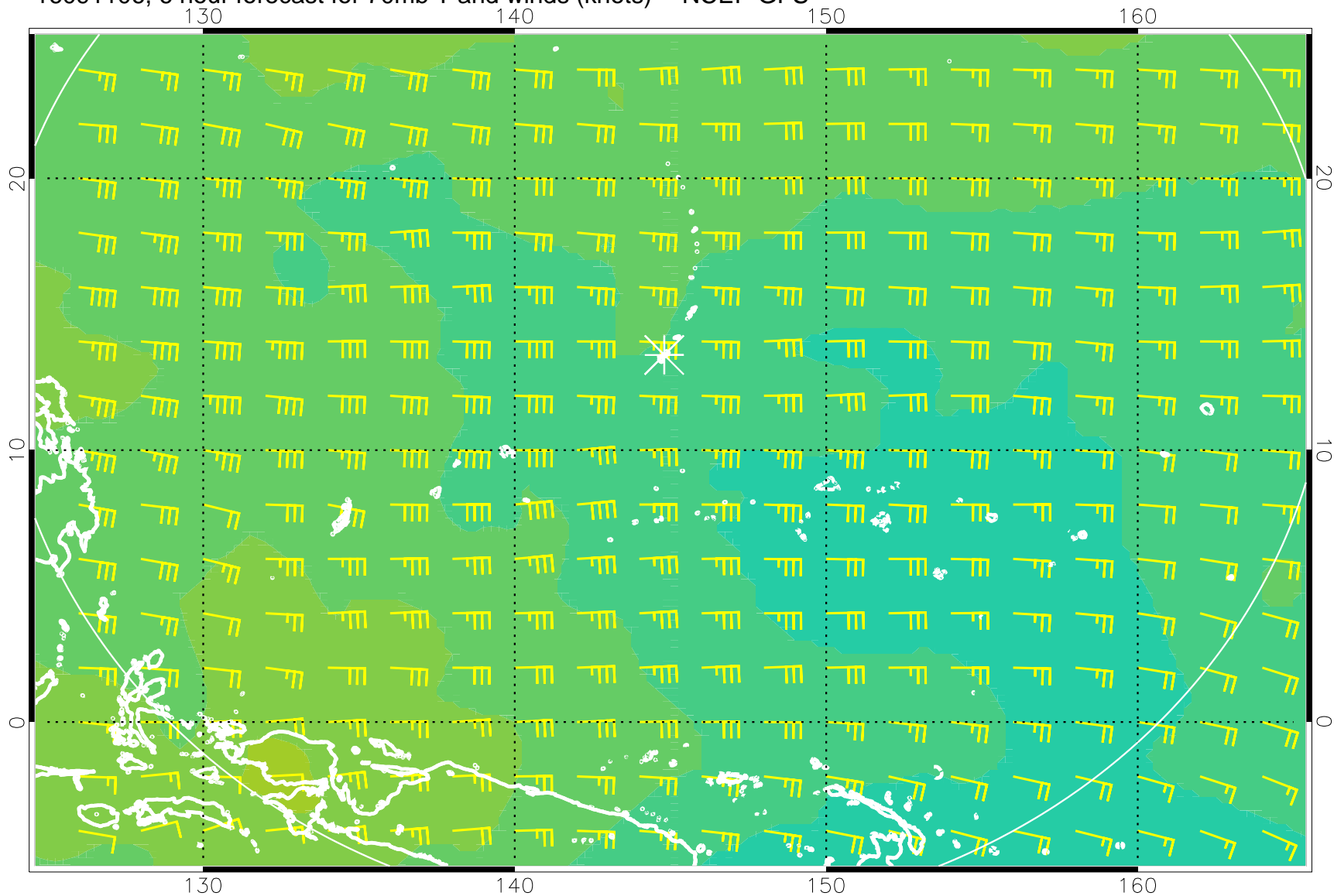
16091106, 6 hour forecast for 70mb T and winds (knots) -- NCEP GFS
