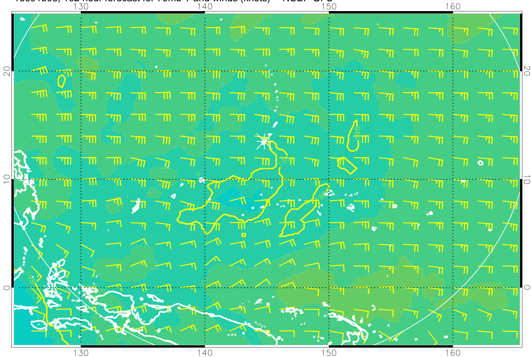
16091506, 102 hour forecast for 70mb T and winds (knots) -- NCEP GFS
