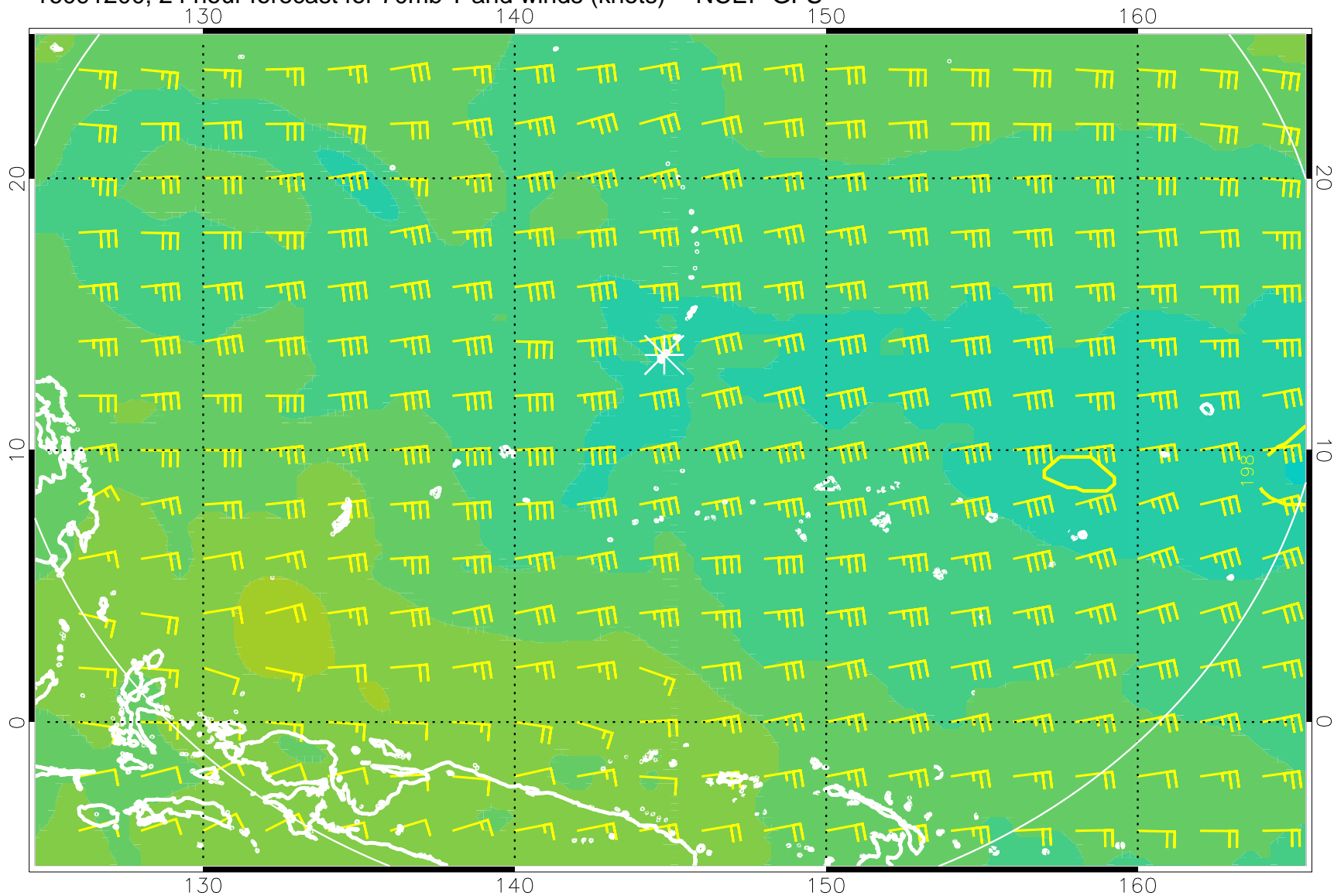
16091200, 24 hour forecast for 70mb T and winds (knots) -- NCEP GFS
