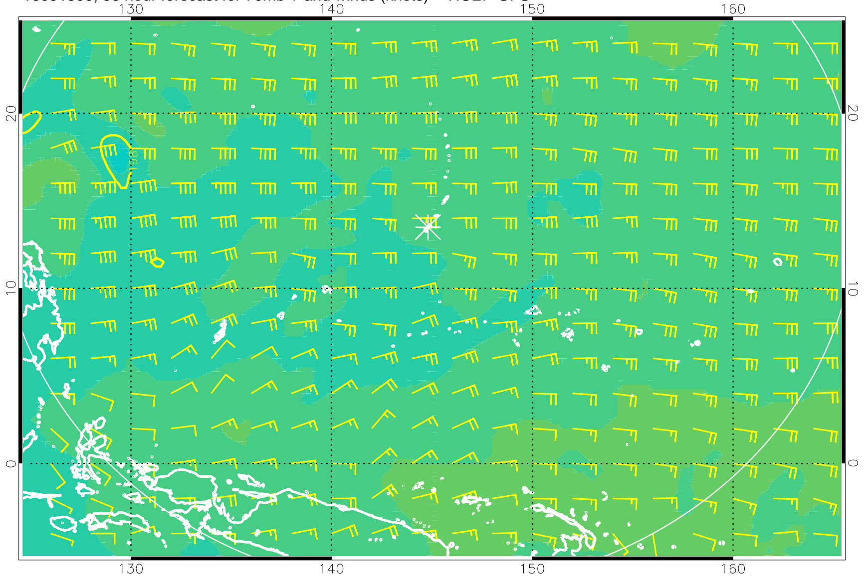
16091500, 96 hour forecast for 70mb T and winds (knots) -- NCEP GFS
