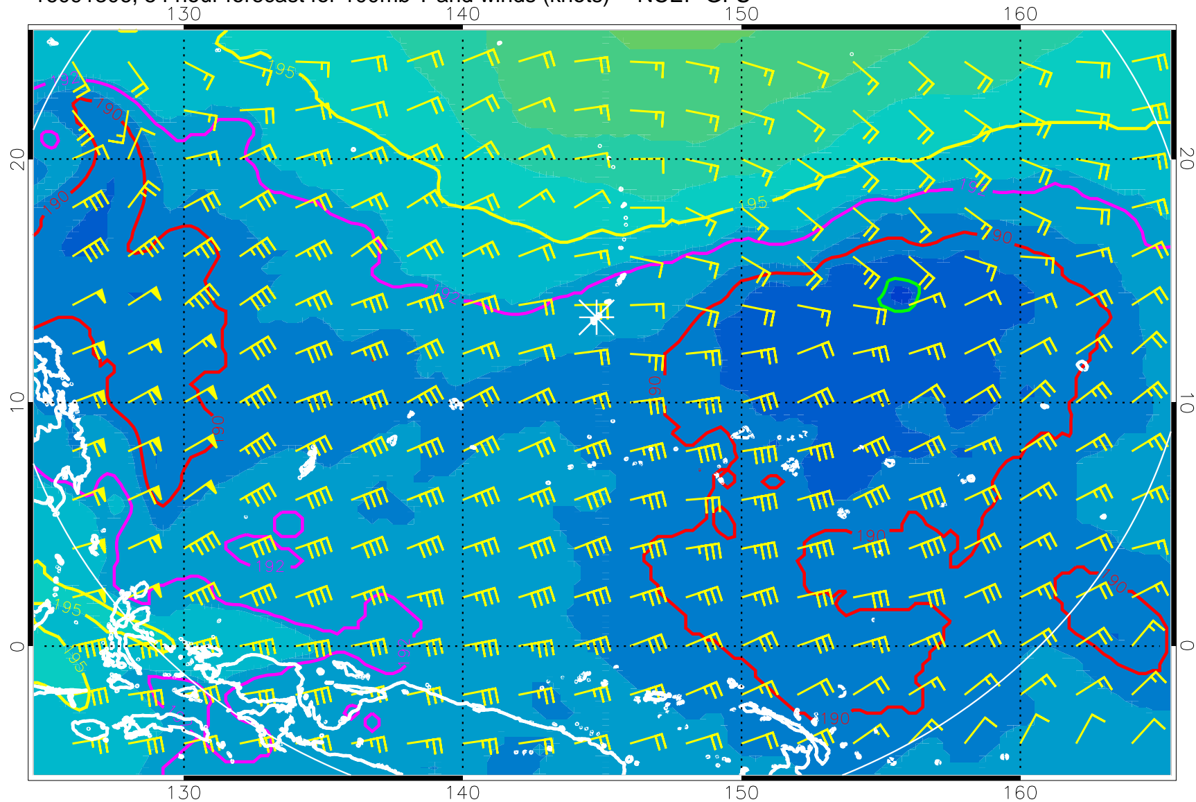
16091306, 54 hour forecast for 100mb T and winds (knots) -- NCEP GFS
