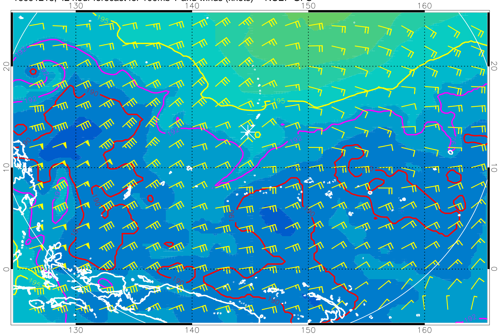
16091218, 42 hour forecast for 100mb T and winds (knots) -- NCEP GFS
