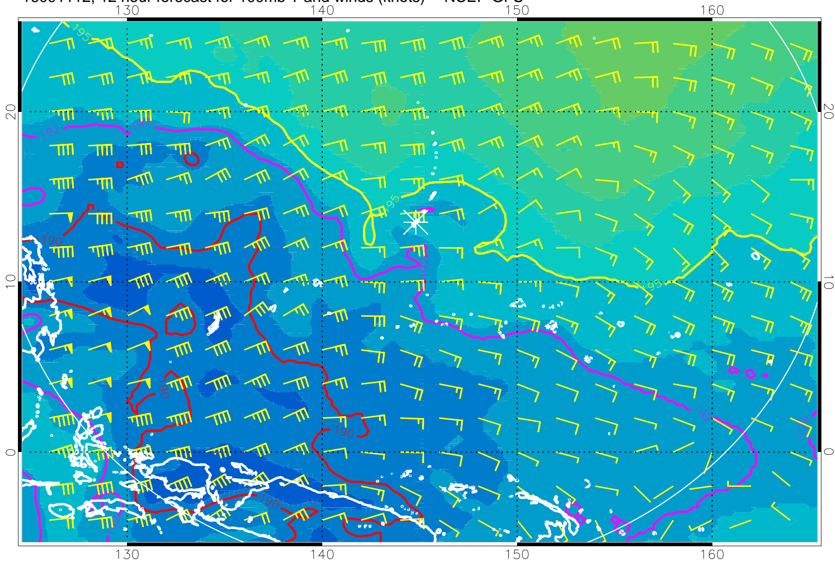
16091112, 12 hour forecast for 100mb T and winds (knots) -- NCEP GFS
