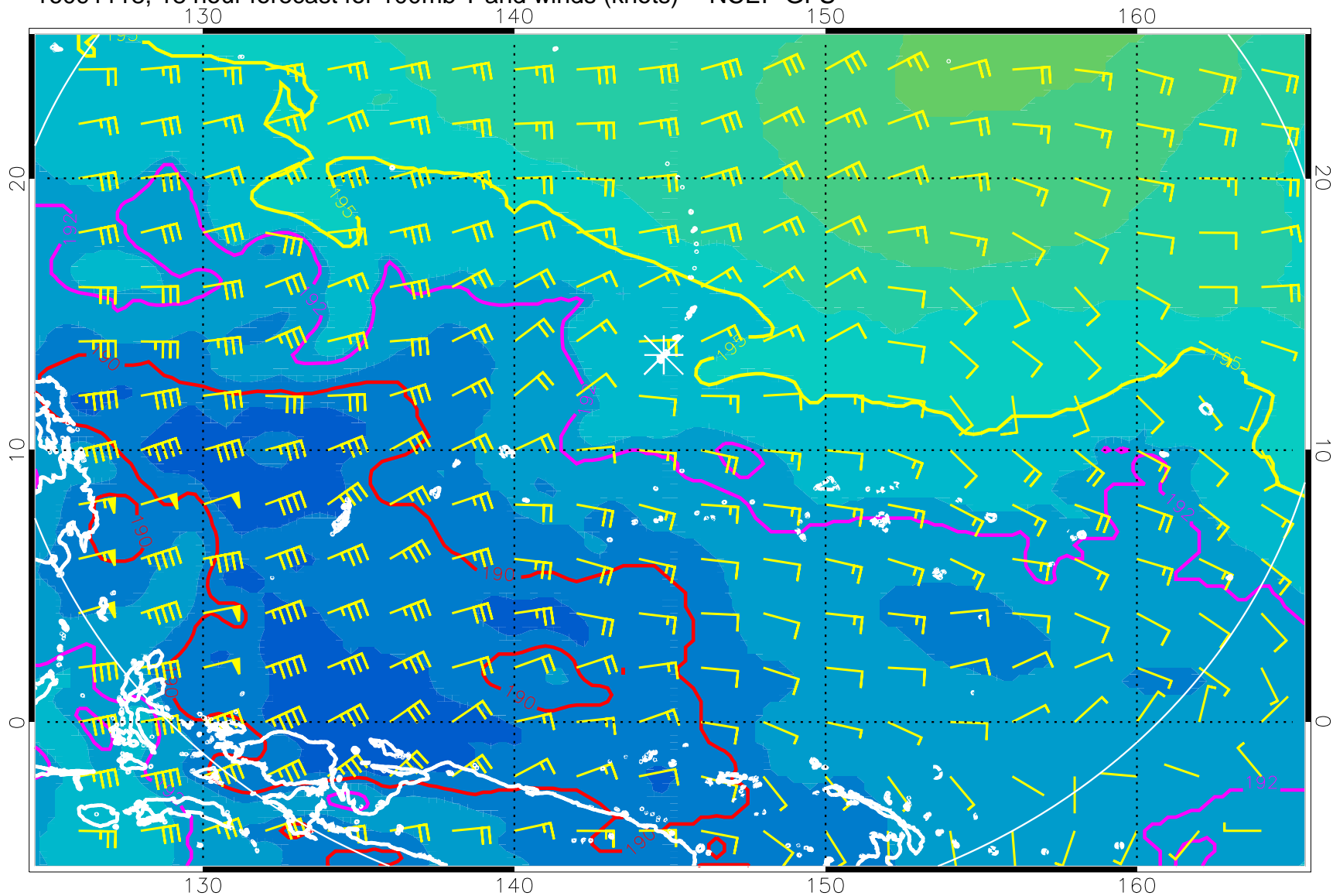
16091118, 18 hour forecast for 100mb T and winds (knots) -- NCEP GFS
