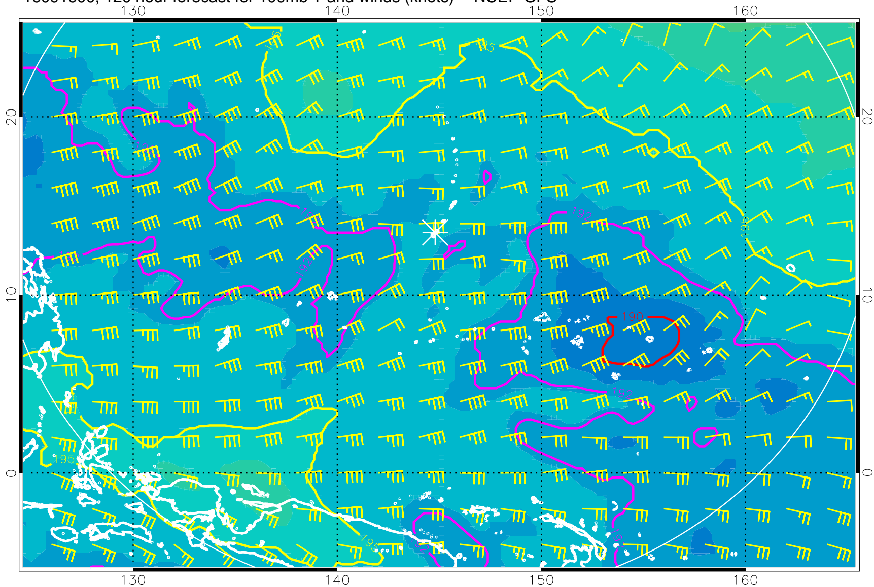
16091600, 120 hour forecast for 100mb T and winds (knots) -- NCEP GFS
