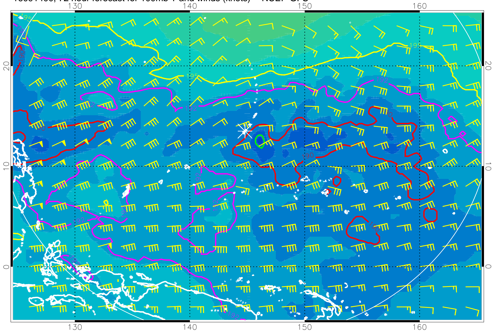
16091400, 72 hour forecast for 100mb T and winds (knots) -- NCEP GFS
