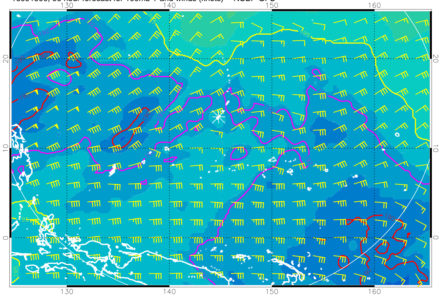
16091500, 96 hour forecast for 100mb T and winds (knots) -- NCEP GFS
