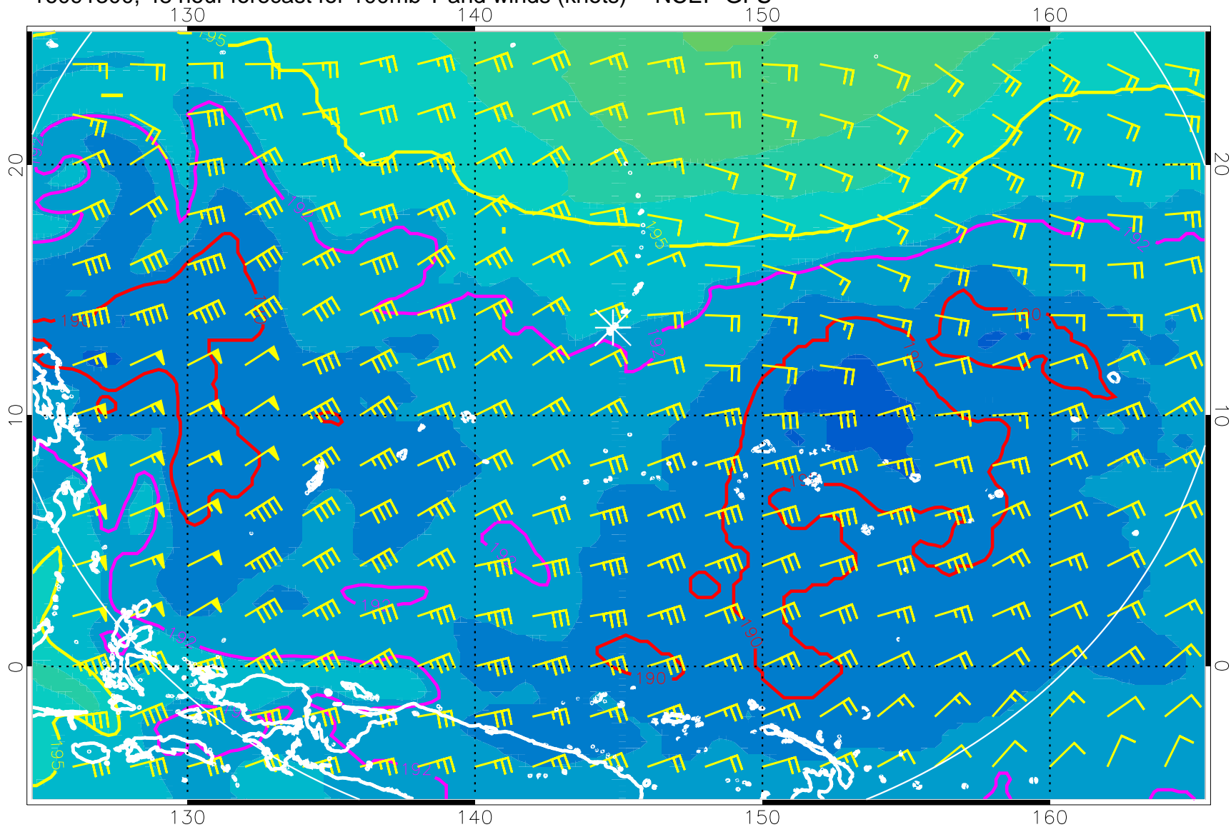
16091300, 48 hour forecast for 100mb T and winds (knots) -- NCEP GFS
