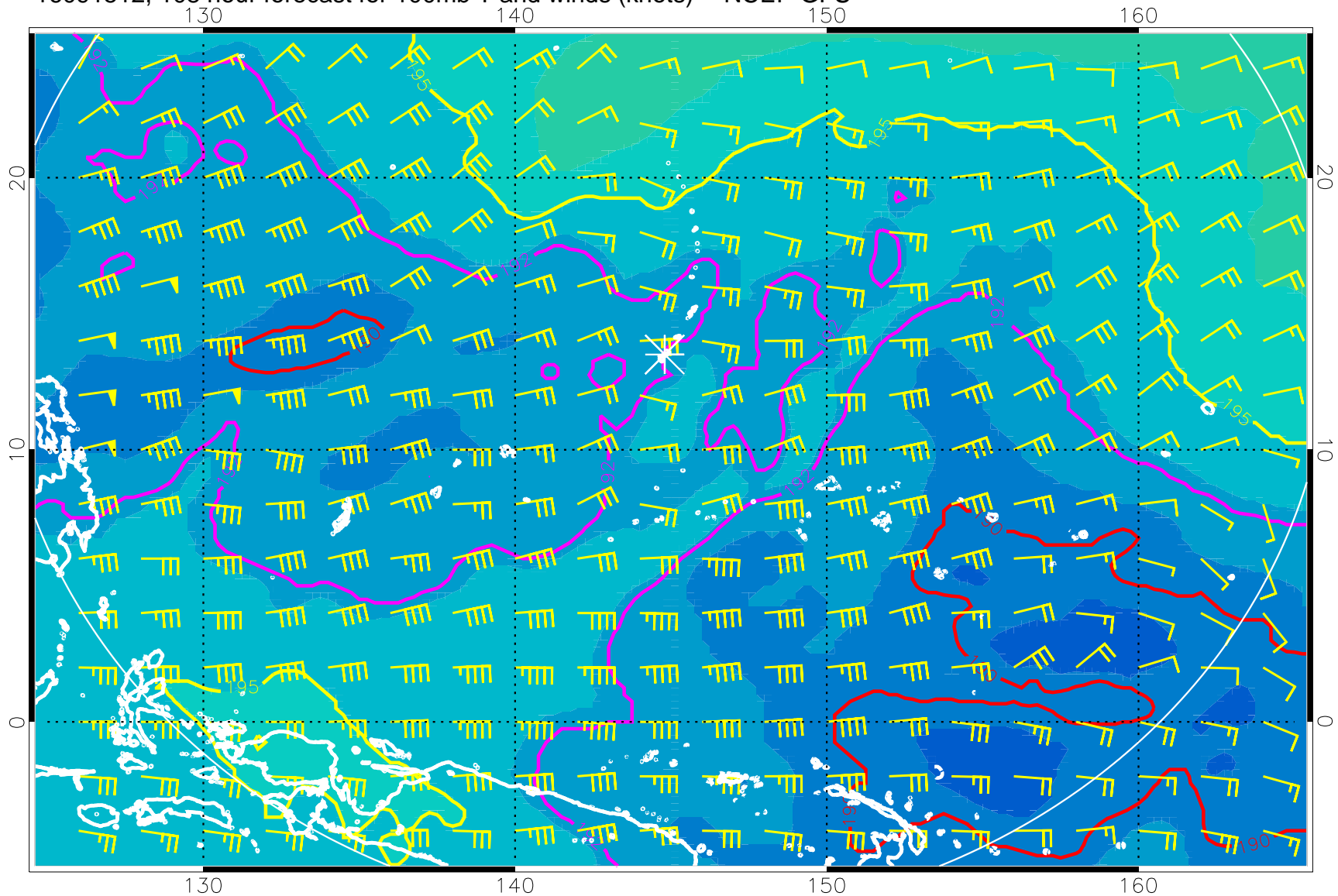
16091512, 108 hour forecast for 100mb T and winds (knots) -- NCEP GFS
