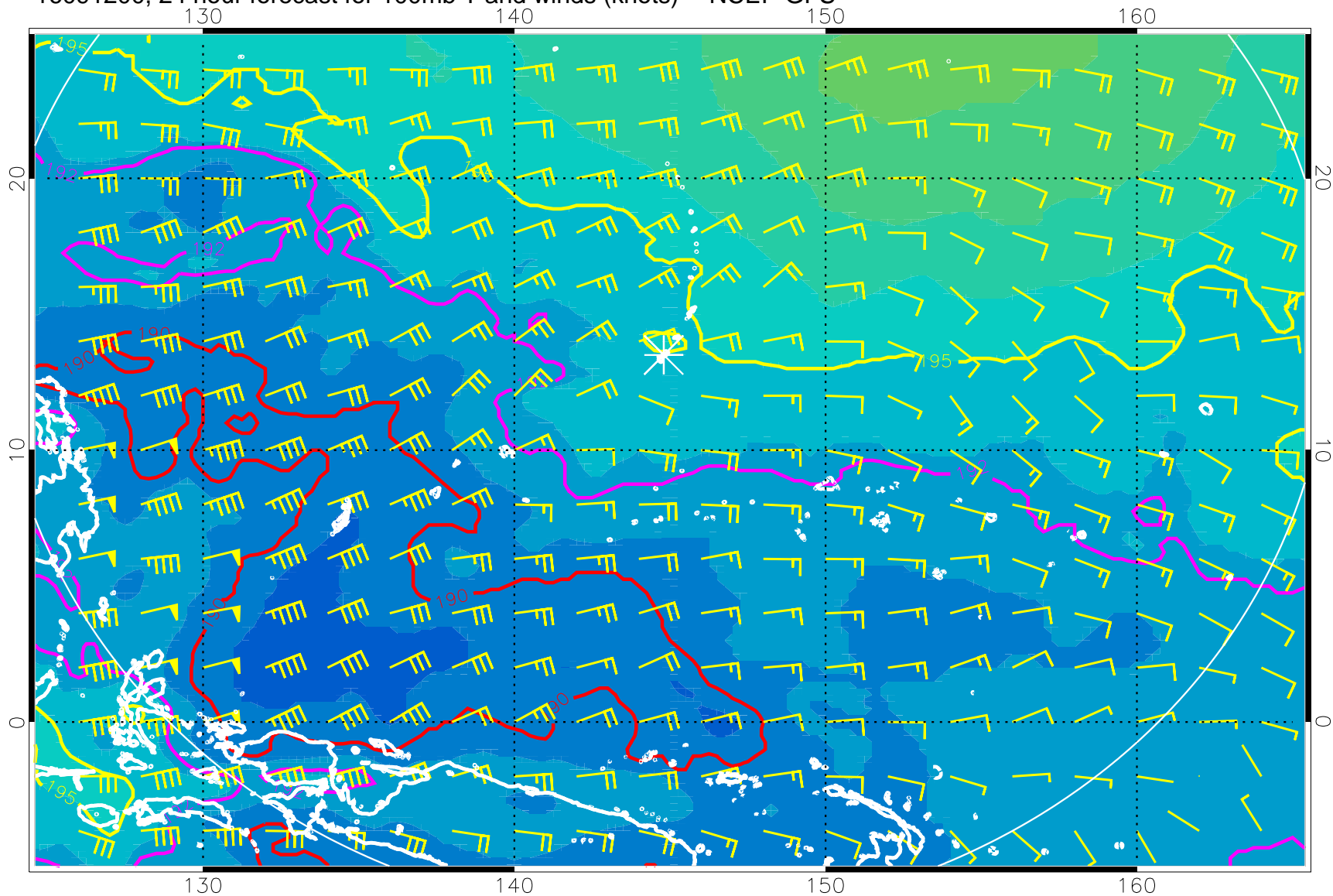
16091200, 24 hour forecast for 100mb T and winds (knots) -- NCEP GFS
