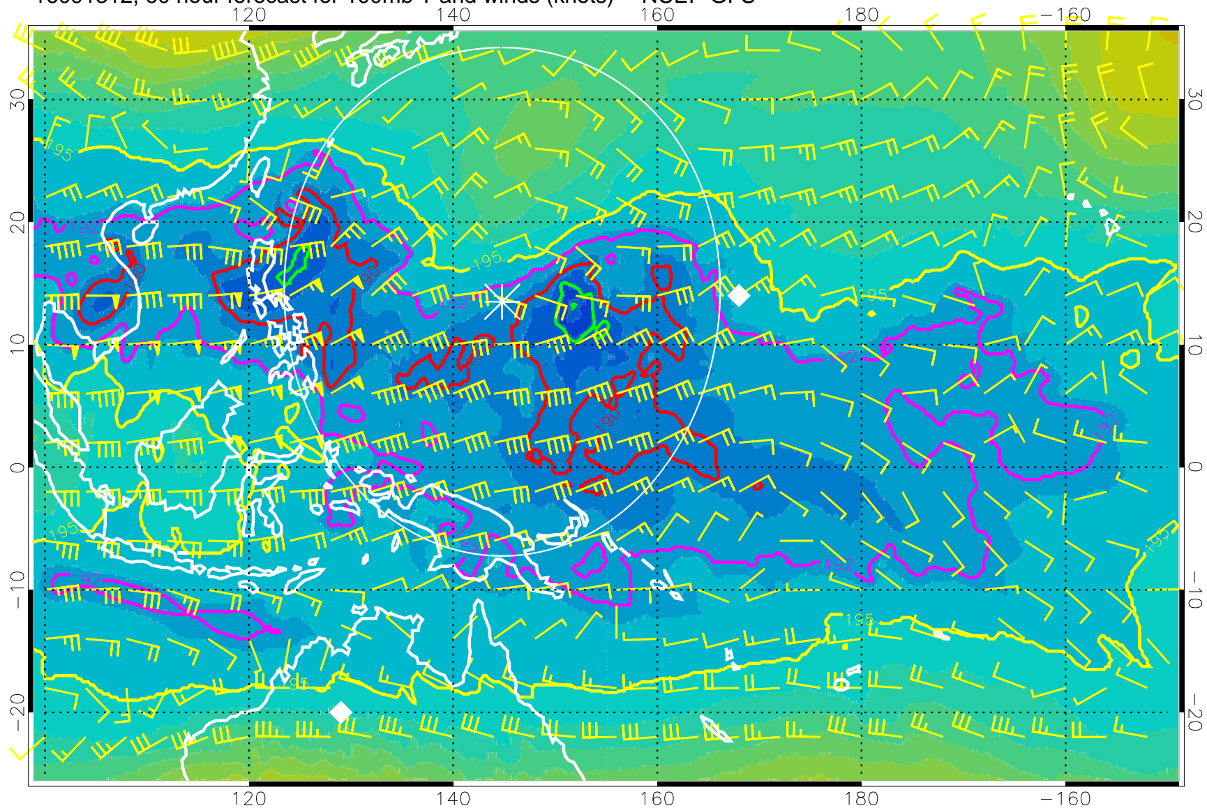
16091312, 60 hour forecast for 100mb T and winds (knots) -- NCEP GFS
