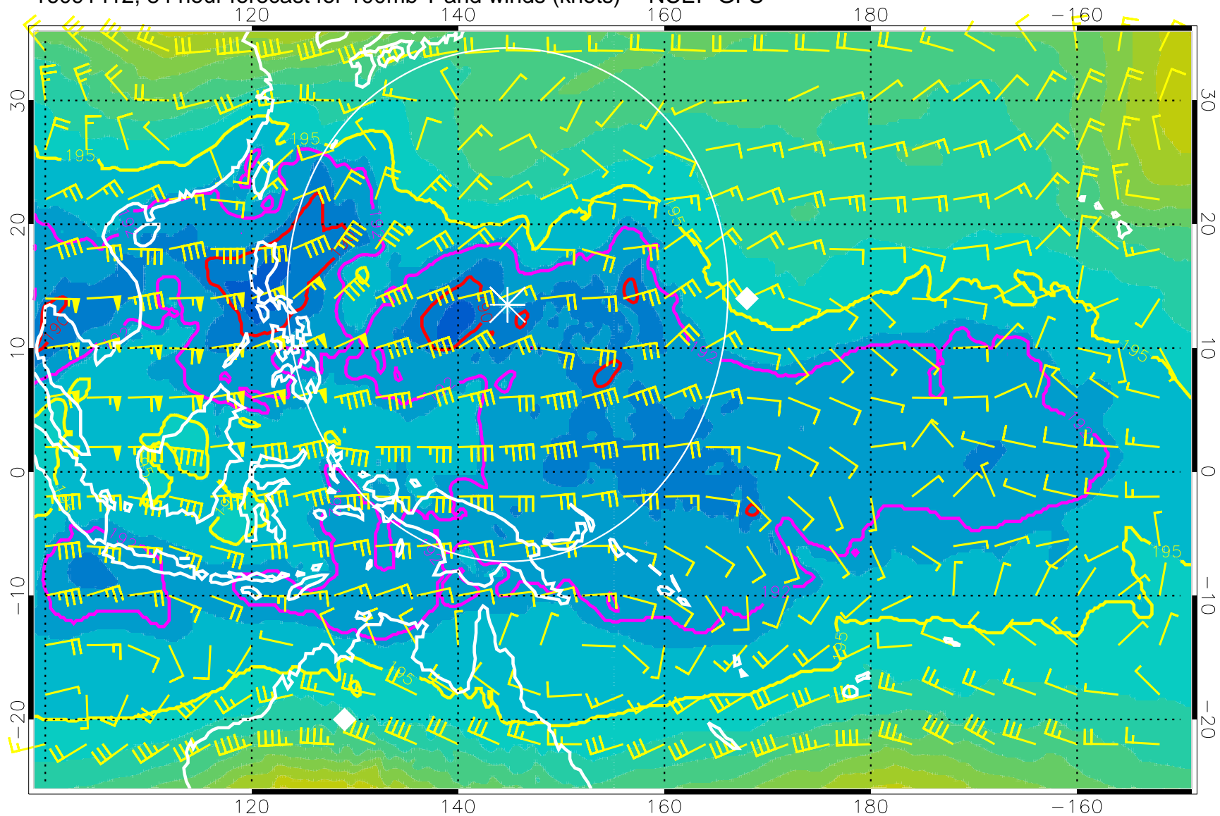
16091412, 84 hour forecast for 100mb T and winds (knots) -- NCEP GFS
