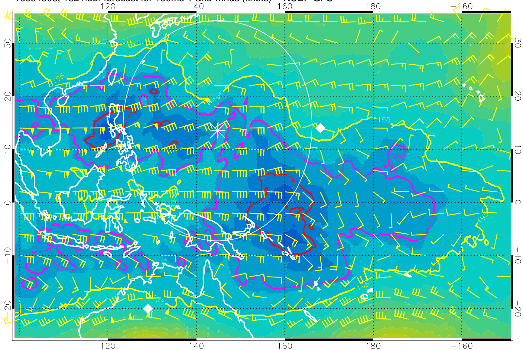
16091506, 102 hour forecast for 100mb T and winds (knots) -- NCEP GFS
