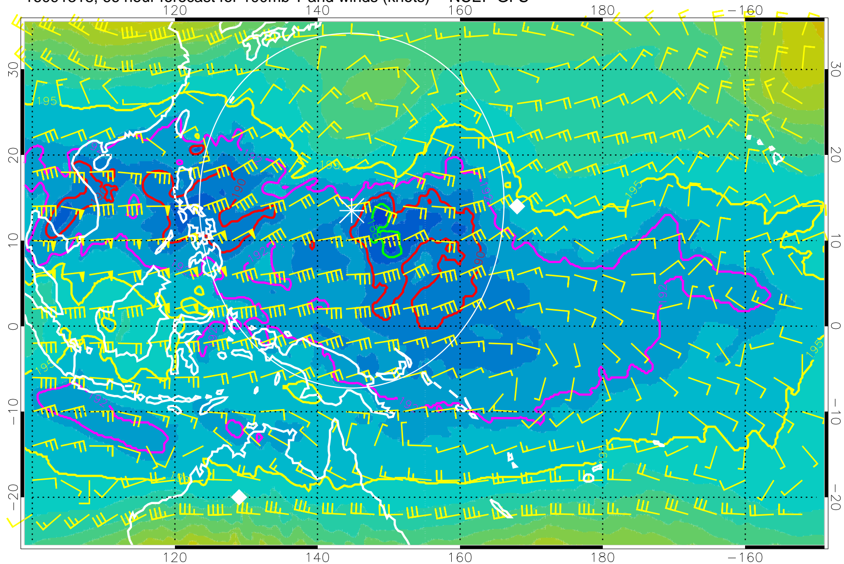
16091318, 66 hour forecast for 100mb T and winds (knots) -- NCEP GFS
