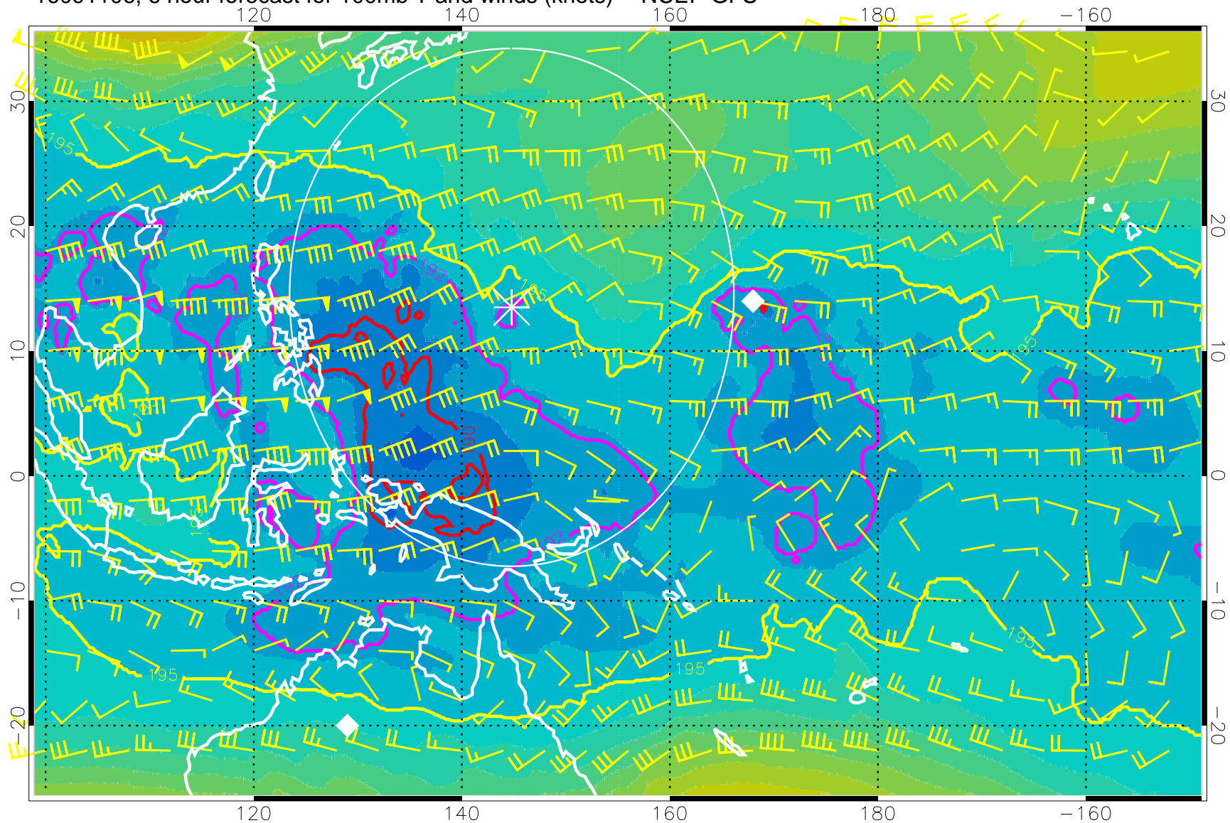
16091106, 6 hour forecast for 100mb T and winds (knots) -- NCEP GFS
