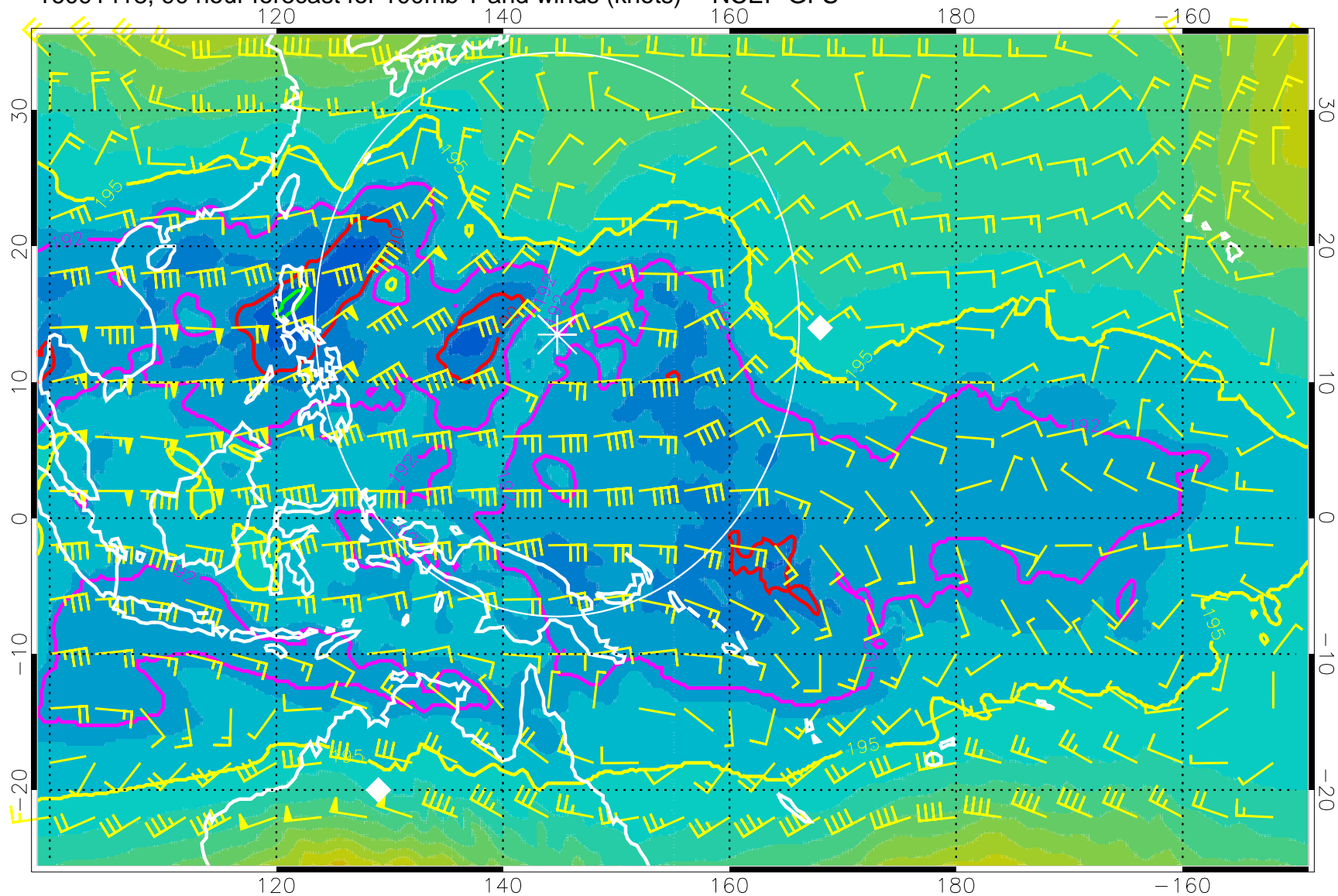
16091418, 90 hour forecast for 100mb T and winds (knots) -- NCEP GFS
