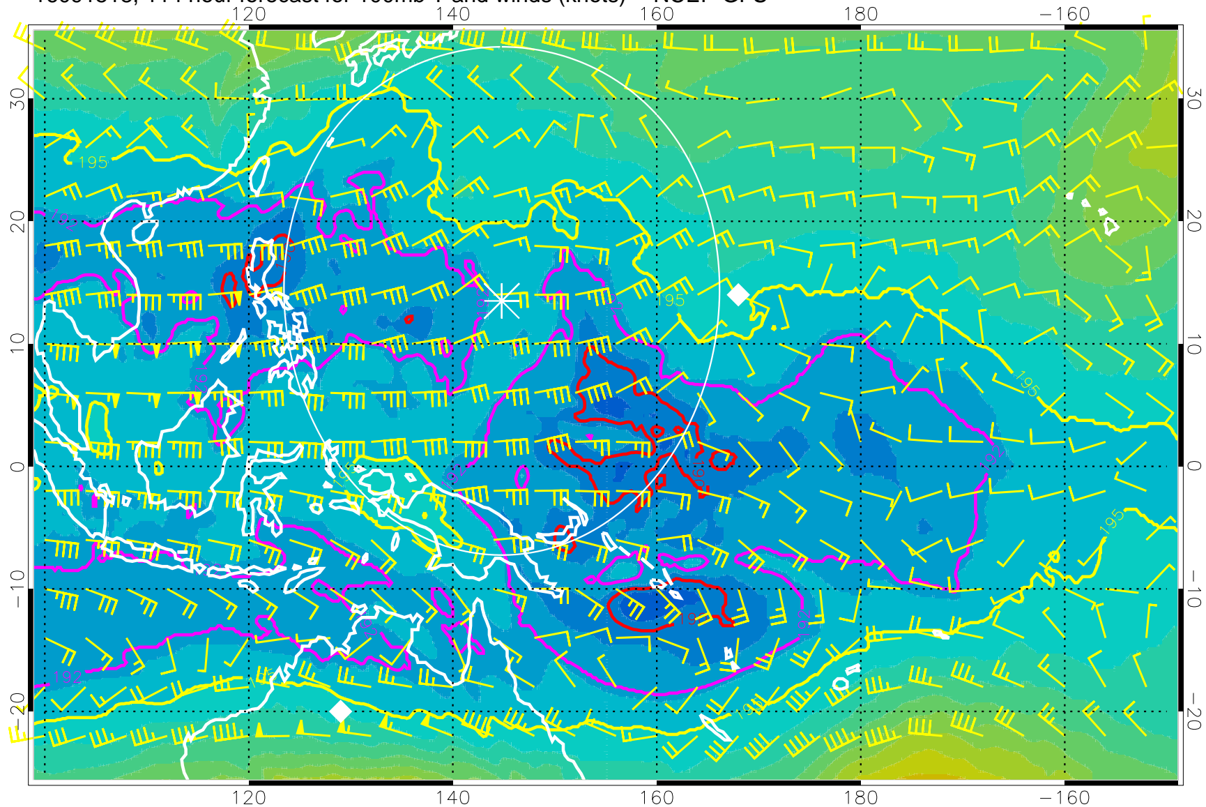
16091518, 114 hour forecast for 100mb T and winds (knots) -- NCEP GFS
