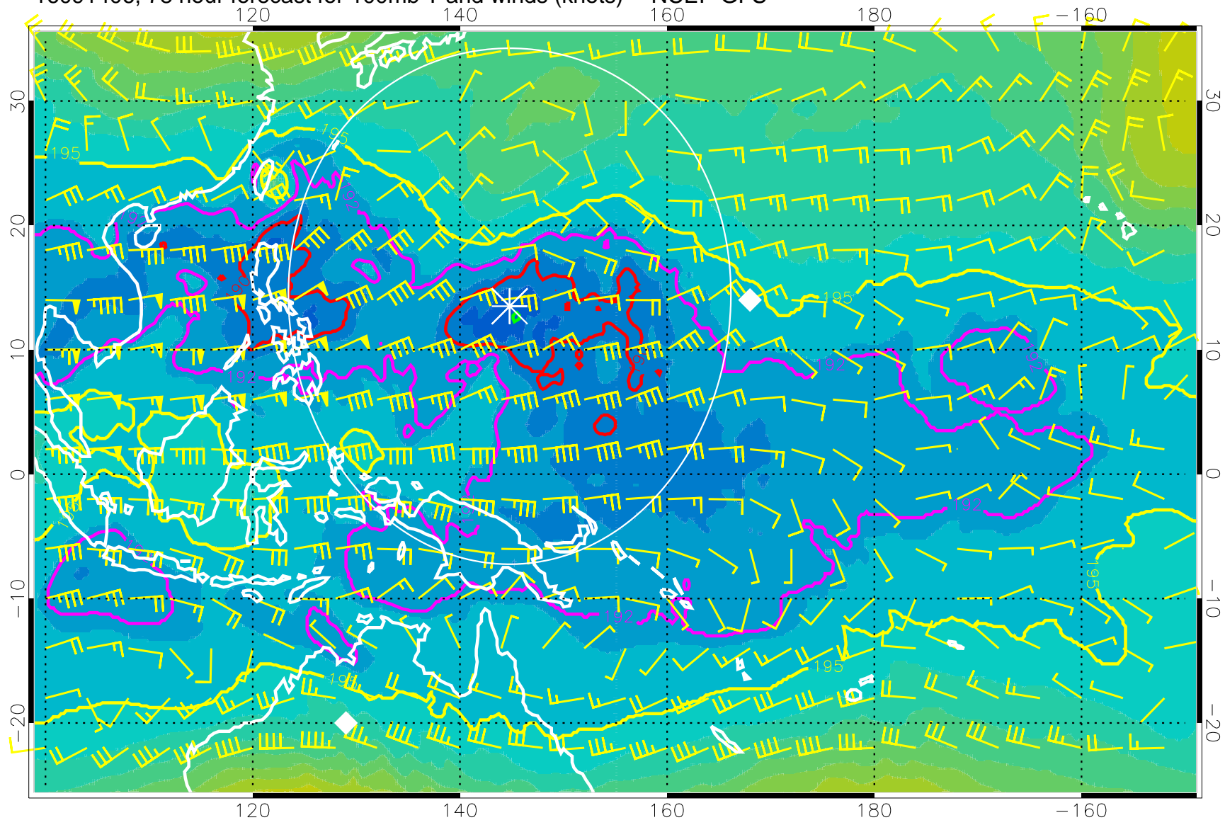
16091406, 78 hour forecast for 100mb T and winds (knots) -- NCEP GFS
