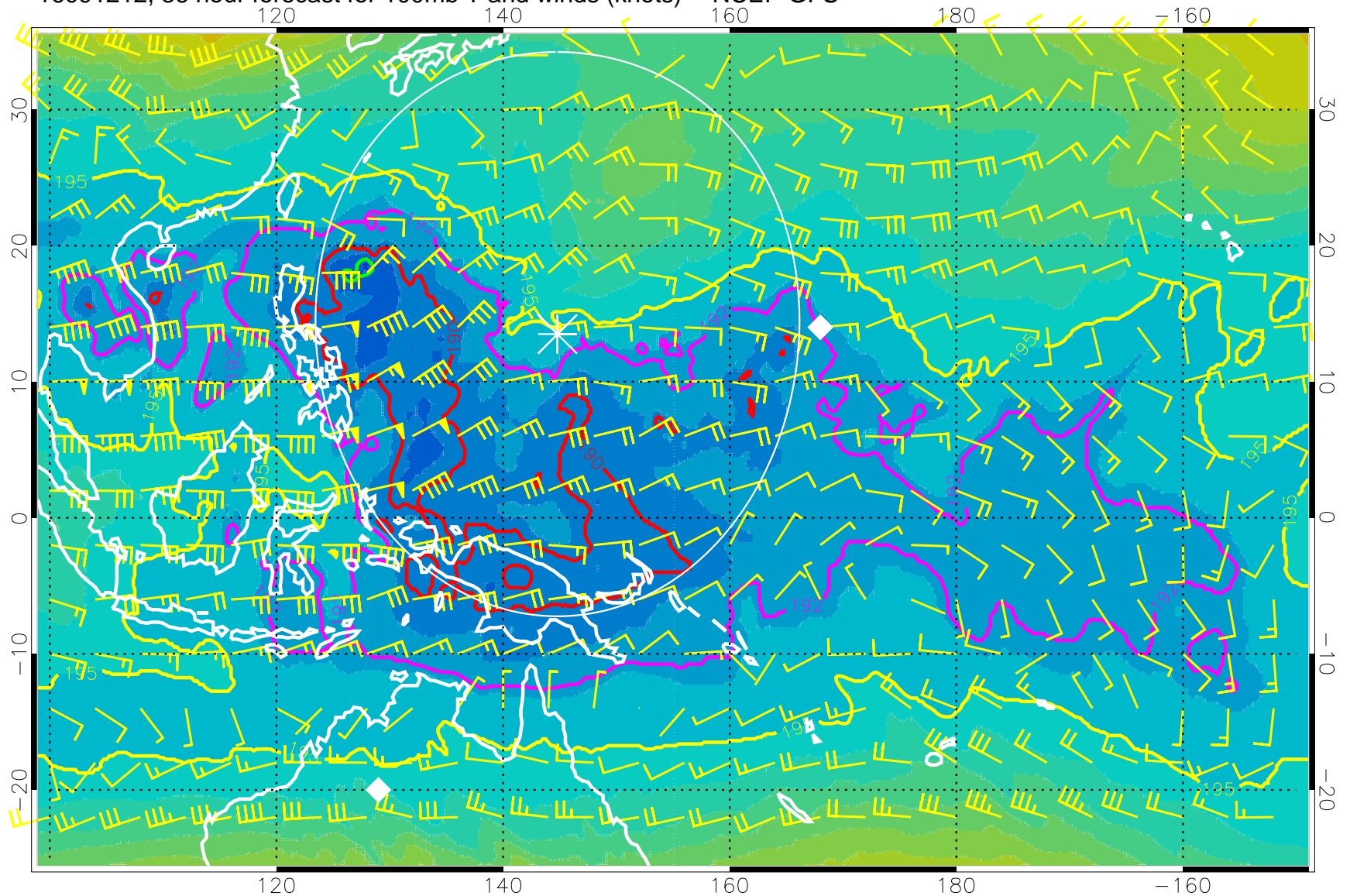
16091212, 36 hour forecast for 100mb T and winds (knots) -- NCEP GFS
