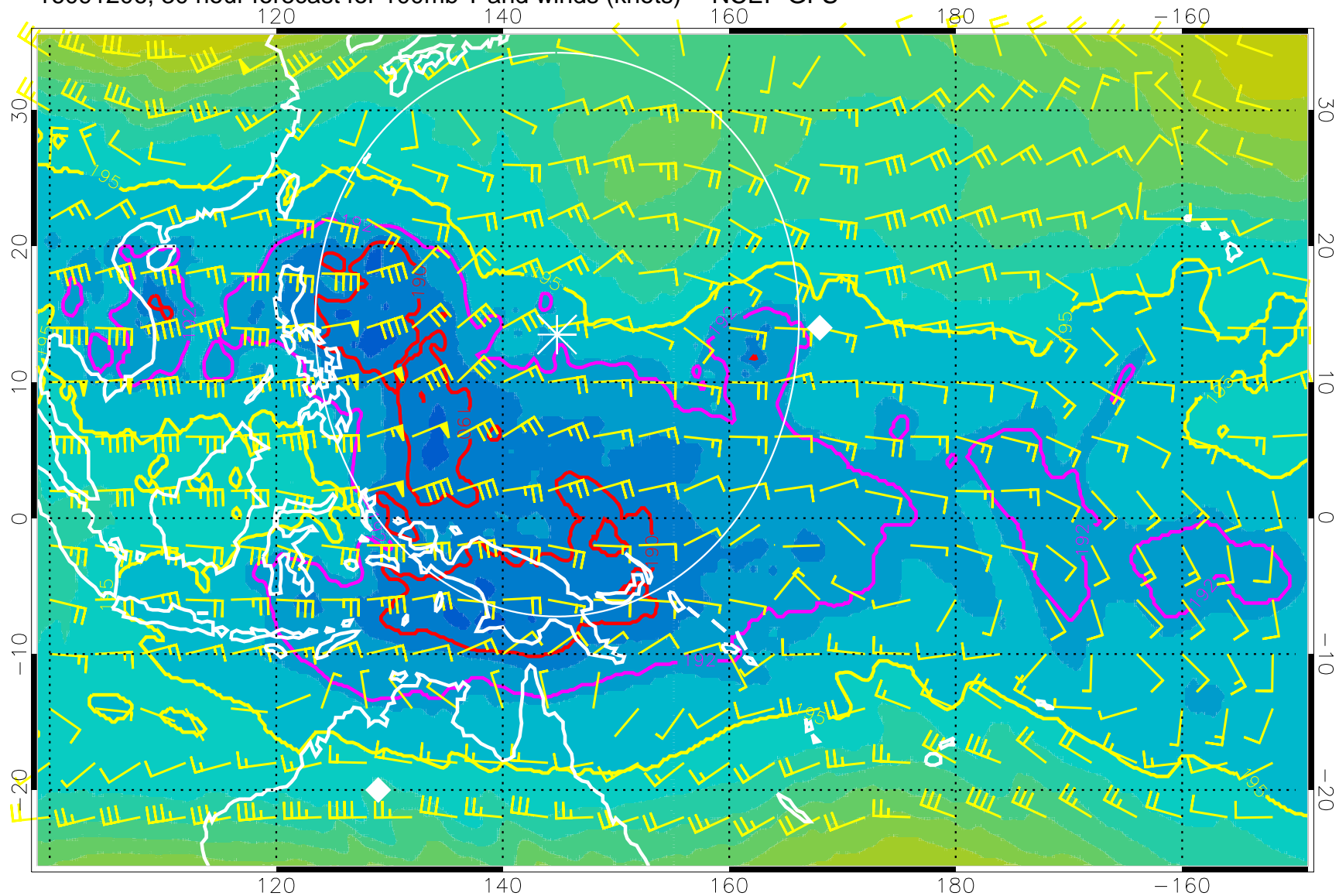
16091206, 30 hour forecast for 100mb T and winds (knots) -- NCEP GFS
