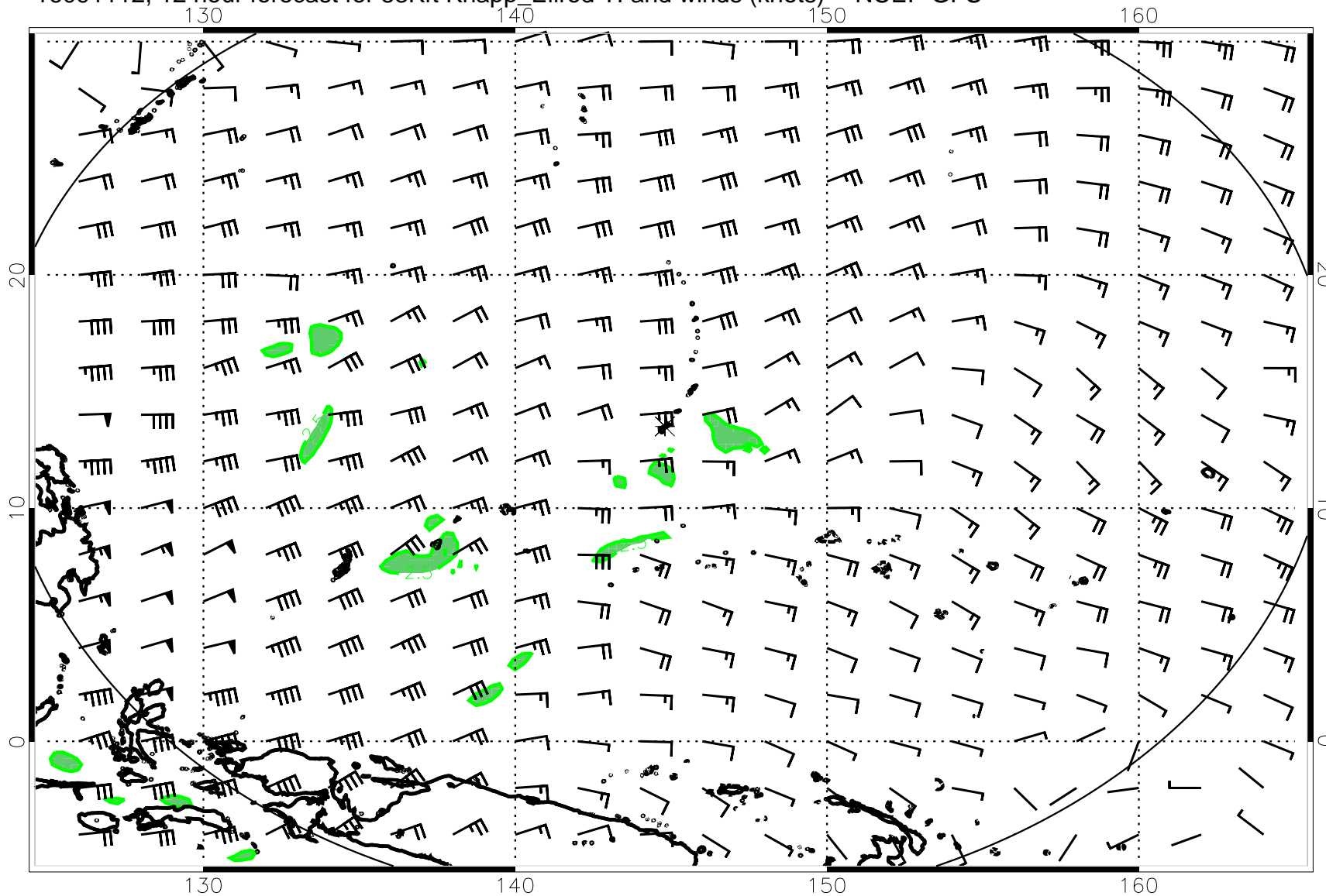
16091112, 12 hour forecast for 53Kft Knapp_Ellrod TI and winds (knots) -- NCEP GFS
