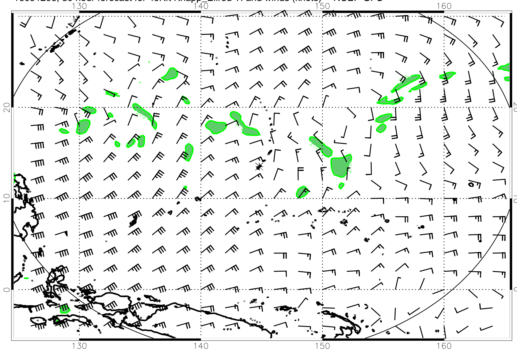
16091206, 30 hour forecast for 49Kft Knapp_Ellrod TI and winds (knots) -- NCEP GFS
