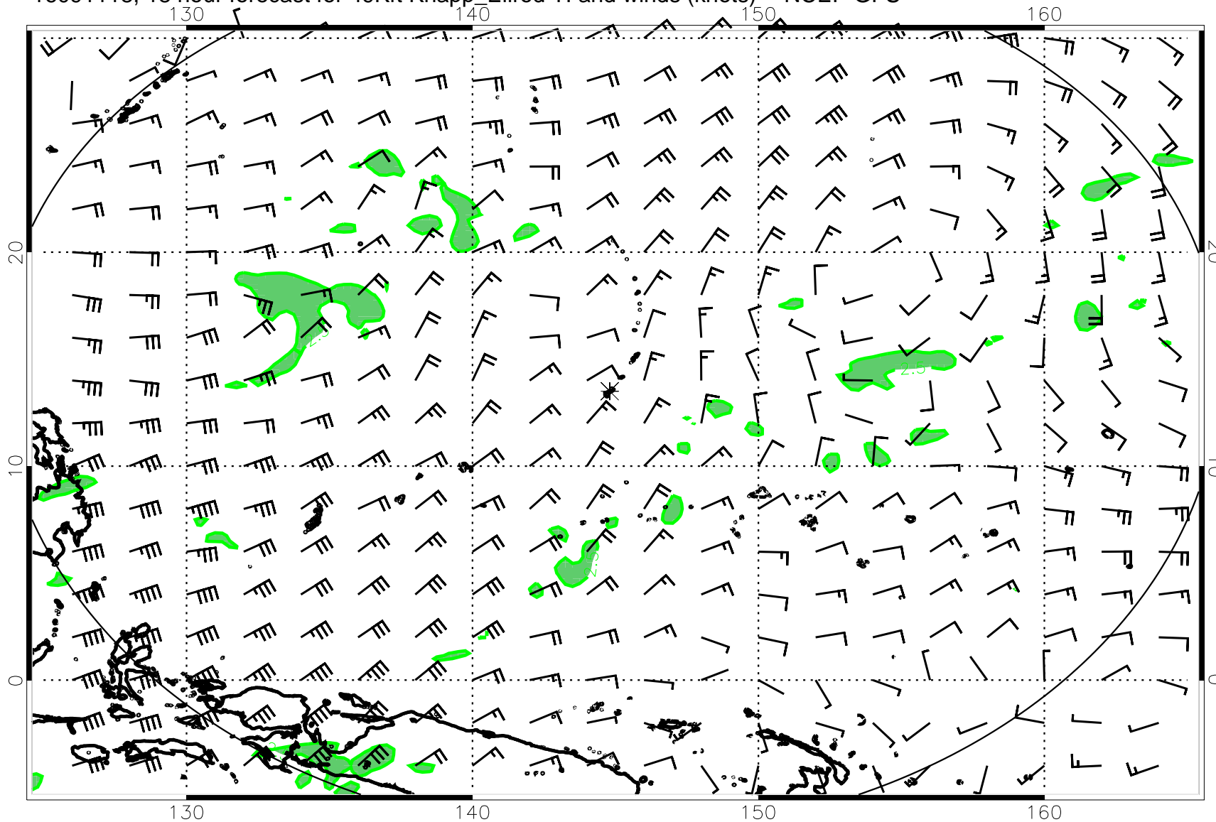
16091118, 18 hour forecast for 49Kft Knapp_Ellrod TI and winds (knots) -- NCEP GFS
