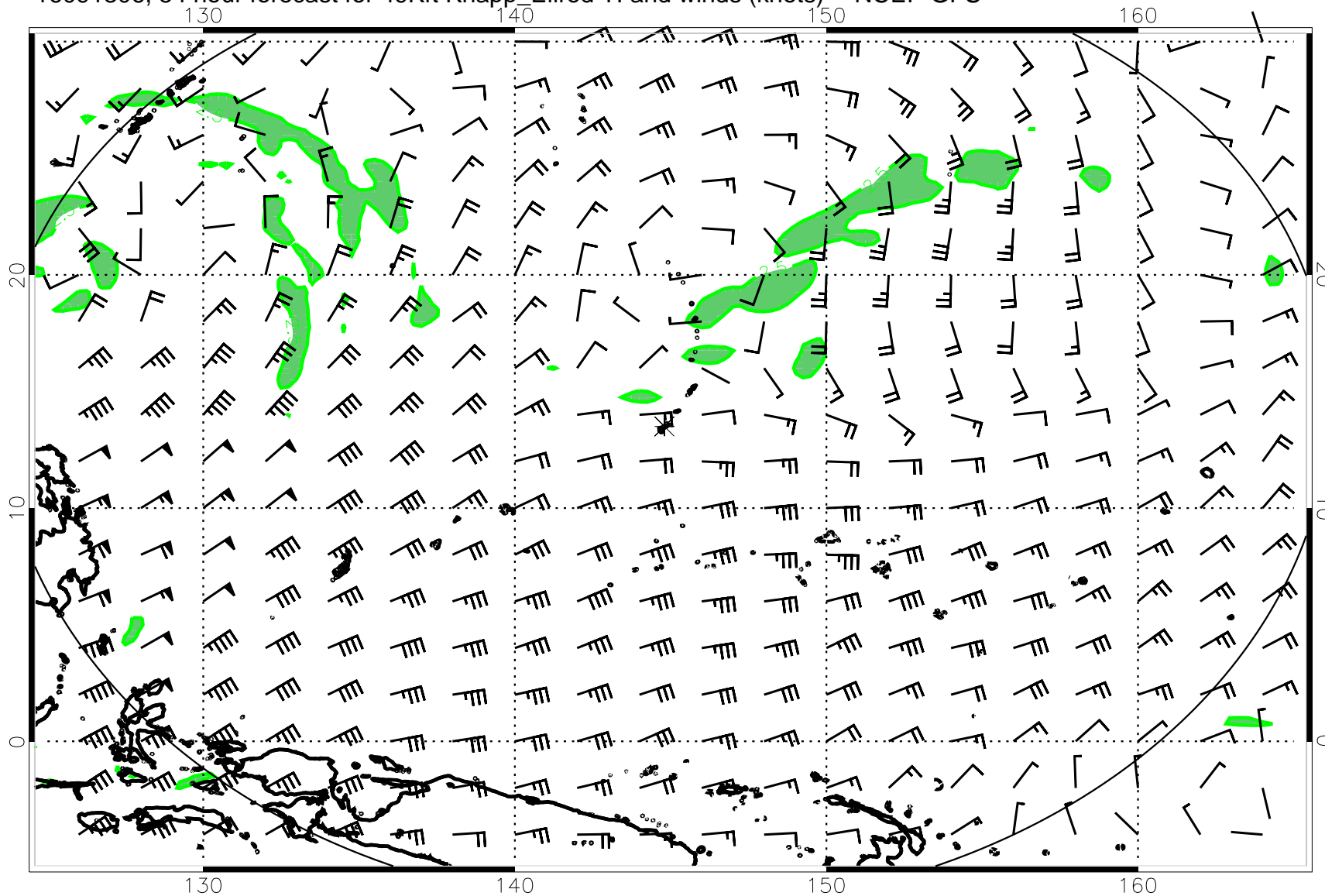
16091306, 54 hour forecast for 49Kft Knapp_Ellrod TI and winds (knots) -- NCEP GFS
