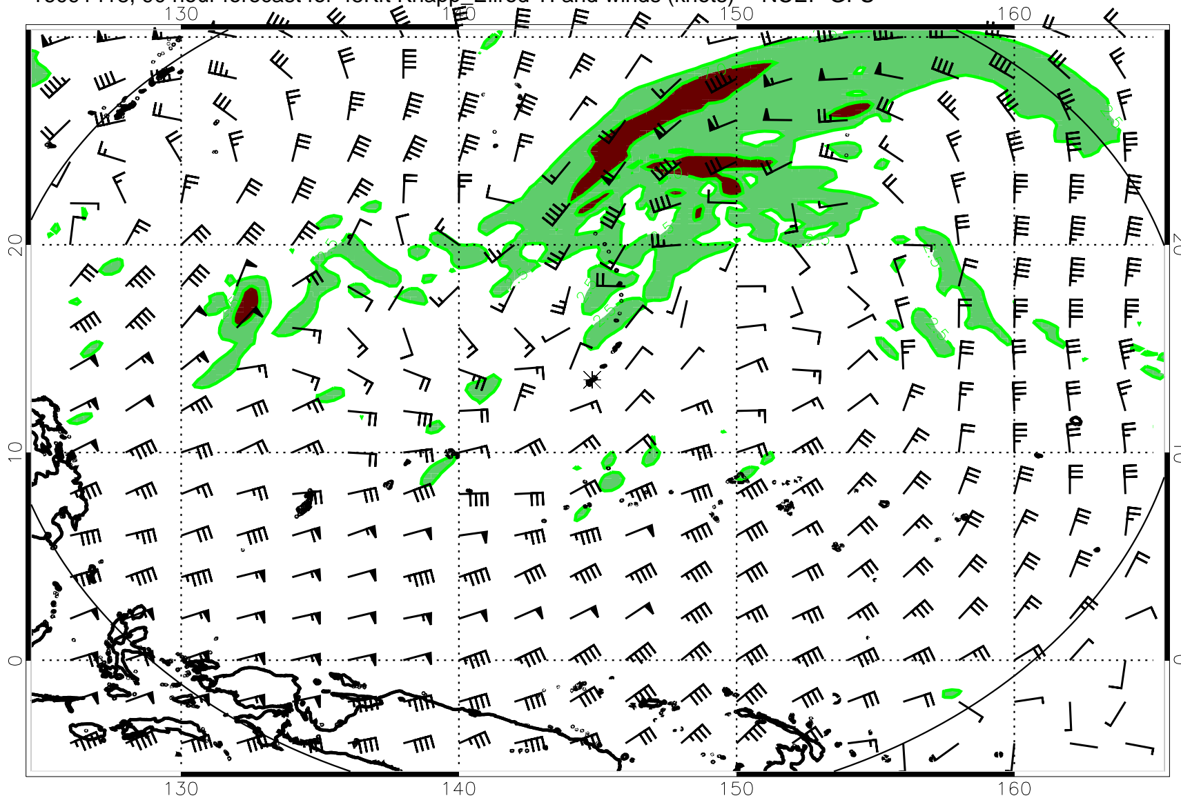
16091418, 90 hour forecast for 45Kft Knapp_Ellrod TI and winds (knots) -- NCEP GFS
