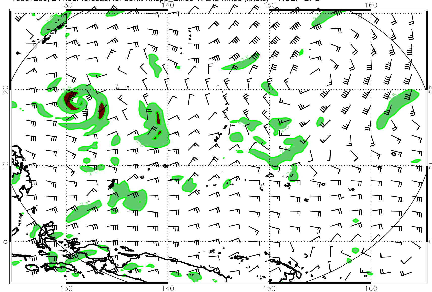
16091200, 24 hour forecast for 36Kft Knapp_Ellrod TI and winds (knots) -- NCEP GFS
