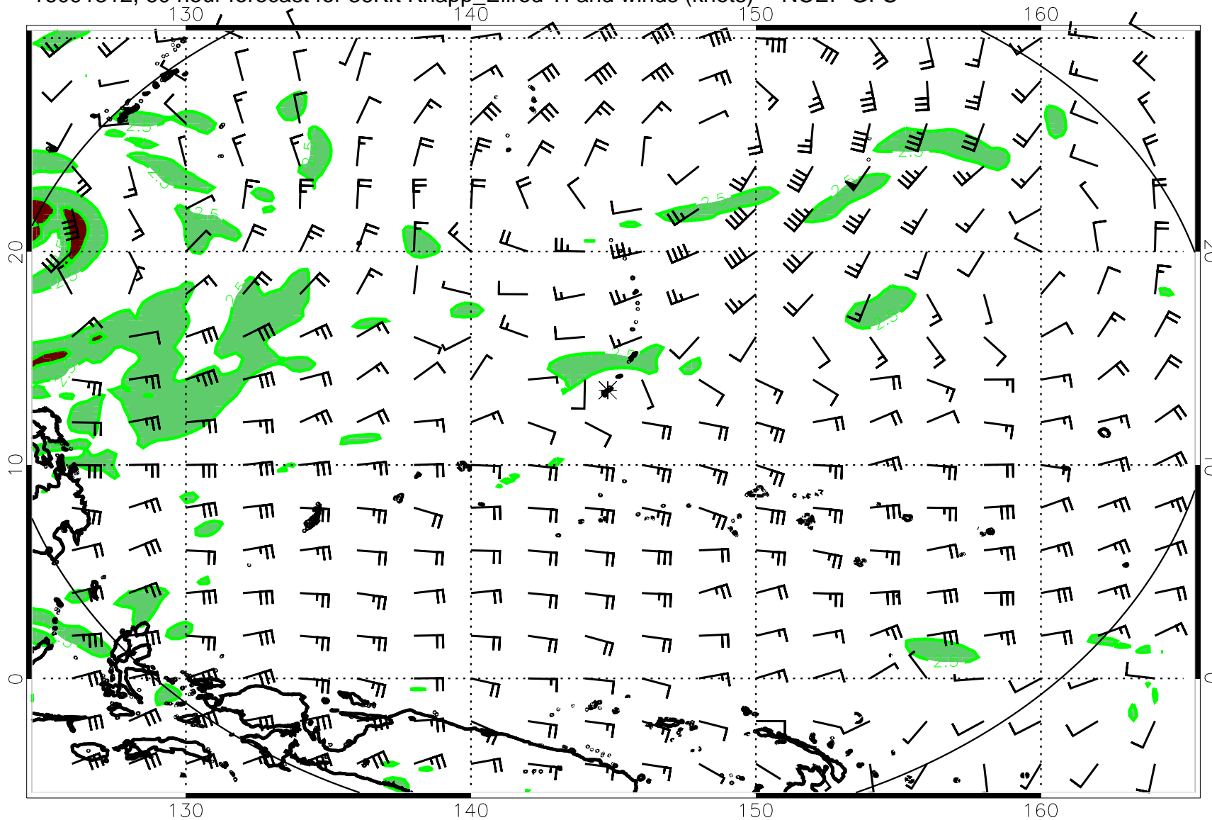
16091312, 60 hour forecast for 36Kft Knapp_Ellrod TI and winds (knots) -- NCEP GFS
