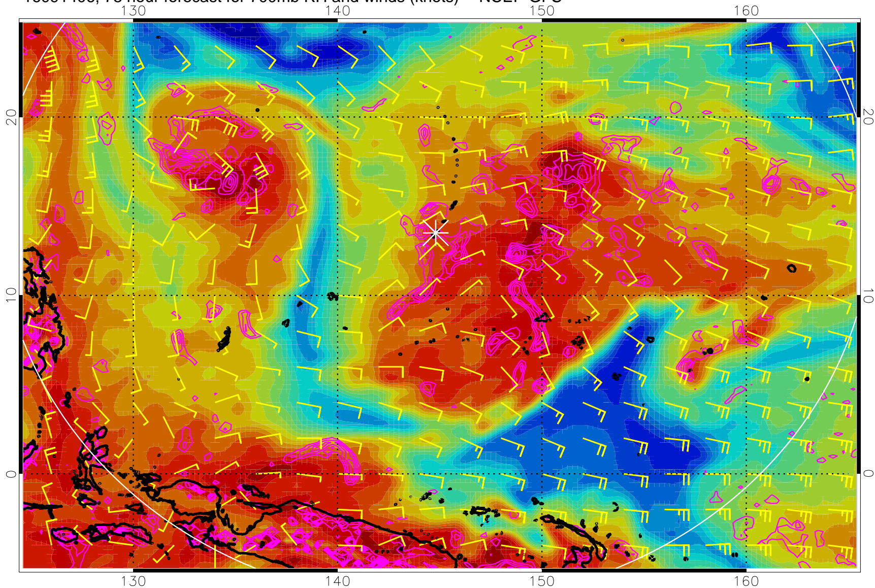
16091406, 78 hour forecast for 700mb RH and winds (knots) -- NCEP GFS
