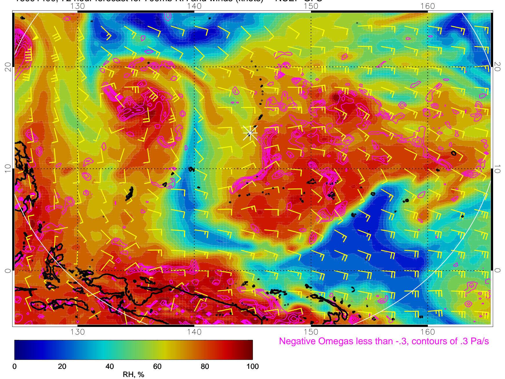
16091400, 72 hour forecast for 700mb RH and winds (knots) -- NCEP GFS
