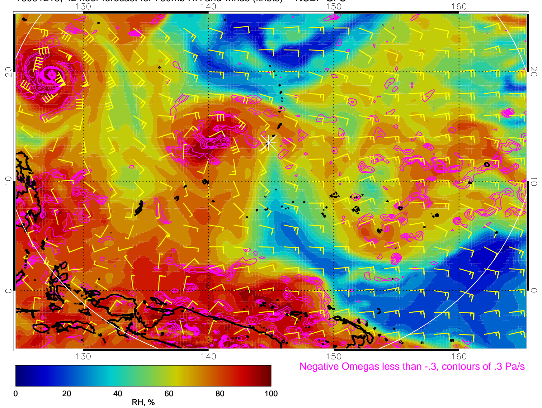
16091218, 42 hour forecast for 700mb RH and winds (knots) -- NCEP GFS
