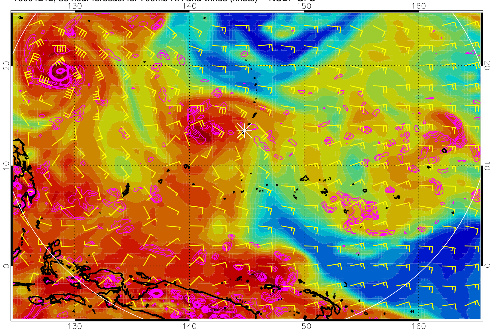
16091212, 36 hour forecast for 700mb RH and winds (knots) -- NCEP GFS
