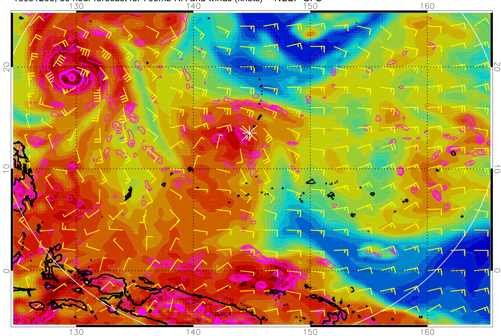
16091206, 30 hour forecast for 700mb RH and winds (knots) -- NCEP GFS
