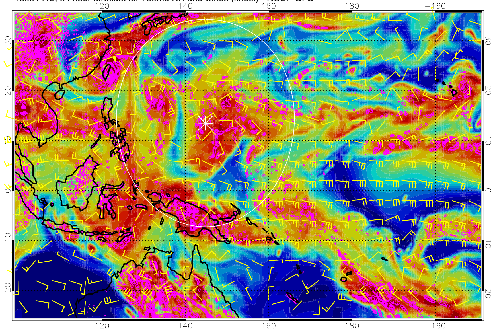
16091412, 84 hour forecast for 700mb RH and winds (knots) - NCEP GFS
