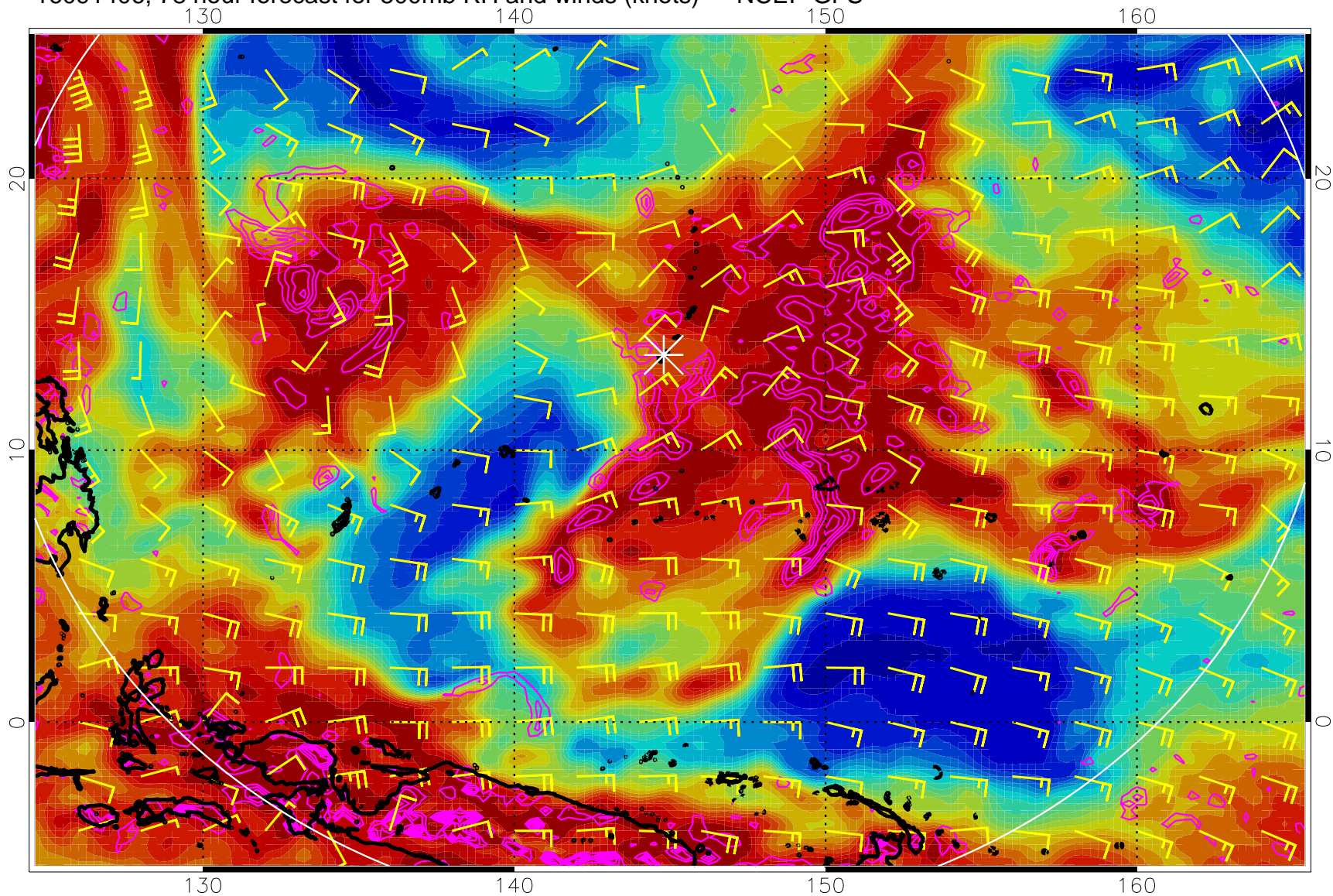
16091406, 78 hour forecast for 500mb RH and winds (knots) -- NCEP GFS
