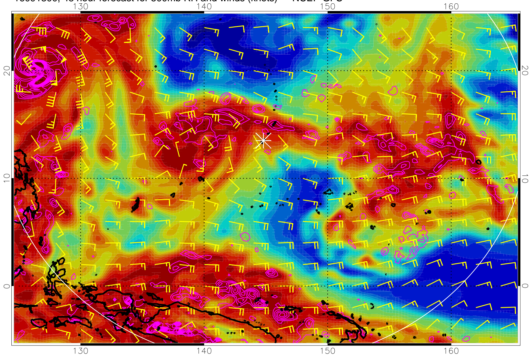
16091300, 48 hour forecast for 500mb RH and winds (knots) -- NCEP GFS
