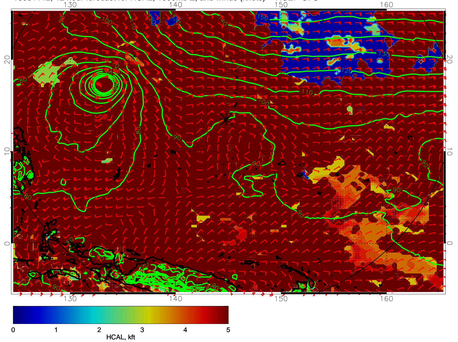
16091112, 12 hour forecast for HCAL, 1000mb Z, and winds (knots) -- NCEP GFS
