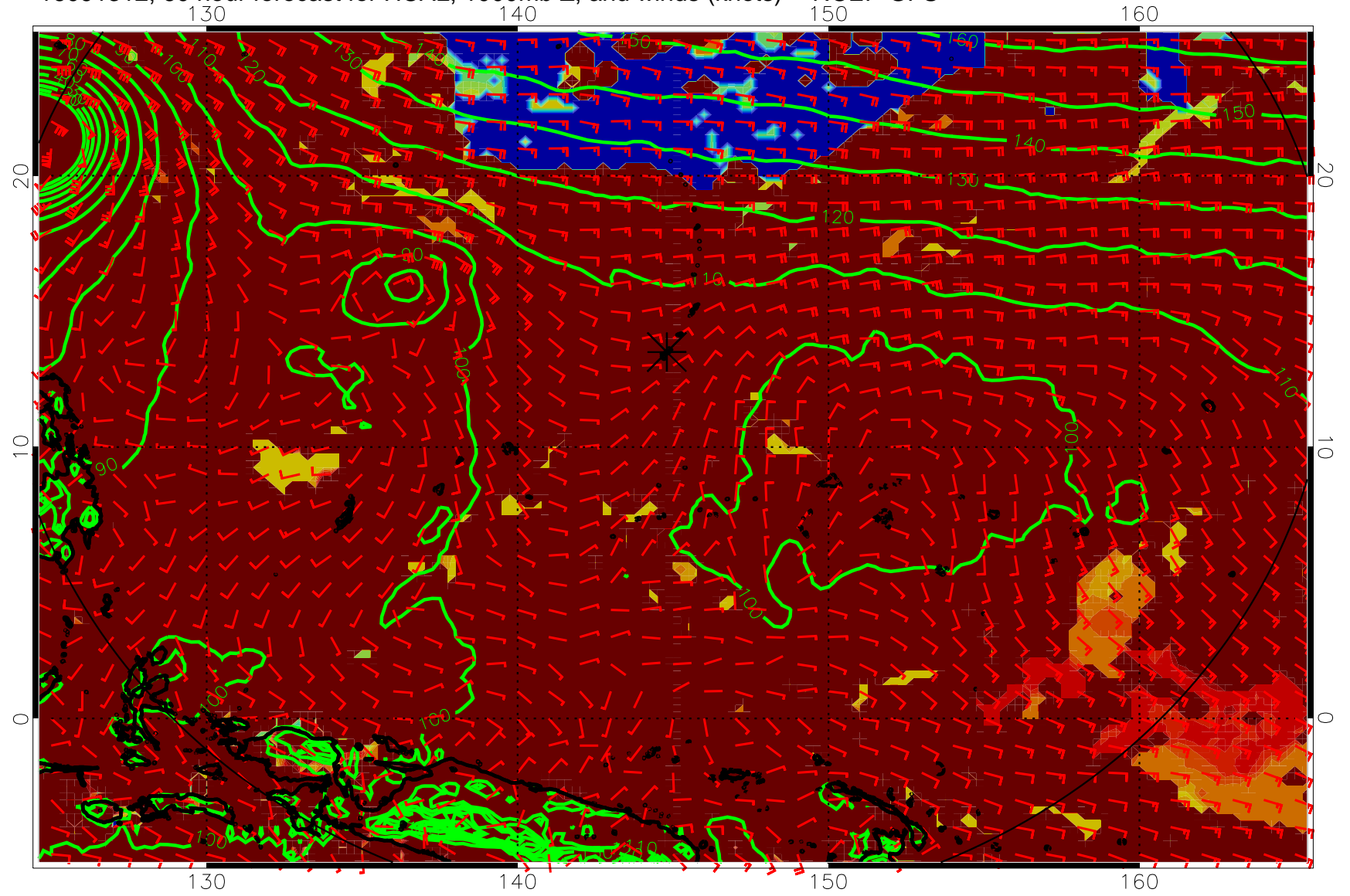
16091312, 60 hour forecast for HCAL, 1000mb Z, and winds (knots) -- NCEP GFS
