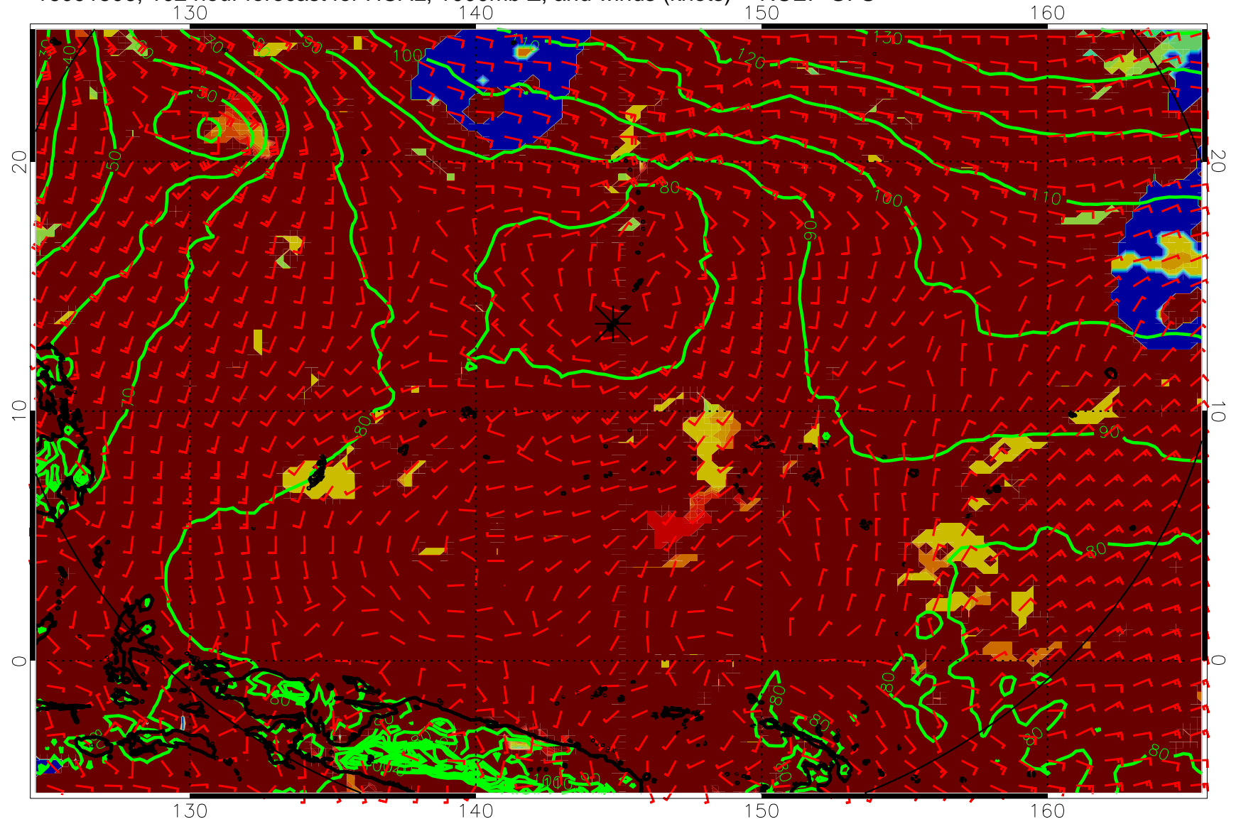
16091506, 102 hour forecast for HCAL, 1000mb Z, and winds (knots) -- NCEP GFS
