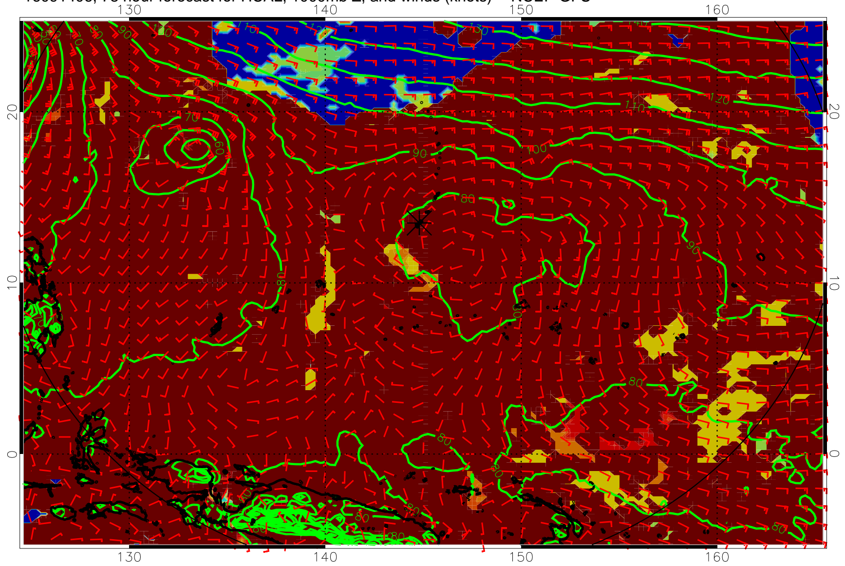
16091406, 78 hour forecast for HCAL, 1000mb Z, and winds (knots) -- NCEP GFS
