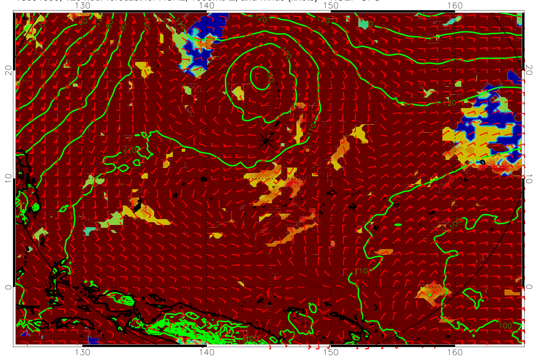
16091600, 120 hour forecast for HCAL, 1000mb Z, and winds (knots) -- NCEP GFS
