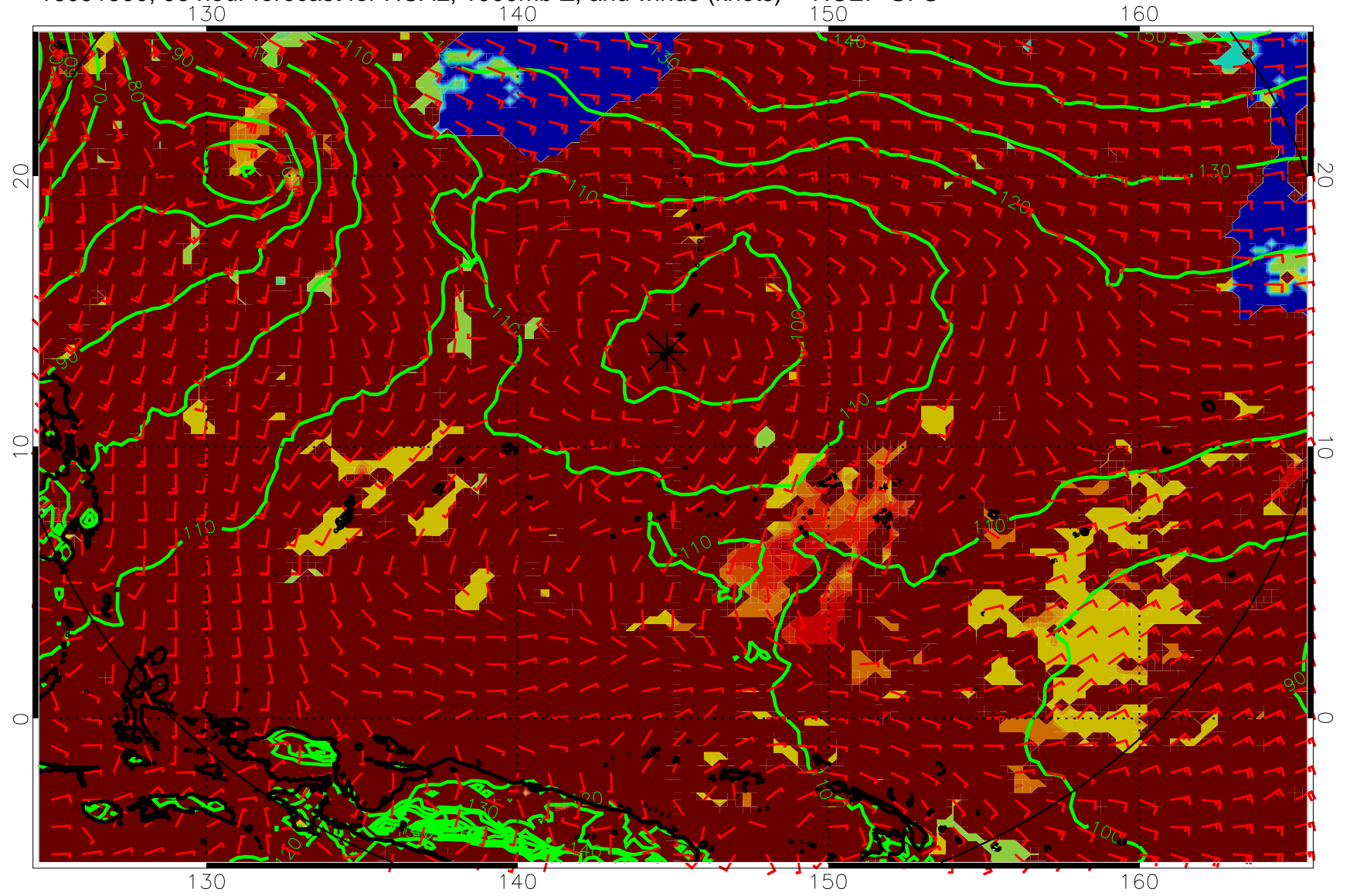
16091500, 96 hour forecast for HCAL, 1000mb Z, and winds (knots) -- NCEP GFS
