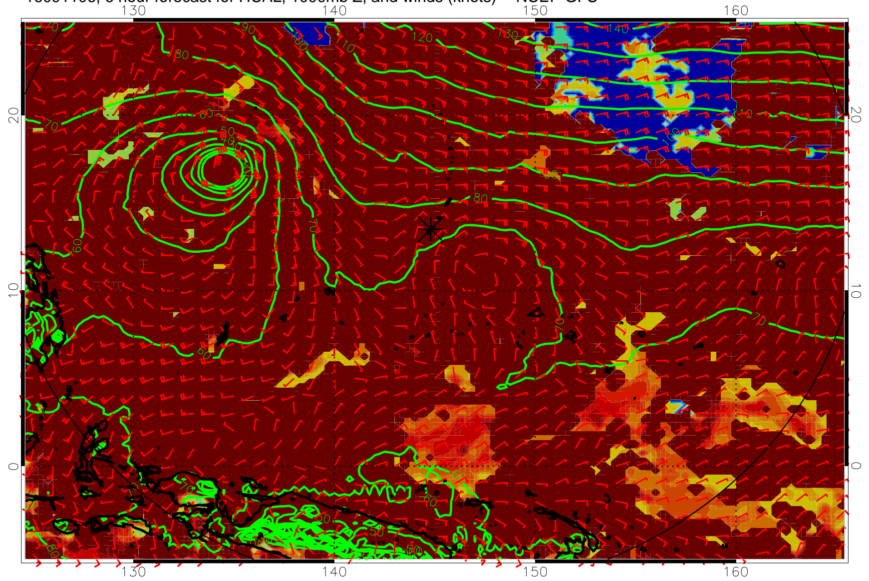
16091106, 6 hour forecast for HCAL, 1000mb Z, and winds (knots) -- NCEP GFS
