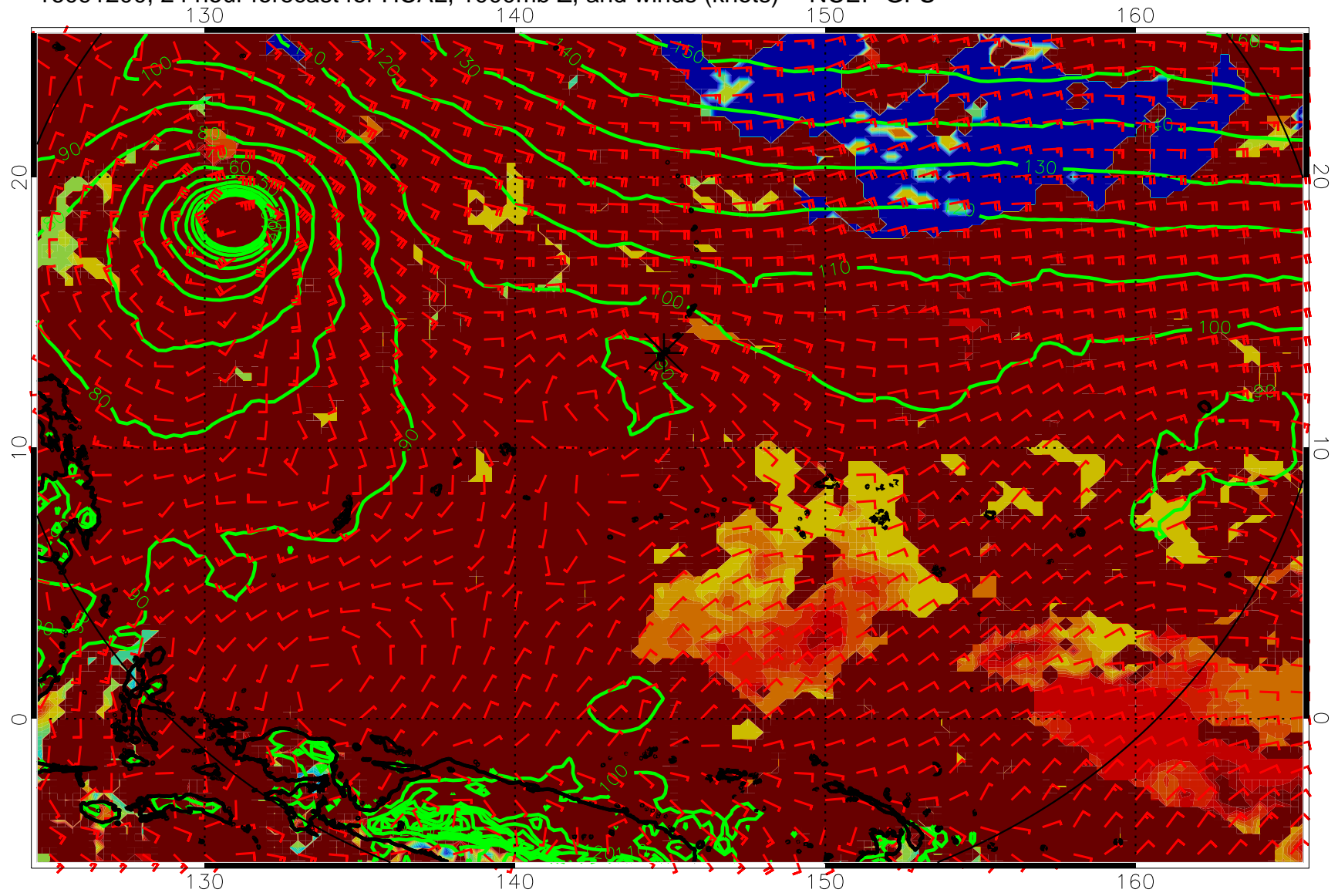
16091200, 24 hour forecast for HCAL, 1000mb Z, and winds (knots) -- NCEP GFS
