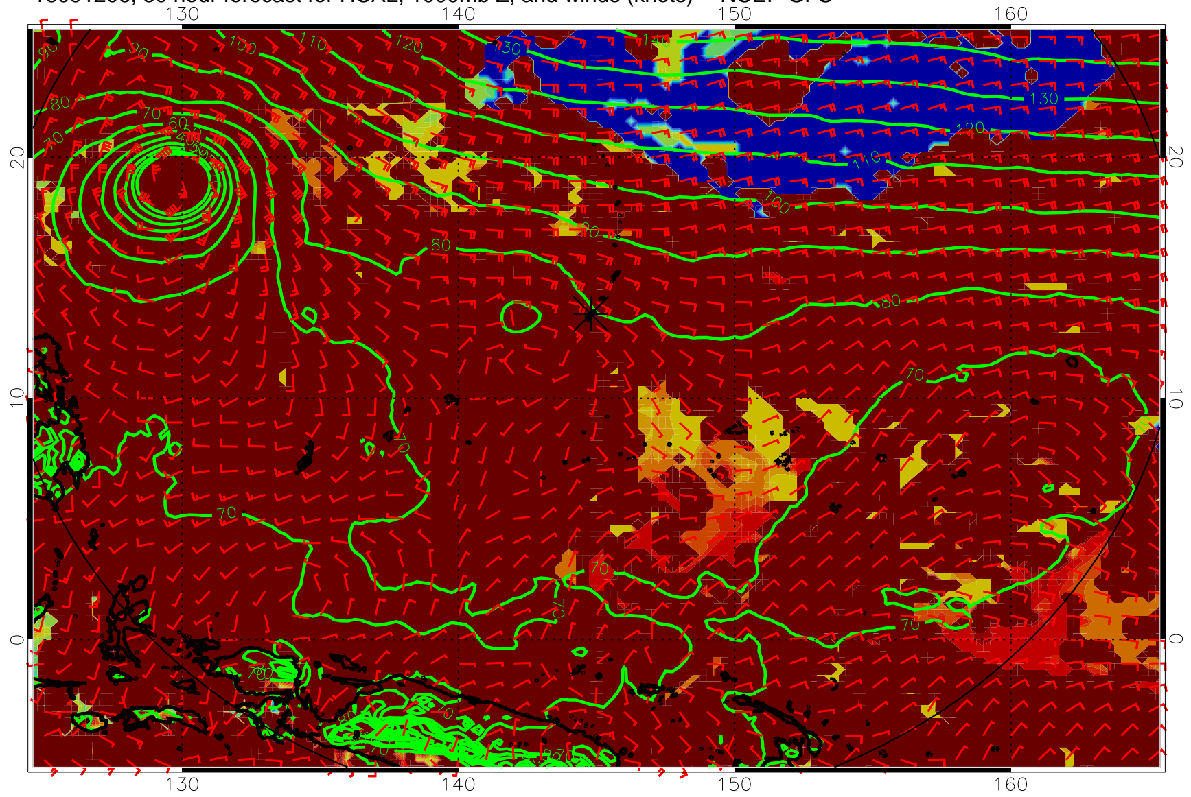
16091206, 30 hour forecast for HCAL, 1000mb Z, and winds (knots) -- NCEP GFS
