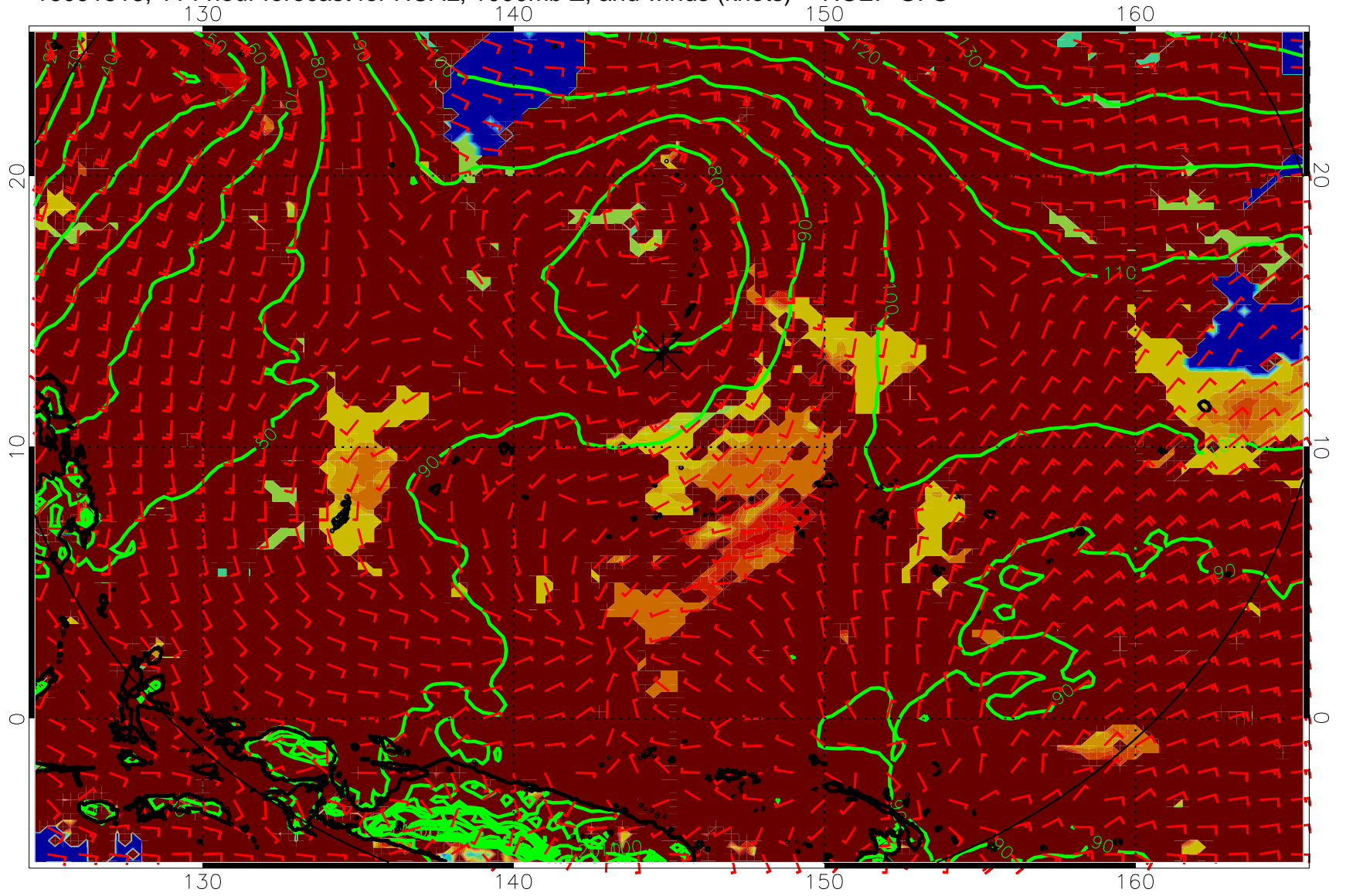
16091518, 114 hour forecast for HCAL, 1000mb Z, and winds (knots) -- NCEP GFS
