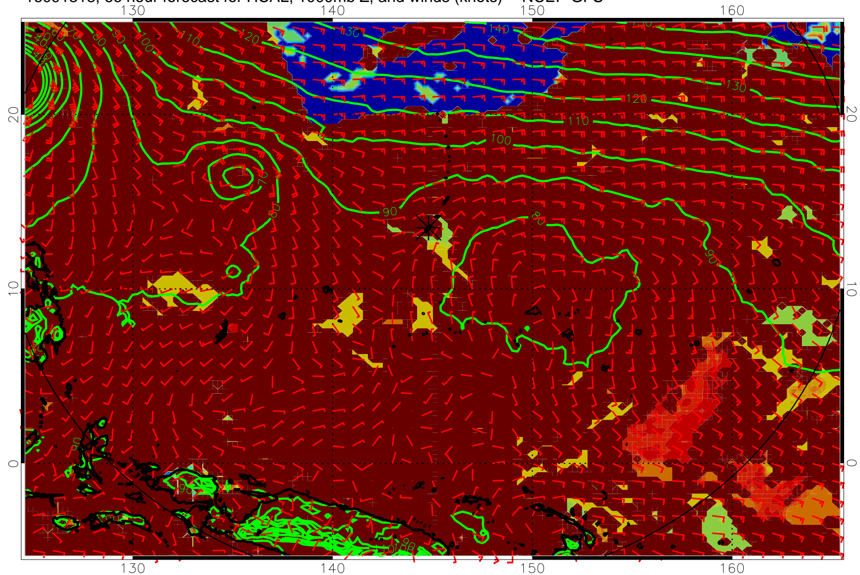
16091318, 66 hour forecast for HCAL, 1000mb Z, and winds (knots) -- NCEP GFS
