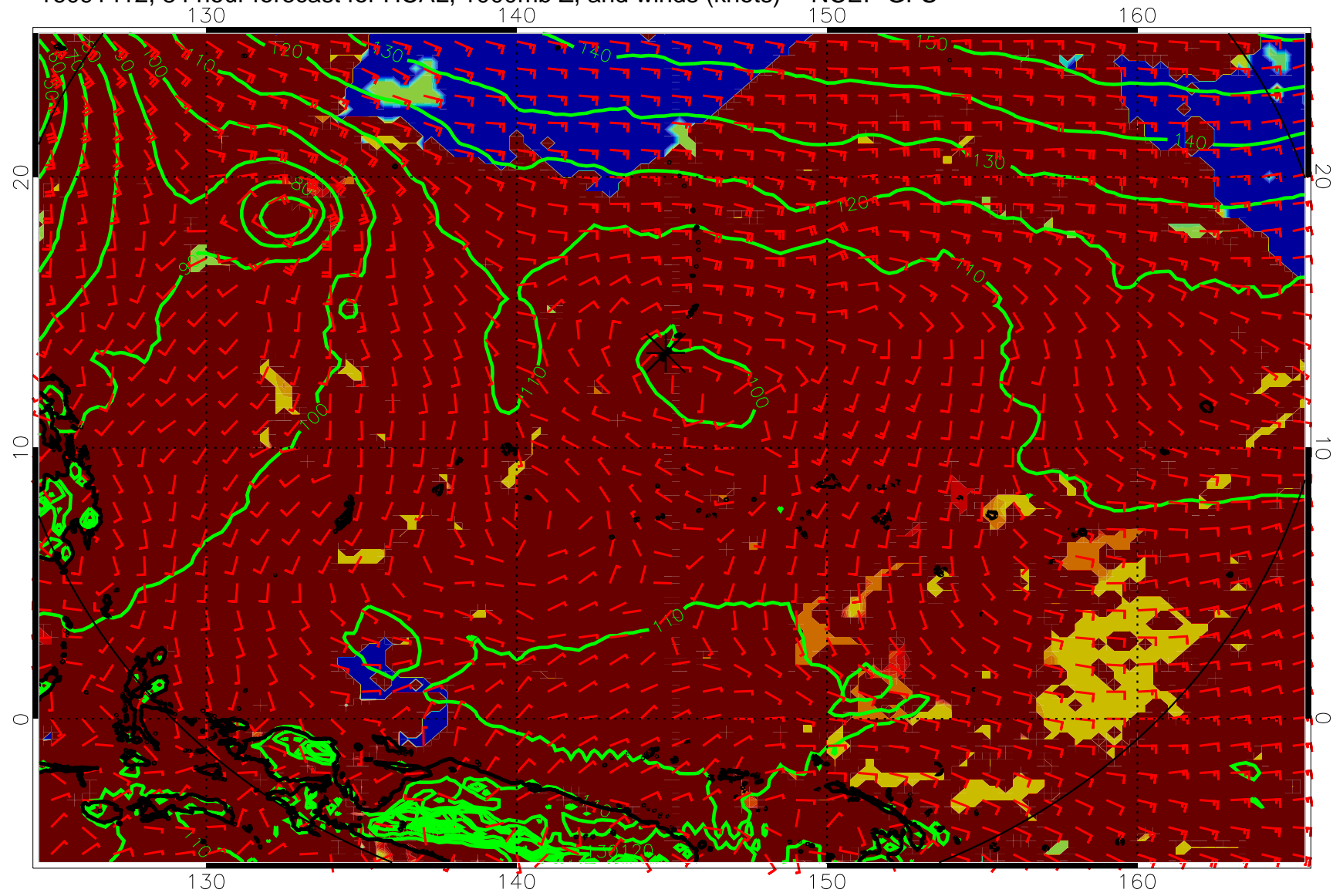
16091412, 84 hour forecast for HCAL, 1000mb Z, and winds (knots) -- NCEP GFS
