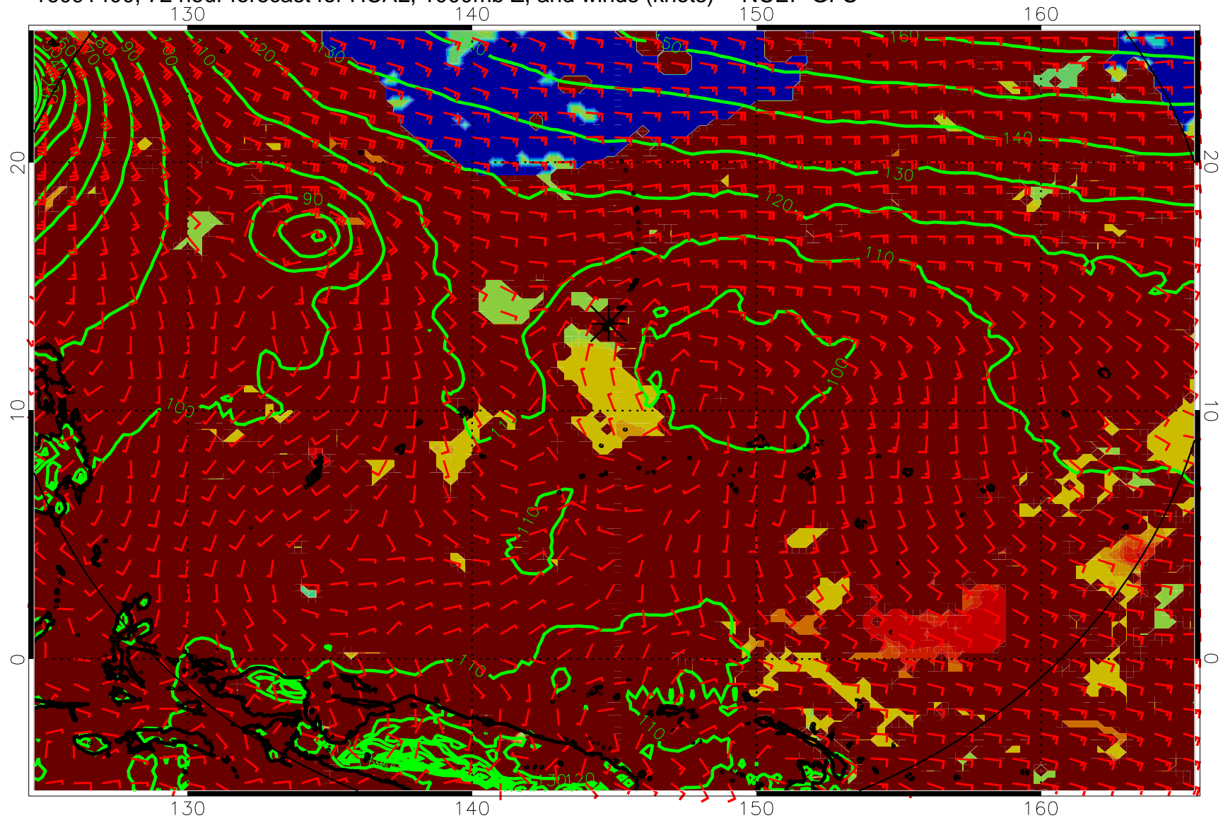
16091400, 72 hour forecast for HCAL, 1000mb Z, and winds (knots) -- NCEP GFS
