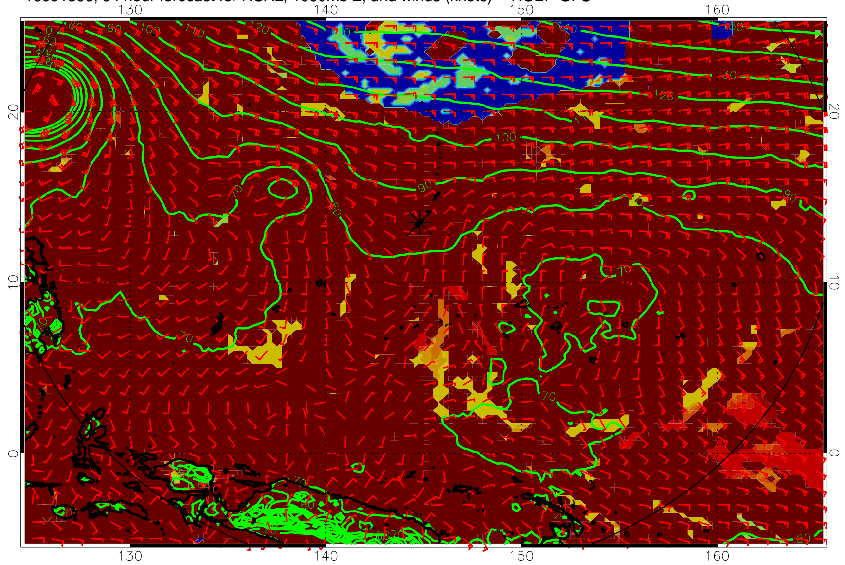
16091306, 54 hour forecast for HCAL, 1000mb Z, and winds (knots) -- NCEP GFS
