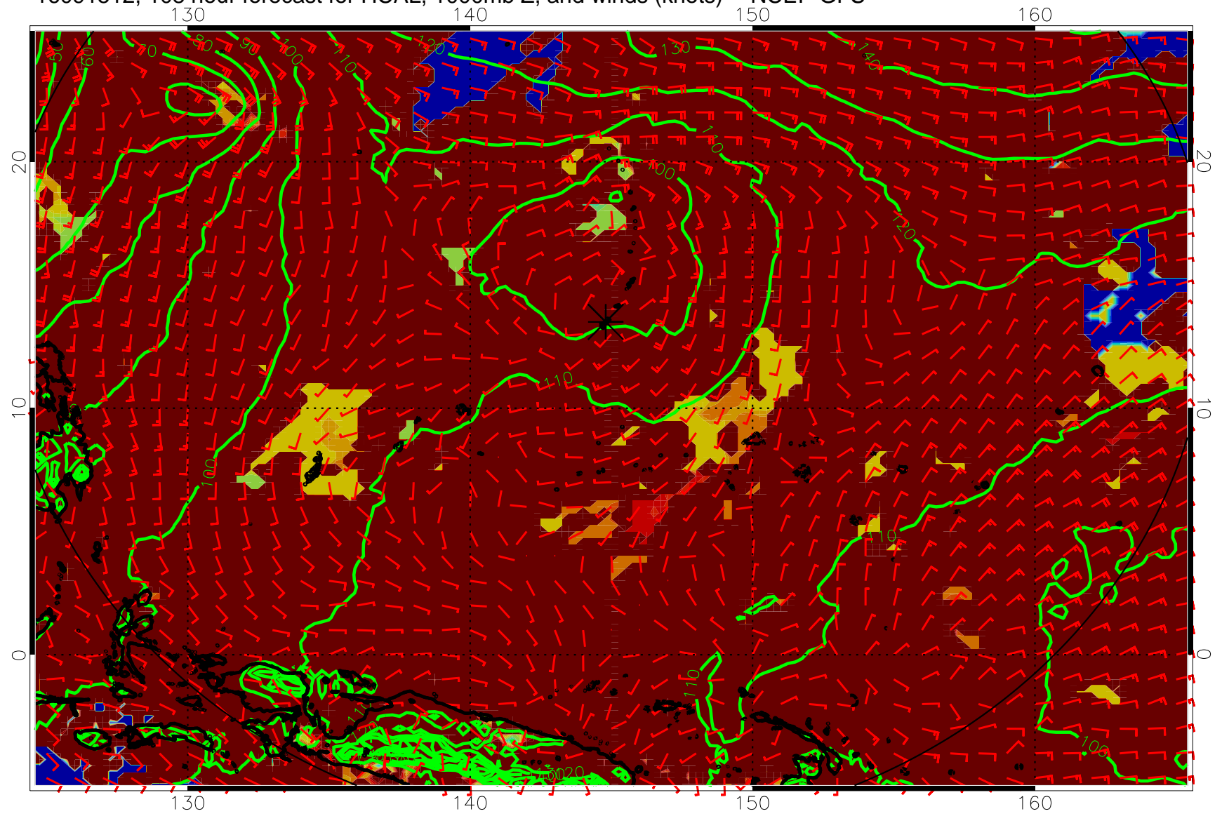
16091512, 108 hour forecast for HCAL, 1000mb Z, and winds (knots) -- NCEP GFS
