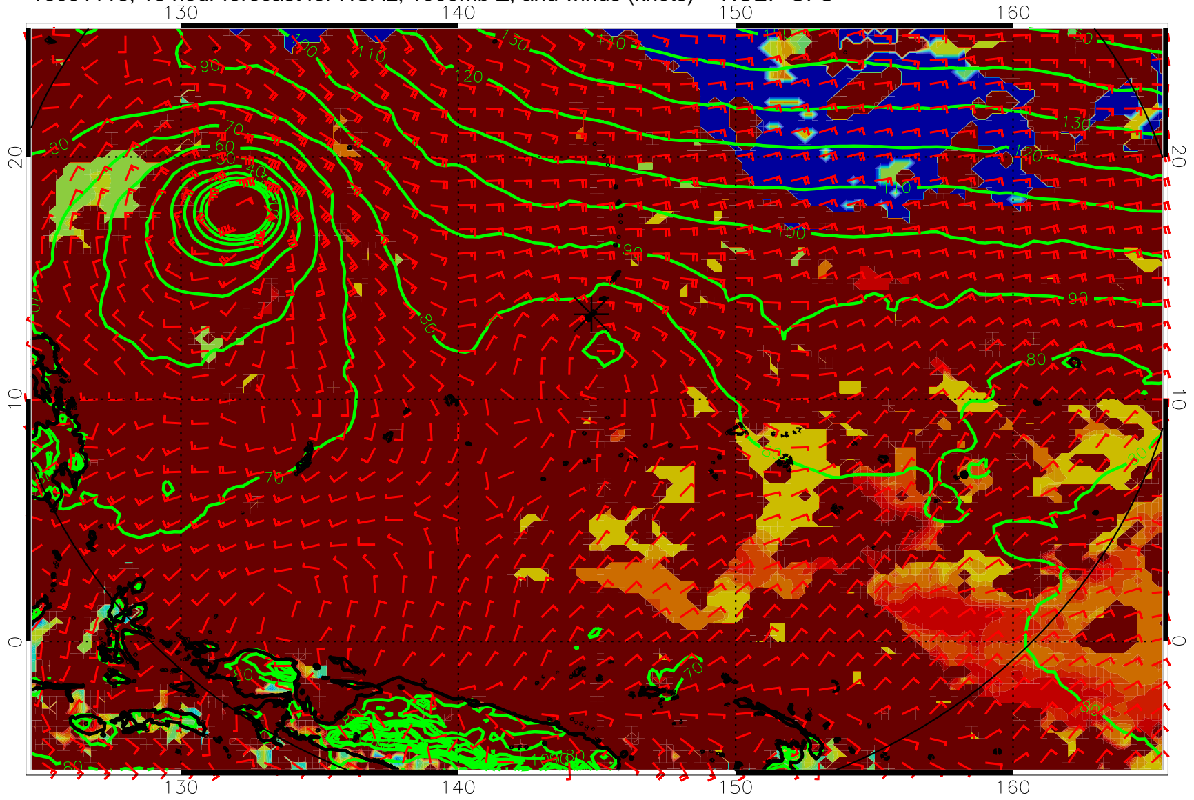
16091118, 18 hour forecast for HCAL, 1000mb Z, and winds (knots) -- NCEP GFS
