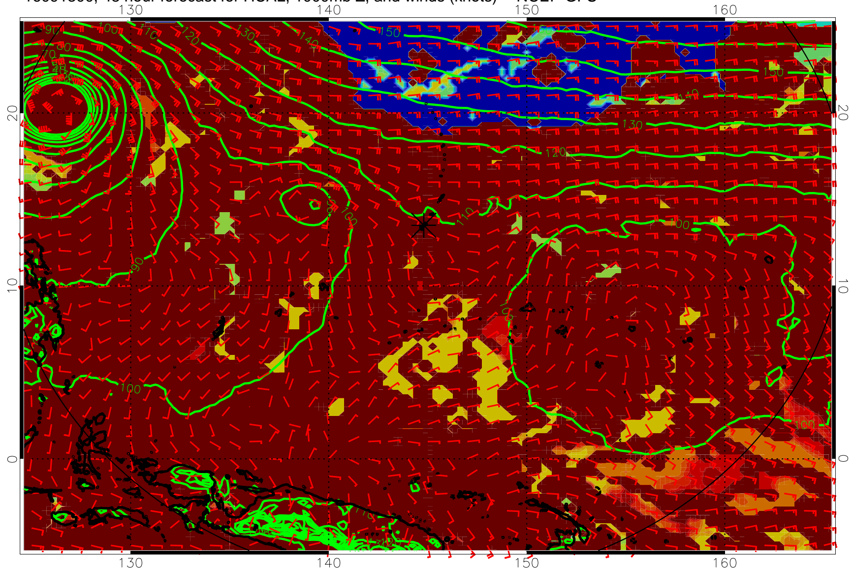
16091300, 48 hour forecast for HCAL, 1000mb Z, and winds (knots) -- NCEP GFS
