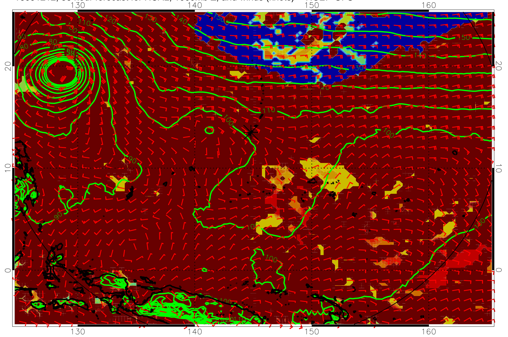
16091212, 36 hour forecast for HCAL, 1000mb Z, and winds (knots) -- NCEP GFS
