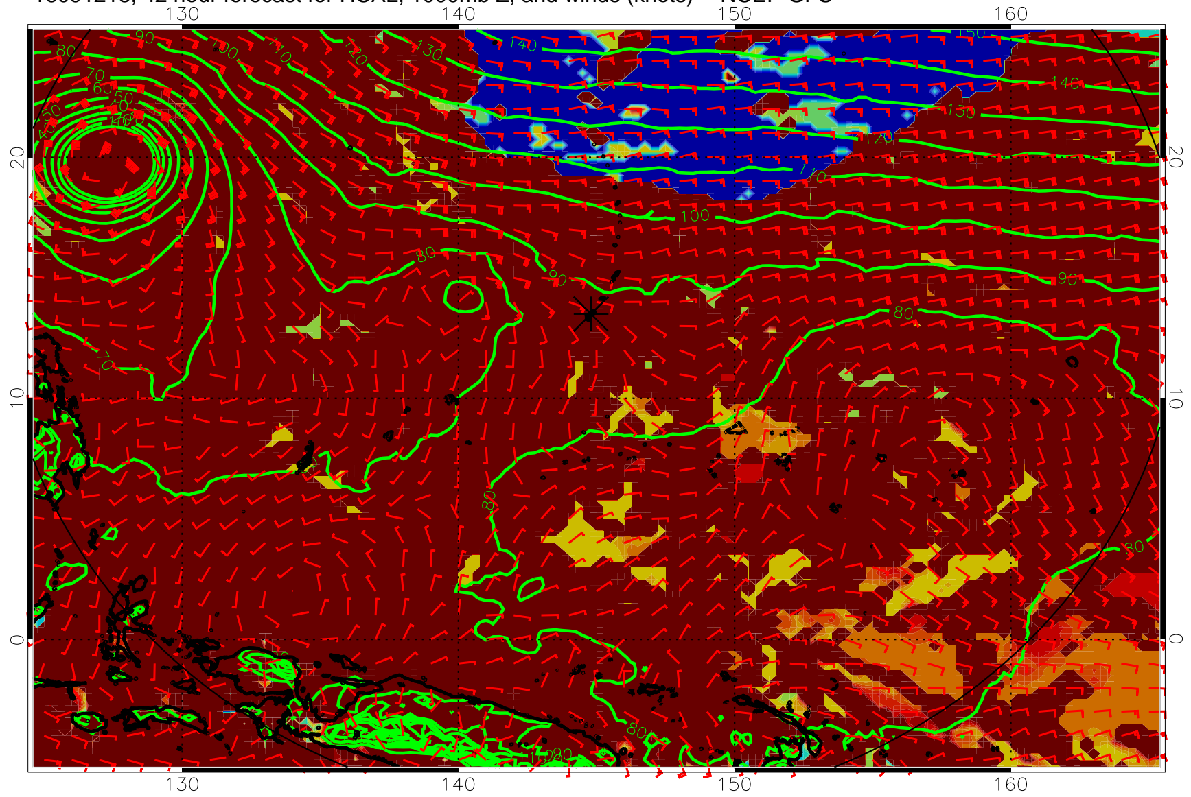
16091218, 42 hour forecast for HCAL, 1000mb Z, and winds (knots) -- NCEP GFS
