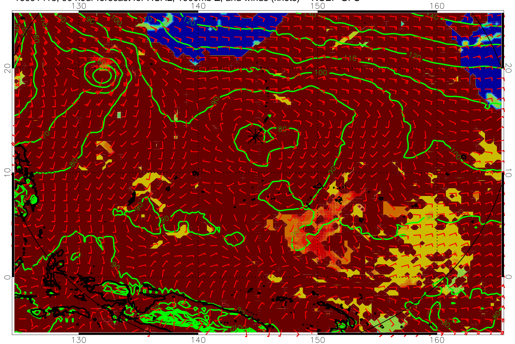
16091418, 90 hour forecast for HCAL, 1000mb Z, and winds (knots) -- NCEP GFS
