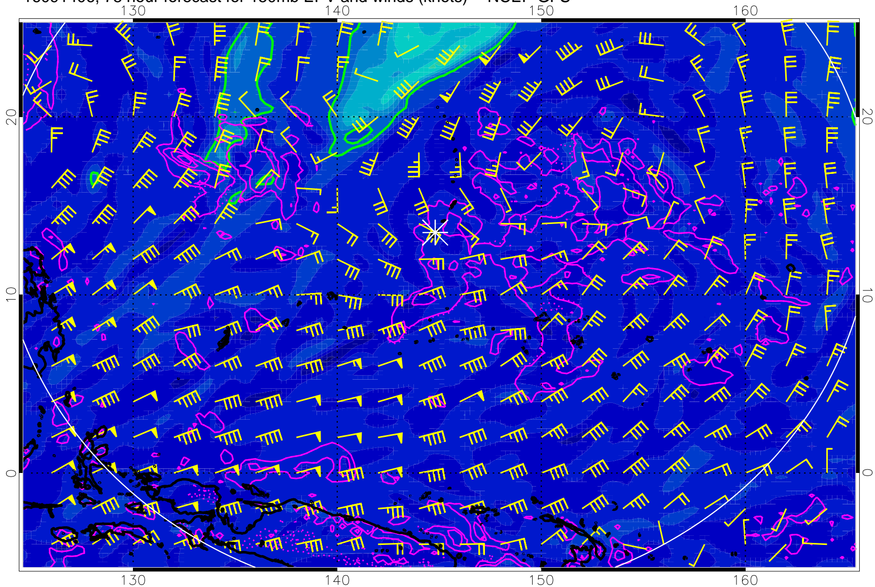
16091406, 78 hour forecast for 150mb EPV and winds (knots) -- NCEP GFS
