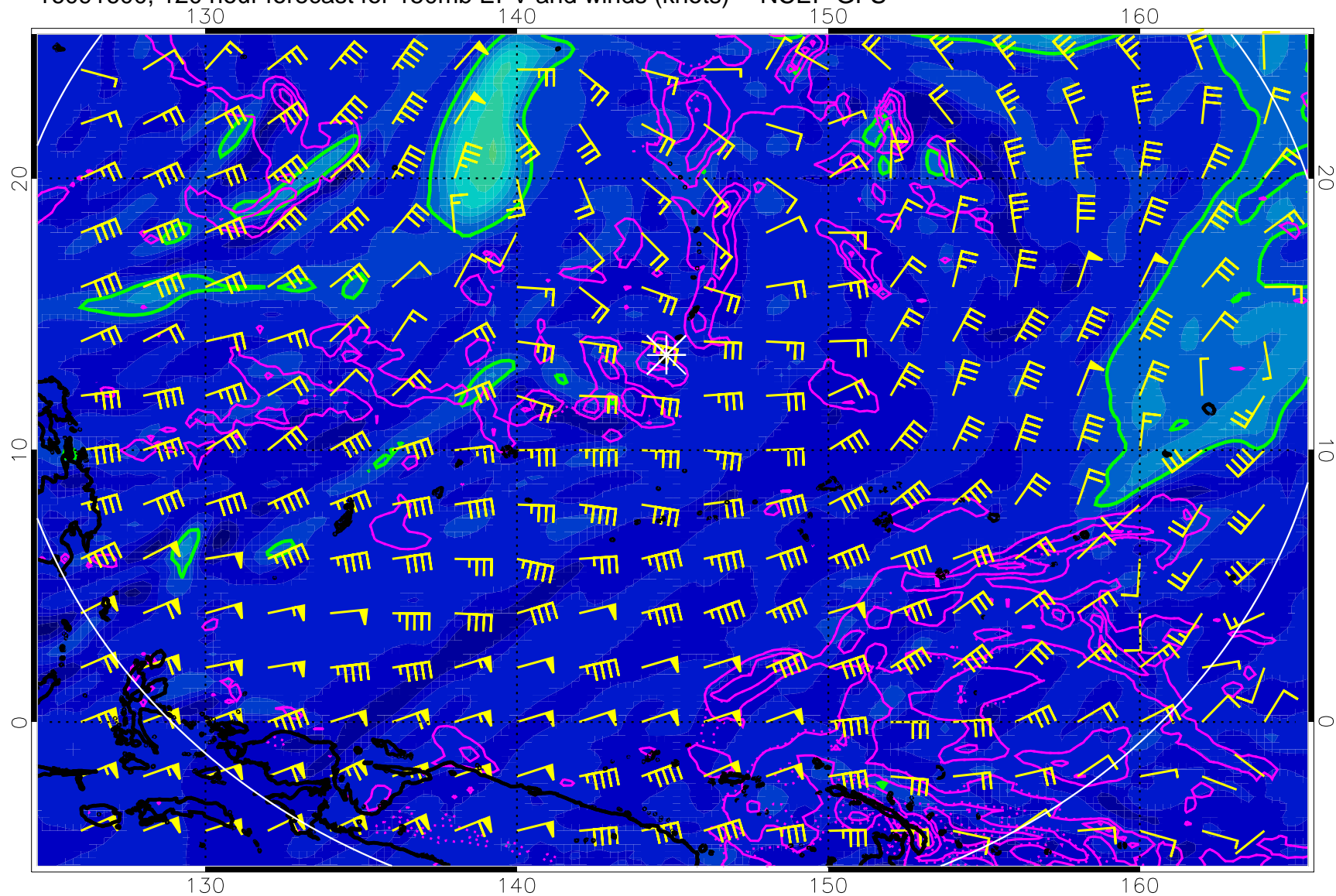
16091600, 120 hour forecast for 150mb EPV and winds (knots) -- NCEP GFS
