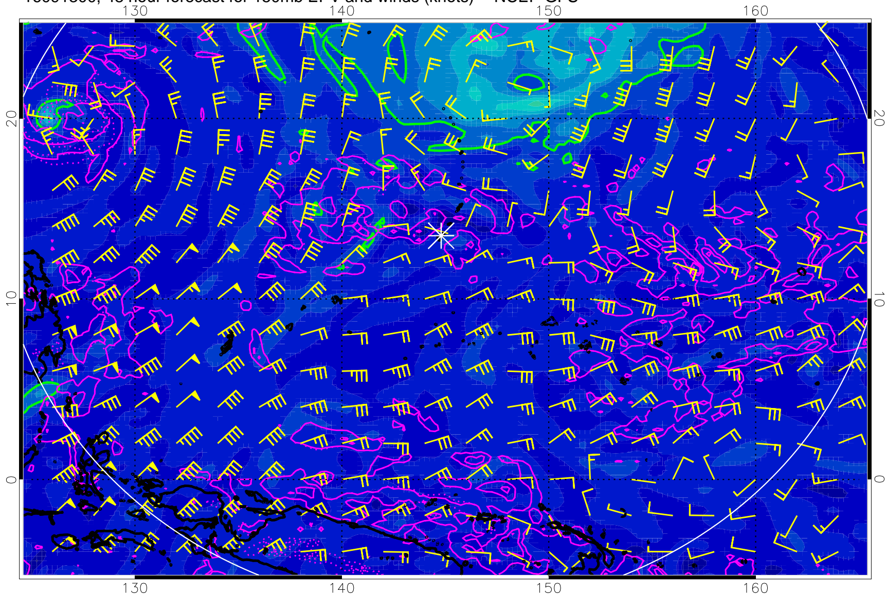
16091300, 48 hour forecast for 150mb EPV and winds (knots) -- NCEP GFS
