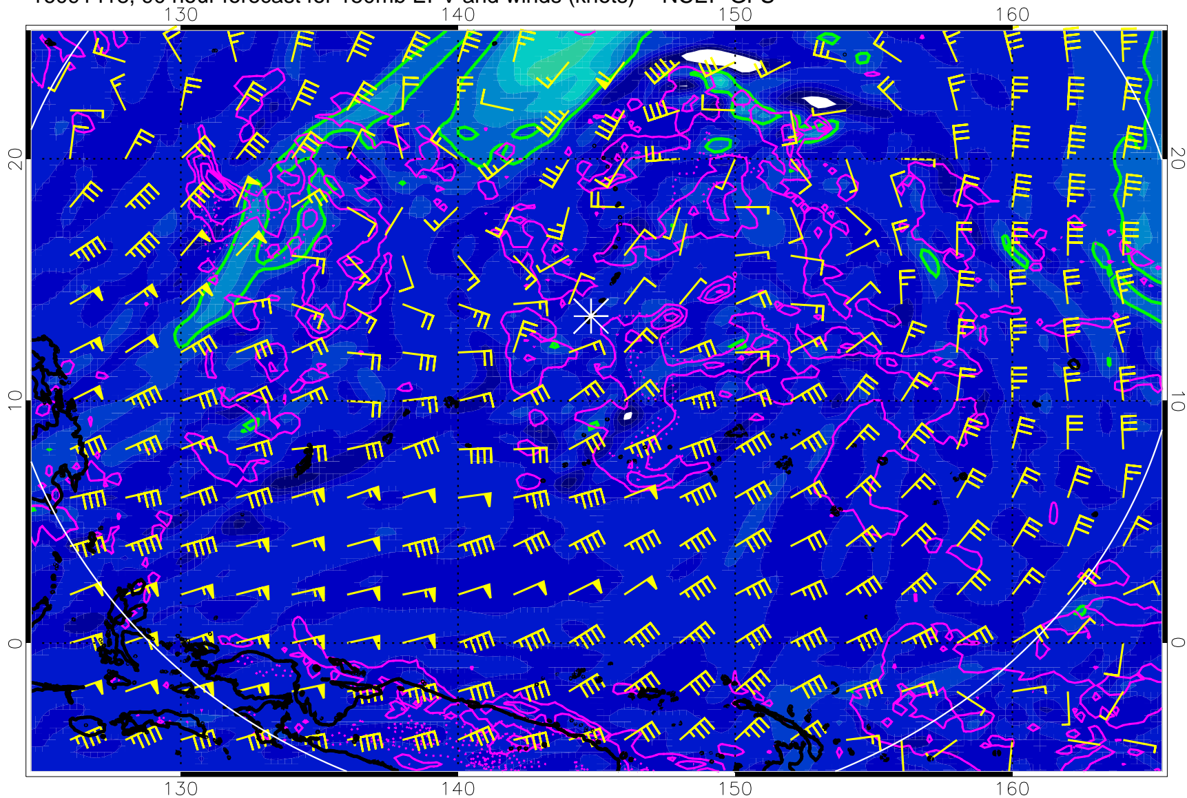
16091418, 90 hour forecast for 150mb EPV and winds (knots) -- NCEP GFS
