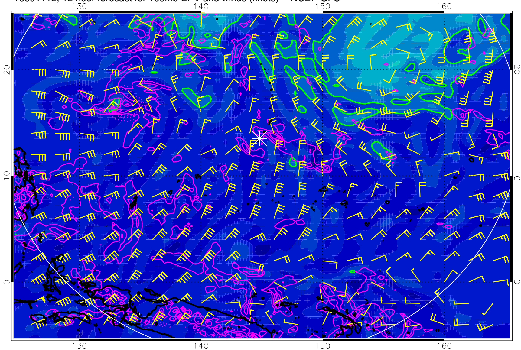
16091112, 12 hour forecast for 150mb EPV and winds (knots) -- NCEP GFS
