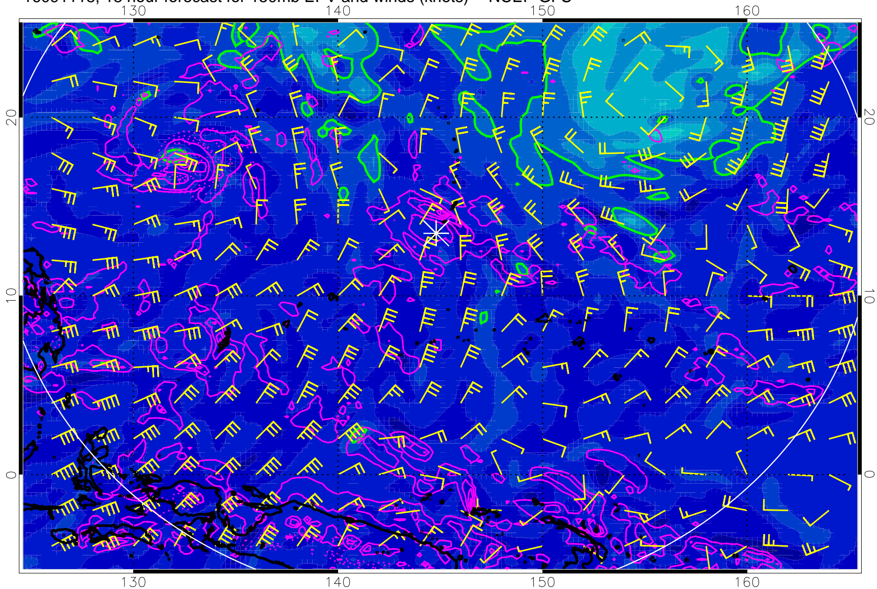
16091118, 18 hour forecast for 150mb EPV and winds (knots) -- NCEP GFS
