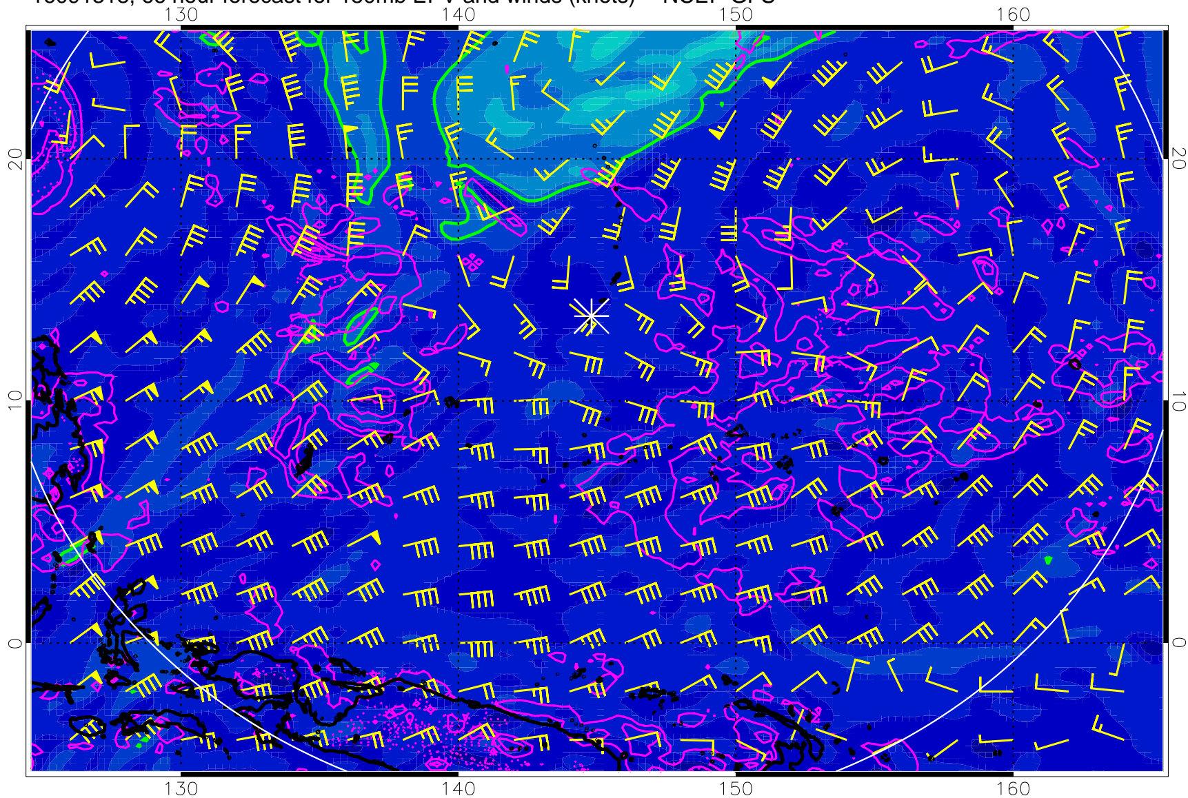
16091318, 66 hour forecast for 150mb EPV and winds (knots) -- NCEP GFS
