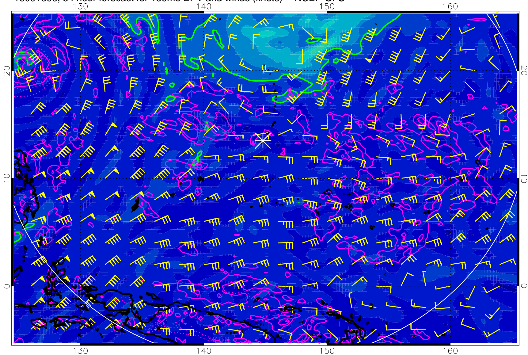
16091306, 54 hour forecast for 150mb EPV and winds (knots) -- NCEP GFS
