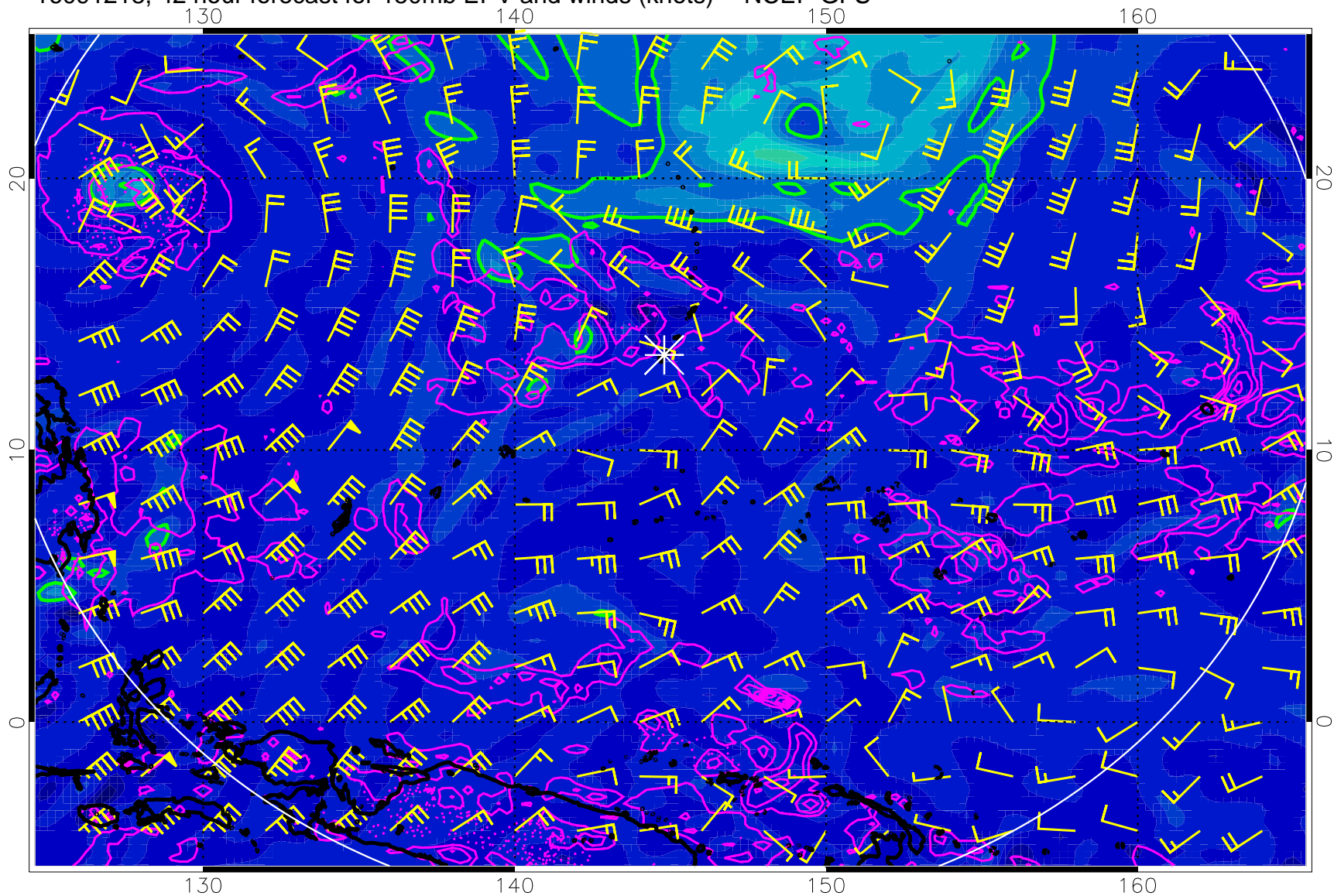
16091218, 42 hour forecast for 150mb EPV and winds (knots) -- NCEP GFS
