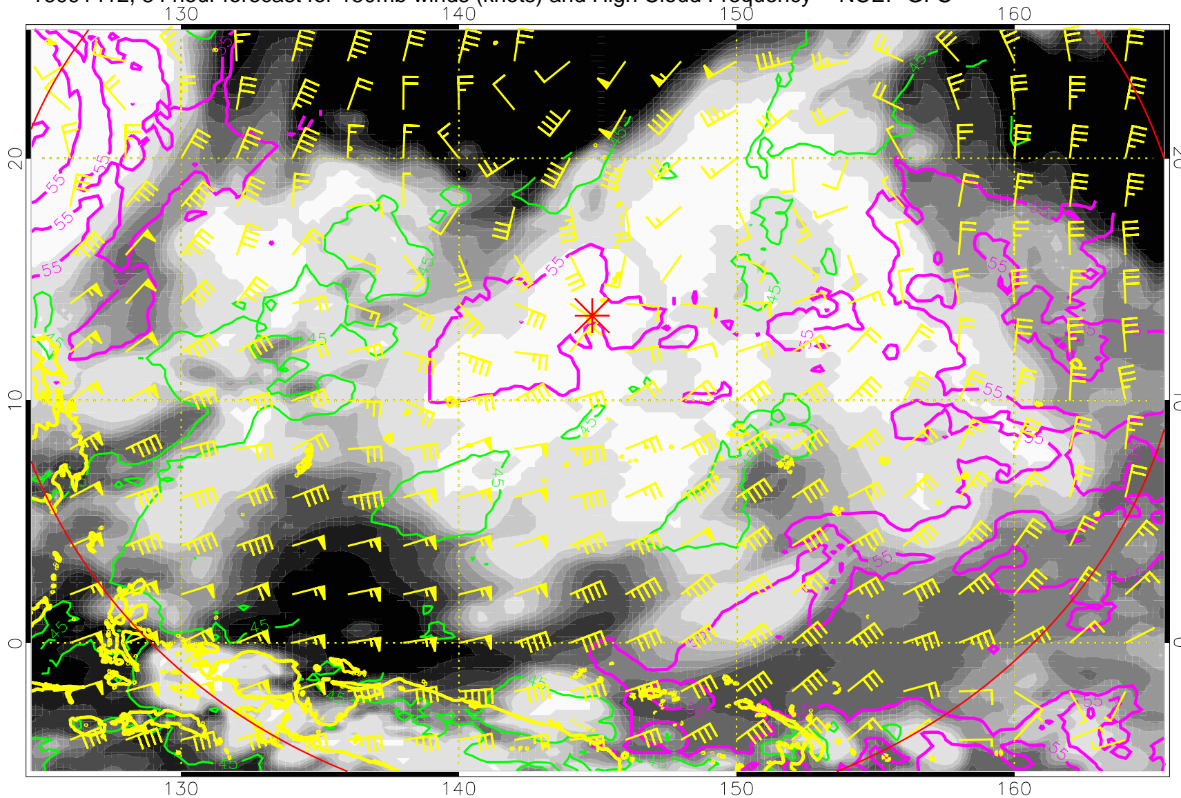
16091412, 84 hour forecast for 150mb winds (knots) and High Cloud Frequency -- NCEP GFS
