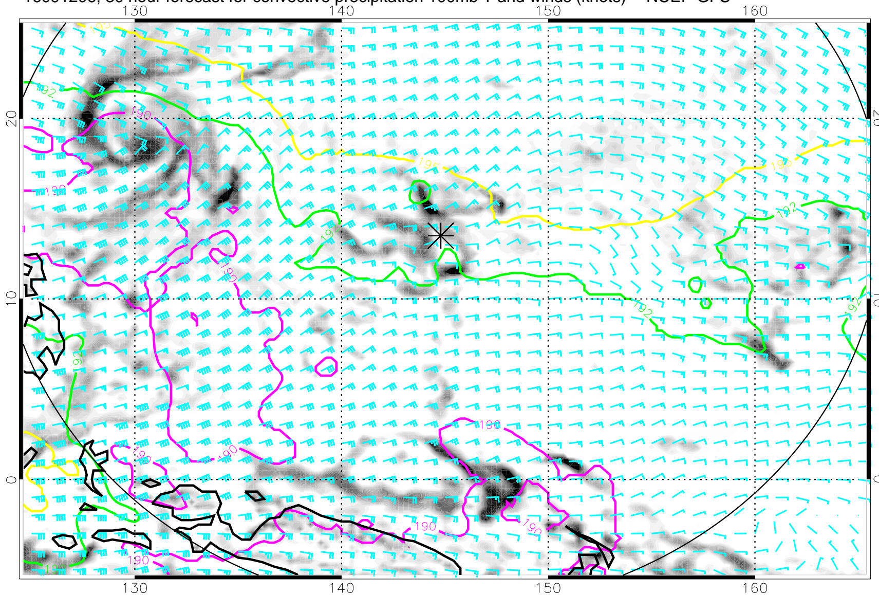
16091206, 30 hour forecast for convective precipitation 100mb T and winds (knots) -- NCEP GFS
