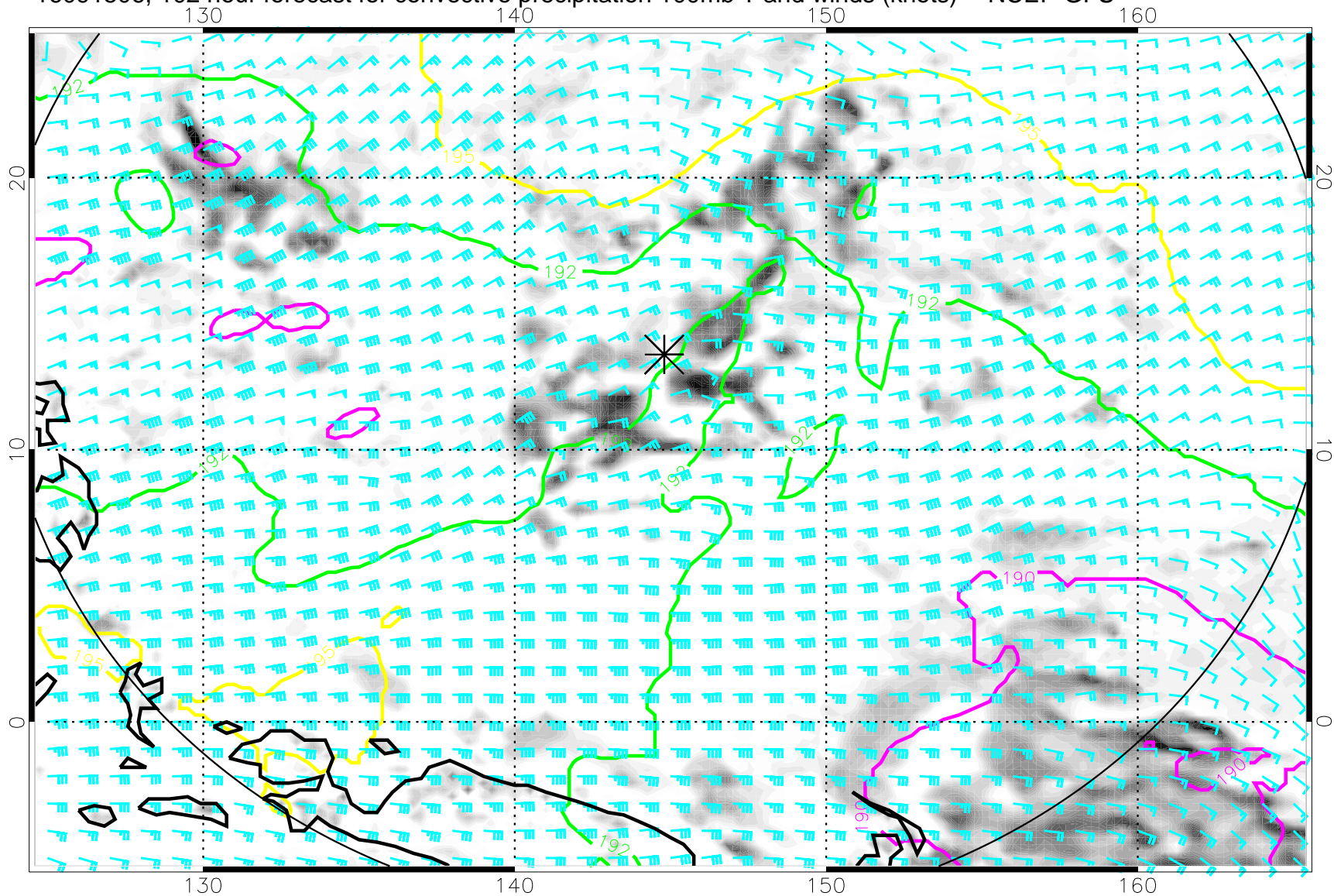
16091506, 102 hour forecast for convective precipitation 100mb T and winds (knots) -- NCEP GFS
