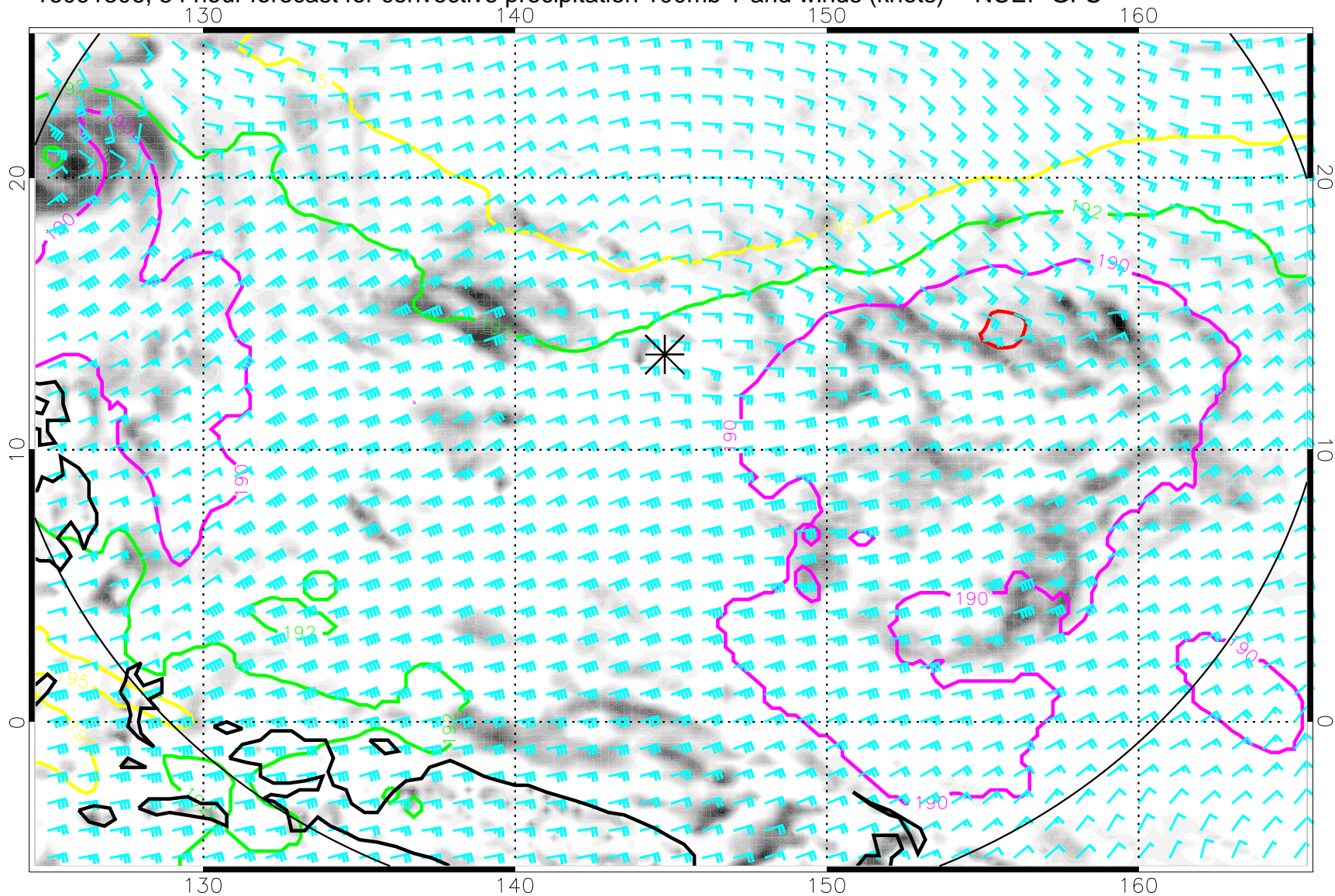
16091306, 54 hour forecast for convective precipitation 100mb T and winds (knots) -- NCEP GFS
