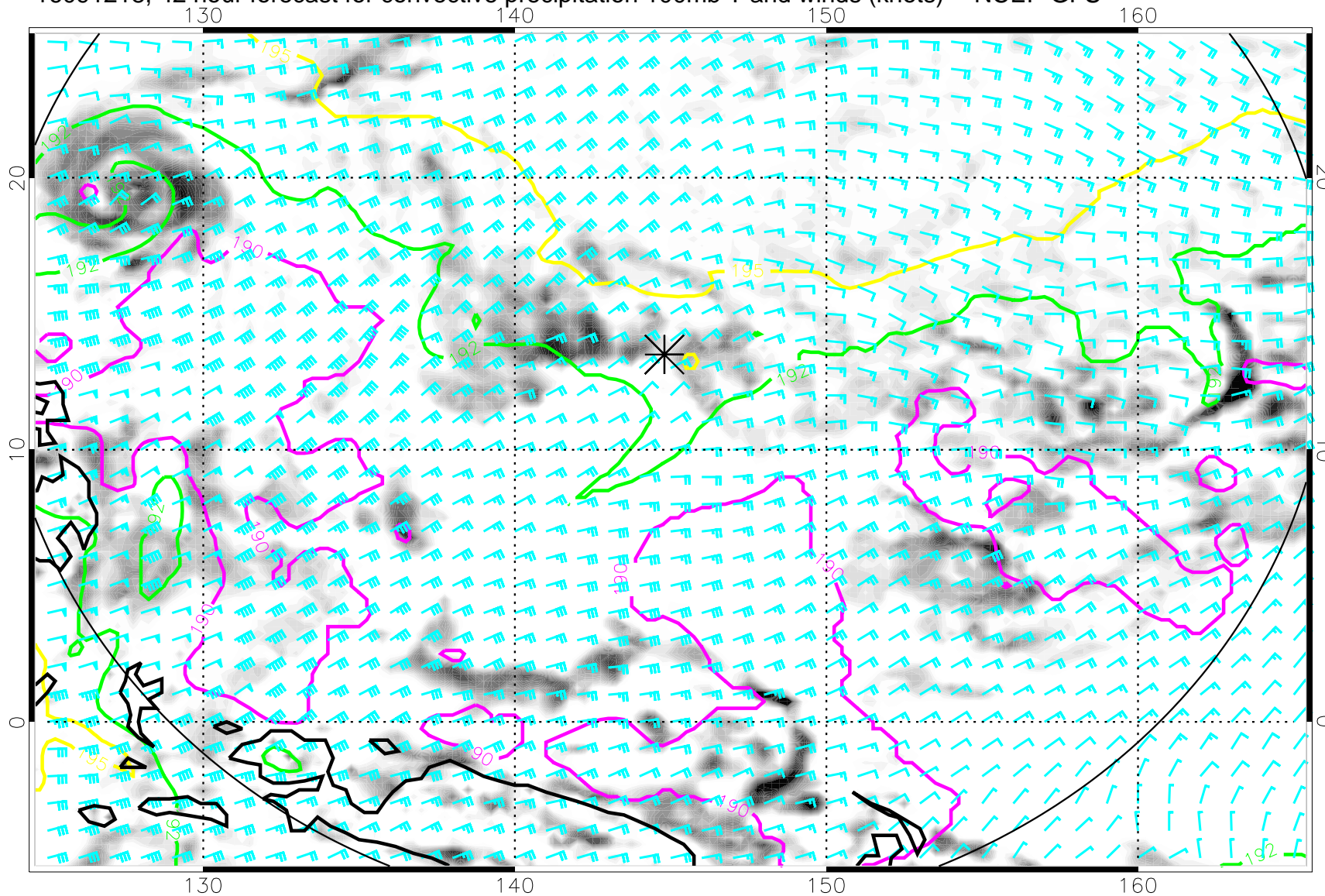
16091218, 42 hour forecast for convective precipitation 100mb T and winds (knots) -- NCEP GFS
