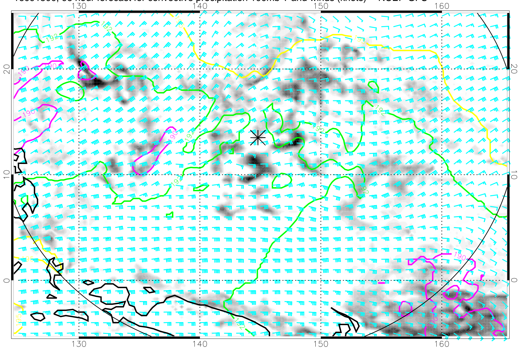
16091500, 96 hour forecast for convective precipitation 100mb T and winds (knots) -- NCEP GFS
