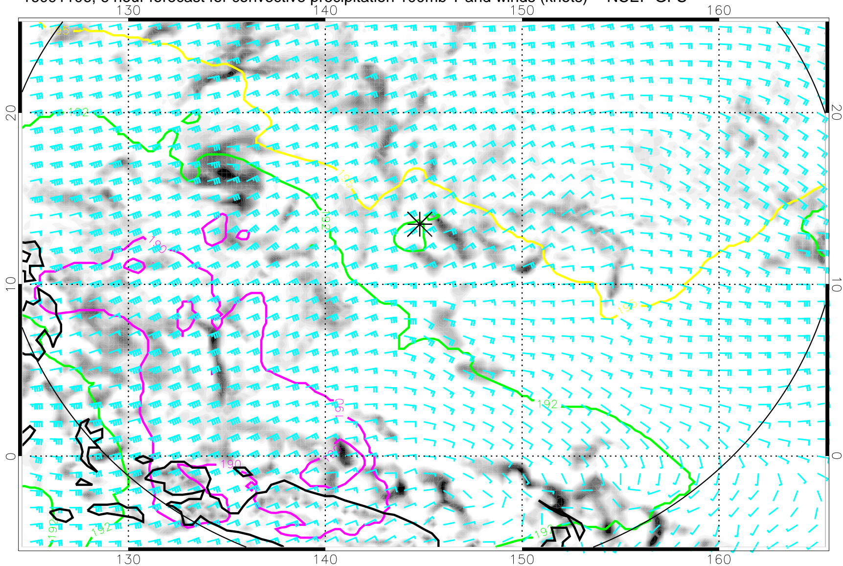
16091106, 6 hour forecast for convective precipitation 100mb T and winds (knots) -- NCEP GFS
