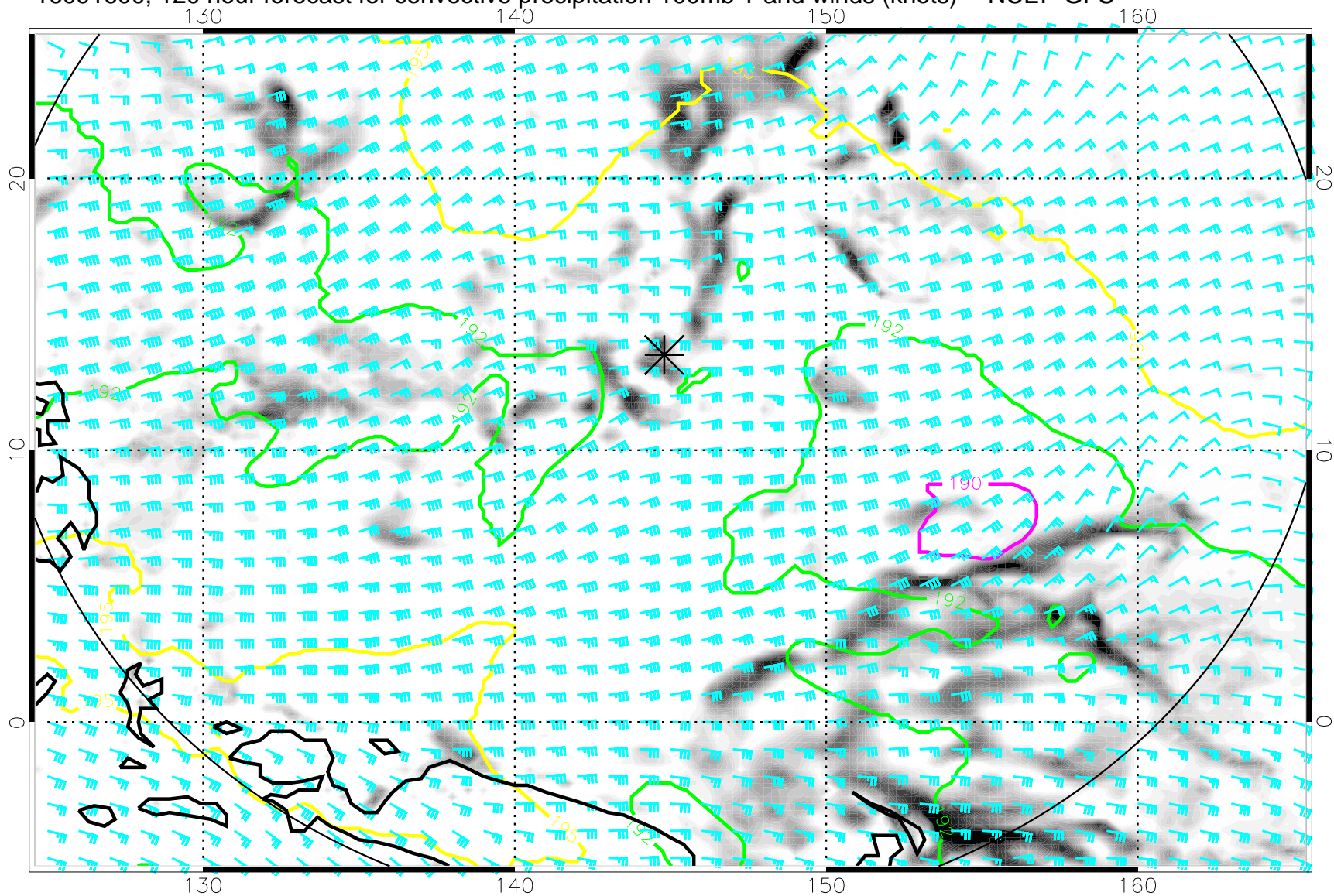
16091600, 120 hour forecast for convective precipitation 100mb T and winds (knots) -- NCEP GFS
