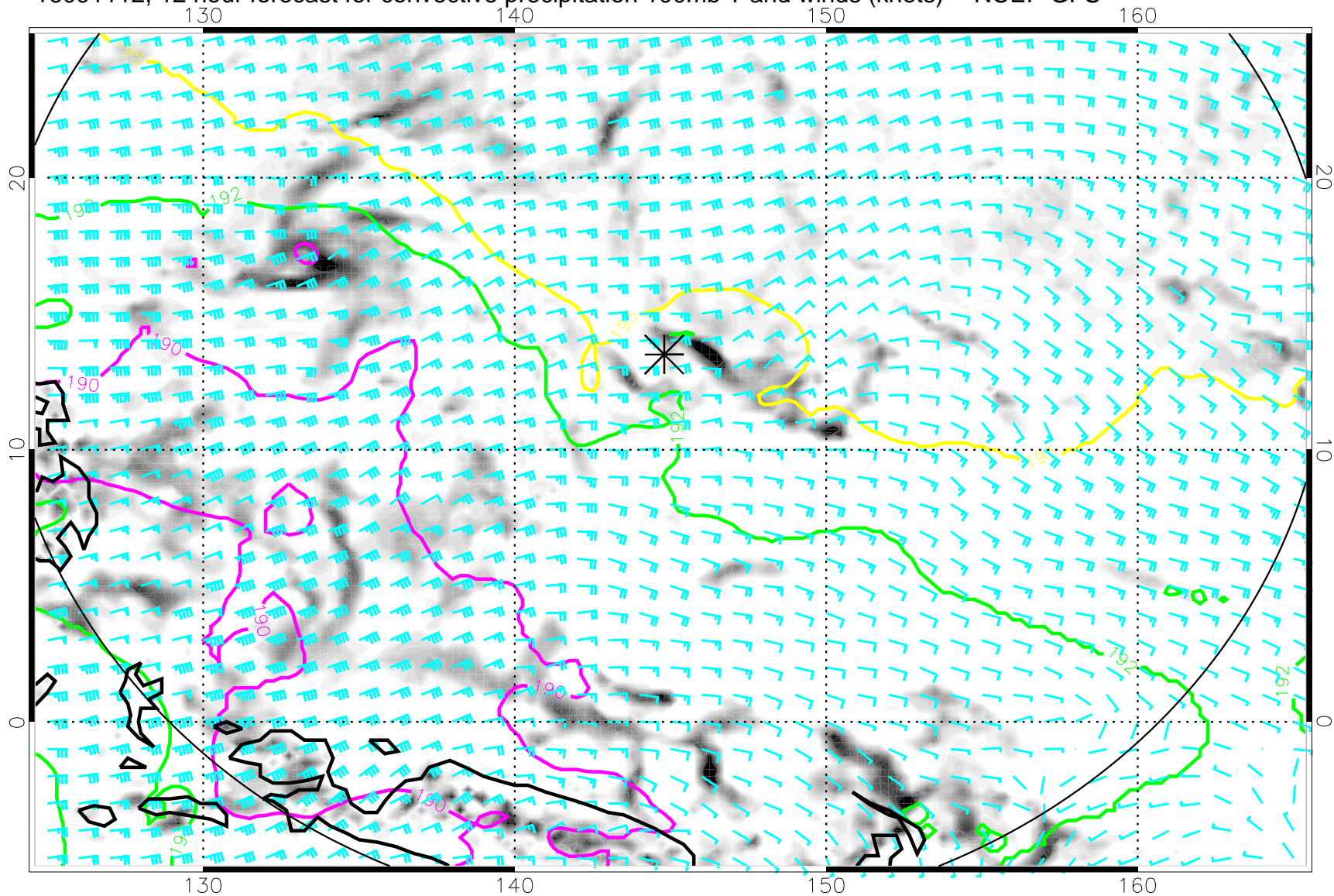
16091112, 12 hour forecast for convective precipitation 100mb T and winds (knots) -- NCEP GFS
