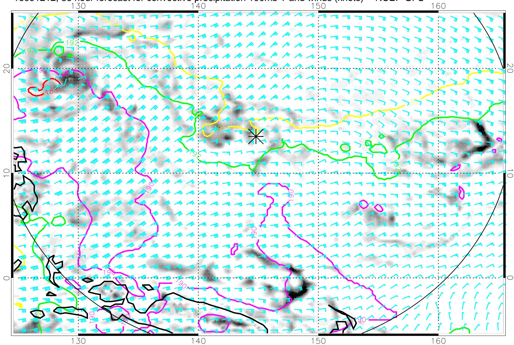
16091212, 36 hour forecast for convective precipitation 100mb T and winds (knots) -- NCEP GFS
