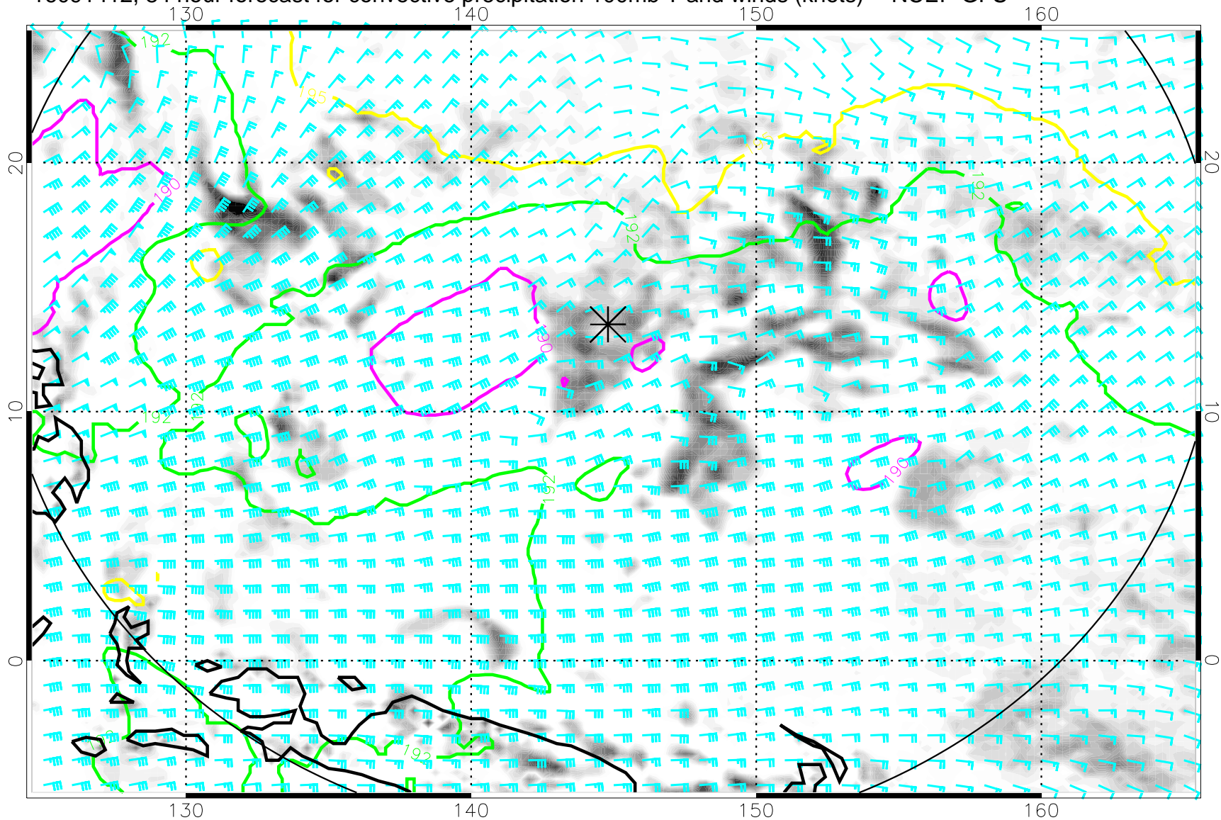
16091412, 84 hour forecast for convective precipitation 100mb T and winds (knots) -- NCEP GFS
