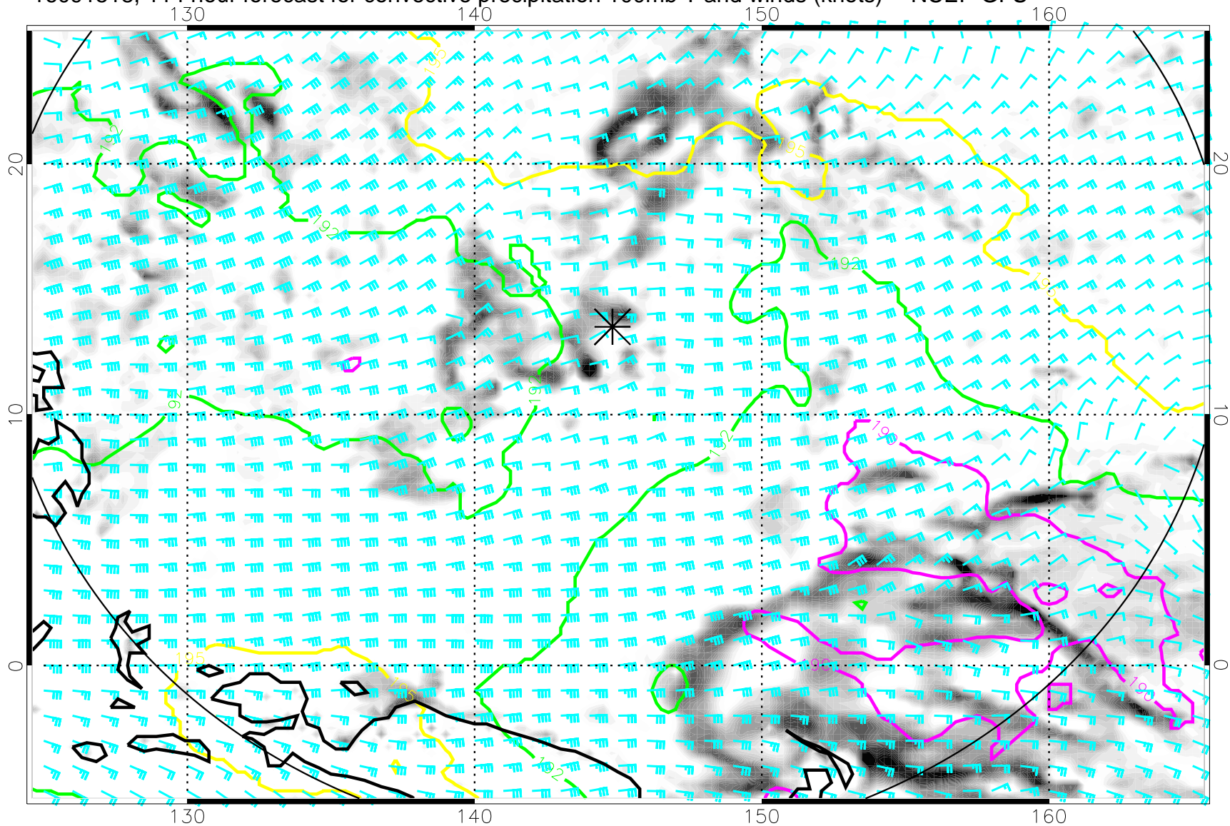
16091518, 114 hour forecast for convective precipitation 100mb T and winds (knots) -- NCEP GFS
