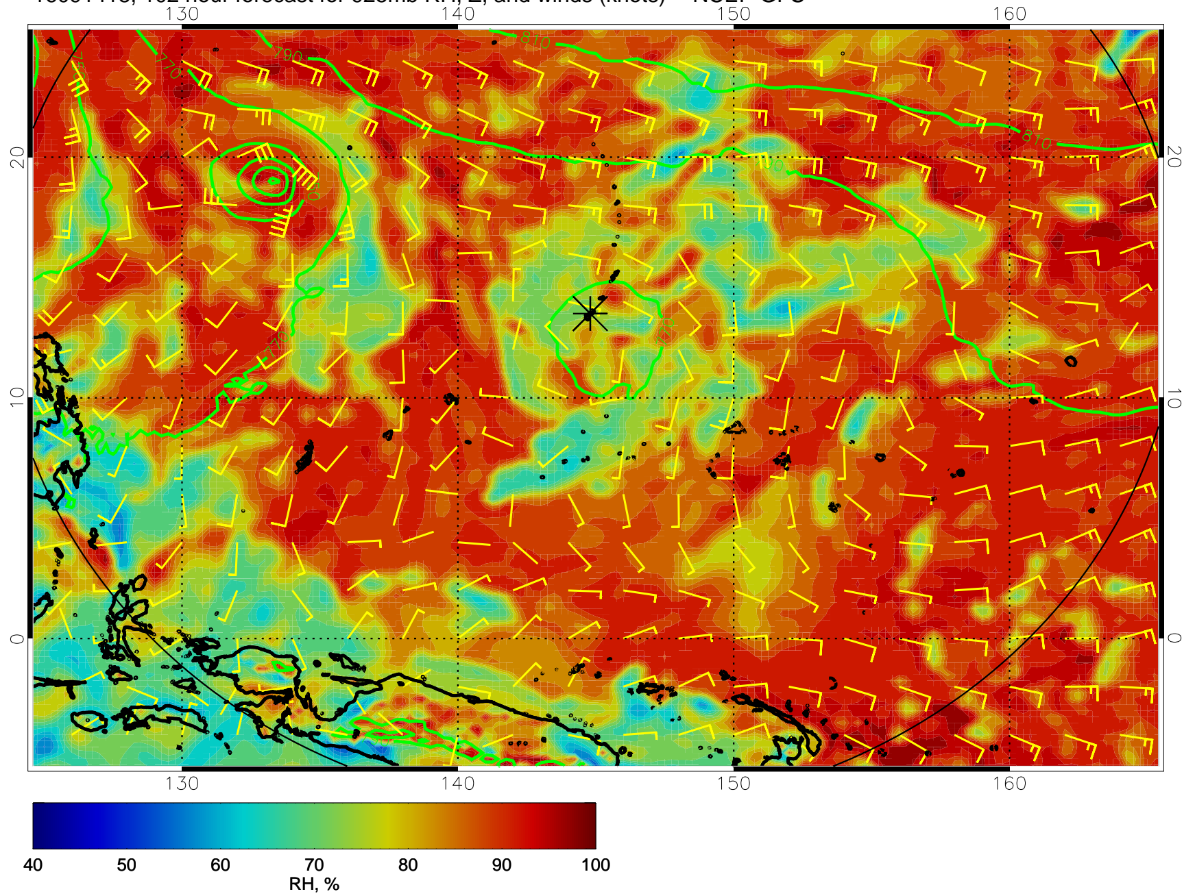
16091418, 102 hour forecast for 925mb RH, Z, and winds (knots) -- NCEP GFS
