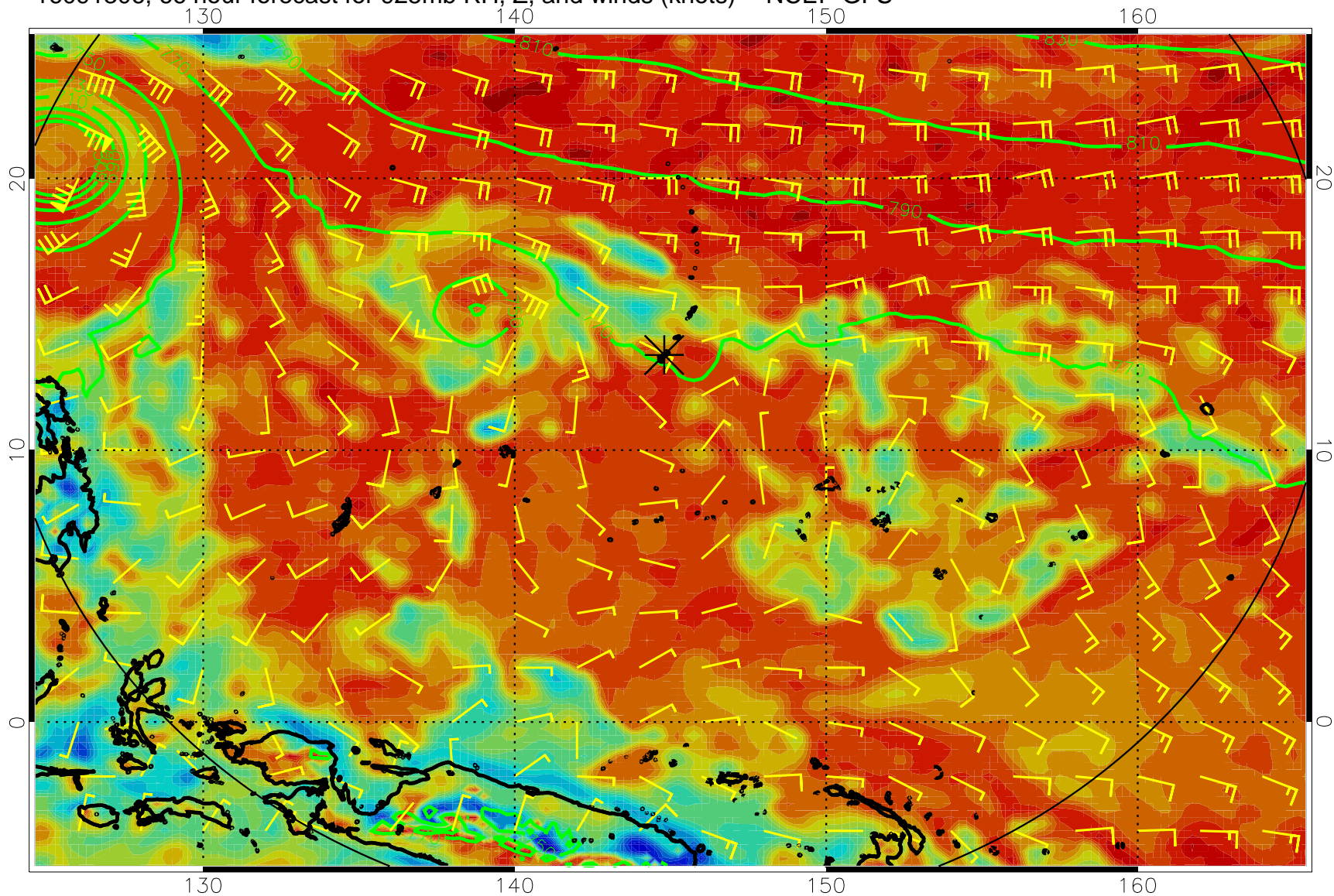
16091306, 66 hour forecast for 925mb RH, Z, and winds (knots) -- NCEP GFS
