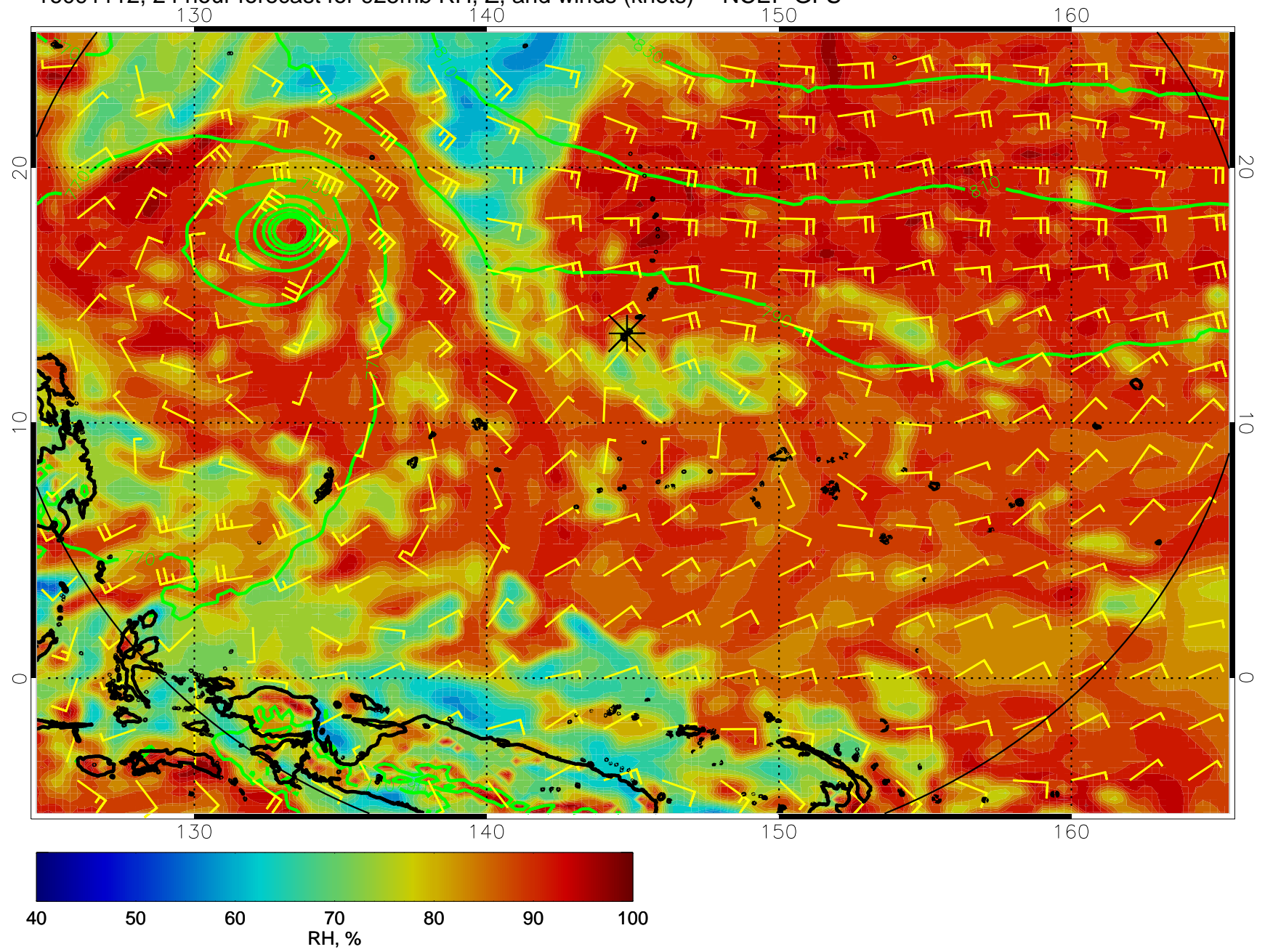
16091112, 24 hour forecast for 925mb RH, Z, and winds (knots) -- NCEP GFS
