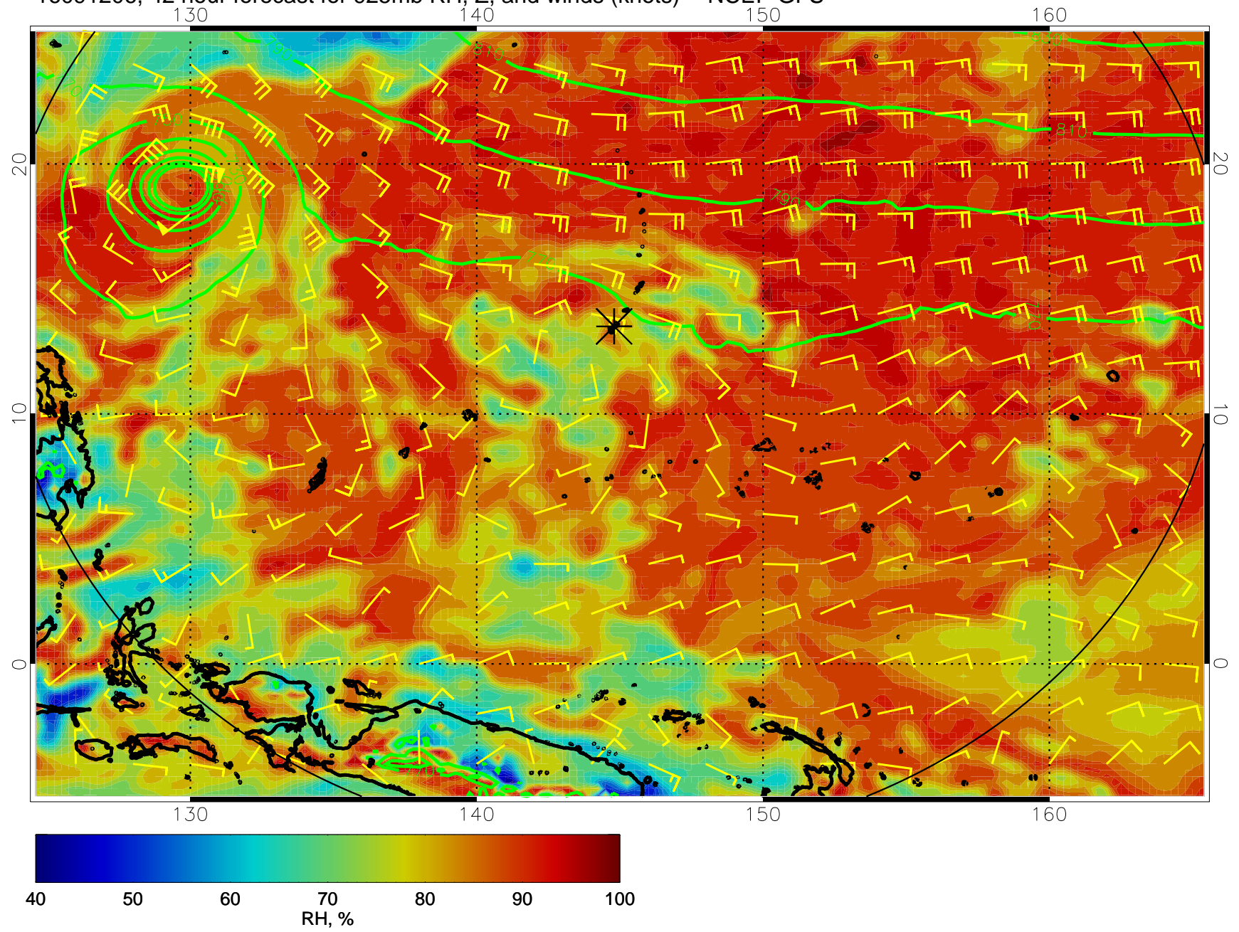
16091206, 42 hour forecast for 925mb RH, Z, and winds (knots) -- NCEP GFS
