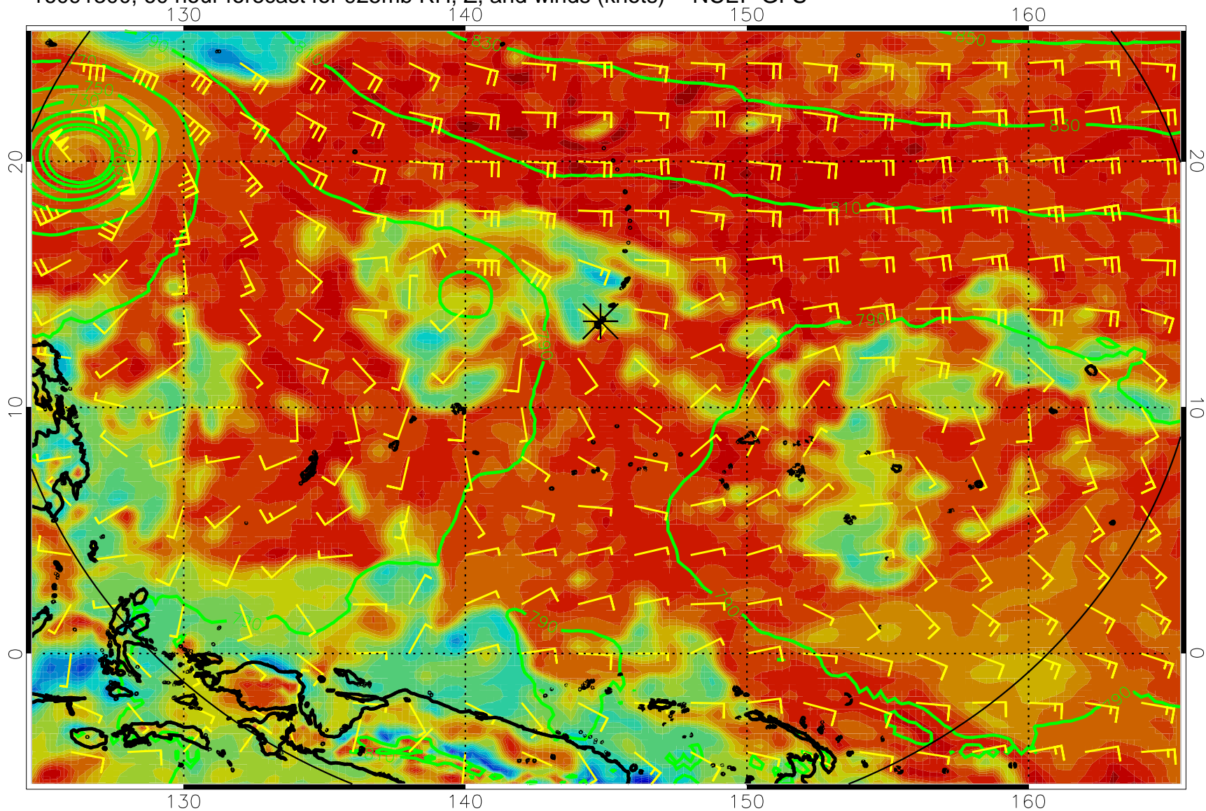
16091300, 60 hour forecast for 925mb RH, Z, and winds (knots) -- NCEP GFS
