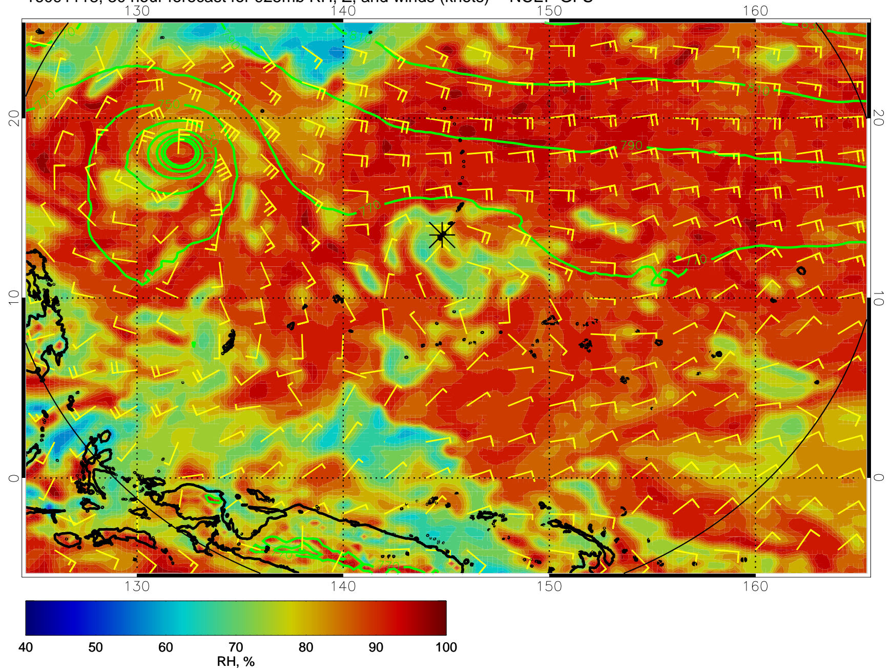
16091118, 30 hour forecast for 925mb RH, Z, and winds (knots) -- NCEP GFS
