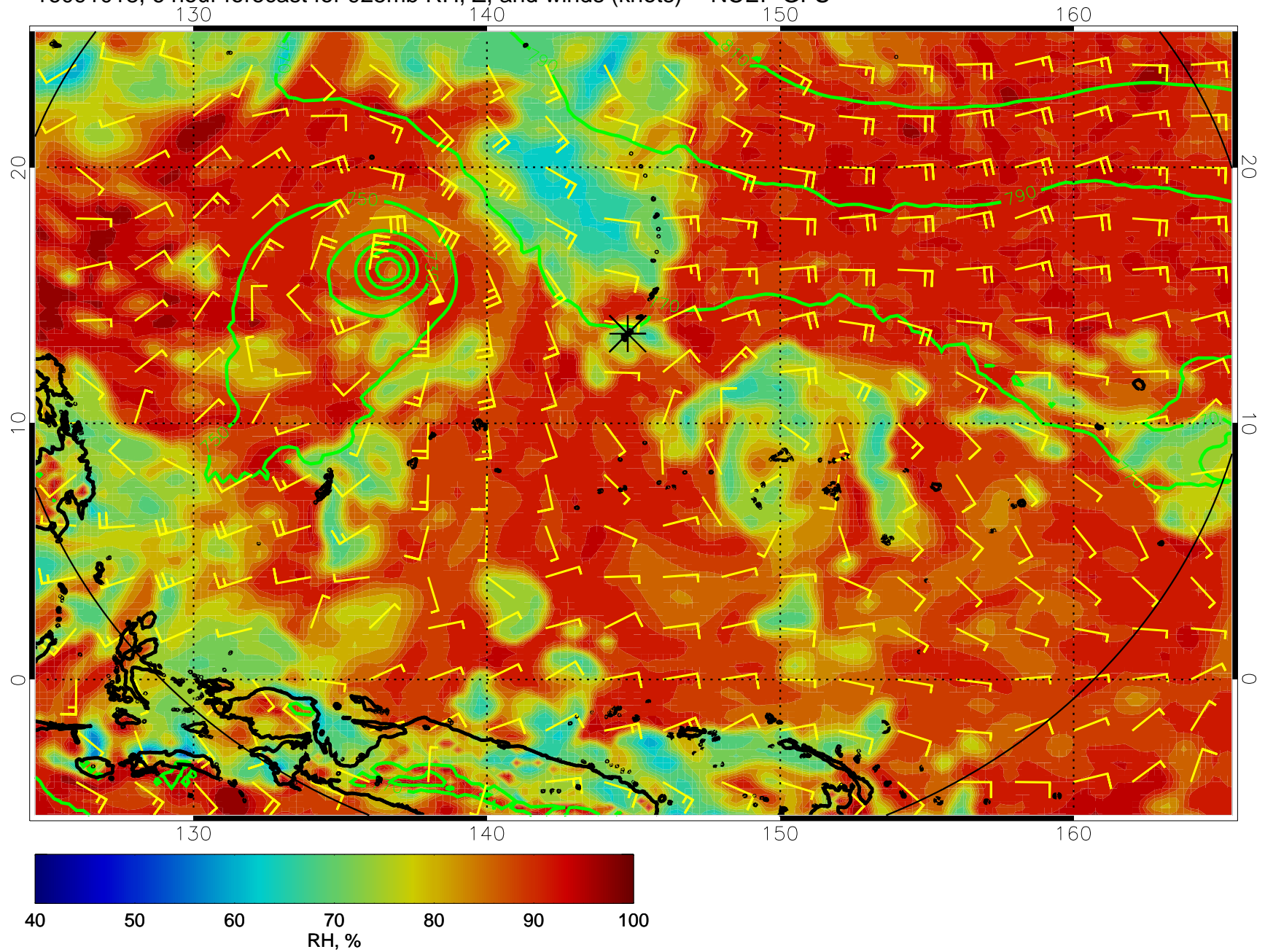
16091018, 6 hour forecast for 925mb RH, Z, and winds (knots) -- NCEP GFS
