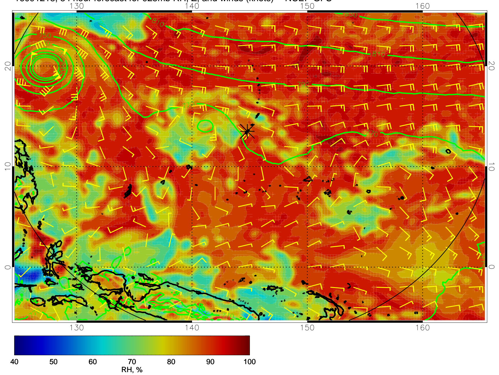
16091218, 54 hour forecast for 925mb RH, Z, and winds (knots) -- NCEP GFS
