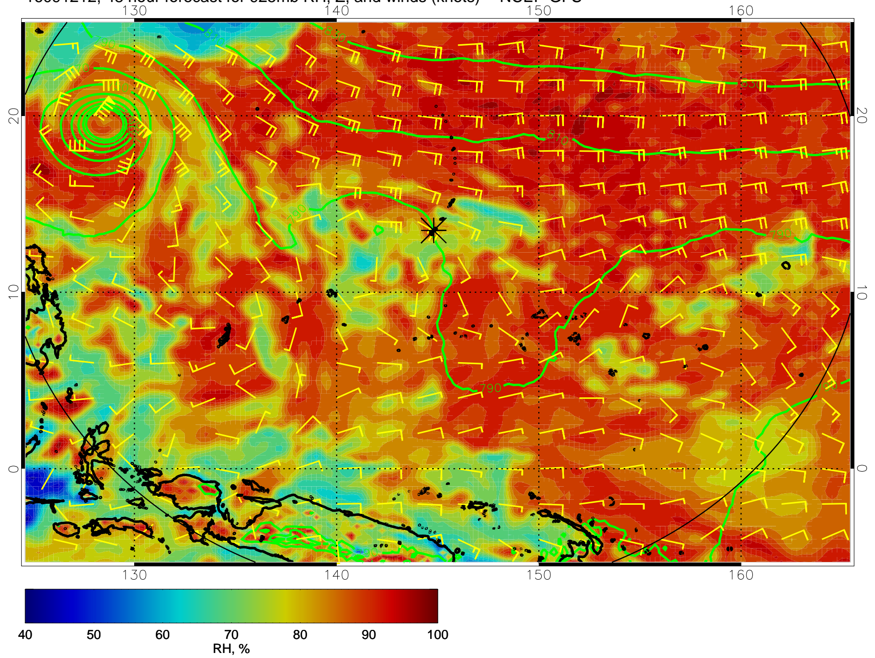
16091212, 48 hour forecast for 925mb RH, Z, and winds (knots) -- NCEP GFS
