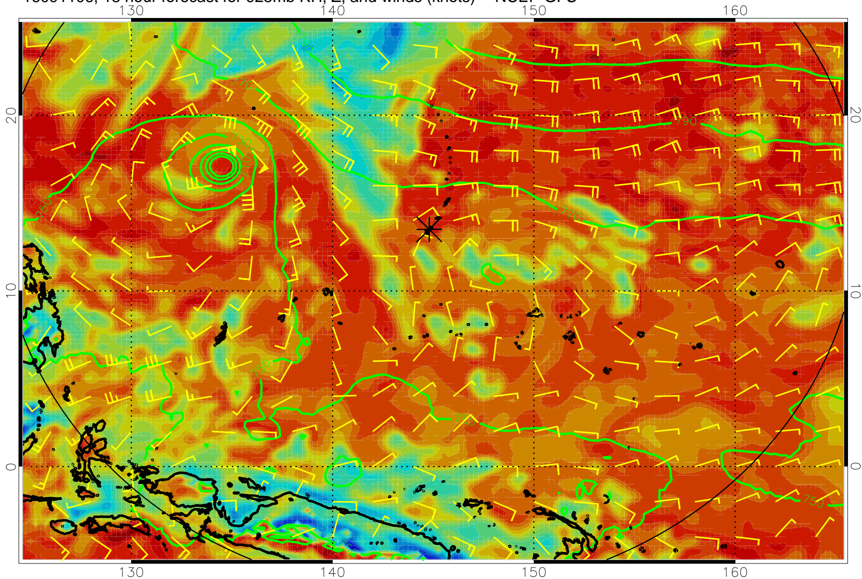
16091106, 18 hour forecast for 925mb RH, Z, and winds (knots) -- NCEP GFS
