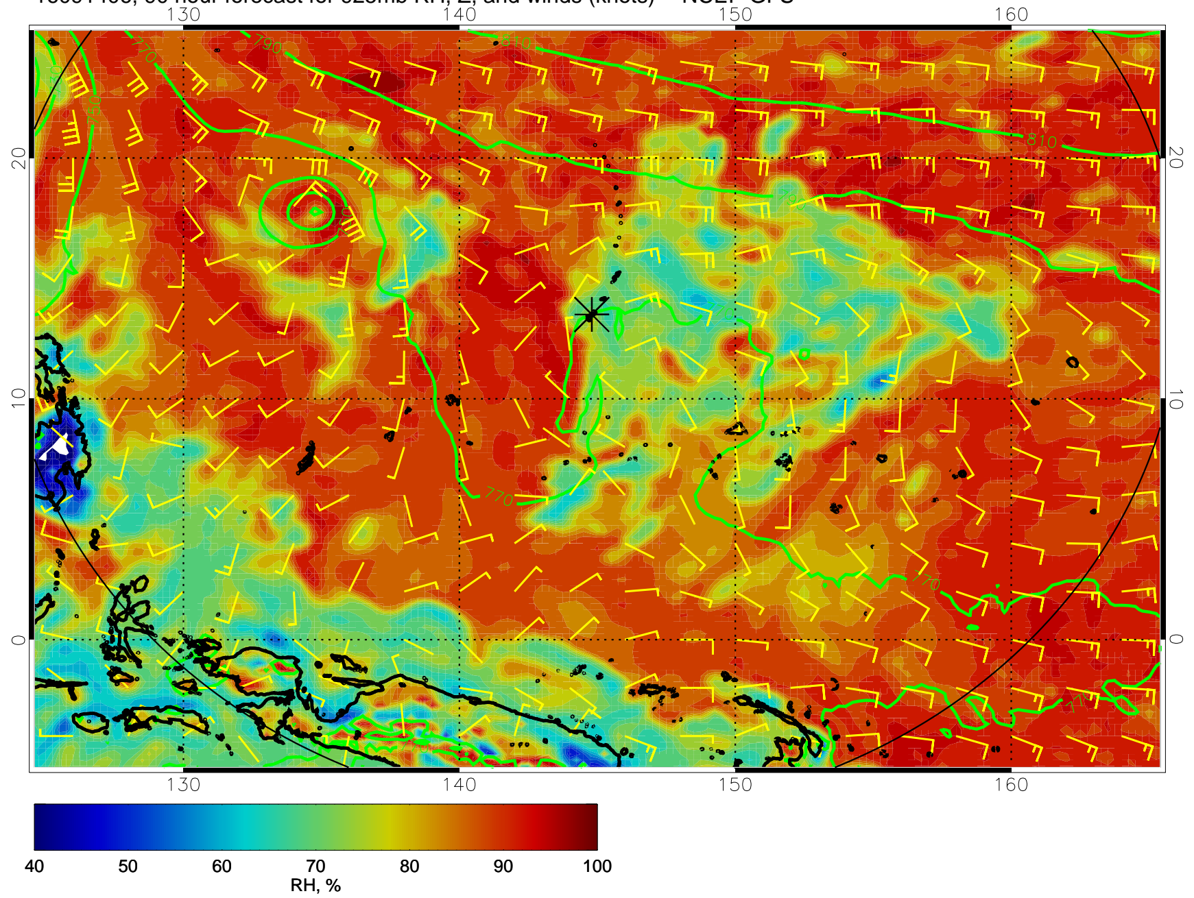
16091406, 90 hour forecast for 925mb RH, Z, and winds (knots) -- NCEP GFS
