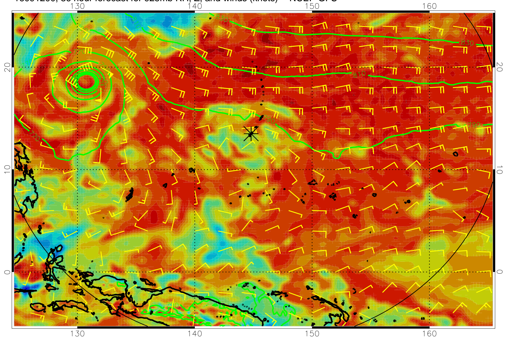
16091200, 36 hour forecast for 925mb RH, Z, and winds (knots) -- NCEP GFS
