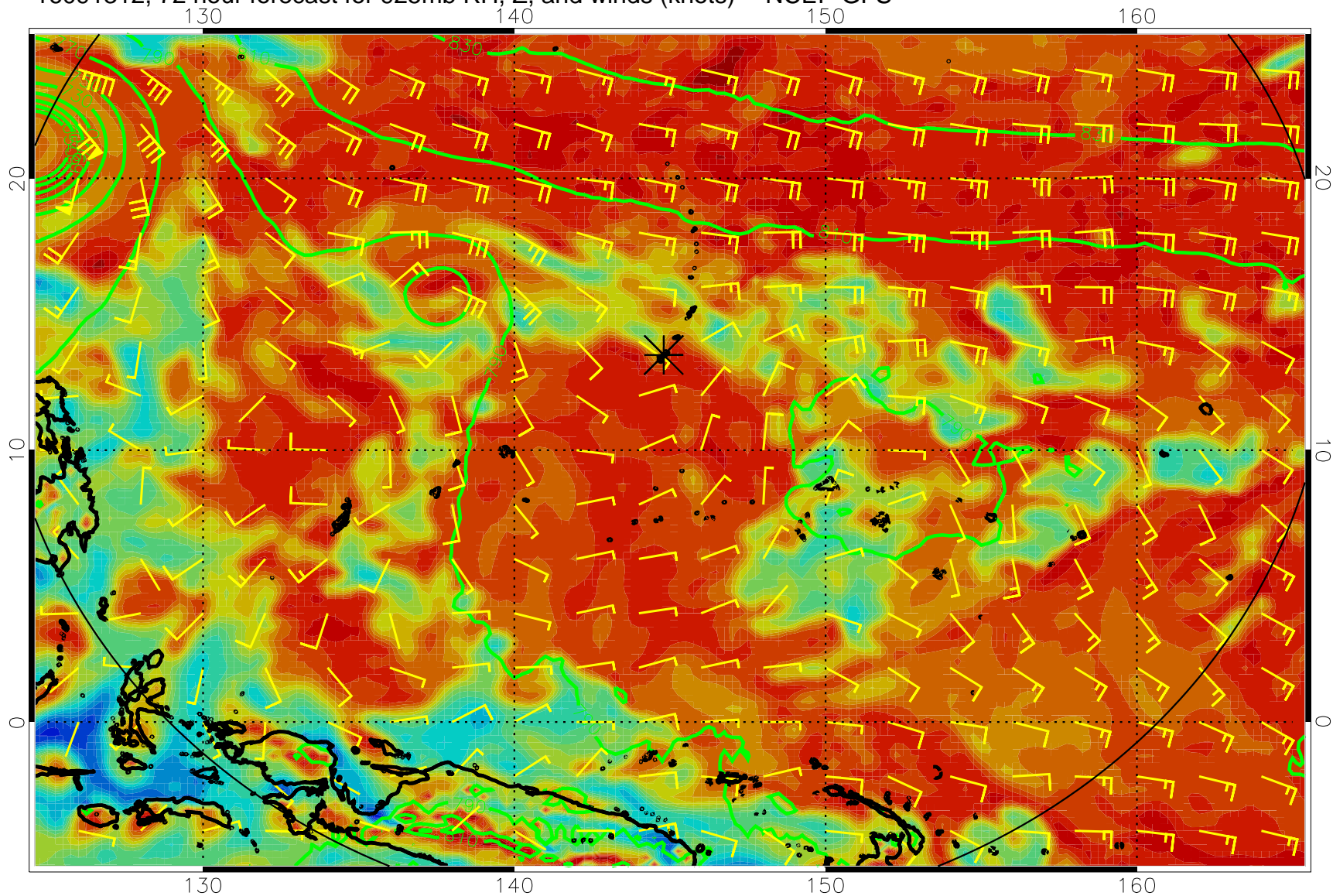
16091312, 72 hour forecast for 925mb RH, Z, and winds (knots) -- NCEP GFS
