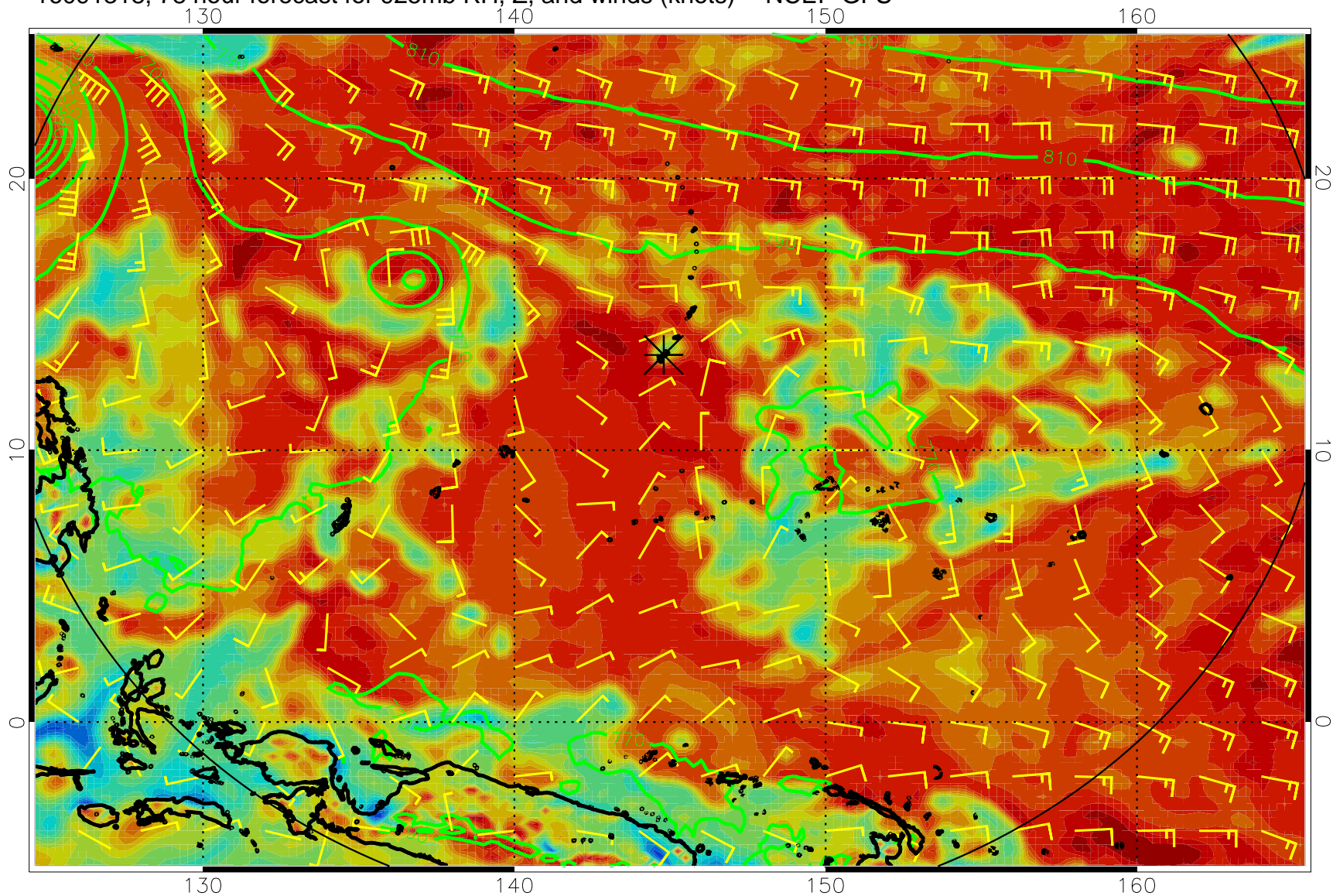
16091318, 78 hour forecast for 925mb RH, Z, and winds (knots) -- NCEP GFS
