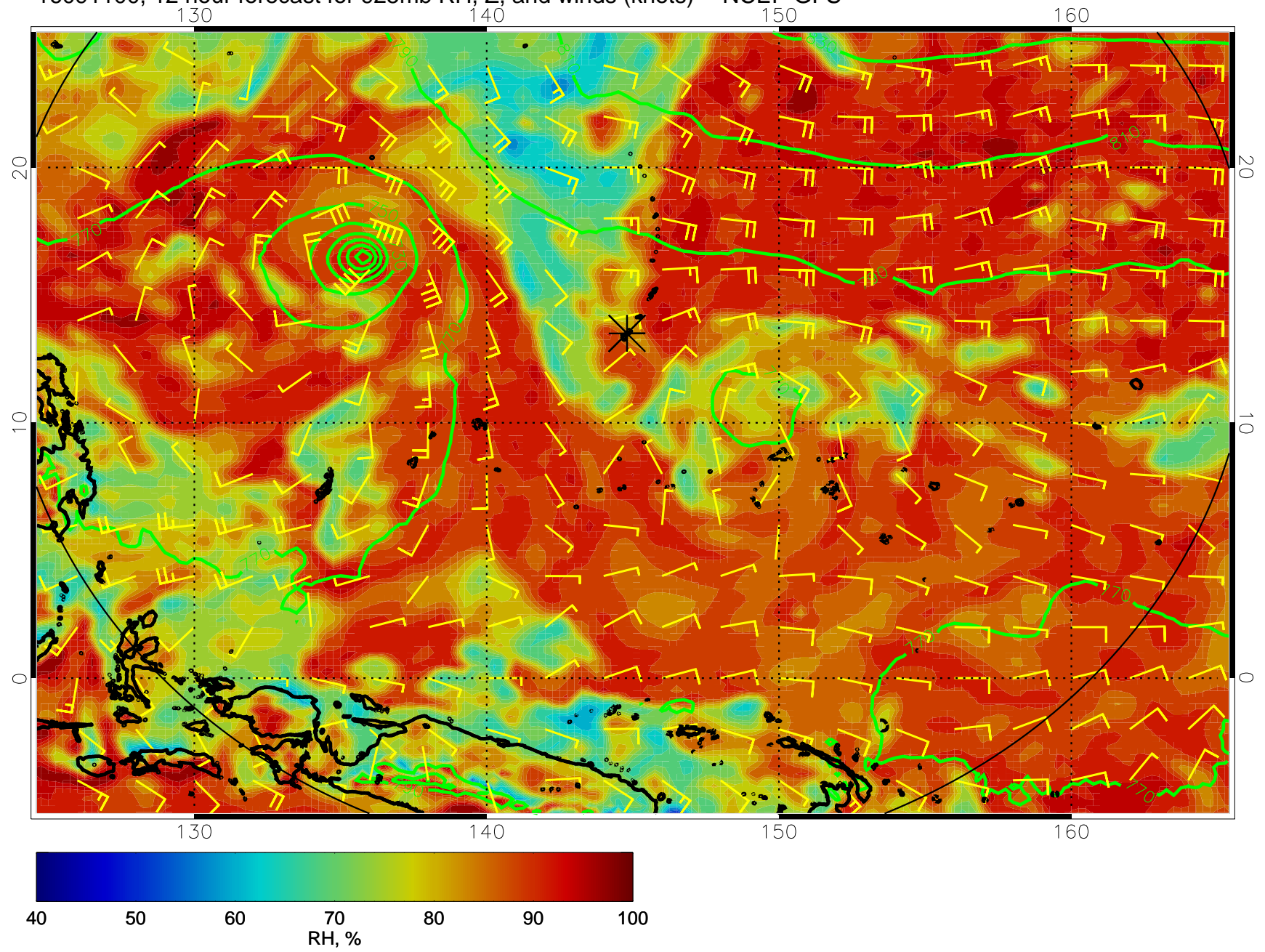
16091100, 12 hour forecast for 925mb RH, Z, and winds (knots) -- NCEP GFS
