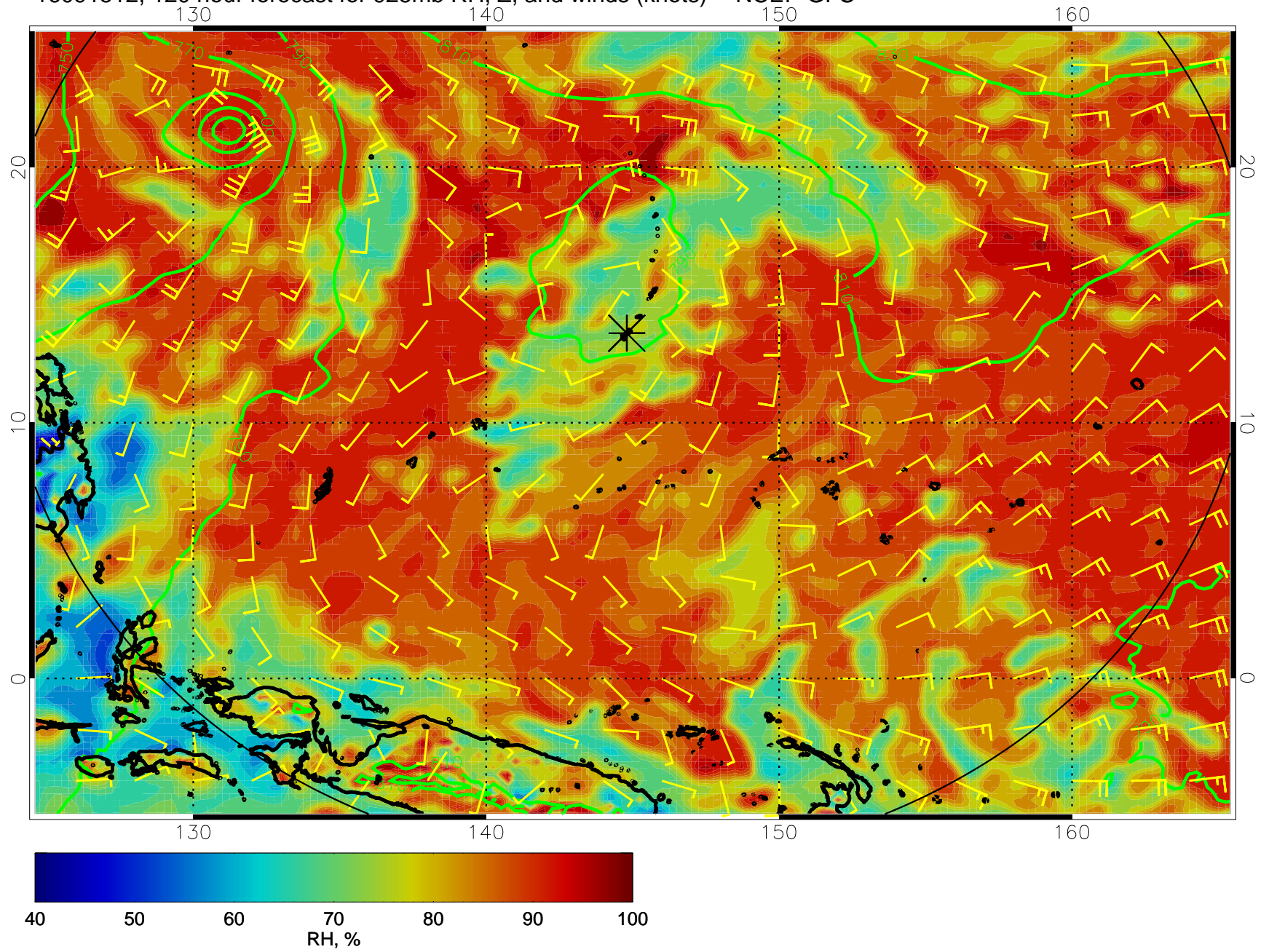
16091512, 120 hour forecast for 925mb RH, Z, and winds (knots) -- NCEP GFS
