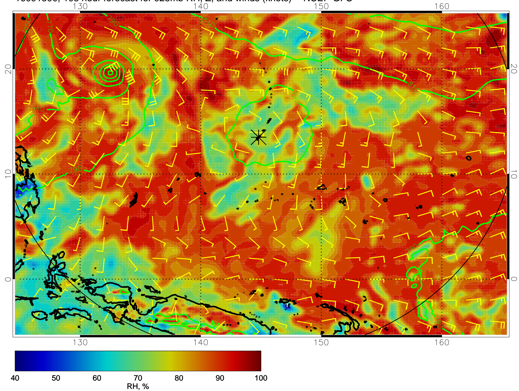
16091500, 108 hour forecast for 925mb RH, Z, and winds (knots) -- NCEP GFS
