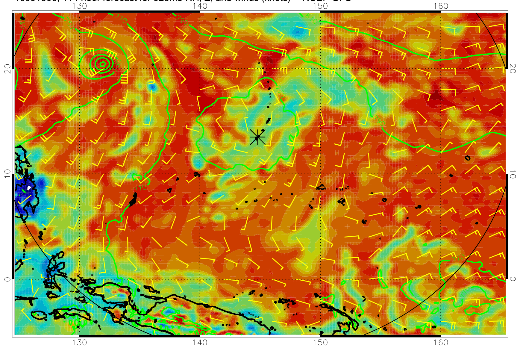
16091506, 114 hour forecast for 925mb RH, Z, and winds (knots) -- NCEP GFS
