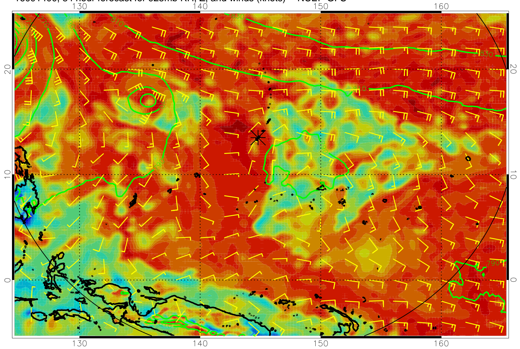
16091400, 84 hour forecast for 925mb RH, Z, and winds (knots) -- NCEP GFS
