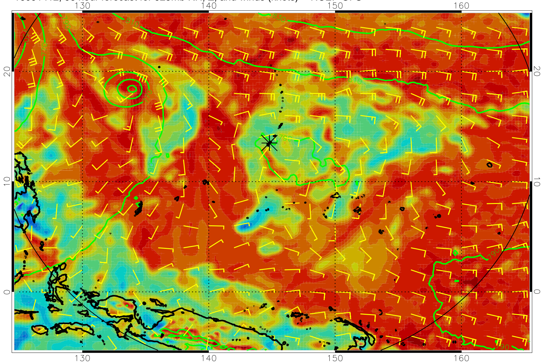
16091412, 96 hour forecast for 925mb RH, Z, and winds (knots) -- NCEP GFS
