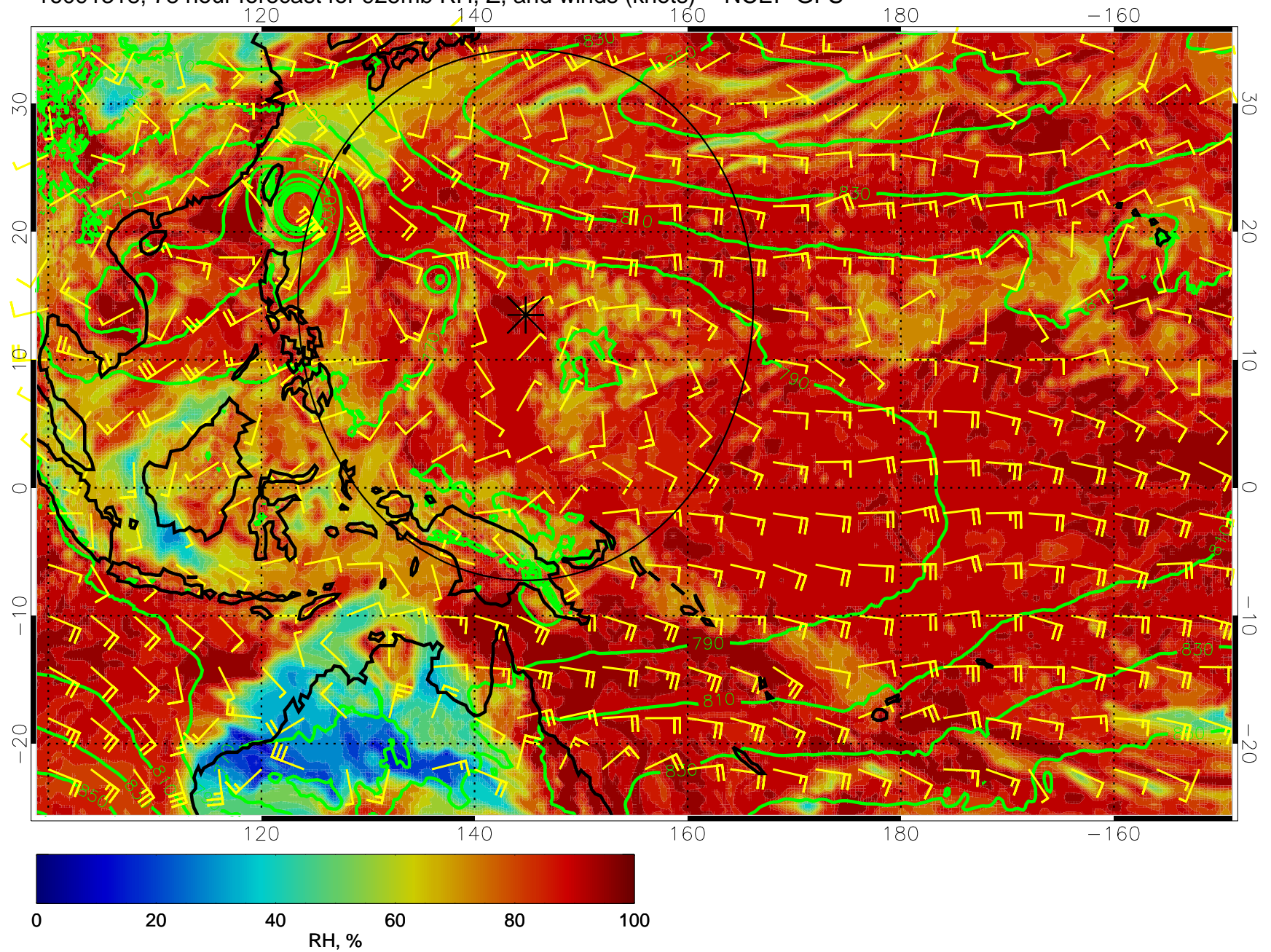
16091318, 78 hour forecast for 925mb RH, Z, and winds (knots) -- NCEP GFS
