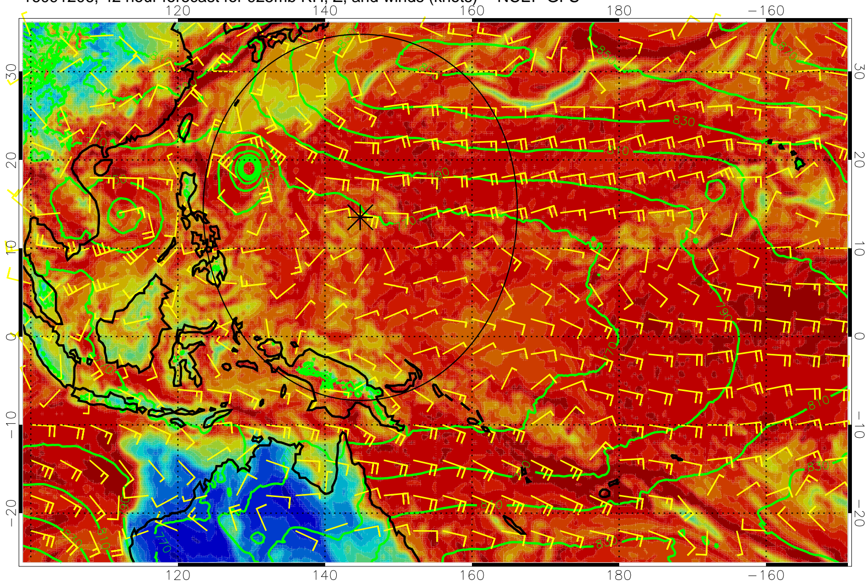
16091206, 42 hour forecast for 925mb RH, Z, and winds (knots) -- NCEP GFS
