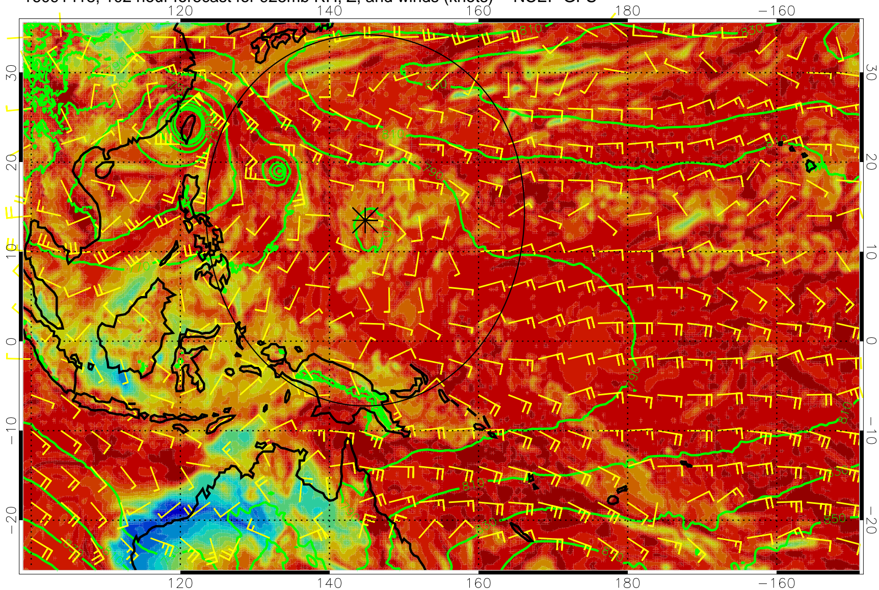
16091418, 102 hour forecast for 925mb RH, Z, and winds (knots) -- NCEP GFS
