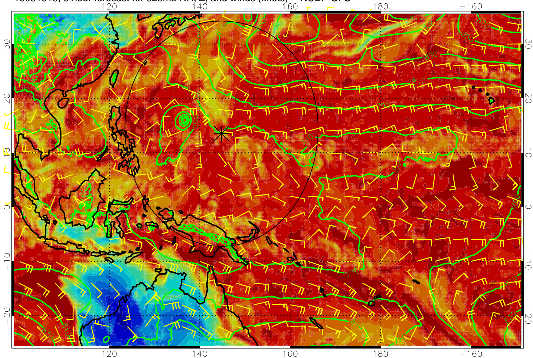
16091018, 6 hour forecast for 925mb RH, Z, and winds (knots) -- NCEP GFS
