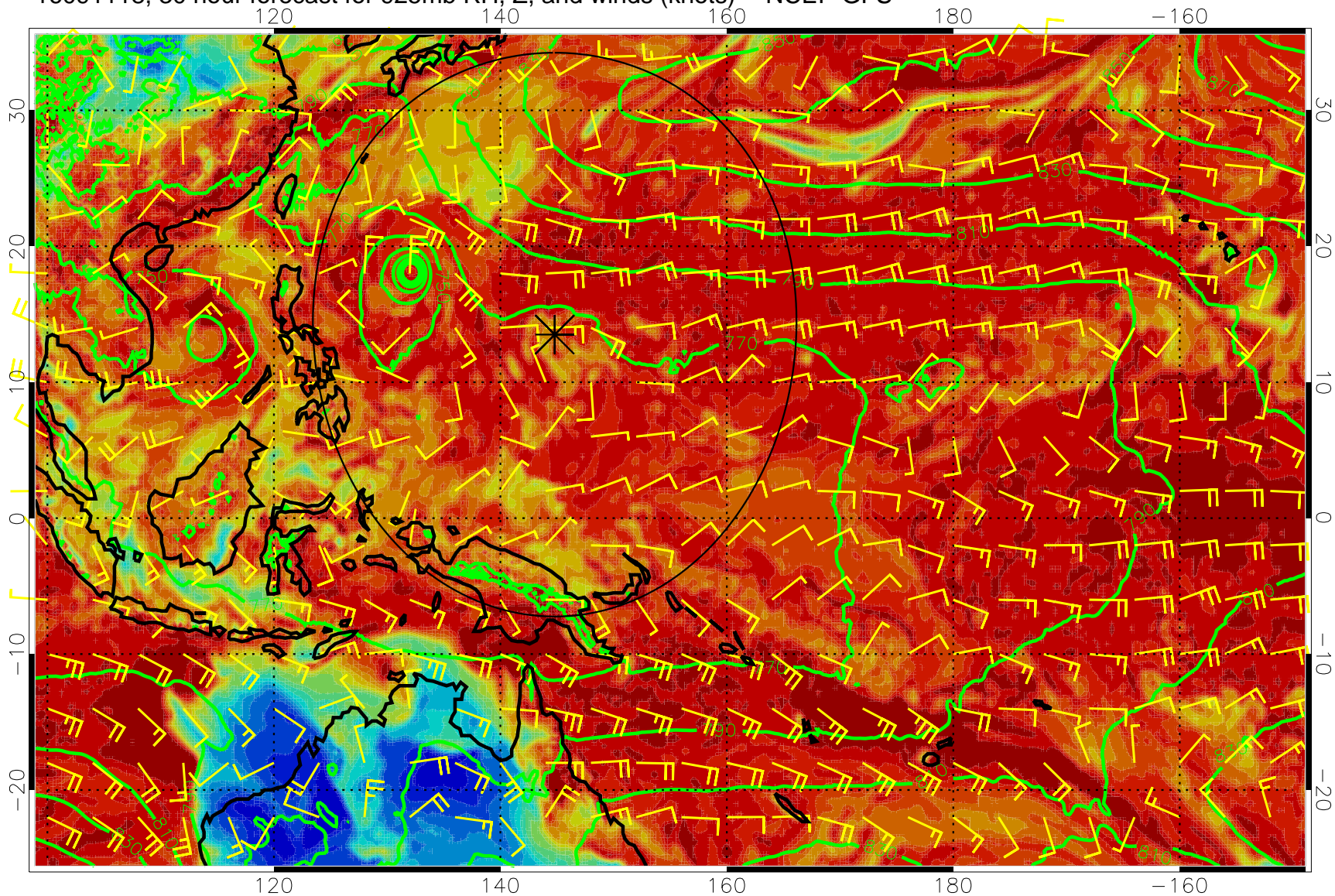
16091118, 30 hour forecast for 925mb RH, Z, and winds (knots) -- NCEP GFS
