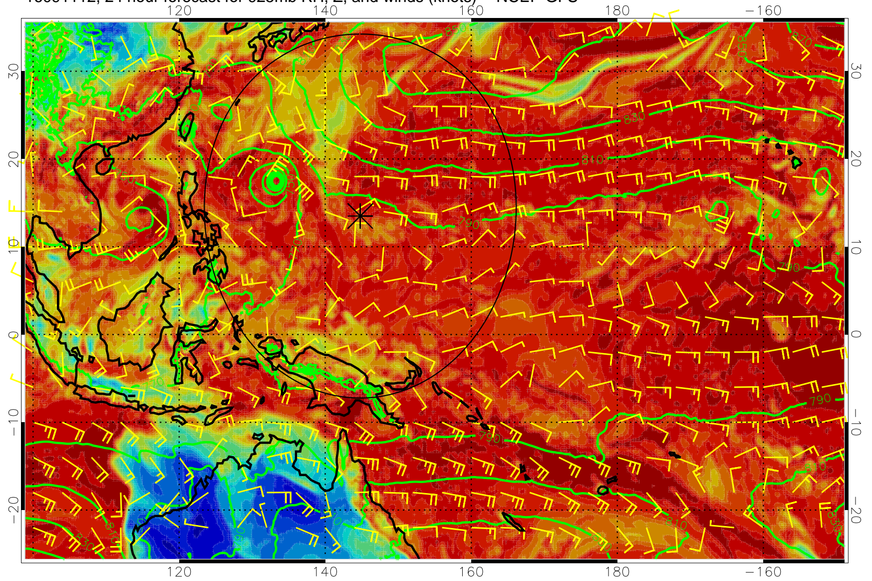
16091112, 24 hour forecast for 925mb RH, Z, and winds (knots) -- NCEP GFS
