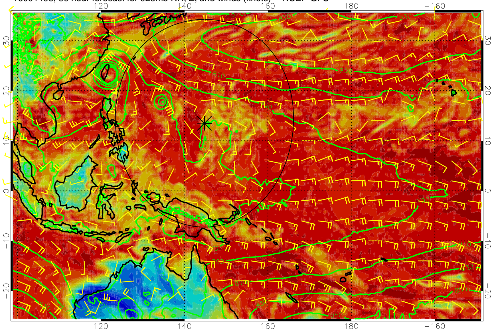
16091406, 90 hour forecast for 925mb RH, Z, and winds (knots) -- NCEP GFS
