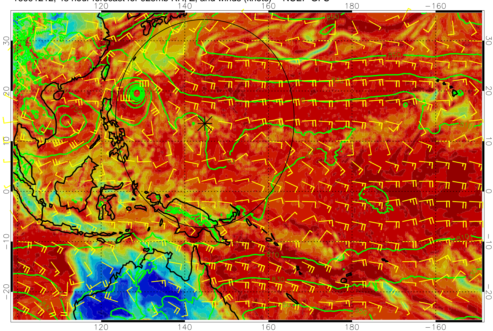
16091212, 48 hour forecast for 925mb RH, Z, and winds (knots) -- NCEP GFS
