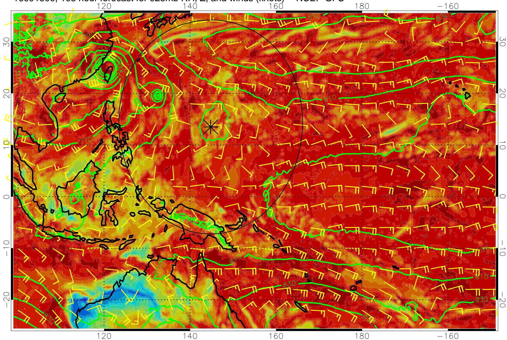
16091500, 108 hour forecast for 925mb RH, Z, and winds (knots) -- NCEP GFS
