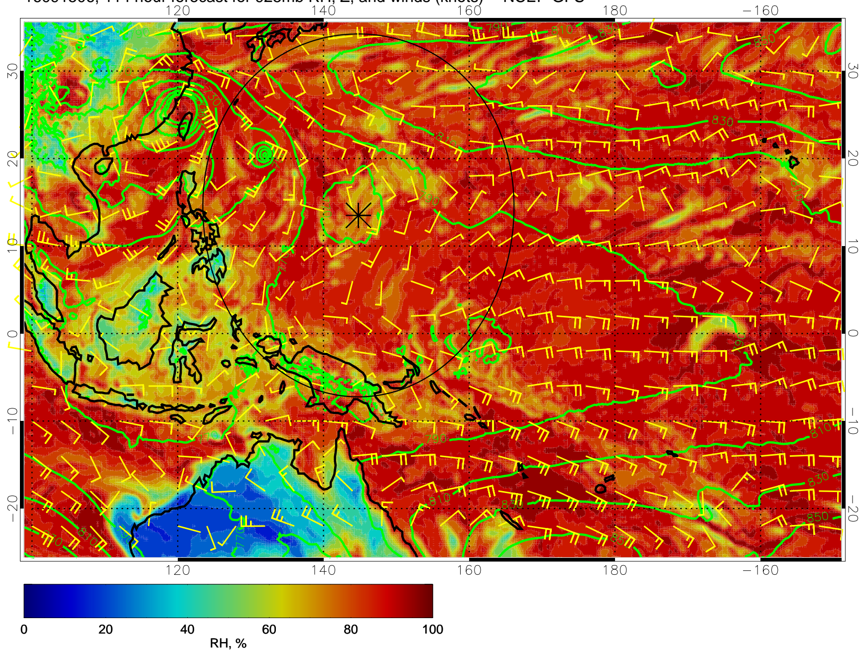
16091506, 114 hour forecast for 925mb RH, Z, and winds (knots) -- NCEP GFS
