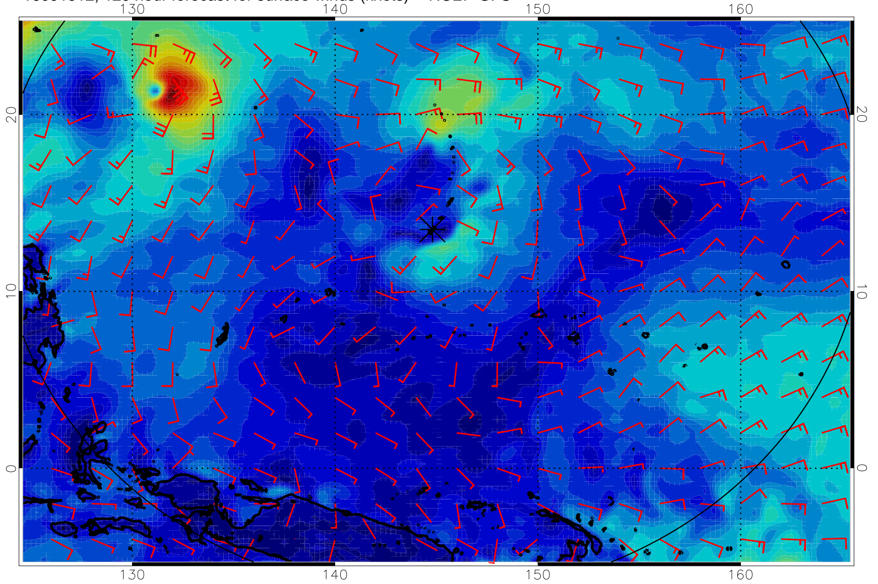
16091512, 120 hour forecast for surface winds (knots) -- NCEP GFS
