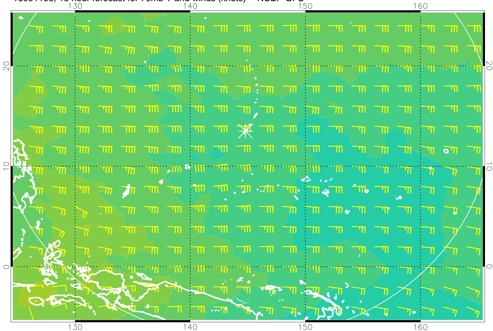
16091106, 18 hour forecast for 70mb T and winds (knots) -- NCEP GFS
