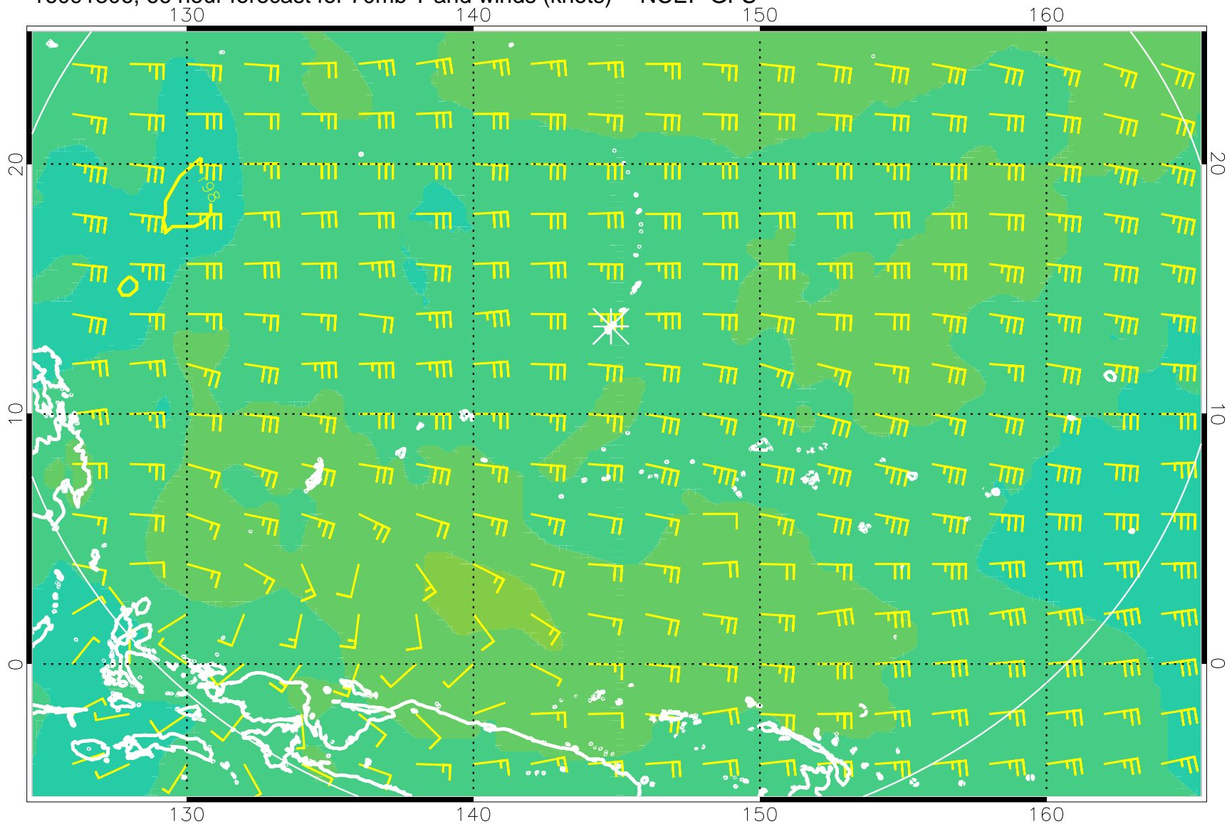
16091306, 66 hour forecast for 70mb T and winds (knots) -- NCEP GFS
