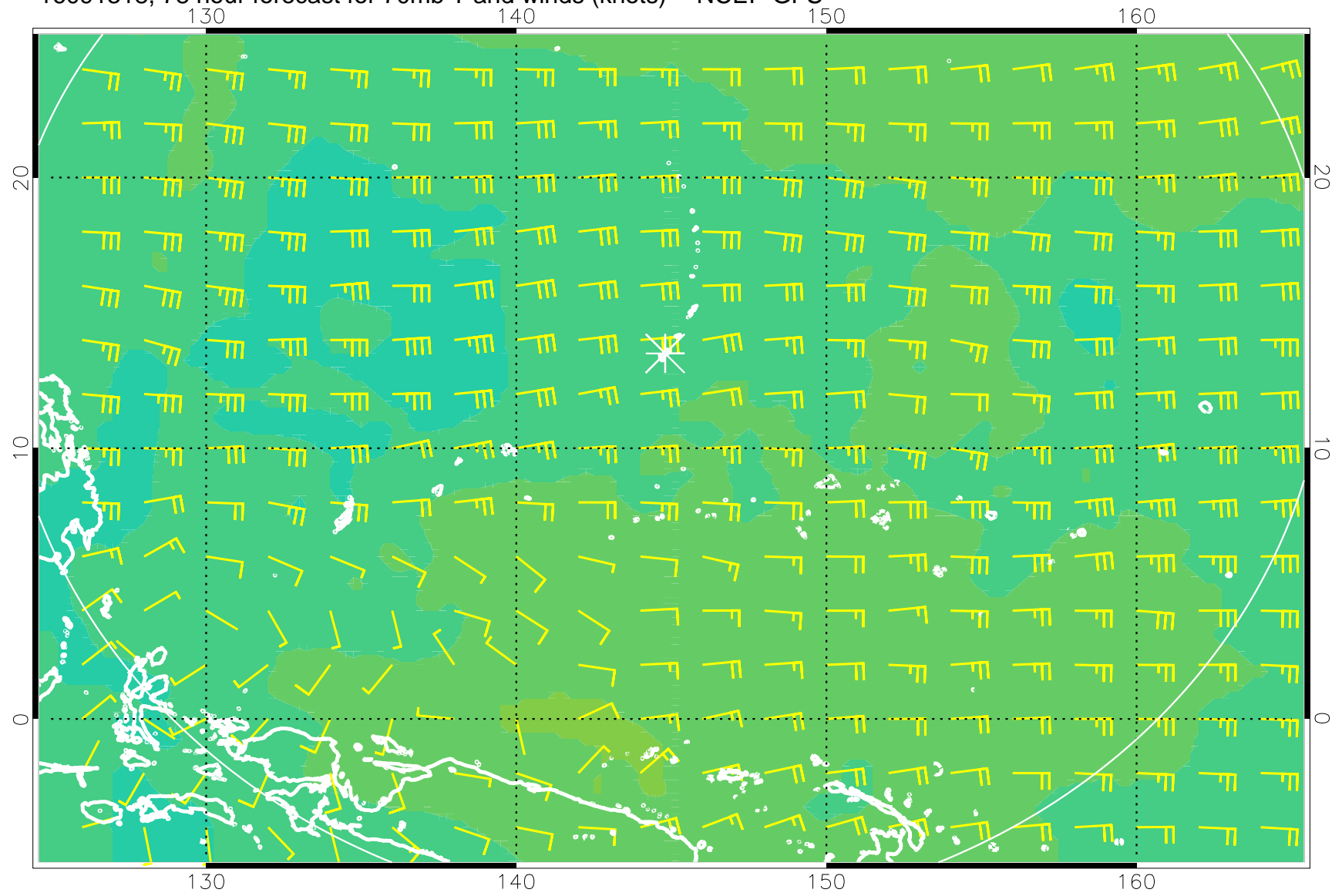
16091318, 78 hour forecast for 70mb T and winds (knots) -- NCEP GFS
