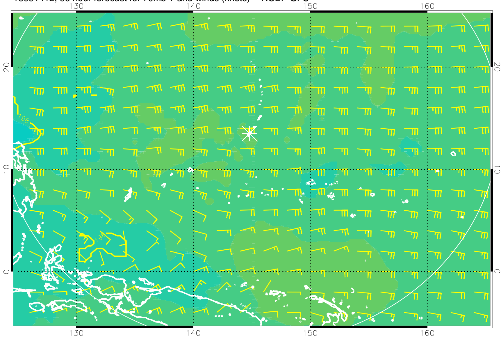
16091412, 96 hour forecast for 70mb T and winds (knots) -- NCEP GFS
