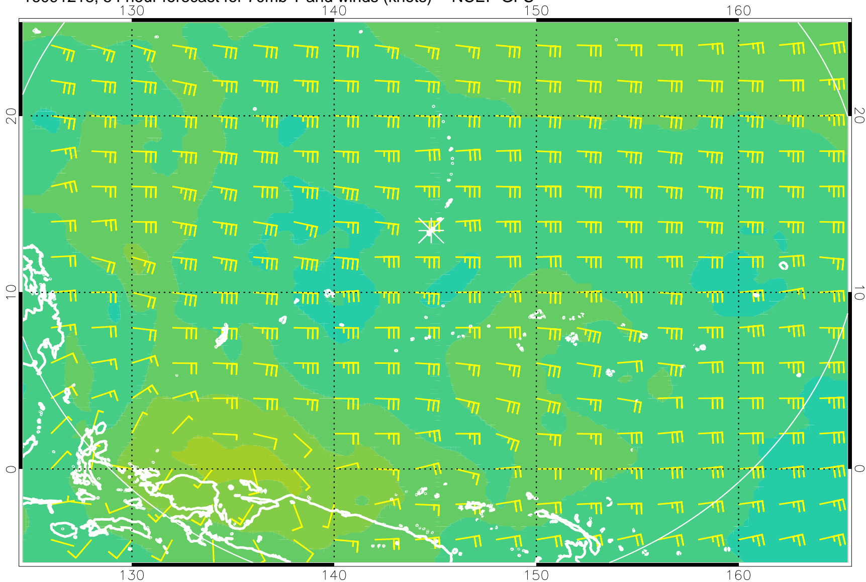
16091218, 54 hour forecast for 70mb T and winds (knots) -- NCEP GFS
