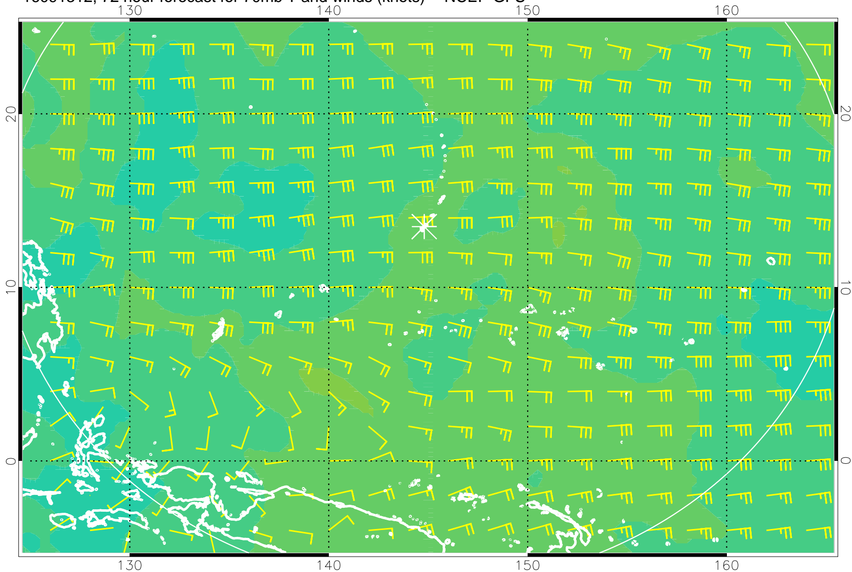
16091312, 72 hour forecast for 70mb T and winds (knots) -- NCEP GFS
