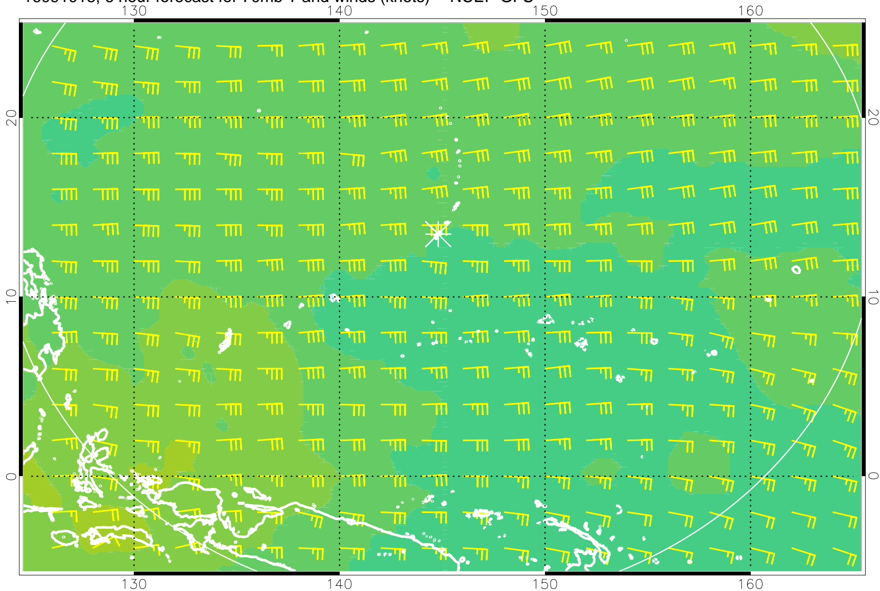
16091018, 6 hour forecast for 70mb T and winds (knots) -- NCEP GFS
