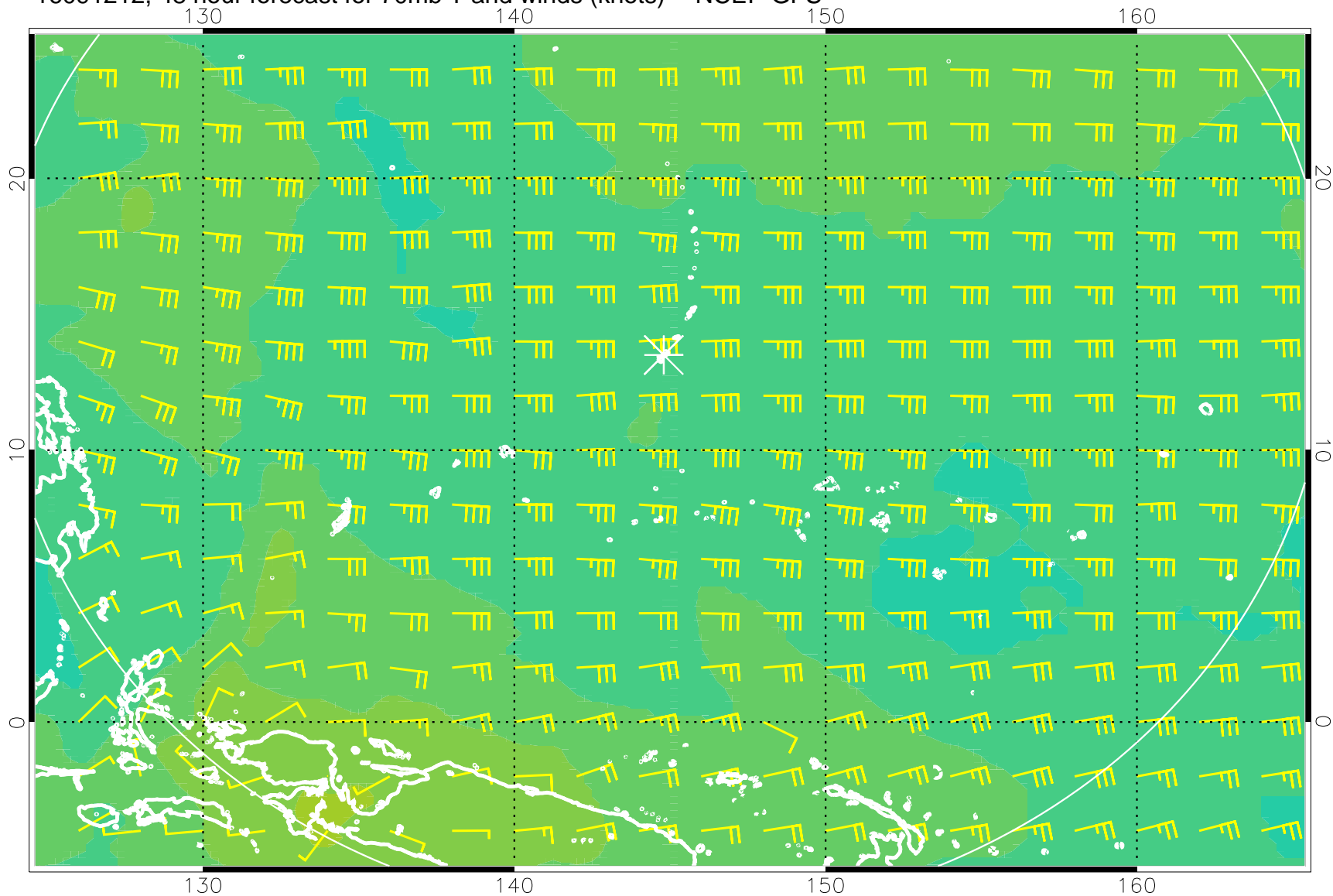
16091212, 48 hour forecast for 70mb T and winds (knots) -- NCEP GFS
