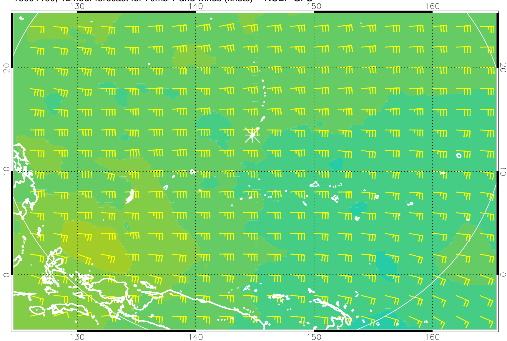
16091100, 12 hour forecast for 70mb T and winds (knots) -- NCEP GFS
