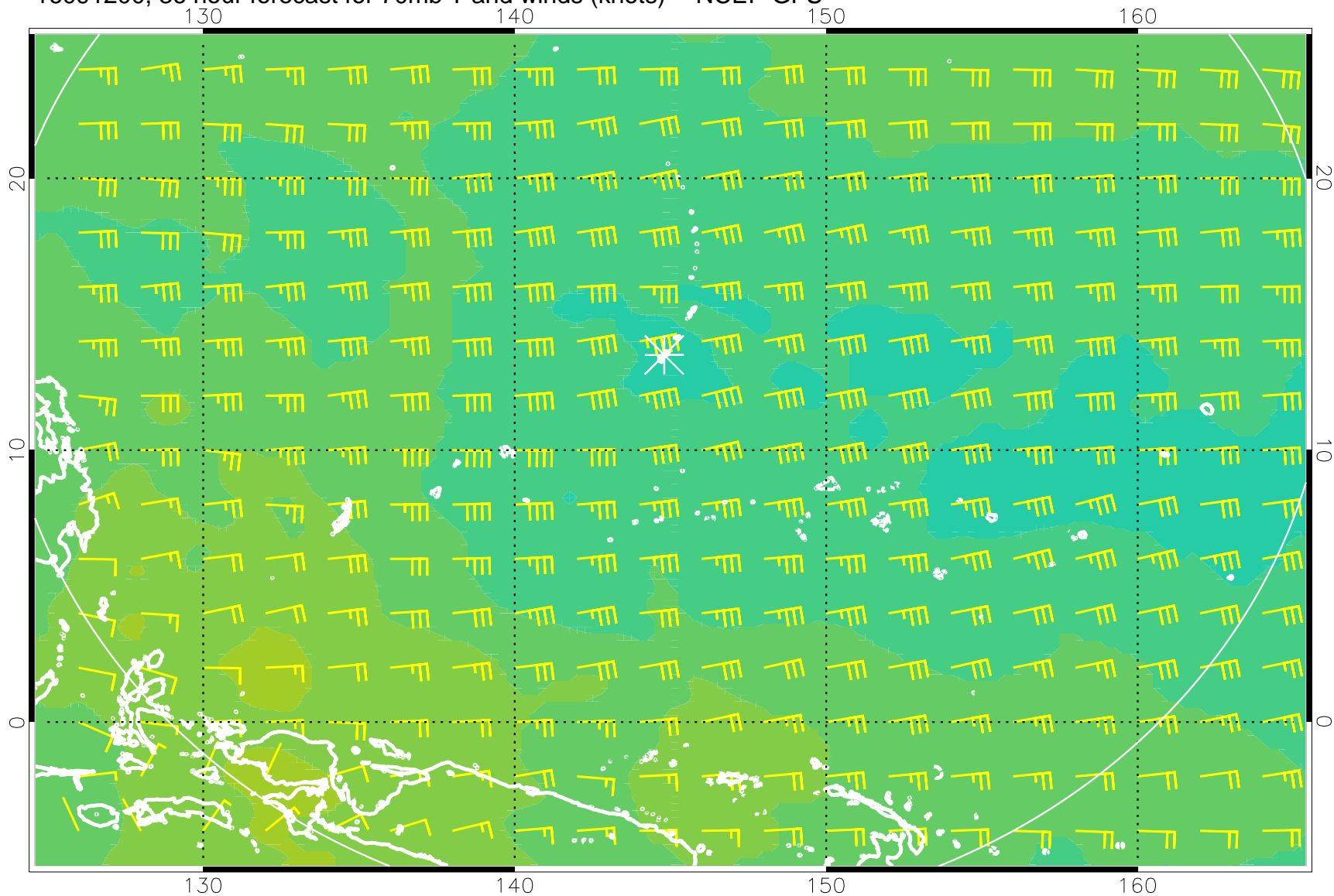
16091200, 36 hour forecast for 70mb T and winds (knots) -- NCEP GFS
