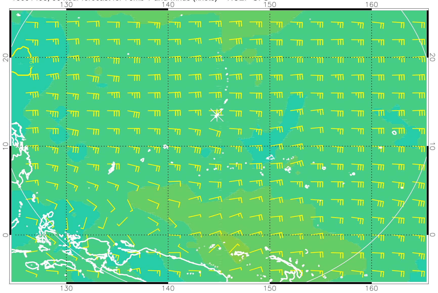
16091406, 90 hour forecast for 70mb T and winds (knots) -- NCEP GFS
