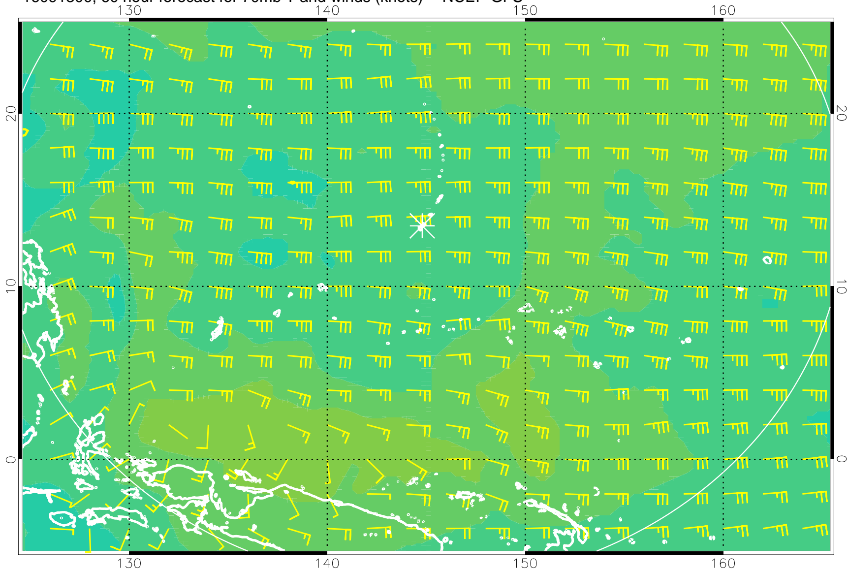
16091300, 60 hour forecast for 70mb T and winds (knots) -- NCEP GFS
