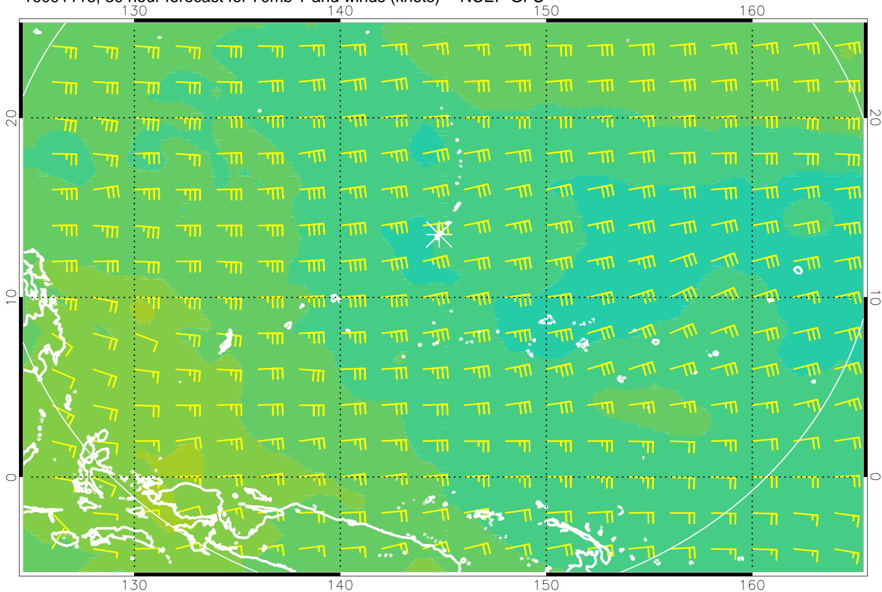
16091118, 30 hour forecast for 70mb T and winds (knots) -- NCEP GFS
