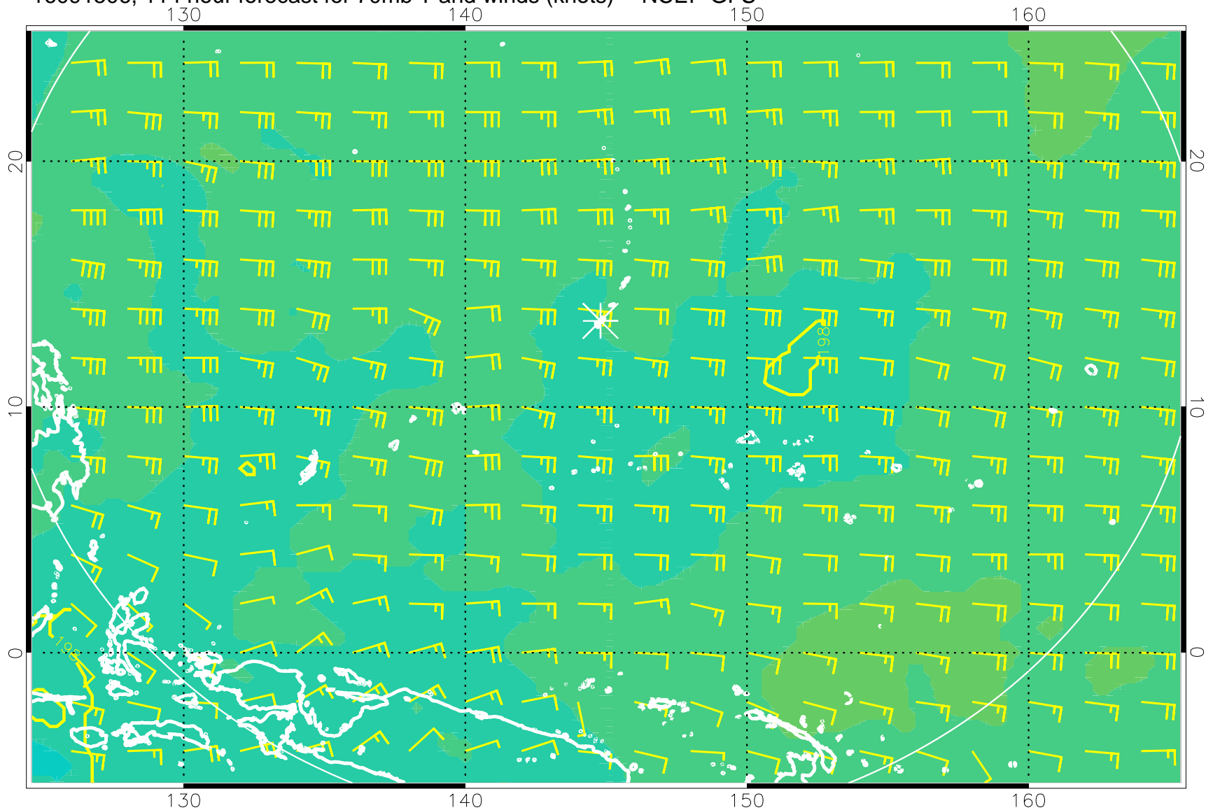
16091506, 114 hour forecast for 70mb T and winds (knots) -- NCEP GFS
