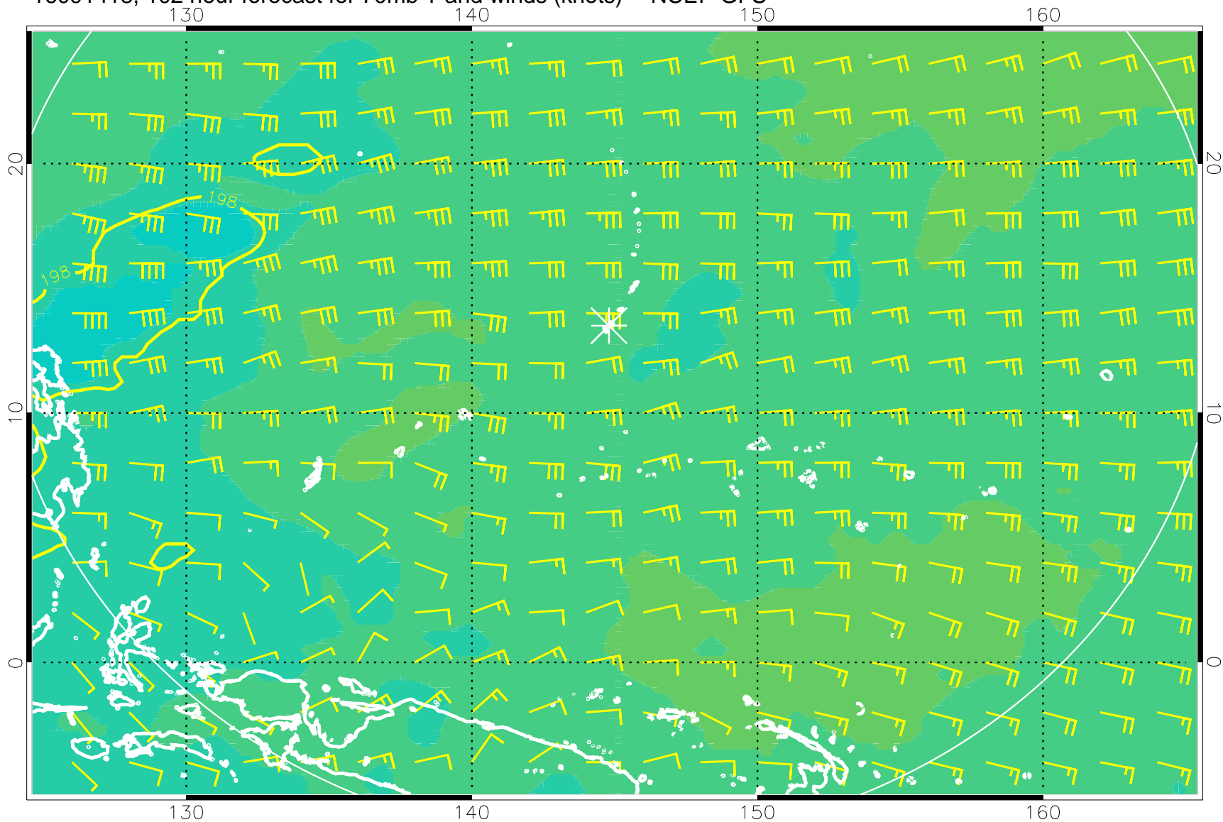
16091418, 102 hour forecast for 70mb T and winds (knots) -- NCEP GFS
