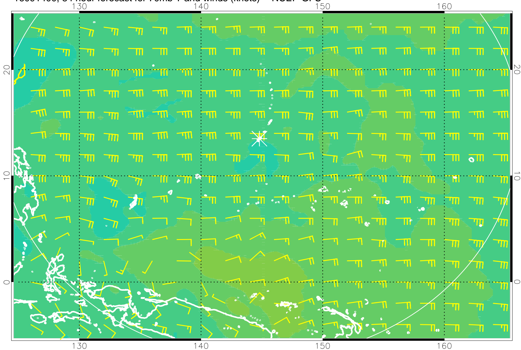
16091400, 84 hour forecast for 70mb T and winds (knots) -- NCEP GFS
