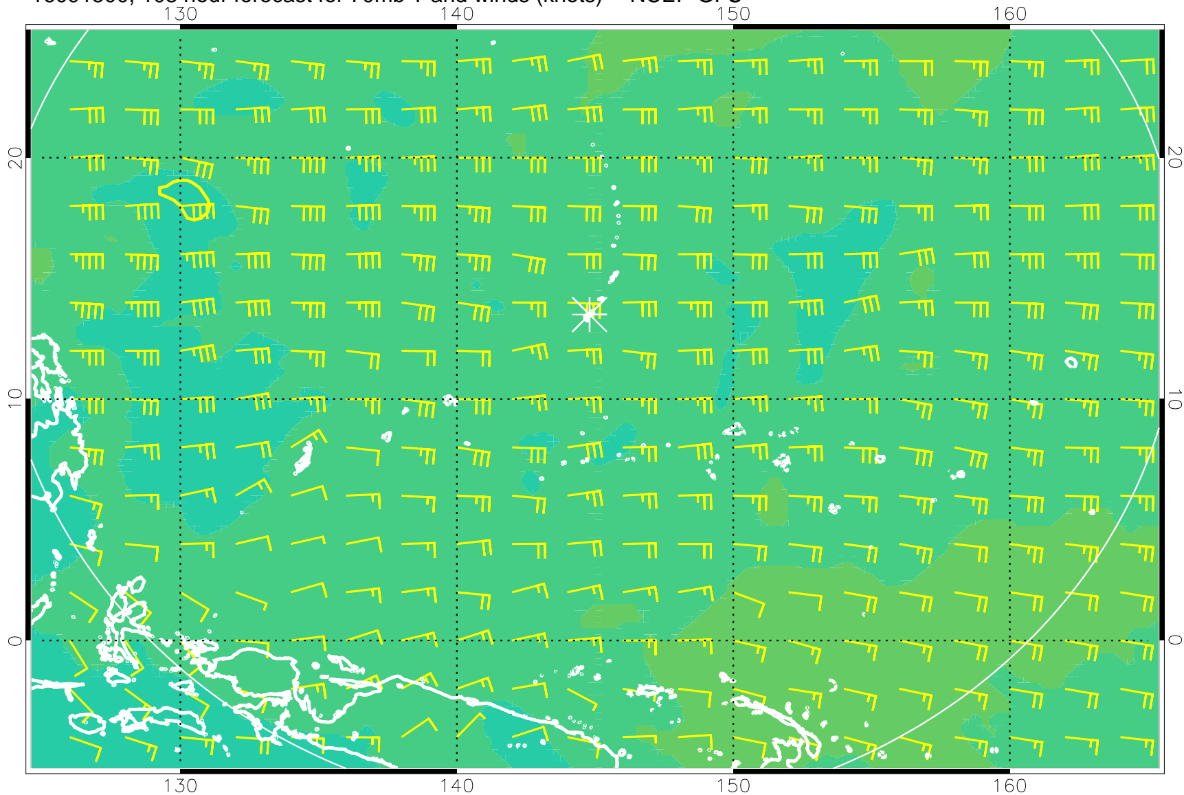
16091500, 108 hour forecast for 70mb T and winds (knots) -- NCEP GFS
