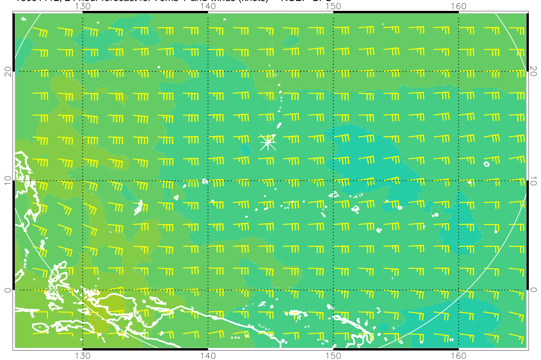
16091112, 24 hour forecast for 70mb T and winds (knots) -- NCEP GFS
