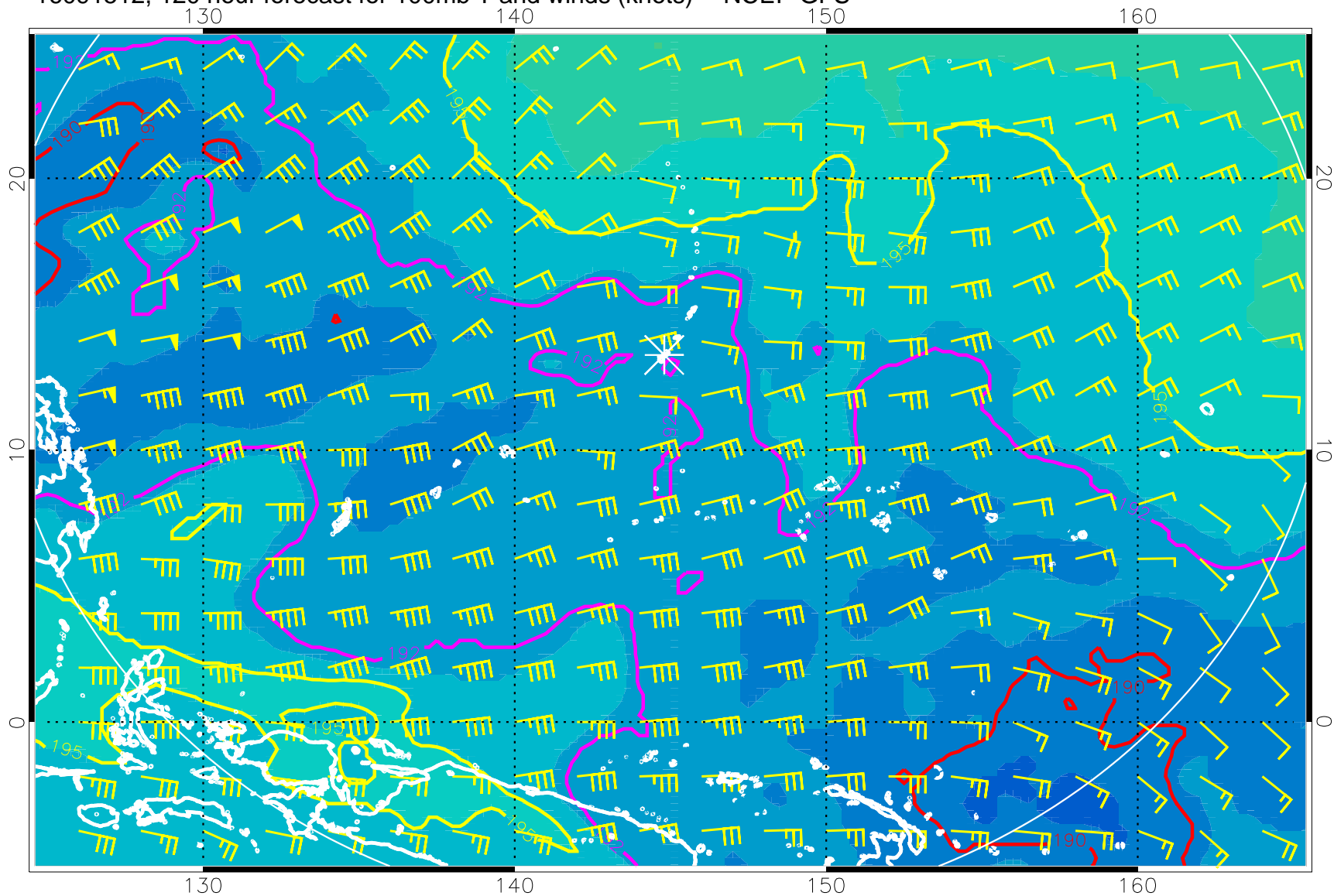
16091512, 120 hour forecast for 100mb T and winds (knots) -- NCEP GFS
