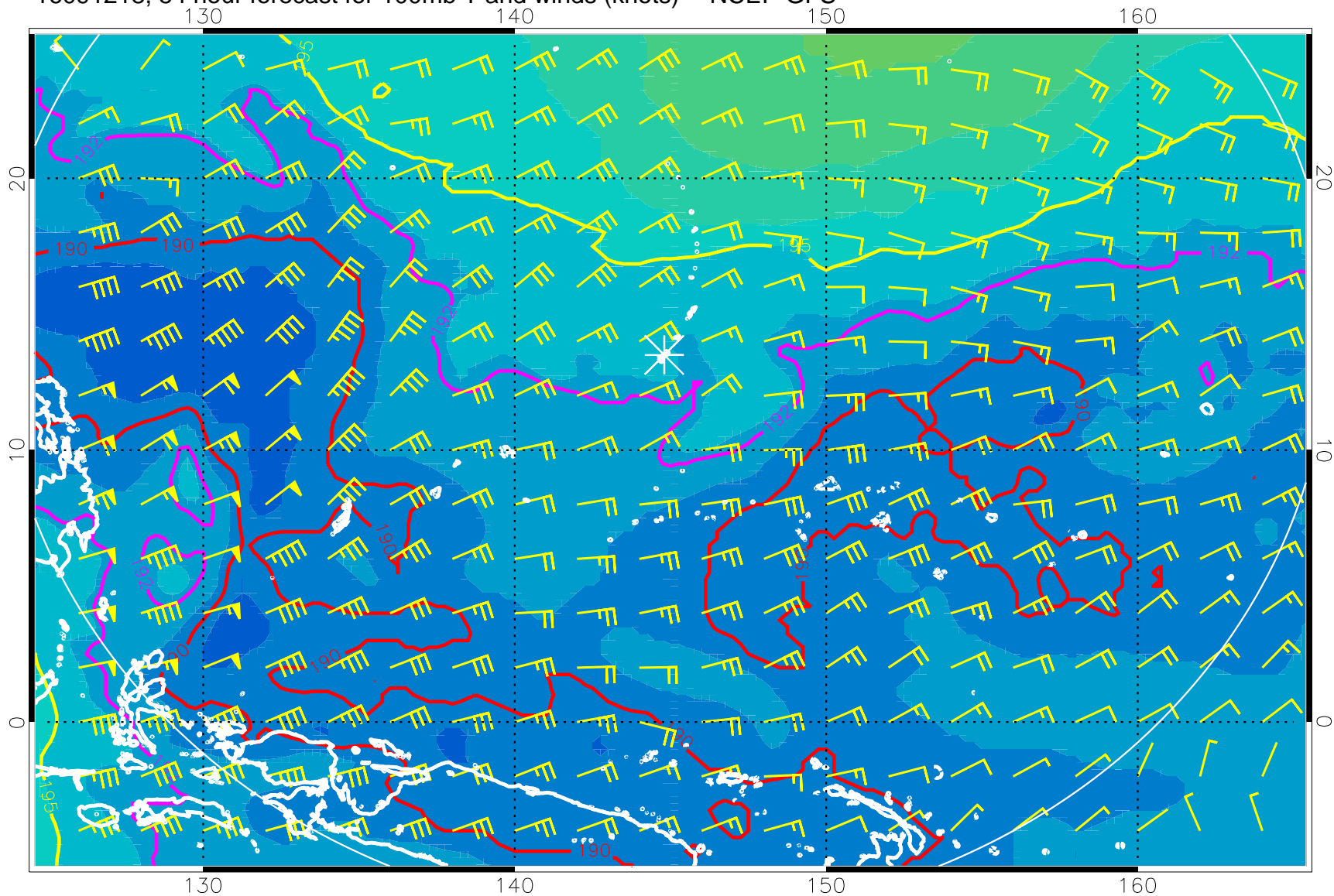
16091218, 54 hour forecast for 100mb T and winds (knots) -- NCEP GFS
