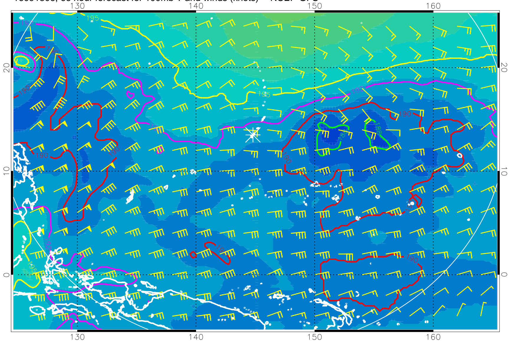
16091306, 66 hour forecast for 100mb T and winds (knots) -- NCEP GFS
