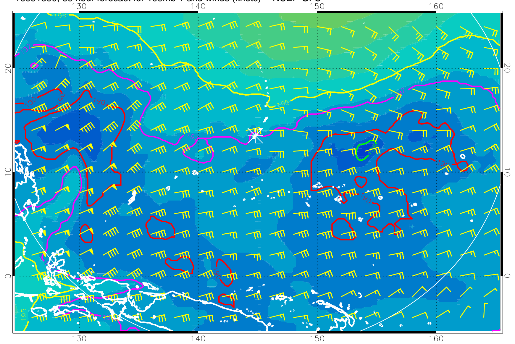
16091300, 60 hour forecast for 100mb T and winds (knots) -- NCEP GFS
