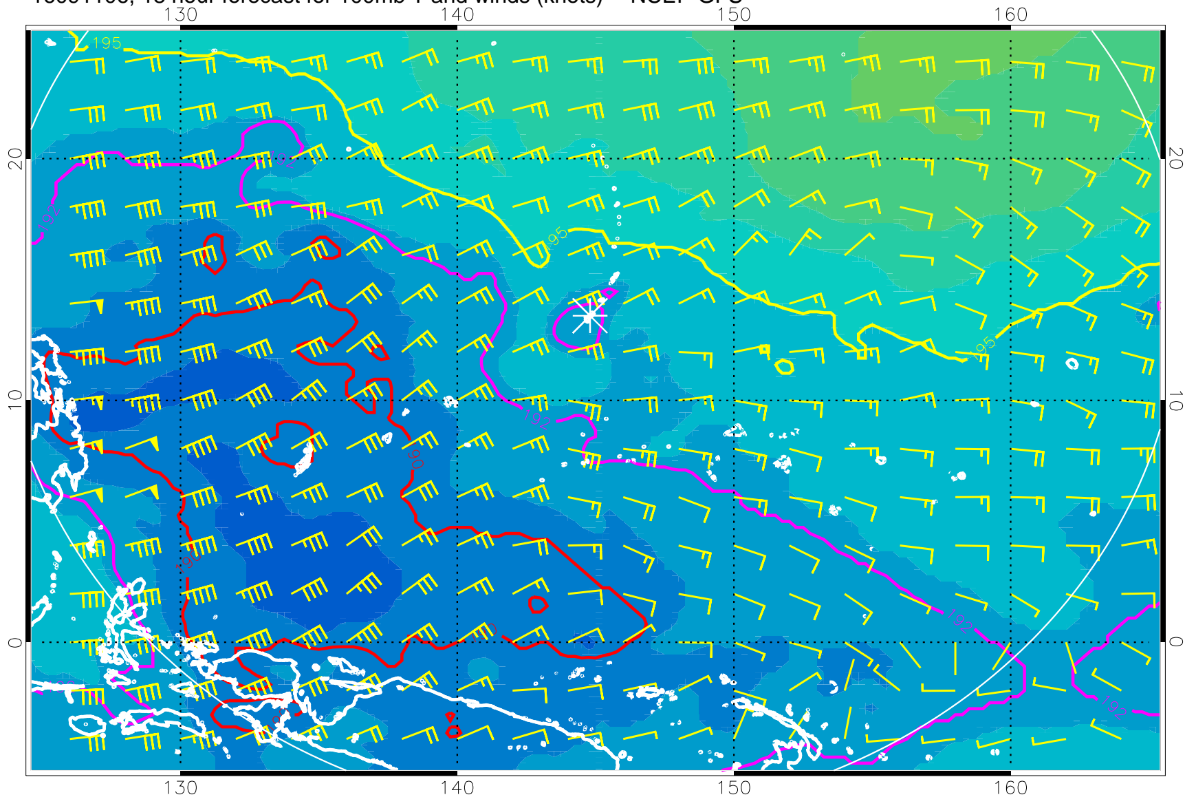
16091106, 18 hour forecast for 100mb T and winds (knots) -- NCEP GFS
