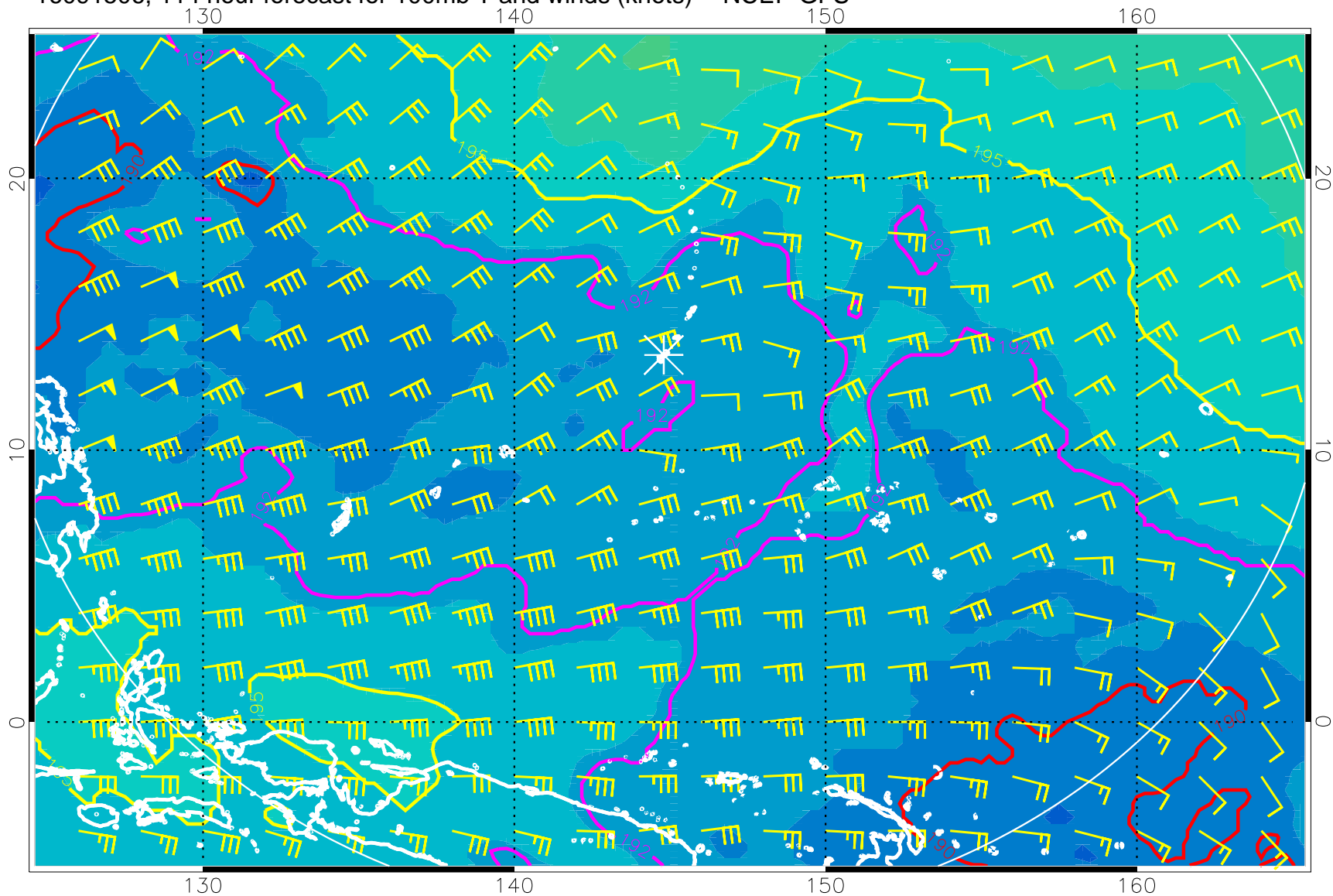
16091506, 114 hour forecast for 100mb T and winds (knots) -- NCEP GFS
