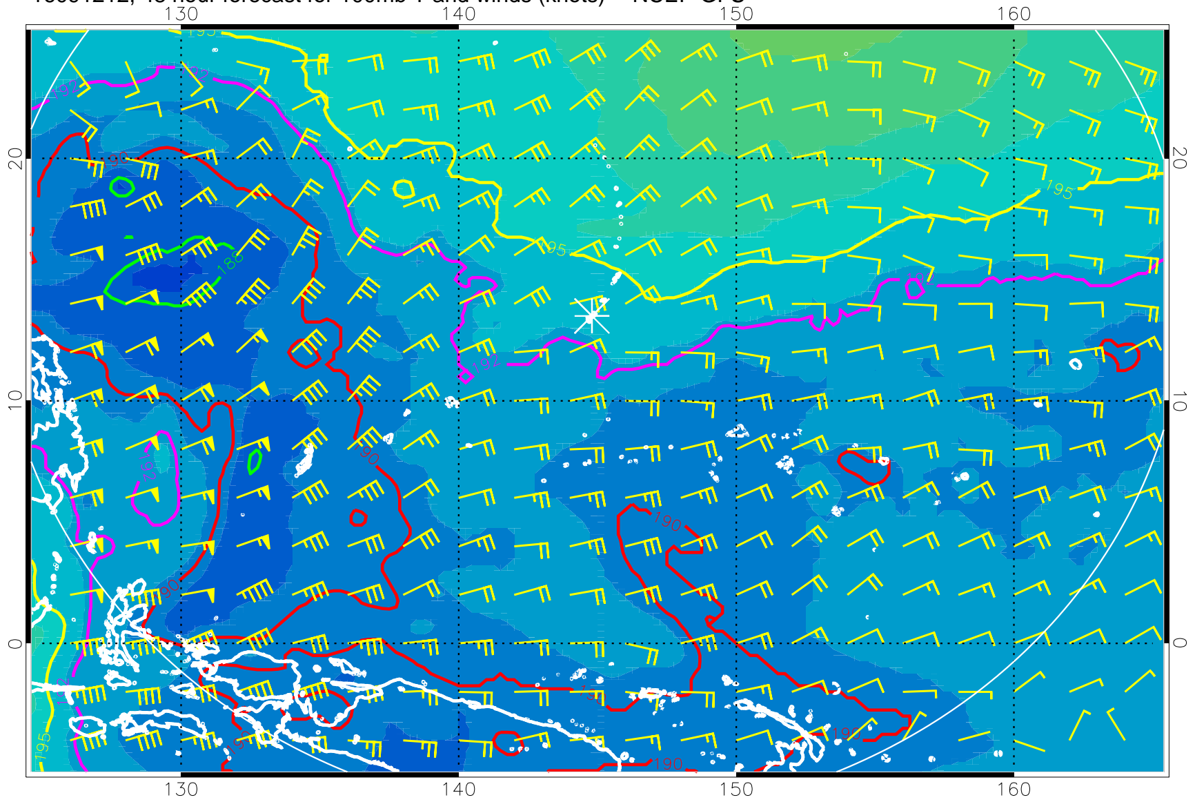
16091212, 48 hour forecast for 100mb T and winds (knots) -- NCEP GFS
