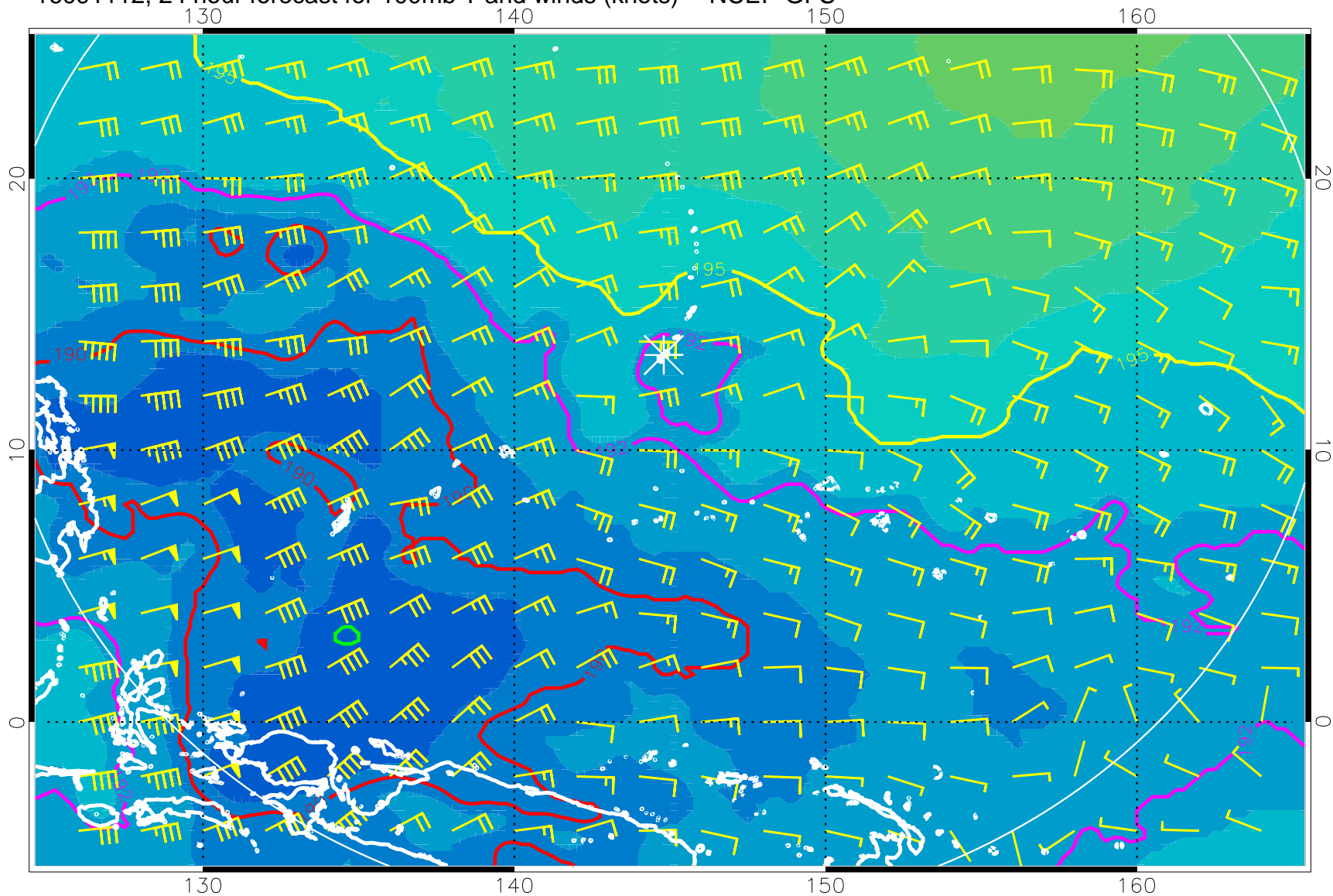
16091112, 24 hour forecast for 100mb T and winds (knots) -- NCEP GFS
