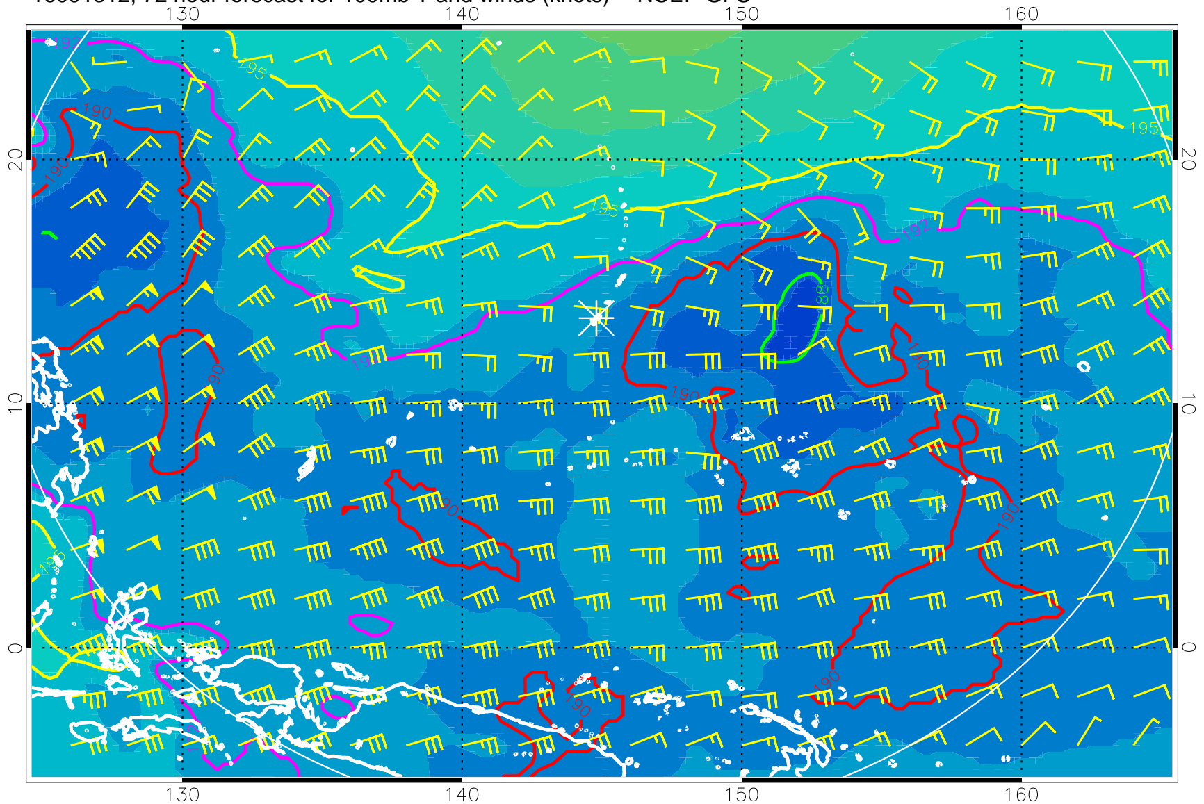
16091312, 72 hour forecast for 100mb T and winds (knots) -- NCEP GFS
