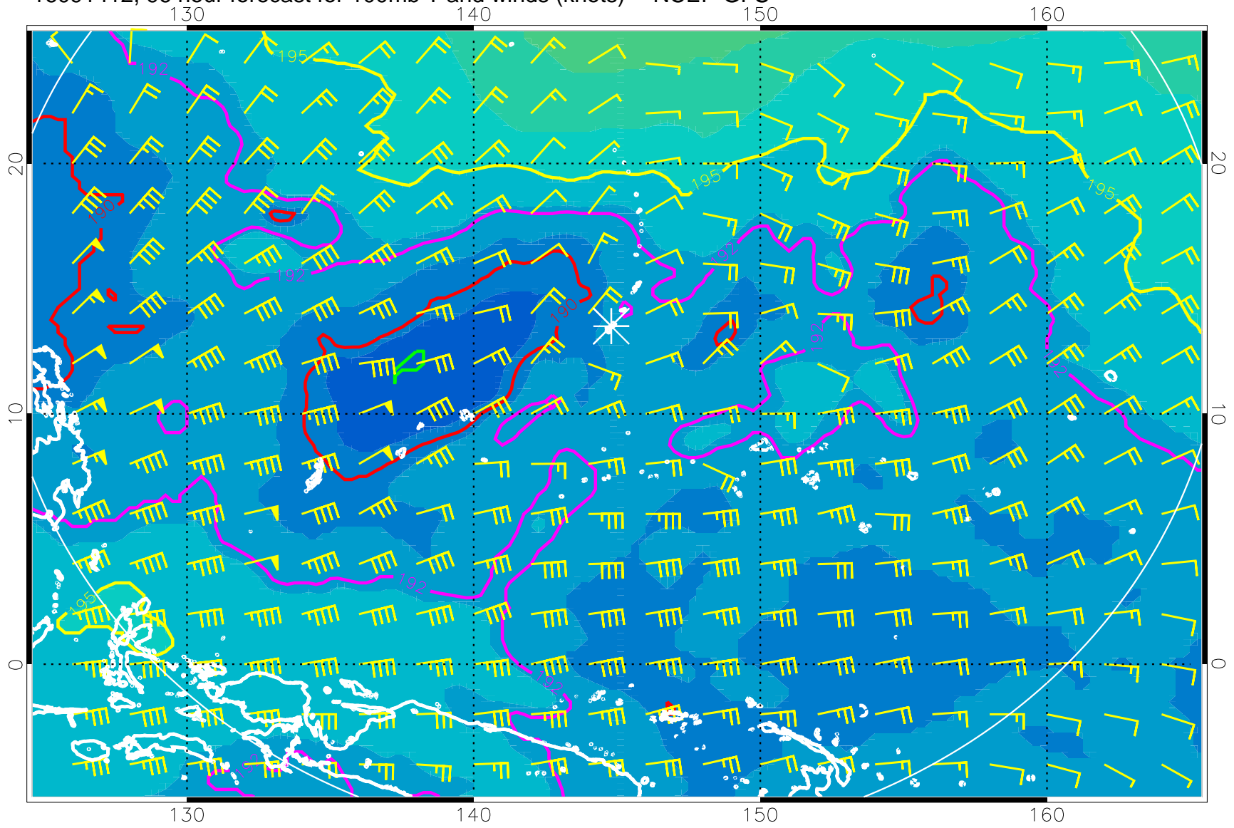
16091412, 96 hour forecast for 100mb T and winds (knots) -- NCEP GFS
