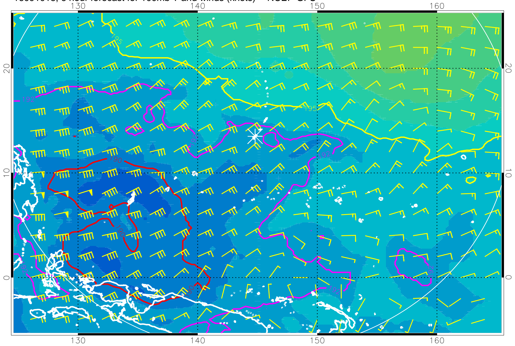
16091018, 6 hour forecast for 100mb T and winds (knots) -- NCEP GFS
