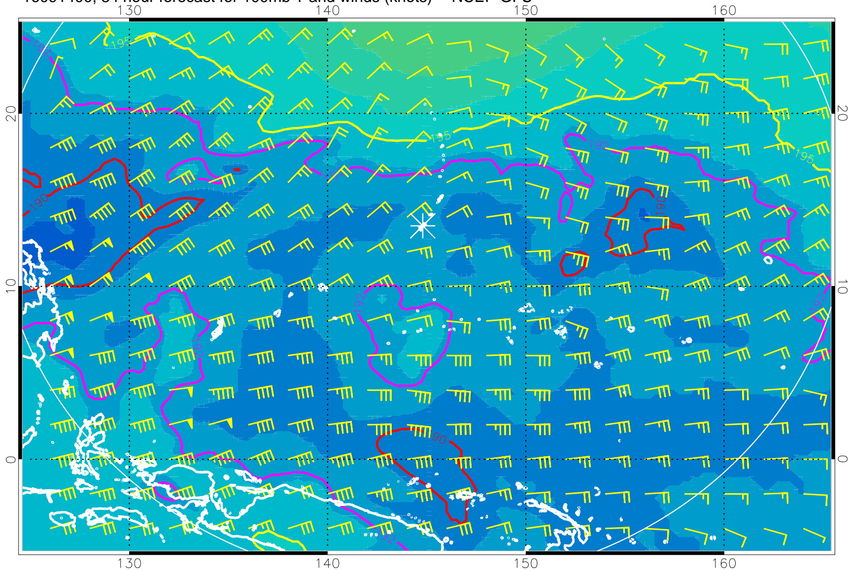
16091400, 84 hour forecast for 100mb T and winds (knots) -- NCEP GFS
