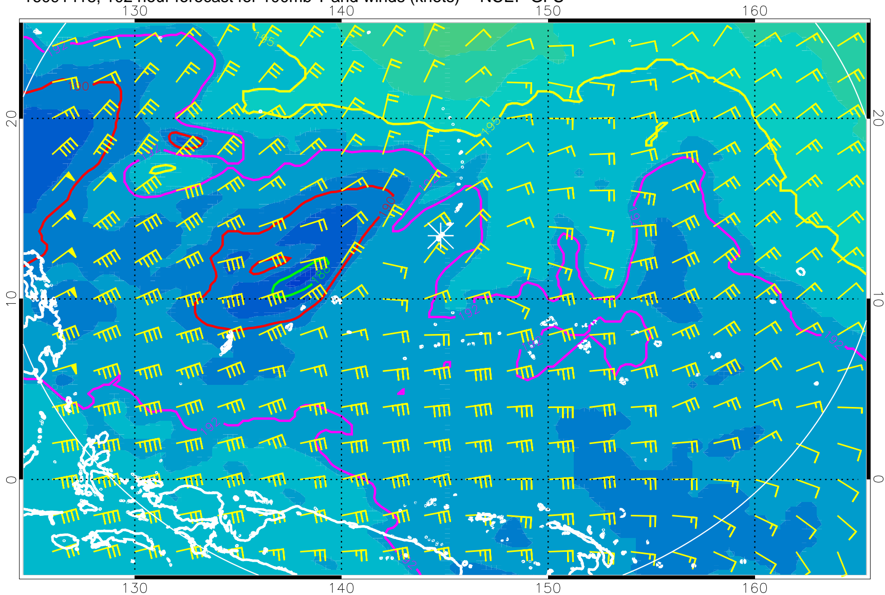
16091418, 102 hour forecast for 100mb T and winds (knots) -- NCEP GFS
