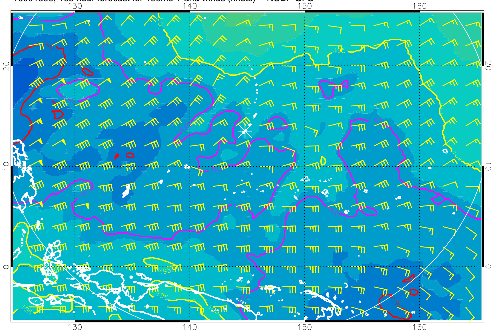
16091500, 108 hour forecast for 100mb T and winds (knots) -- NCEP GFS
