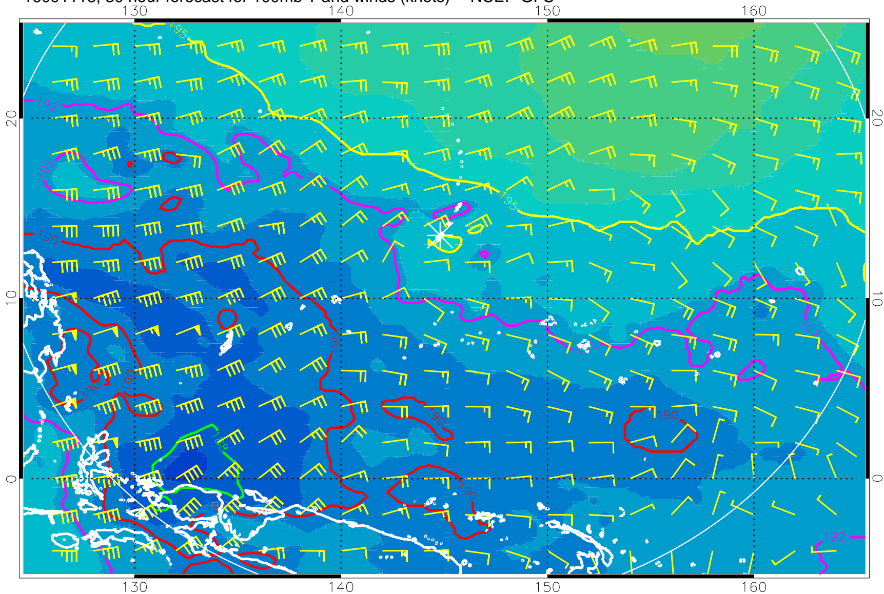
16091118, 30 hour forecast for 100mb T and winds (knots) -- NCEP GFS
