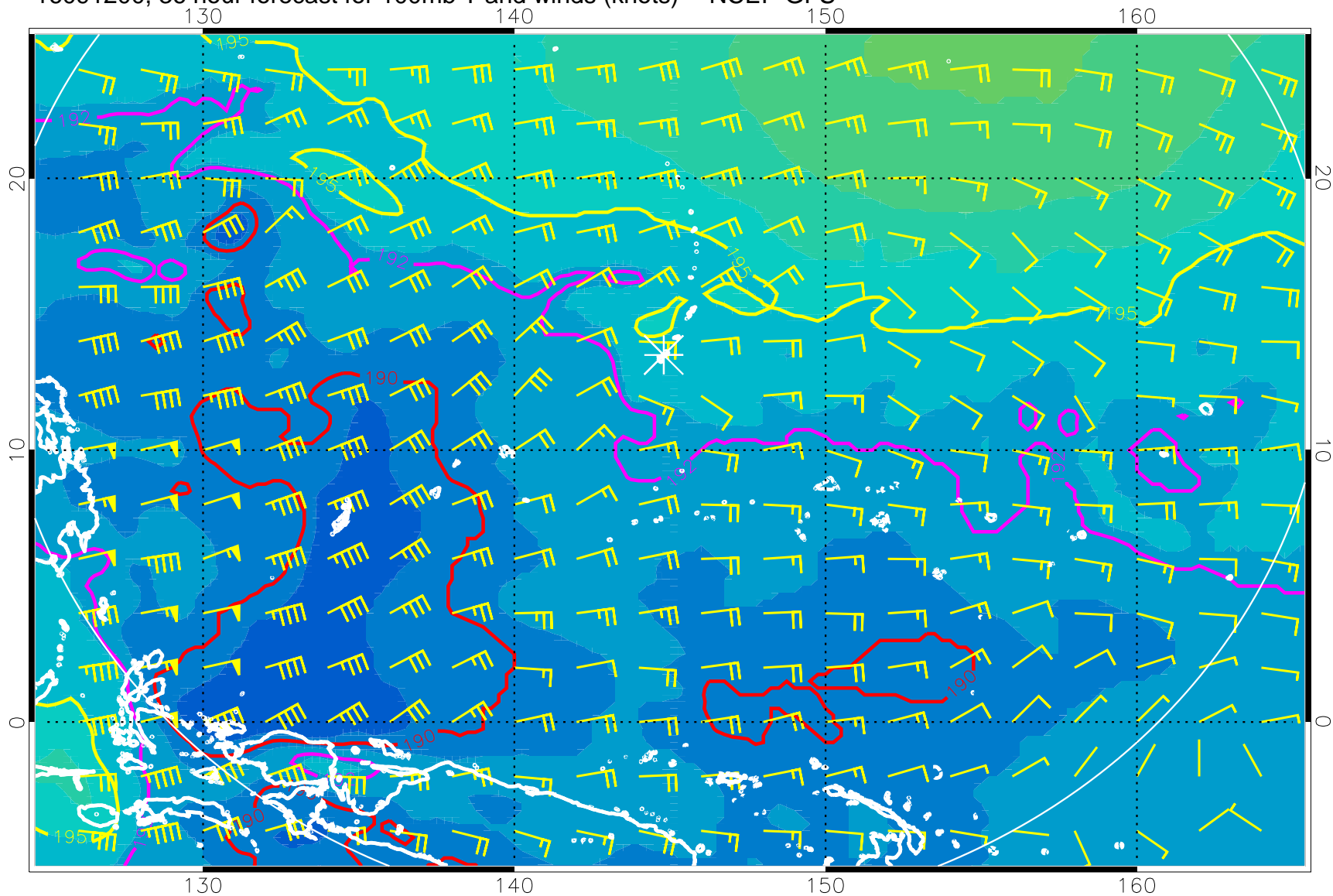
16091200, 36 hour forecast for 100mb T and winds (knots) -- NCEP GFS
