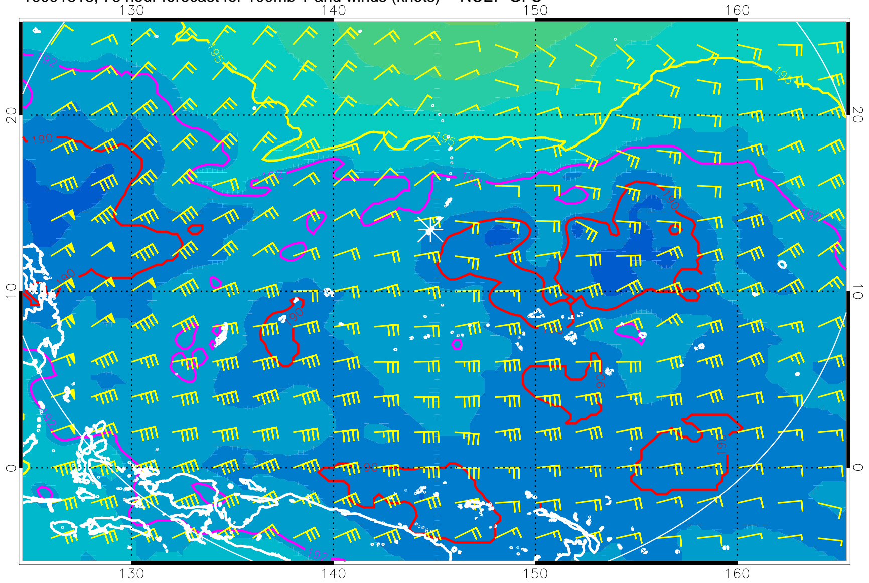
16091318, 78 hour forecast for 100mb T and winds (knots) -- NCEP GFS
