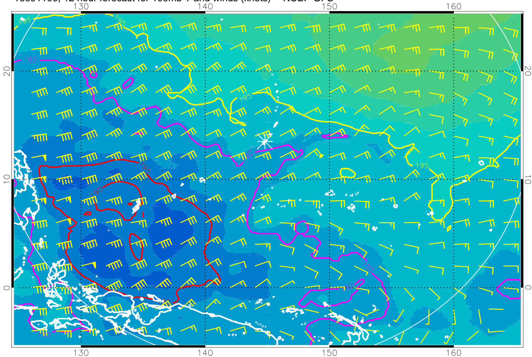
16091100, 12 hour forecast for 100mb T and winds (knots) -- NCEP GFS
