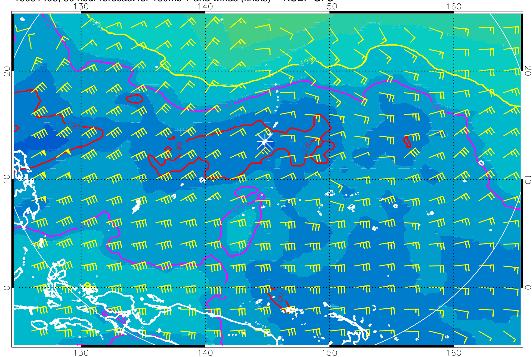
16091406, 90 hour forecast for 100mb T and winds (knots) -- NCEP GFS
