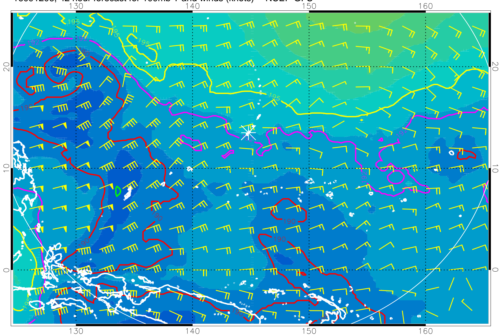
16091206, 42 hour forecast for 100mb T and winds (knots) -- NCEP GFS
