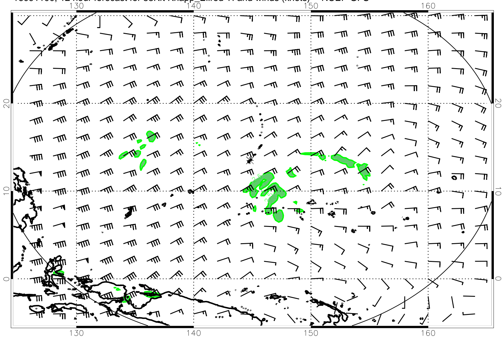
16091100, 12 hour forecast for 53Kft Knapp_Ellrod TI and winds (knots) -- NCEP GFS
