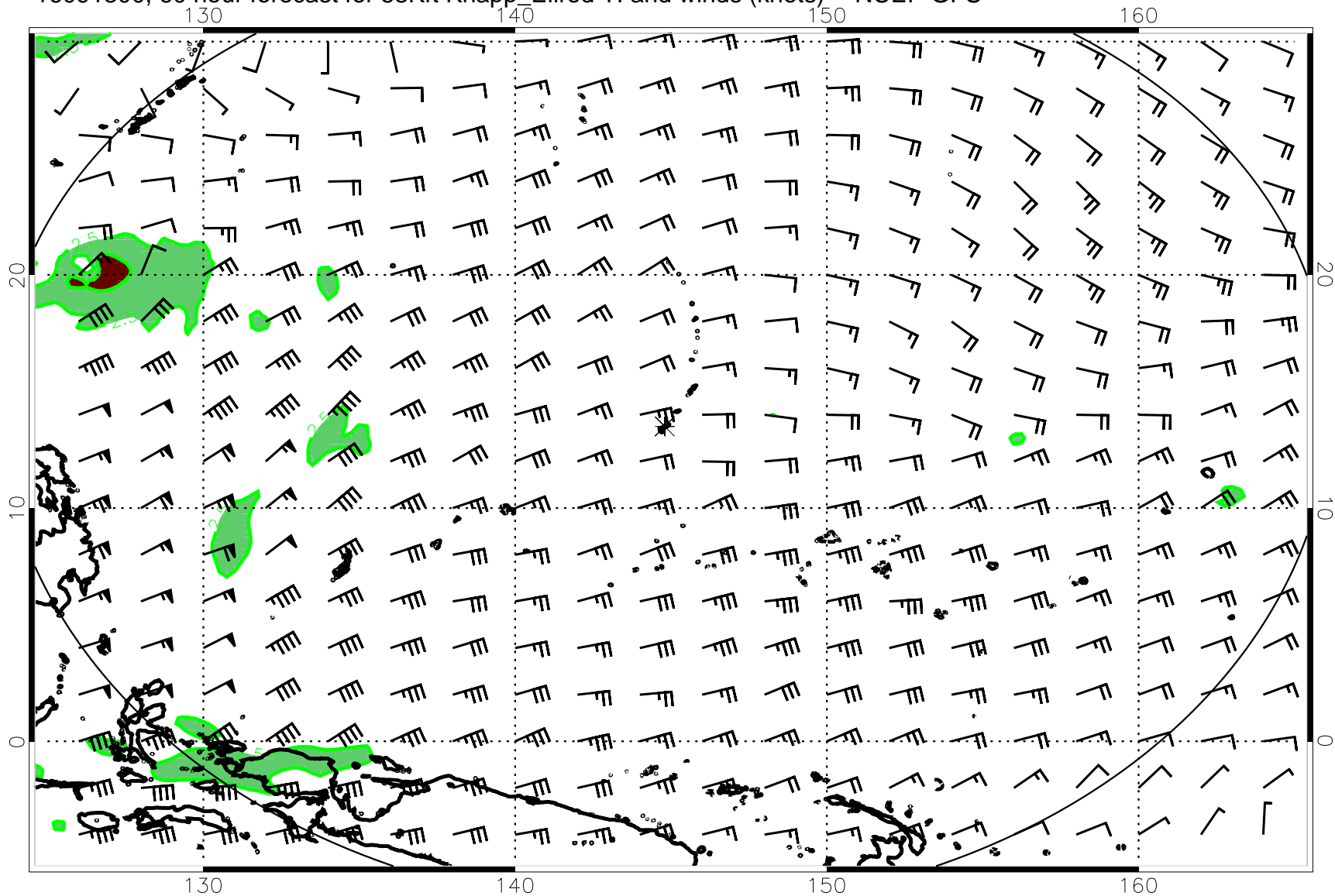
16091300, 60 hour forecast for 53Kft Knapp_Ellrod TI and winds (knots) -- NCEP GFS
