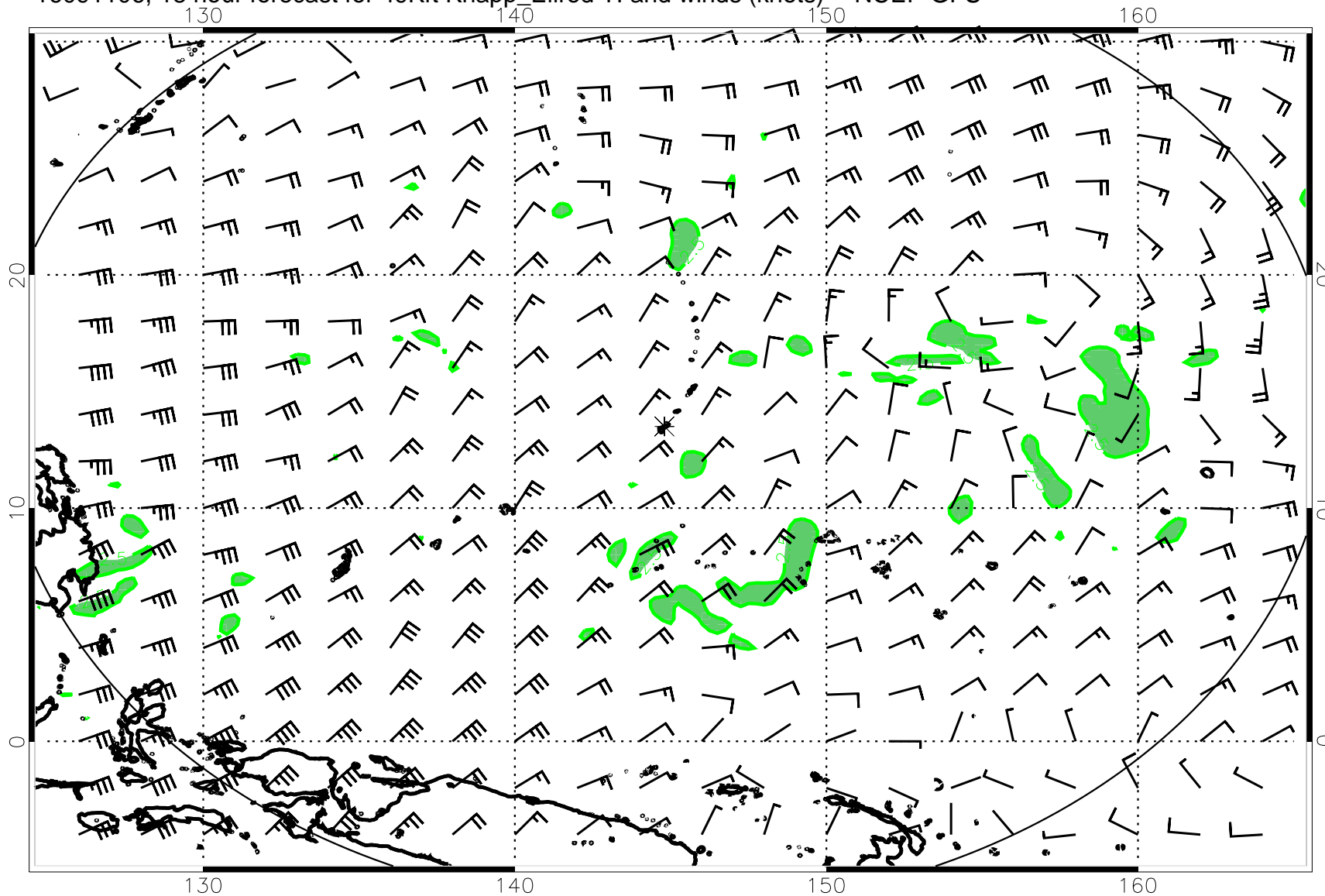
16091106, 18 hour forecast for 49Kft Knapp_Ellrod TI and winds (knots) -- NCEP GFS
