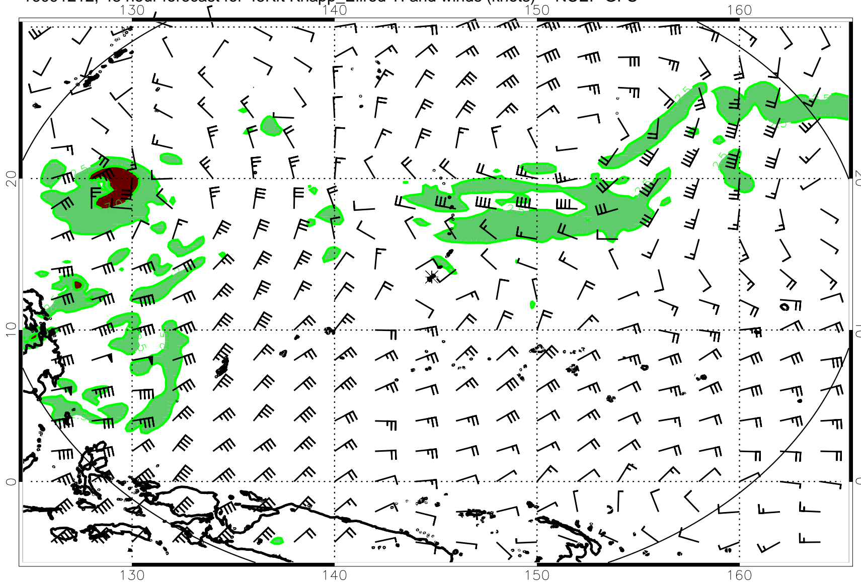
16091212, 48 hour forecast for 45Kft Knapp_Ellrod TI and winds (knots) -- NCEP GFS
