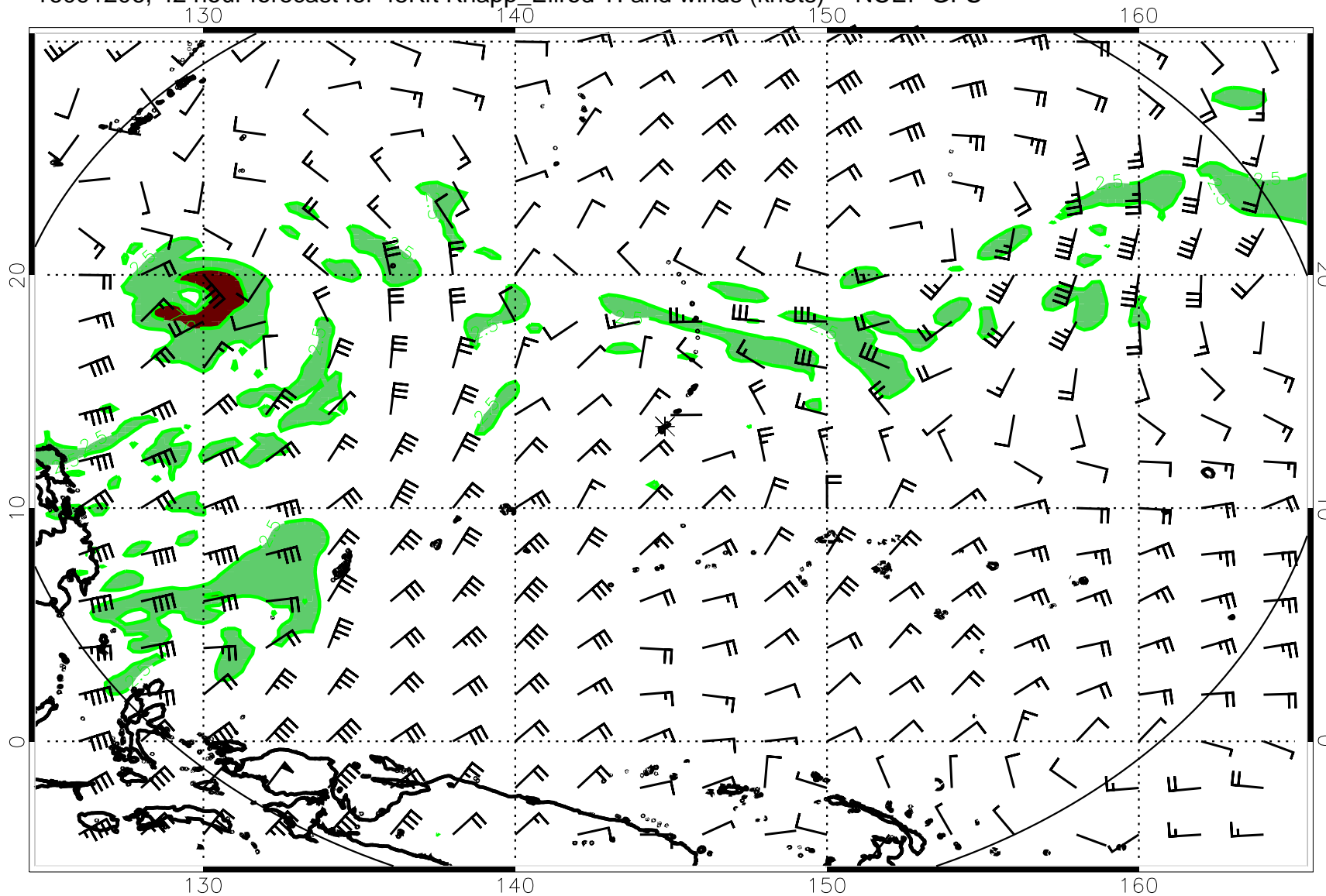
16091206, 42 hour forecast for 45Kft Knapp_Ellrod TI and winds (knots) -- NCEP GFS
