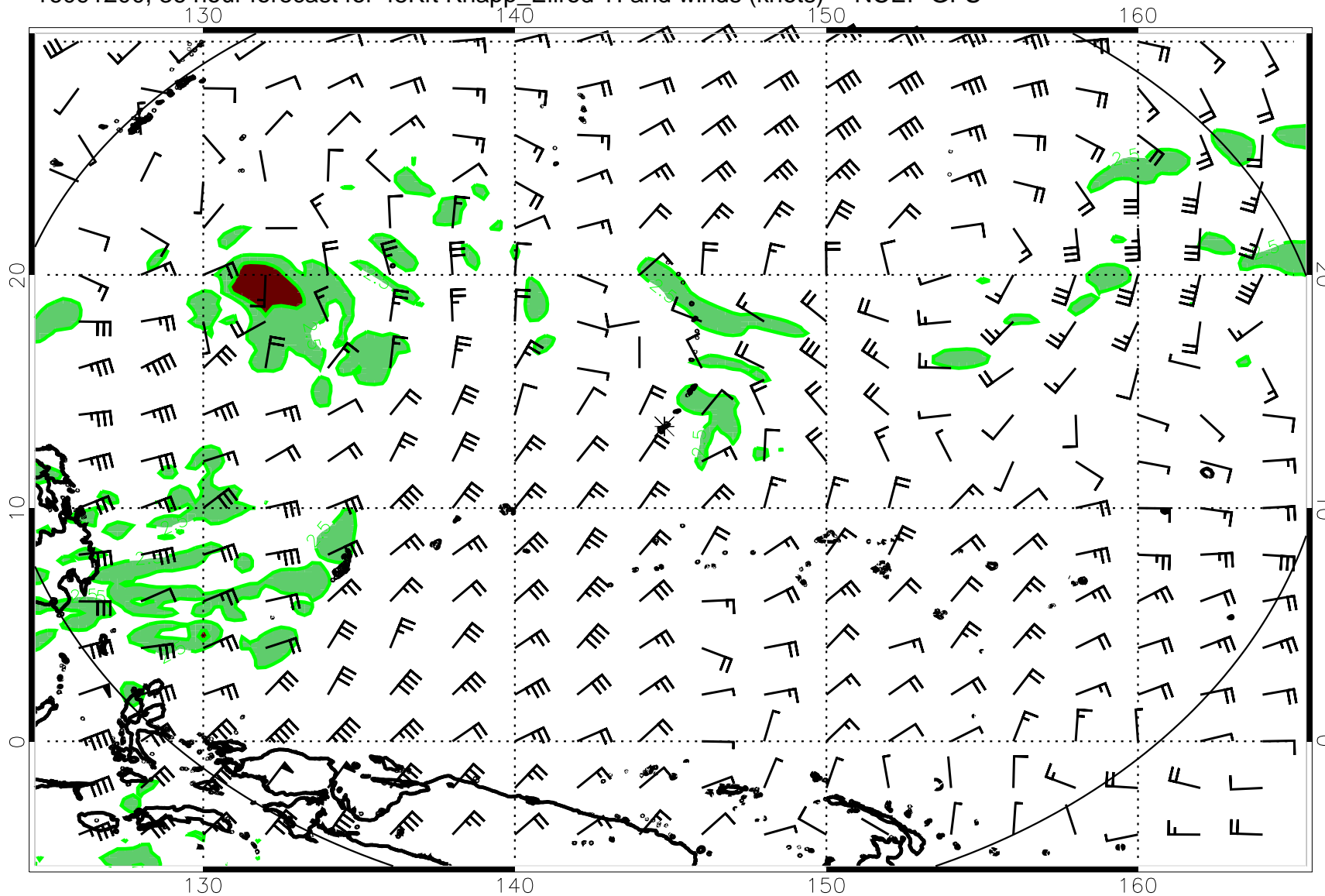
16091200, 36 hour forecast for 45Kft Knapp_Ellrod TI and winds (knots) -- NCEP GFS
