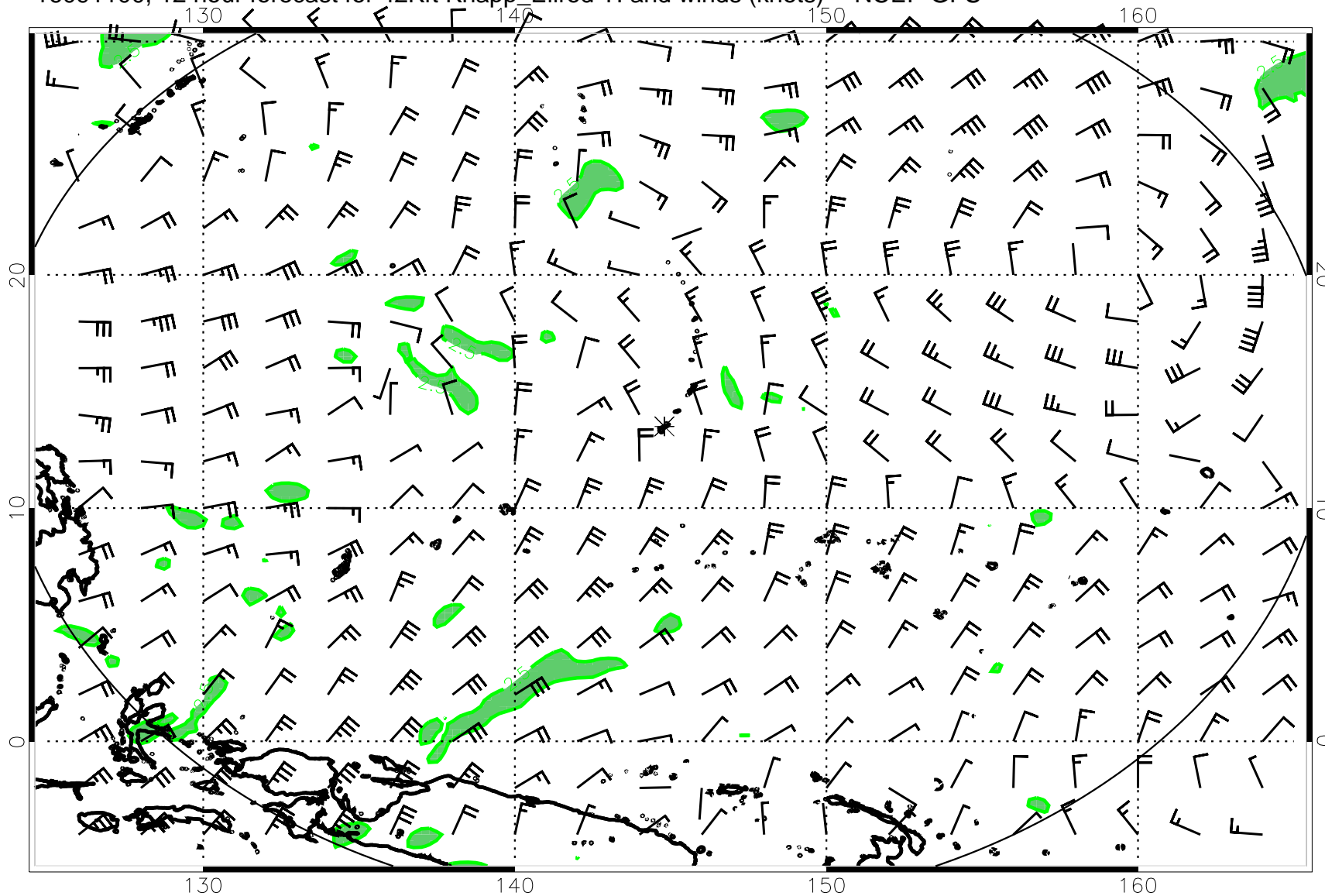
16091100, 12 hour forecast for 42Kft Knapp_Ellrod TI and winds (knots) -- NCEP GFS
