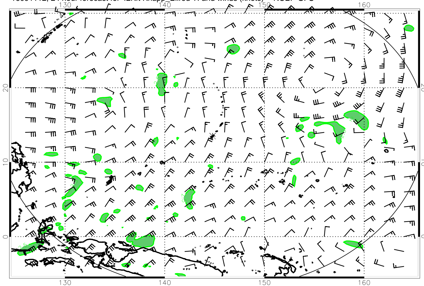
16091112, 24 hour forecast for 42Kft Knapp_Ellrod TI and winds (knots) -- NCEP GFS
