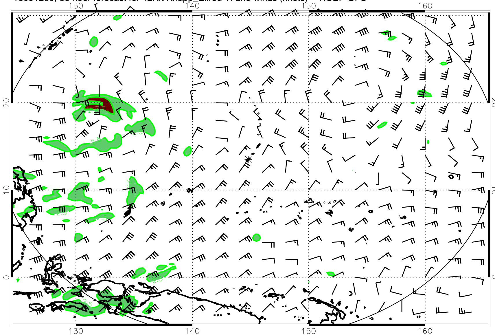
16091200, 36 hour forecast for 42Kft Knapp_Ellrod TI and winds (knots) -- NCEP GFS
