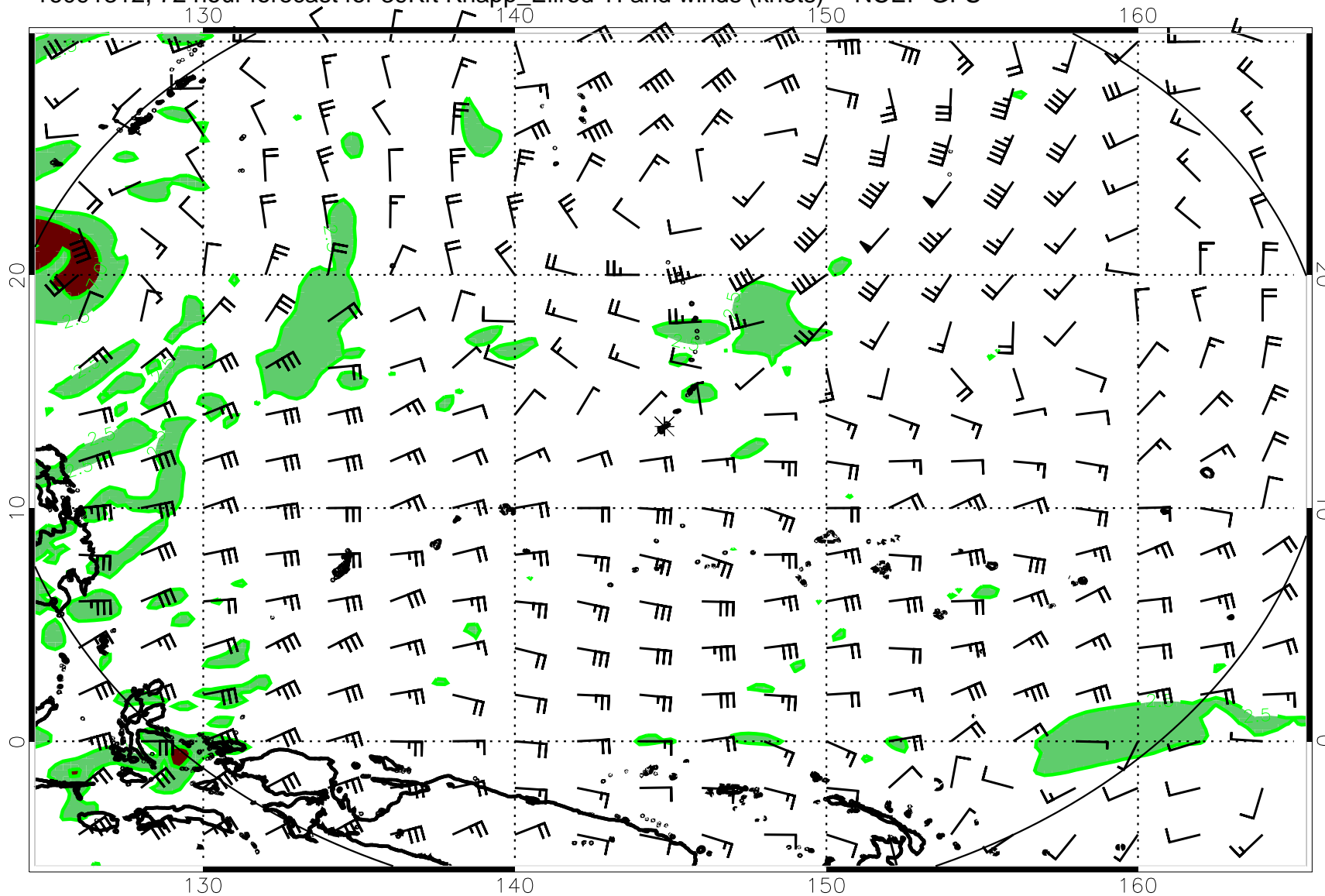
16091312, 72 hour forecast for 39Kft Knapp_Ellrod TI and winds (knots) -- NCEP GFS
