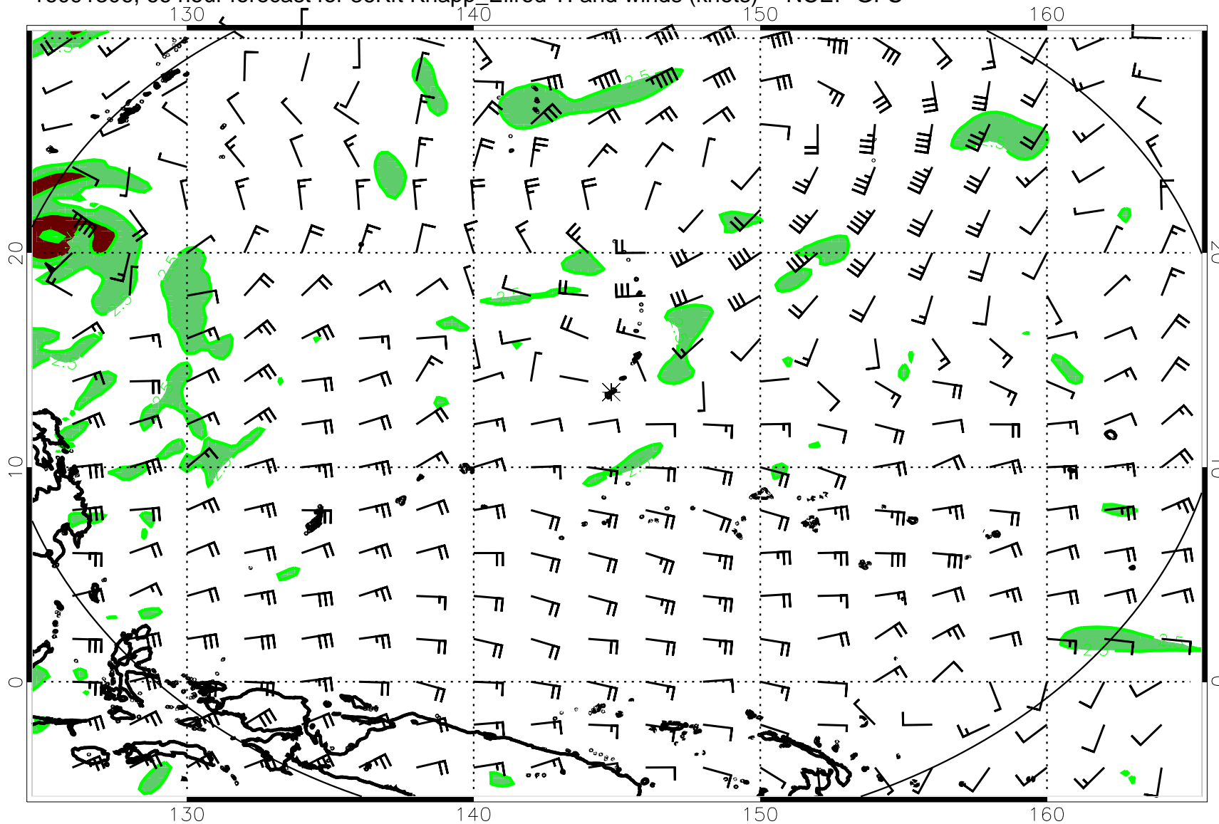
16091306, 66 hour forecast for 36Kft Knapp_Ellrod TI and winds (knots) -- NCEP GFS
