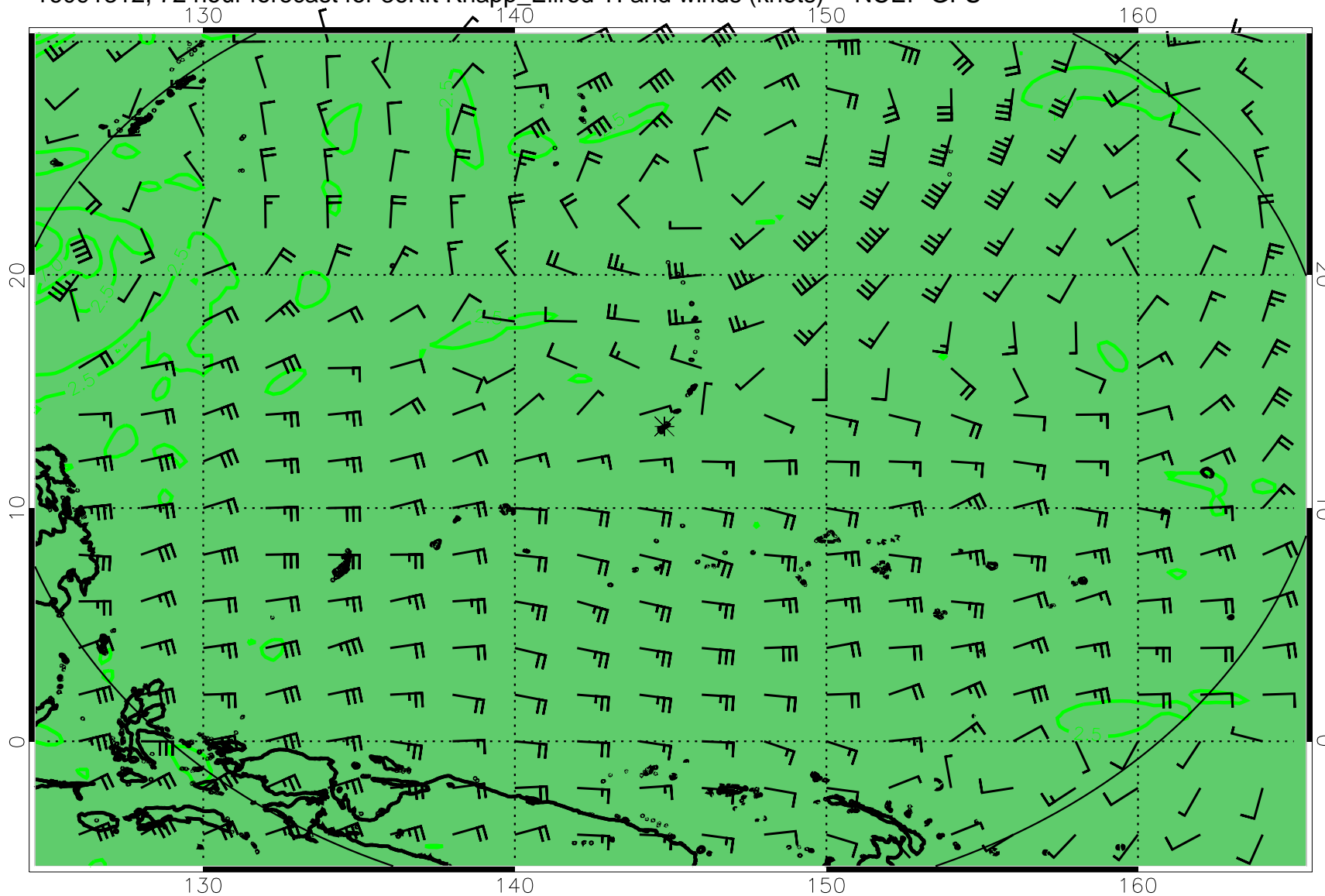
16091312, 72 hour forecast for 36Kft Knapp_Ellrod TI and winds (knots) -- NCEP GFS
