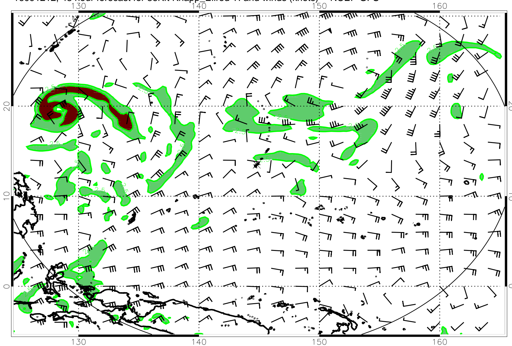
16091212, 48 hour forecast for 36Kft Knapp_Ellrod TI and winds (knots) -- NCEP GFS
