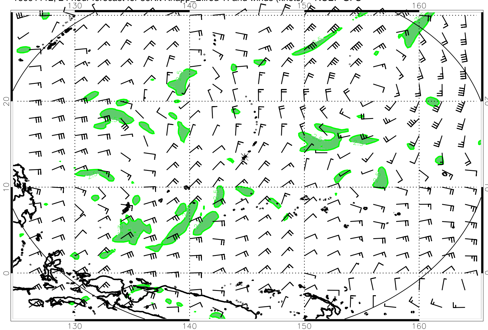
16091112, 24 hour forecast for 36Kft Knapp_Ellrod TI and winds (knots) -- NCEP GFS
