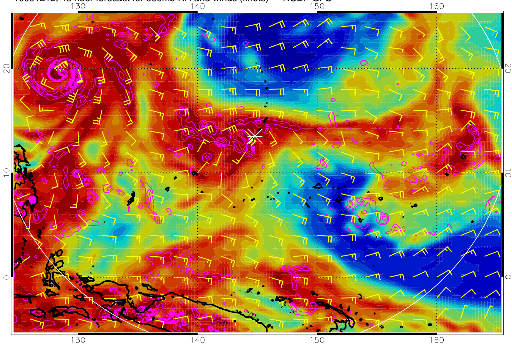
16091212, 48 hour forecast for 500mb RH and winds (knots) -- NCEP GFS
