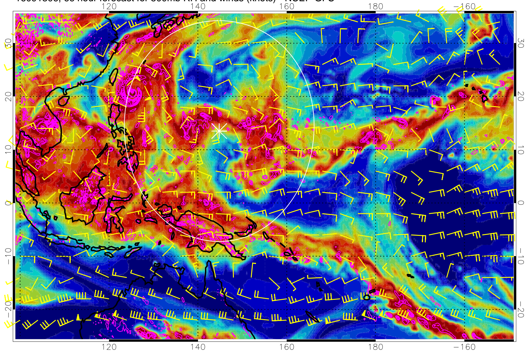
16091306, 66 hour forecast for 500mb RH and winds (knots) - NCEP GFS
