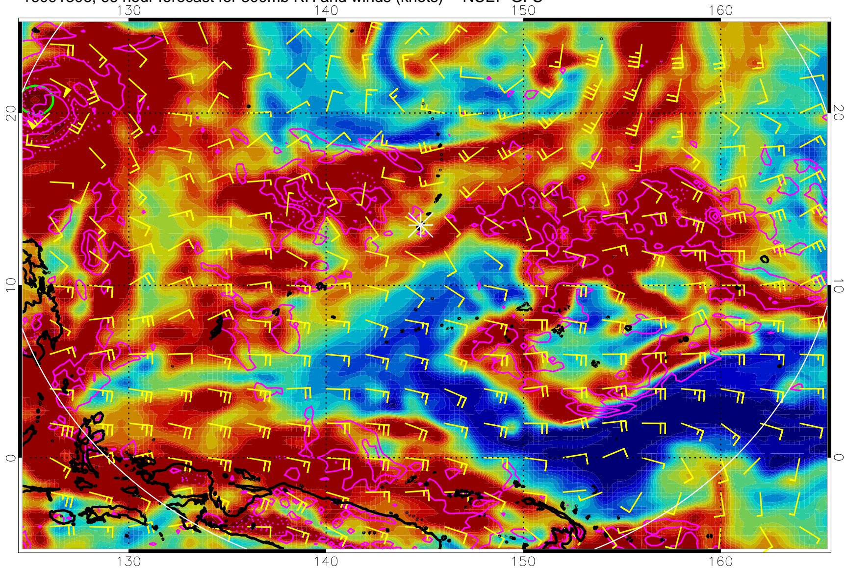
16091306, 66 hour forecast for 300mb RH and winds (knots) -- NCEP GFS
