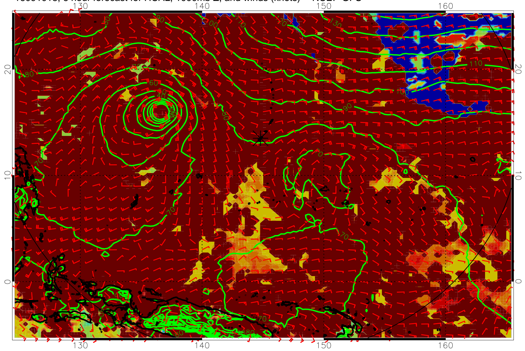
16091018, 6 hour forecast for HCAL, 1000mb Z, and winds (knots) -- NCEP GFS
