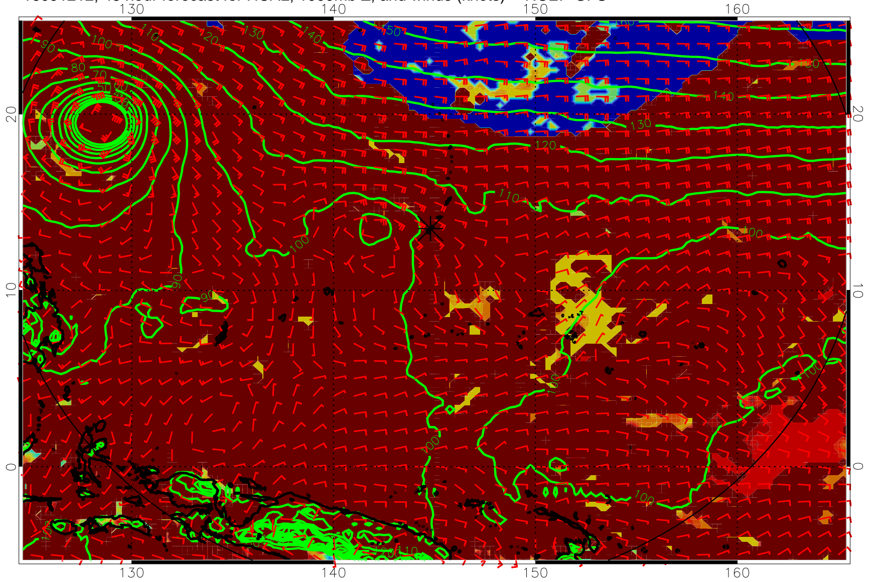
16091212, 48 hour forecast for HCAL, 1000mb Z, and winds (knots) -- NCEP GFS
