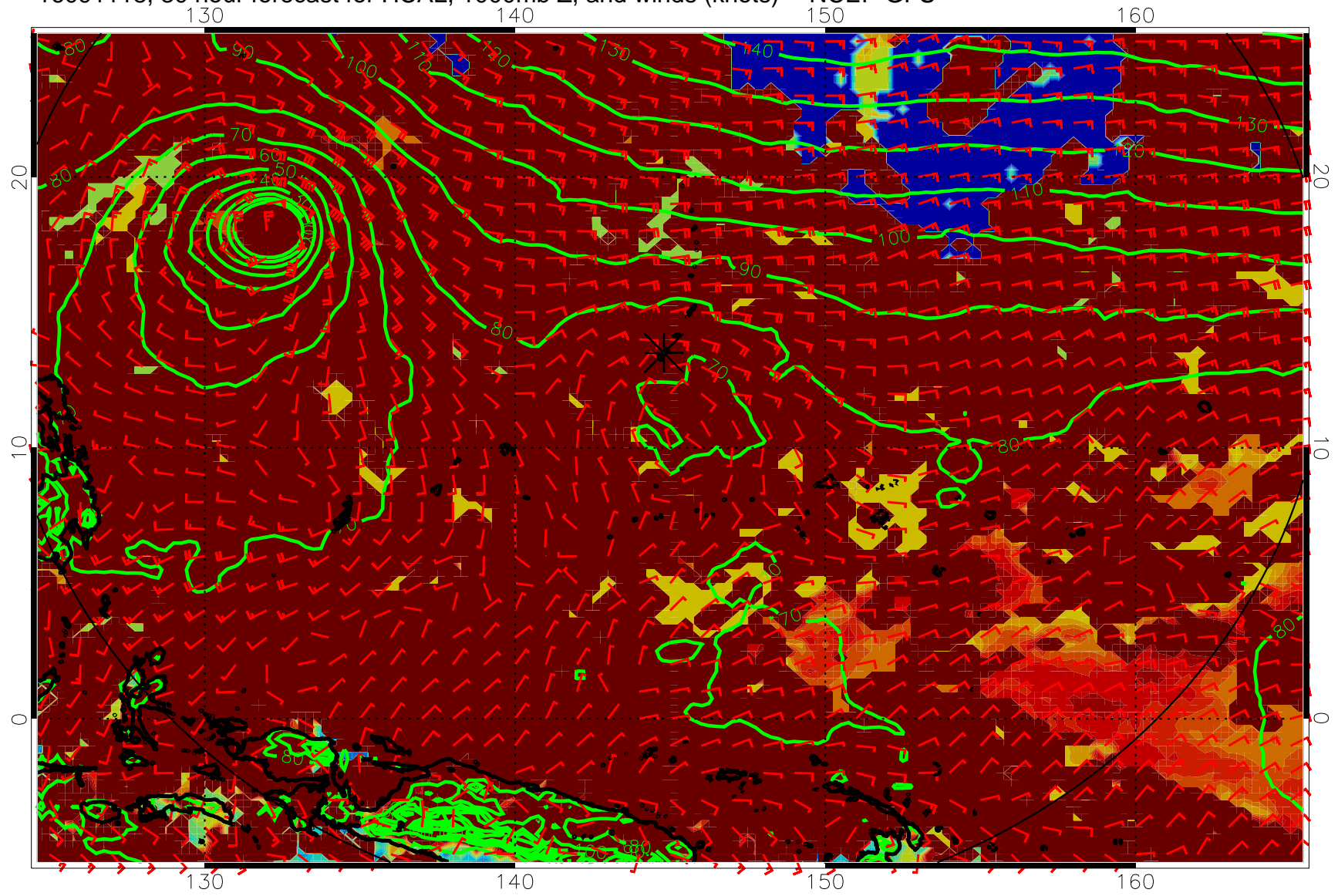
16091118, 30 hour forecast for HCAL, 1000mb Z, and winds (knots) -- NCEP GFS
