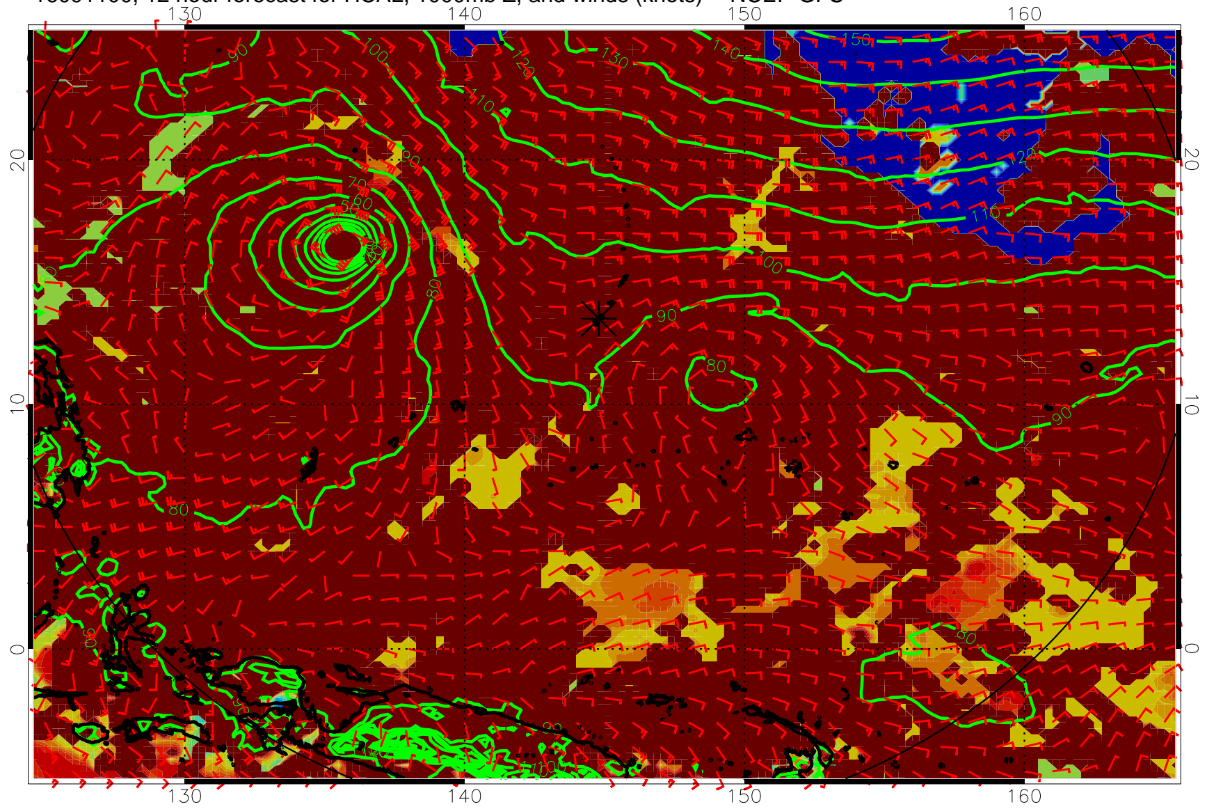
16091100, 12 hour forecast for HCAL, 1000mb Z, and winds (knots) -- NCEP GFS
