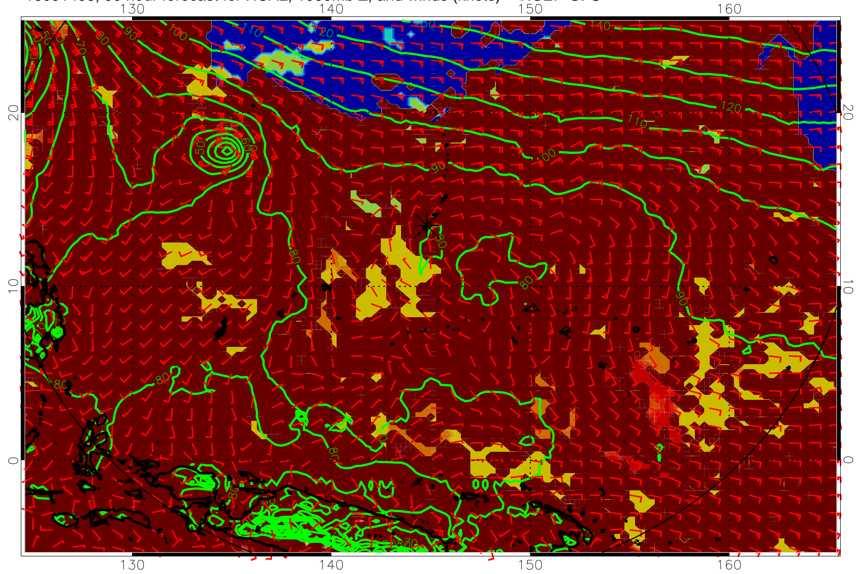
16091406, 90 hour forecast for HCAL, 1000mb Z, and winds (knots) -- NCEP GFS
