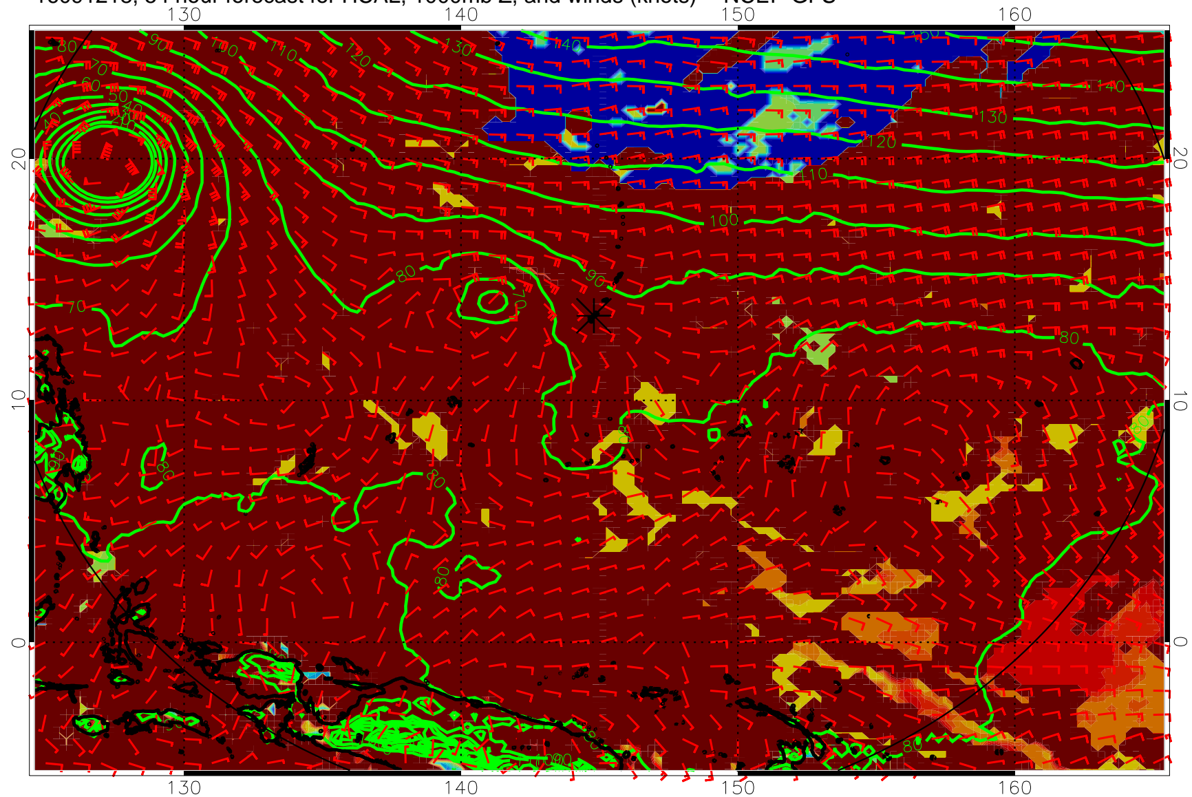
16091218, 54 hour forecast for HCAL, 1000mb Z, and winds (knots) -- NCEP GFS
