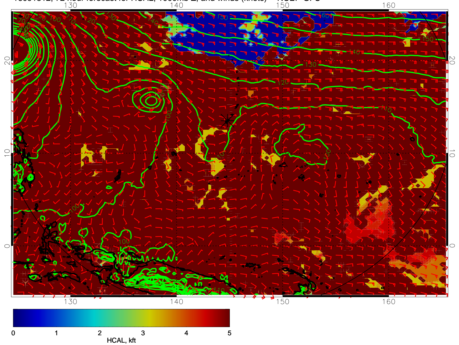
16091312, 72 hour forecast for HCAL, 1000mb Z, and winds (knots) -- NCEP GFS
