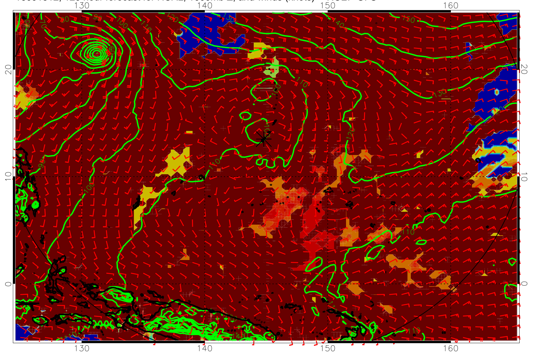
16091512, 120 hour forecast for HCAL, 1000mb Z, and winds (knots) -- NCEP GFS
