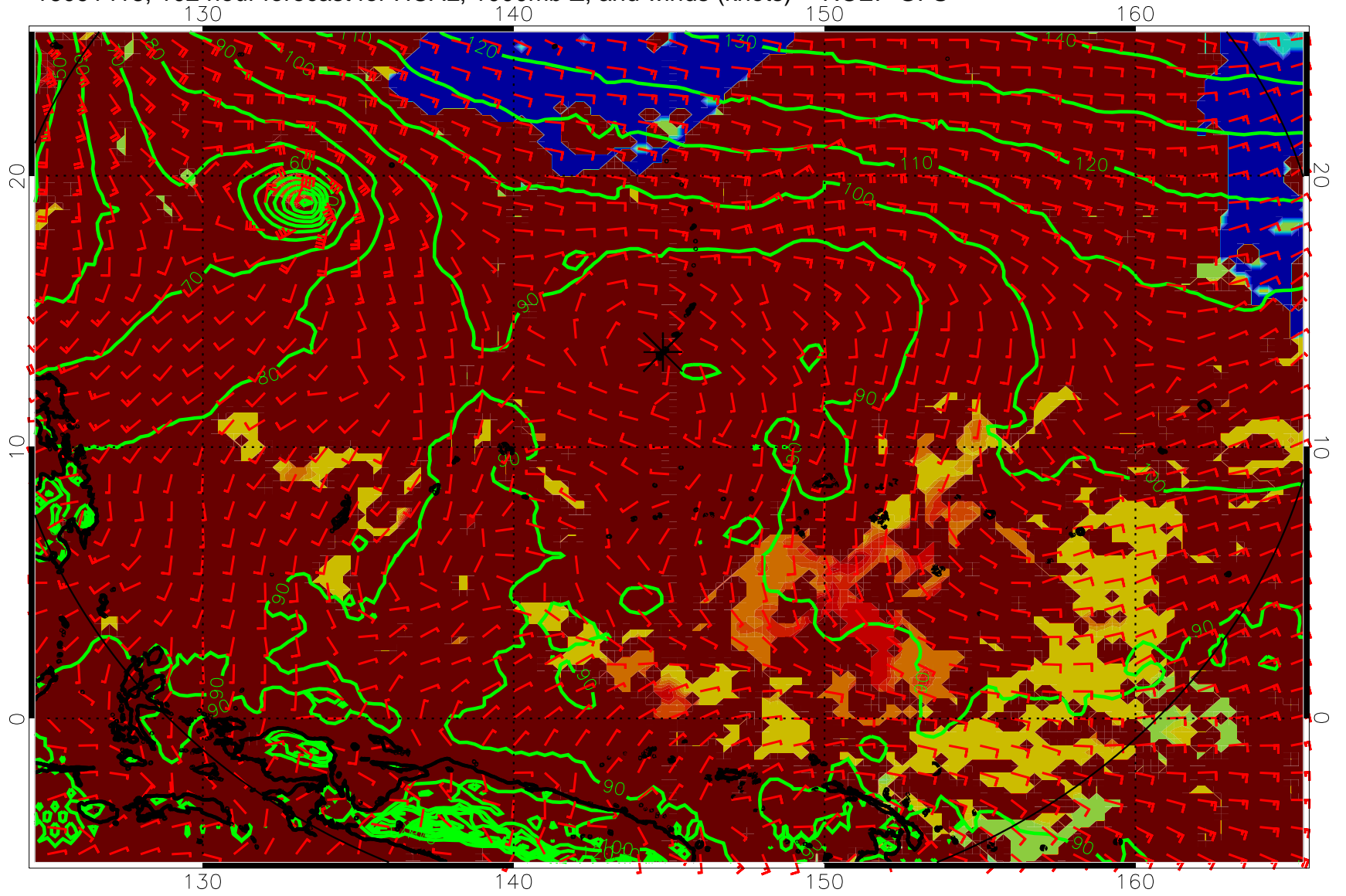
16091418, 102 hour forecast for HCAL, 1000mb Z, and winds (knots) -- NCEP GFS
