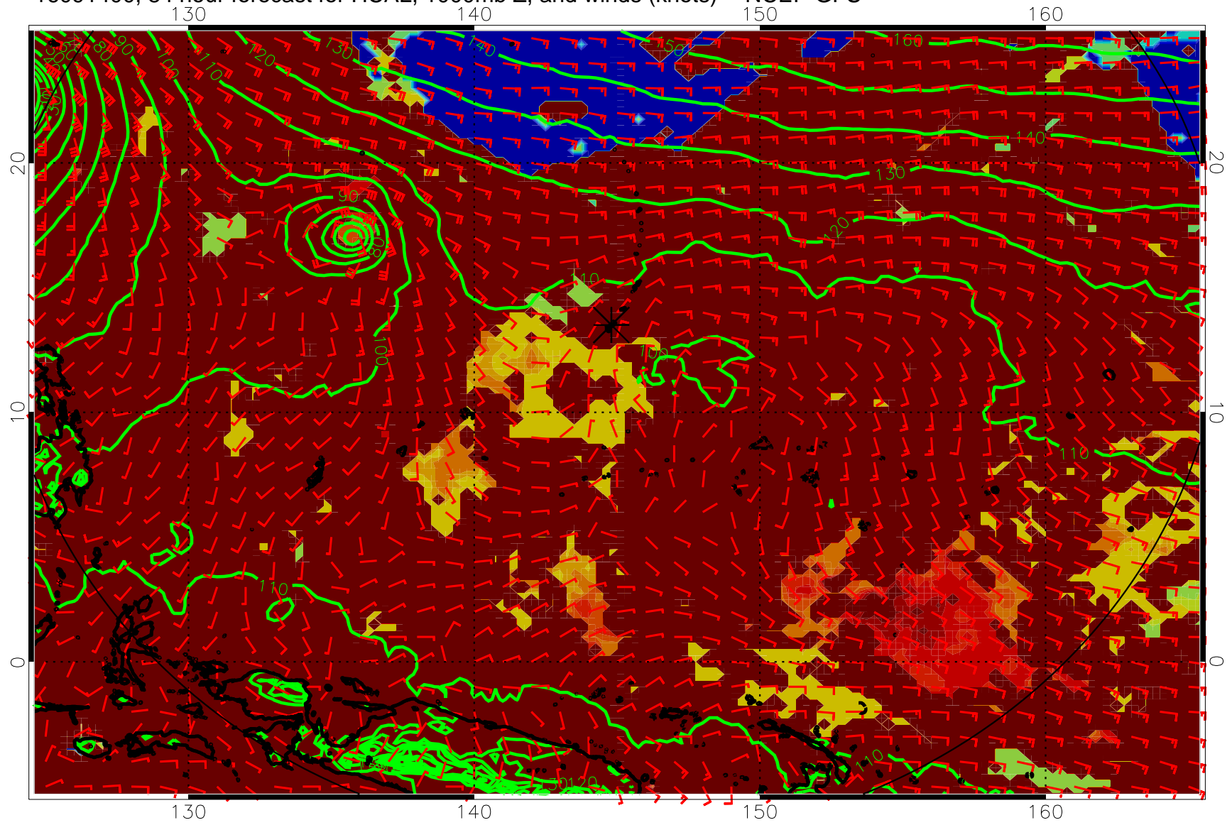
16091400, 84 hour forecast for HCAL, 1000mb Z, and winds (knots) -- NCEP GFS
