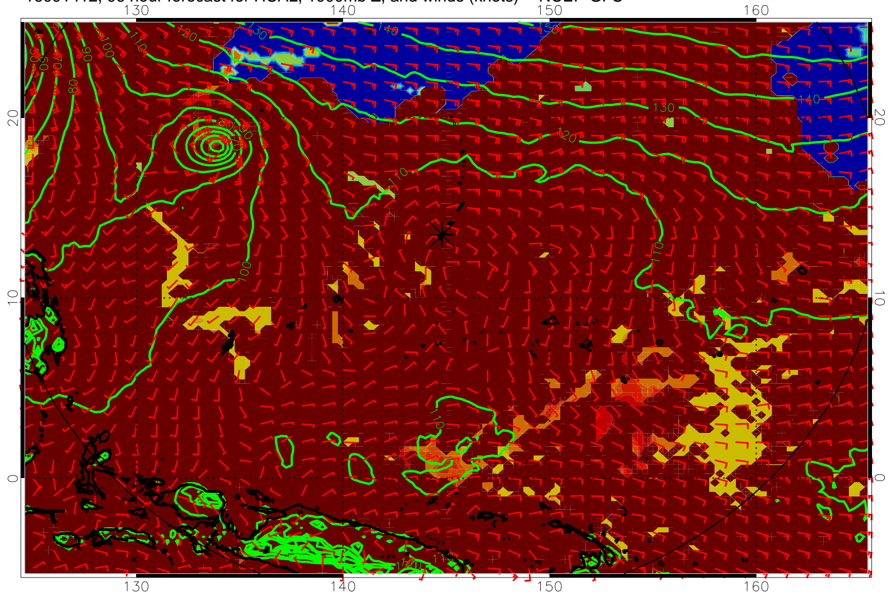
16091412, 96 hour forecast for HCAL, 1000mb Z, and winds (knots) -- NCEP GFS
