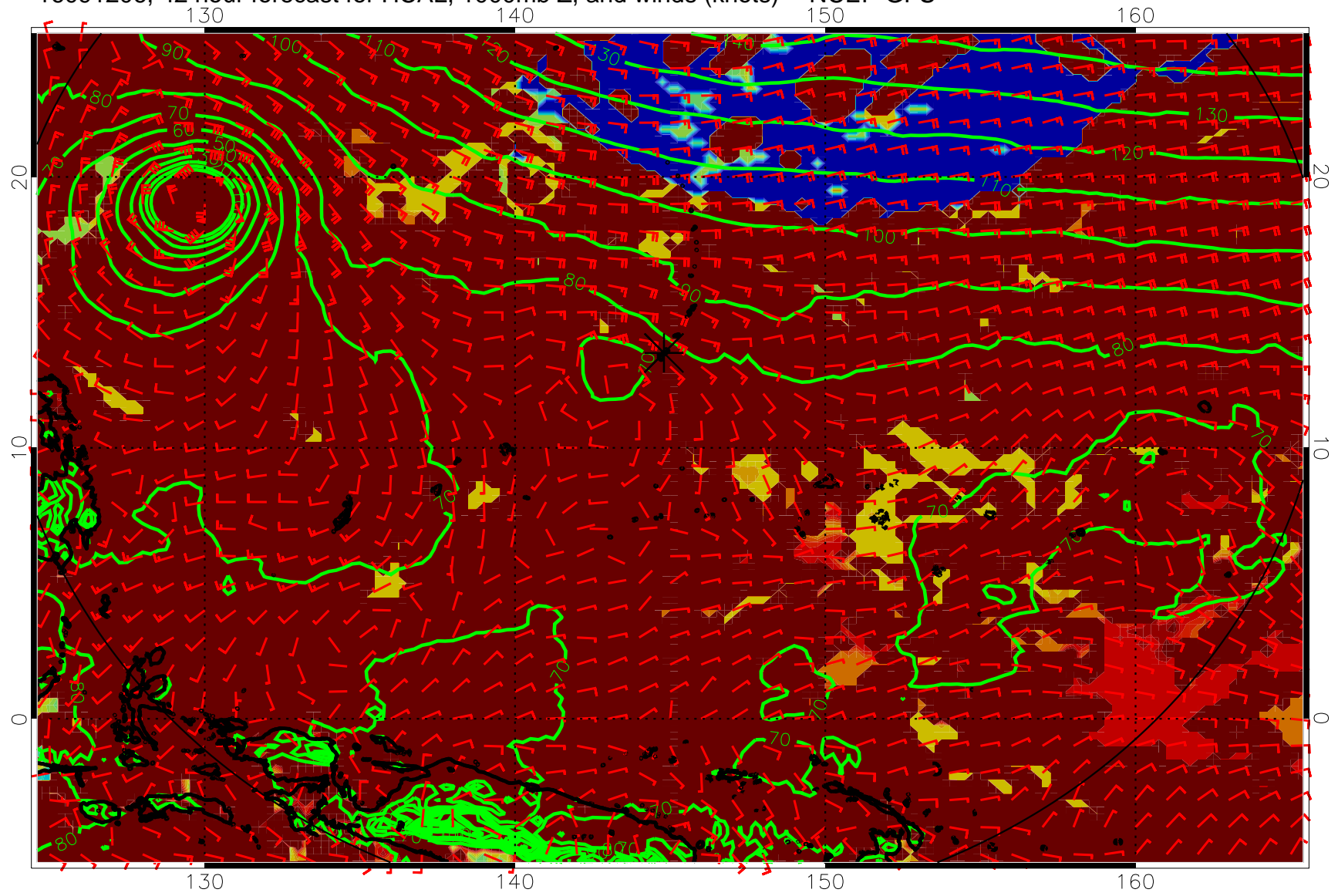
16091206, 42 hour forecast for HCAL, 1000mb Z, and winds (knots) -- NCEP GFS
