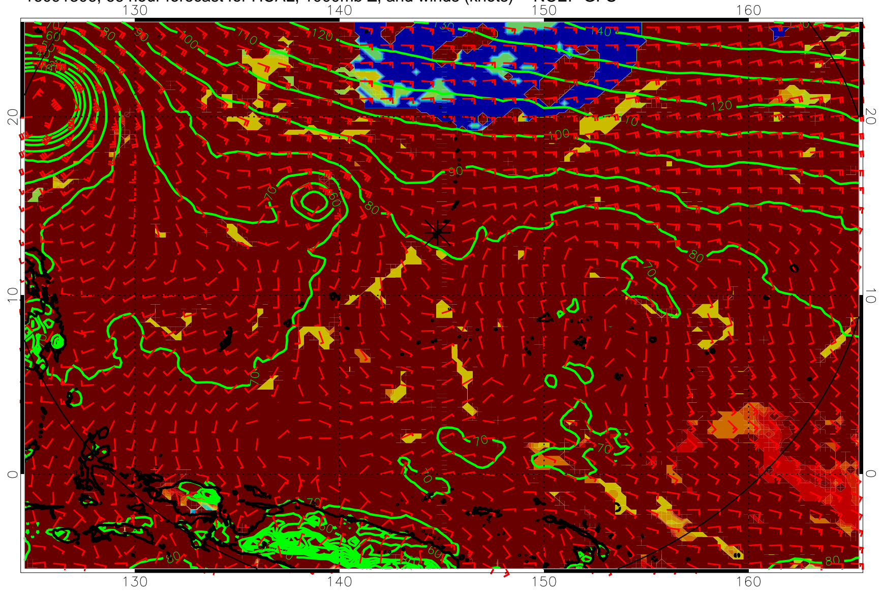
16091306, 66 hour forecast for HCAL, 1000mb Z, and winds (knots) -- NCEP GFS
