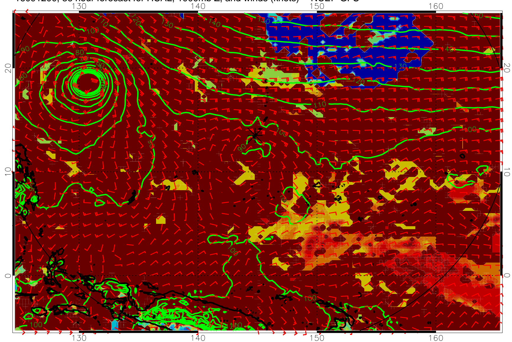
16091200, 36 hour forecast for HCAL, 1000mb Z, and winds (knots) -- NCEP GFS
