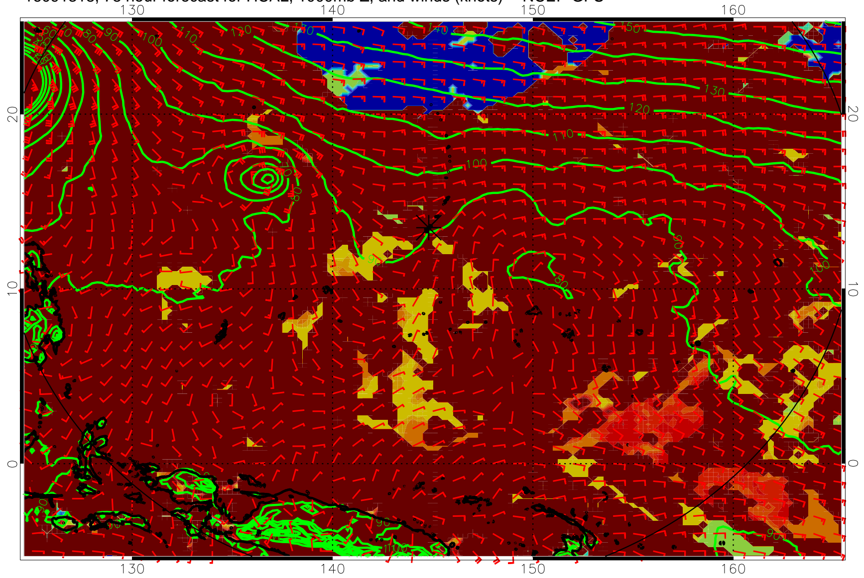
16091318, 78 hour forecast for HCAL, 1000mb Z, and winds (knots) -- NCEP GFS
