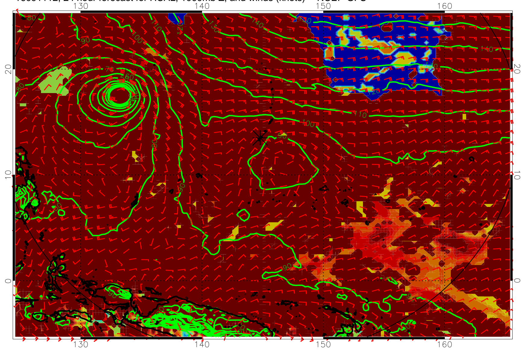
16091112, 24 hour forecast for HCAL, 1000mb Z, and winds (knots) -- NCEP GFS
