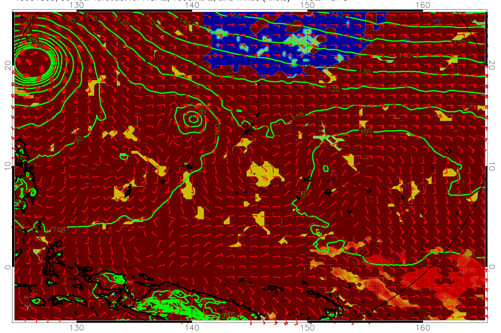
16091300, 60 hour forecast for HCAL, 1000mb Z, and winds (knots) -- NCEP GFS
