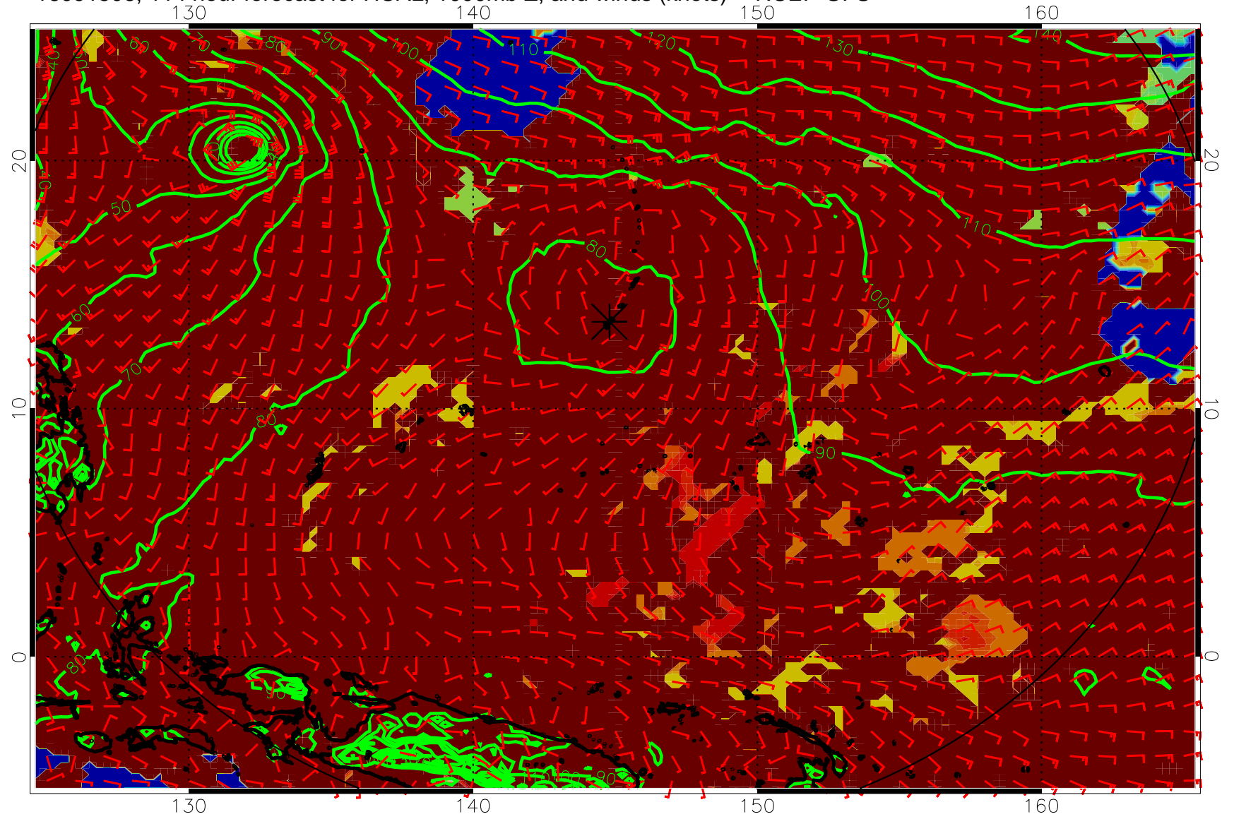
16091506, 114 hour forecast for HCAL, 1000mb Z, and winds (knots) -- NCEP GFS
