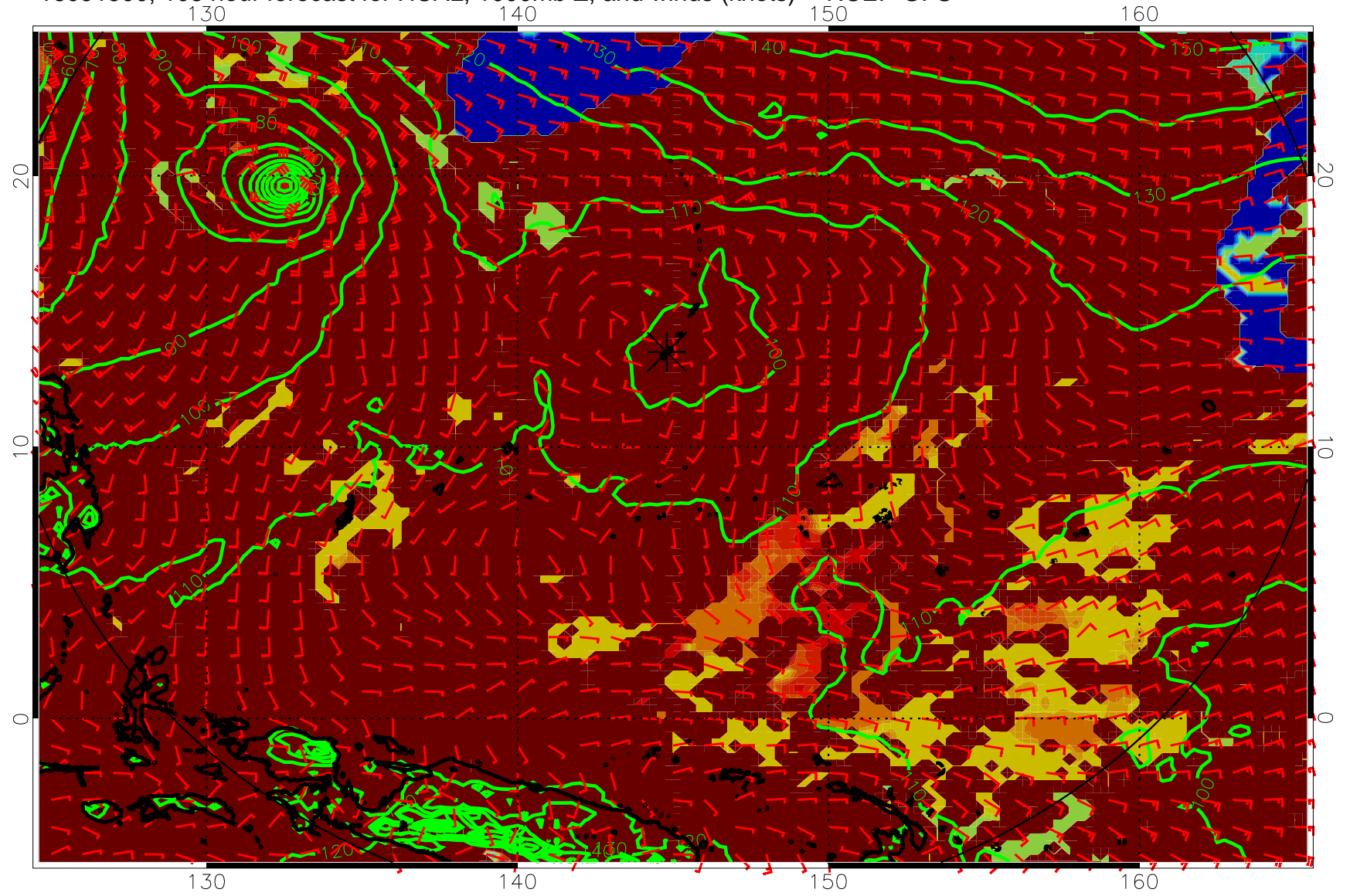
16091500, 108 hour forecast for HCAL, 1000mb Z, and winds (knots) -- NCEP GFS
