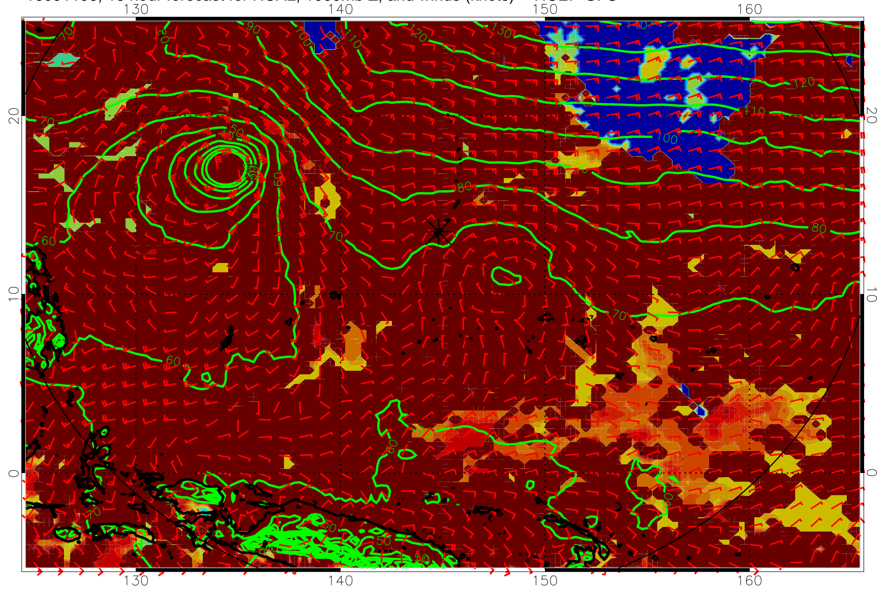
16091106, 18 hour forecast for HCAL, 1000mb Z, and winds (knots) -- NCEP GFS
