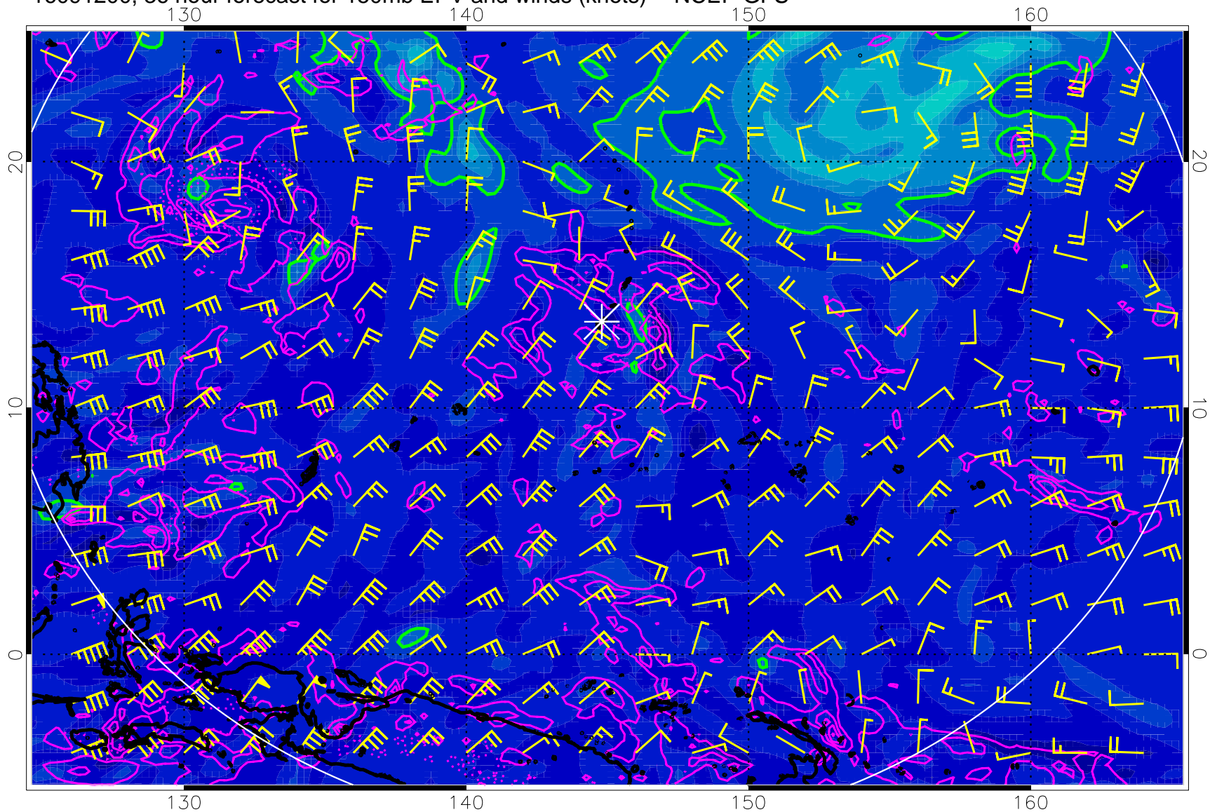
16091200, 36 hour forecast for 150mb EPV and winds (knots) -- NCEP GFS
