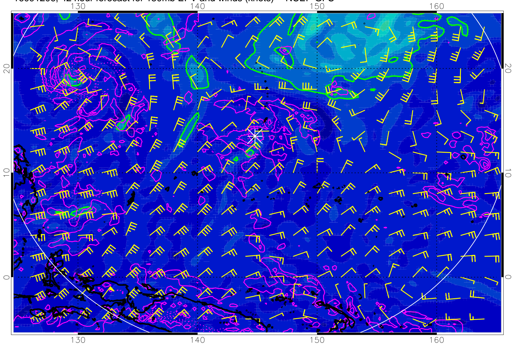
16091206, 42 hour forecast for 150mb EPV and winds (knots) -- NCEP GFS
