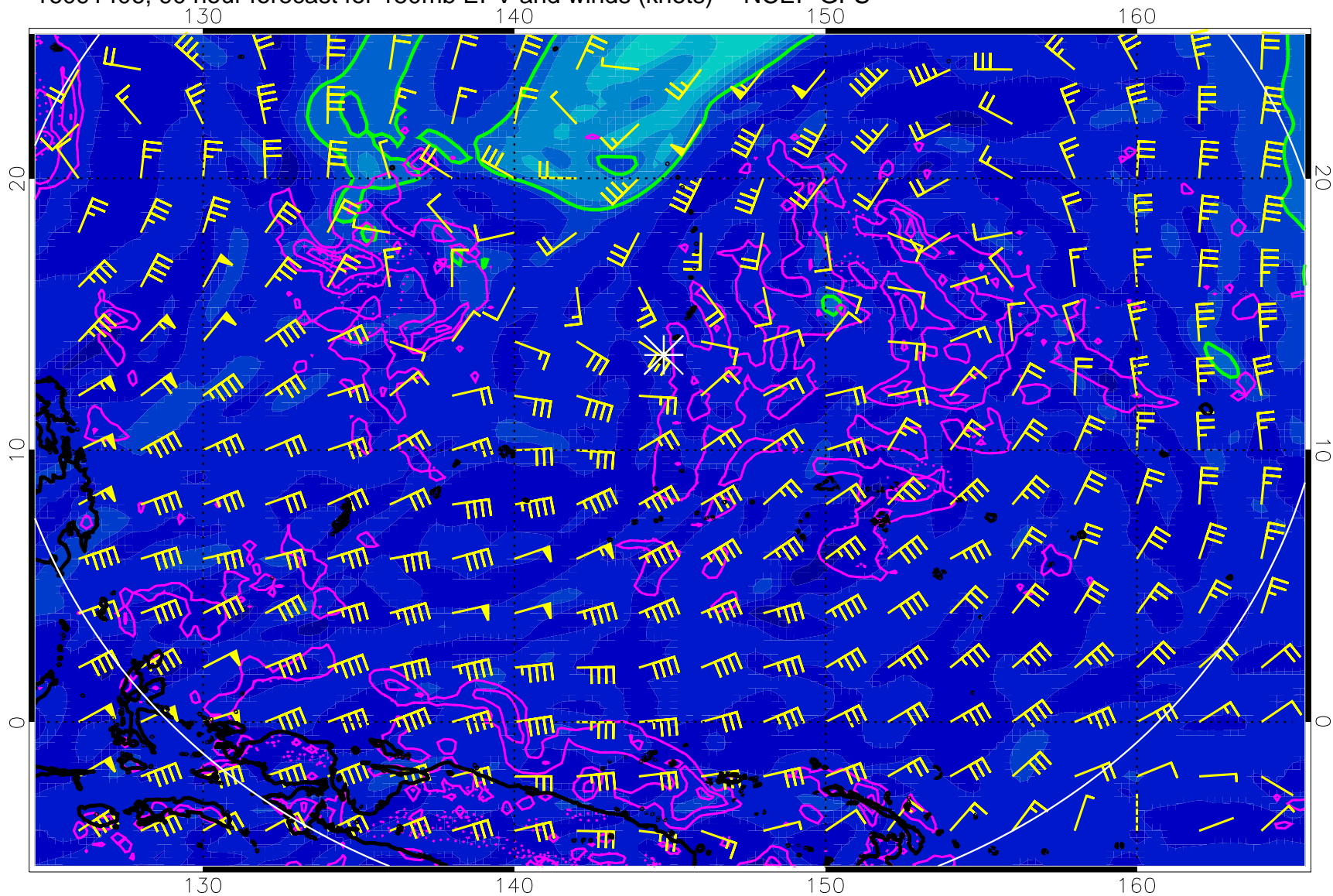
16091406, 90 hour forecast for 150mb EPV and winds (knots) -- NCEP GFS
