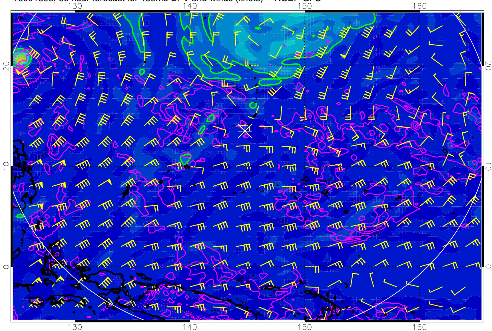
16091306, 66 hour forecast for 150mb EPV and winds (knots) -- NCEP GFS
