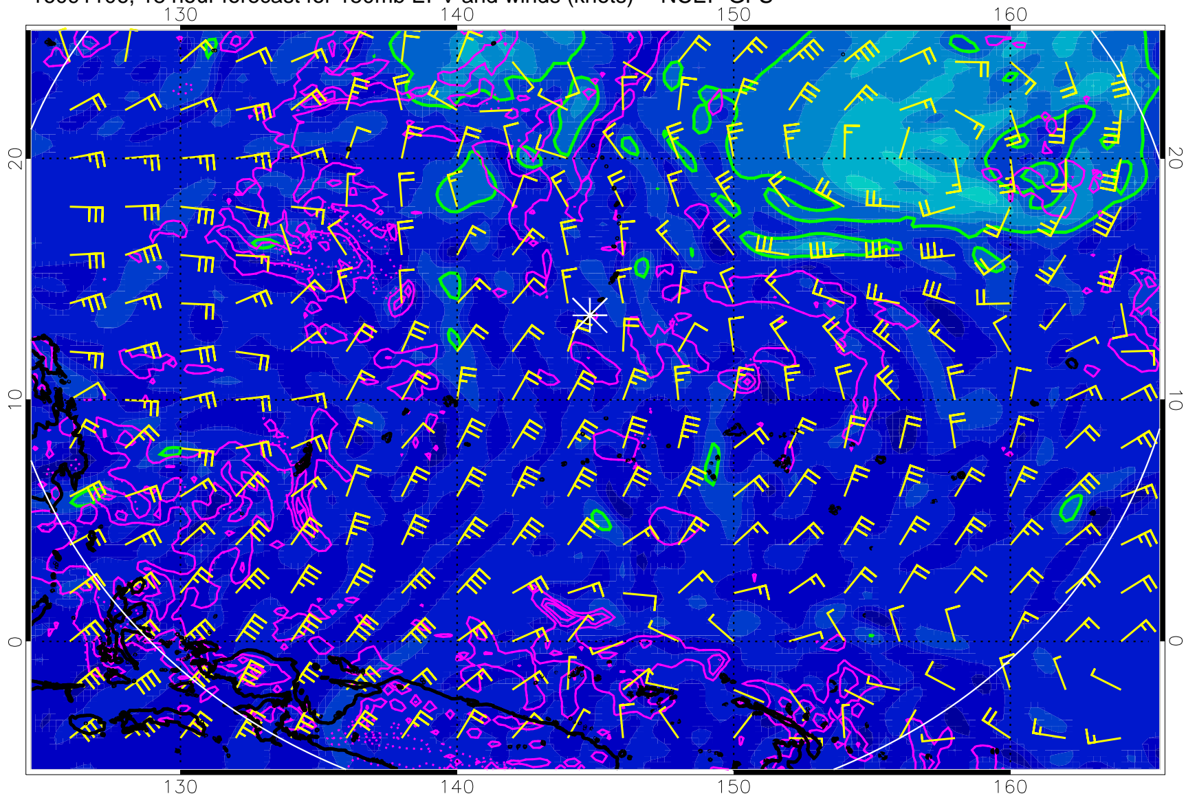
16091106, 18 hour forecast for 150mb EPV and winds (knots) -- NCEP GFS
