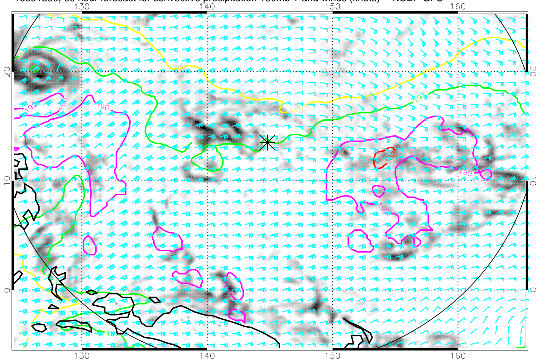
16091300, 60 hour forecast for convective precipitation 100mb T and winds (knots) -- NCEP GFS
