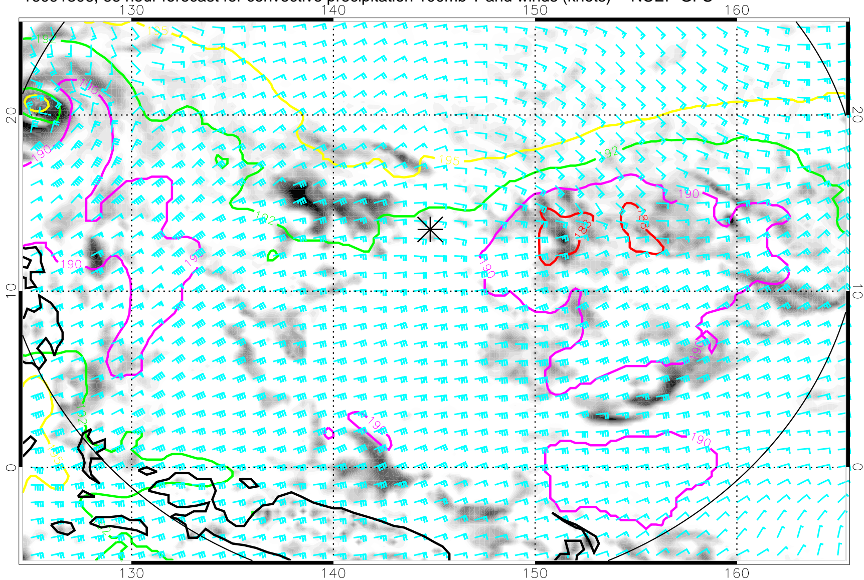
16091306, 66 hour forecast for convective precipitation 100mb T and winds (knots) -- NCEP GFS
