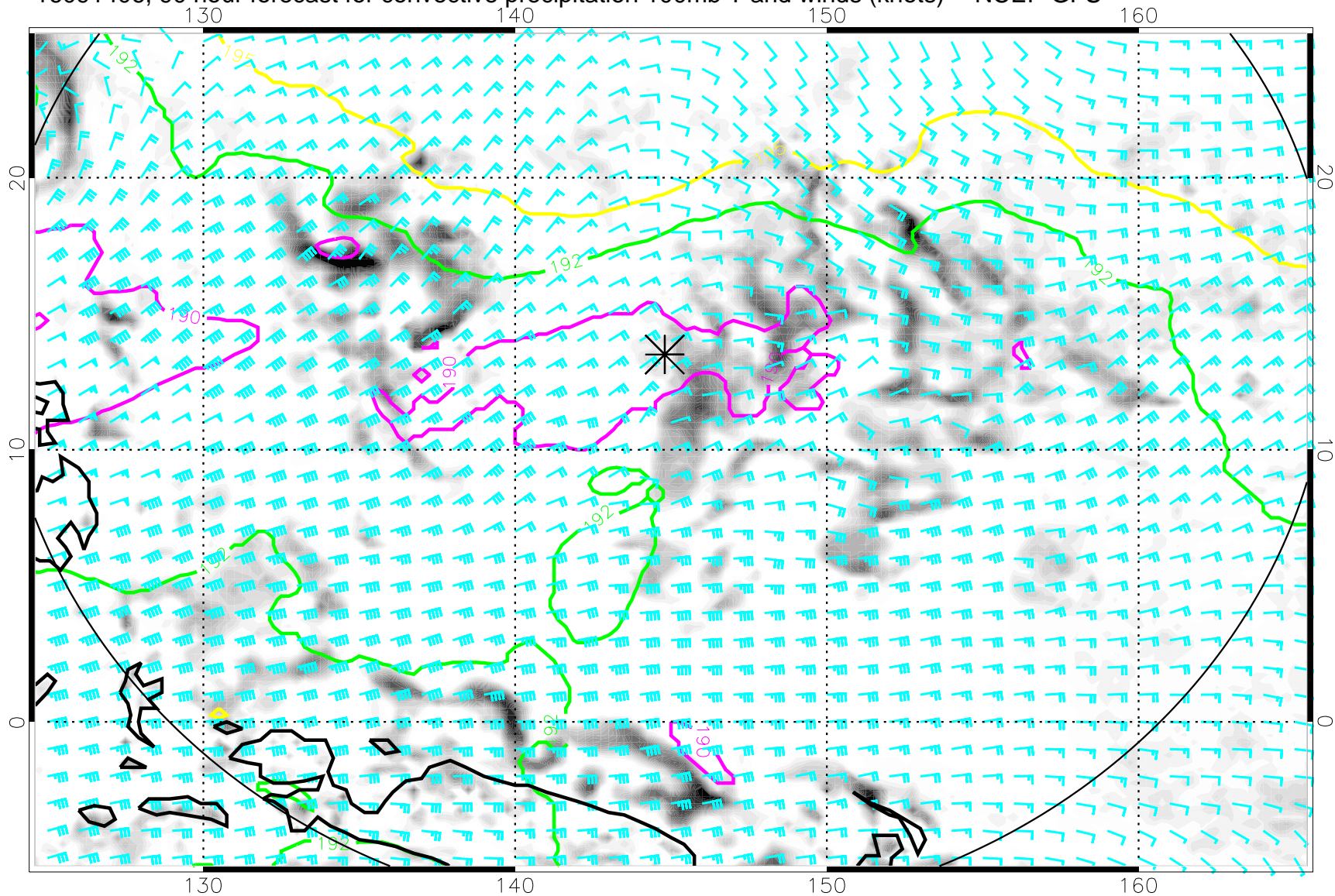
16091406, 90 hour forecast for convective precipitation 100mb T and winds (knots) -- NCEP GFS
