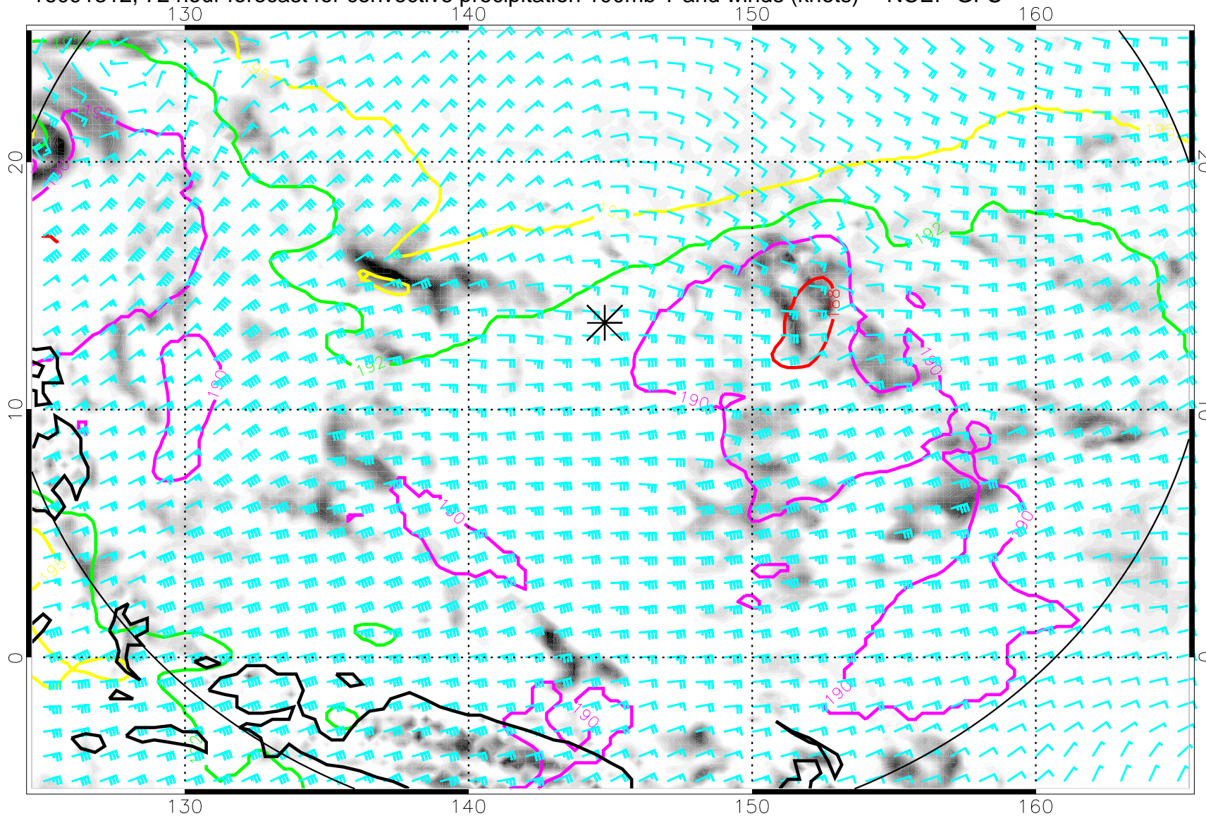
16091312, 72 hour forecast for convective precipitation 100mb T and winds (knots) -- NCEP GFS
