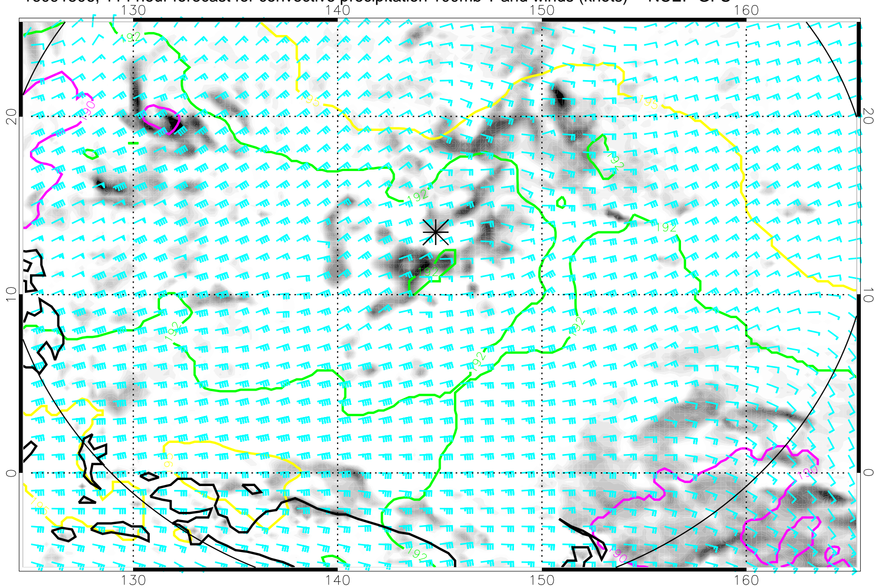
16091506, 114 hour forecast for convective precipitation 100mb T and winds (knots) -- NCEP GFS
