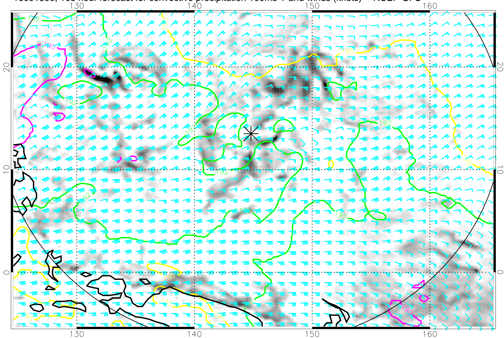
16091500, 108 hour forecast for convective precipitation 100mb T and winds (knots) -- NCEP GFS
