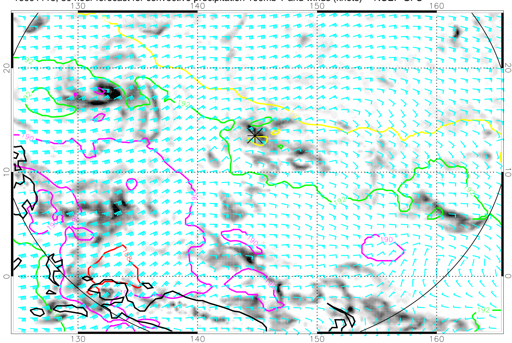
16091118, 30 hour forecast for convective precipitation 100mb T and winds (knots) -- NCEP GFS
