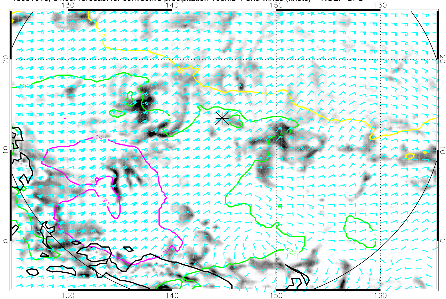
16091018, 6 hour forecast for convective precipitation 100mb T and winds (knots) -- NCEP GFS
