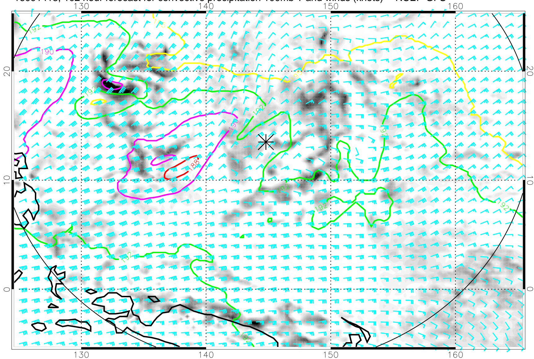
16091418, 102 hour forecast for convective precipitation 100mb T and winds (knots) -- NCEP GFS
