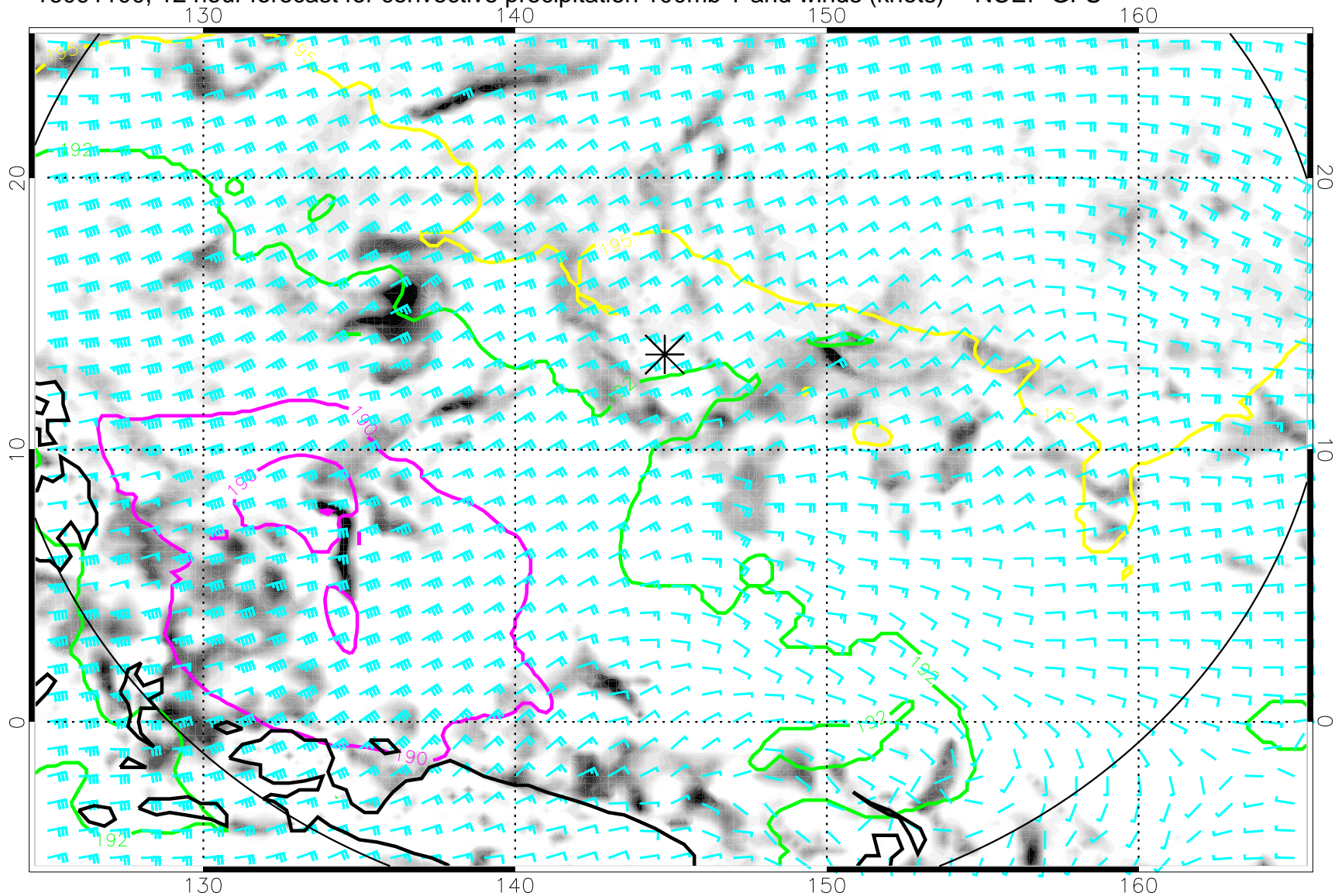
16091100, 12 hour forecast for convective precipitation 100mb T and winds (knots) -- NCEP GFS
