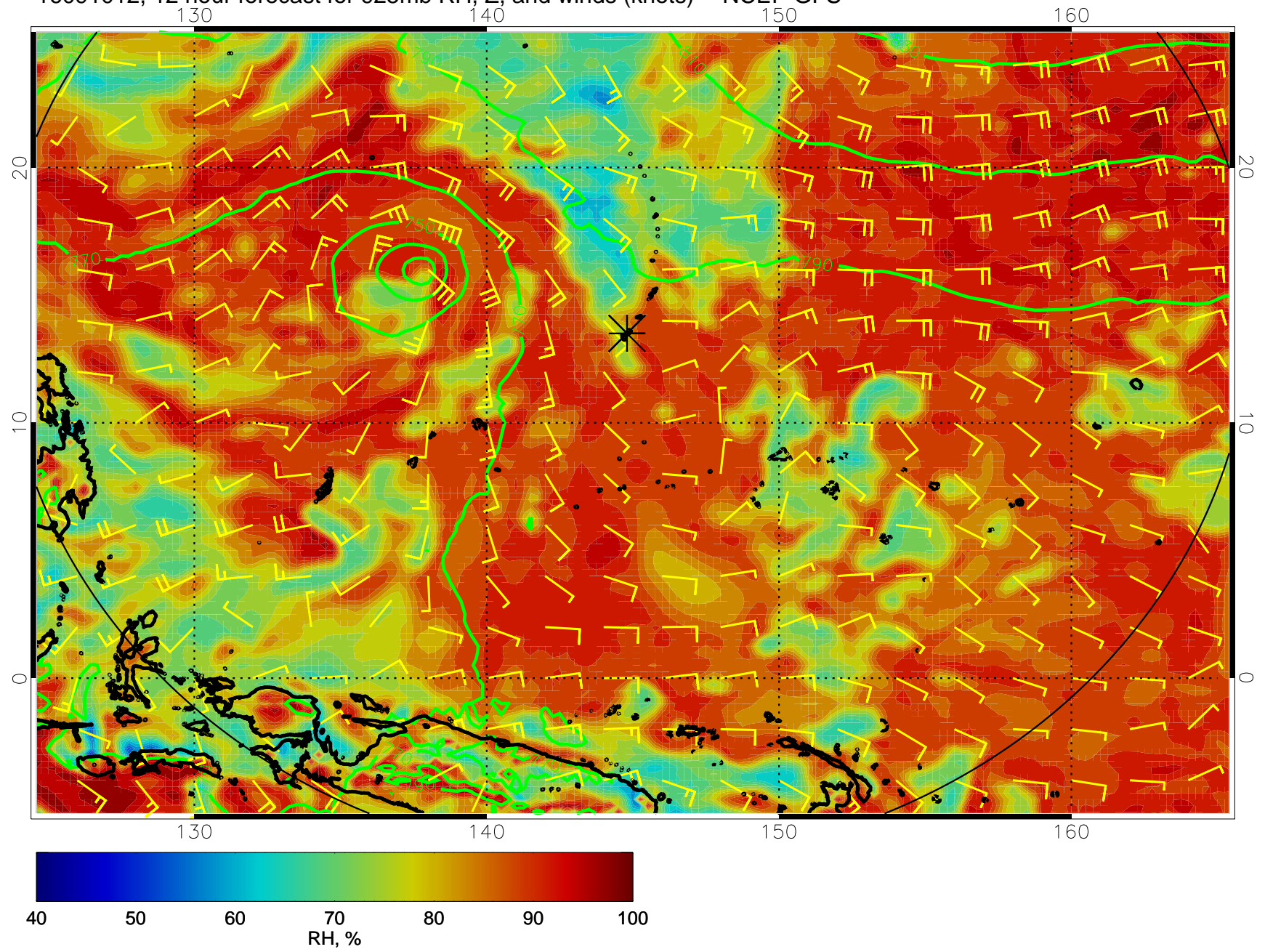
16091012, 12 hour forecast for 925mb RH, Z, and winds (knots) -- NCEP GFS
