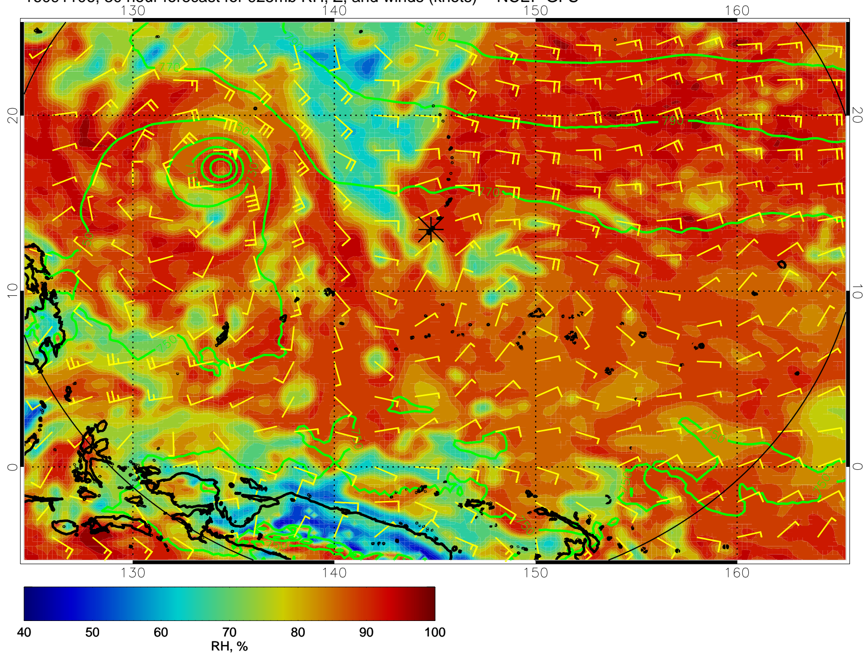
16091106, 30 hour forecast for 925mb RH, Z, and winds (knots) -- NCEP GFS
