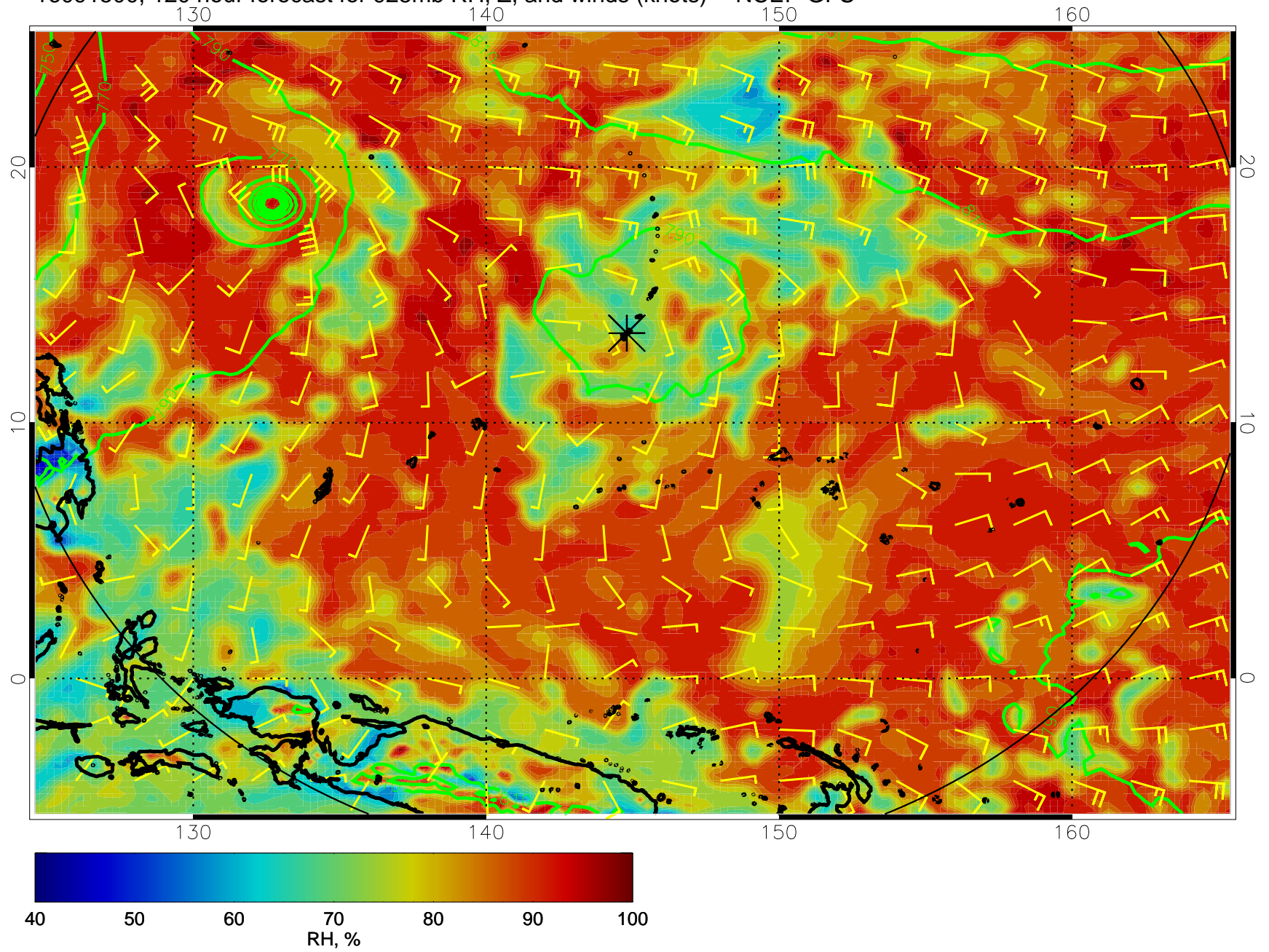
16091500, 120 hour forecast for 925mb RH, Z, and winds (knots) -- NCEP GFS
