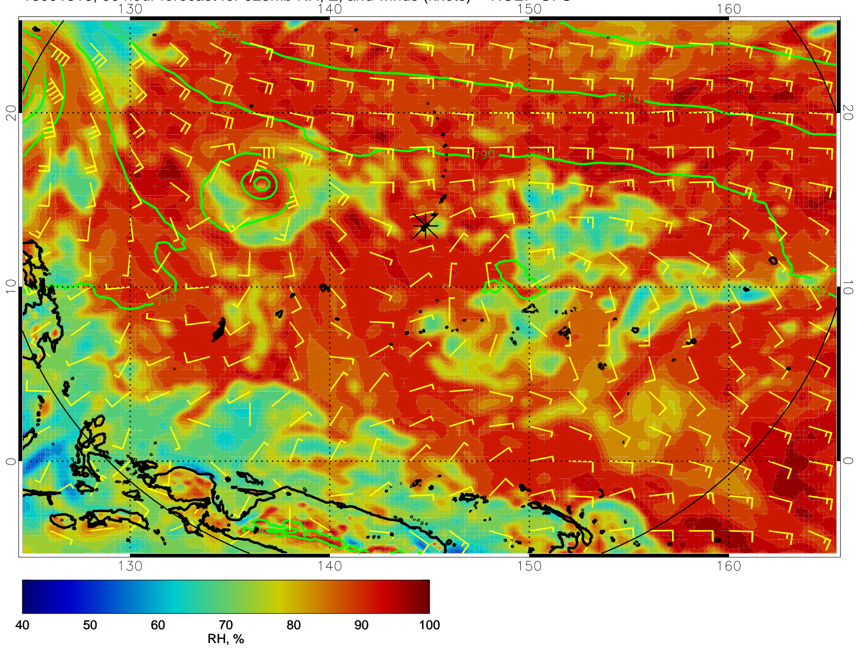
16091318, 90 hour forecast for 925mb RH, Z, and winds (knots) -- NCEP GFS
