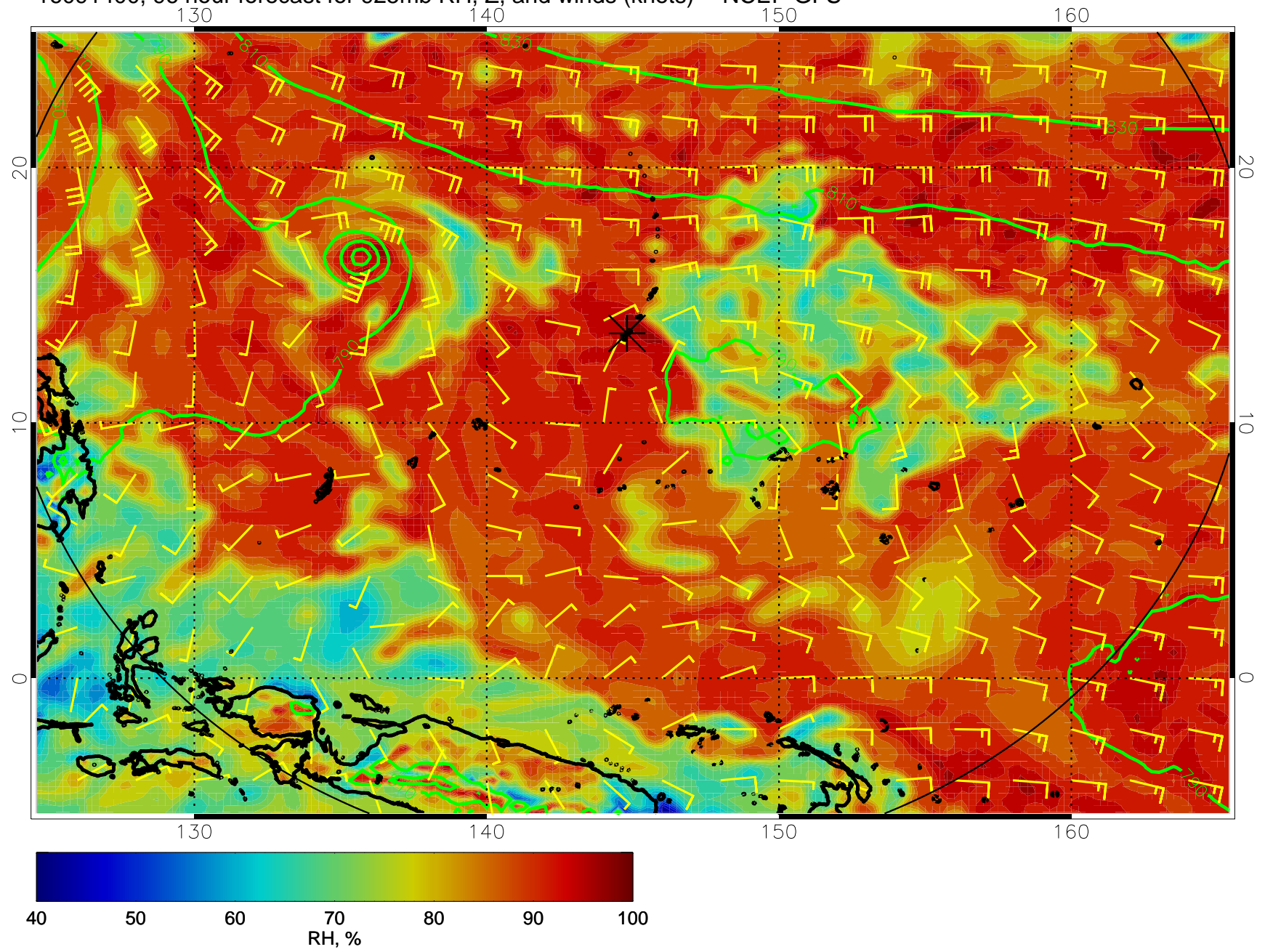
16091400, 96 hour forecast for 925mb RH, Z, and winds (knots) -- NCEP GFS
