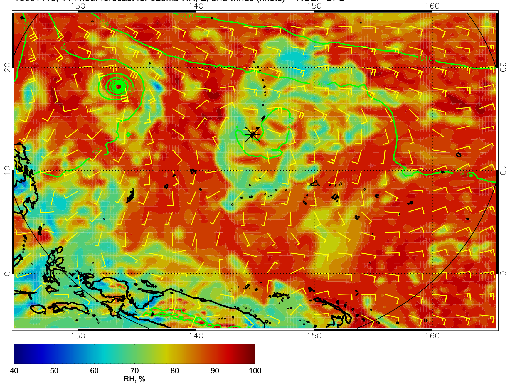
16091418, 114 hour forecast for 925mb RH, Z, and winds (knots) -- NCEP GFS
