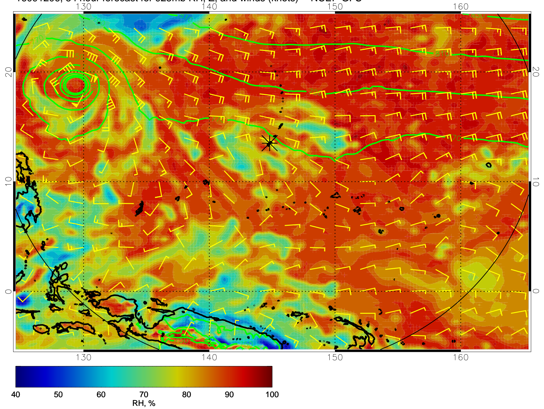
16091206, 54 hour forecast for 925mb RH, Z, and winds (knots) -- NCEP GFS
