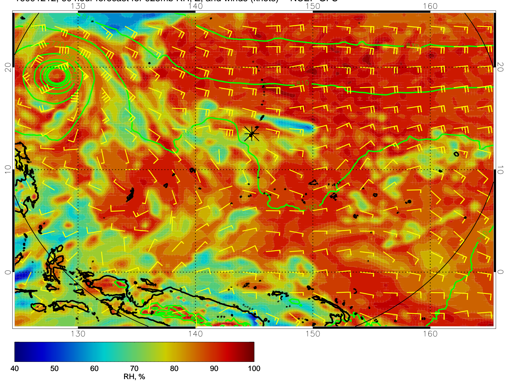
16091212, 60 hour forecast for 925mb RH, Z, and winds (knots) -- NCEP GFS
