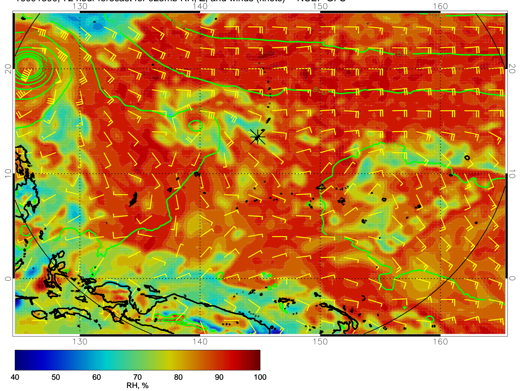
16091300, 72 hour forecast for 925mb RH, Z, and winds (knots) -- NCEP GFS
