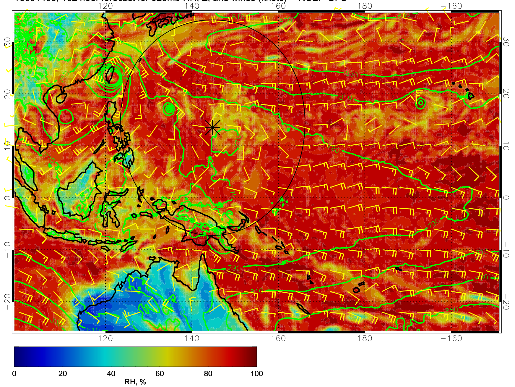
16091406, 102 hour forecast for 925mb RH, Z, and winds (knots) -- NCEP GFS
