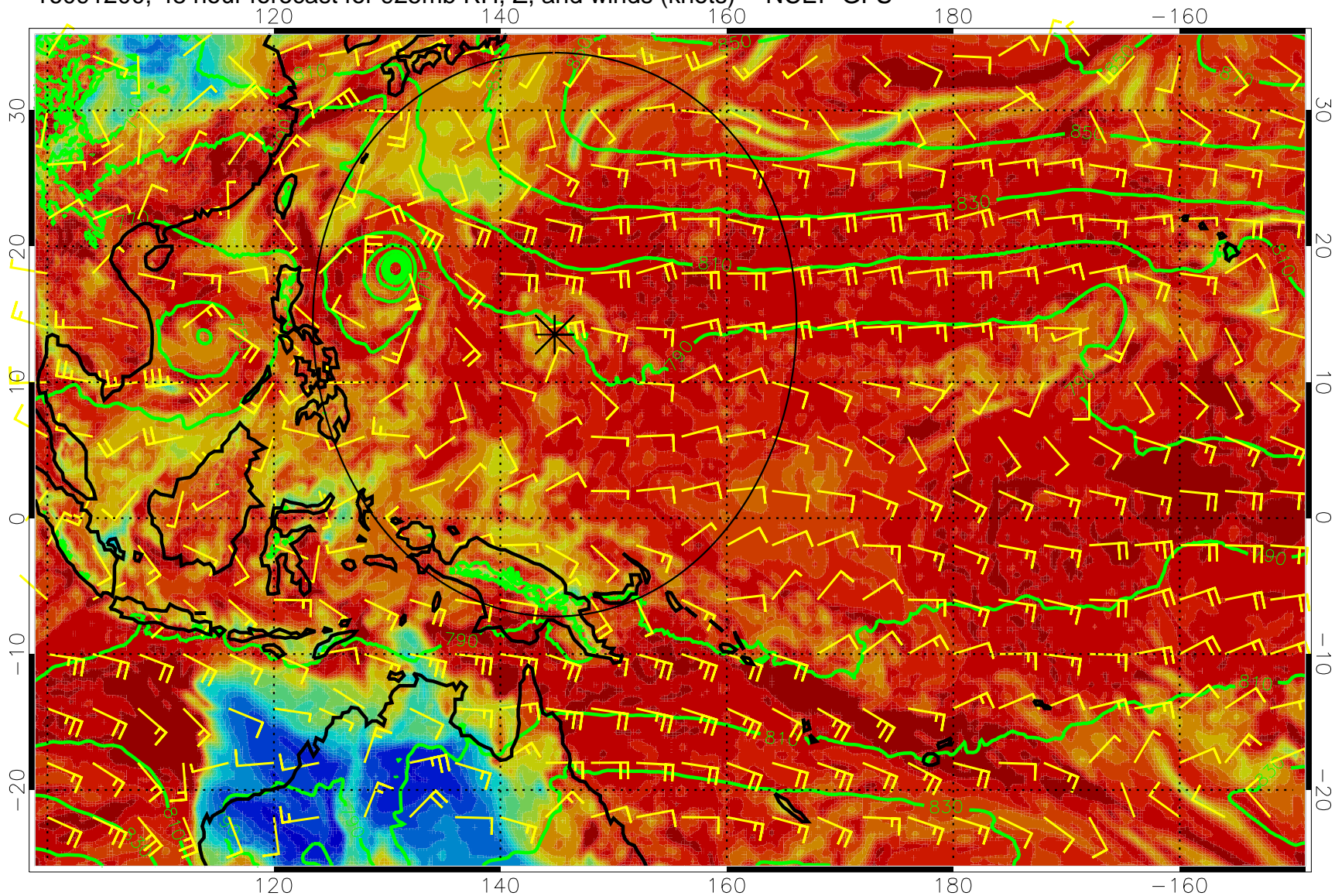
16091200, 48 hour forecast for 925mb RH, Z, and winds (knots) -- NCEP GFS
