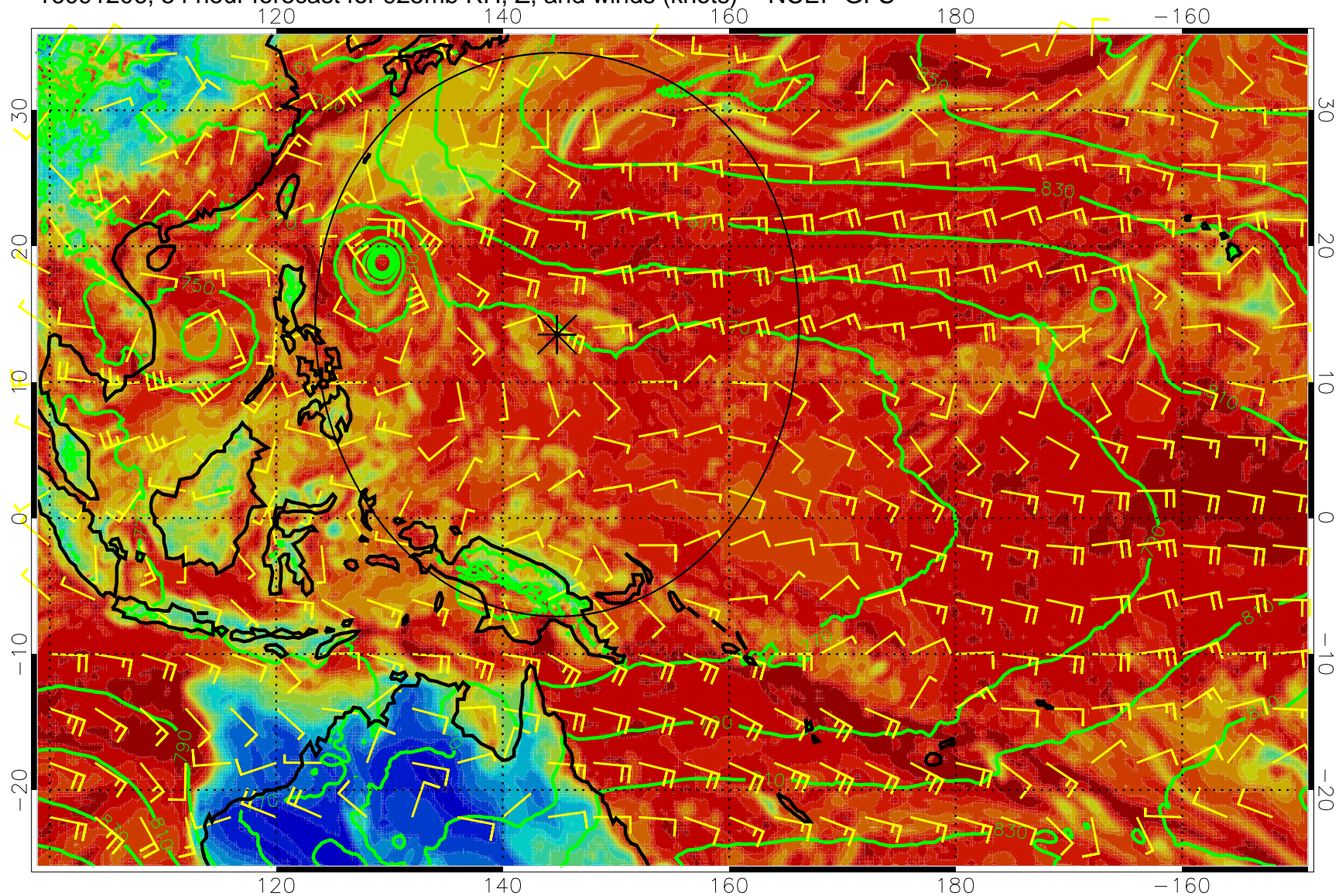
16091206, 54 hour forecast for 925mb RH, Z, and winds (knots) -- NCEP GFS
