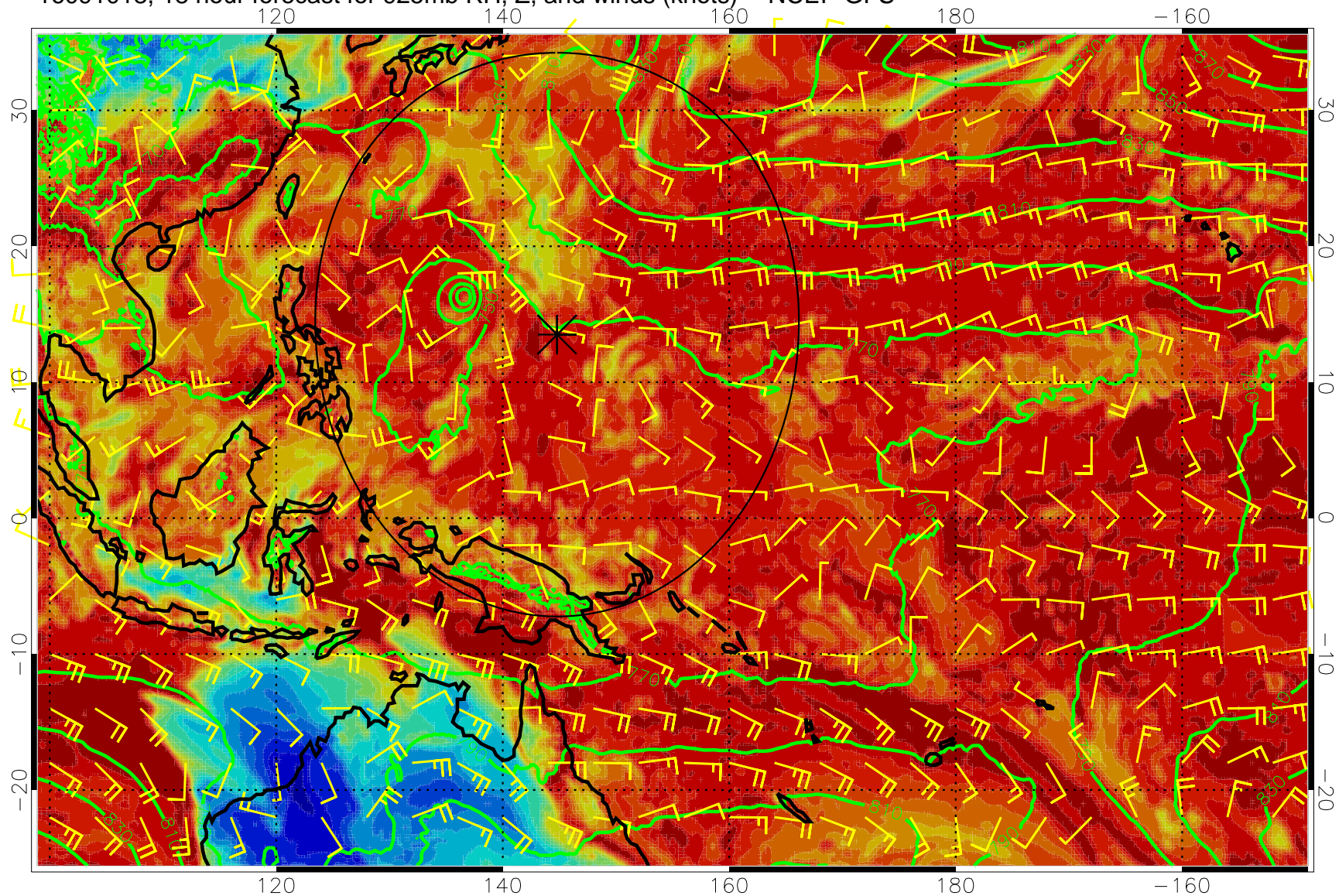
16091018, 18 hour forecast for 925mb RH, Z, and winds (knots) -- NCEP GFS
