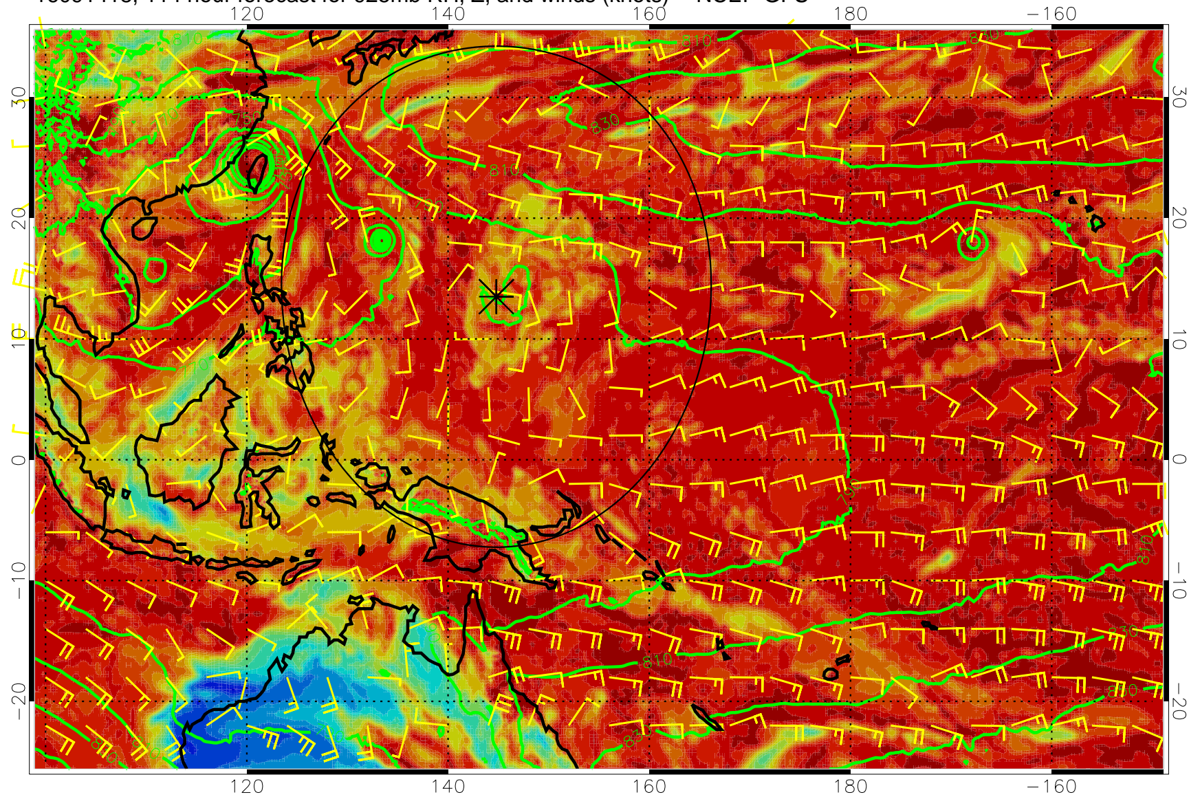
16091418, 114 hour forecast for 925mb RH, Z, and winds (knots) -- NCEP GFS
