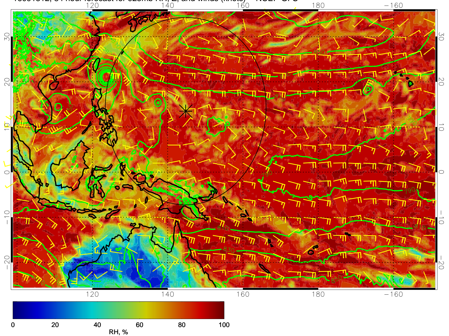
16091312, 84 hour forecast for 925mb RH, Z, and winds (knots) -- NCEP GFS
