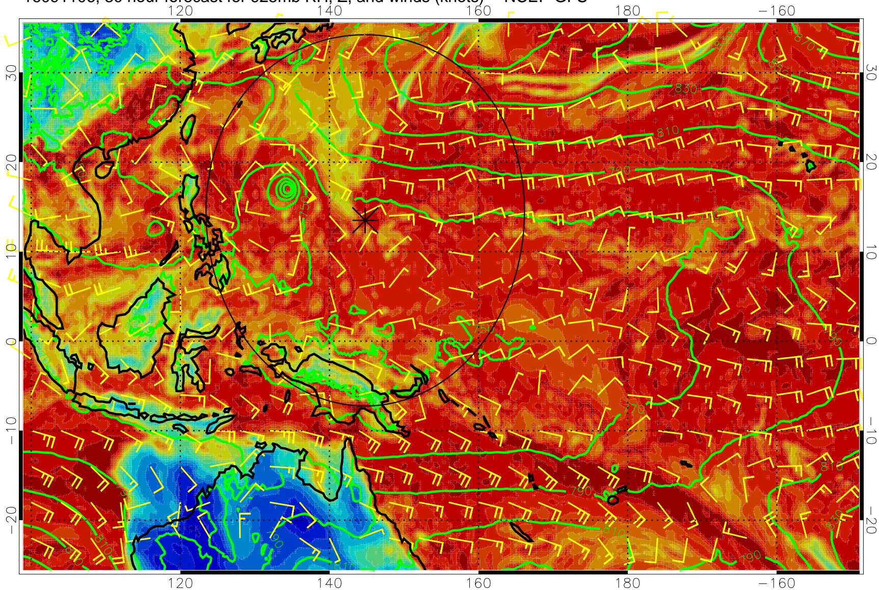
16091106, 30 hour forecast for 925mb RH, Z, and winds (knots) -- NCEP GFS
