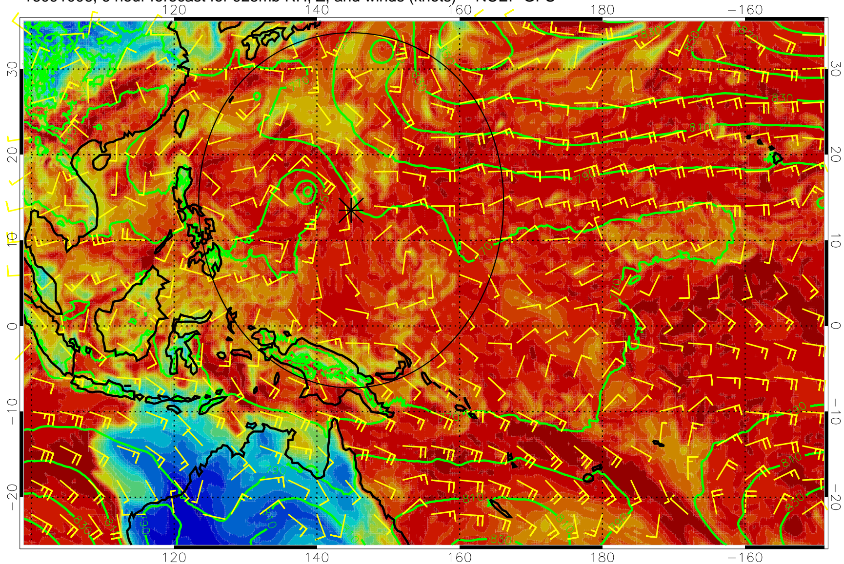
16091006, 6 hour forecast for 925mb RH, Z, and winds (knots) -- NCEP GFS
