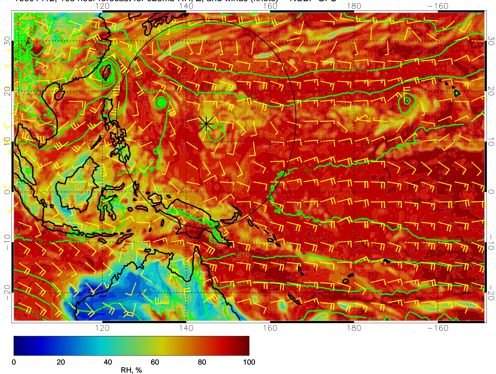
16091412, 108 hour forecast for 925mb RH, Z, and winds (knots) -- NCEP GFS
