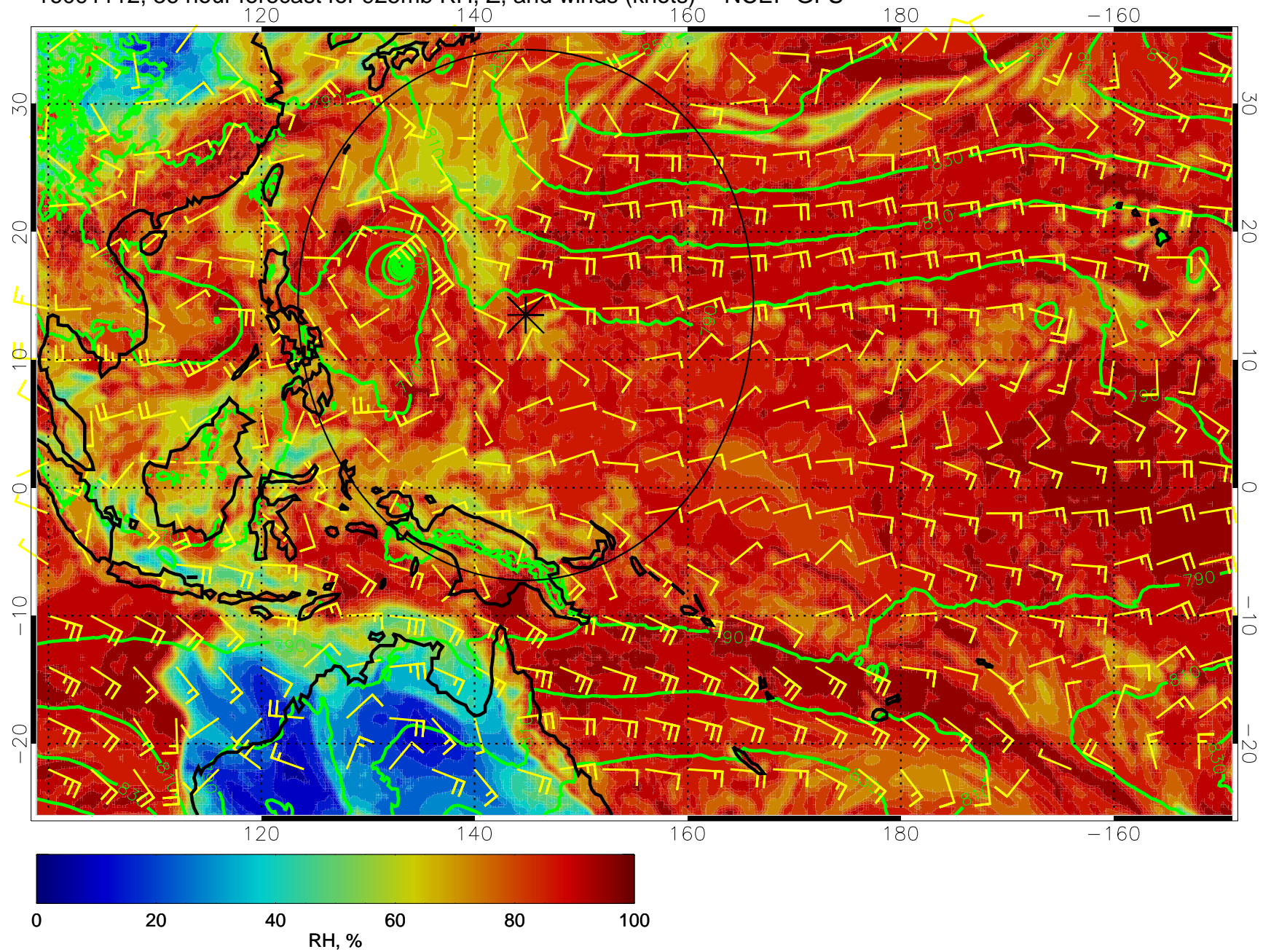
16091112, 36 hour forecast for 925mb RH, Z, and winds (knots) -- NCEP GFS
