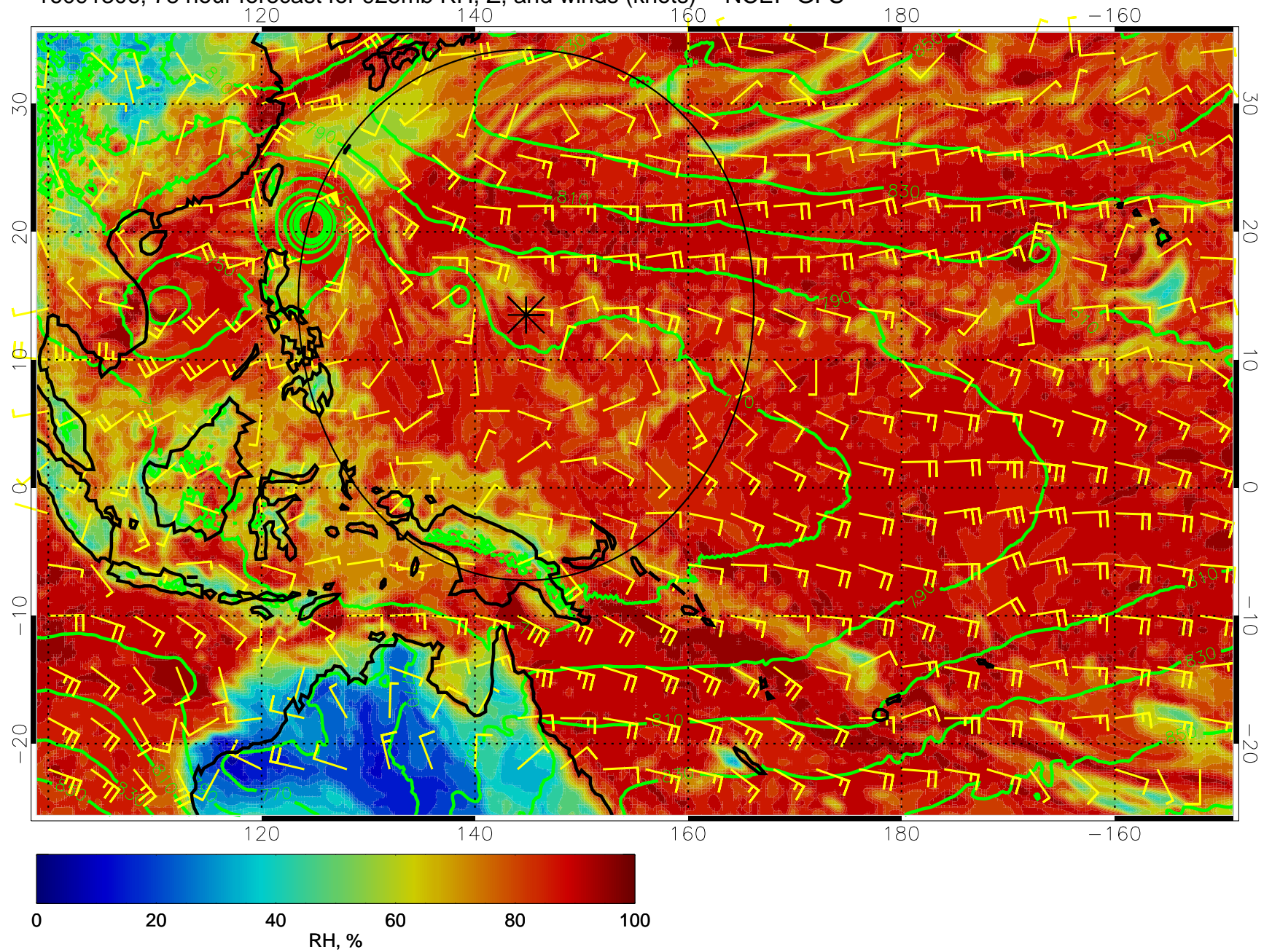
16091306, 78 hour forecast for 925mb RH, Z, and winds (knots) -- NCEP GFS
