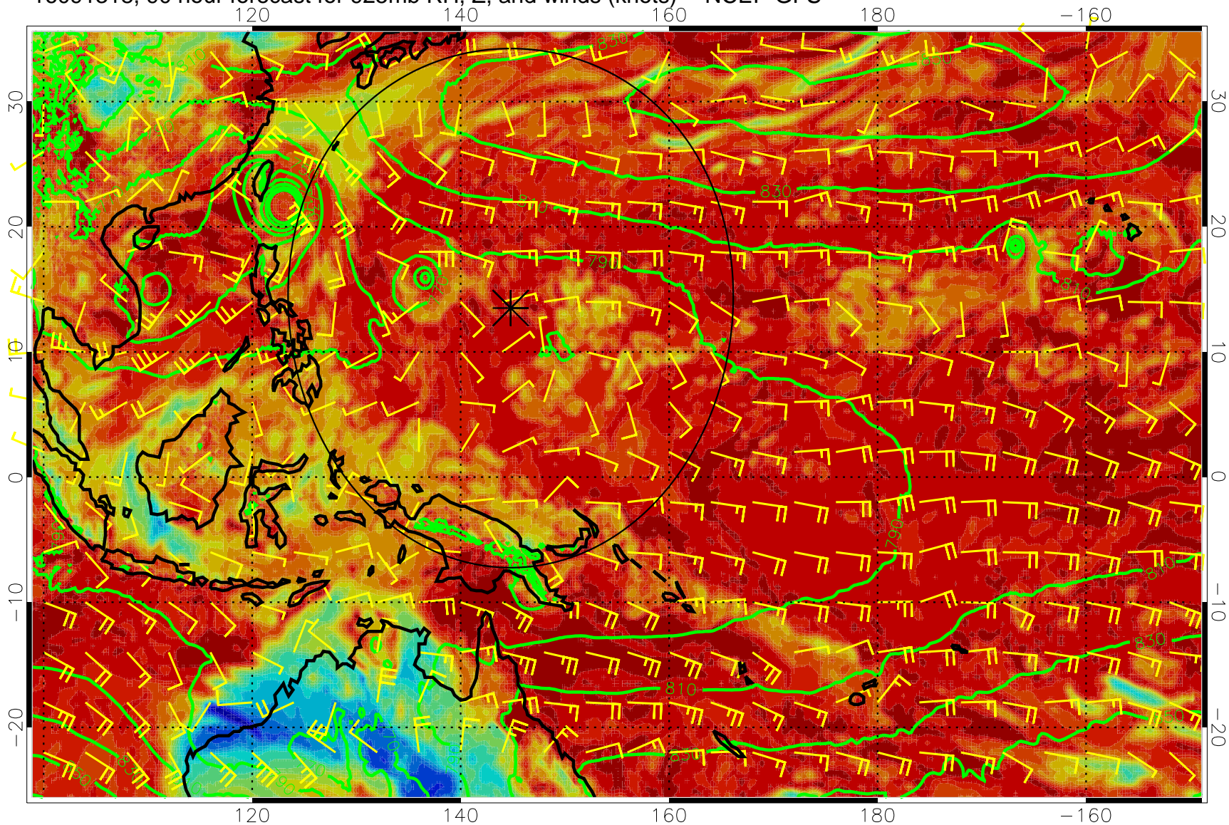
16091318, 90 hour forecast for 925mb RH, Z, and winds (knots) -- NCEP GFS
