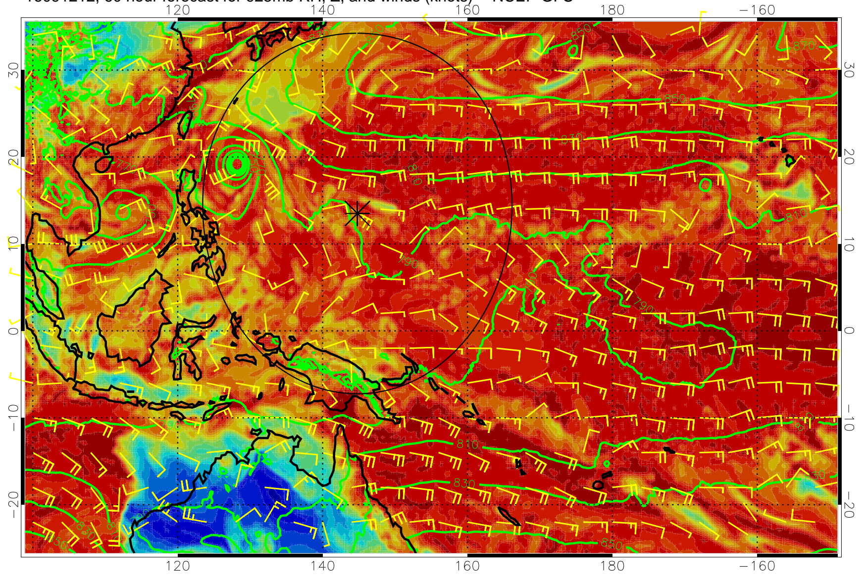
16091212, 60 hour forecast for 925mb RH, Z, and winds (knots) -- NCEP GFS
