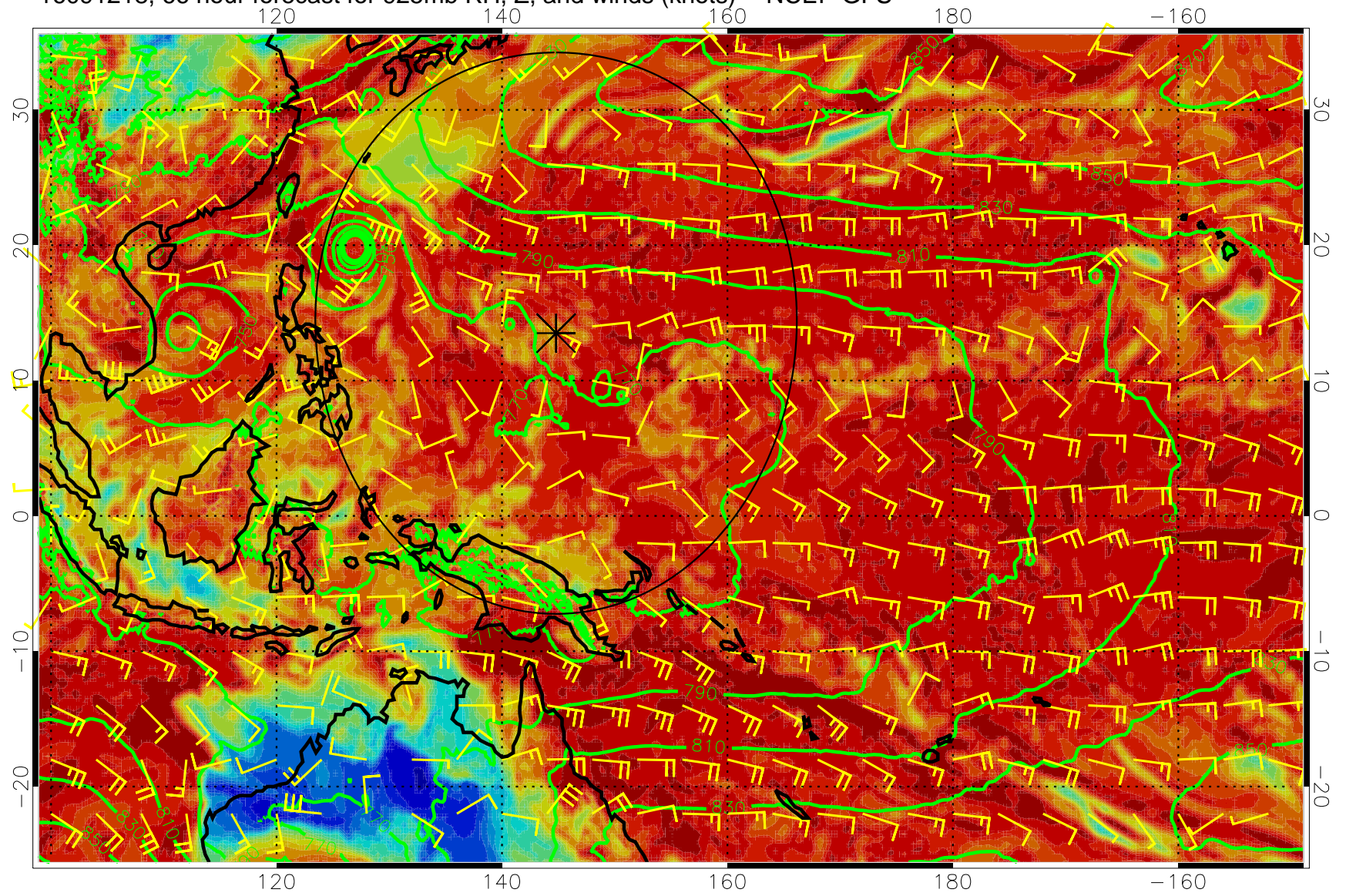
16091218, 66 hour forecast for 925mb RH, Z, and winds (knots) -- NCEP GFS
