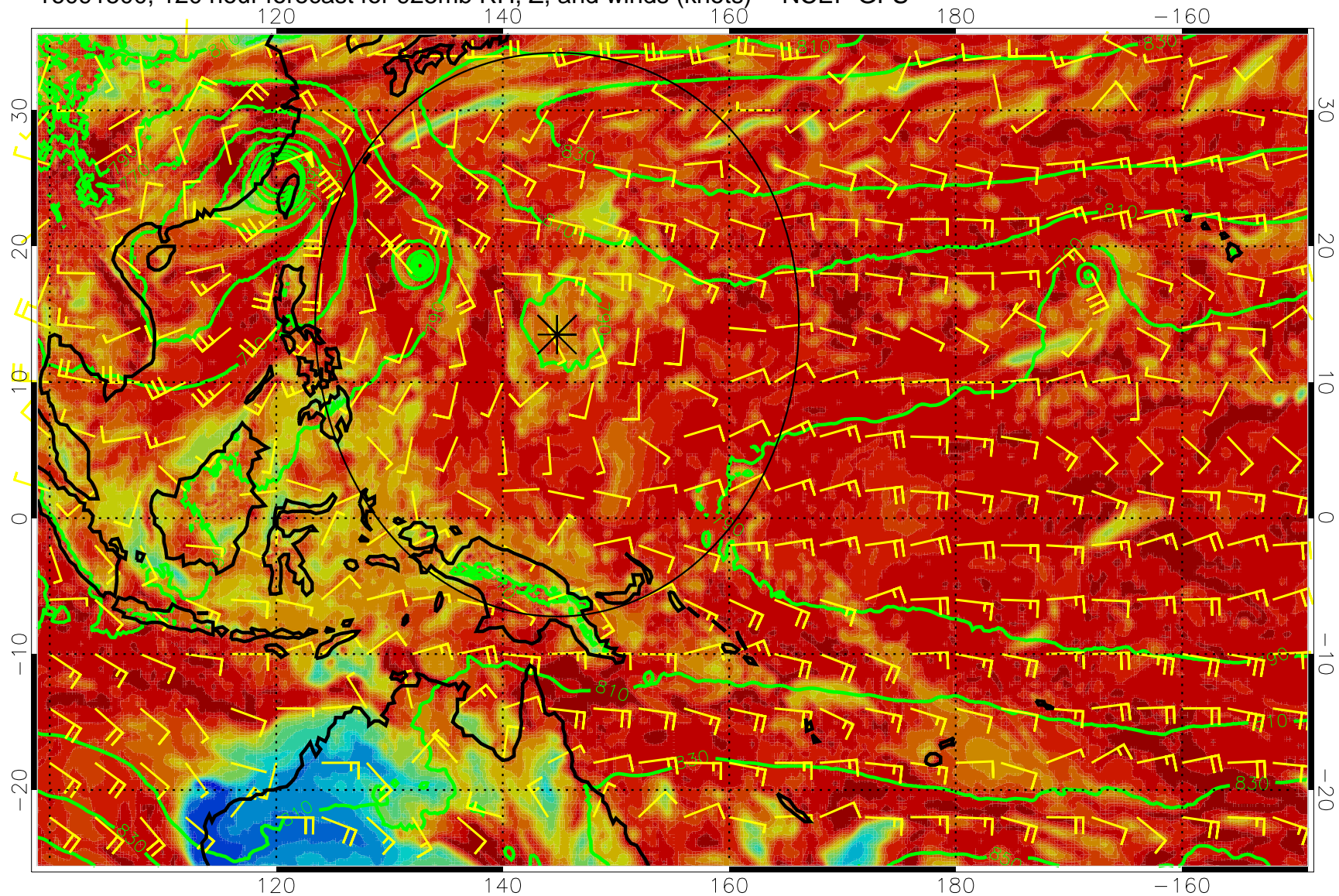
16091500, 120 hour forecast for 925mb RH, Z, and winds (knots) -- NCEP GFS
