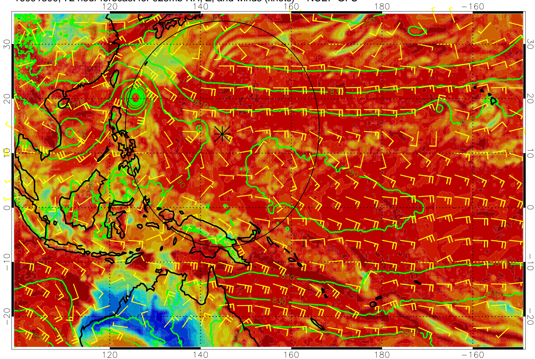
16091300, 72 hour forecast for 925mb RH, Z, and winds (knots) -- NCEP GFS
