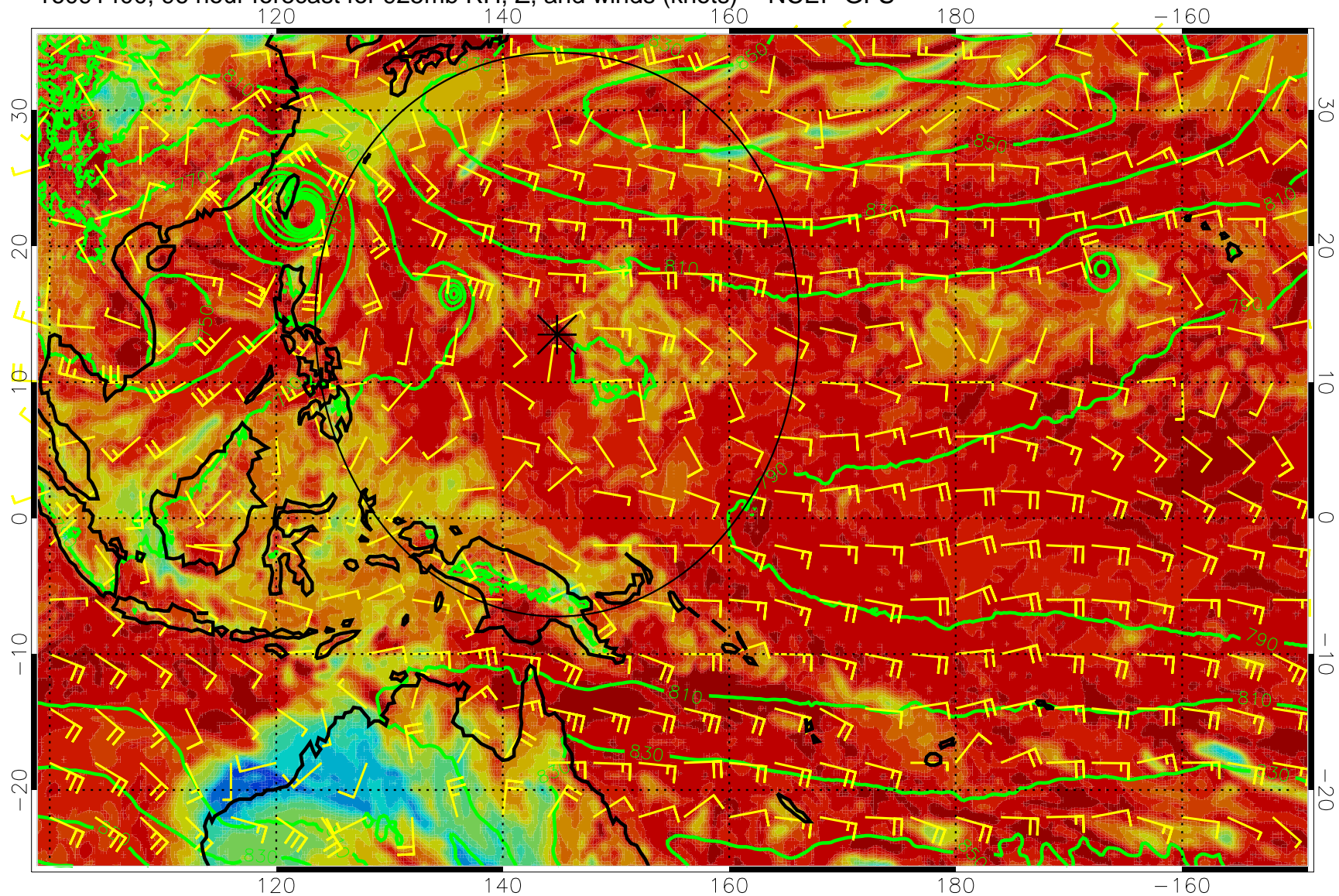
16091400, 96 hour forecast for 925mb RH, Z, and winds (knots) -- NCEP GFS
