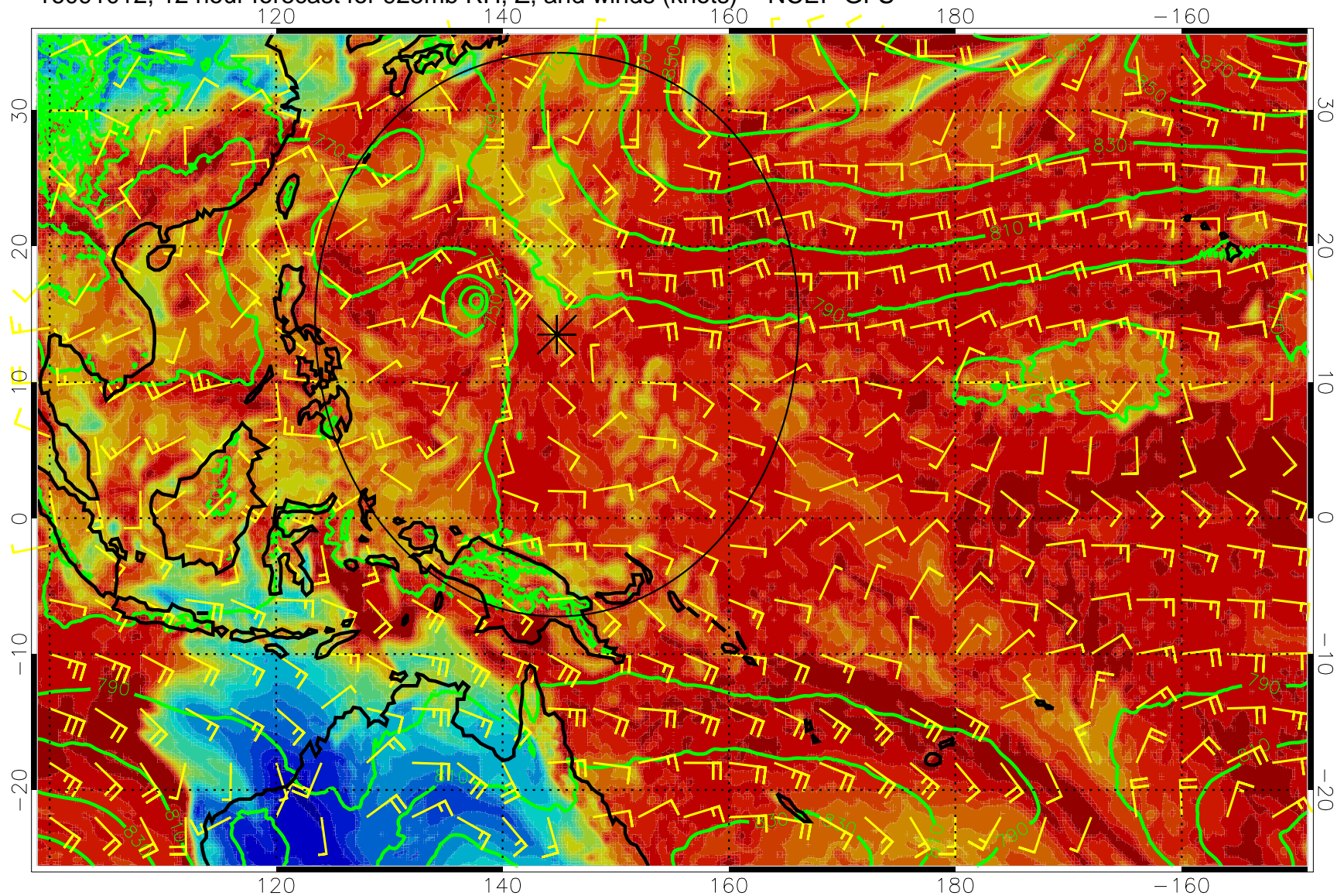
16091012, 12 hour forecast for 925mb RH, Z, and winds (knots) -- NCEP GFS
