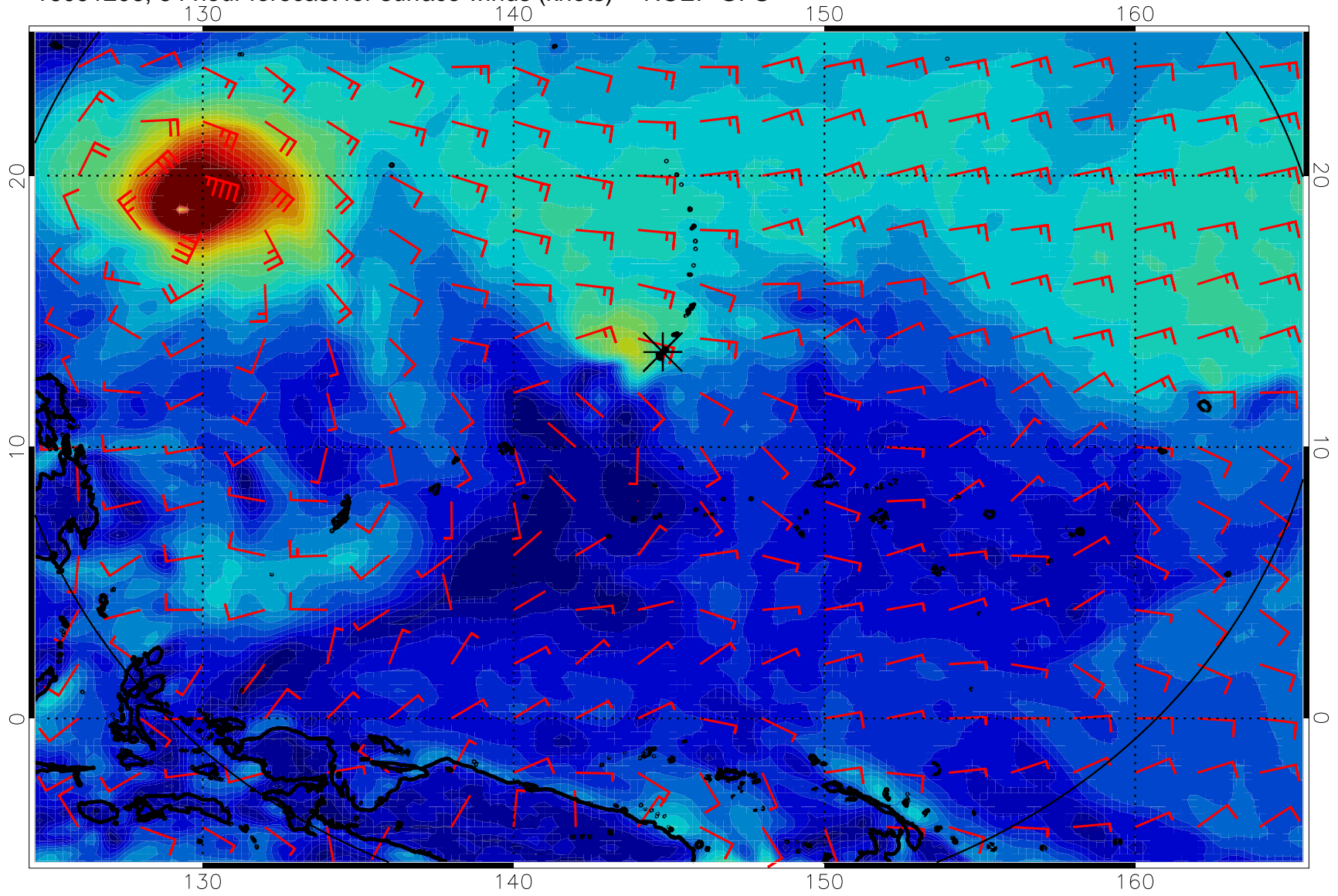
16091206, 54 hour forecast for surface winds (knots) -- NCEP GFS
