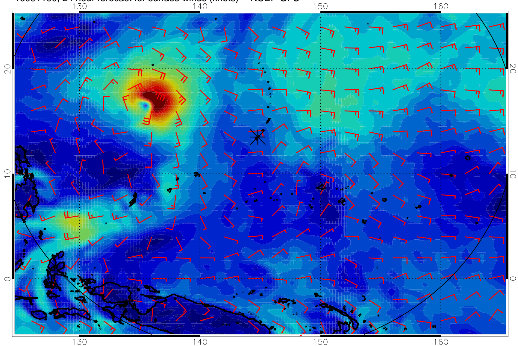
16091100, 24 hour forecast for surface winds (knots) -- NCEP GFS
