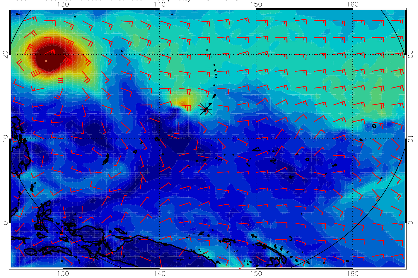
16091212, 60 hour forecast for surface winds (knots) -- NCEP GFS
