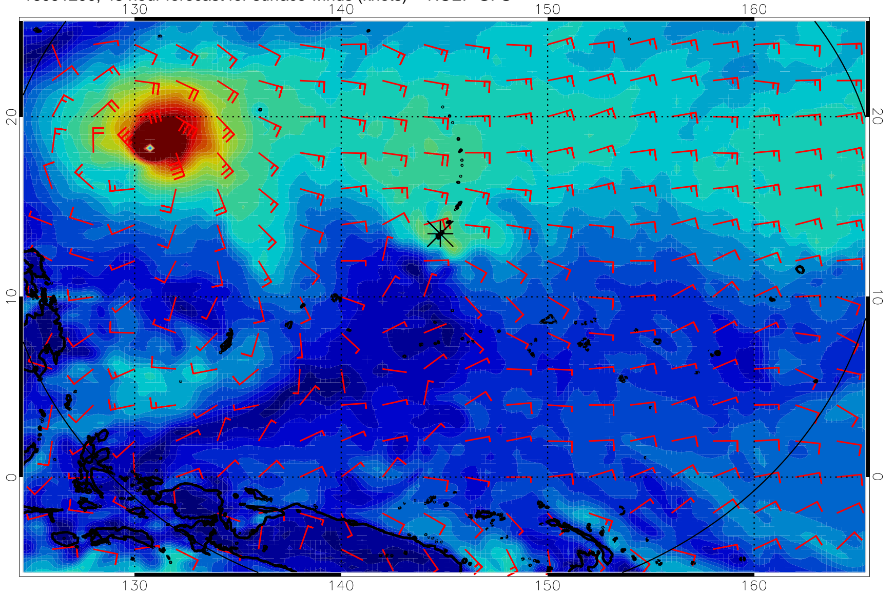
16091200, 48 hour forecast for surface winds (knots) -- NCEP GFS
