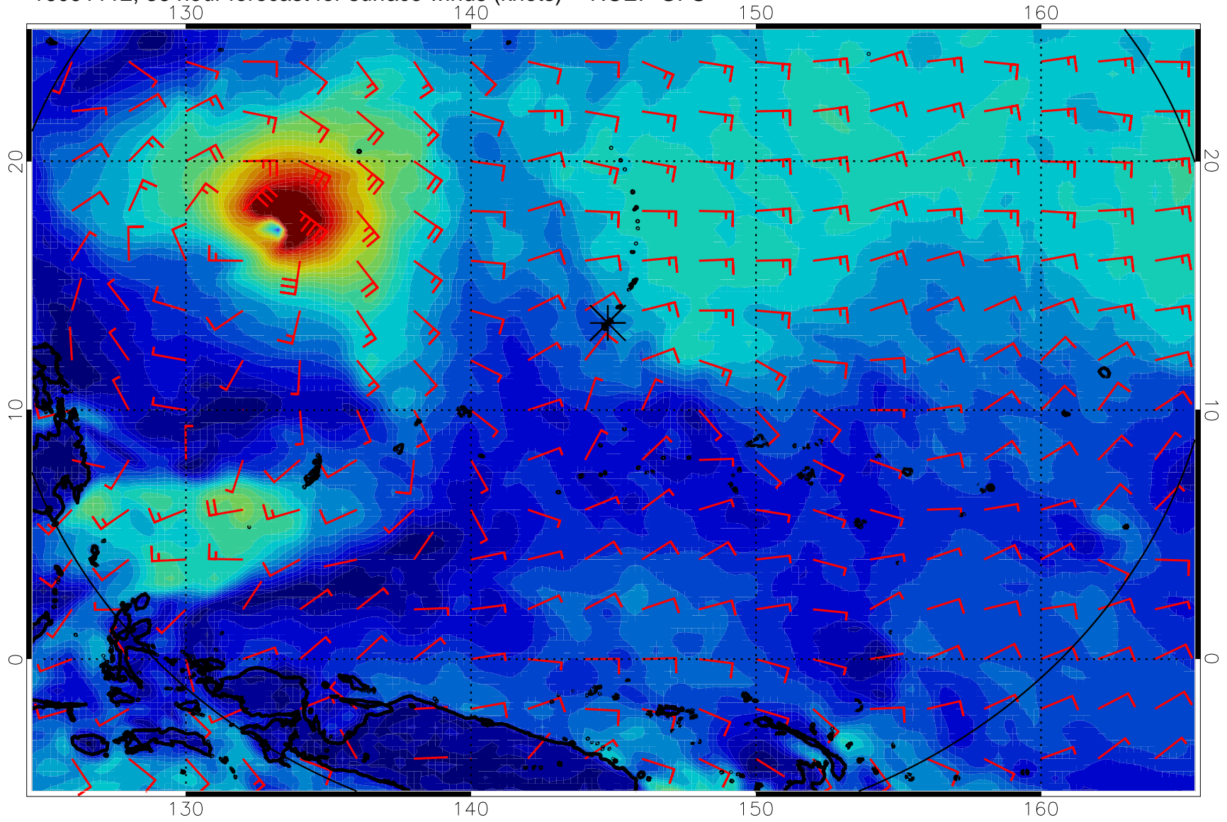
16091112, 36 hour forecast for surface winds (knots) -- NCEP GFS
