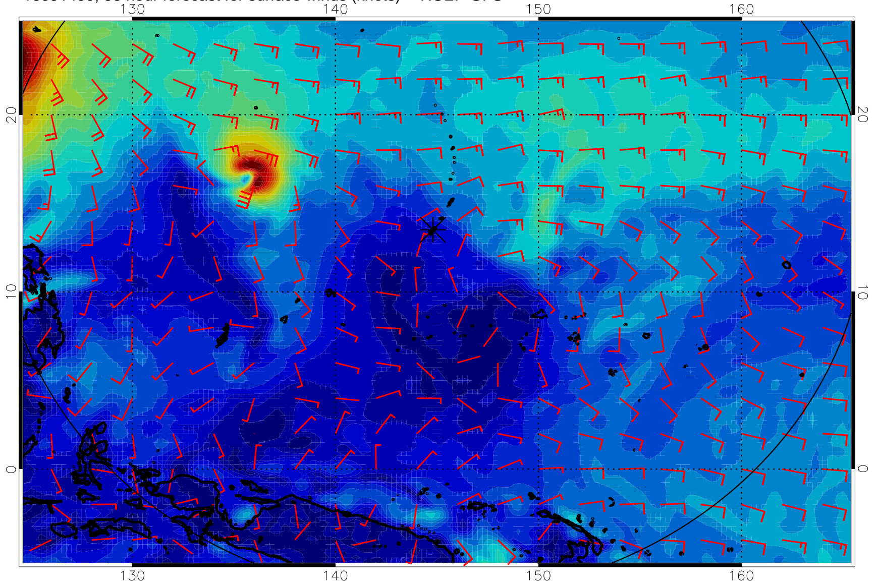
16091400, 96 hour forecast for surface winds (knots) -- NCEP GFS
