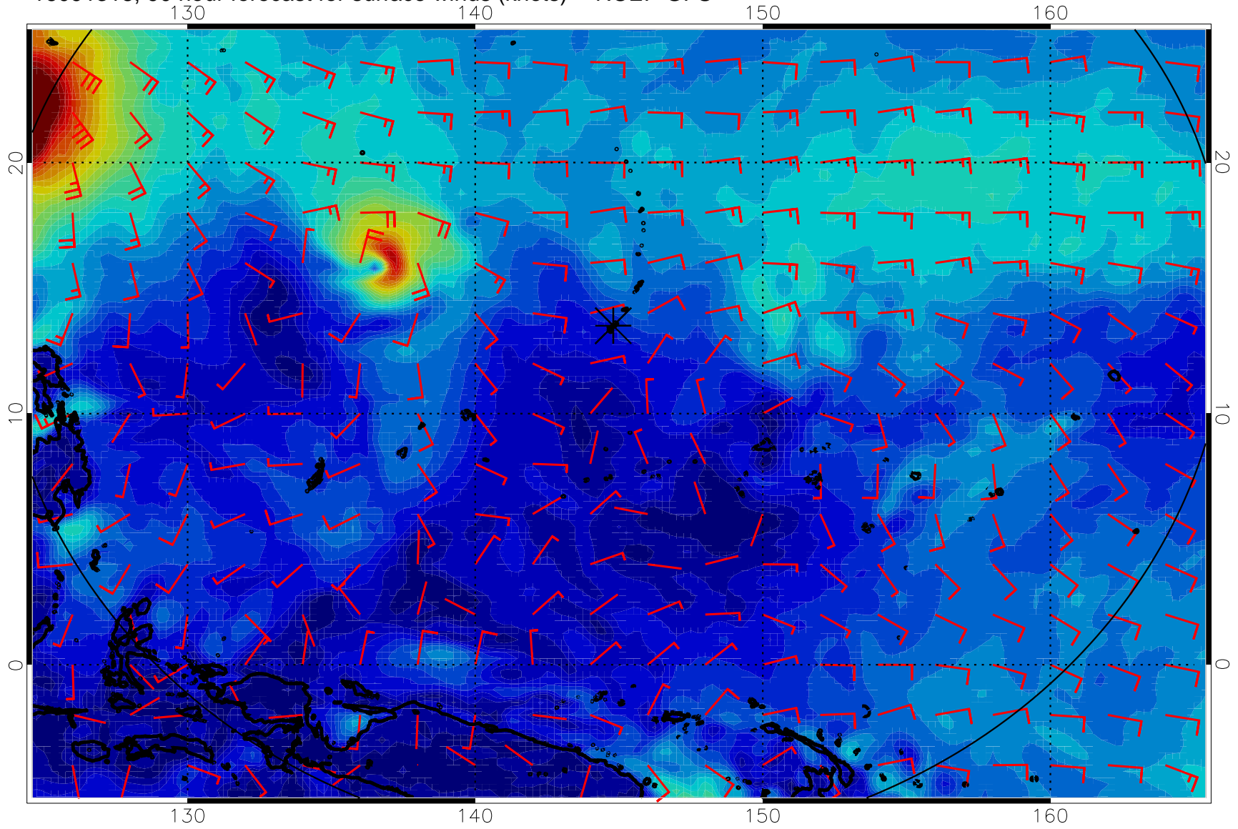
16091318, 90 hour forecast for surface winds (knots) -- NCEP GFS
