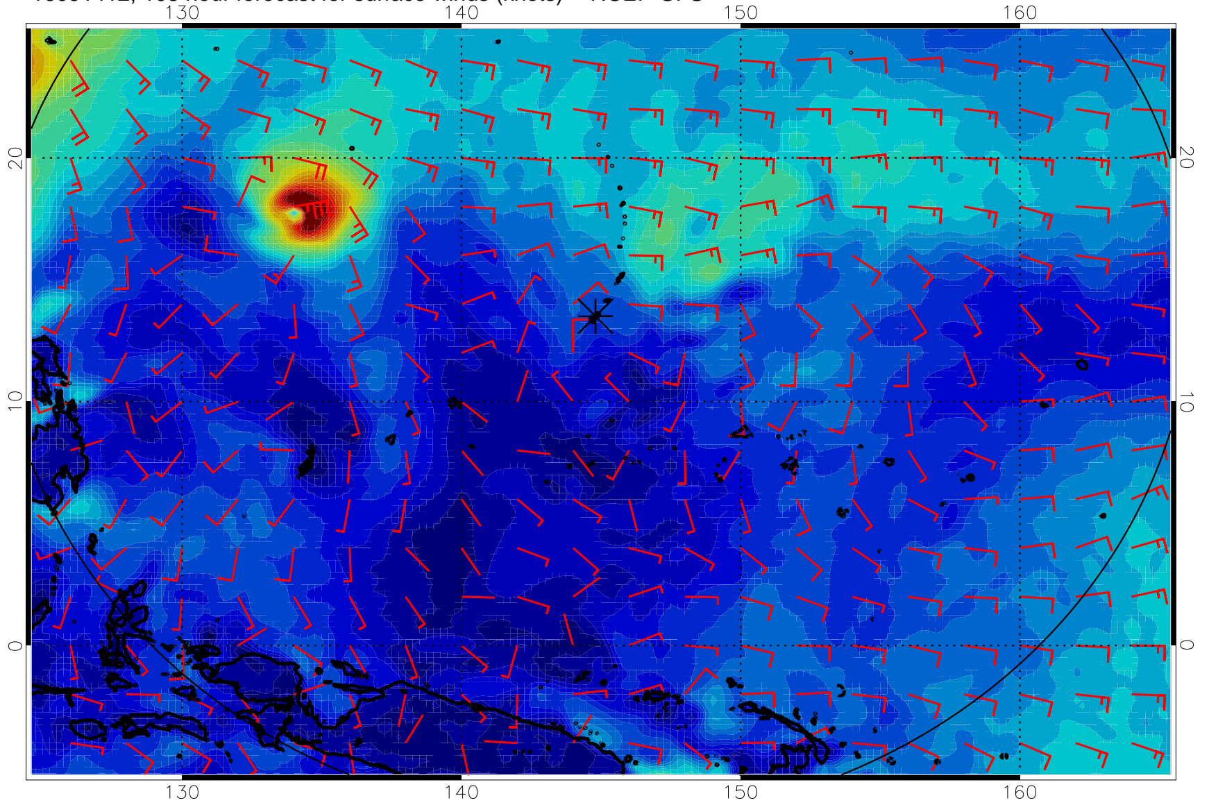
16091412, 108 hour forecast for surface winds (knots) -- NCEP GFS
