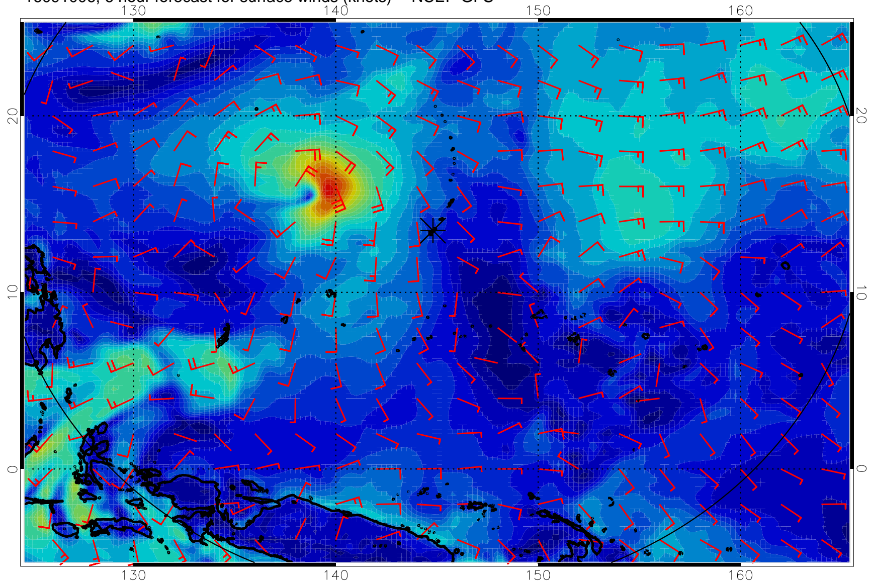
16091006, 6 hour forecast for surface winds (knots) -- NCEP GFS
