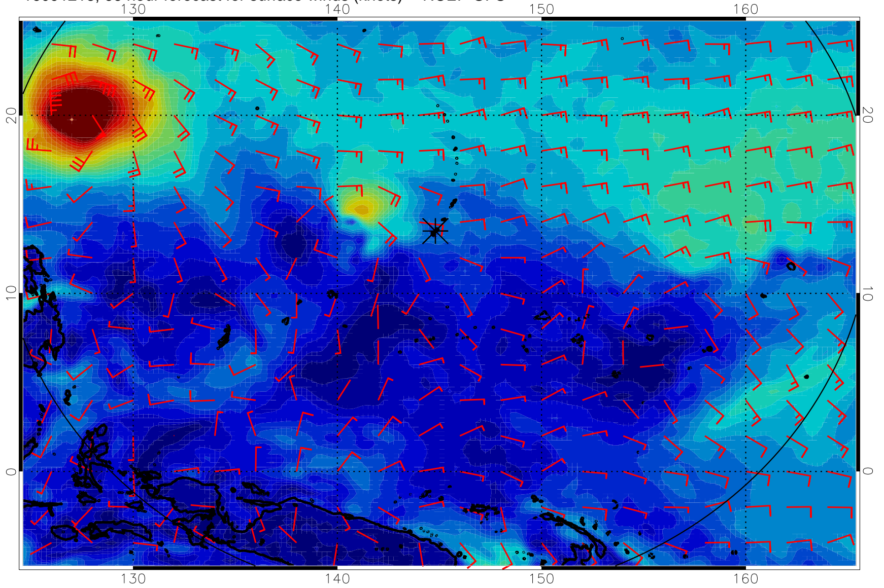
16091218, 66 hour forecast for surface winds (knots) -- NCEP GFS
