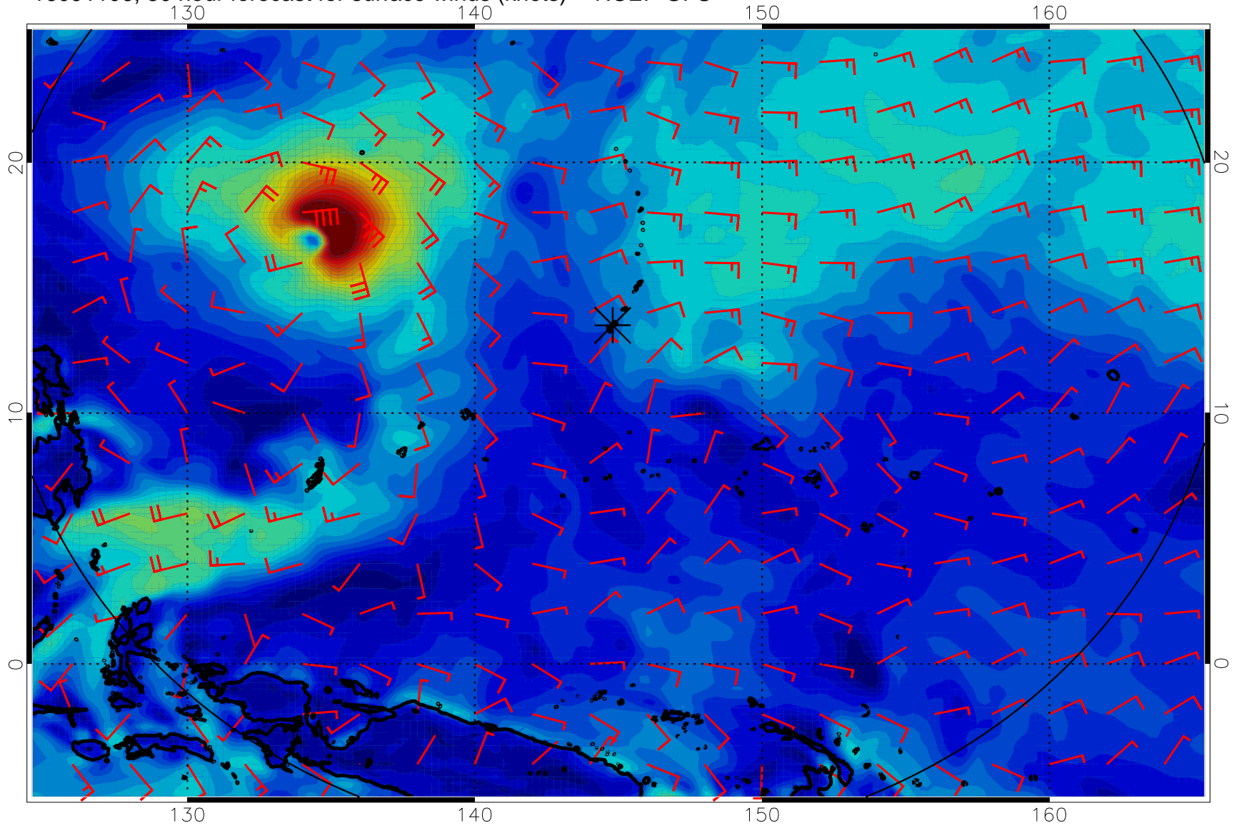
16091106, 30 hour forecast for surface winds (knots) -- NCEP GFS
