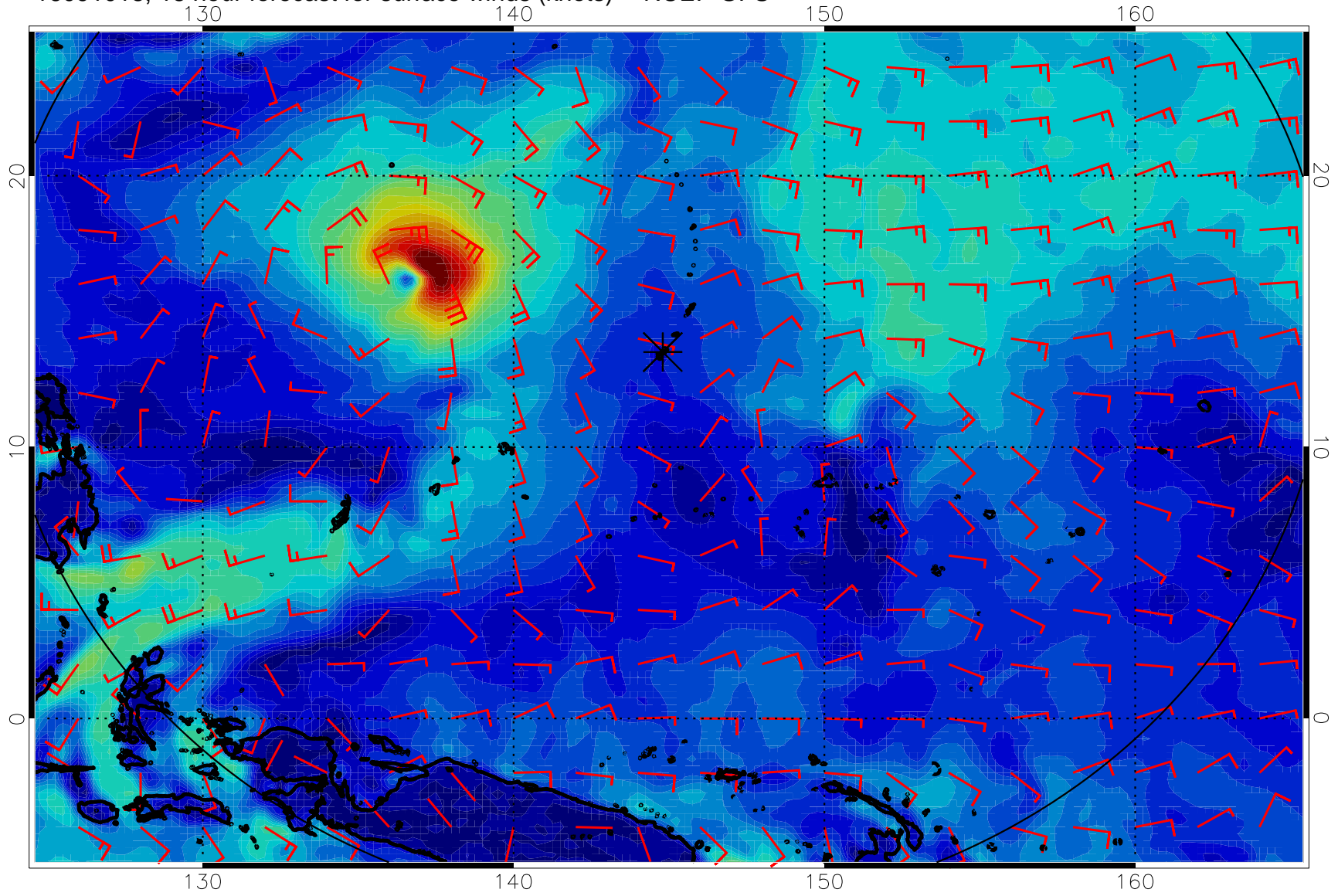
16091018, 18 hour forecast for surface winds (knots) -- NCEP GFS
