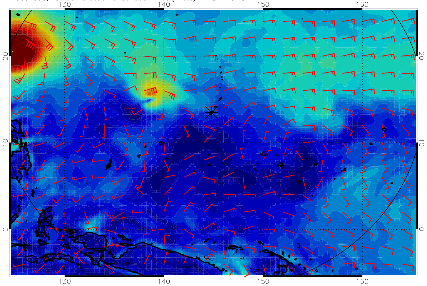
16091306, 78 hour forecast for surface winds (knots) -- NCEP GFS
