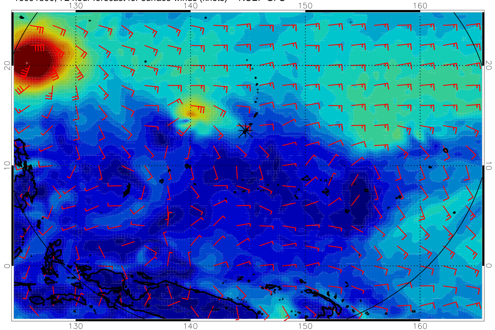
16091300, 72 hour forecast for surface winds (knots) -- NCEP GFS
