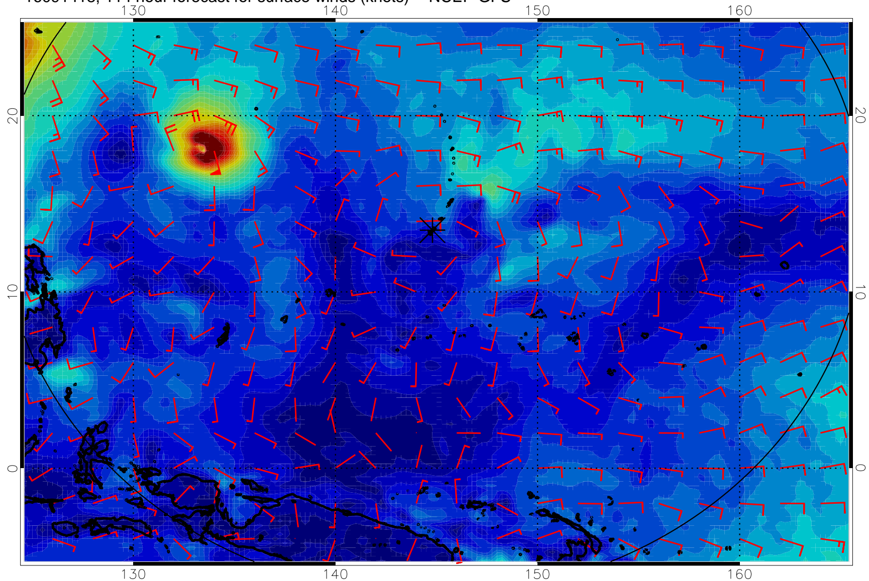
16091418, 114 hour forecast for surface winds (knots) -- NCEP GFS
