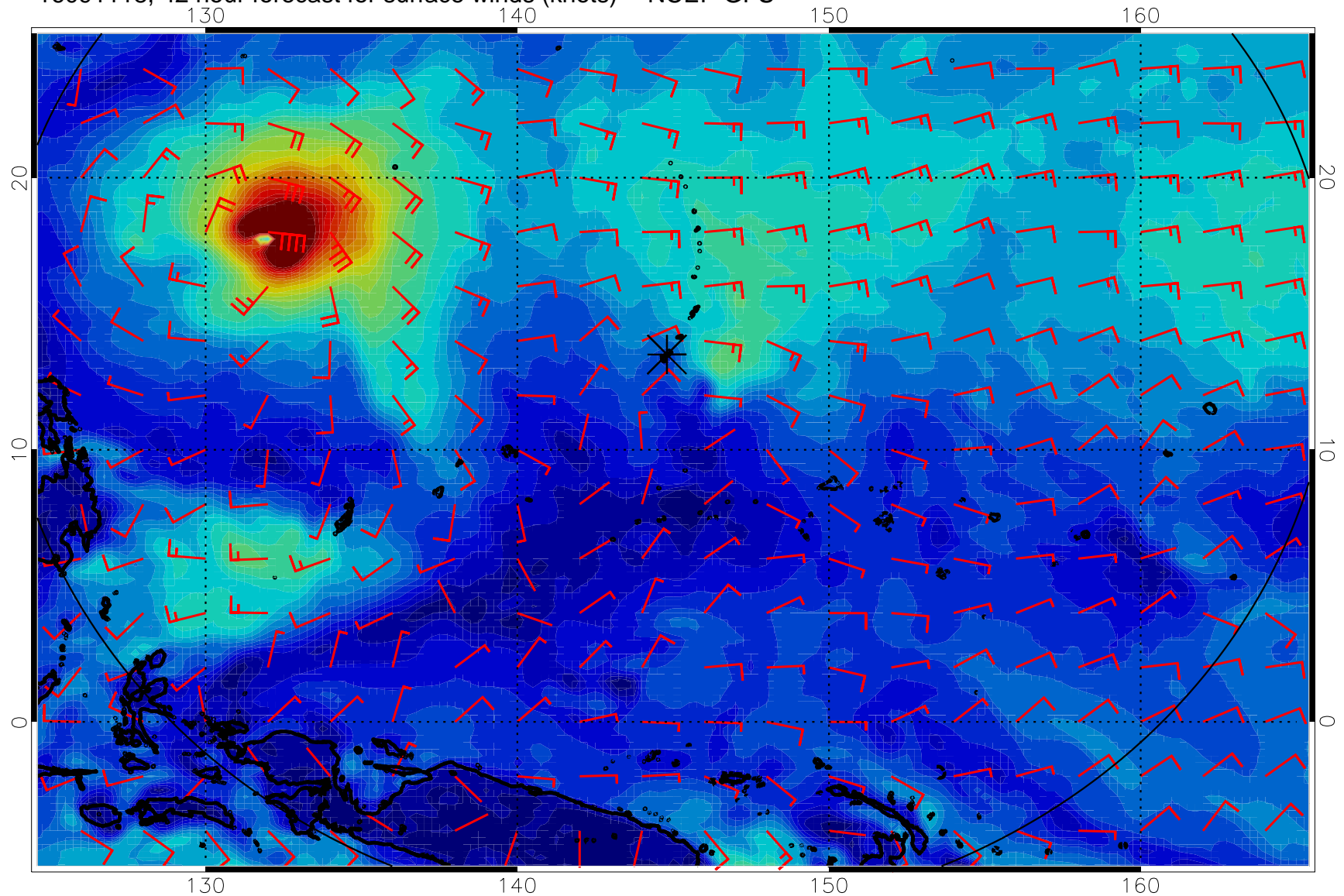
16091118, 42 hour forecast for surface winds (knots) -- NCEP GFS
