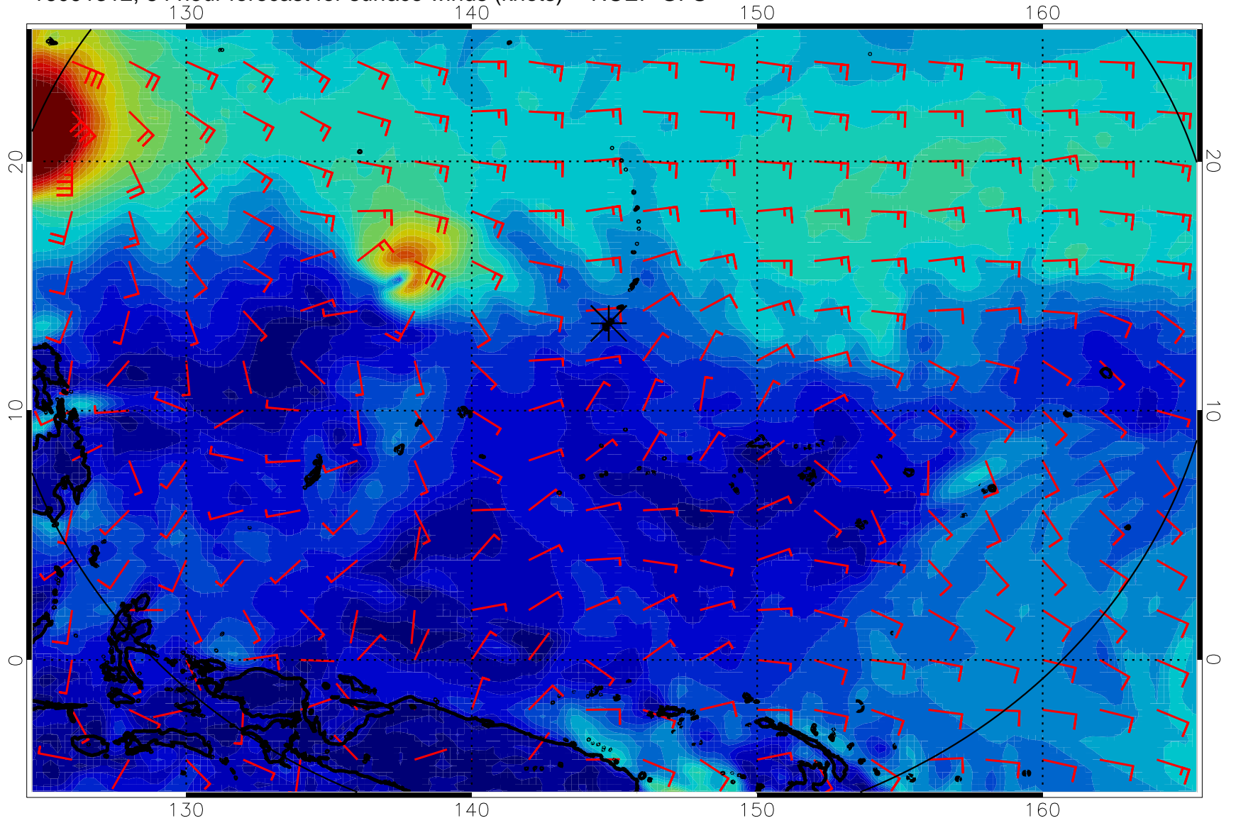
16091312, 84 hour forecast for surface winds (knots) -- NCEP GFS
