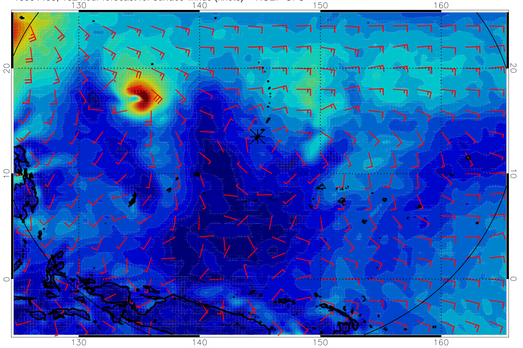
16091406, 102 hour forecast for surface winds (knots) -- NCEP GFS
