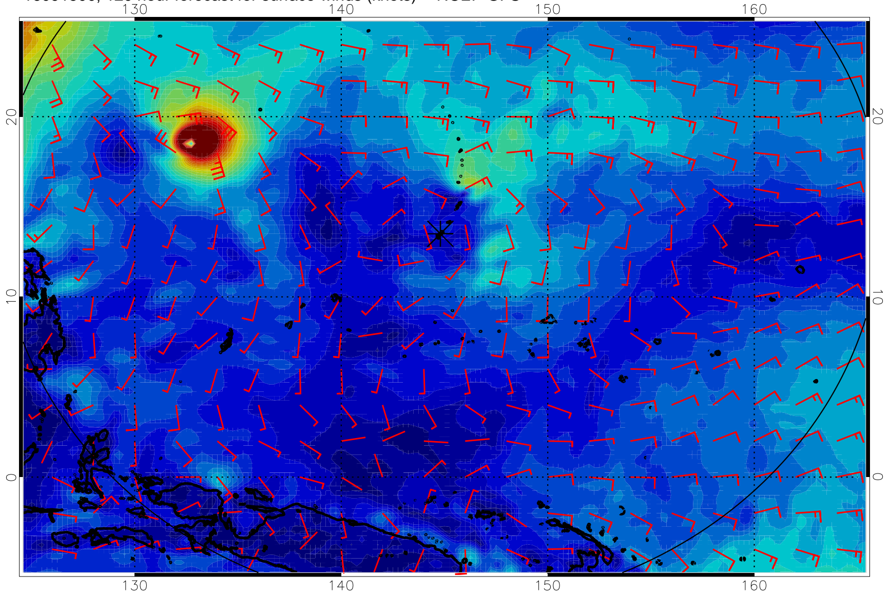
16091500, 120 hour forecast for surface winds (knots) -- NCEP GFS
