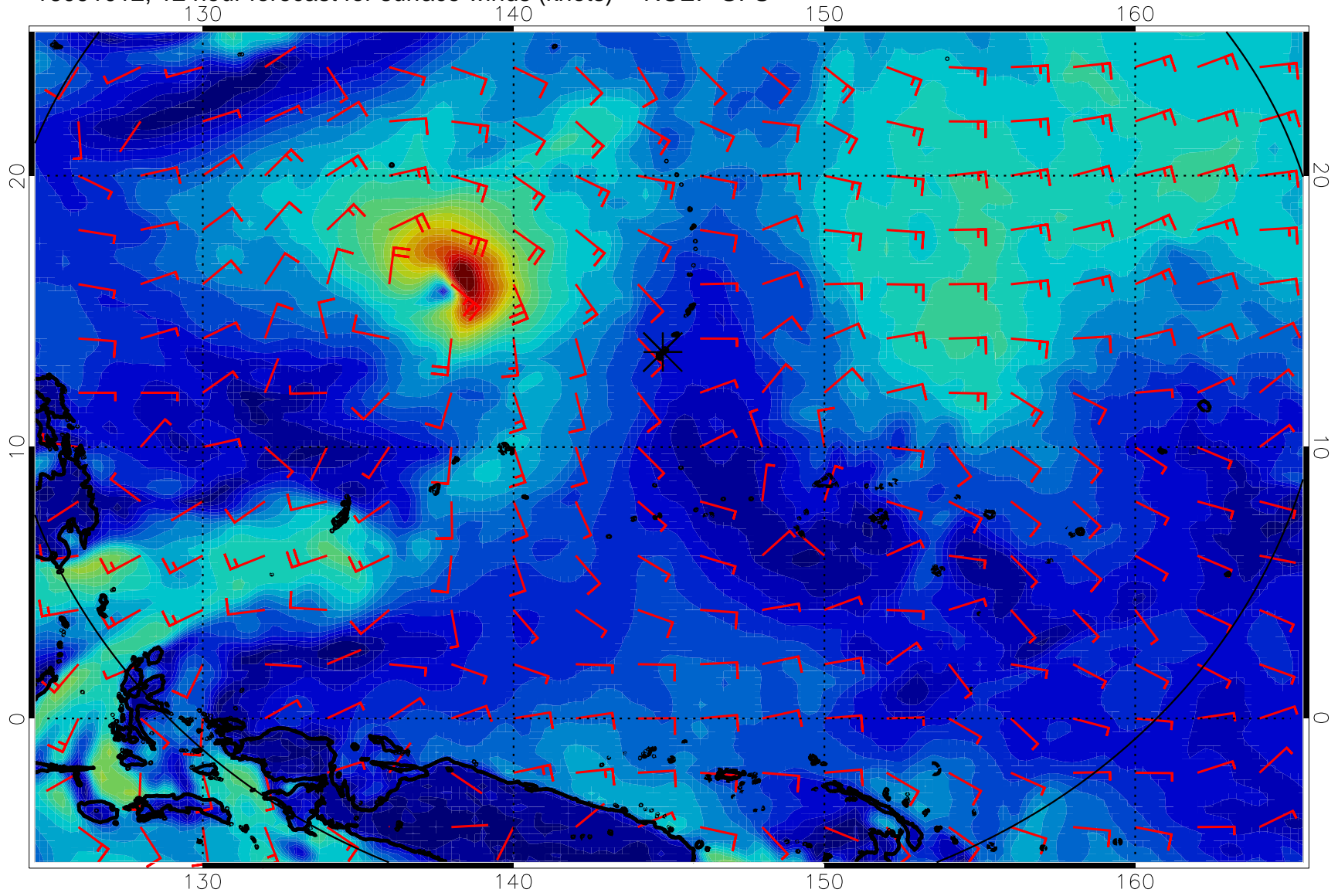
16091012, 12 hour forecast for surface winds (knots) -- NCEP GFS
