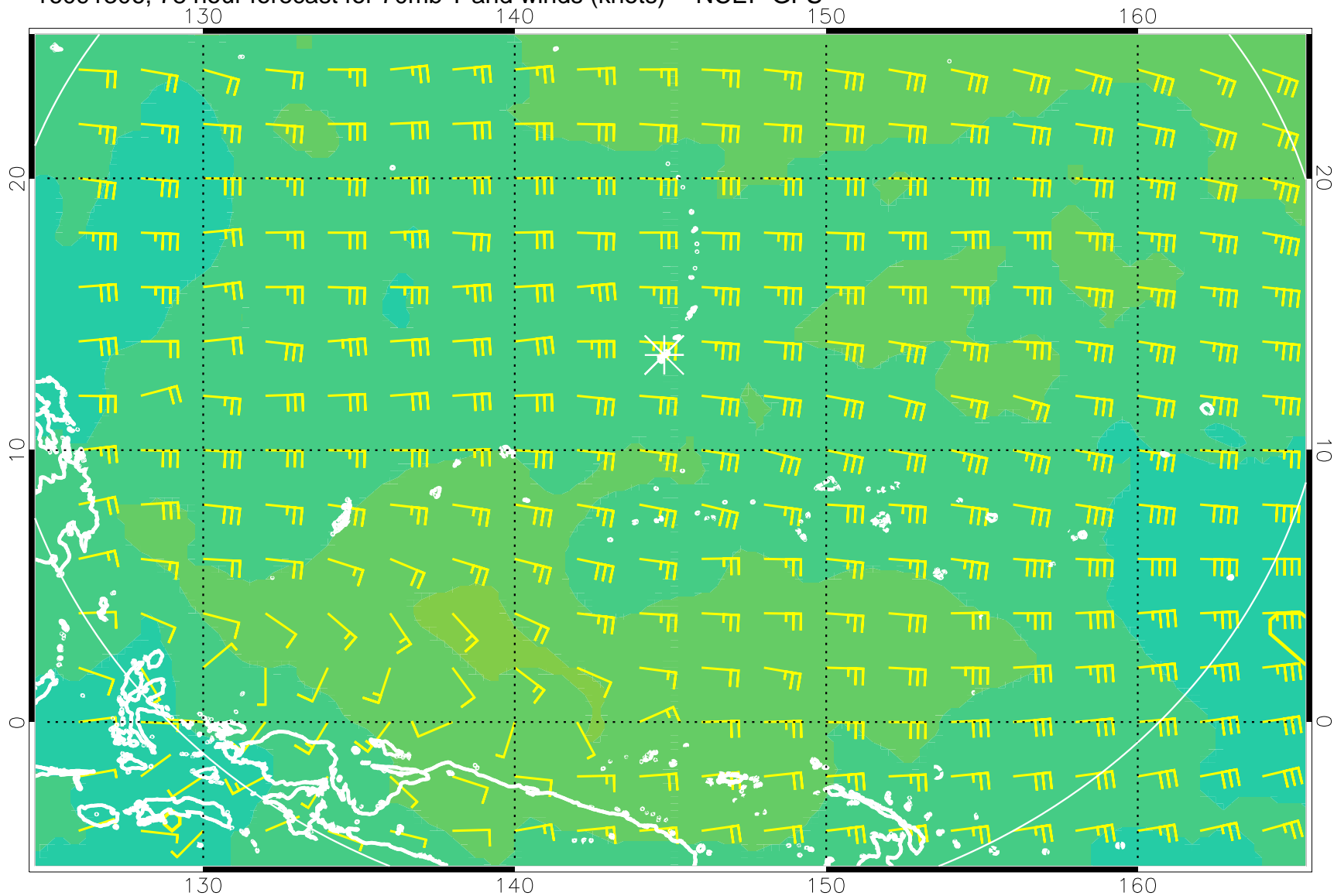
16091306, 78 hour forecast for 70mb T and winds (knots) -- NCEP GFS
