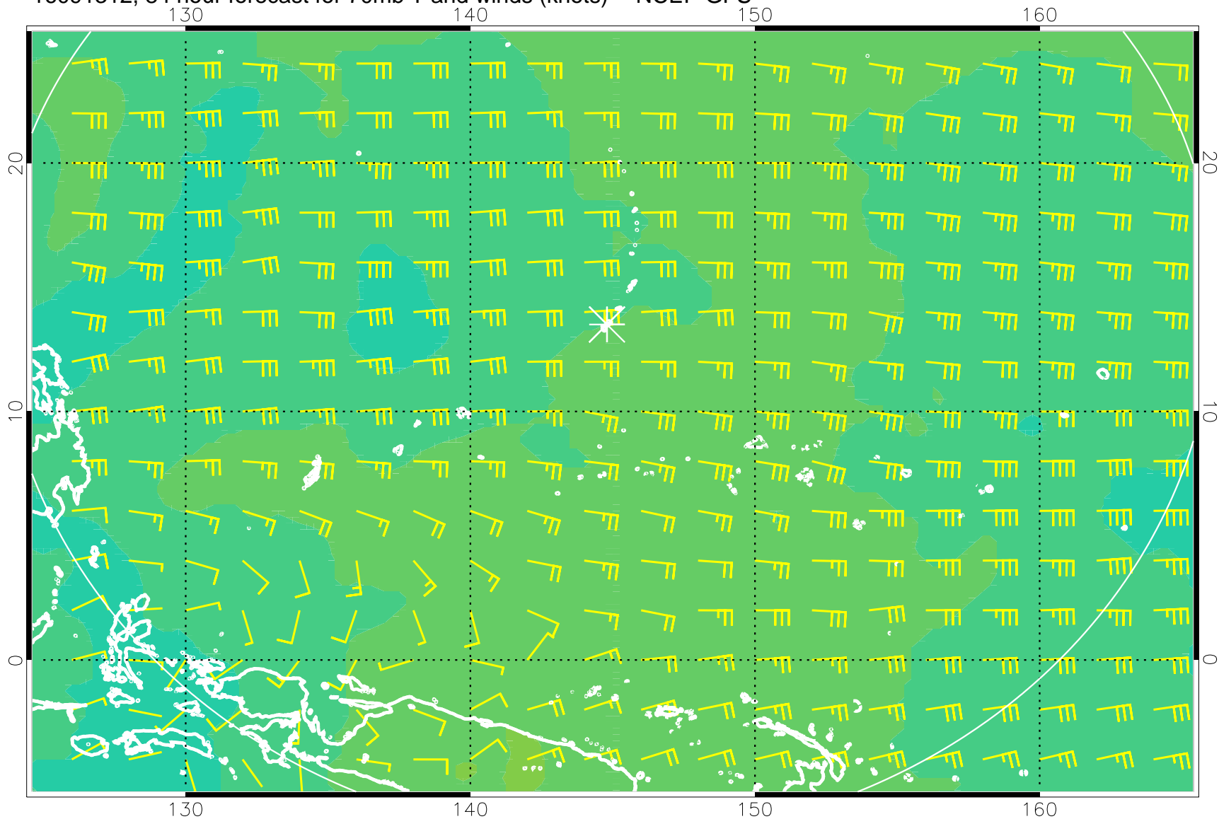
16091312, 84 hour forecast for 70mb T and winds (knots) -- NCEP GFS
