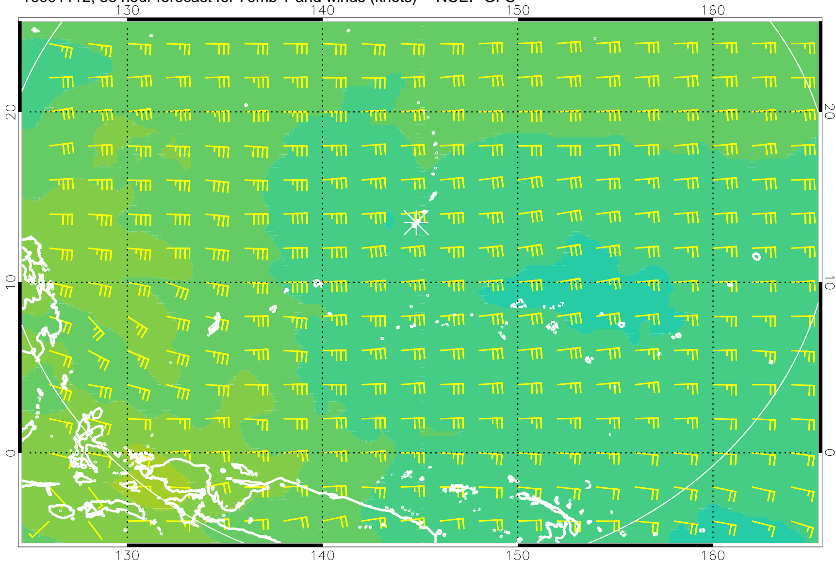
16091112, 36 hour forecast for 70mb T and winds (knots) -- NCEP GFS
