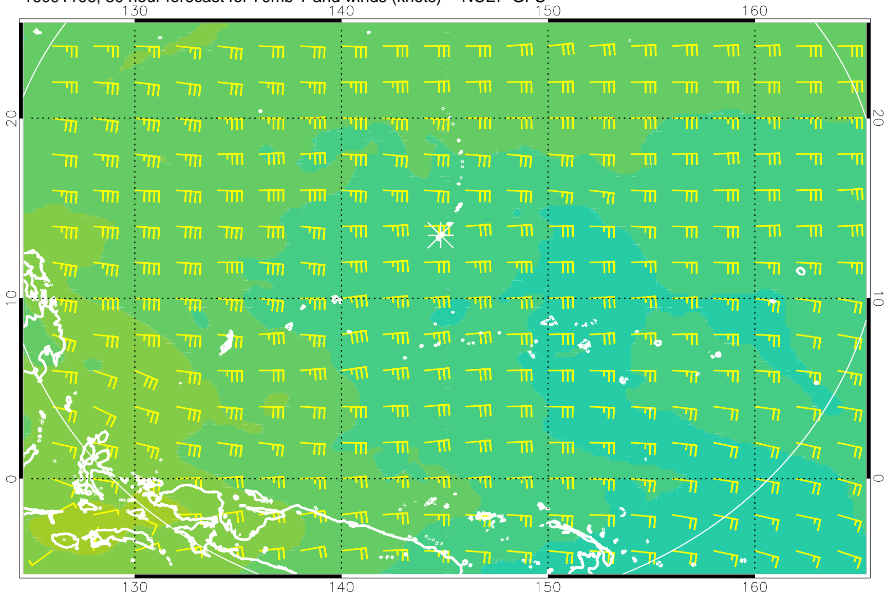
16091106, 30 hour forecast for 70mb T and winds (knots) -- NCEP GFS
