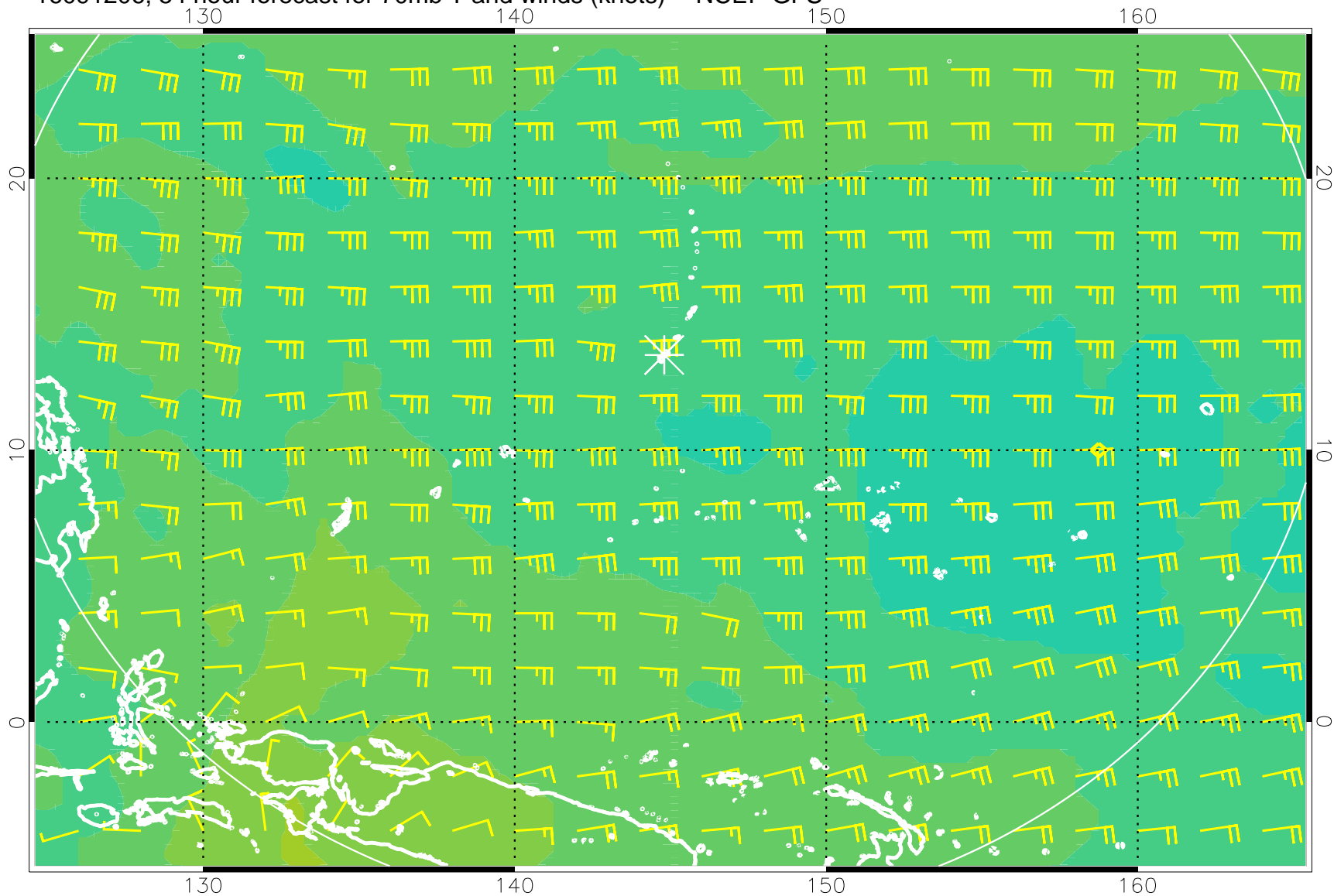
16091206, 54 hour forecast for 70mb T and winds (knots) -- NCEP GFS
