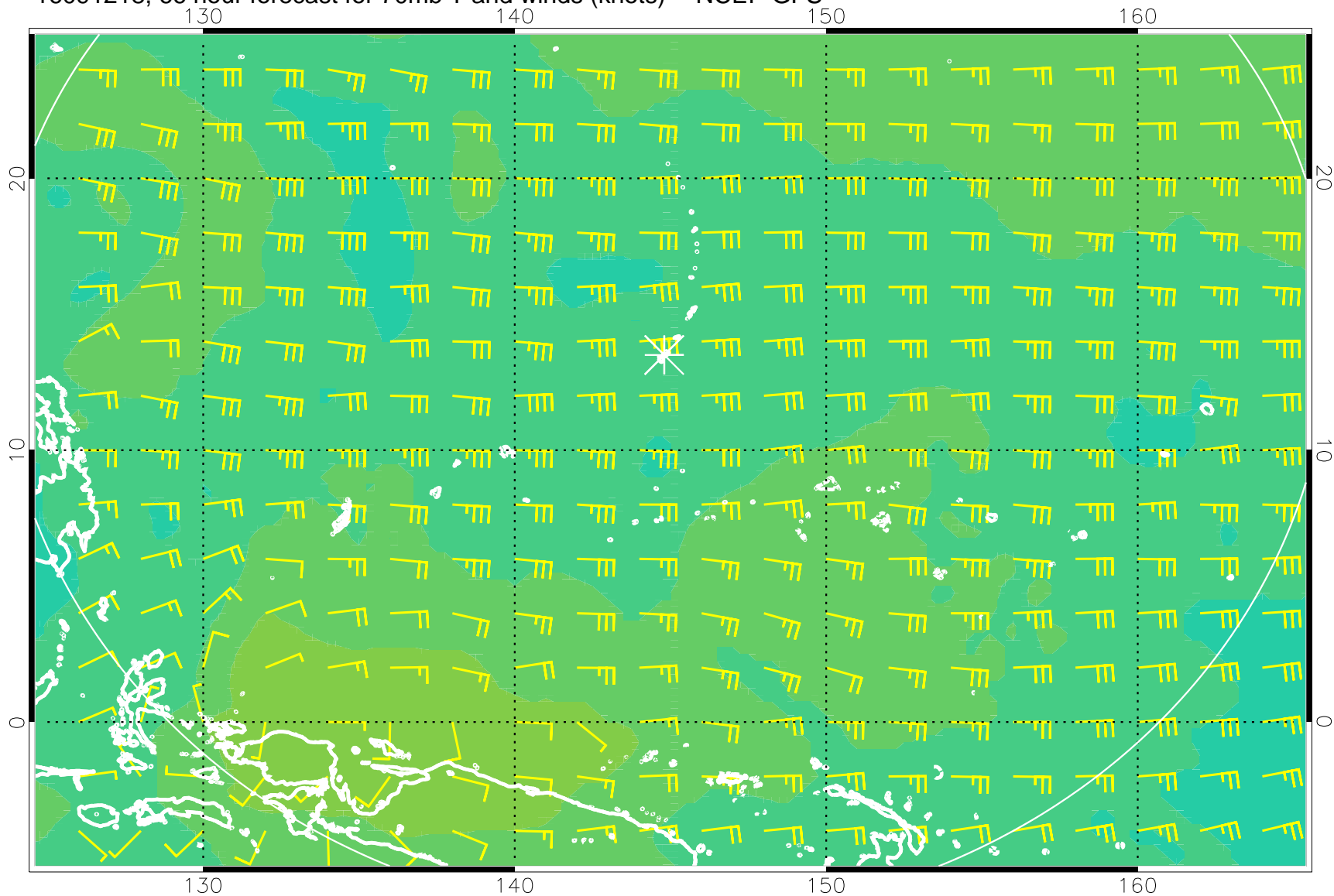
16091218, 66 hour forecast for 70mb T and winds (knots) -- NCEP GFS
