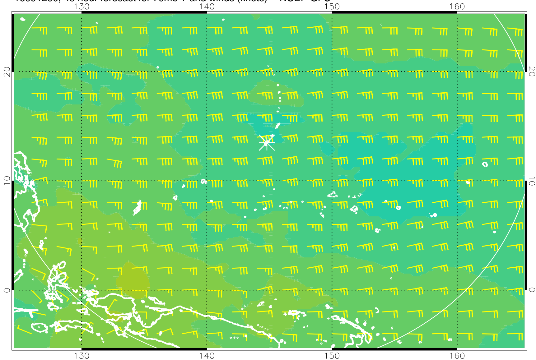
16091200, 48 hour forecast for 70mb T and winds (knots) -- NCEP GFS
