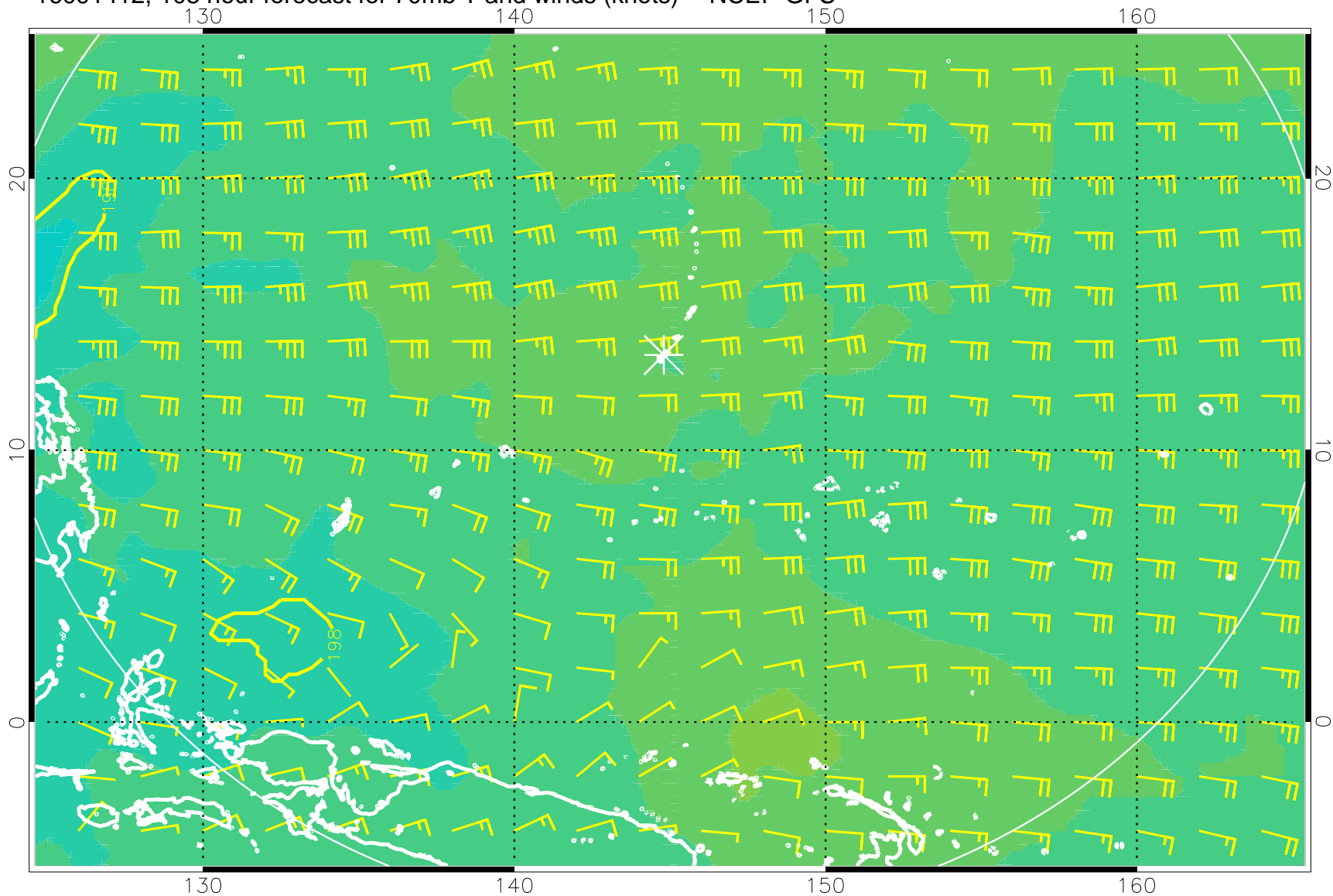
16091412, 108 hour forecast for 70mb T and winds (knots) -- NCEP GFS
