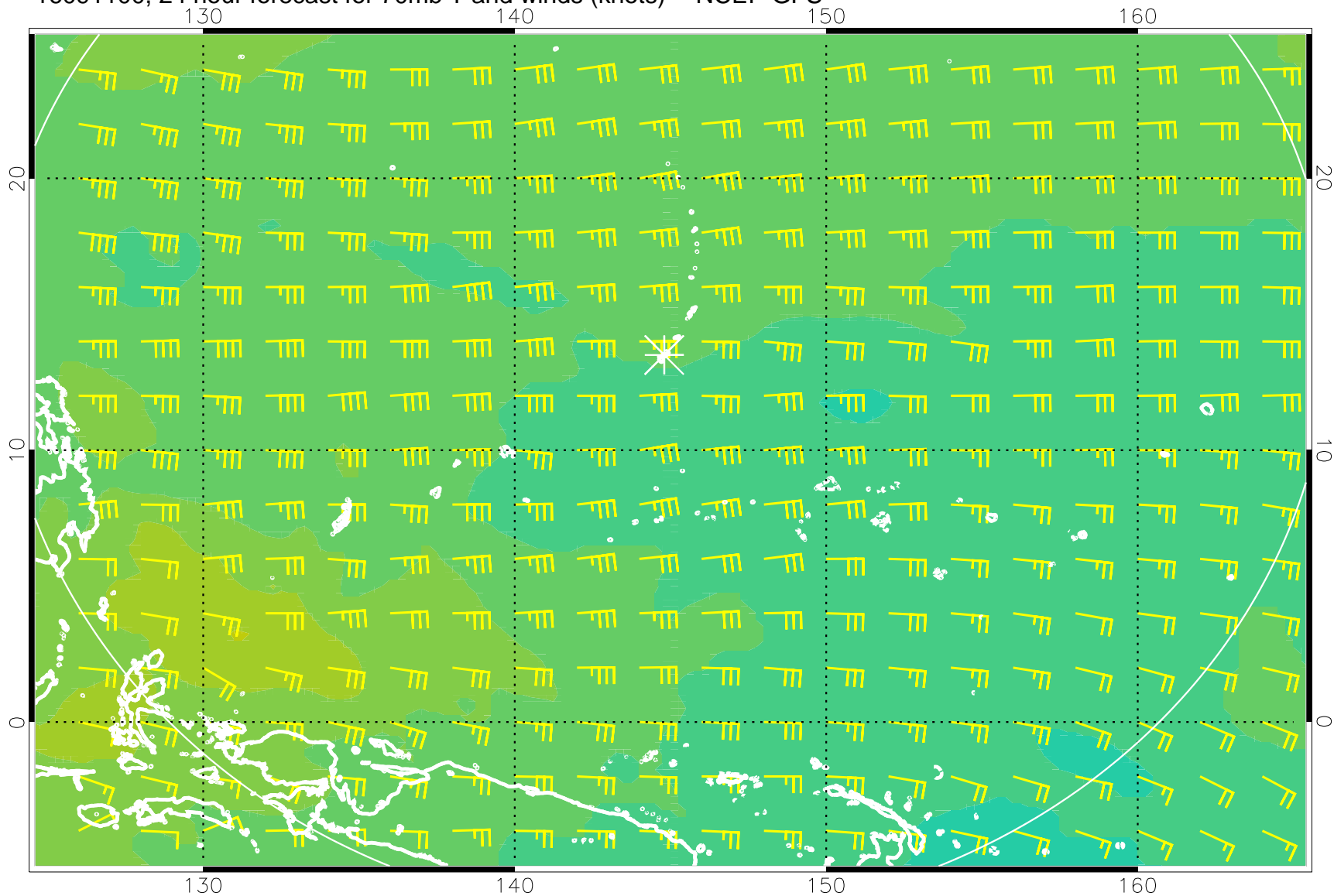
16091100, 24 hour forecast for 70mb T and winds (knots) -- NCEP GFS
