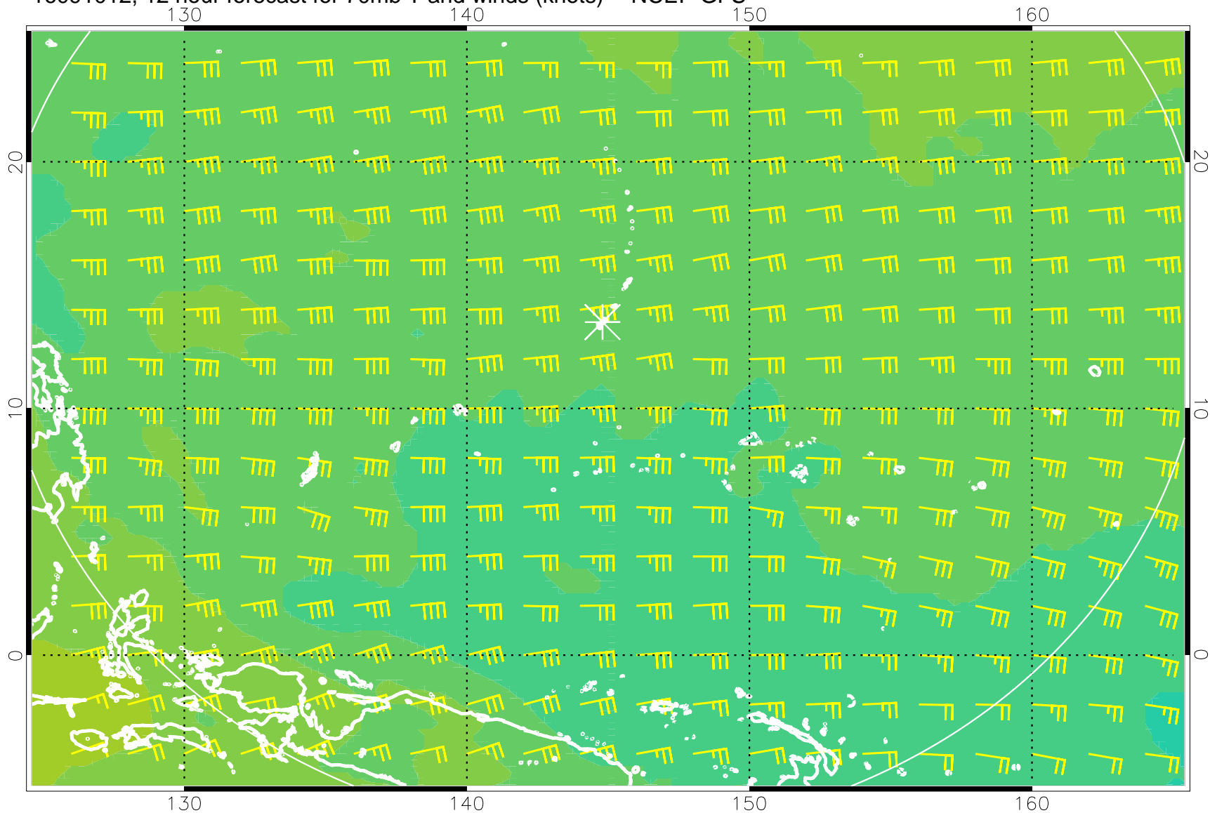
16091012, 12 hour forecast for 70mb T and winds (knots) -- NCEP GFS
