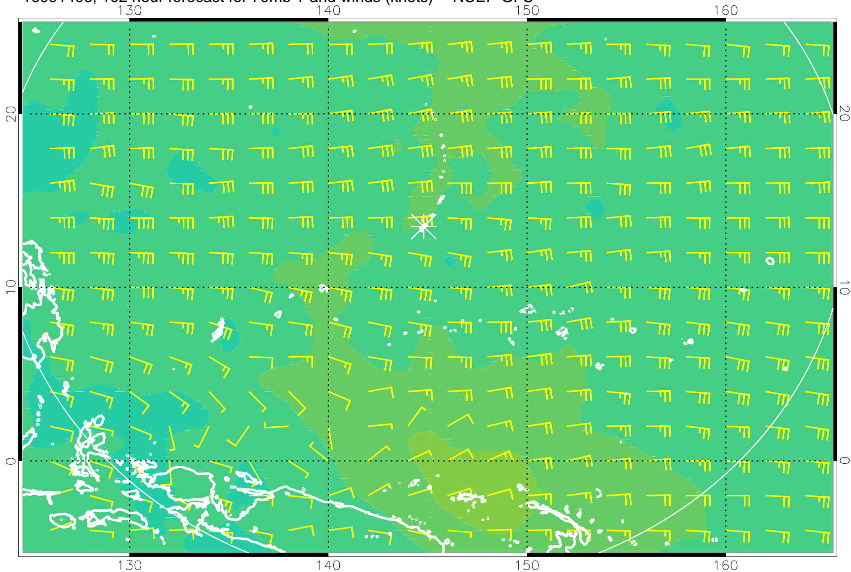
16091406, 102 hour forecast for 70mb T and winds (knots) -- NCEP GFS
