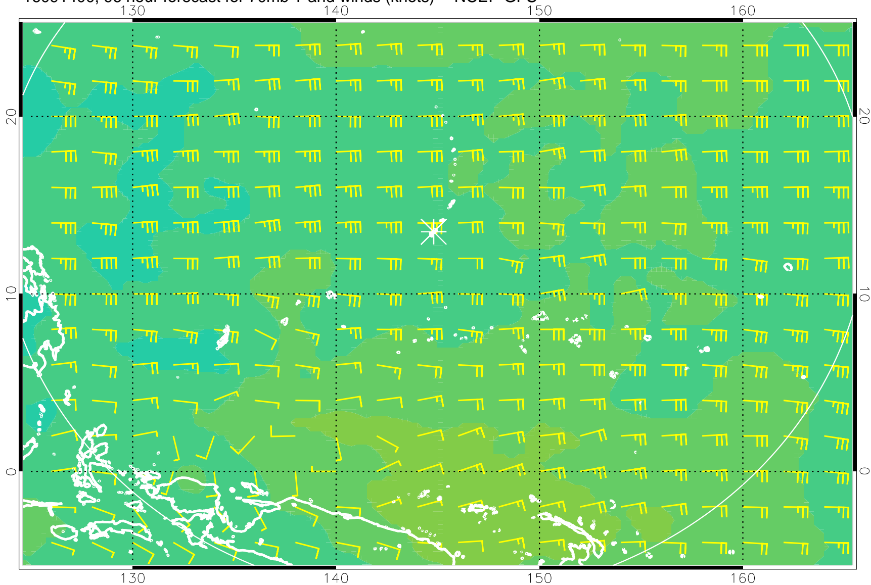
16091400, 96 hour forecast for 70mb T and winds (knots) -- NCEP GFS
