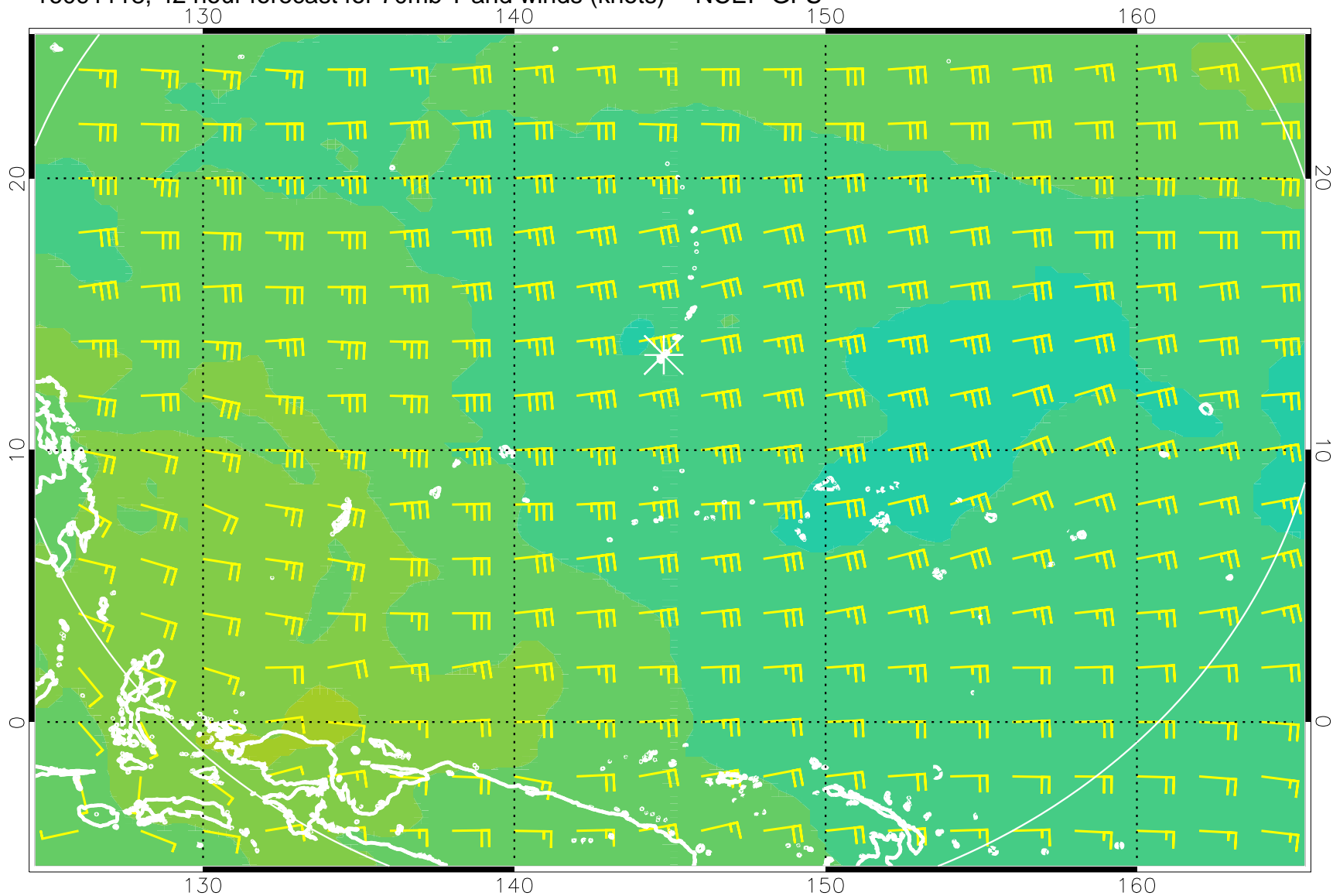
16091118, 42 hour forecast for 70mb T and winds (knots) -- NCEP GFS
