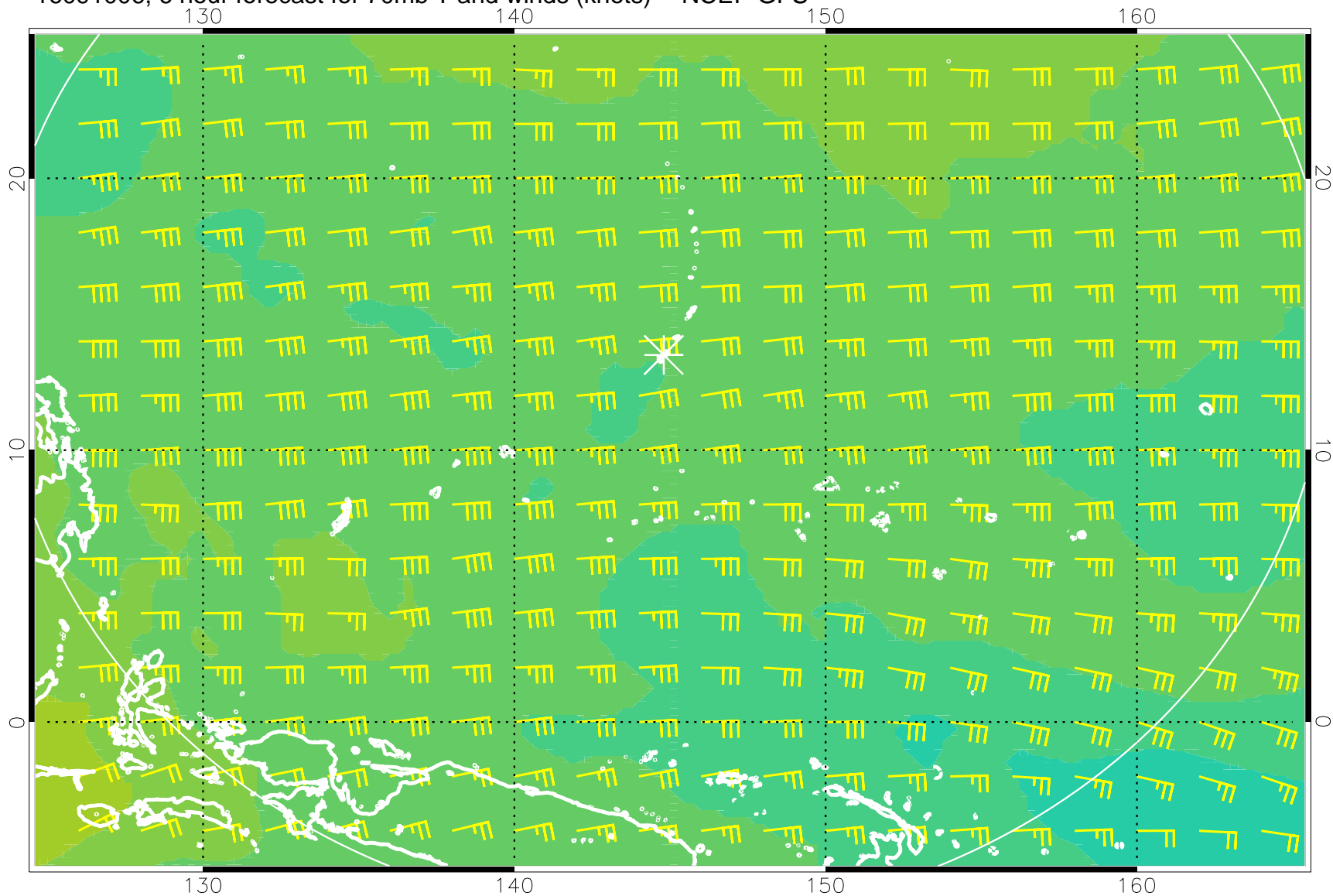
16091006, 6 hour forecast for 70mb T and winds (knots) -- NCEP GFS
