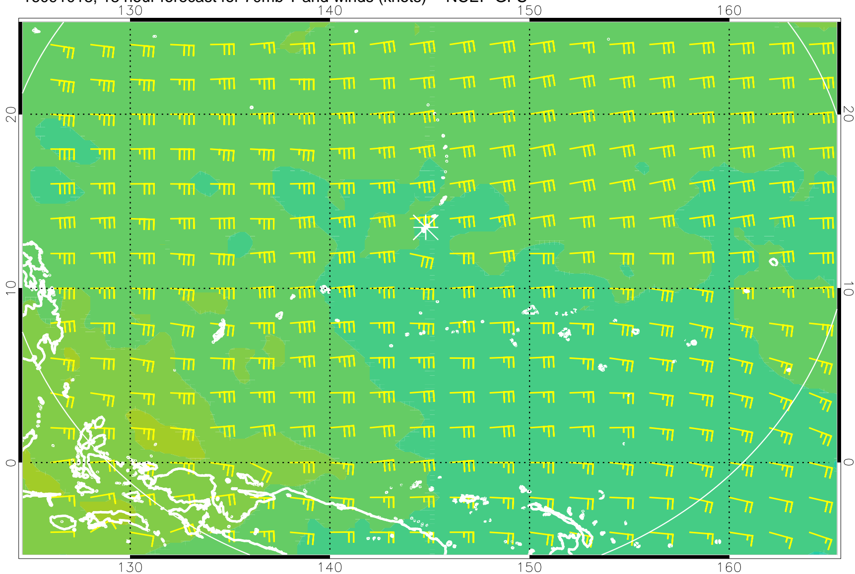
16091018, 18 hour forecast for 70mb T and winds (knots) -- NCEP GFS
