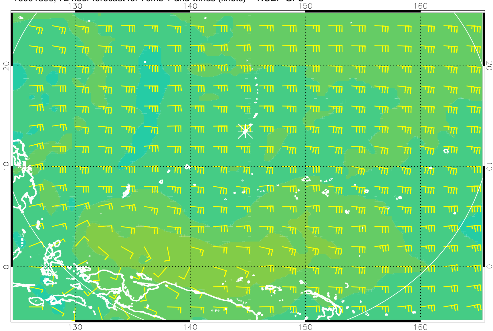
16091300, 72 hour forecast for 70mb T and winds (knots) -- NCEP GFS
