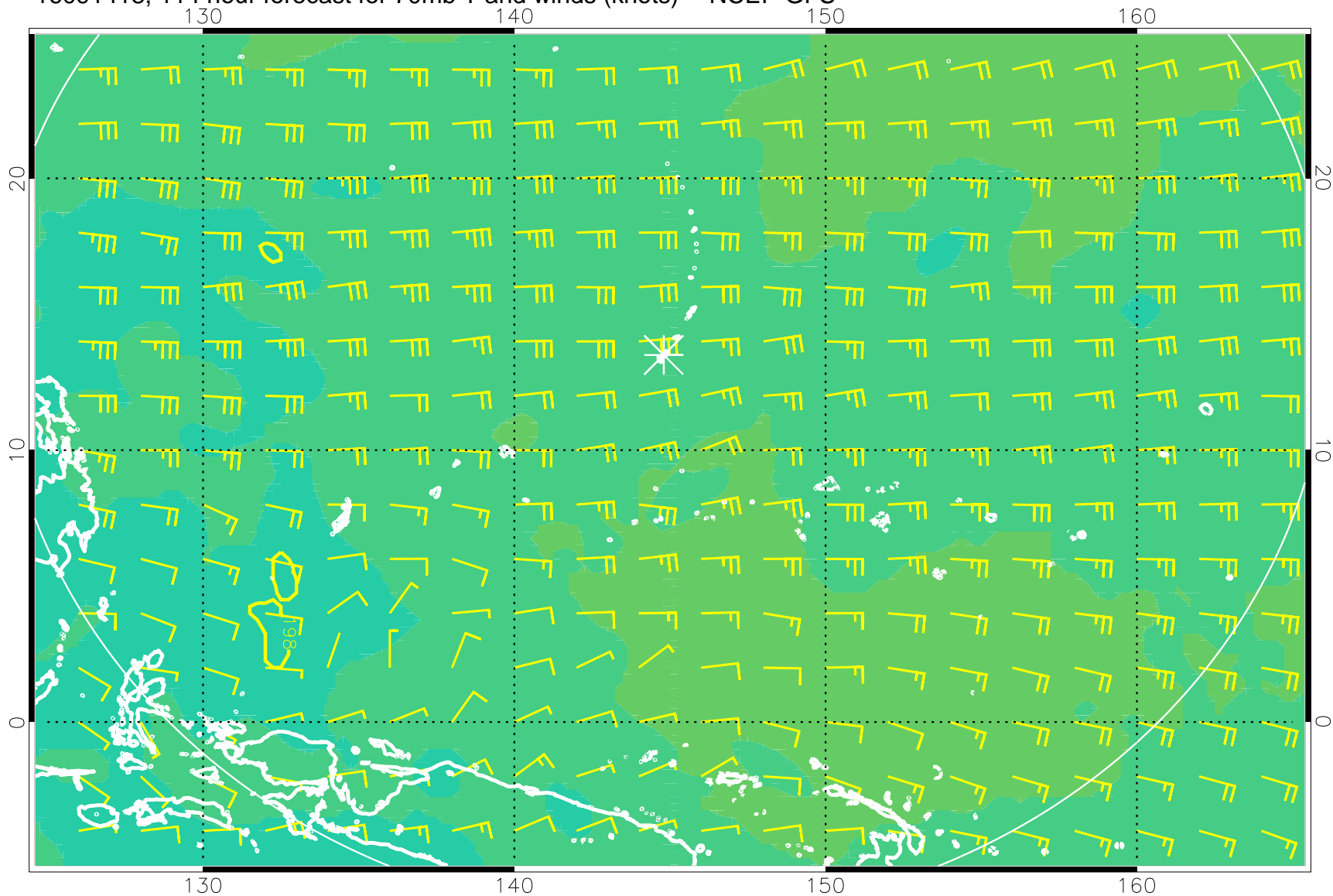
16091418, 114 hour forecast for 70mb T and winds (knots) -- NCEP GFS
