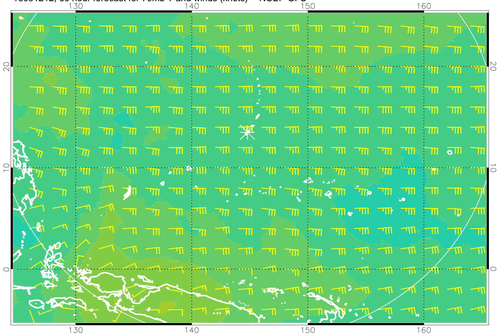
16091212, 60 hour forecast for 70mb T and winds (knots) -- NCEP GFS
