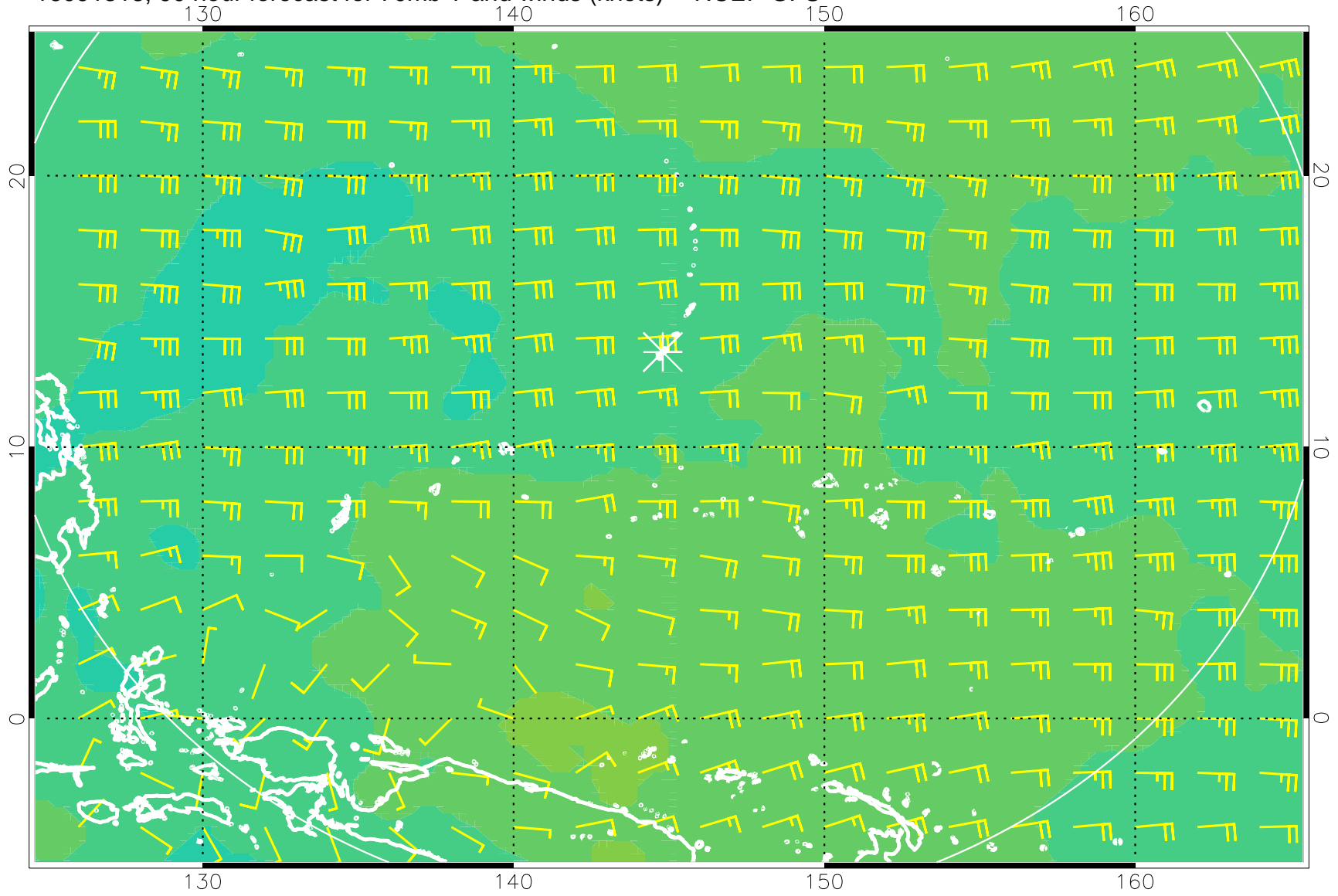
16091318, 90 hour forecast for 70mb T and winds (knots) -- NCEP GFS
