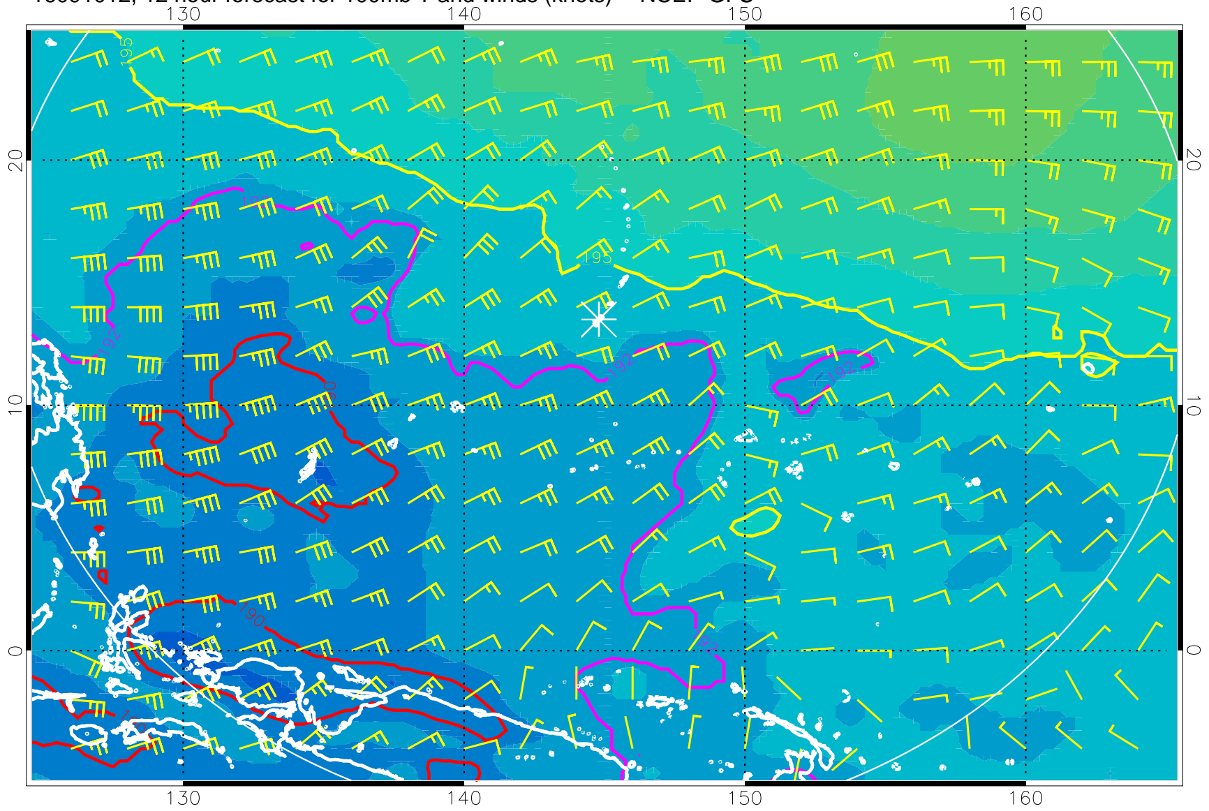
16091012, 12 hour forecast for 100mb T and winds (knots) -- NCEP GFS
