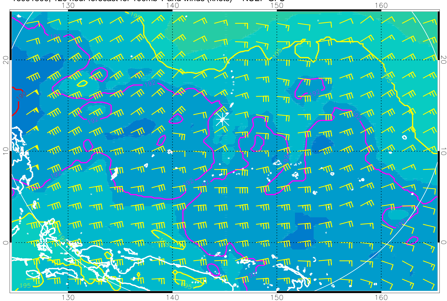
16091500, 120 hour forecast for 100mb T and winds (knots) -- NCEP GFS
