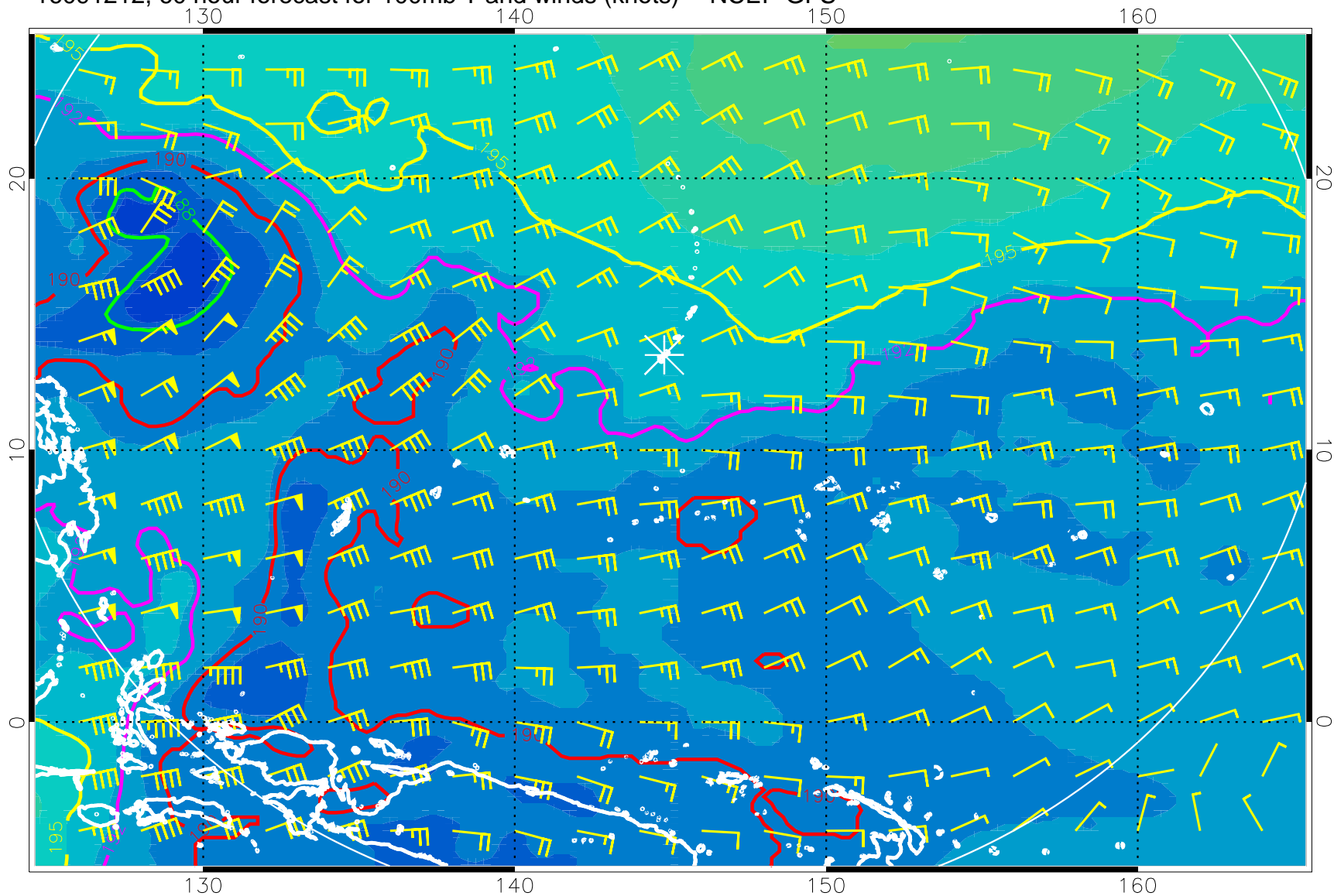
16091212, 60 hour forecast for 100mb T and winds (knots) -- NCEP GFS
