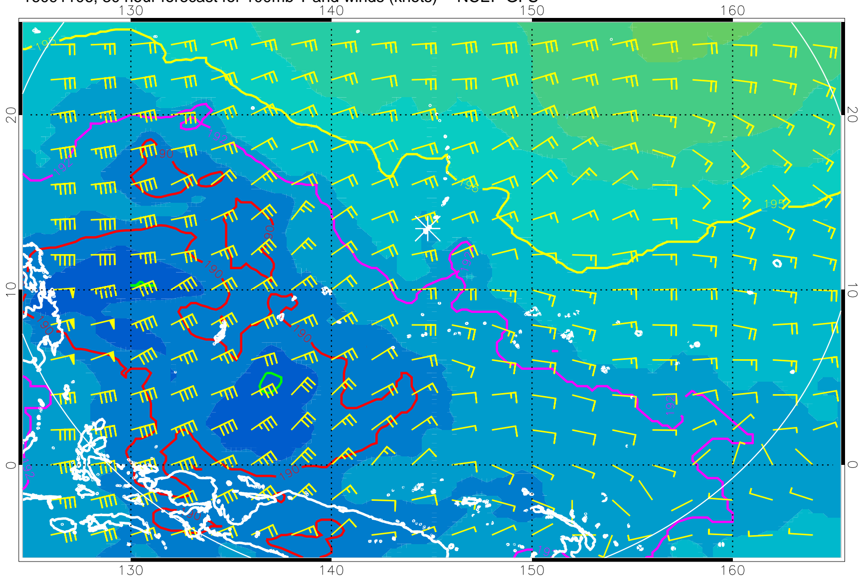
16091106, 30 hour forecast for 100mb T and winds (knots) -- NCEP GFS
