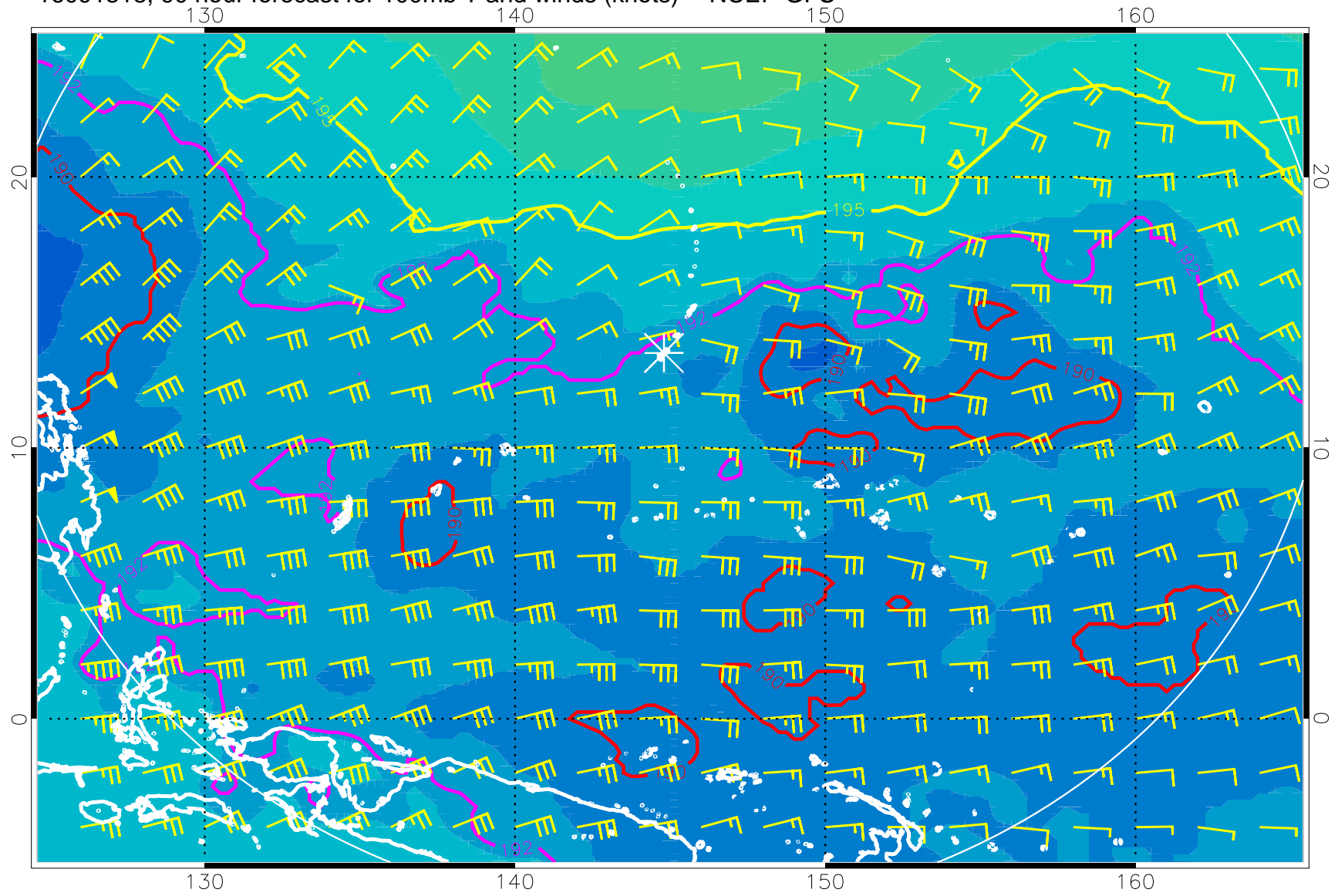
16091318, 90 hour forecast for 100mb T and winds (knots) -- NCEP GFS
