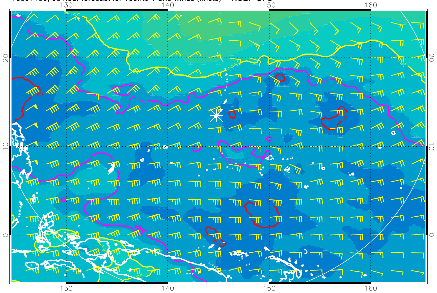
16091400, 96 hour forecast for 100mb T and winds (knots) -- NCEP GFS
