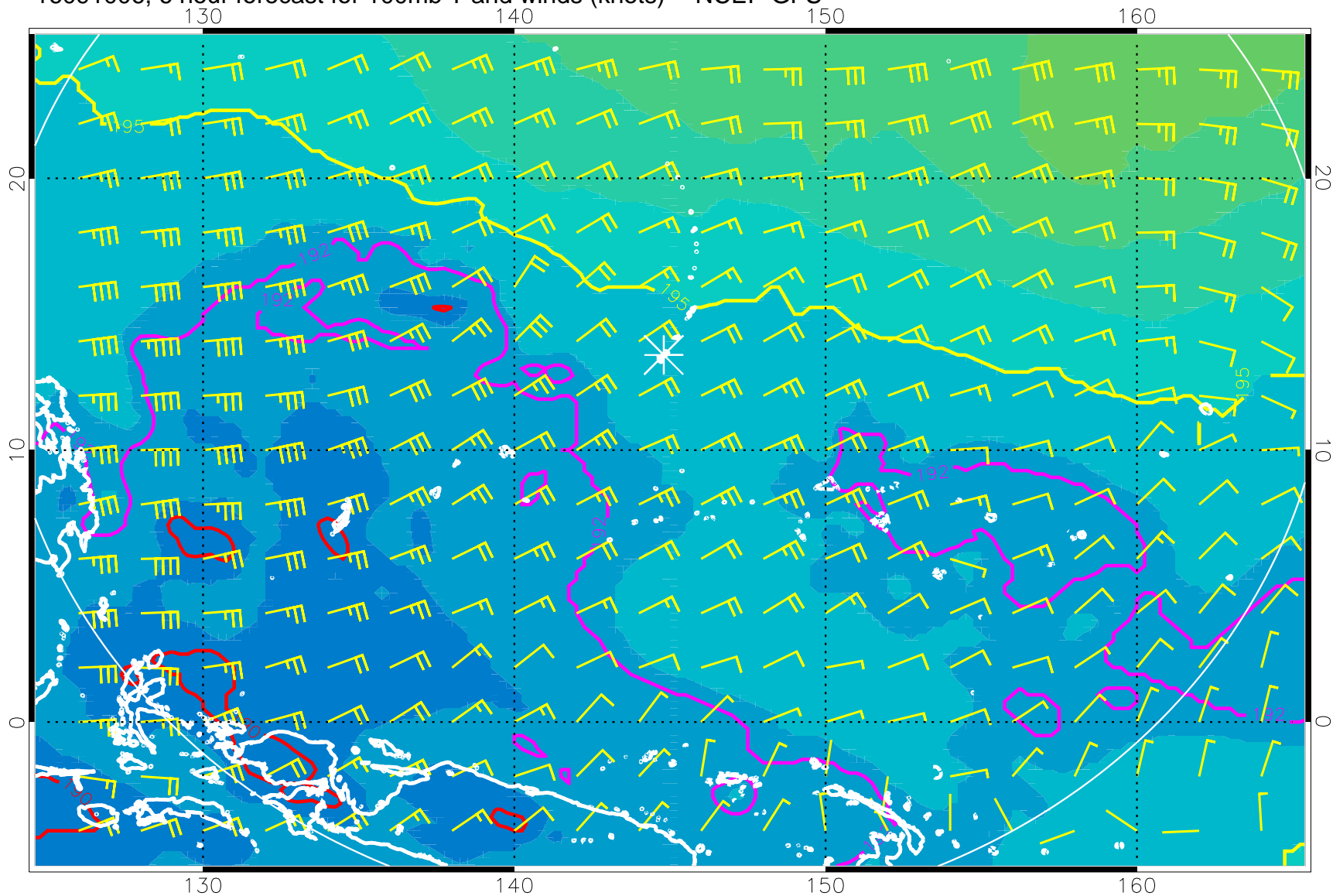
16091006, 6 hour forecast for 100mb T and winds (knots) -- NCEP GFS
