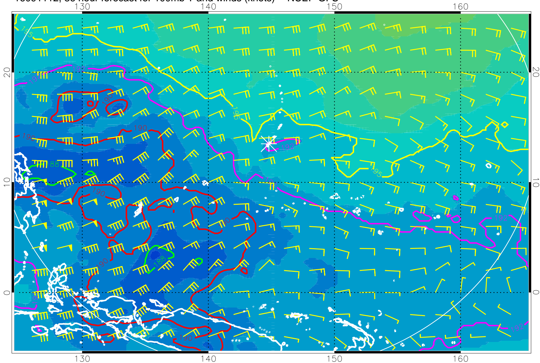
16091112, 36 hour forecast for 100mb T and winds (knots) -- NCEP GFS
