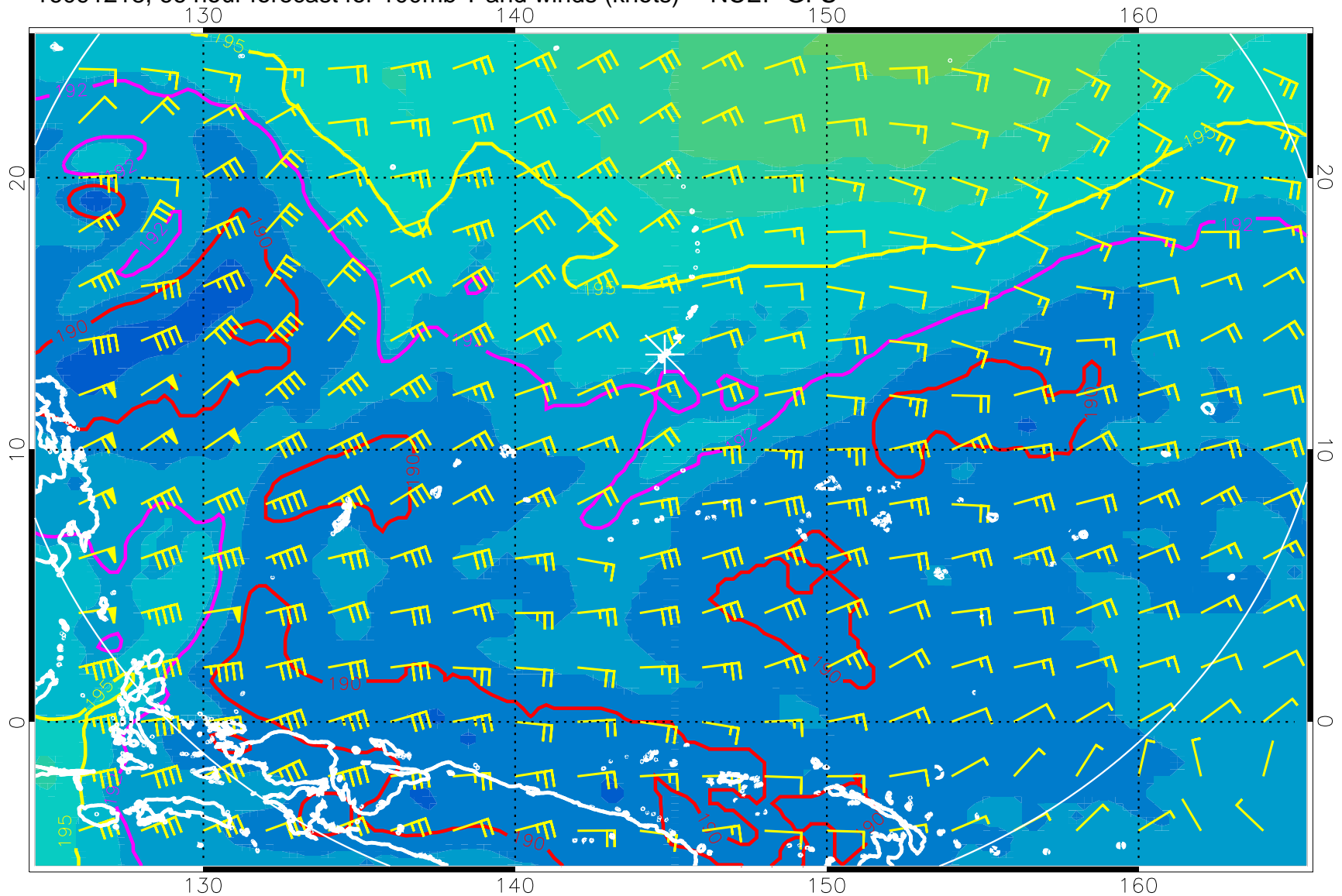
16091218, 66 hour forecast for 100mb T and winds (knots) -- NCEP GFS
