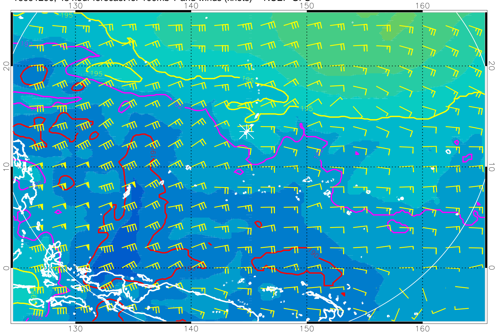
16091200, 48 hour forecast for 100mb T and winds (knots) -- NCEP GFS
