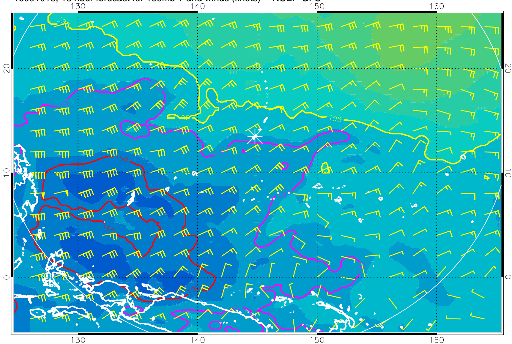
16091018, 18 hour forecast for 100mb T and winds (knots) -- NCEP GFS
