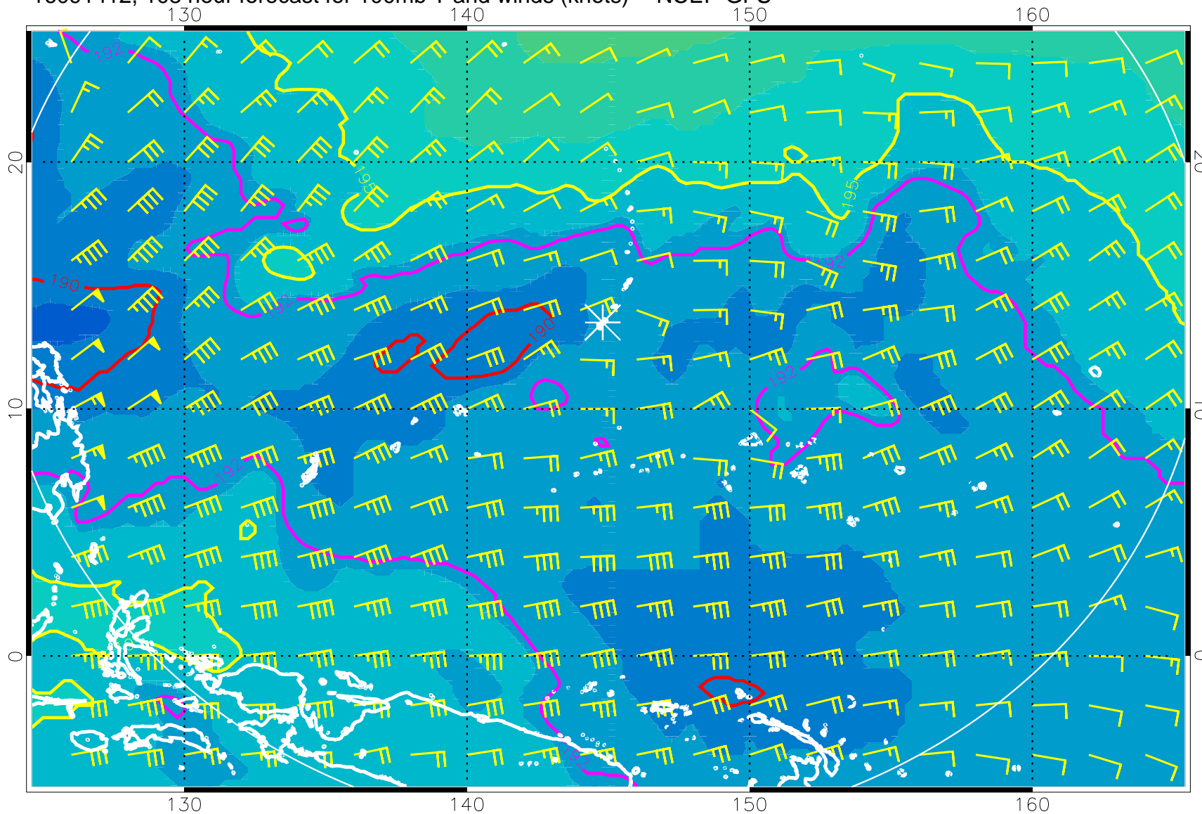
16091412, 108 hour forecast for 100mb T and winds (knots) -- NCEP GFS
