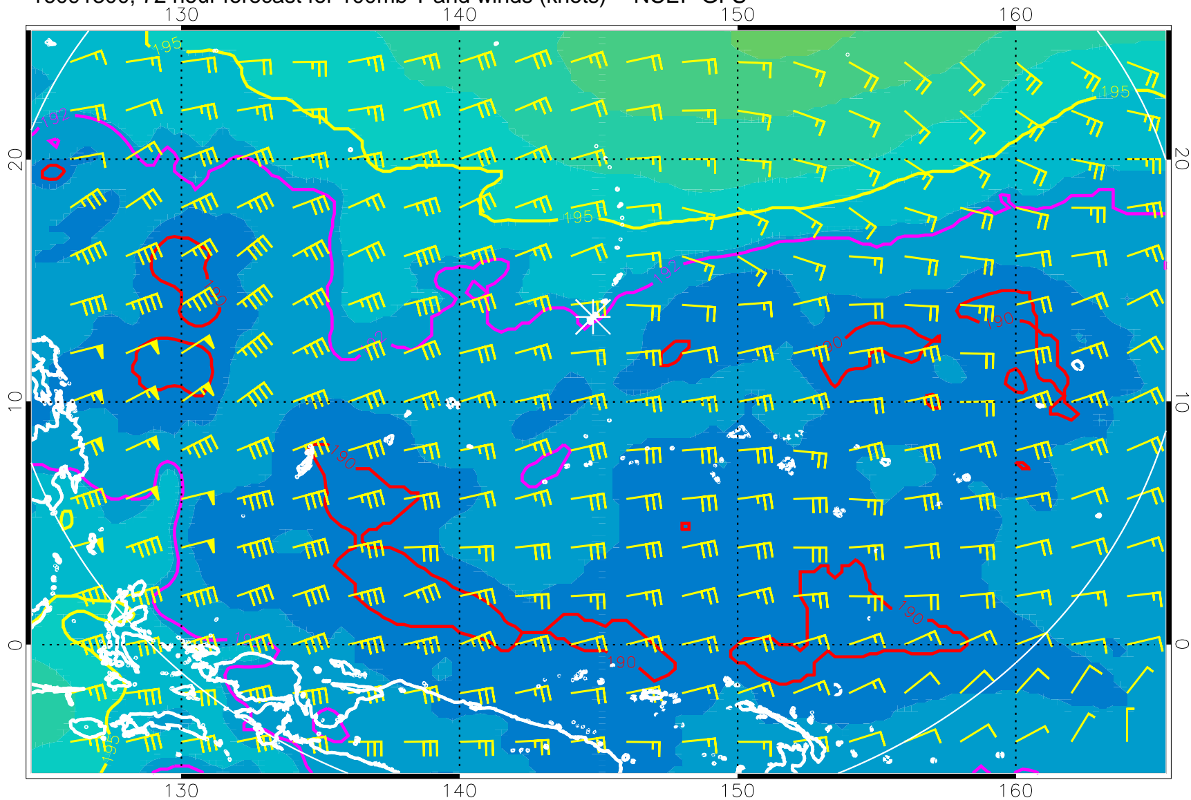
16091300, 72 hour forecast for 100mb T and winds (knots) -- NCEP GFS
