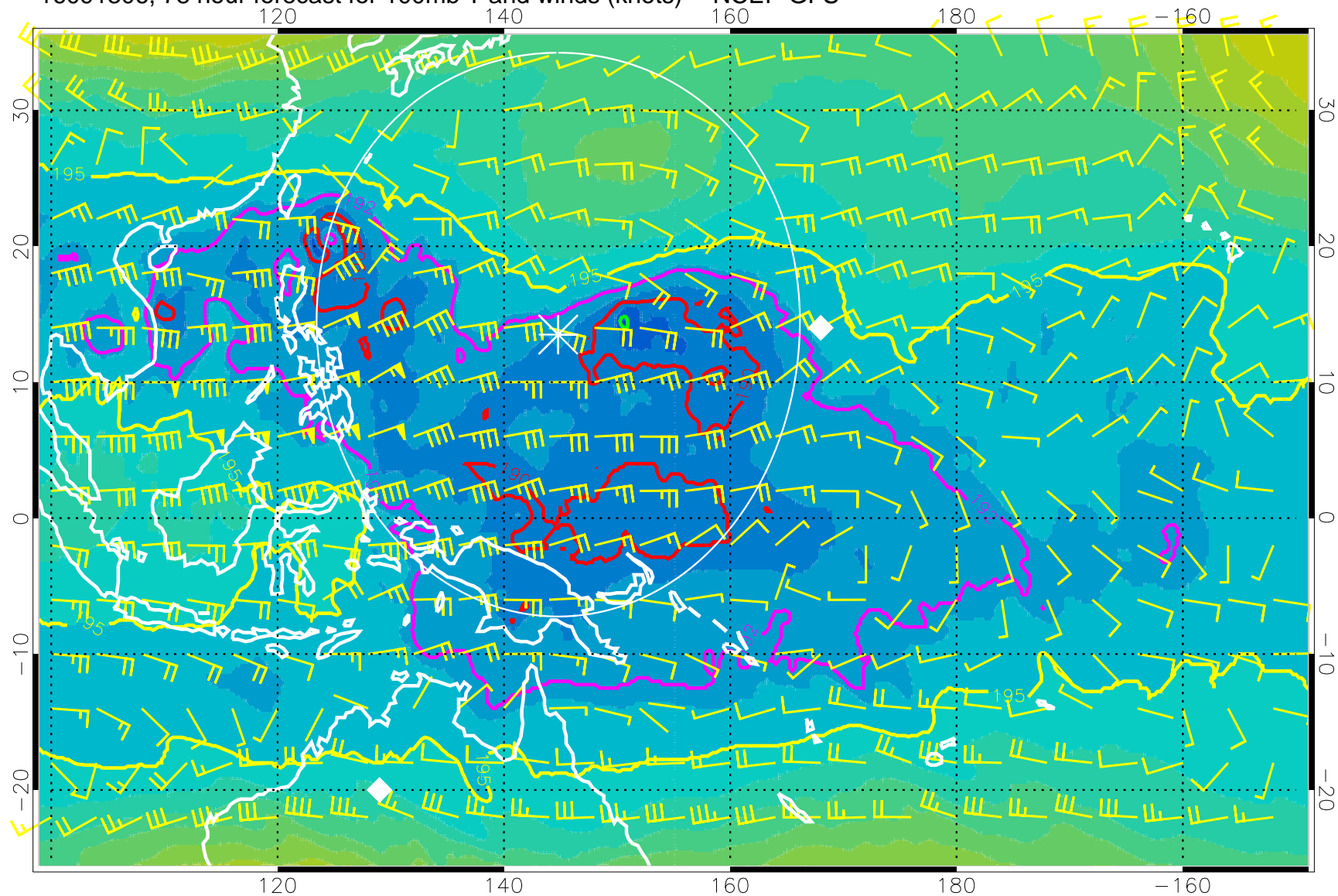
16091306, 78 hour forecast for 100mb T and winds (knots) -- NCEP GFS
