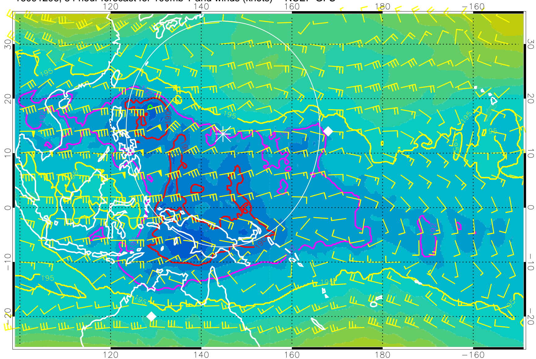
16091206, 54 hour forecast for 100mb T and winds (knots) -- NCEP GFS
