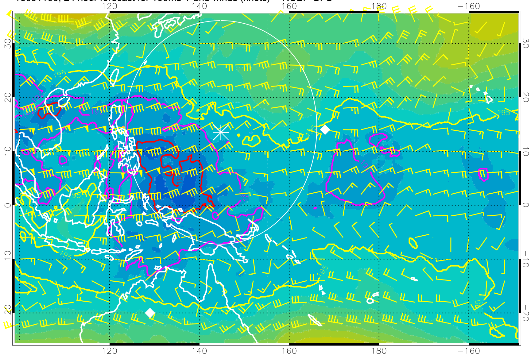
16091100, 24 hour forecast for 100mb T and winds (knots) -- NCEP GFS
