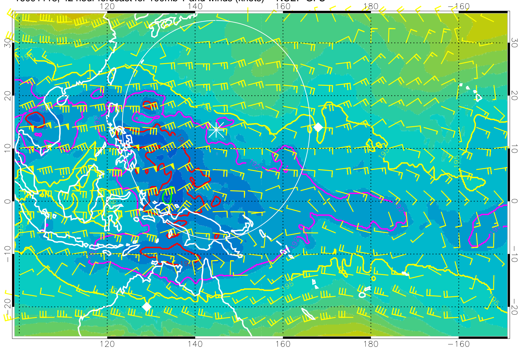
16091118, 42 hour forecast for 100mb T and winds (knots) -- NCEP GFS
