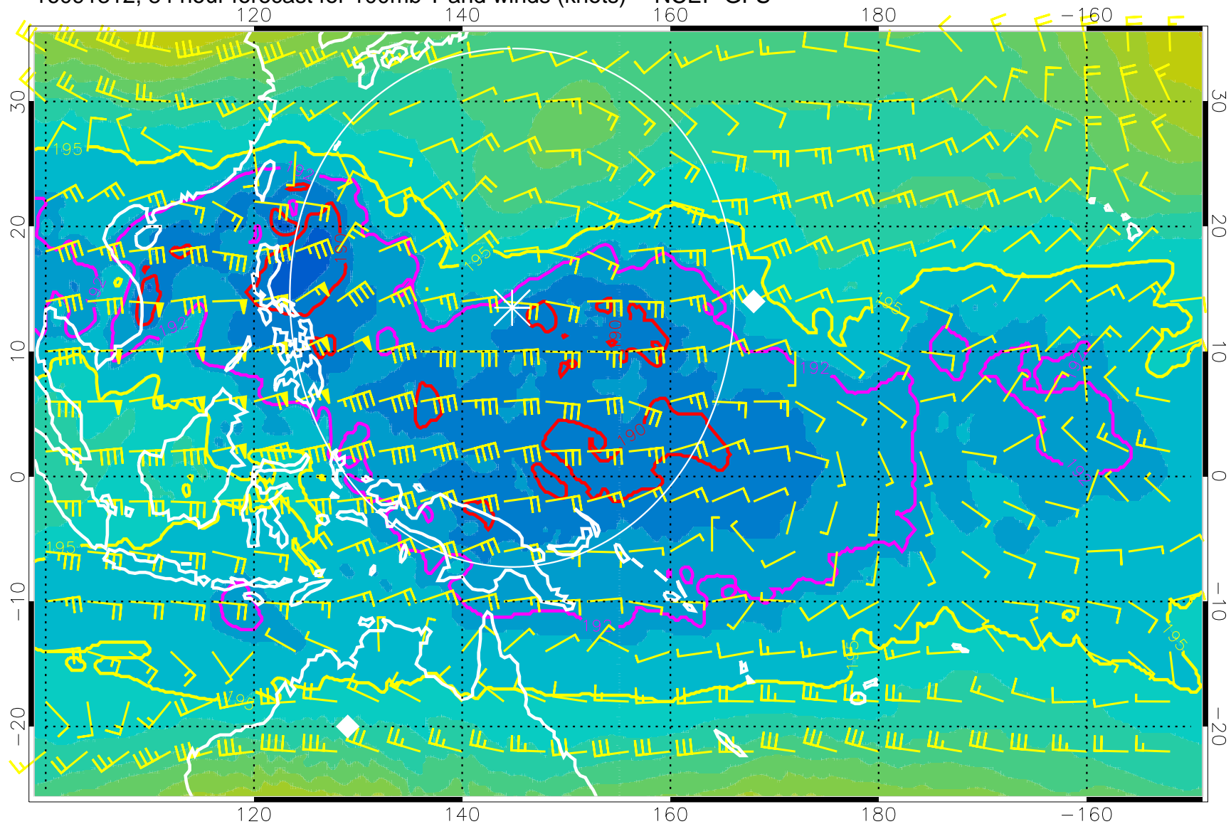
16091312, 84 hour forecast for 100mb T and winds (knots) -- NCEP GFS
