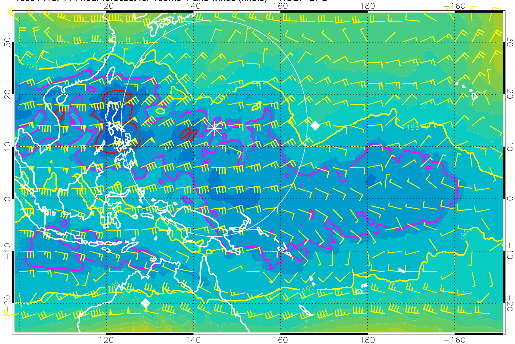
16091418, 114 hour forecast for 100mb T and winds (knots) -- NCEP GFS
